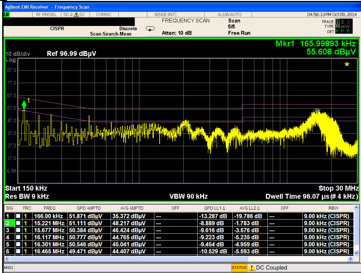
Plot 6-44. Line-Conducted Test Plot (L1)
