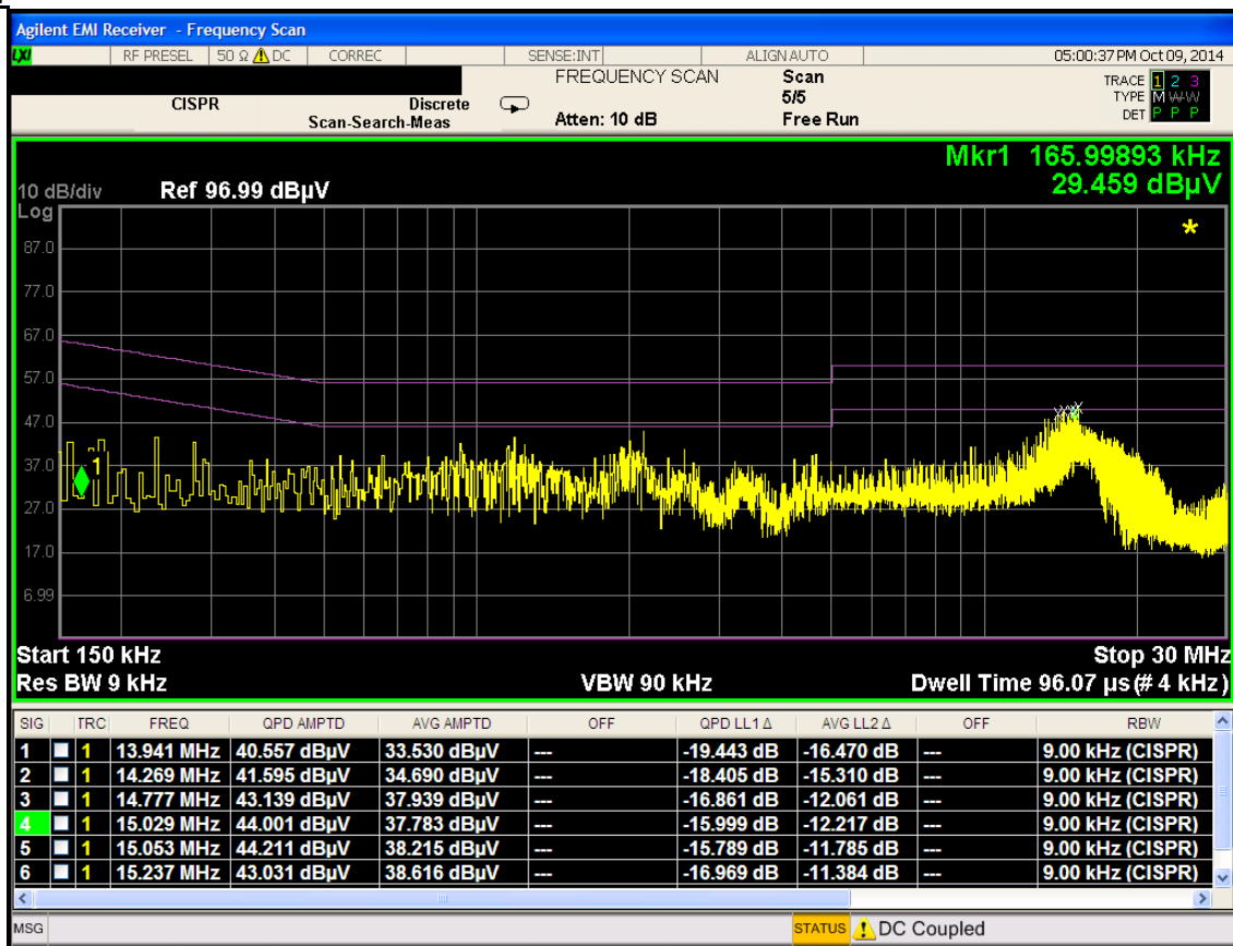
Plot 6-45. Line-Conducted Test Plot (N)
