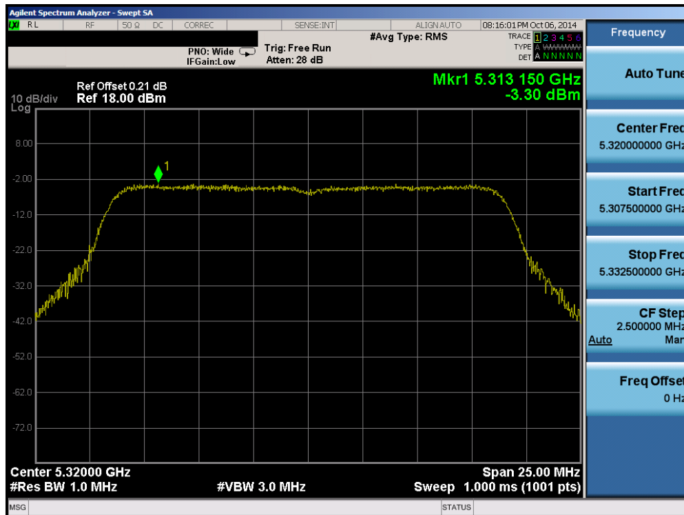
Plot 6-44. Peak Power Spectral Density Plot (20MHz BW 802.11a/n (UNII Band 2A) – Ch. 64)
