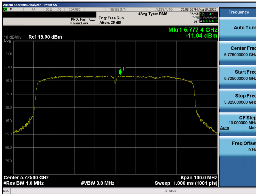
Plot 6-74. Power Spectral Density Plot (80MHz BW 802.11ac (UNII Band 3) – Ch. 155)
