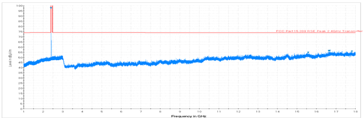
Plot 6-2. Radiated Spurious Plot above 1GHz (BT – Ch. 0, Ant. Pol. V)
