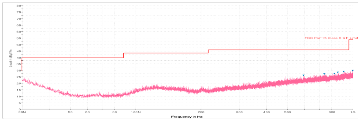
Plot 6-12. Radiated Spurious Plot below 1GHz (Pol. V)
