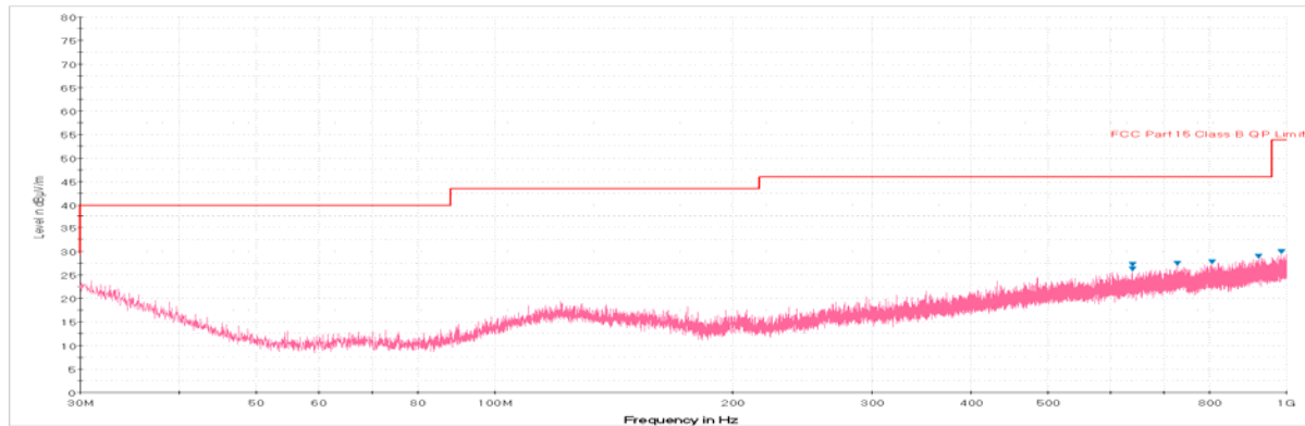
Plot 6-11. Radiated Spurious Plot below 1GHz (Pol. H)
