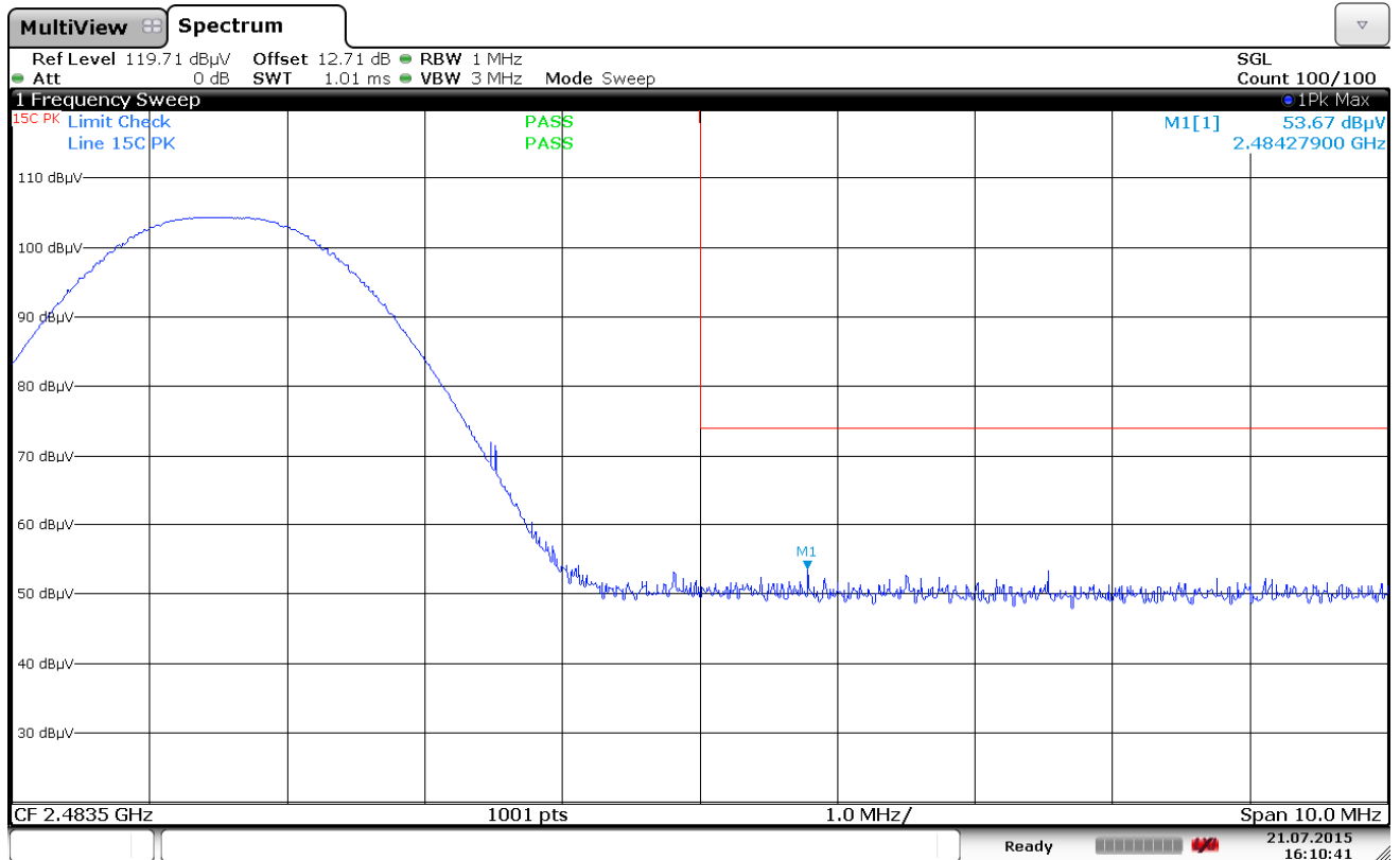
Plot 6-10. Radiated Restricted Upper Band Edge Measurement (Peak)
