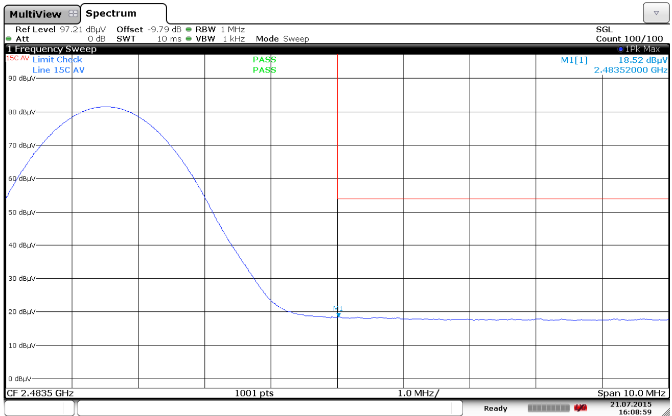
Plot 6-9. Radiated Restricted Upper Band Edge Measurement (Average)
