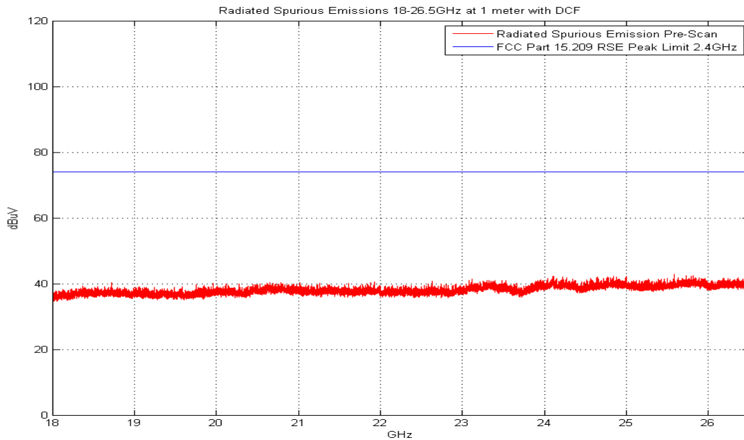
Plot 6-8. Radiated Spurious Plot above 18GHz (Pol. V)
