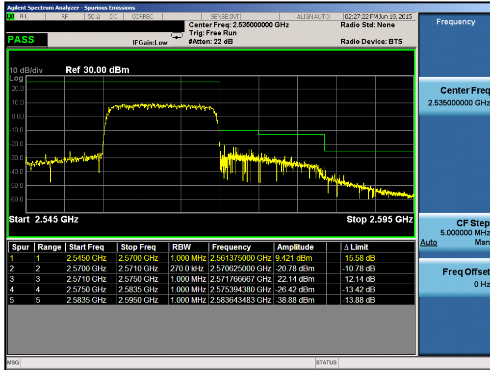
Plot 6-171. Upper ACP Plot (Band 7 – 15.0MHz QPSK – RB Size 75)
