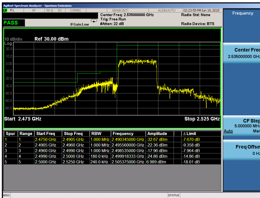
Plot 6-168. Lower ACP Plot (Band 7 – 10.0MHz QPSK – RB Size 50)
