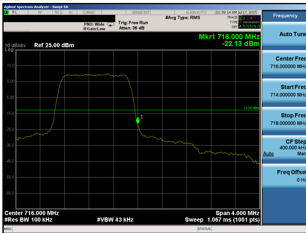
Plot 6-95. Upper Band Edge Plot (Band 12 – 1.4MHz QPSK – RB Size 6)
