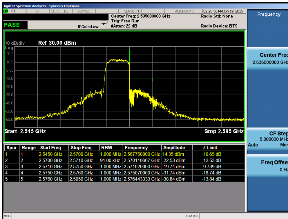
Plot 6-167. Upper ACP Plot (Band 7 – 5.0MHz QPSK – RB Size 25)
