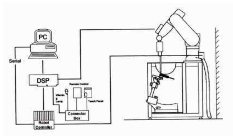
Figure 2. HCT SAR Lab. Test Measurement Set-up
