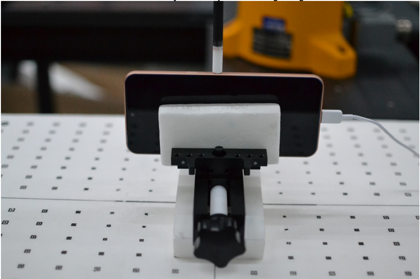
Near-Field Power Density Test Setup Photo 5 – Right Edge at 2 mm
