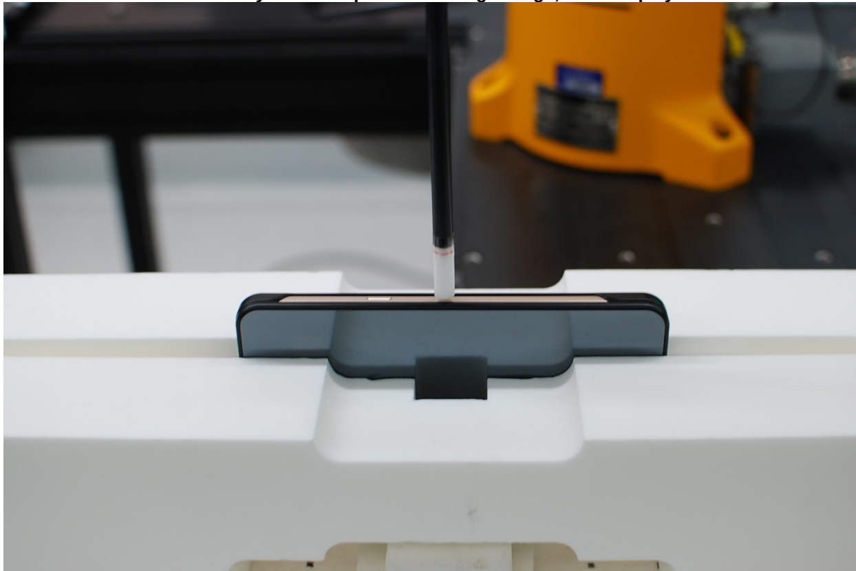
Near-Field Power Density Test Setup Photo 6 – Right Edge, Dual Display Closed at 2 mm
