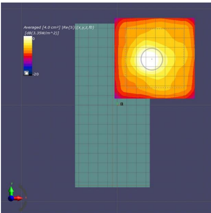
Figure 8-2: 4cm2-averaged power density distribution measured at input.power.limit of -0.3 dBm on the back surface for n261 beam 39
