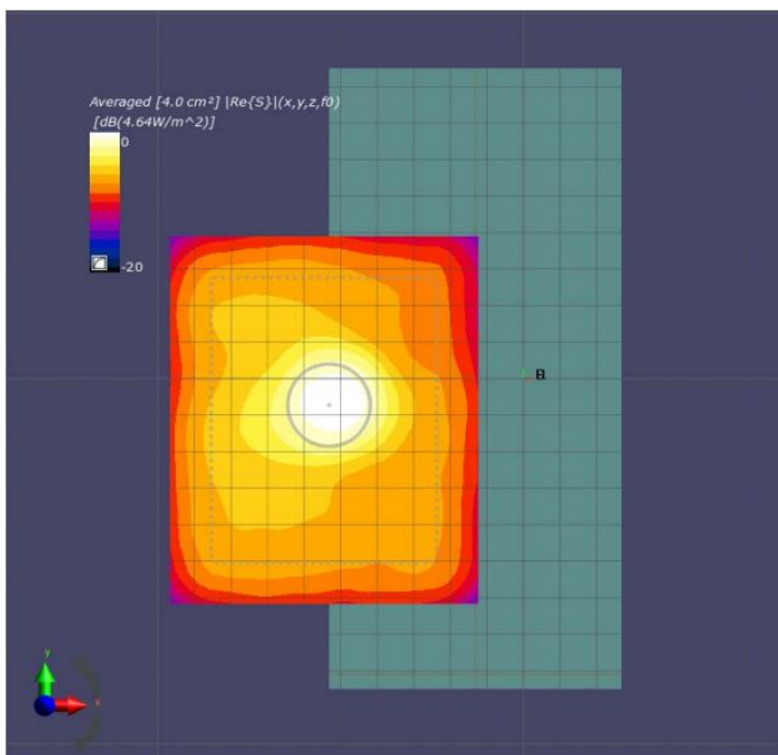
Figure 8-2: 4cm2-averaged power density distribution measured at input.power.limit of -0.3 dBm on the back surface for n261 beam 39
