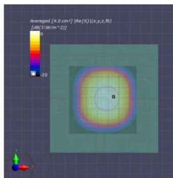
30GHz System Verification
