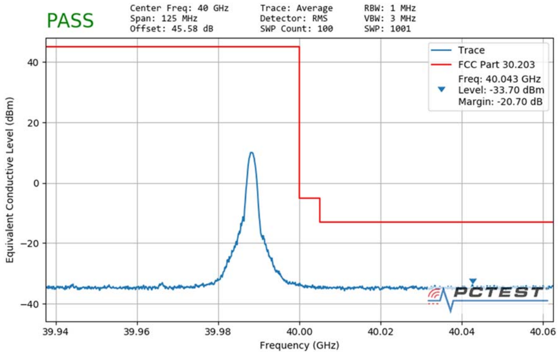
Plot 7-186. Ant3 Upper Band Edge (50MHz-1CC – QPSK 1 RB)
