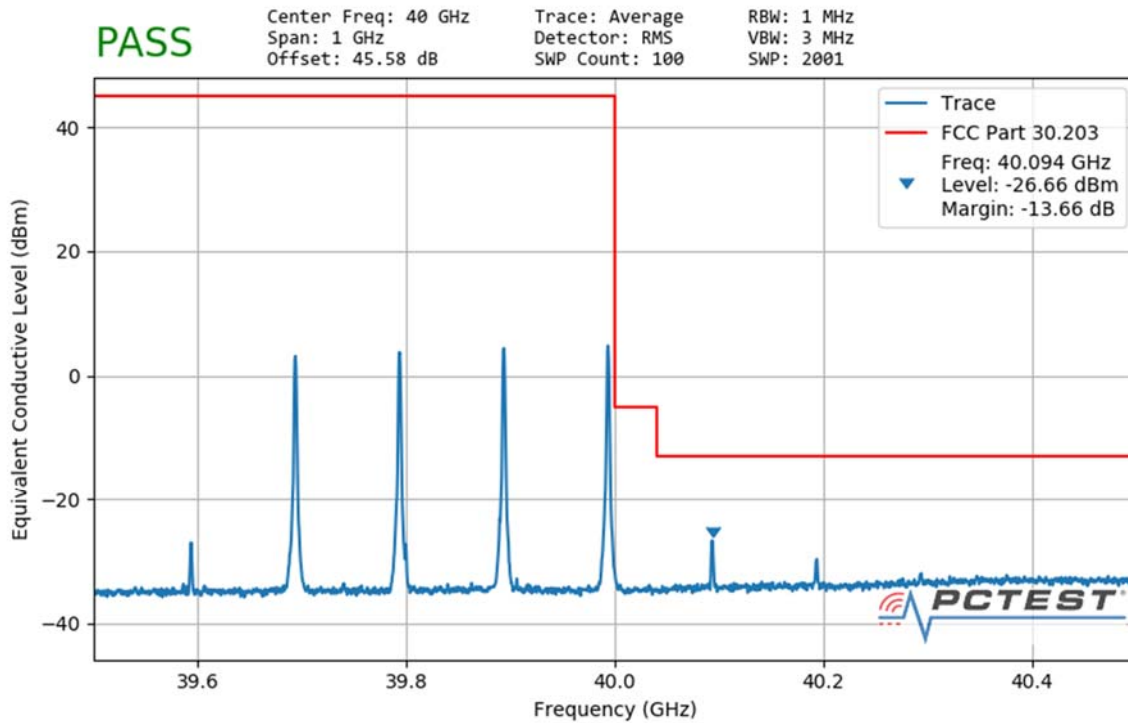
Plot 7-182. Ant2 Upper Band Edge (100MHz-4CC – QPSK 1 RB)
