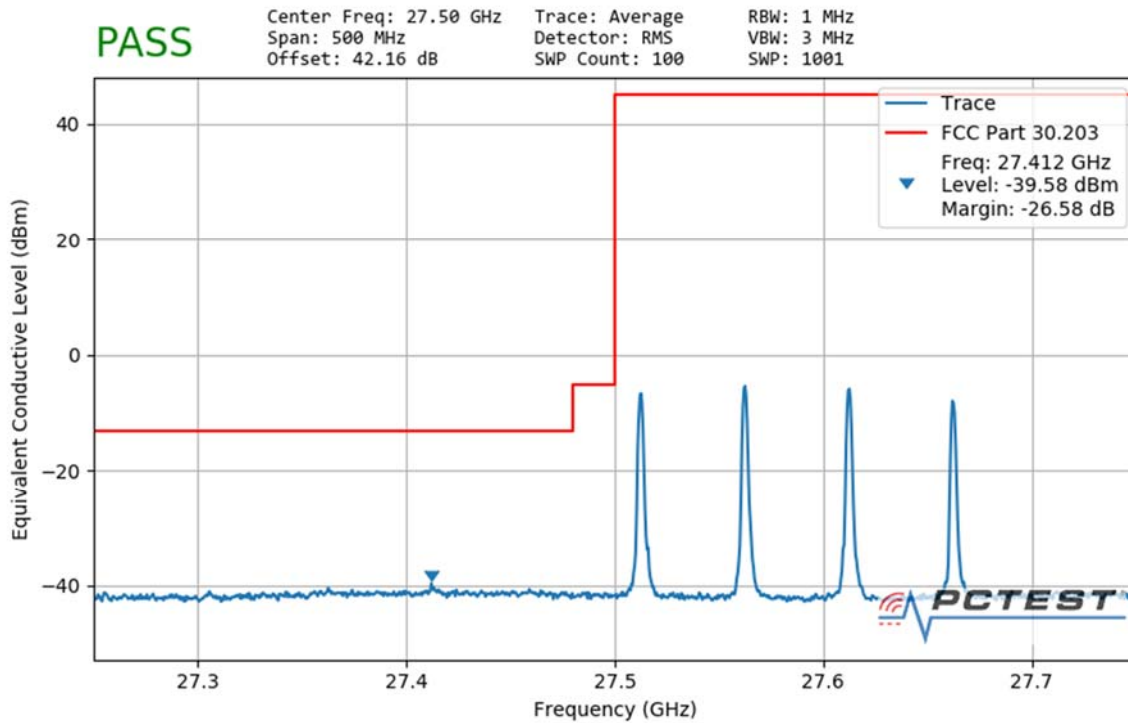
Plot 7-188. Ant3 Lower Band Edge (50MHz-4CC – QPSK 1 RB)
