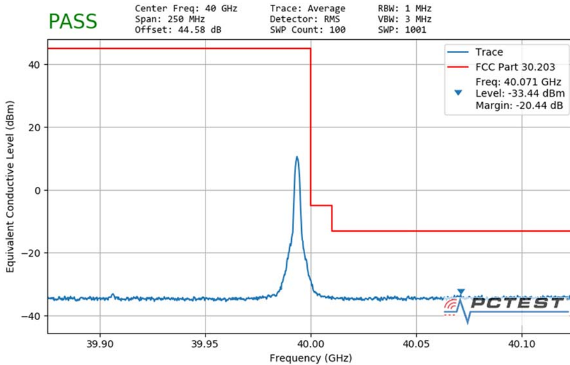
Plot 7-194. Ant3 Upper Band Edge (100MHz-1CC – QPSK 1 RB)
