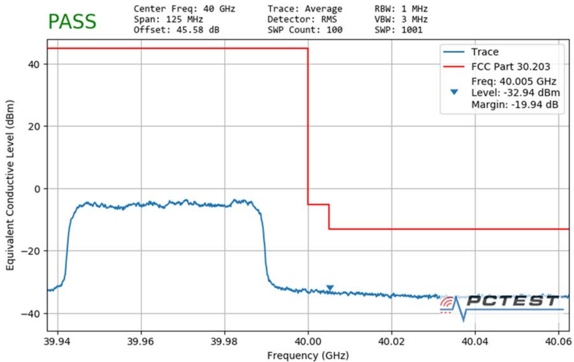
Plot 7-185. Ant3 Upper Band Edge (50MHz-1CC – QPSK Full RB)
