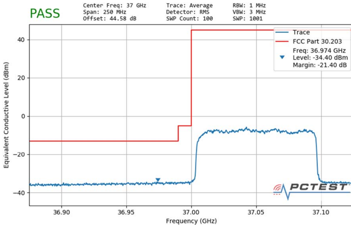
Plot 7-191. Ant3 Lower Band Edge (100MHz-1CC – QPSK Full RB)
