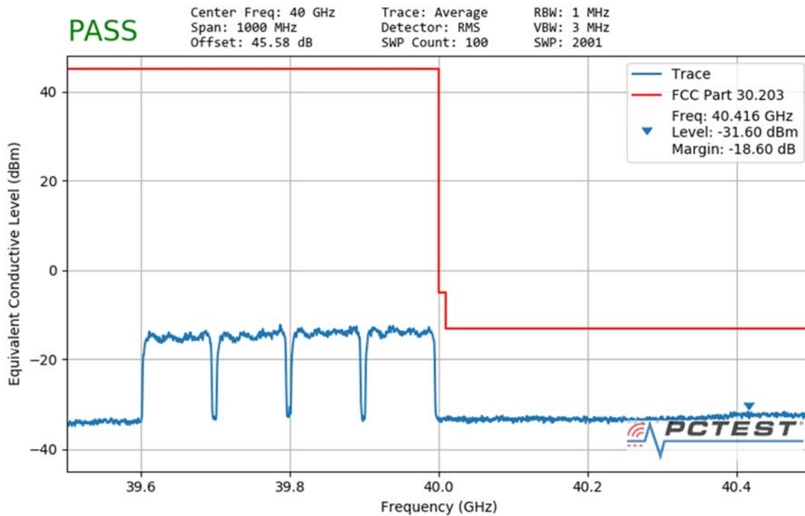
Plot 7-197. Ant3 Upper Band Edge (100MHz-4CC – QPSK Full RB)
