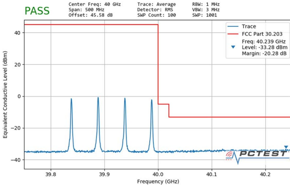
Plot 7-190. Ant3 Upper Band Edge (50MHz-4CC – QPSK 1 RB)
