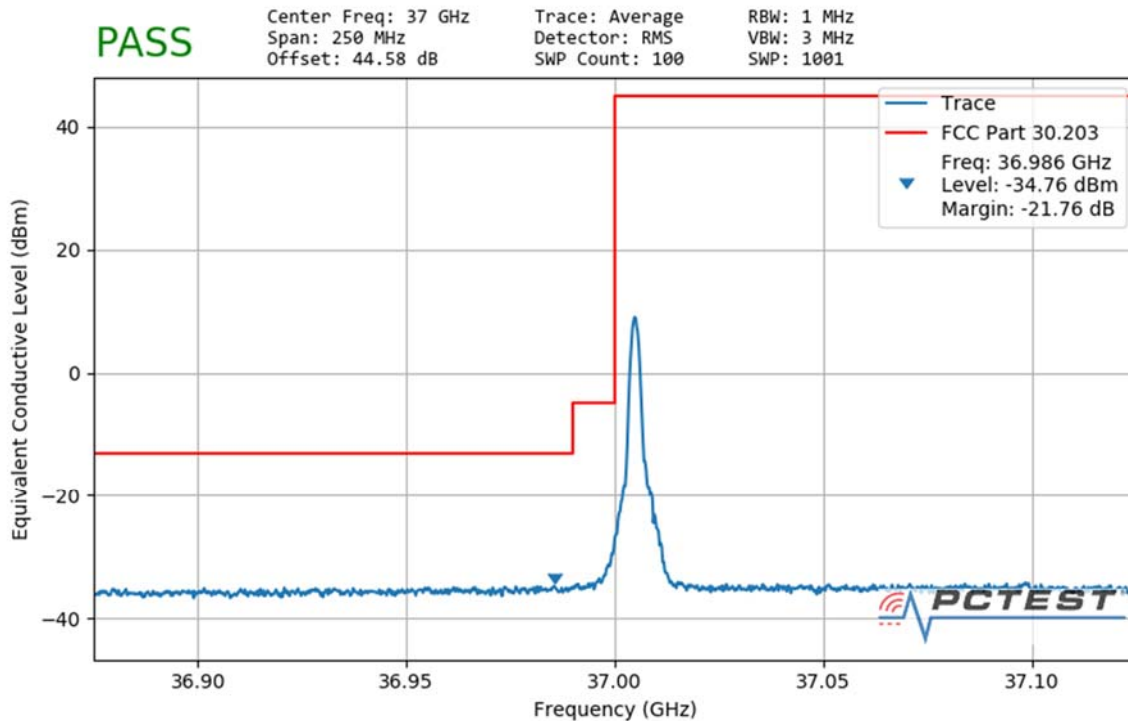
Plot 7-192. Ant3 Lower Band Edge (100MHz-1CC – QPSK 1 RB)
