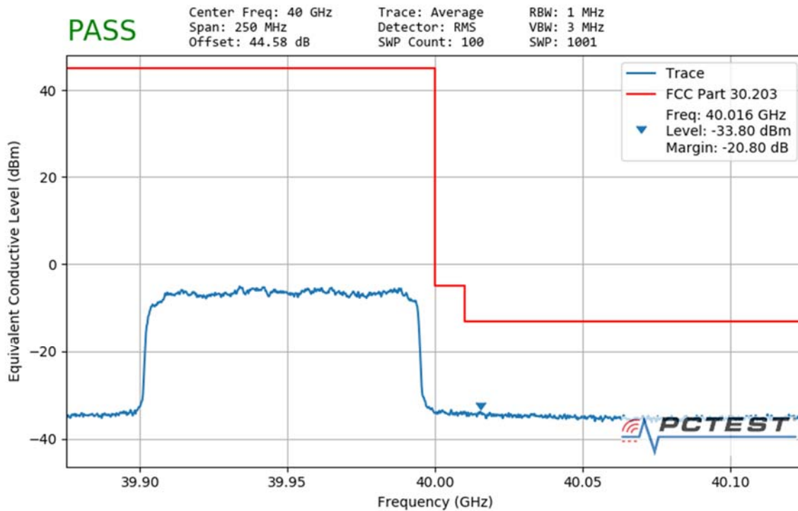
Plot 7-193. Ant3 Upper Band Edge (100MHz-1CC – QPSK Full RB)
