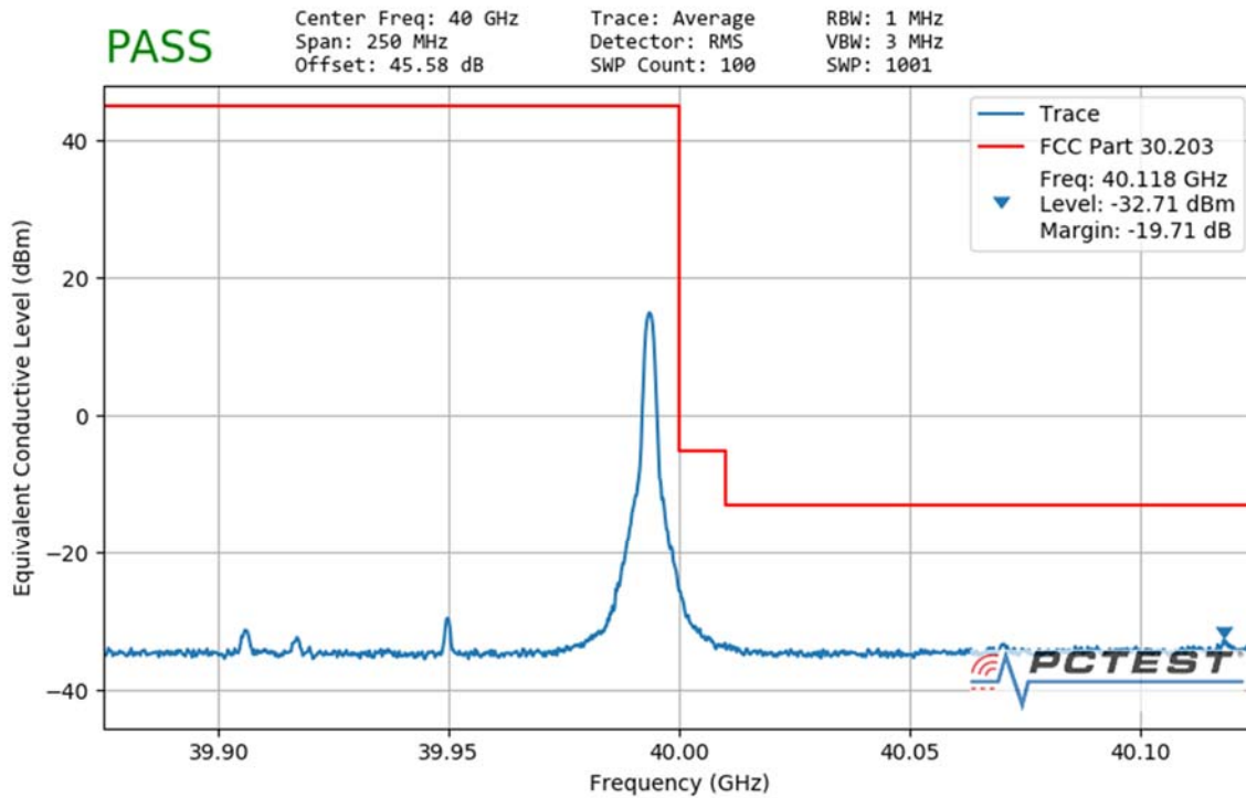
Plot 7-178. Ant2 Upper Band Edge (100MHz-1CC – QPSK 1 RB)
