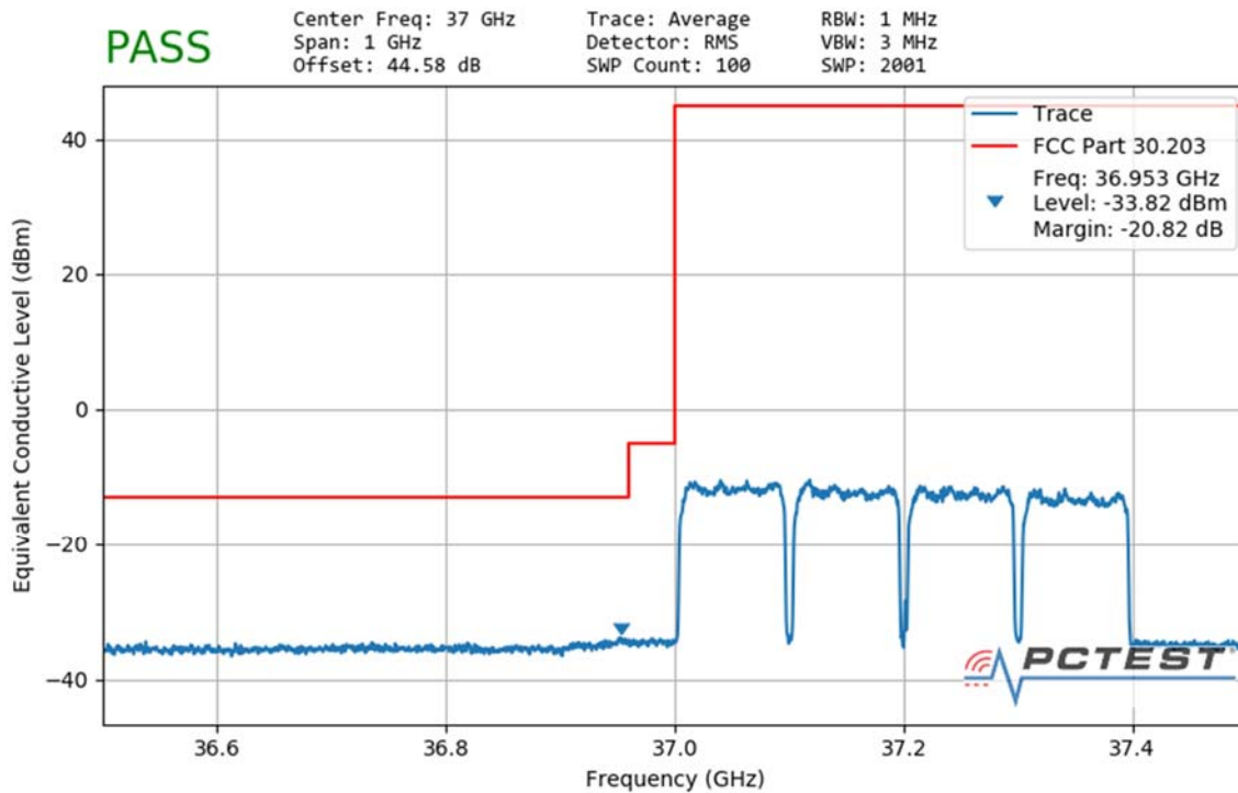
Plot 7-179. Ant2 Lower Band Edge (100MHz-4CC – QPSK Full RB)
