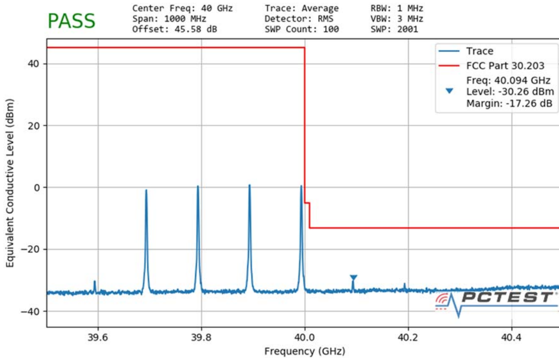
Plot 7-198. Ant3 Upper Band Edge (100MHz-4CC – QPSK 1 RB)
