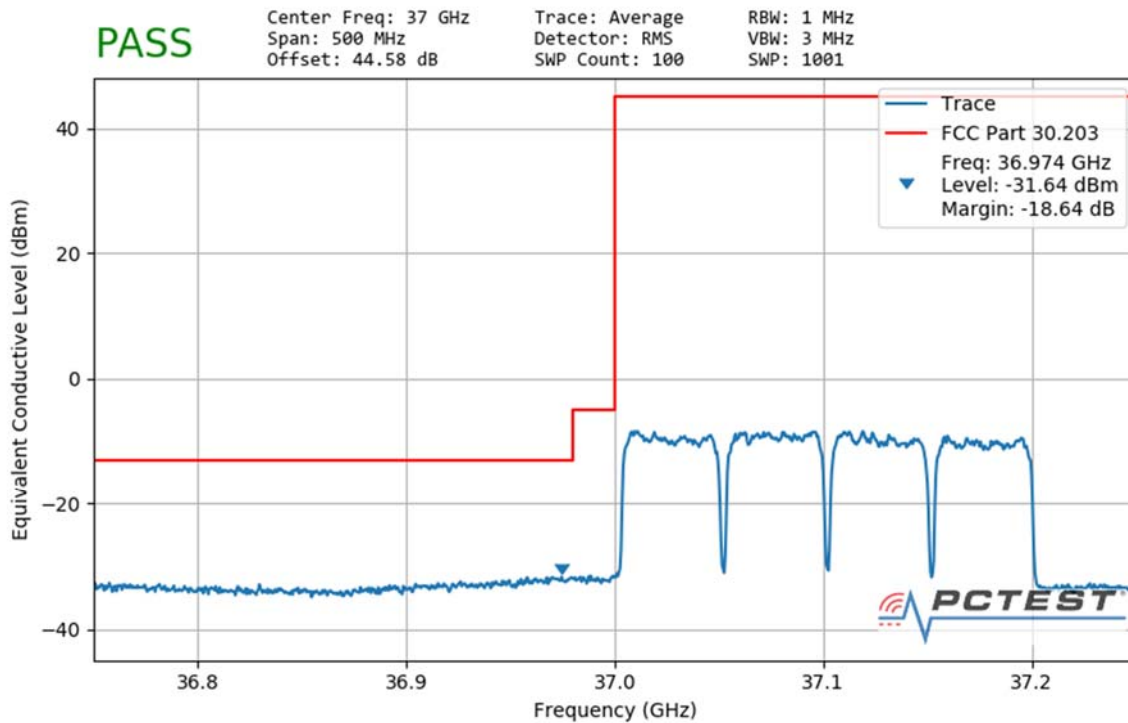
Plot 7-187. Ant3 Lower Band Edge (50MHz-4CC – QPSK Full RB)
