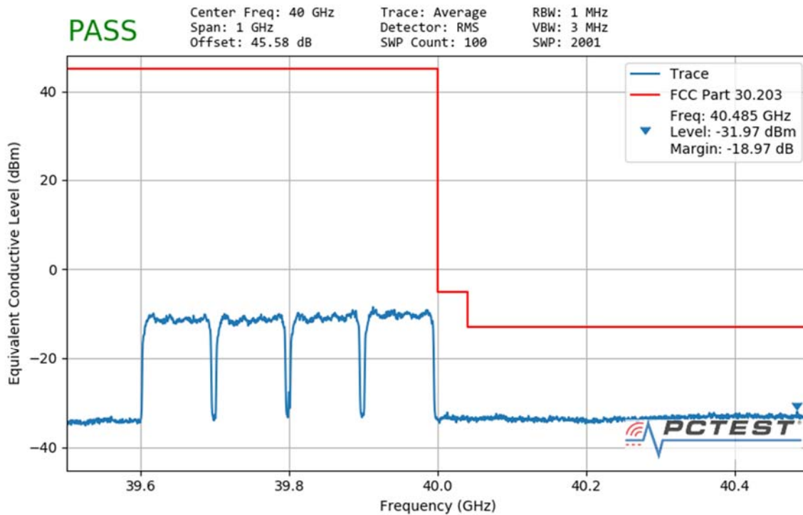
Plot 7-181. Ant2 Upper Band Edge (100MHz-4CC – QPSK Full RB)
