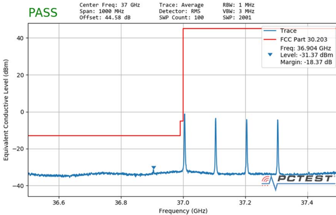
Plot 7-196. Ant3 Lower Band Edge (100MHz-4CC – QPSK 1 RB)
