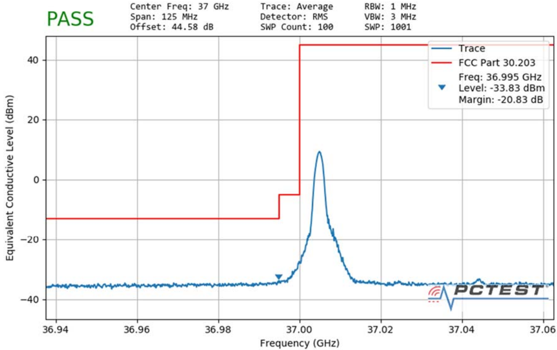
Plot 7-184. Ant3 Lower Band Edge (50MHz-1CC – QPSK 1 RB)
