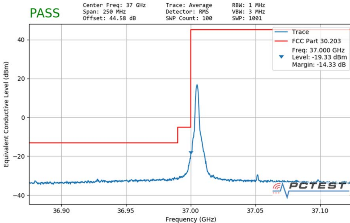
Plot 7-176. Ant2 Lower Band Edge (100MHz-1CC – QPSK 1 RB)
