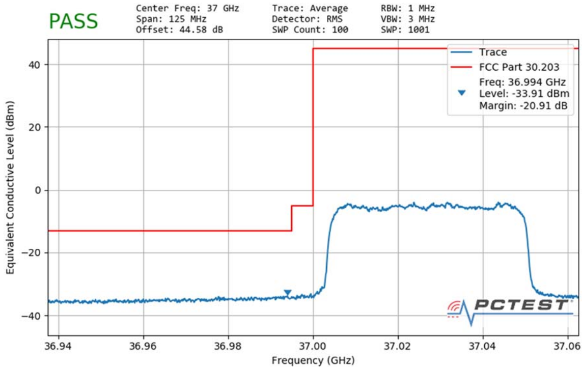
Plot 7-183. Ant3 Lower Band Edge (50MHz-1CC – QPSK Full RB)
