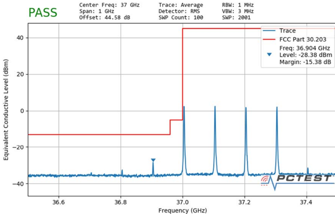
Plot 7-180. Ant2 Lower Band Edge (100MHz-4CC – QPSK 1 RB)
