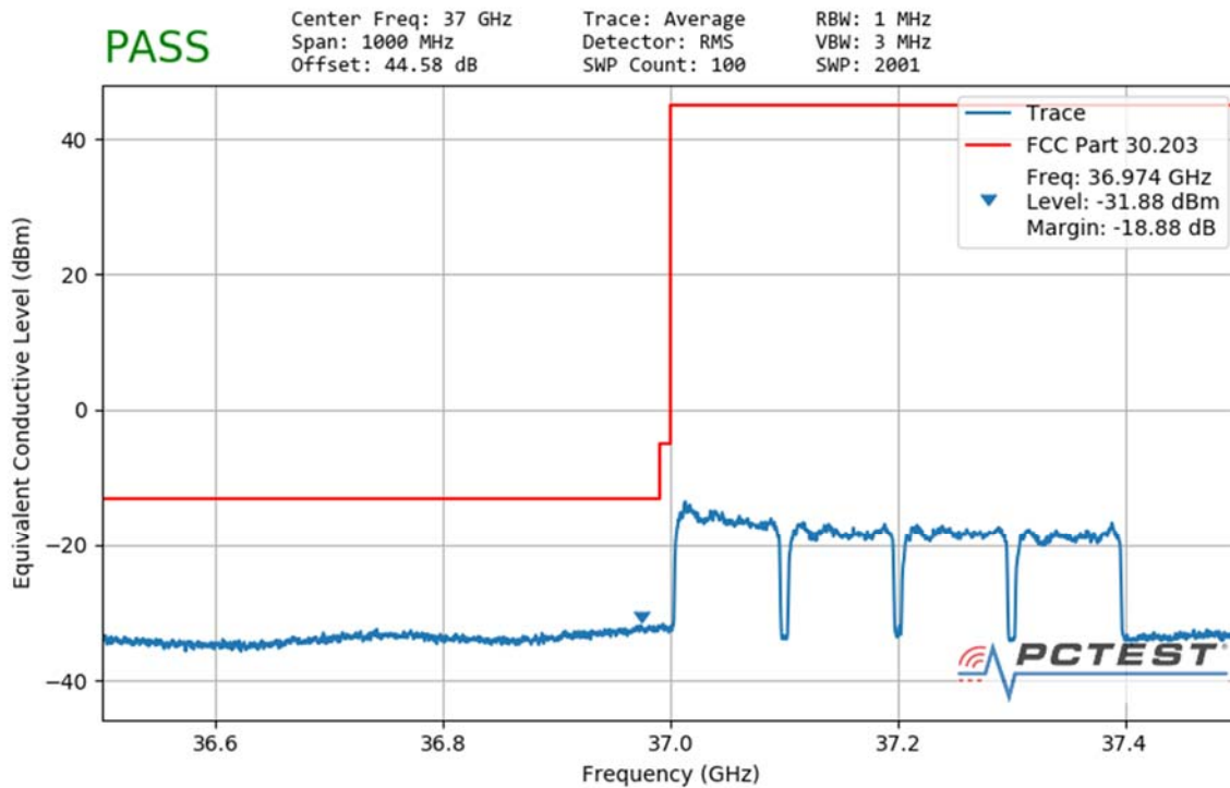
Plot 7-195. Ant3 Lower Band Edge (100MHz-4CC – QPSK Full RB)
