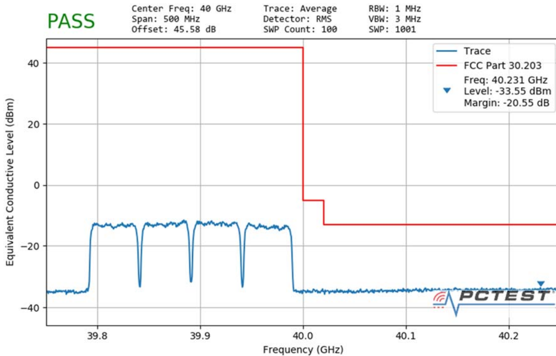
Plot 7-189. Ant3 Upper Band Edge (50MHz-4CC – QPSK Full RB)
