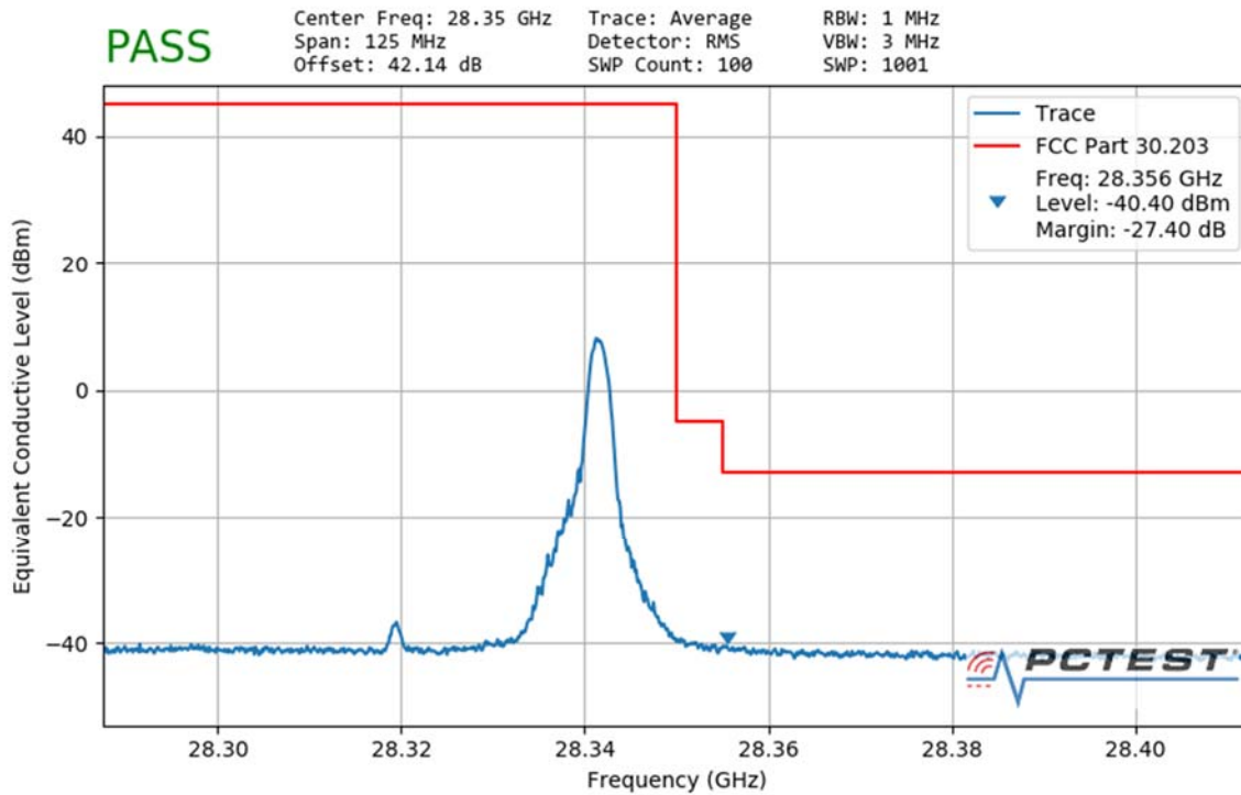
Plot 7-138. Ant3 Upper Band Edge (50MHz-1CC – QPSK 1 RB)
