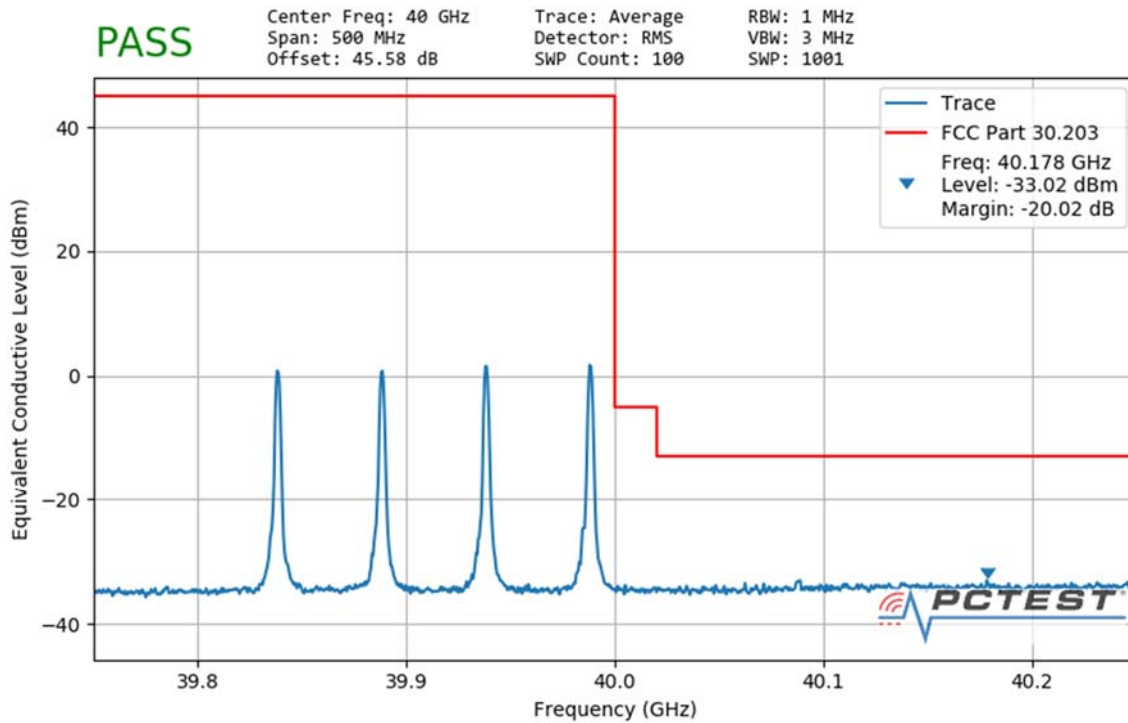
Plot 7-158. Ant1 Upper Band Edge (50MHz-4CC – QPSK 1 RB)
