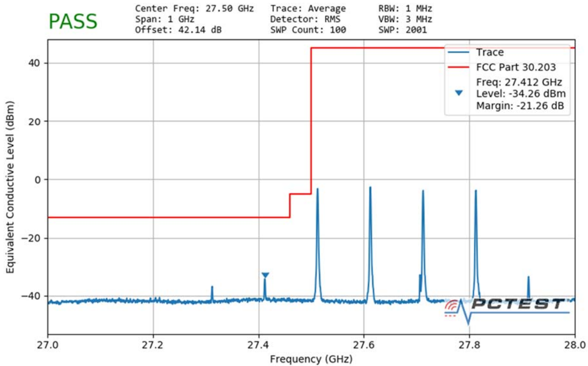
Plot 7-132. Ant2 Lower Band Edge (100MHz-4CC – QPSK 1 RB)
