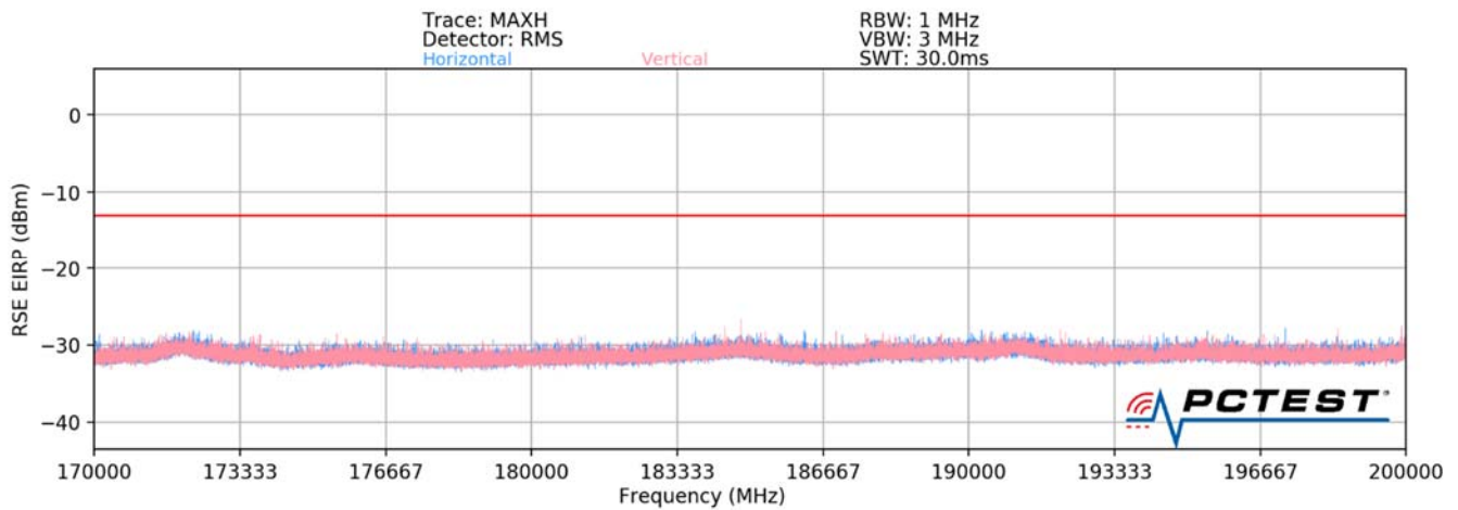
Plot 7-88. Ant2-n260 Radiated Spurious Plot (1CC QPSK Mid Channel V Beam)
