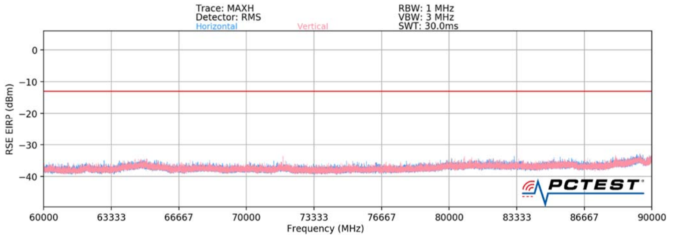
Plot 7-81. Ant2-n260 Radiated Spurious Plot (1CC QPSK Mid Channel H Beam)
