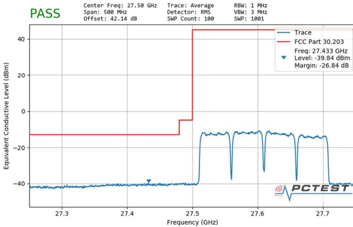
Plot 7-123. Ant2 Lower Band Edge (50MHz-4CC – QPSK Full RB)
