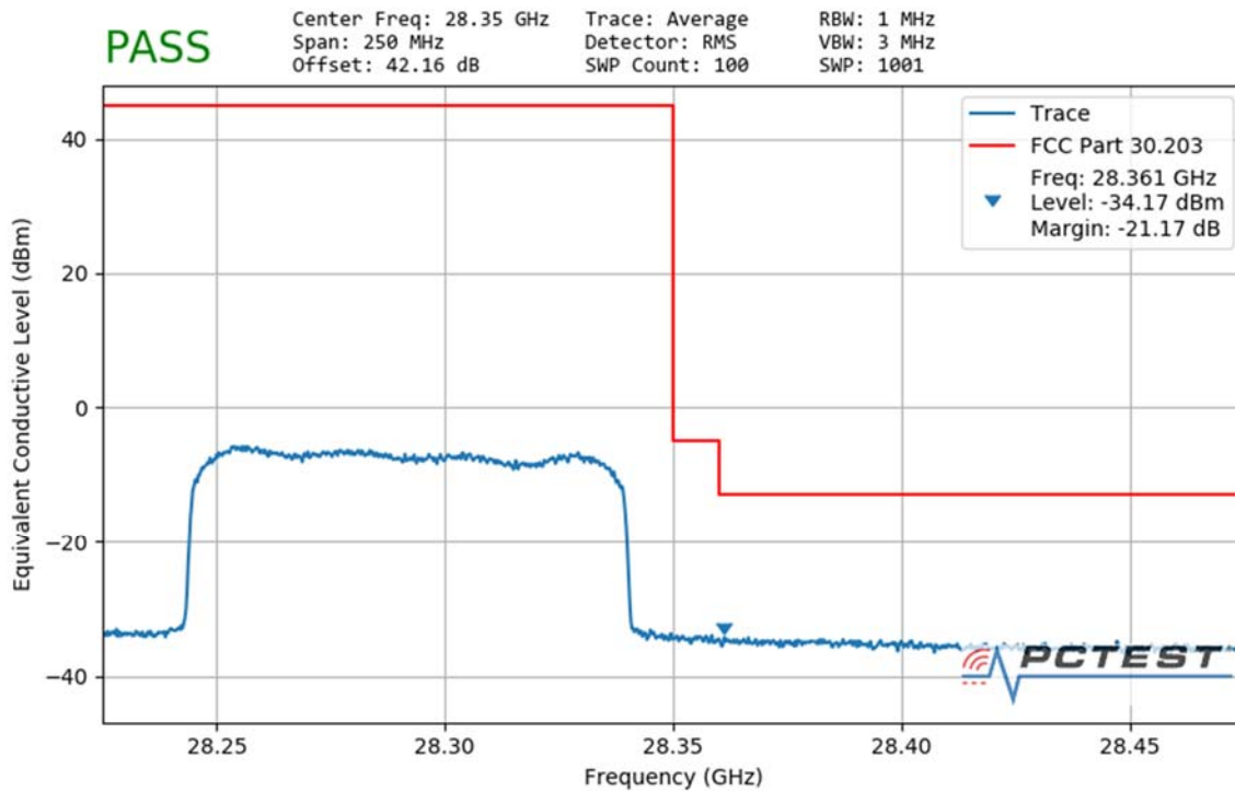
Plot 7-113. Ant1 Upper Band Edge (100MHz-1CC – QPSK Full RB)
