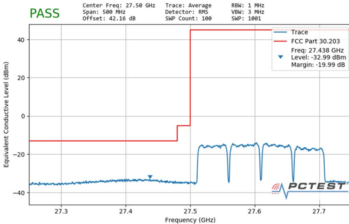
Plot 7-107. Ant1 Lower Band Edge (50MHz-4CC – QPSK Full RB)
