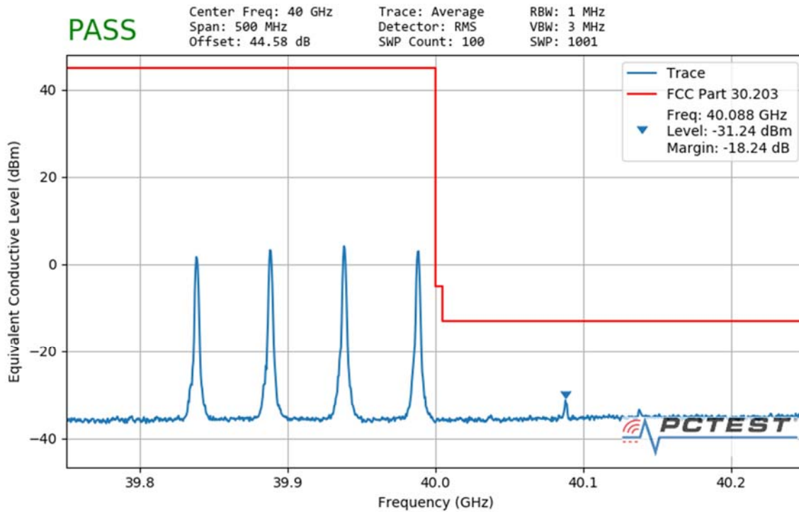
Plot 7-174. Ant2 Upper Band Edge (50MHz-4CC – QPSK 1 RB)
