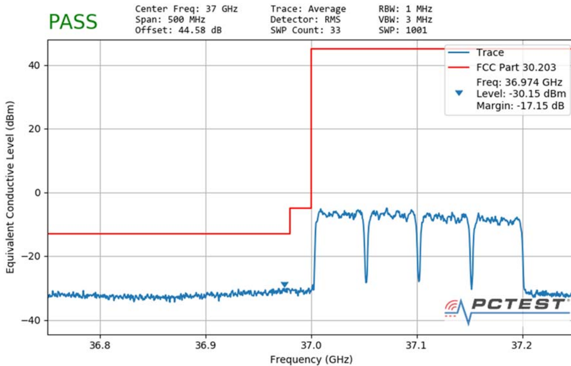
Plot 7-155. Ant1 Lower Band Edge (50MHz-4CC – QPSK Full RB)
