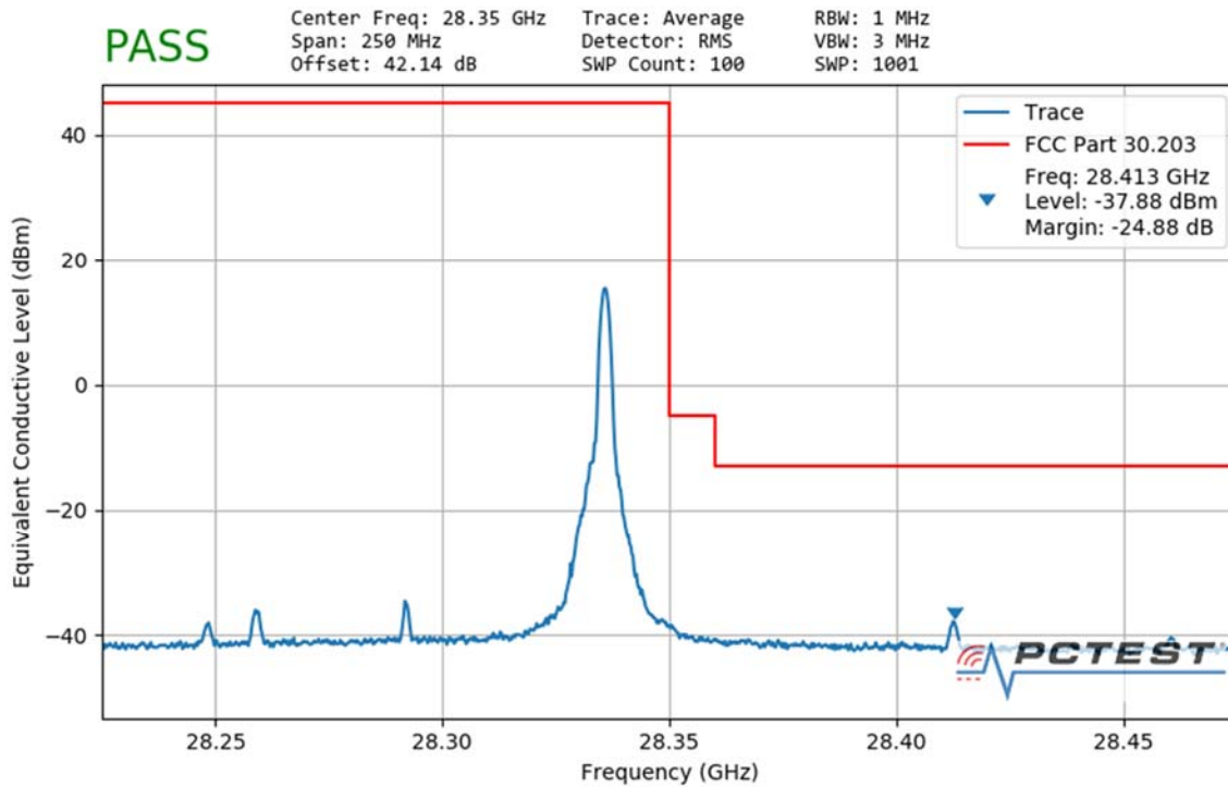
Plot 7-130. Ant2 Upper Band Edge (100MHz-1CC – QPSK 1 RB)
