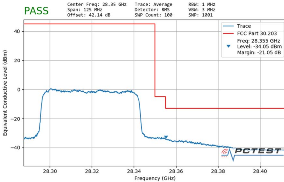
Plot 7-121. Ant2 Upper Band Edge (50MHz-1CC – QPSK Full RB)
