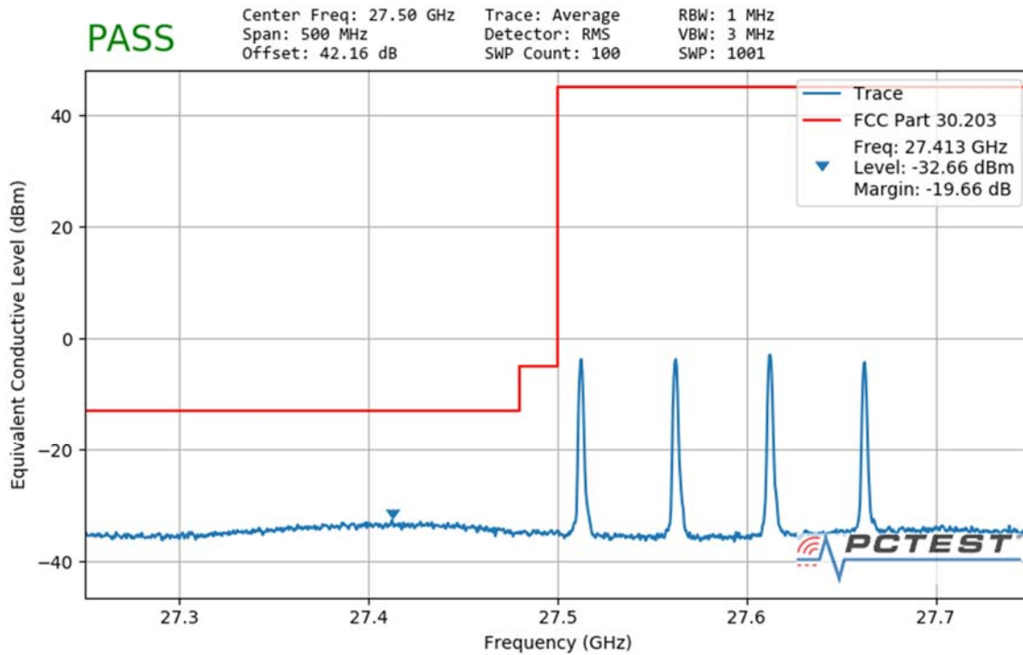
Plot 7-108. Ant1 Lower Band Edge (50MHz-4CC – QPSK 1 RB)
