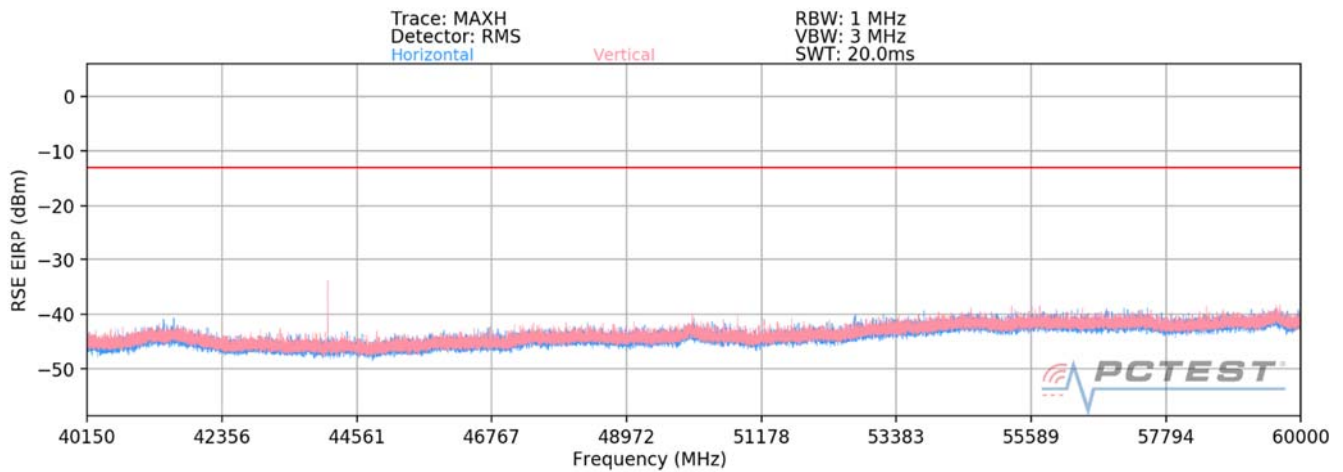
Plot 7-79. Ant2-n260 Radiated Spurious Plot (1CC QPSK Mid Channel H Beam)
