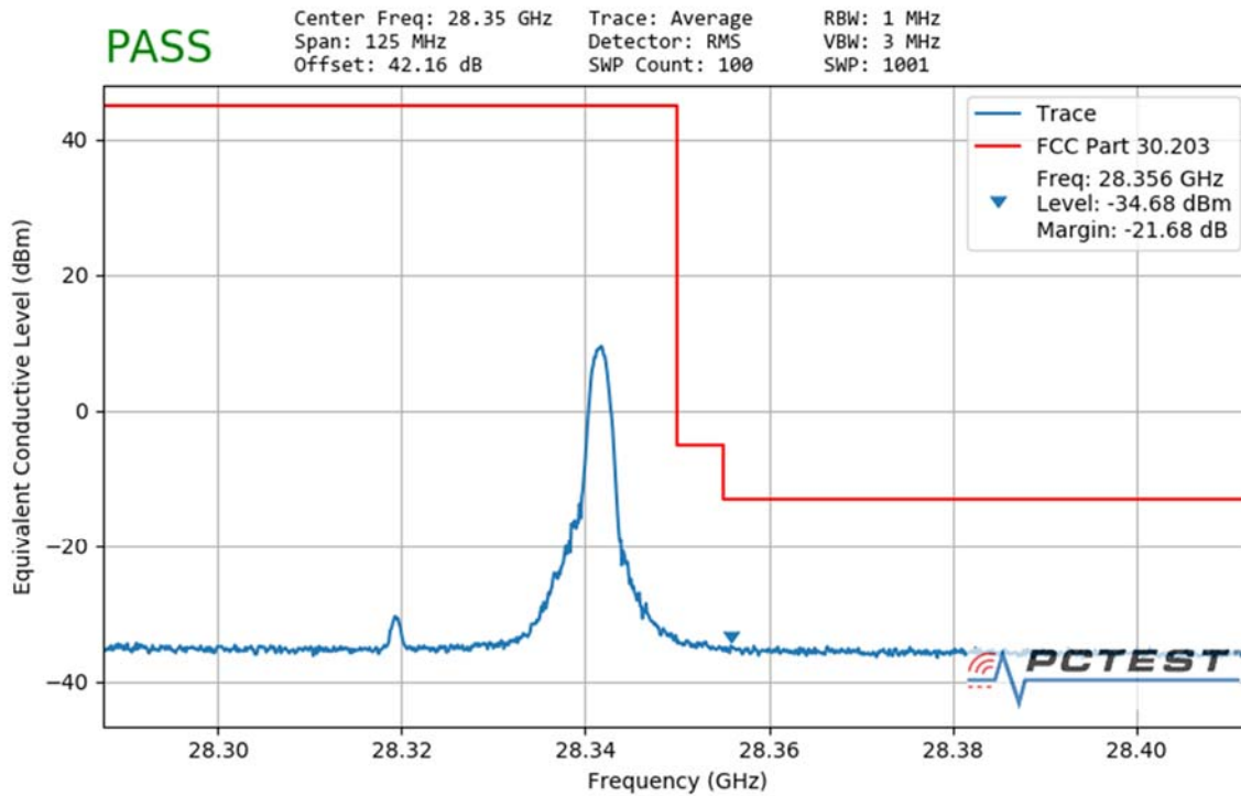
Plot 7-106. Ant1 Upper Band Edge (50MHz-1CC – QPSK 1 RB)
