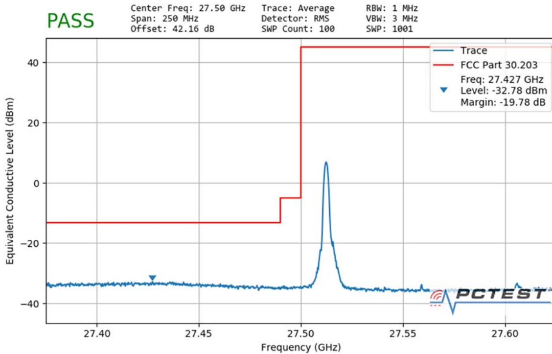
Plot 7-112. Ant1 Lower Band Edge (100MHz-1CC – QPSK 1 RB)
