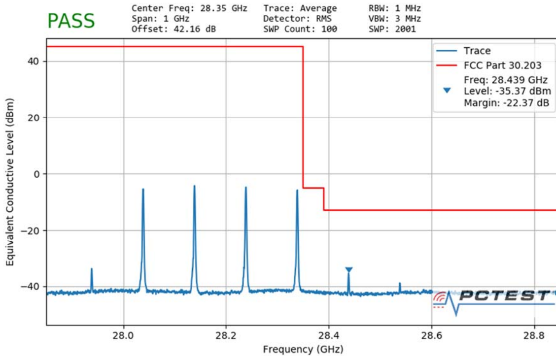
Plot 7-150. Ant3 Upper Band Edge (100MHz-4CC – QPSK 1 RB)
