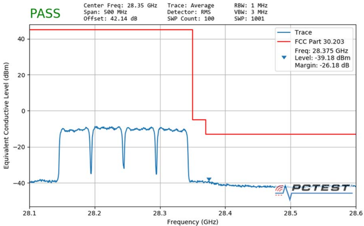
Plot 7-125. Ant2 Upper Band Edge (50MHz-4CC – QPSK Full RB)
