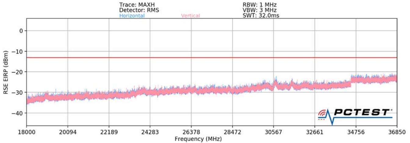
Plot 7-91. Ant3-n260 Radiated Spurious Plot (1CC QPSK Mid Channel H Beam)
