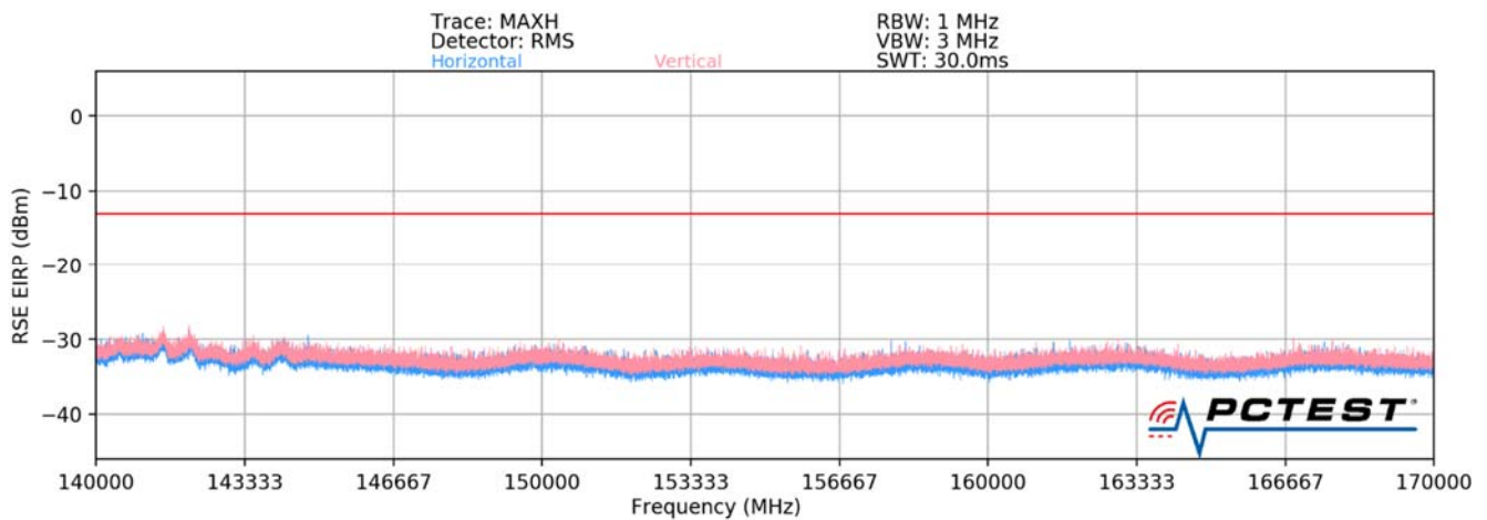
Plot 7-86. Ant2-n260 Radiated Spurious Plot (1CC QPSK Mid Channel V Beam)
