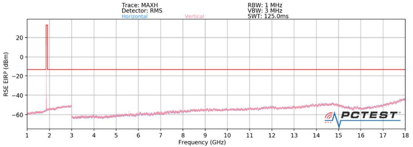
Plot 7-76. Ant2-n260 Radiated Spurious Plot 1GHz - 18GHz (1CC QPSK Mid Channel)
