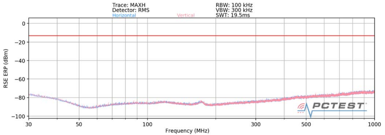
Plot 7-89. Ant3-n260 Radiated Spurious Plot (1CC QPSK Mid Channel)
