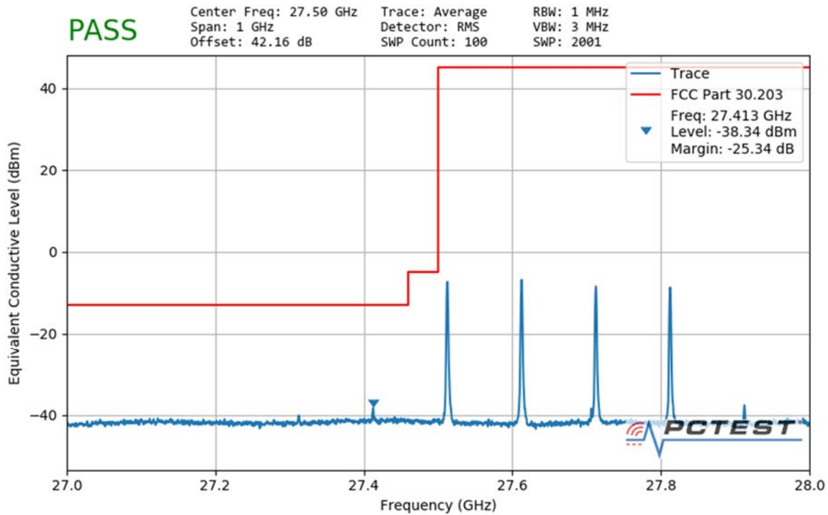
Plot 7-148. Ant3 Lower Band Edge (100MHz-4CC – QPSK 1 RB)
