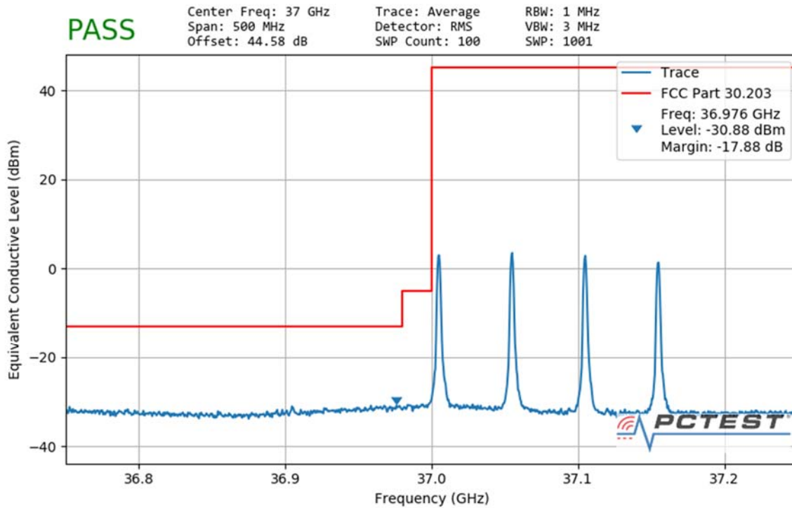
Plot 7-156. Ant1 Lower Band Edge (50MHz-4CC – QPSK 1 RB)
