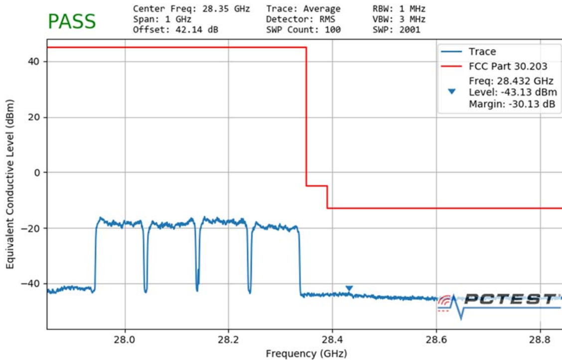
Plot 7-133. Ant2 Upper Band Edge (100MHz-4CC – QPSK Full RB)
