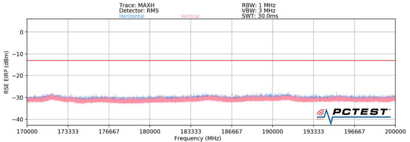
Plot 7-101. Ant3-n260 Radiated Spurious Plot (1CC QPSK Mid Channel H Beam)
