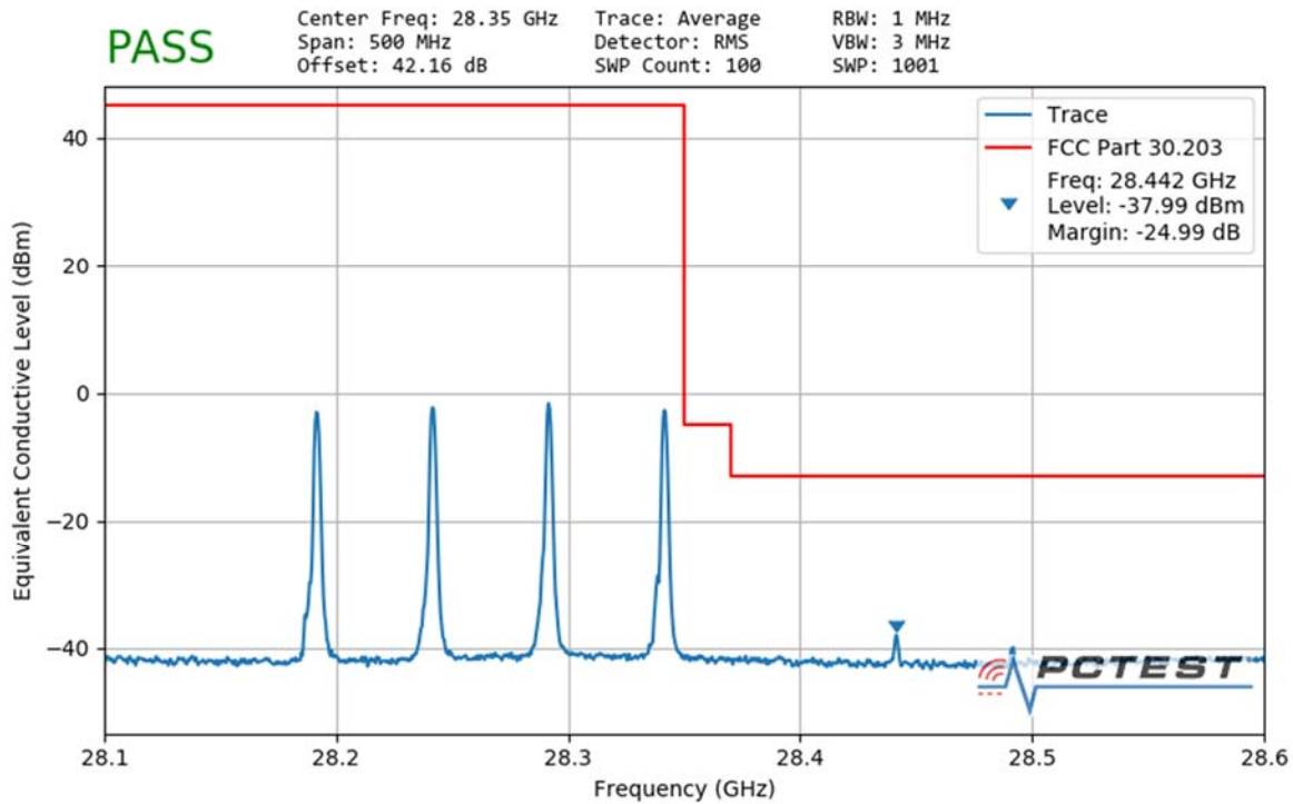
Plot 7-142. Ant3 Upper Band Edge (50MHz-4CC – QPSK 1 RB)
