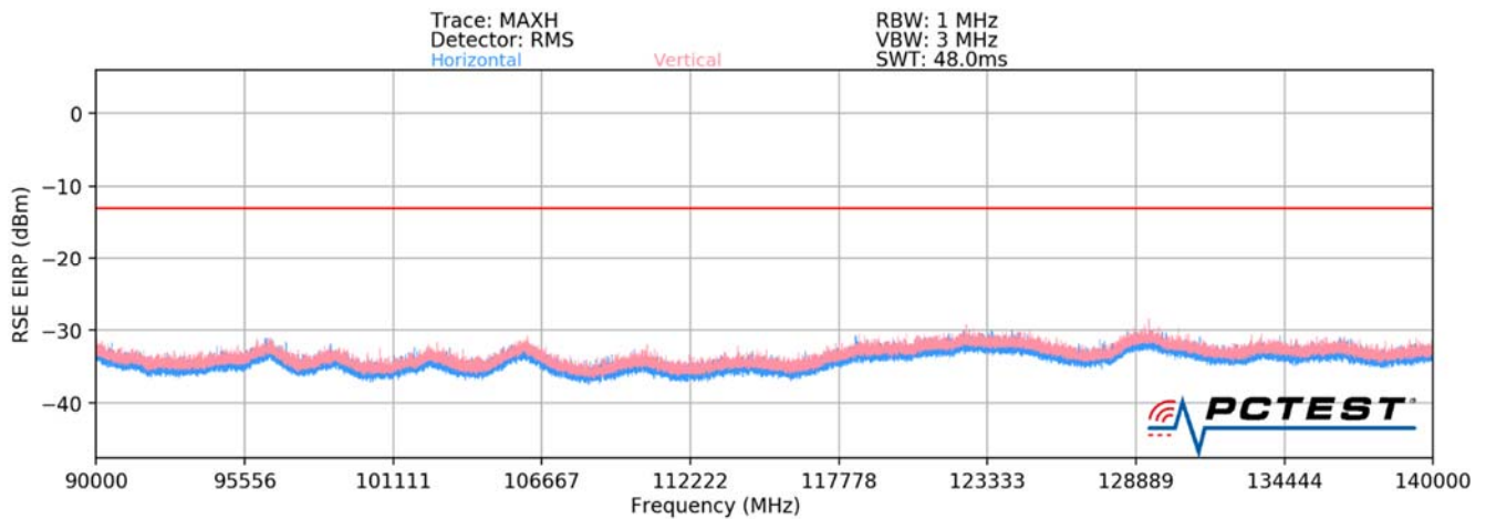
Plot 7-98. Ant3-n260 Radiated Spurious Plot (1CC QPSK Mid Channel V Beam)
