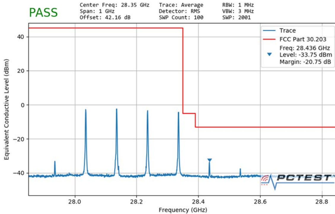
Plot 7-118. Ant1 Upper Band Edge (100MHz-4CC – QPSK 1 RB)
