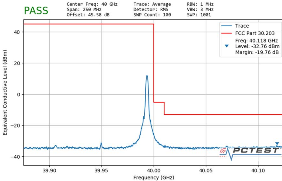
Plot 7-162. Ant1 Upper Band Edge (100MHz-1CC – QPSK 1 RB)
