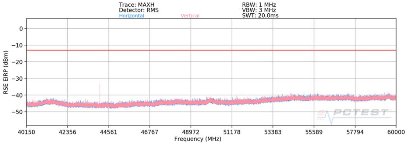
Plot 7-93. Ant3-n260 Radiated Spurious Plot (1CC QPSK Mid Channel H Beam)
