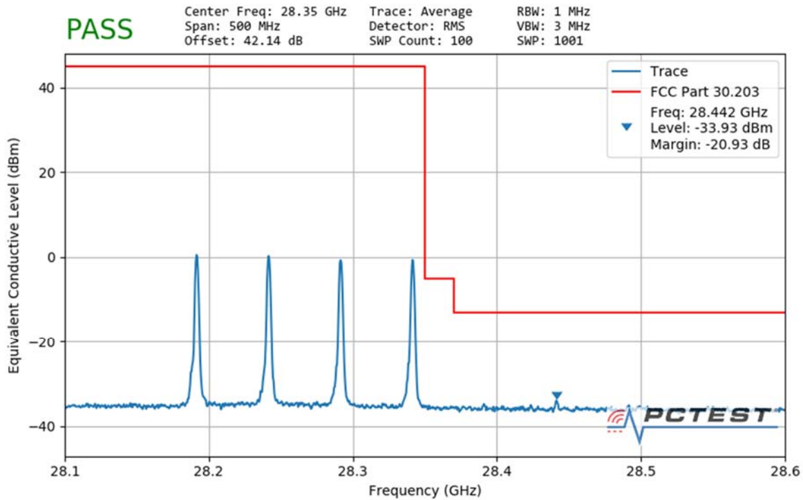
Plot 7-110. Ant1 Upper Band Edge (50MHz-4CC – QPSK 1 RB)
