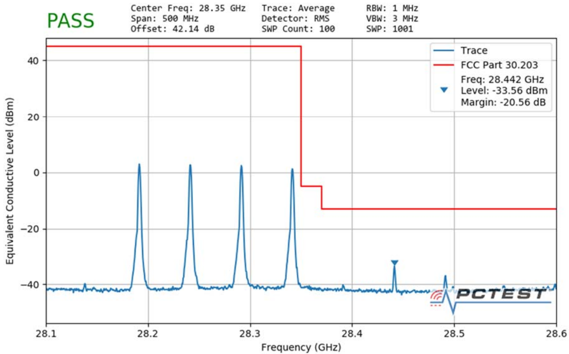
Plot 7-126. Ant2 Upper Band Edge (50MHz-4CC – QPSK 1 RB)
