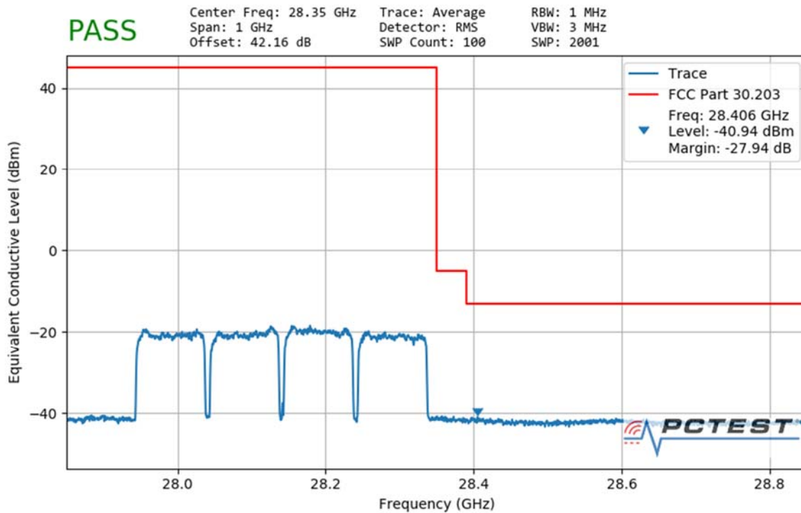
Plot 7-149. Ant3 Upper Band Edge (100MHz-4CC – QPSK Full RB)
