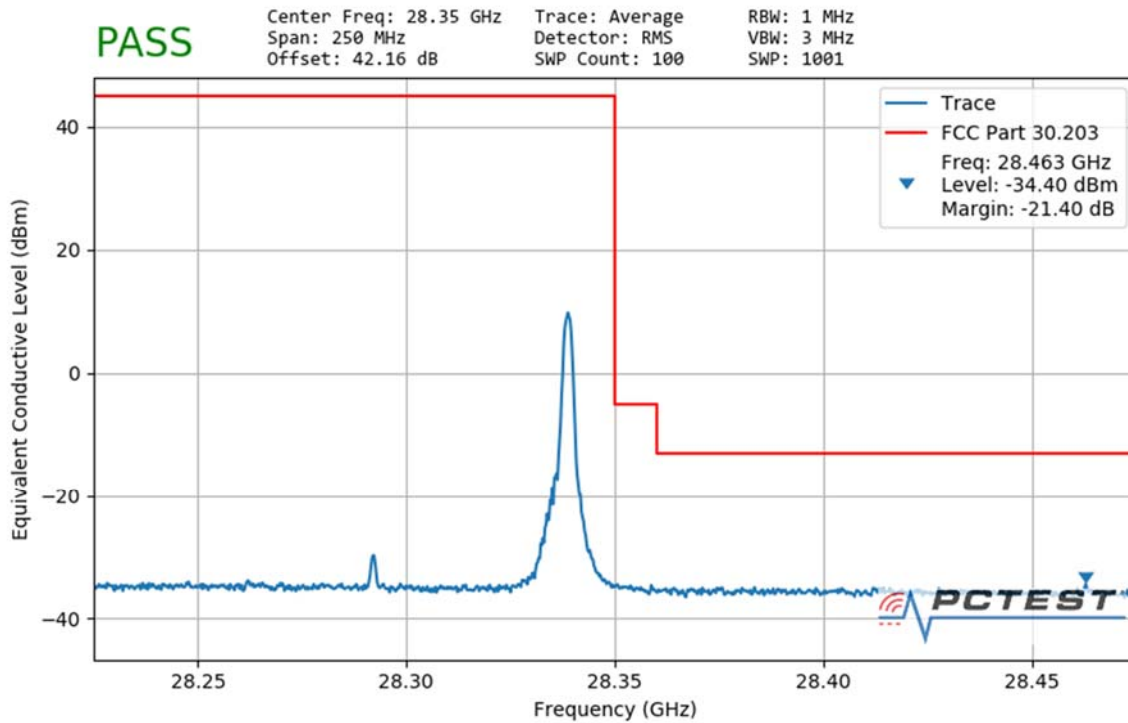
Plot 7-114. Ant1 Upper Band Edge (100MHz-1CC – QPSK 1 RB)
