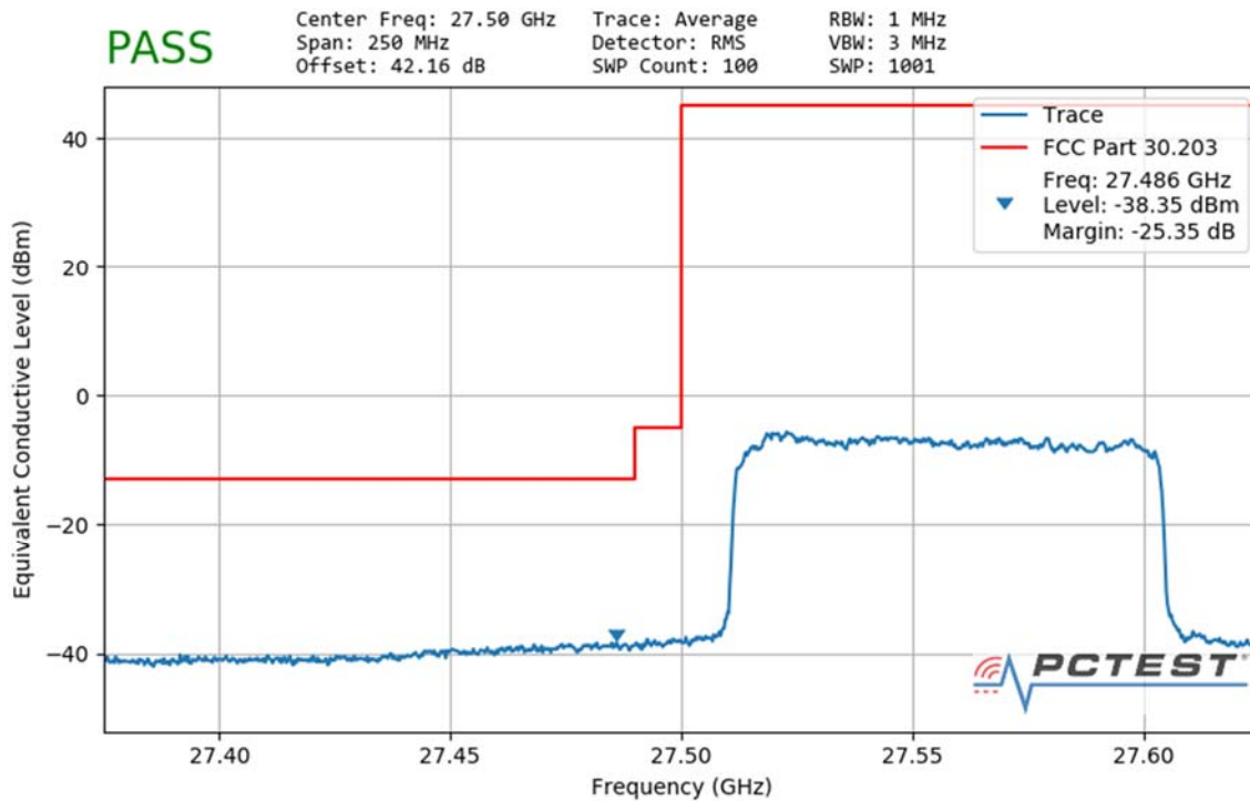
Plot 7-143. Ant3 Lower Band Edge (100MHz-1CC – QPSK Full RB)
