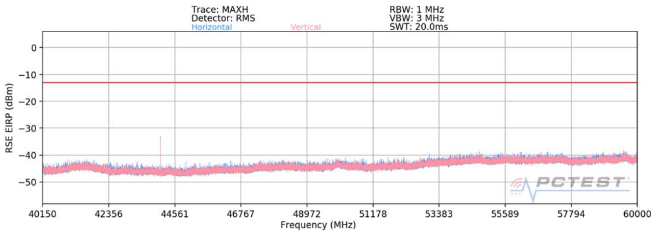
Plot 7-94. Ant3-n260 Radiated Spurious Plot (1CC QPSK Mid Channel V Beam)
