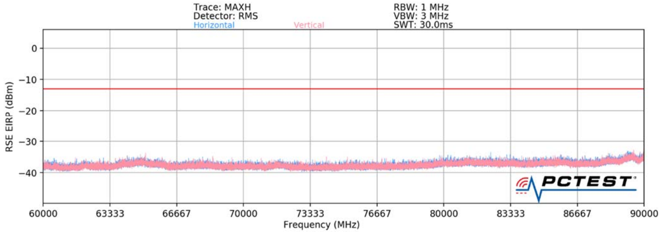
Plot 7-95. Ant3-n260 Radiated Spurious Plot (1CC QPSK Mid Channel H Beam)
