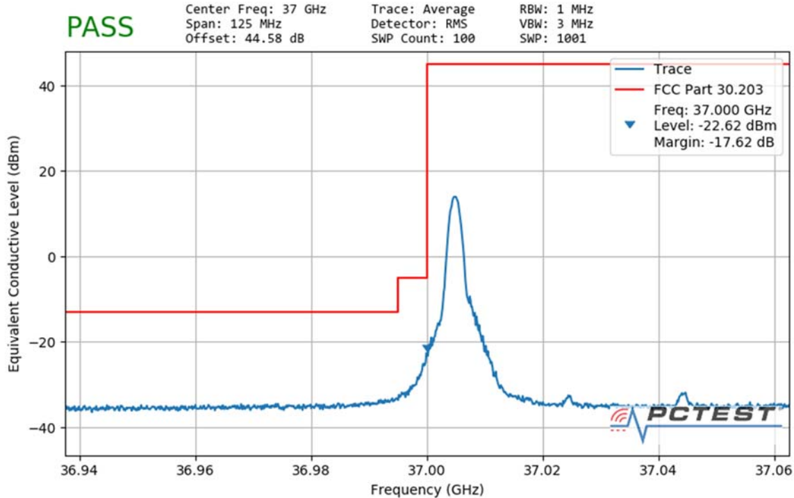
Plot 7-168. Ant2 Lower Band Edge (50MHz-1CC – QPSK 1 RB)
