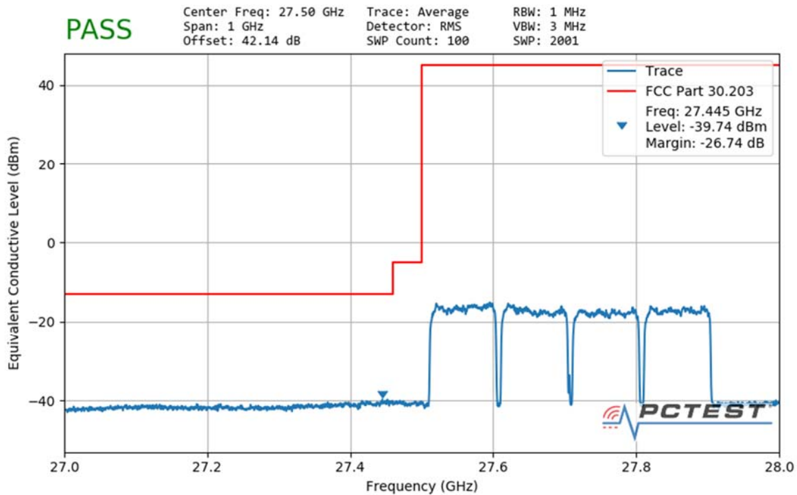
Plot 7-131. Ant2 Lower Band Edge (100MHz-4CC – QPSK Full RB)
