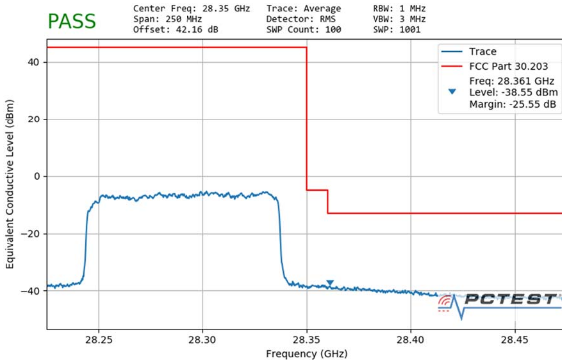
Plot 7-145. Ant3 Upper Band Edge (100MHz-1CC – QPSK Full RB)
