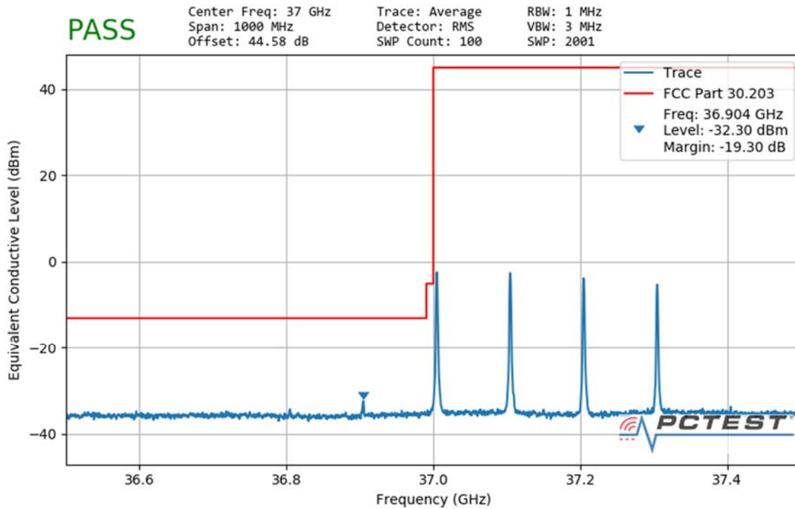
Plot 7-164. Ant1 Lower Band Edge (100MHz-4CC – QPSK 1 RB)
