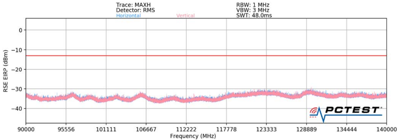
Plot 7-97. Ant3-n260 Radiated Spurious Plot (1CC QPSK Mid Channel H Beam)
