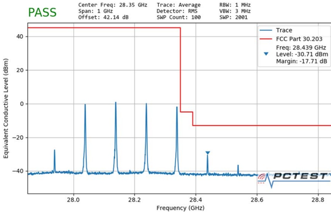
Plot 7-134. Ant2 Upper Band Edge (100MHz-4CC – QPSK 1 RB)
