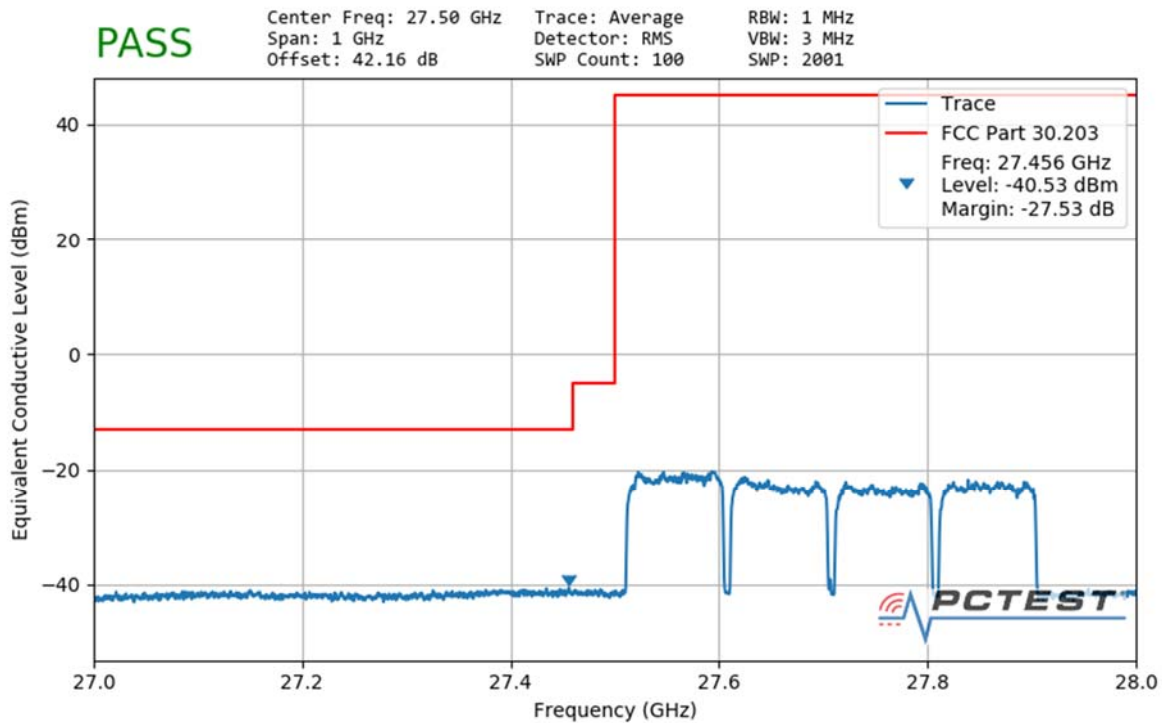
Plot 7-147. Ant3 Lower Band Edge (100MHz-4CC – QPSK Full RB)
