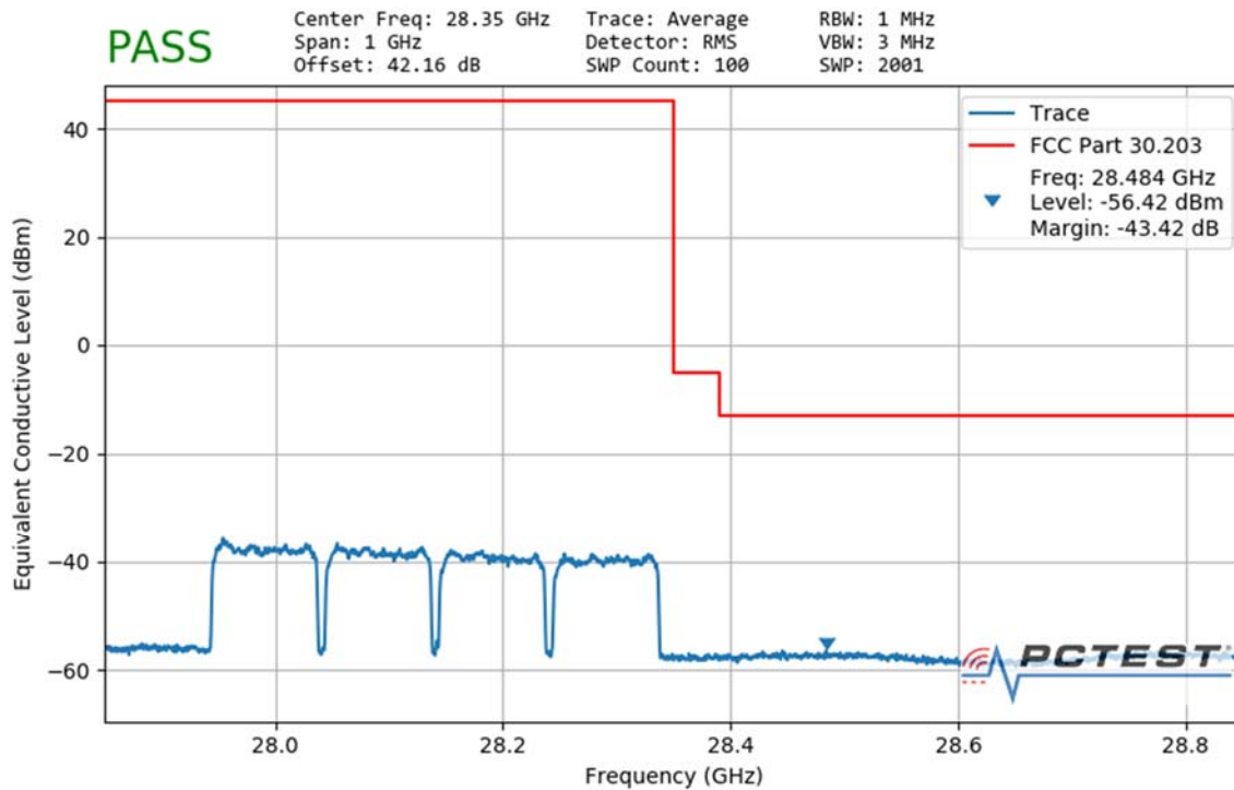
Plot 7-117. Ant1 Upper Band Edge (100MHz-4CC – QPSK Full RB)
