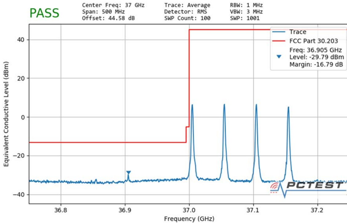
Plot 7-172. Ant2 Lower Band Edge (50MHz-4CC – QPSK 1 RB)
