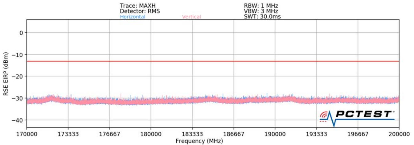
Plot 7-73. Ant1-n260 Radiated Spurious Plot (1CC QPSK Mid Channel H Beam)
