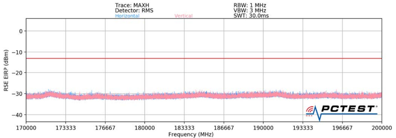
Plot 7-102. Ant3-n260 Radiated Spurious Plot (1CC QPSK Mid Channel V Beam)
