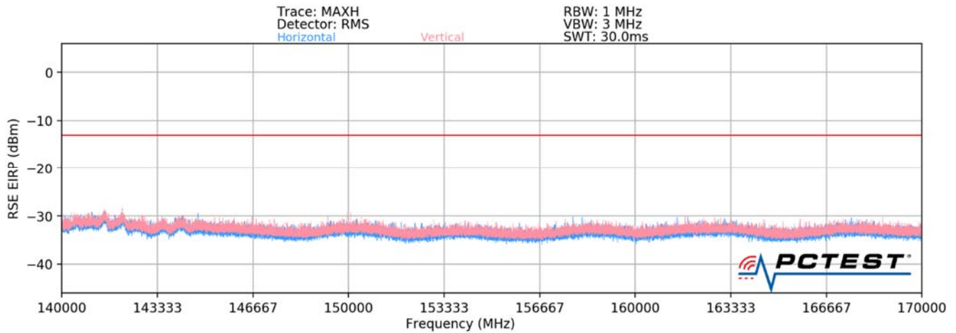
Plot 7-85. Ant2-n260 Radiated Spurious Plot (1CC QPSK Mid Channel H Beam)
