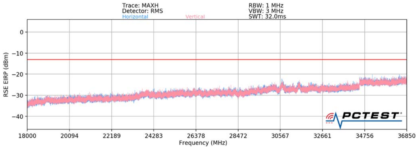
Plot 7-77. Ant2-n260 Radiated Spurious Plot (1CC QPSK Mid Channel H Beam)
