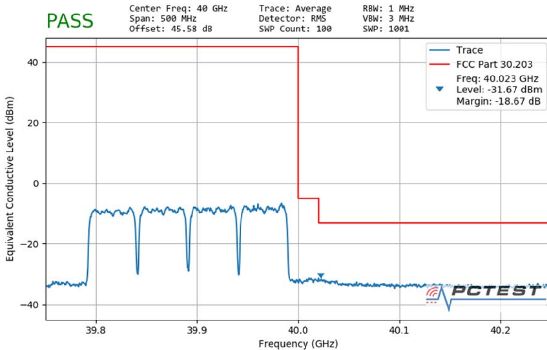
Plot 7-157. Ant1 Upper Band Edge (50MHz-4CC – QPSK Full RB)
