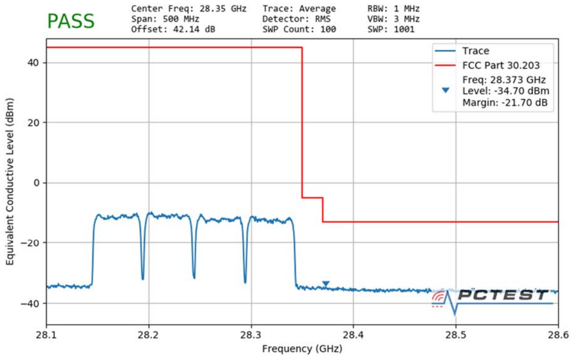
Plot 7-109. Ant1 Upper Band Edge (50MHz-4CC – QPSK Full RB)
