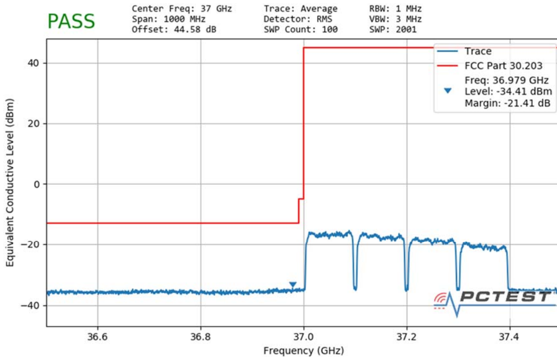
Plot 7-163. Ant1 Lower Band Edge (100MHz-4CC – QPSK Full RB)
