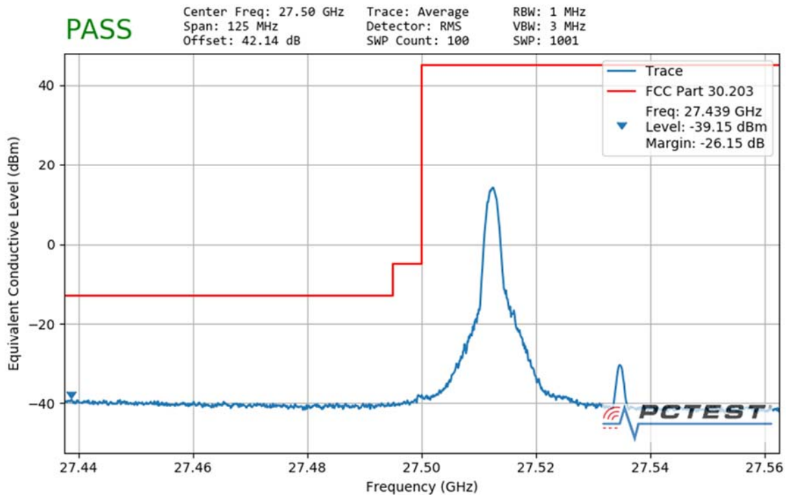
Plot 7-120. Ant2 Lower Band Edge (50MHz-1CC – QPSK 1 RB)
