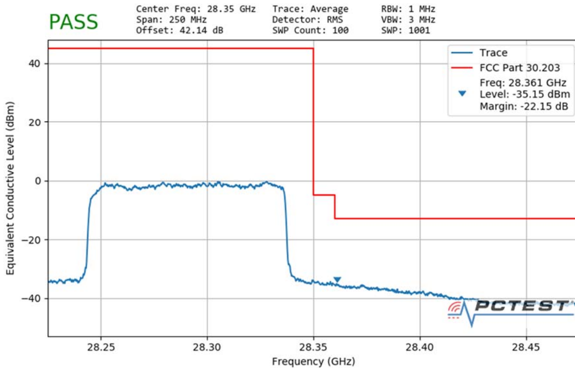
Plot 7-129. Ant2 Upper Band Edge (100MHz-1CC – QPSK Full RB)
