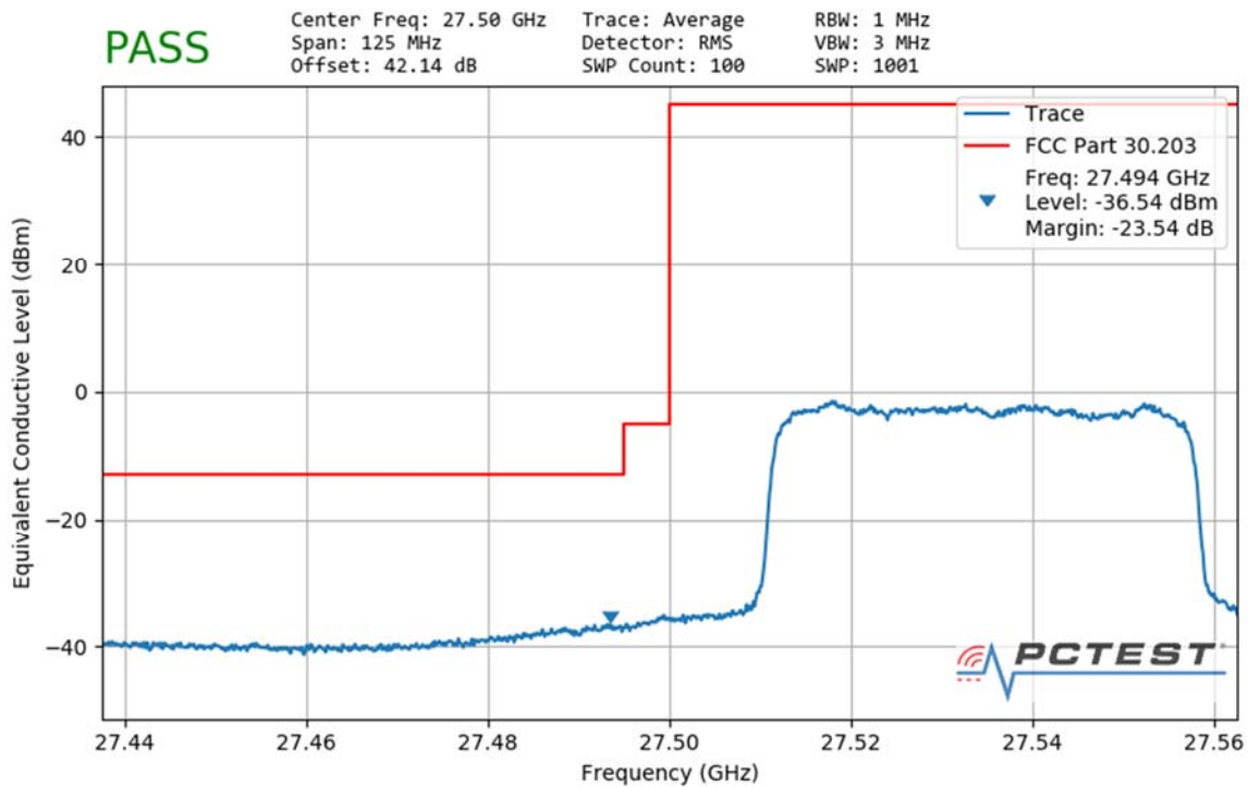
Plot 7-135. Ant3 Lower Band Edge (50MHz-1CC – QPSK Full RB)
