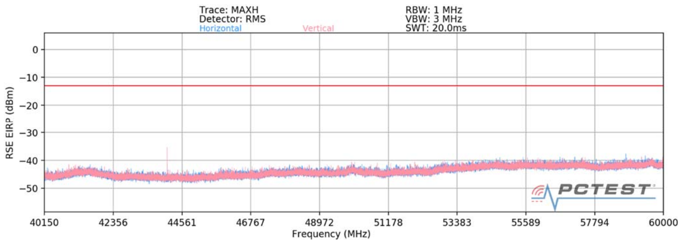
Plot 7-80. Ant2-n260 Radiated Spurious Plot (1CC QPSK Mid Channel V Beam)
