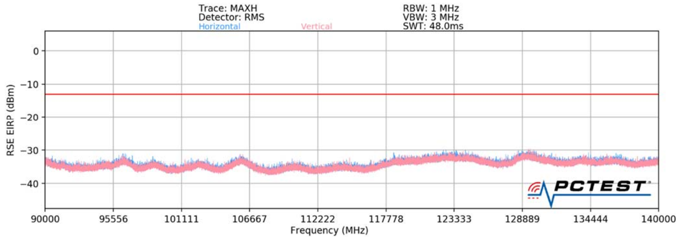
Plot 7-83. Ant2-n260 Radiated Spurious Plot (1CC QPSK Mid Channel H Beam)
