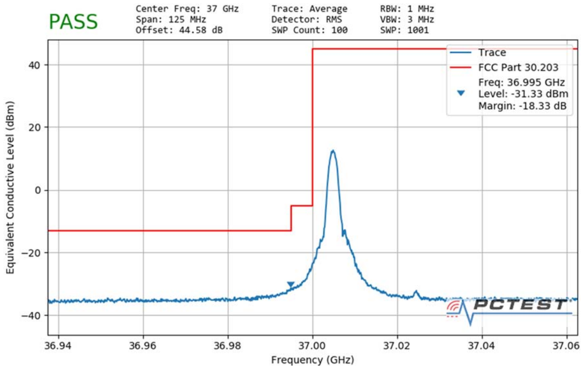
Plot 7-152. Ant1 Lower Band Edge (50MHz-1CC – QPSK 1 RB)
