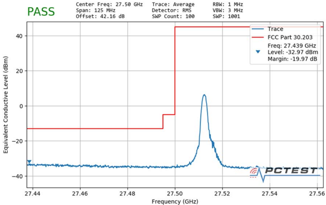
Plot 7-104. Ant1 Lower Band Edge (50MHz-1CC – QPSK 1 RB)
