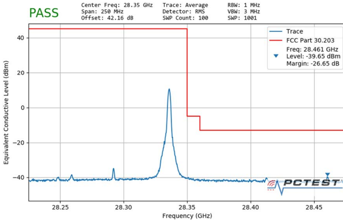
Plot 7-146. Ant3 Upper Band Edge (100MHz-1CC – QPSK 1 RB)
