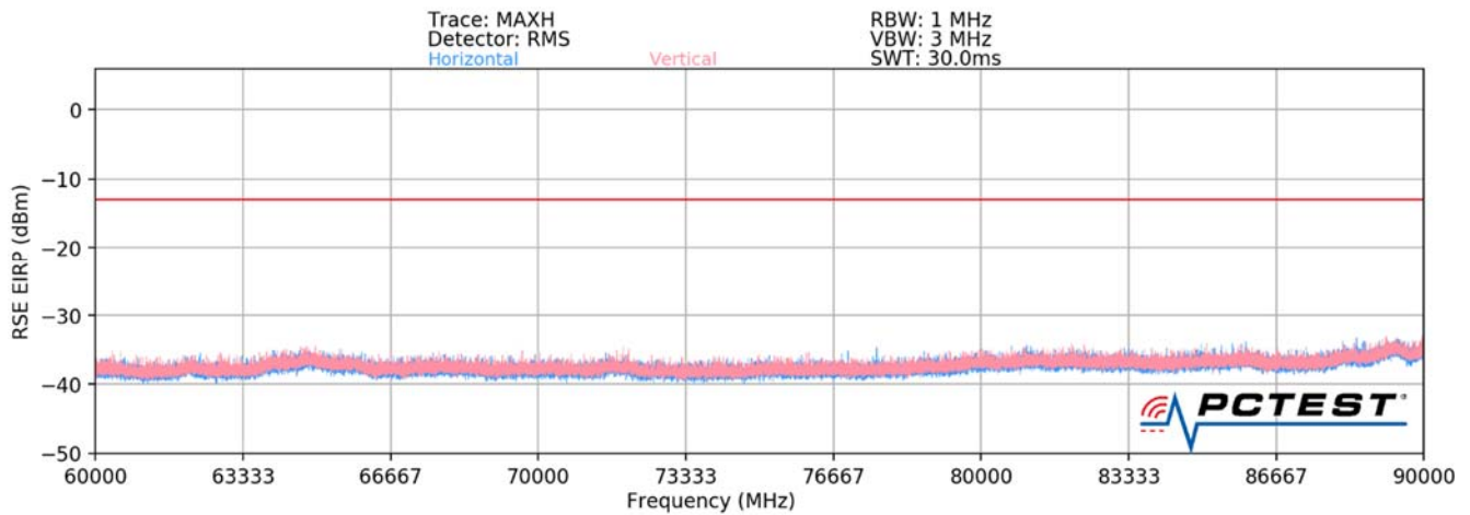
Plot 7-82. Ant2-n260 Radiated Spurious Plot (1CC QPSK Mid Channel V Beam)
