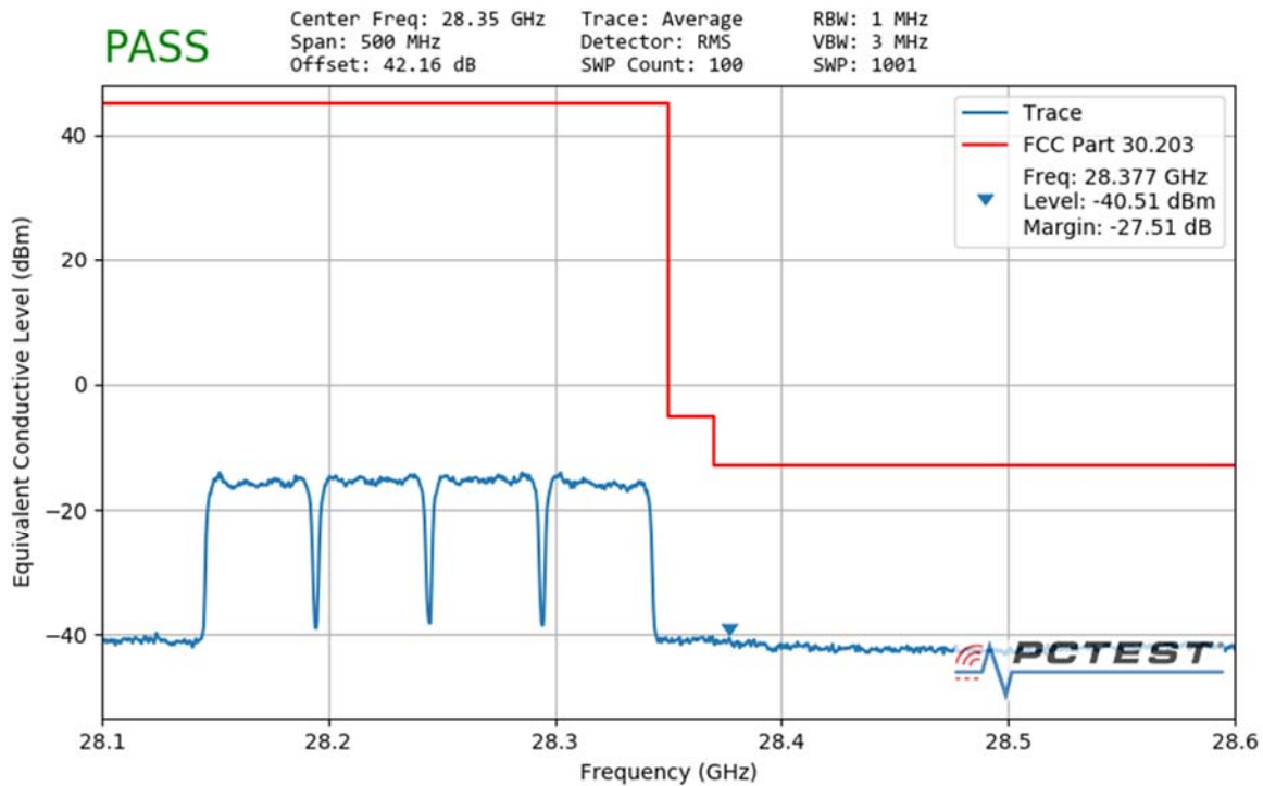
Plot 7-141. Ant3 Upper Band Edge (50MHz-4CC – QPSK Full RB)
