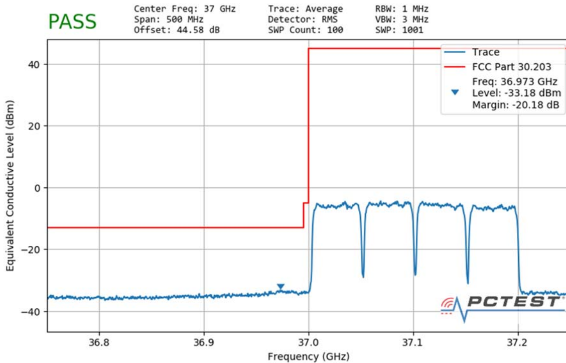
Plot 7-171. Ant2 Lower Band Edge (50MHz-4CC – QPSK Full RB)
