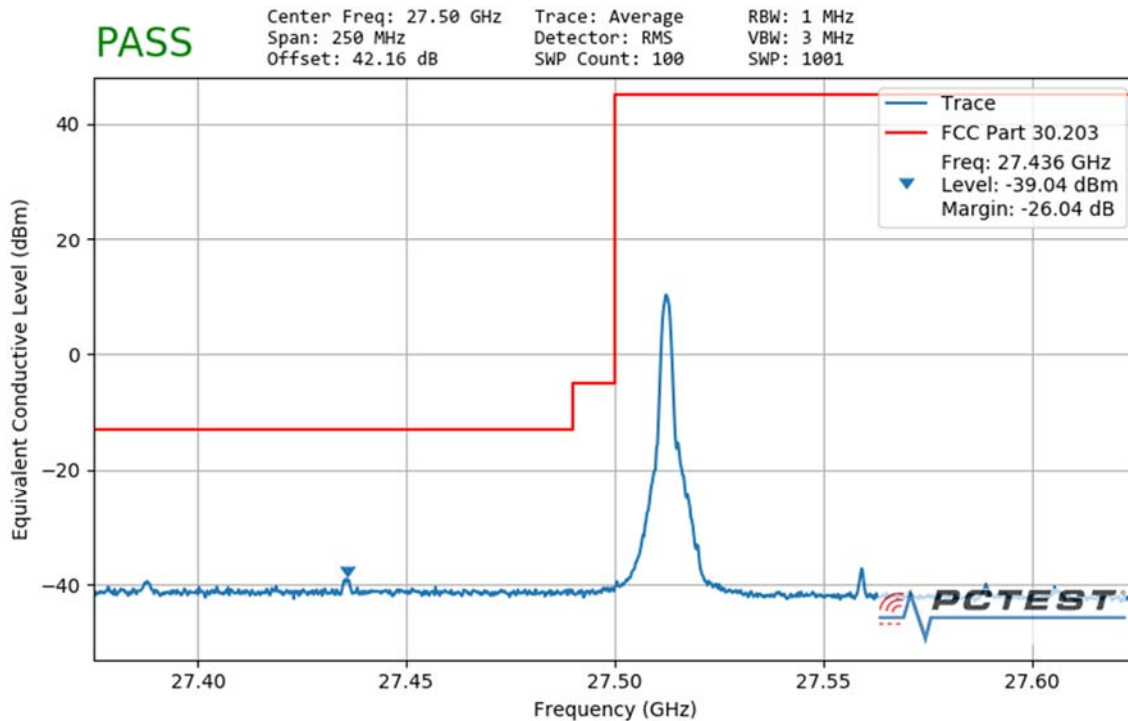
Plot 7-144. Ant3 Lower Band Edge (100MHz-1CC – QPSK 1 RB)
