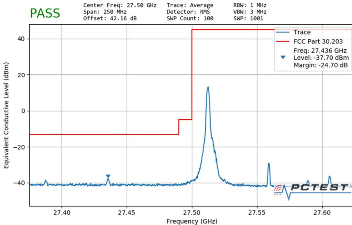
Plot 7-128. Ant2 Lower Band Edge (100MHz-1CC – QPSK 1 RB)
