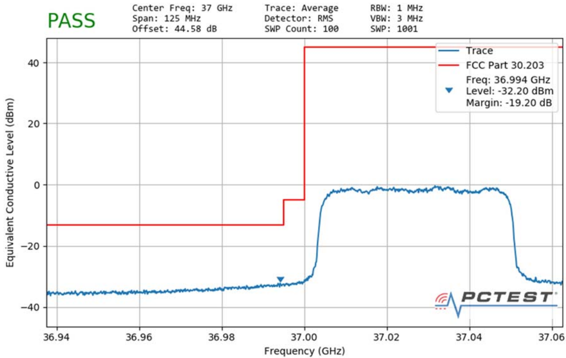
Plot 7-151. Ant1 Lower Band Edge (50MHz-1CC – QPSK Full RB)
