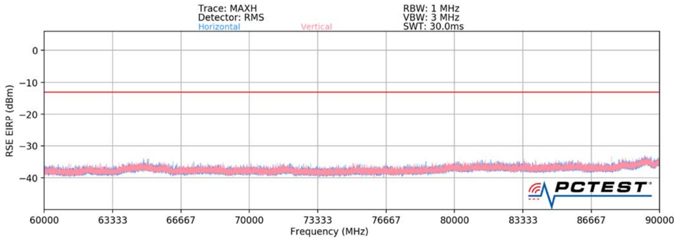
Plot 7-96. Ant3-n260 Radiated Spurious Plot (1CC QPSK Mid Channel V Beam)
