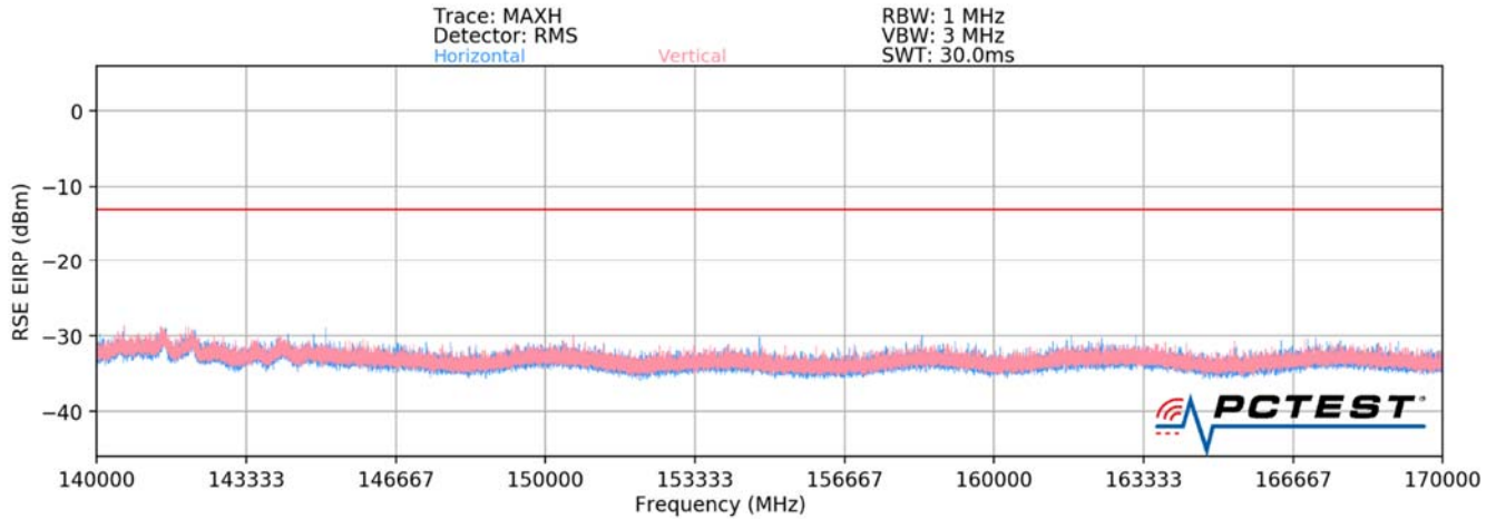
Plot 7-99. Ant3-n260 Radiated Spurious Plot (1CC QPSK Mid Channel H Beam)
