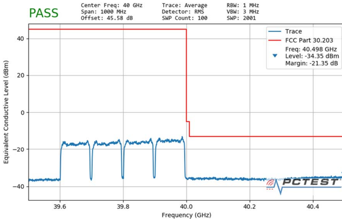
Plot 7-165. Ant1 Upper Band Edge (100MHz-4CC – QPSK Full RB)
