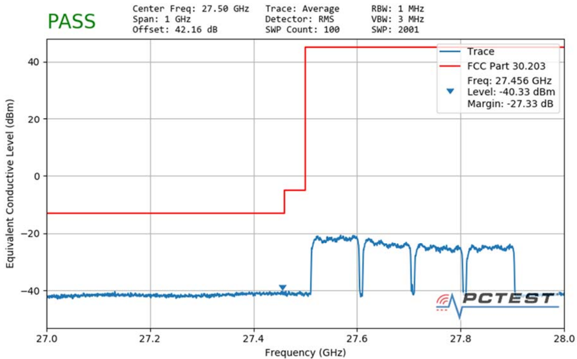
Plot 7-115. Ant1 Lower Band Edge (100MHz-4CC – QPSK Full RB)
