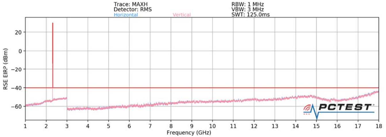
Plot 7-90. Ant3-n260 Radiated Spurious Plot 1GHz - 18GHz (1CC QPSK Mid Channel)
