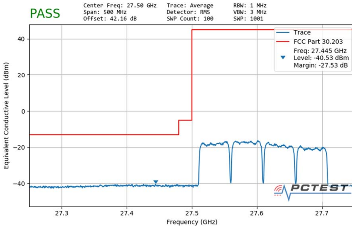
Plot 7-139. Ant3 Lower Band Edge (50MHz-4CC – QPSK Full RB)
