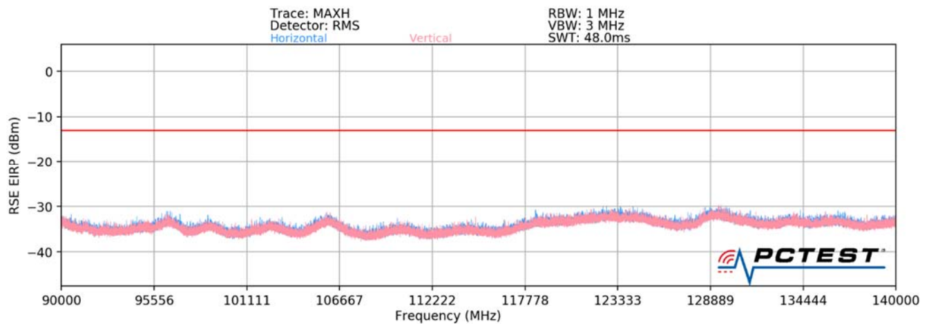
Plot 7-84. Ant2-n260 Radiated Spurious Plot (1CC QPSK Mid Channel V Beam)
