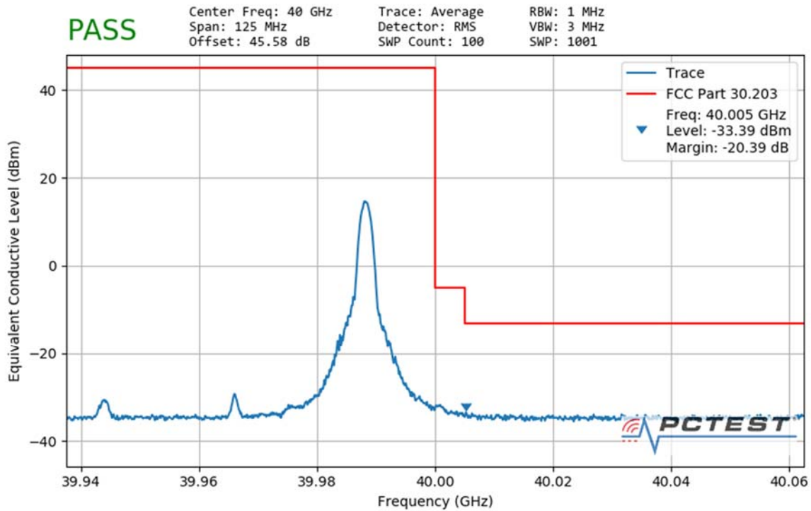
Plot 7-170. Ant2 Upper Band Edge (50MHz-1CC – QPSK 1 RB)
