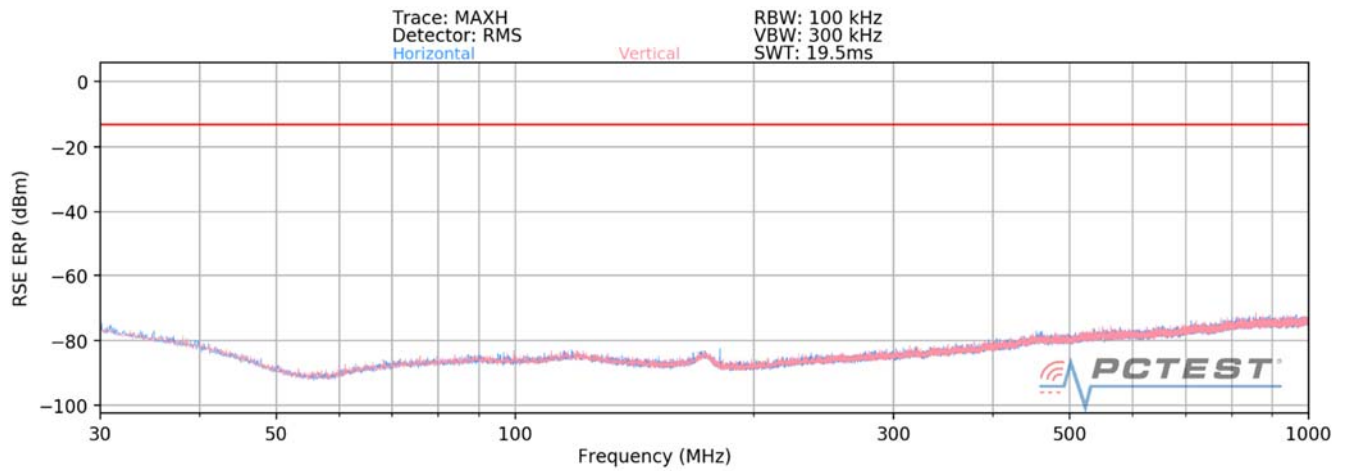
Plot 7-75. Ant2-n260 Radiated Spurious Plot (1CC QPSK Mid Channel)
