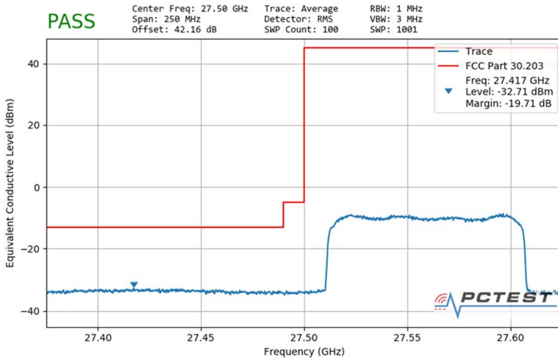
Plot 7-111. Ant1 Lower Band Edge (100MHz-1CC – QPSK Full RB)
