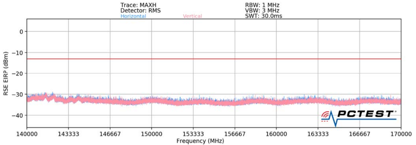
Plot 7-71. Ant1-n260 Radiated Spurious Plot (1CC QPSK Mid Channel H Beam)
