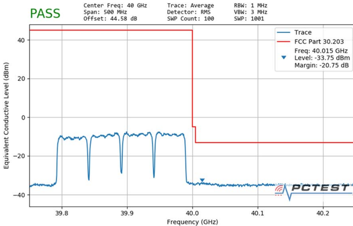
Plot 7-173. Ant2 Upper Band Edge (50MHz-4CC – QPSK Full RB)
