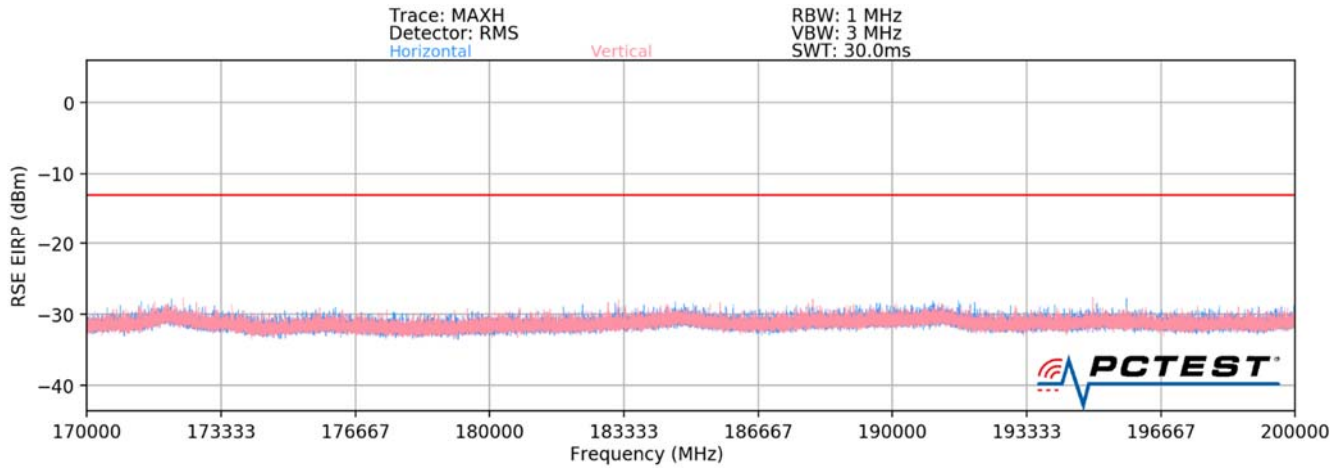
Plot 7-87. Ant2-n260 Radiated Spurious Plot (1CC QPSK Mid Channel H Beam)
