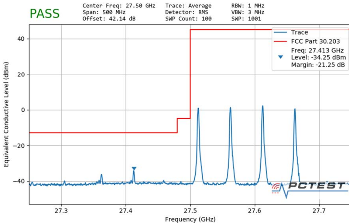
Plot 7-124. Ant2 Lower Band Edge (50MHz-4CC – QPSK 1 RB)
