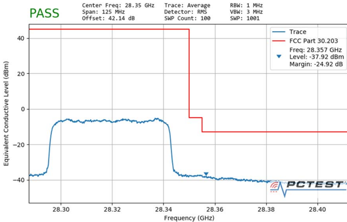
Plot 7-137. Ant3 Upper Band Edge (50MHz-1CC – QPSK Full RB)
