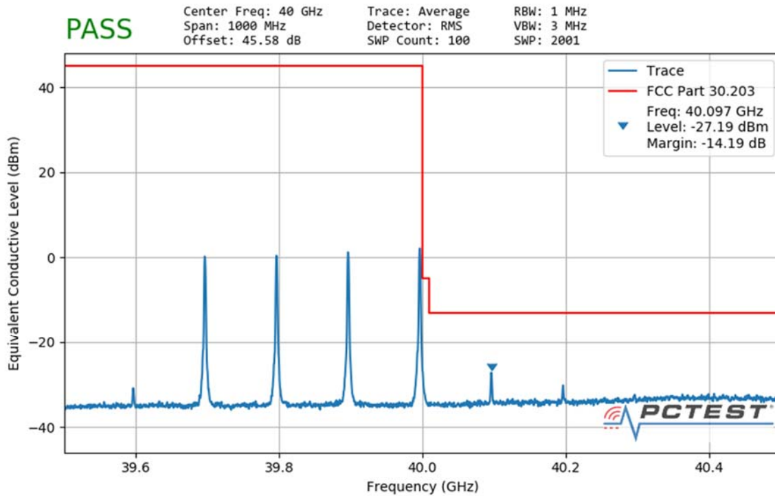
Plot 7-166. Ant1 Upper Band Edge (100MHz-4CC – QPSK 1 RB)
