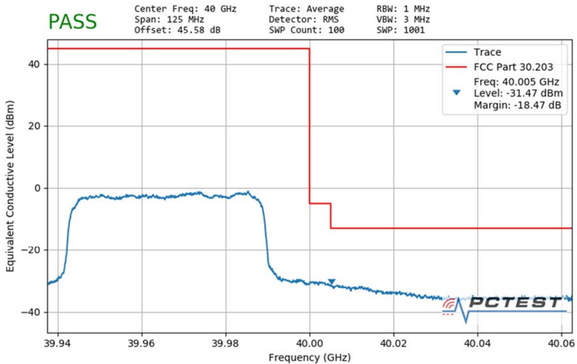
Plot 7-153. Ant1 Upper Band Edge (50MHz-1CC – QPSK Full RB)
