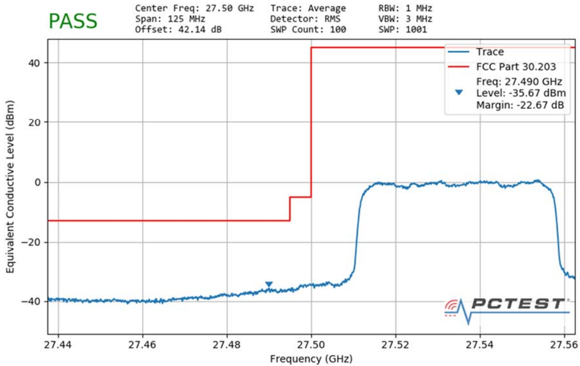
Plot 7-119. Ant2 Lower Band Edge (50MHz-1CC – QPSK Full RB)
