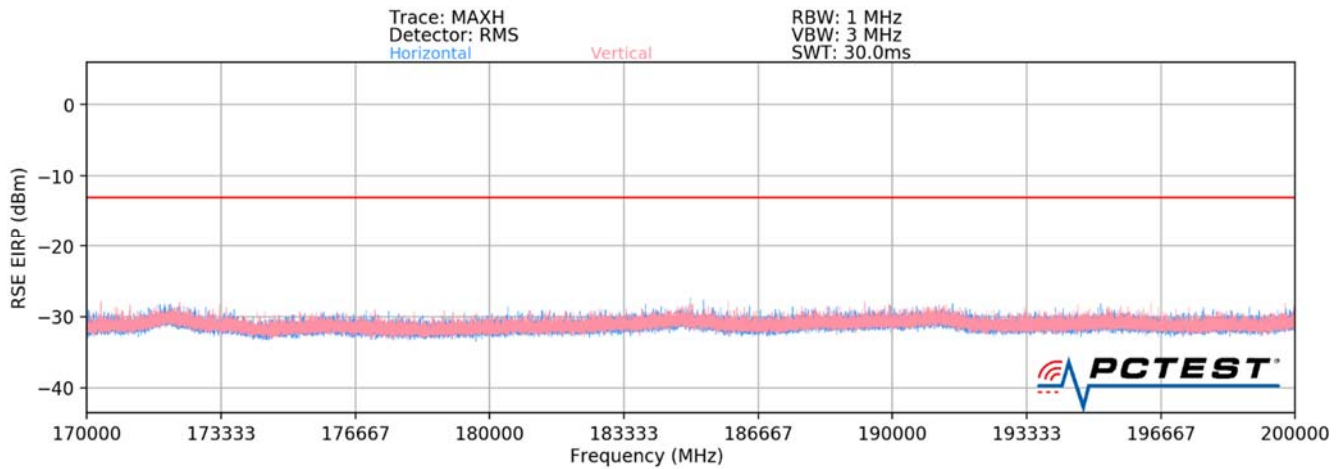
Plot 7-74. Ant1-n260 Radiated Spurious Plot (1CC QPSK Mid Channel V Beam)
