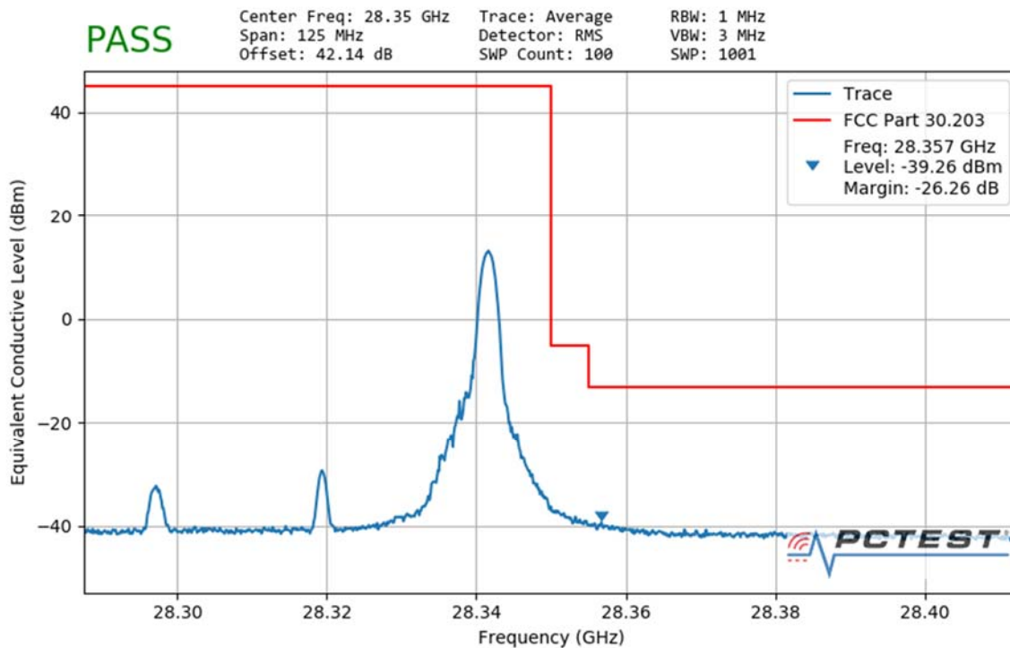
Plot 7-122. Ant2 Upper Band Edge (50MHz-1CC – QPSK 1 RB)
