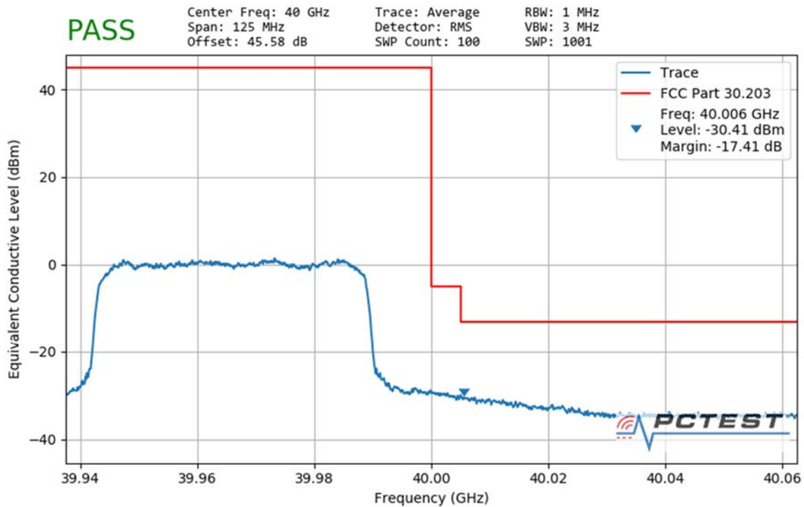
Plot 7-169. Ant2 Upper Band Edge (50MHz-1CC – QPSK Full RB)
