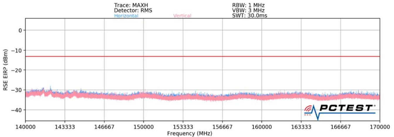
Plot 7-100. Ant3-n260 Radiated Spurious Plot (1CC QPSK Mid Channel V Beam)
