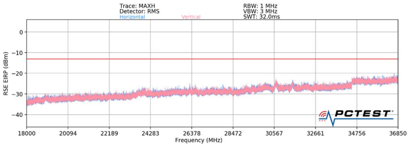
Plot 7-78. Ant2-n260 Radiated Spurious Plot (1CC QPSK Mid Channel V Beam)
