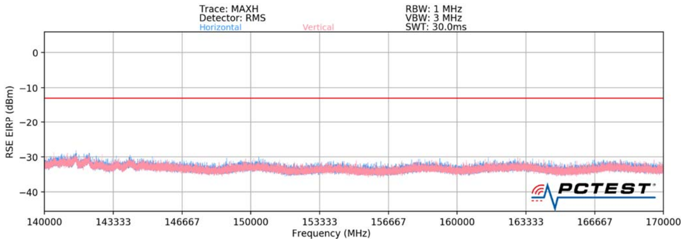
Plot 7-72. Ant1-n260 Radiated Spurious Plot (1CC QPSK Mid Channel V Beam)
