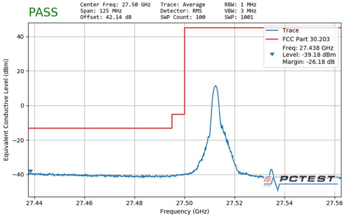
Plot 7-136. Ant3 Lower Band Edge (50MHz-1CC – QPSK 1 RB)
