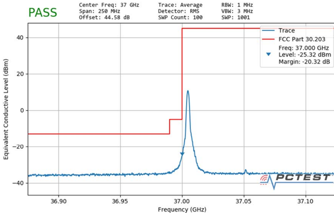
Plot 7-160. Ant1 Lower Band Edge (100MHz-1CC – QPSK 1 RB)
