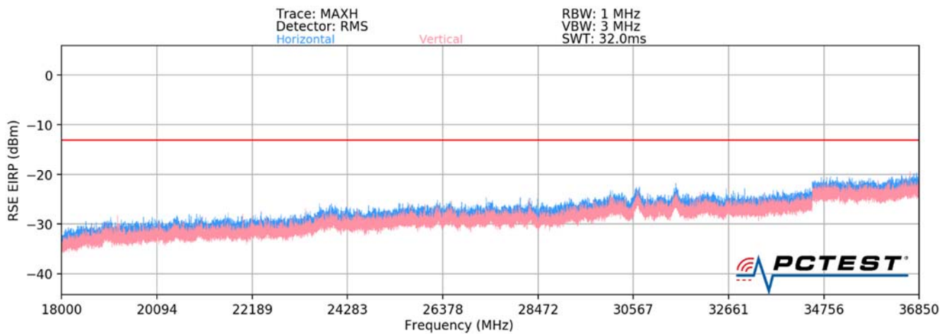
Plot 7-92. Ant3-n260 Radiated Spurious Plot (1CC QPSK Mid Channel V Beam)
