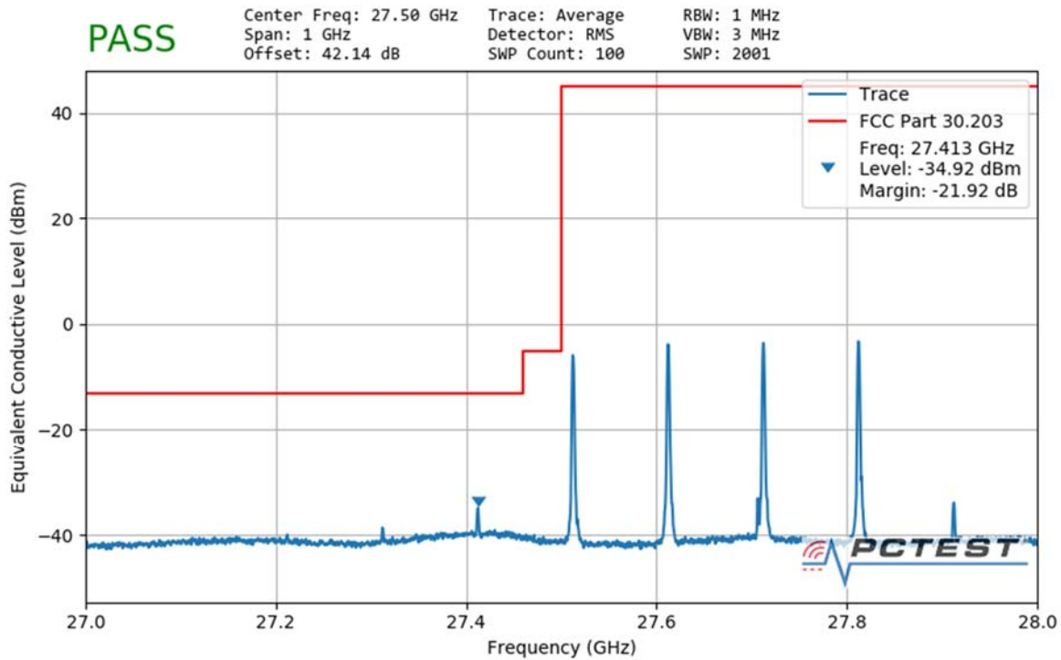
Plot 7-116. Ant1 Lower Band Edge (100MHz-4CC – QPSK 1 RB)
