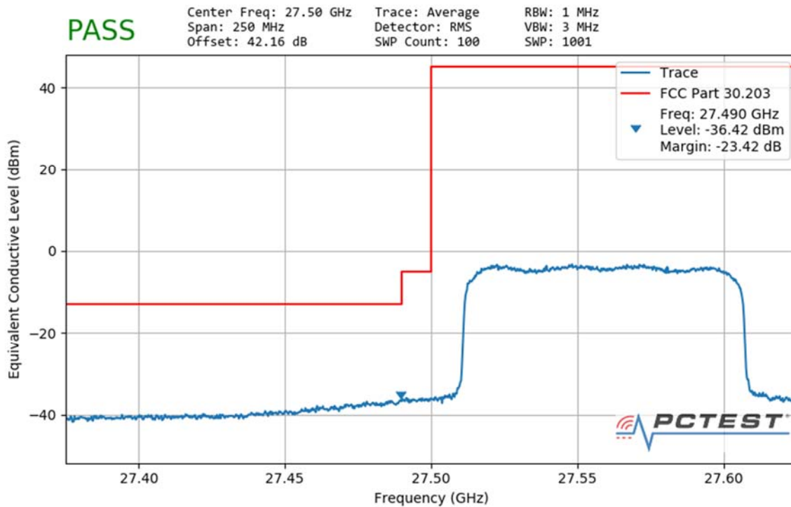
Plot 7-127. Ant2 Lower Band Edge (100MHz-1CC – QPSK Full RB)
