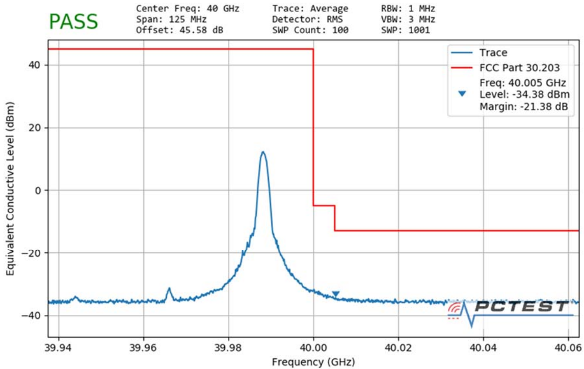
Plot 7-154. Ant1 Upper Band Edge (50MHz-1CC – QPSK 1 RB)
