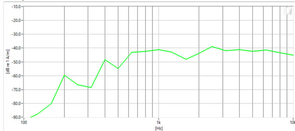
Noise Spectrum
