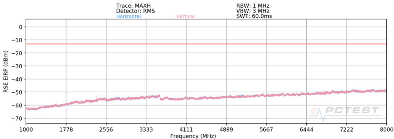
Plot 7-2. Radiated Spurious Plot (Band 14)
