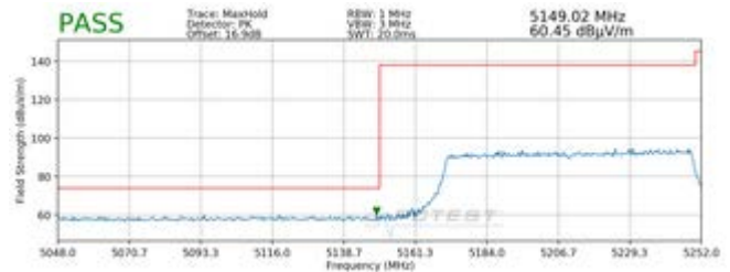
Plot 7-73. Radiated Lower Band Edge Plot SISO ANT2 (Peak - UNII Band 1 - 996 Tones)
