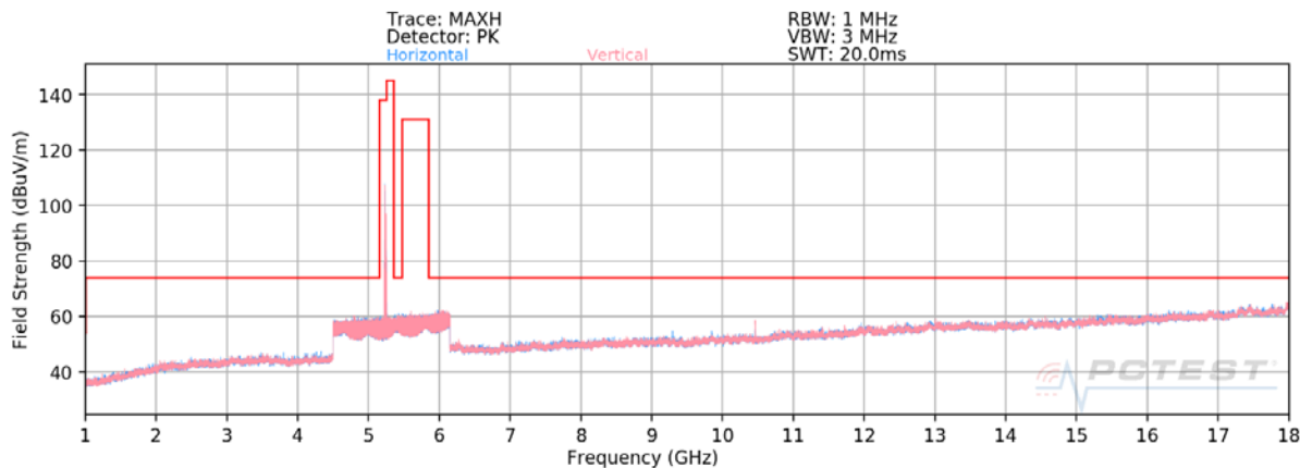
Plot 7-13. Radiated Spurious Plot above 1GHz SISO ANT2 (802.11ax – U1 Ch. 40 – 26 Tones)
