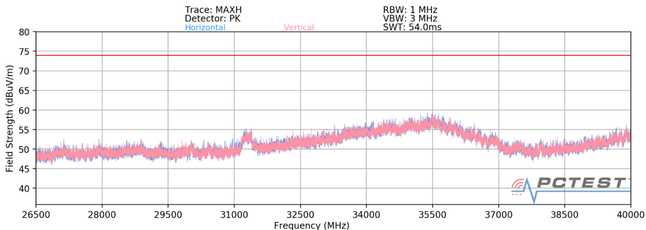
Plot 7-18. Radiated Spurious Plot 26.5GHz - 40GHz SISO ANT2 (802.11ax - 26 Tones)
