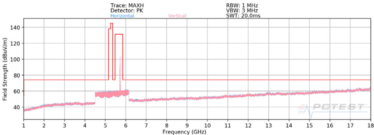
Plot 7-3. Radiated Spurious Plot above 1GHz SISO ANT1 (802.11ax – U2C Ch. 120 – 26 Tones)
