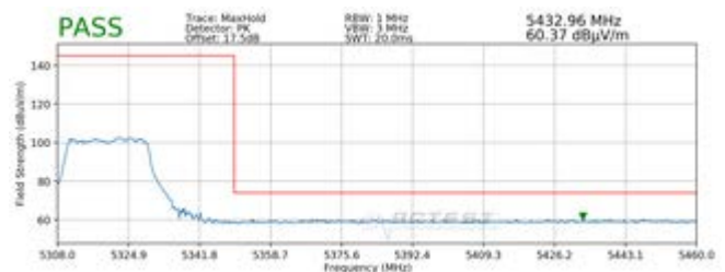
Plot 7-61. Radiated Upper Band Edge Plot SISO ANT2 (Peak - UNII Band 2A - 242 Tones)
