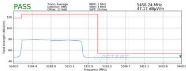
Plot 7-53. Radiated Upper Band Edge Plot SISO ANT1 (Average - UNII Band 2A - 996 Tones)
