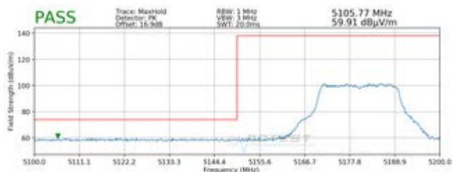
Plot 7-38. Radiated Lower Band Edge Plot SISO ANT1 (Peak - UNII Band 1 - 242 Tones)
