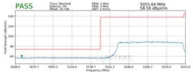
Plot 7-94. Radiated Lower Band Edge Plot MIMO (Peak – UNII Band 1 – 996 Tones)
