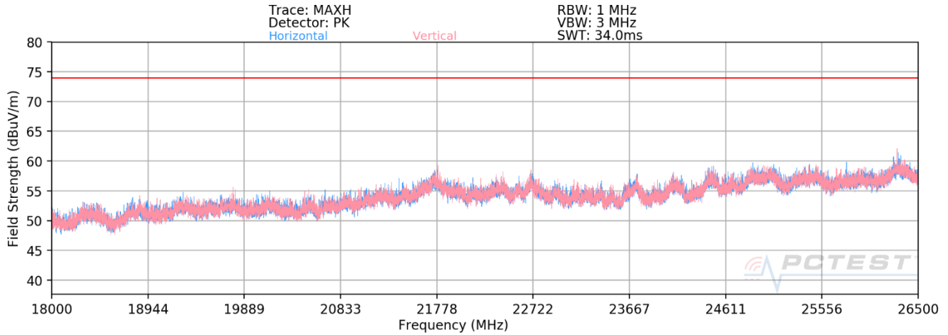
Plot 7-29. Radiated Spurious Plot 18GHz - 26.5GHz MIMO (802.11ax – 26 Tones)
