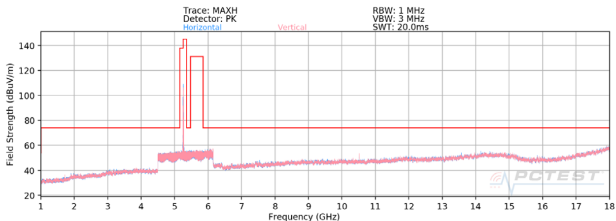
Plot 7-26. Radiated Spurious Plot above 1GHz MIMO (802.11ax – U2A Ch. 56 – 26 Tones)
