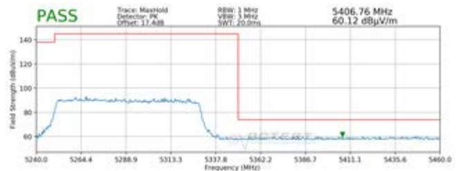
Plot 7-54. Radiated Upper Band Edge Plot SISO ANT1 (Peak - UNII Band 2A - 996 Tones)
