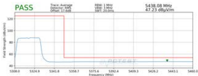
Plot 7-39. Radiated Upper Band Edge Plot SISO ANT1 (Average - UNII Band 2A - 242 Tones)
