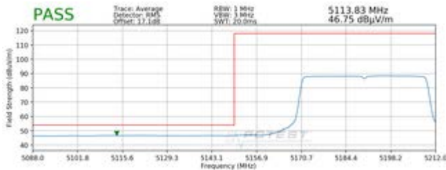
Plot 7-65. Radiated Lower Band Edge Plot SISO ANT2 (Average - UNII Band 1 - 484 Tones)
