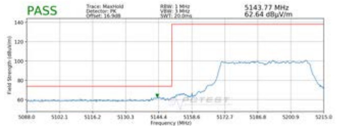
Plot 7-66. Radiated Lower Band Edge Plot SISO ANT2 (Peak - UNII Band 1 - 484 Tones)
