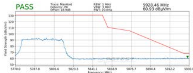
Plot 7-50. Radiated Upper Band Edge Plot SISO ANT1 (Peak – UNII Band 3 – 484 Tones)
