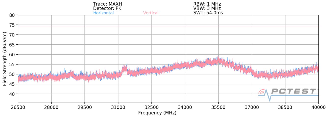
Plot 7-36. Radiated Spurious Plot 26.5GHz - 40GHz MIMO (802.11ax - 242 Tones)
