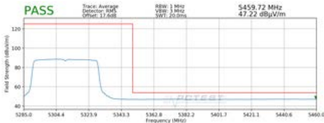
Plot 7-67. Radiated Upper Band Edge Plot SISO ANT2 (Average - UNII Band 2A - 484 Tones)
