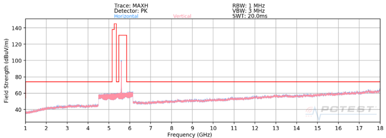
Plot 7-21. Radiated Spurious Plot above 1GHz SISO ANT2 (802.11ax – U2C Ch. 120 – 242 Tones)
