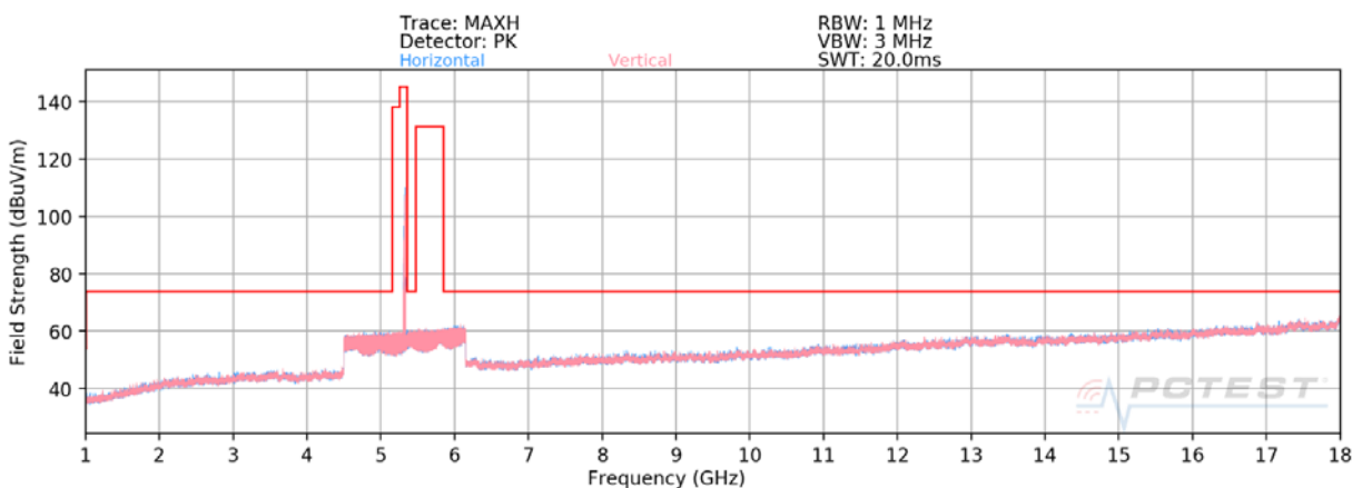
Plot 7-2. Radiated Spurious Plot above 1GHz SISO ANT1 (802.11ax – U2A Ch. 56 – 26 Tones)
