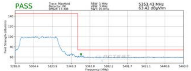
Plot 7-68. Radiated Upper Band Edge Plot SISO ANT2 (Peak - UNII Band 2A - 484 Tones)
