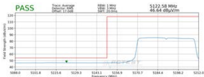
Plot 7-44. Radiated Lower Band Edge Plot SISO ANT1 (Average - UNII Band 1 - 484 Tones)
