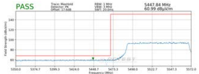
Plot 7-56. Radiated Lower Band Edge Plot SISO ANT1 (Peak – UNII Band 2C – 996 Tones)
