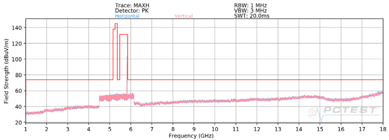
Plot 7-28. Radiated Spurious Plot above 1GHz MIMO (802.11ax – U3 Ch. 157 – 26 Tones)
