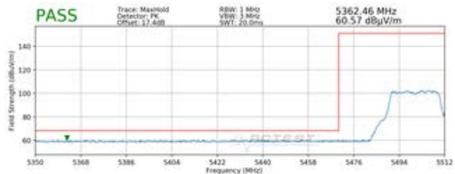
Plot 7-42. Radiated Lower Band Edge Plot SISO ANT1 (Peak - UNII Band 2C - 242 Tones)
