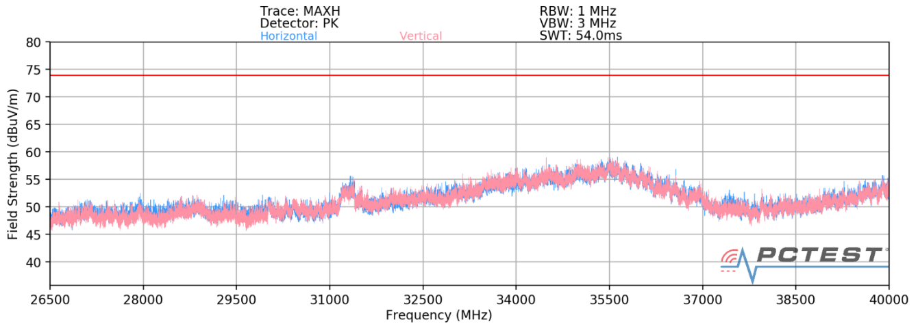
Plot 7-30. Radiated Spurious Plot 26.5GHz - 40GHz MIMO (802.11ax – 26 Tones)
