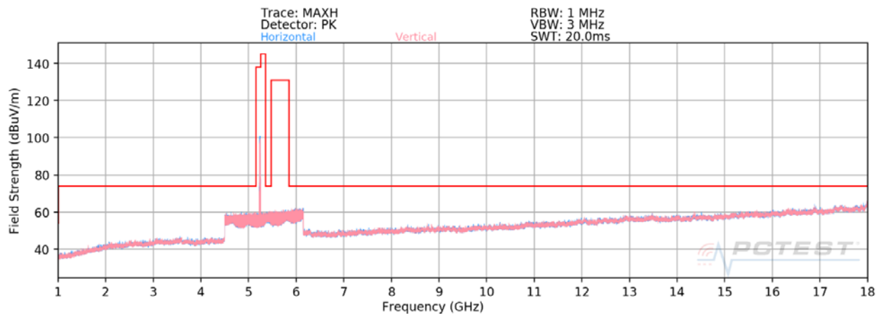
Plot 7-19. Radiated Spurious Plot above 1GHz SISO ANT2 (802.11ax – U1 Ch. 40 – 242 Tones)
