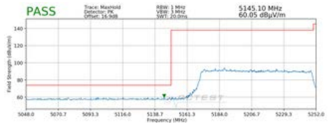
Plot 7-52. Radiated Lower Band Edge Plot SISO ANT1 (Peak - UNII Band 1 - 996 Tones)
