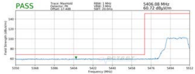
Plot 7-63. Radiated Lower Band Edge Plot SISO ANT2 (Peak - UNII Band 2C - 242 Tones)
