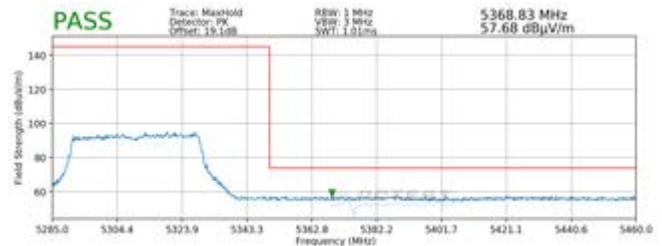
Plot 7-89. Radiated Upper Band Edge Plot MIMO (Peak - UNII Band 2A - 484 Tones)
