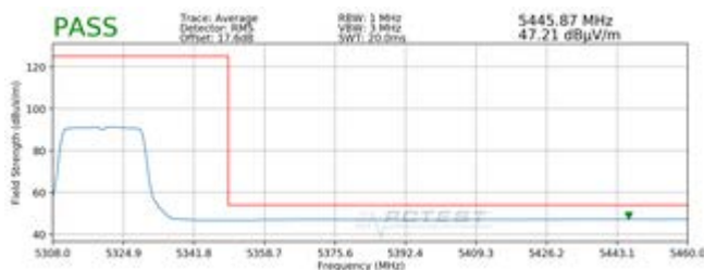
Plot 7-60. Radiated Upper Band Edge Plot SISO ANT2 (Average - UNII Band 2A - 242 Tones)
