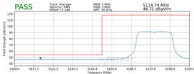
Plot 7-58. Radiated Lower Band Edge Plot SISO ANT2 (Average - UNII Band 1 - 242 Tones)
