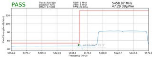
Plot 7-76. Radiated Lower Band Edge Plot SISO ANT2 (Average – UNII Band 2C – 996 Tones)
