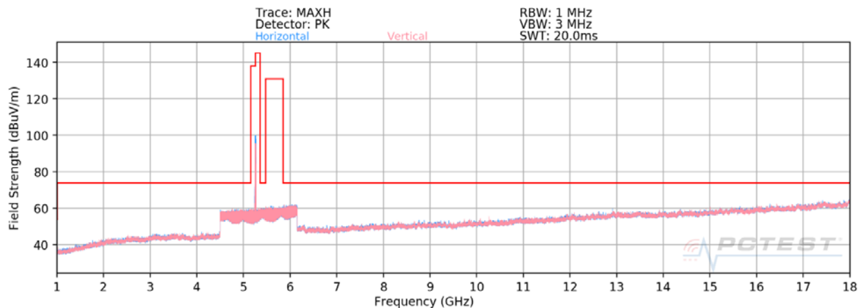
Plot 7-8. Radiated Spurious Plot above 1GHz SISO ANT1 (802.11ax – U2A Ch. 56 – 242 Tones)
