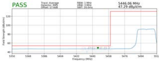
Plot 7-62. Radiated Lower Band Edge Plot SISO ANT2 (Average - UNII Band 2C - 242 Tones)
