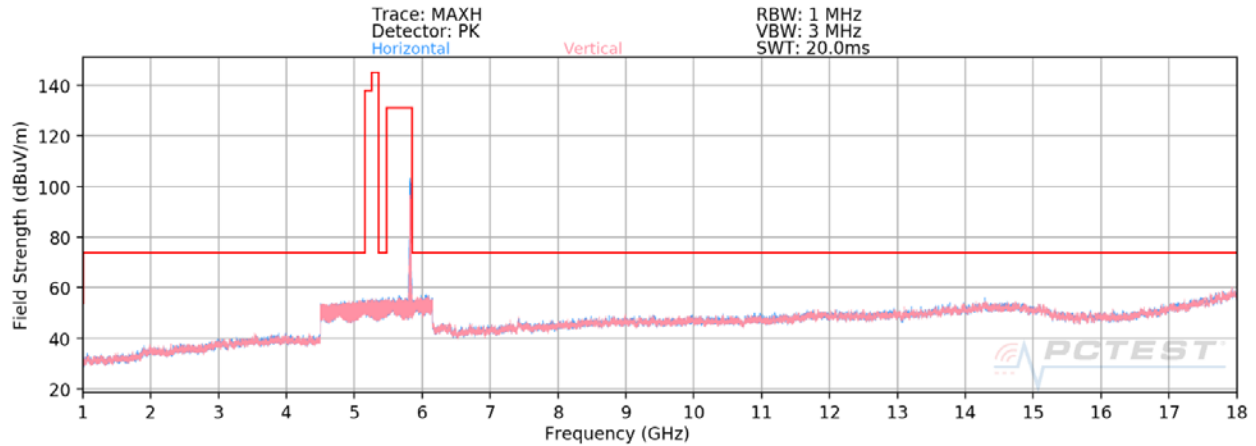
Plot 7-34. Radiated Spurious Plot above 1GHz MIMO (802.11ax – U3 Ch. 157 – 242 Tones)
