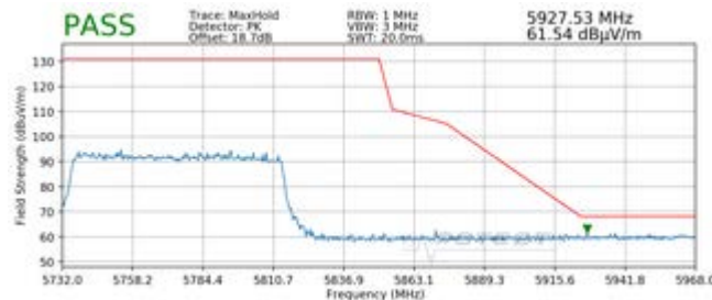
Plot 7-78. Radiated Upper Band Edge Plot SISO ANT2 (Peak – UNII Band 3 – 996 Tones)
