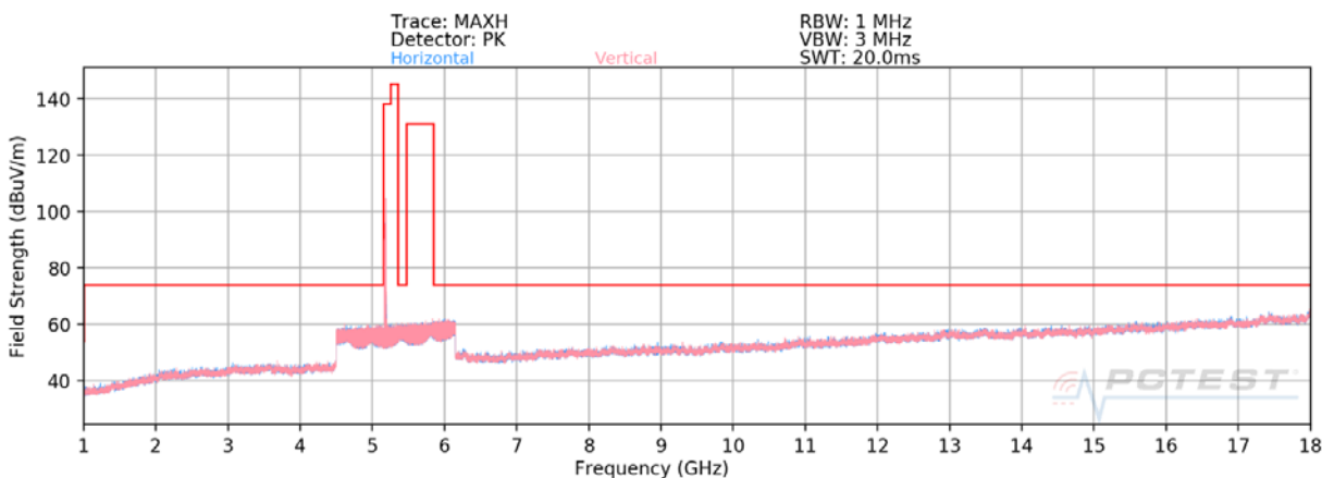
Plot 7-1. Radiated Spurious Plot above 1GHz SISO ANT1 (802.11ax – U1 Ch. 40 – 26 Tones)
