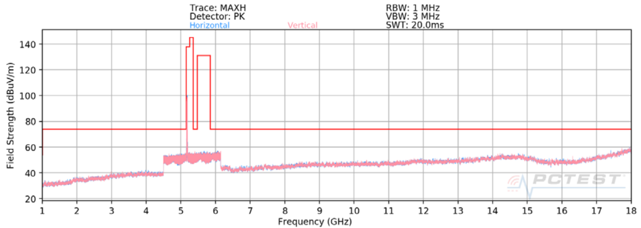
Plot 7-31. Radiated Spurious Plot above 1GHz MIMO (802.11ax – U1 Ch. 40 – 242 Tones)
