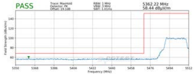
Plot 7-84. Radiated Lower Band Edge Plot MIMO (Peak - UNII Band 2C - 242 Tones)
