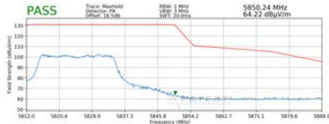
Plot 7-64. Radiated Upper Band Edge Plot SISO ANT2 (Peak - UNII Band 3 - 242 Tones)
