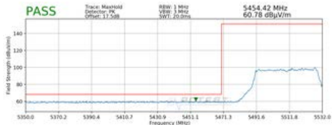
Plot 7-49. Radiated Lower Band Edge Plot SISO ANT1 (Peak – UNII Band 2C – 484 Tones)
