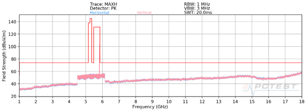
Plot 7-4. Radiated Spurious Plot above 1GHz SISO ANT1 (802.11ax – U3 Ch. 157 – 26 Tones)
