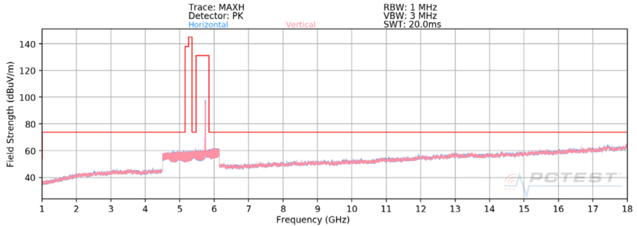
Plot 7-10. Radiated Spurious Plot above 1GHz SISO ANT1 (802.11ax – U3 Ch. 157 – 242 Tones)
