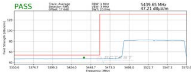
Plot 7-55. Radiated Lower Band Edge Plot SISO ANT1 (Average – UNII Band 2C – 996 Tones)
