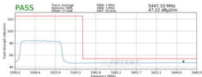
Plot 7-46. Radiated Upper Band Edge Plot SISO ANT1 (Average - UNII Band 2A - 484 Tones)
