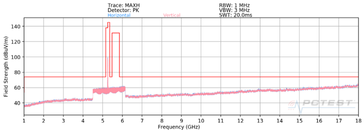
Plot 7-20. Radiated Spurious Plot above 1GHz SISO ANT2 (802.11ax – U2A Ch. 56 – 242 Tones)
