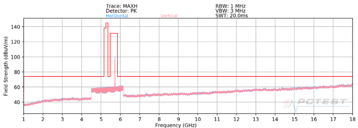
Plot 7-9. Radiated Spurious Plot above 1GHz SISO ANT1 (802.11ax – U2C Ch. 120 – 242 Tones)
