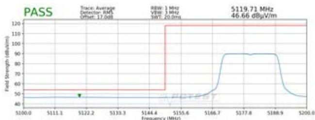
Plot 7-37. Radiated Lower Band Edge Plot SISO ANT1 (Average - UNII Band 1 - 242 Tones)
