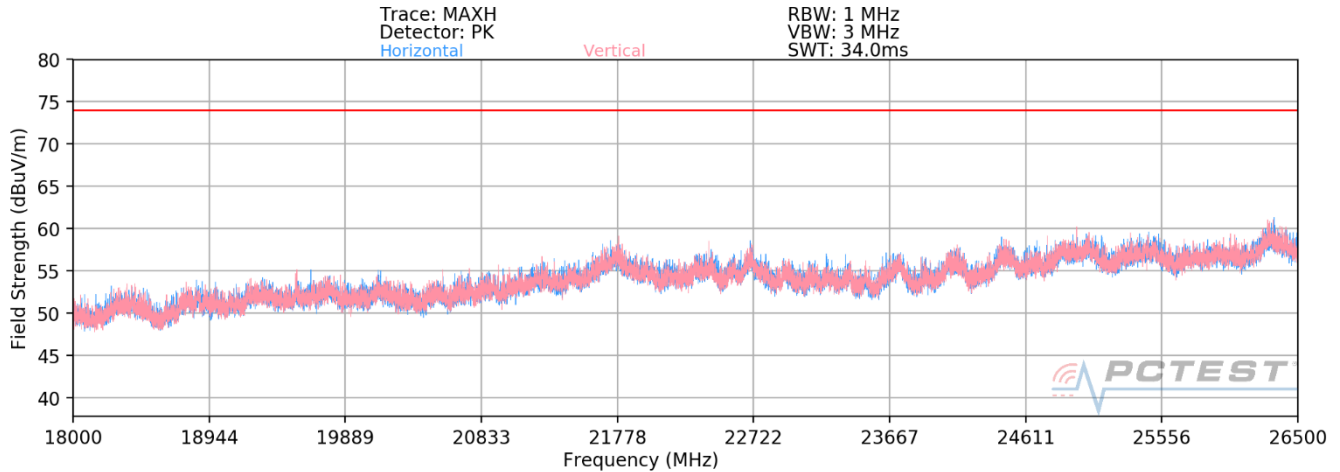
Plot 7-5. Radiated Spurious Plot 18GHz - 26.5GHz SISO ANT1 (802.11ax - 26 Tones)
