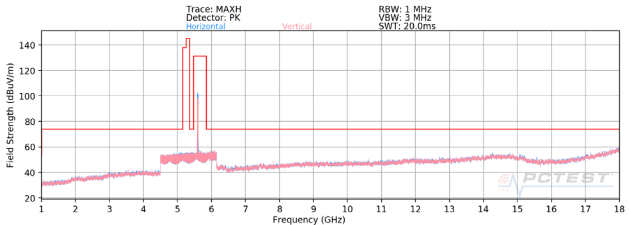
Plot 7-33. Radiated Spurious Plot above 1GHz MIMO (802.11ax – U2C Ch. 120 – 242 Tones)
