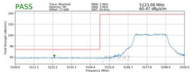
Plot 7-59. Radiated Lower Band Edge Plot SISO ANT2 (Peak - UNII Band 1 - 242 Tones)
