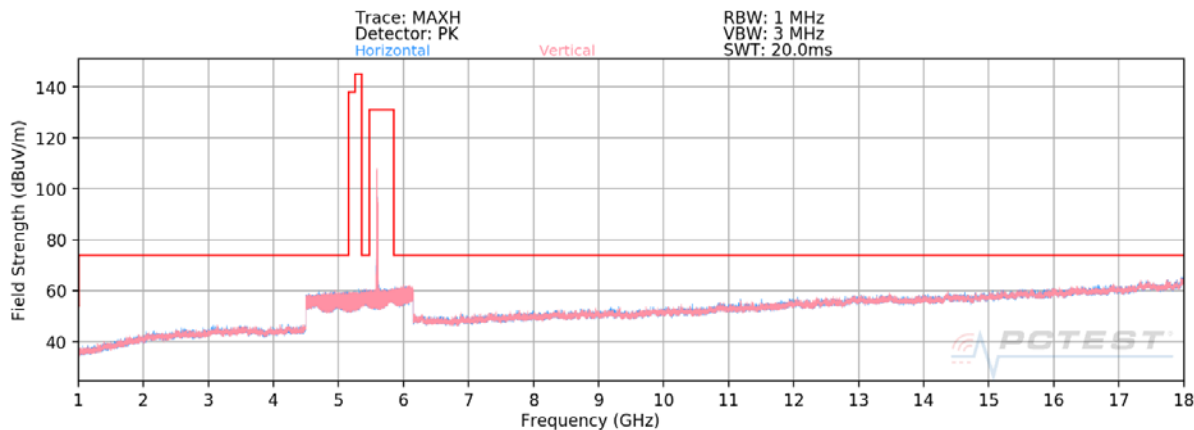
Plot 7-15. Radiated Spurious Plot above 1GHz SISO ANT2 (802.11ax – U2C Ch. 120 – 26 Tones)
