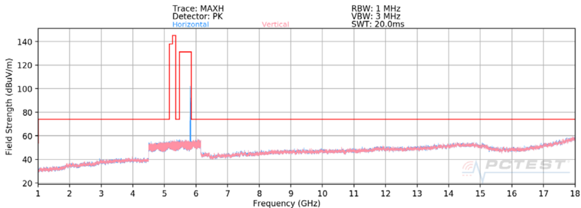
Plot 7-16. Radiated Spurious Plot above 1GHz SISO ANT2 (802.11ax – U3 Ch. 157 – 26 Tones)
