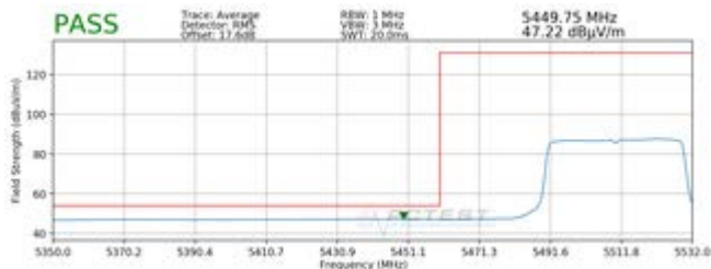
Plot 7-48. Radiated Lower Band Edge Plot SISO ANT1 (Average – UNII Band 2C – 484 Tones)
