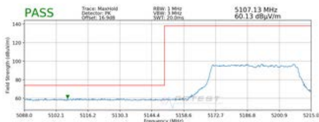
Plot 7-45. Radiated Lower Band Edge Plot SISO ANT1 (Peak - UNII Band 1 - 484 Tones)
