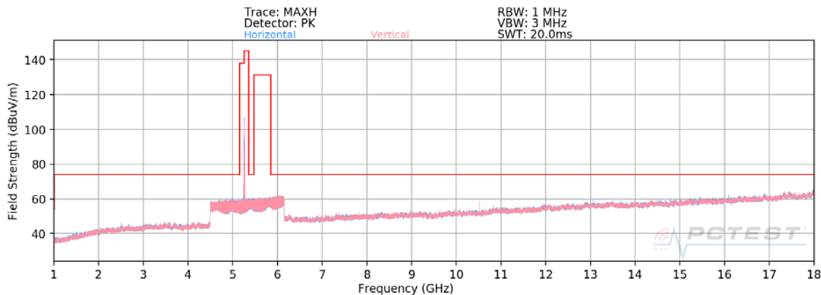
Plot 7-14. Radiated Spurious Plot above 1GHz SISO ANT2 (802.11ax – U2A Ch. 56 – 26 Tones)
