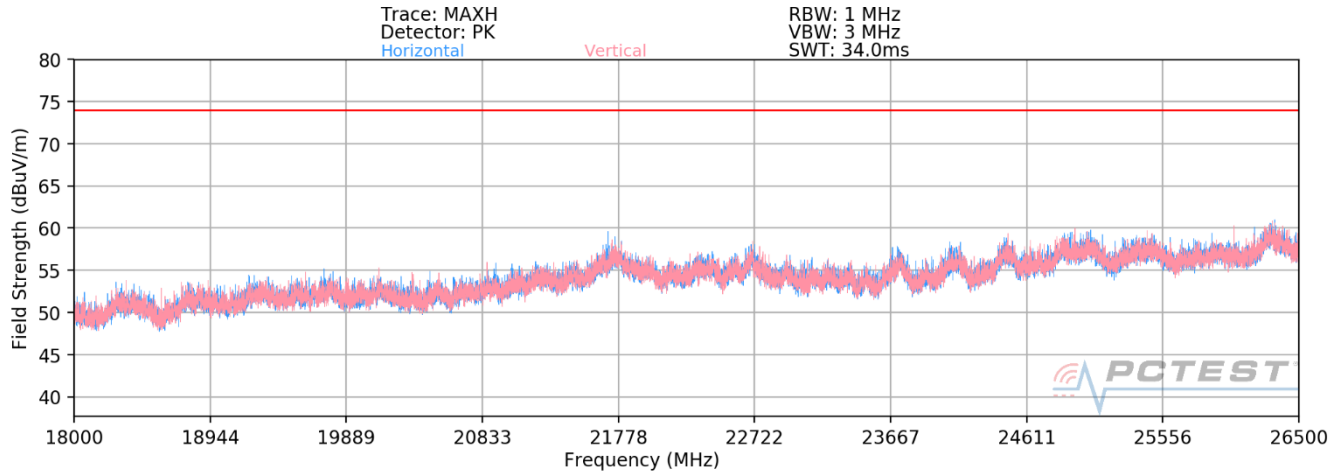
Plot 7-23. Radiated Spurious Plot 18GHz - 26.5GHz SISO ANT2 (802.11ax - 242 Tones)
