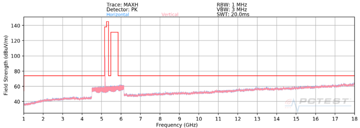
Plot 7-7. Radiated Spurious Plot above 1GHz SISO ANT1 (802.11ax – U1 Ch. 40 – 242 Tones)
