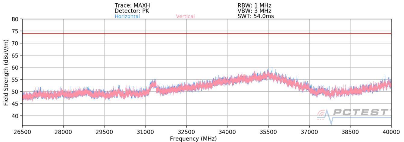
Plot 7-24. Radiated Spurious Plot 26.5GHz - 40GHz SISO ANT2 (802.11ax - 242 Tones)
