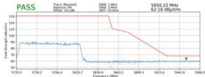
Plot 7-57. Radiated Upper Band Edge Plot SISO ANT1 (Peak – UNII Band 3 – 996 Tones)
