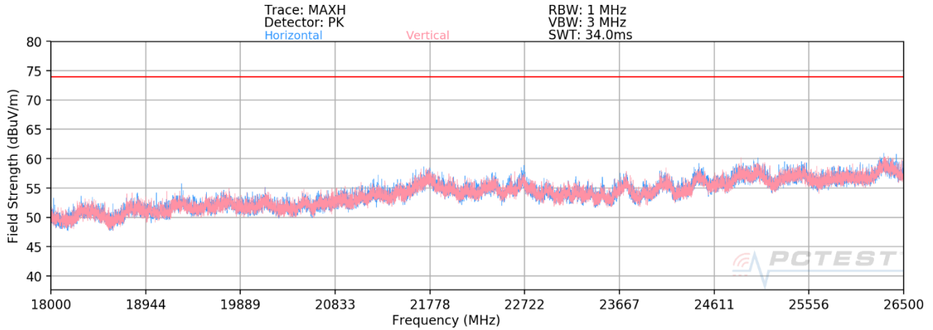
Plot 7-35. Radiated Spurious Plot 18GHz - 26.5GHz MIMO (802.11ax - 242 Tones)
