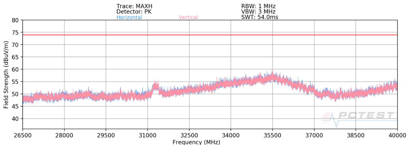
Plot 7-12. Radiated Spurious Plot 26.5GHz - 40GHz SISO ANT1 (802.11ax - 242 Tones)
