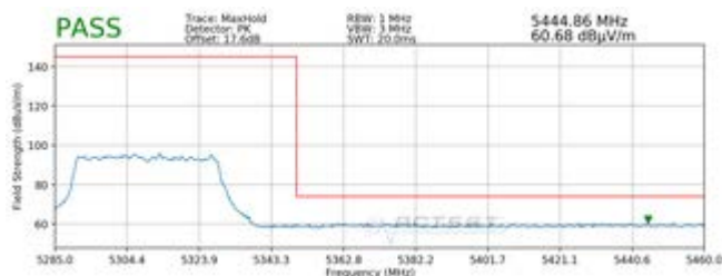
Plot 7-47. Radiated Upper Band Edge Plot SISO ANT1 (Peak - UNII Band 2A - 484 Tones)
