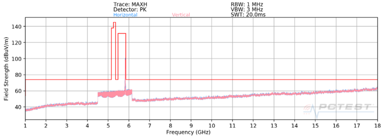
Plot 7-22. Radiated Spurious Plot above 1GHz SISO ANT2 (802.11ax – U3 Ch. 157 – 242 Tones)
