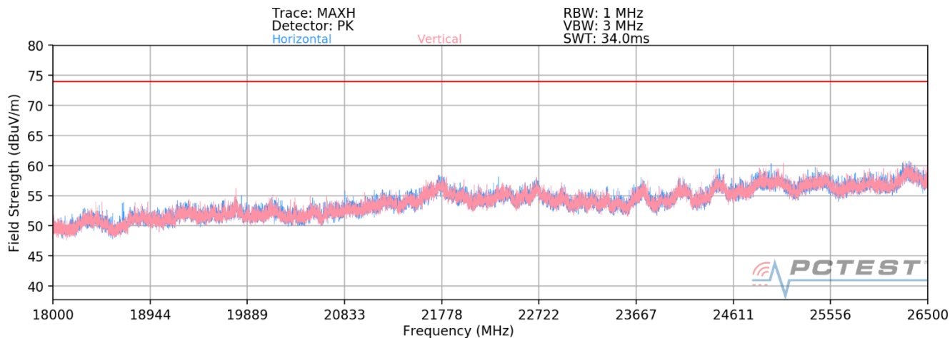
Plot 7-11. Radiated Spurious Plot 18GHz - 26.5GHz SISO ANT1 (802.11ax - 242 Tones)
