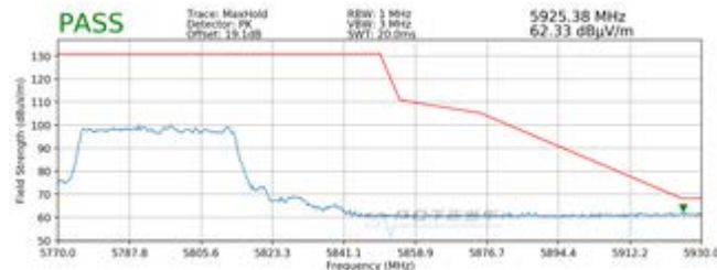
Plot 7-71. Radiated Upper Band Edge Plot SISO ANT2 (Peak - UNII Band 3 - 484 Tones)
