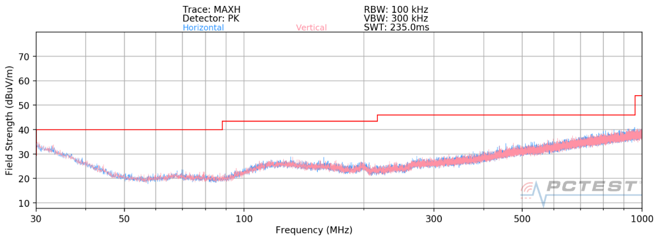
Plot 7-101. Radiated Spurious Plot below 1GHz MIMO (802.11ax – 242 Tones – U3 Ch. 157)
