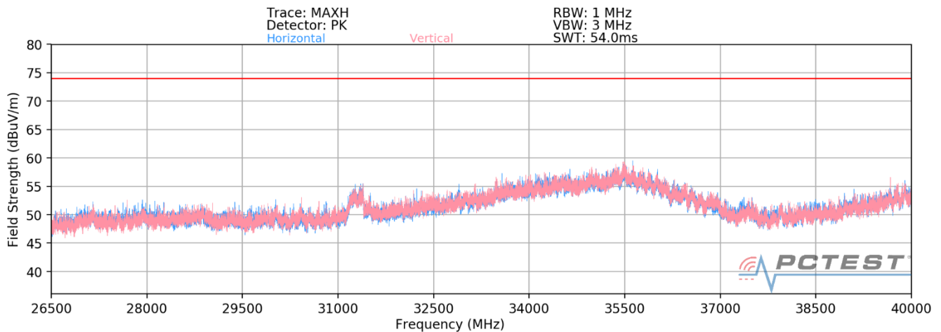
Plot 7-6. Radiated Spurious Plot 26.5GHz - 40GHz SISO ANT1 (802.11ax - 26 Tones)
