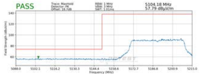
Plot 7-87. Radiated Lower Band Edge Plot MIMO (Peak - UNII Band 1 - 484 Tones)
