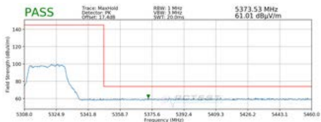
Plot 7-40. Radiated Upper Band Edge Plot SISO ANT1 (Peak - UNII Band 2A - 242 Tones)
