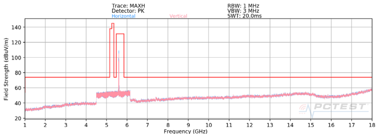
Plot 7-27. Radiated Spurious Plot above 1GHz MIMO (802.11ax – U2C Ch. 120 – 26 Tones)
