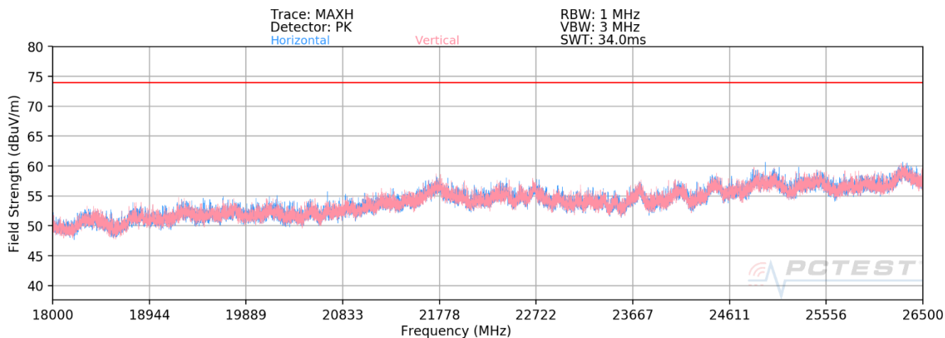
Plot 7-17. Radiated Spurious Plot 18GHz - 26.5GHz SISO ANT2 (802.11ax - 26 Tones)
