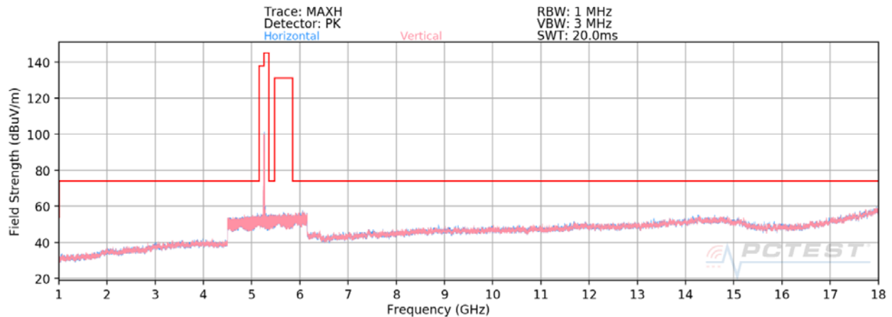
Plot 7-32. Radiated Spurious Plot above 1GHz MIMO (802.11ax – U2A Ch. 56 – 242 Tones)
