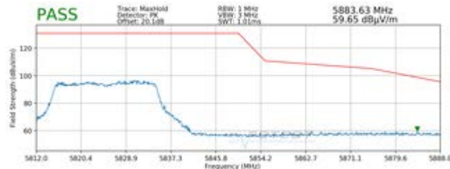
Plot 7-85. Radiated Upper Band Edge Plot MIMO (Peak - UNII Band 3 - 242 Tones)
