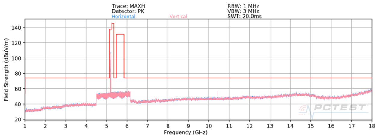
Plot 7-25. Radiated Spurious Plot above 1GHz MIMO (802.11ax – U1 Ch. 40 – 26 Tones)
