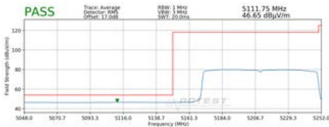
Plot 7-51. Radiated Lower Band Edge Plot SISO ANT1 (Average - UNII Band 1 - 996 Tones)
