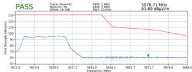
Plot 7-43. Radiated Upper Band Edge Plot SISO ANT1 (Peak - UNII Band 3 - 242 Tones)
