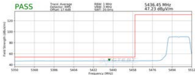
Plot 7-41. Radiated Lower Band Edge Plot SISO ANT1 (Average - UNII Band 2C - 242 Tones)
