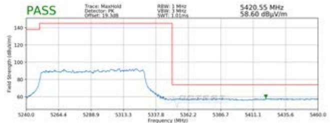
Plot 7-96. Radiated Upper Band Edge Plot MIMO (Peak – UNII Band 2A – 996 Tones)
