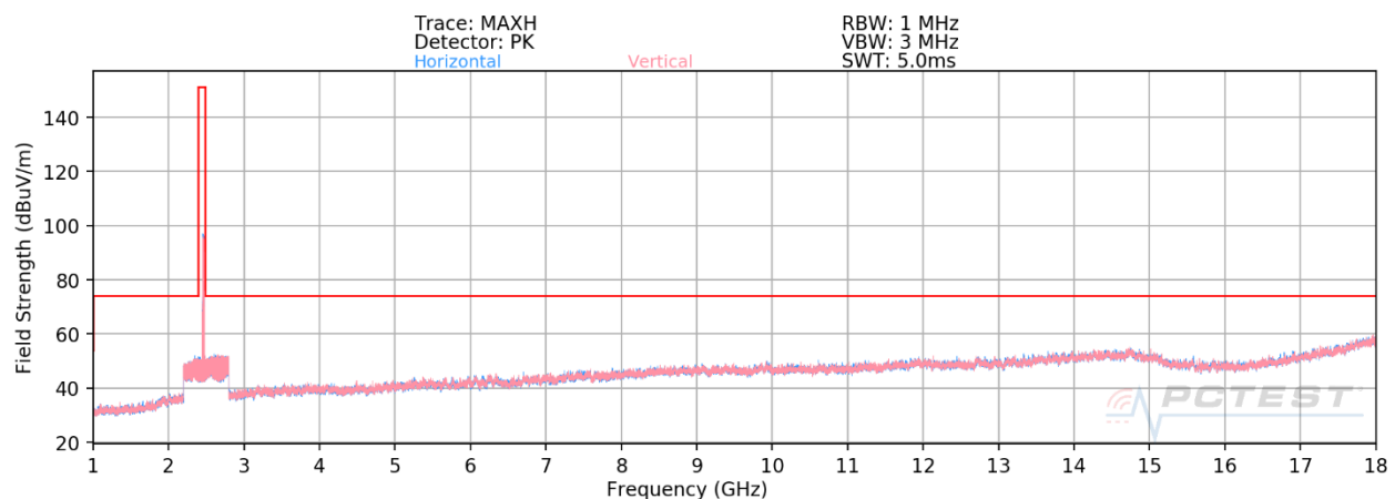
Plot 7-14. Radiated Spurious Plot above 1GHz SISO ANT2 (802.11ax OFDMA – 242 Tones – Ch. 11)
