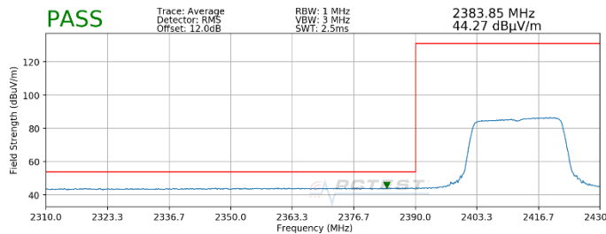
Plot 7-37. Radiated Restricted Lower Band Edge Measurement SISO ANT2 (Average – 242 Tones)
