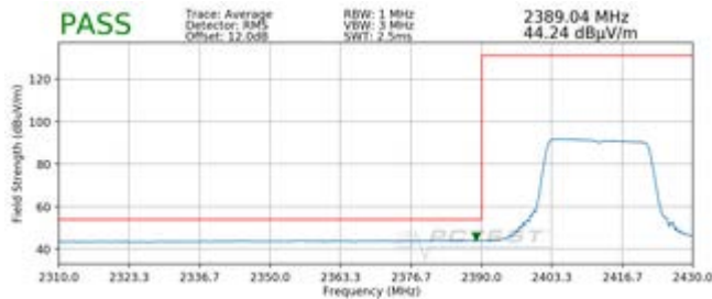
Plot 7-29. Radiated Restricted Lower Band Edge Measurement SISO ANT1 (Average – 242 Tones)
