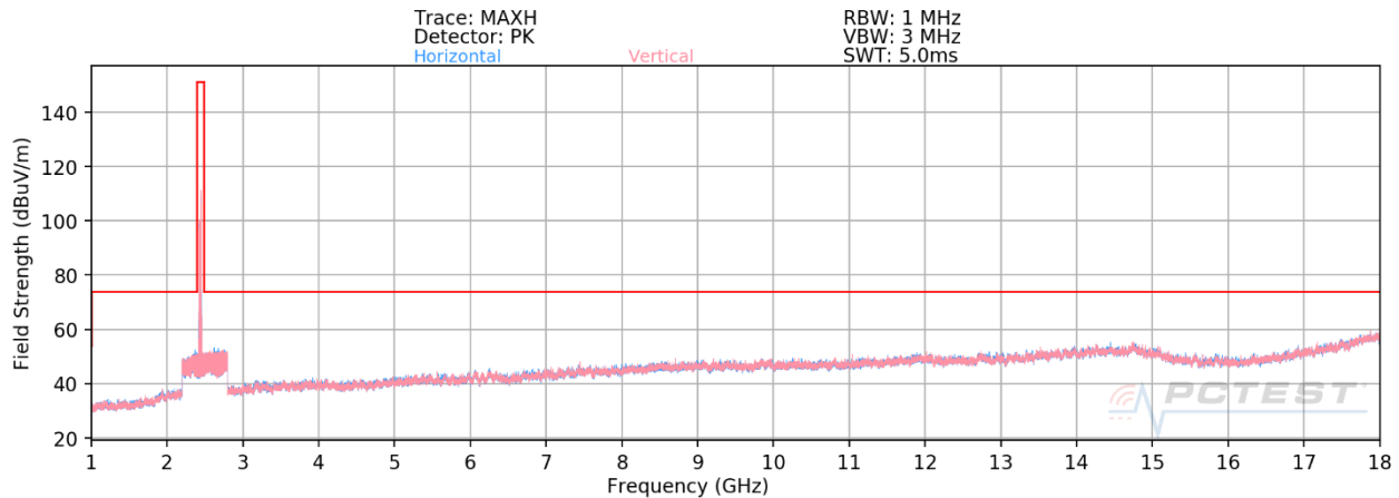
Plot 7-18. Radiated Spurious Plot above 1GHz MIMO (802.11ax OFDMA - 26 Tones - Ch. 6)
