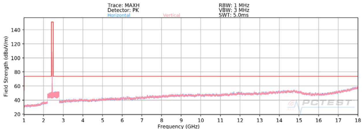
Plot 7-2. Radiated Spurious Plot above 1GHz SISO ANT1 (802.11ax OFDMA – 26 Tones – Ch. 6)
