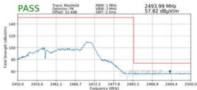
Plot 7-44. Radiated Restricted Upper Band Edge Measurement MIMO (Peak – 26 Tones)
