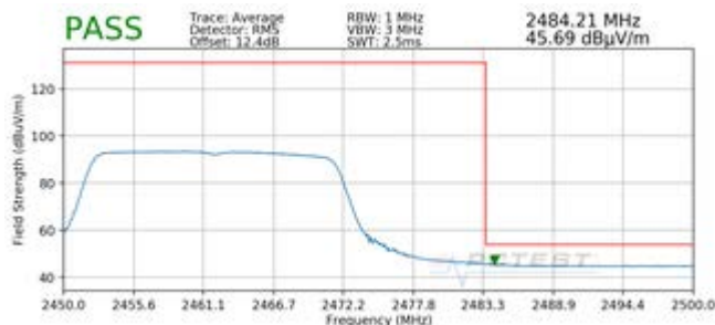
Plot 7-47. Radiated Restricted Upper Band Edge Measurement MIMO (Average – 242 Tones)
