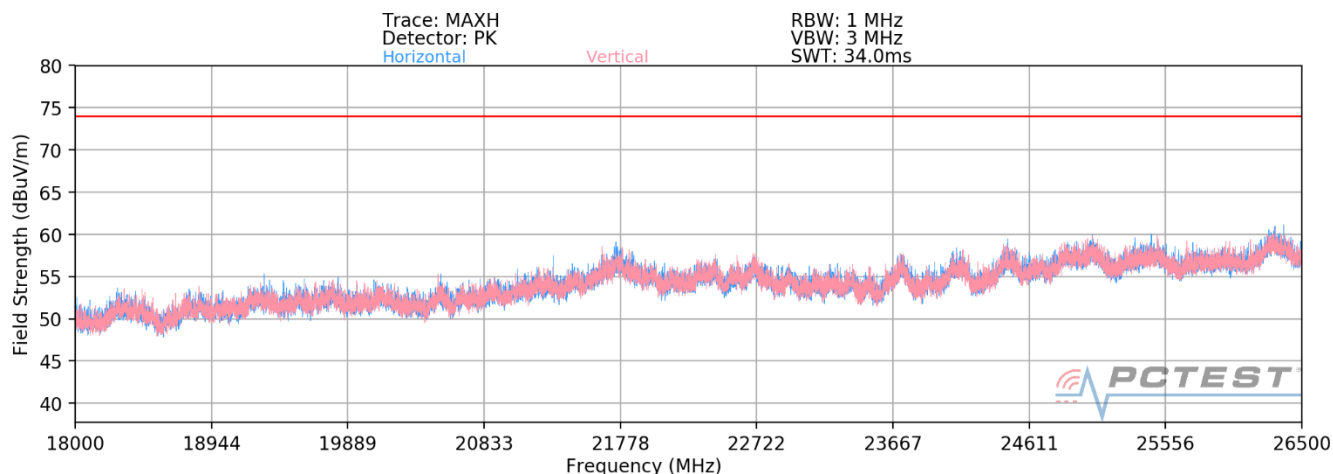
Plot 7-7. Radiated Spurious Plot above 18GHz SISO ANT1 (802.11ax OFDMA – 26 Tones)
