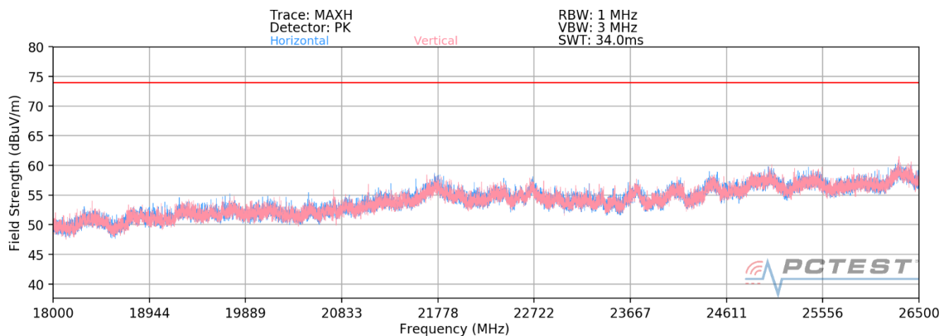
Plot 7-8. Radiated Spurious Plot above 18GHz SISO ANT1 (802.11ax OFDMA – 242 Tones)
