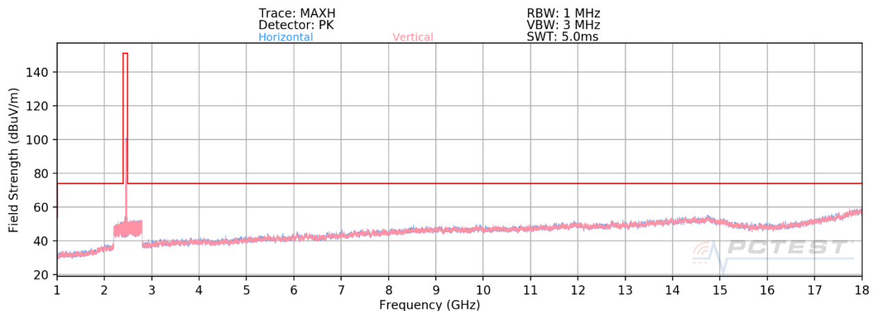
Plot 7-22. Radiated Spurious Plot above 1GHz MIMO (802.11ax OFDMA – 242 Tones – Ch. 11)
