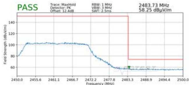
Plot 7-48. Radiated Restricted Upper Band Edge Measurement MIMO (Peak – 242 Tones)
