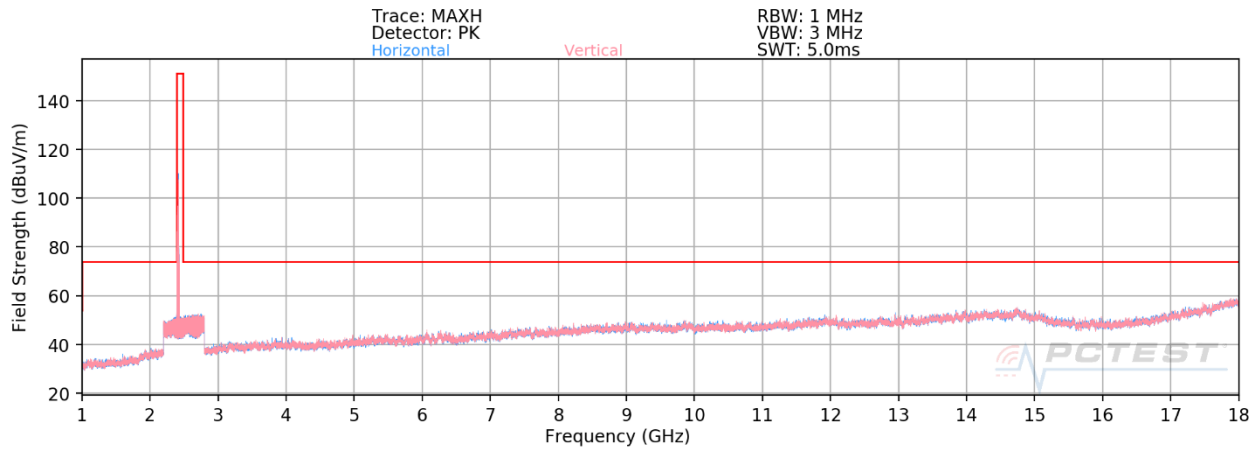
Plot 7-17. Radiated Spurious Plot above 1GHz MIMO (802.11ax OFDMA - 26 Tones - Ch. 1)
