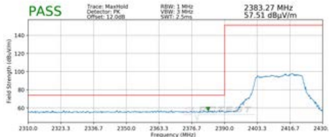
Plot 7-38. Radiated Restricted Lower Band Edge Measurement SISO ANT2 (Peak – 242 Tones)
