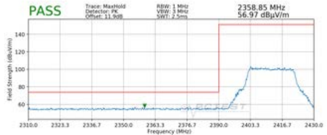
Plot 7-30. Radiated Restricted Lower Band Edge Measurement SISO ANT1 (Peak – 242 Tones)
