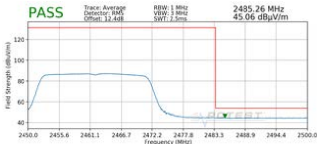
Plot 7-39. Radiated Restricted Upper Band Edge Measurement SISO ANT2 (Average – 242 Tones)
