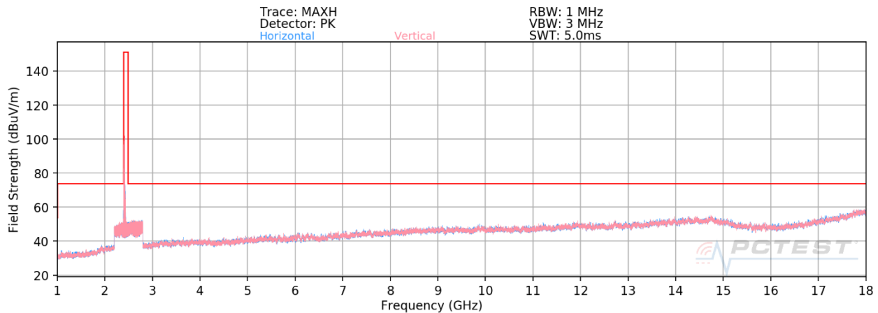
Plot 7-20. Radiated Spurious Plot above 1GHz MIMO (802.11ax OFDMA – 242 Tones – Ch. 1)
