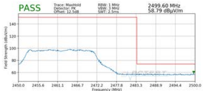
Plot 7-40. Radiated Restricted Upper Band Edge Measurement SISO ANT2 (Peak – 242 Tones)
