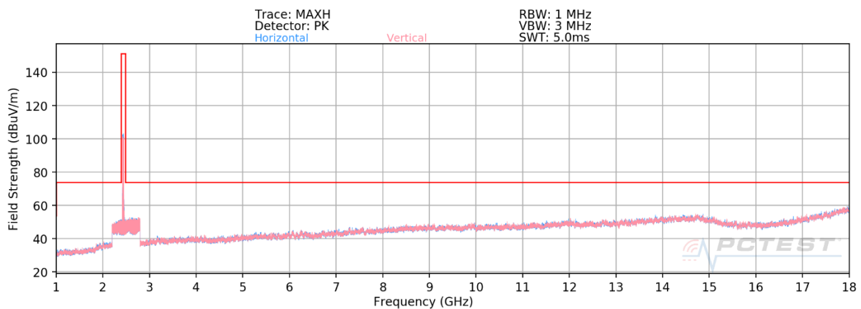
Plot 7-21. Radiated Spurious Plot above 1GHz MIMO (802.11ax OFDMA – 242 Tones – Ch. 6)
