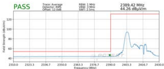
Plot 7-33. Radiated Restricted Lower Band Edge Measurement SISO ANT2 (Average – 26 Tones)
