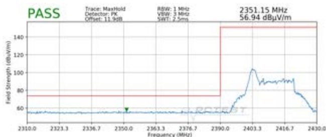
Plot 7-34. Radiated Restricted Lower Band Edge Measurement SISO ANT2 (Peak – 26 Tones)
