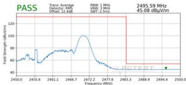
Plot 7-43. Radiated Restricted Upper Band Edge Measurement MIMO (Average – 26 Tones)
