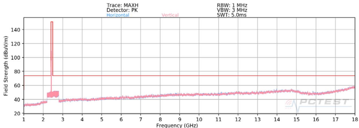
Plot 7-1. Radiated Spurious Plot above 1GHz SISO ANT1 (802.11ax OFDMA – 26 Tones – Ch. 1)
