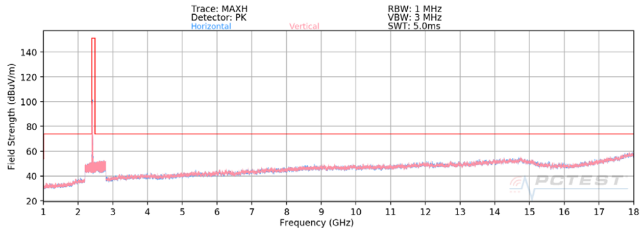
Plot 7-4. Radiated Spurious Plot above 1GHz SISO ANT1 (802.11ax OFDMA – 242 Tones – Ch. 1)
