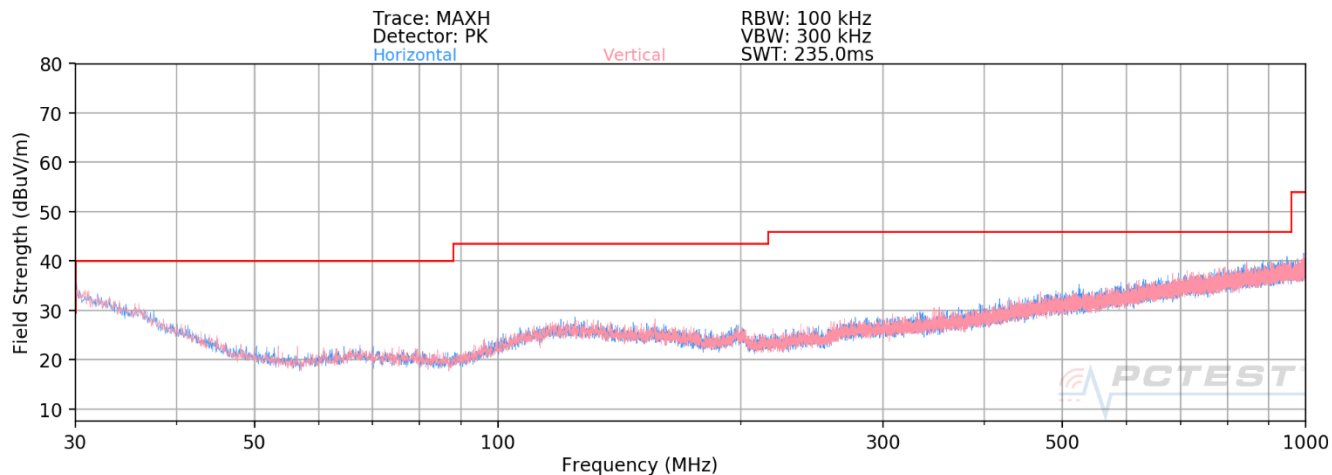
Plot 7-49. Radiated Spurious Plot below 1GHz MIMO (26 Tones)
