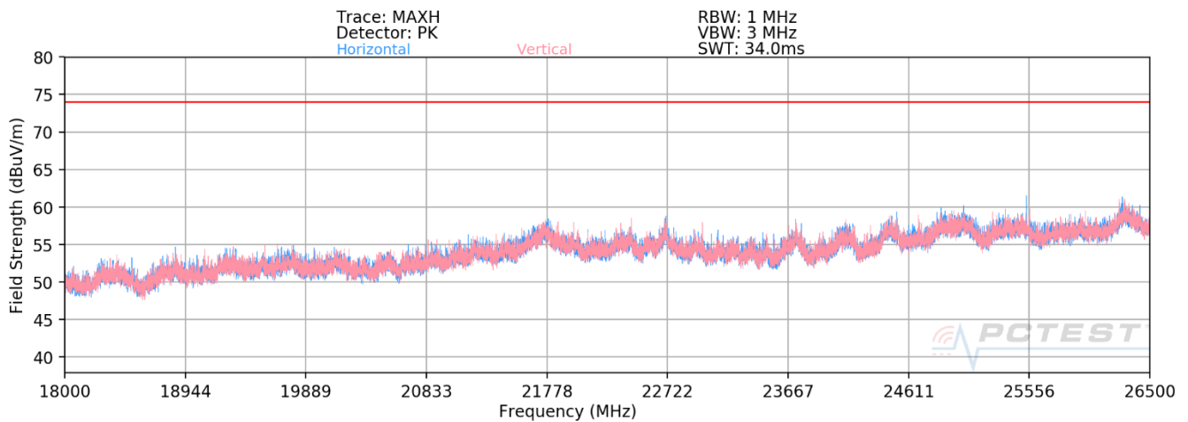
Plot 7-24. Radiated Spurious Plot above 18GHz MIMO (802.11ax OFDMA – 242 Tones)
