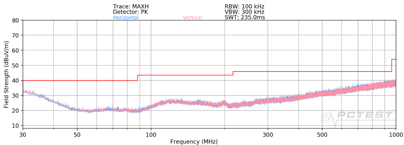
Plot 7-50. Radiated Spurious Plot below 1GHz MIMO (242 Tones)
