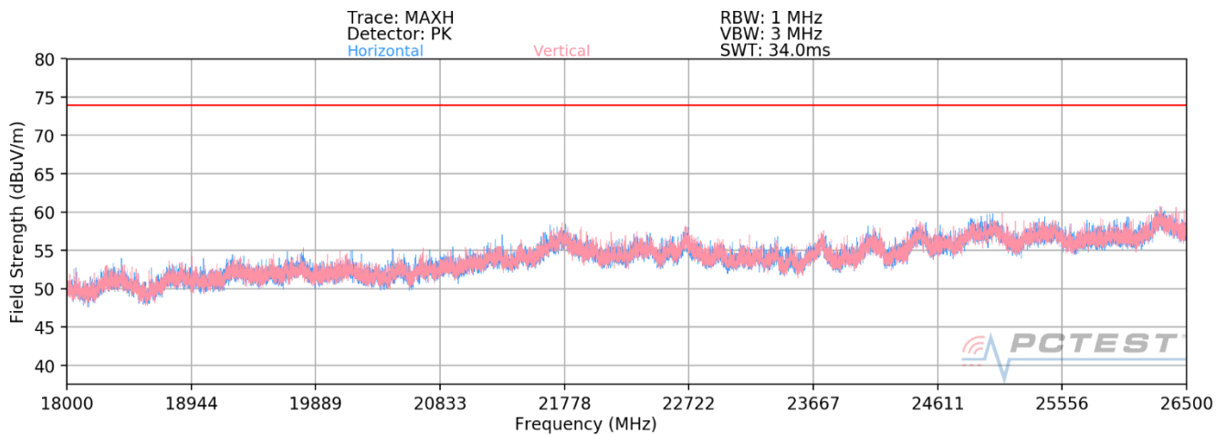
Plot 7-16. Radiated Spurious Plot above 18GHz SISO ANT2 (802.11ax OFDMA – 242 Tones)
