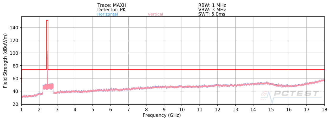
Plot 7-11. Radiated Spurious Plot above 1GHz SISO ANT2 (802.11ax OFDMA – 26 Tones – Ch. 11)
