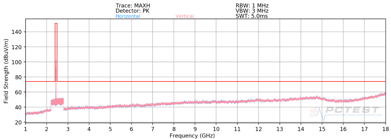
Plot 7-10. Radiated Spurious Plot above 1GHz SISO ANT2 (802.11ax OFDMA – 26 Tones – Ch. 6)
