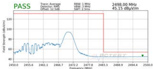
Plot 7-35. Radiated Restricted Upper Band Edge Measurement SISO ANT2 (Average – 26 Tones)
