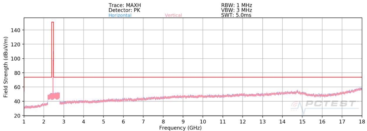
Plot 7-19. Radiated Spurious Plot above 1GHz MIMO (802.11ax OFDMA - 26 Tones - Ch. 11)
