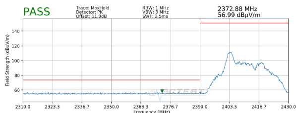
Plot 7-42. Radiated Restricted Lower Band Edge Measurement MIMO (Peak – 26 Tones)
