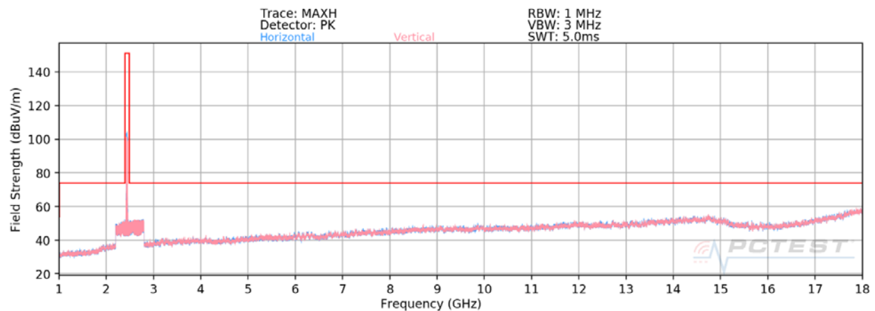
Plot 7-5. Radiated Spurious Plot above 1GHz SISO ANT1 (802.11ax OFDMA – 242 Tones – Ch. 6)
