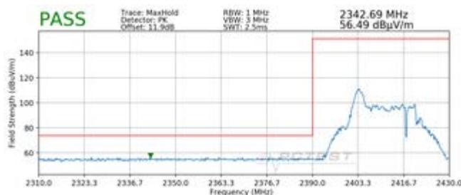
Plot 7-26. Radiated Restricted Lower Band Edge Measurement SISO ANT1 (Peak – 26 Tones)
