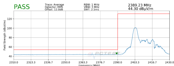
Plot 7-41. Radiated Restricted Lower Band Edge Measurement MIMO (Average – 26 Tones)
