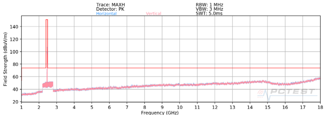
Plot 7-3. Radiated Spurious Plot above 1GHz SISO ANT1 (802.11ax OFDMA – 26 Tones – Ch. 11)
