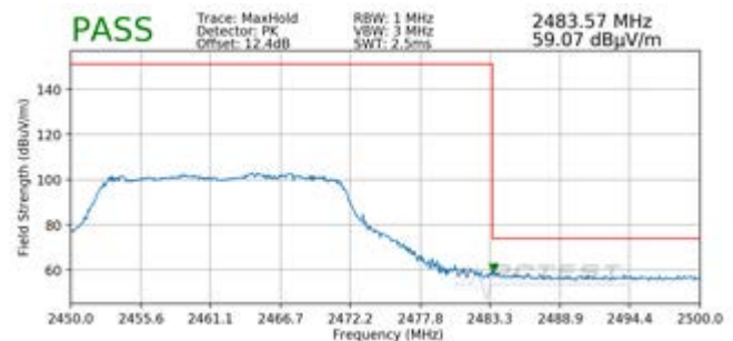
Plot 7-32. Radiated Restricted Upper Band Edge Measurement SISO ANT1 (Peak – 242 Tones)
