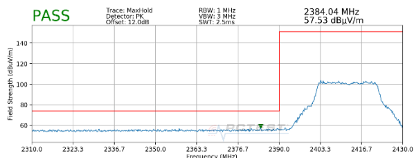
Plot 7-46. Radiated Restricted Lower Band Edge Measurement MIMO (Peak – 242 Tones)
