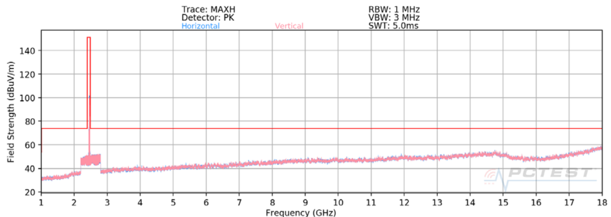
Plot 7-6. Radiated Spurious Plot above 1GHz SISO ANT1 (802.11ax OFDMA – 242 Tones – Ch. 11)
