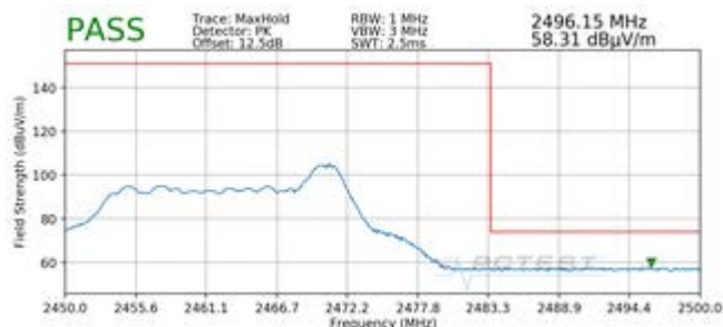
Plot 7-36. Radiated Restricted Upper Band Edge Measurement SISO ANT2 (Peak – 26 Tones)
