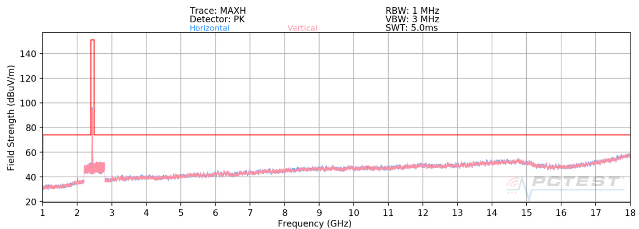
Plot 7-13. Radiated Spurious Plot above 1GHz SISO ANT2 (802.11ax OFDMA – 242 Tones – Ch. 6)
