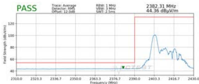
Plot 7-25. Radiated Restricted Lower Band Edge Measurement SISO ANT1 (Average – 26 Tones)
