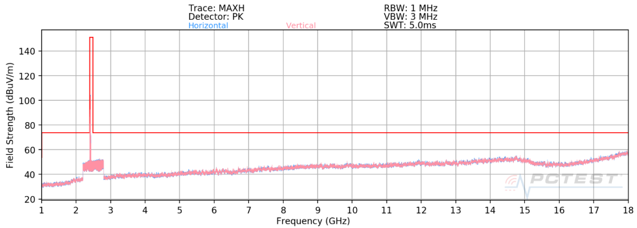
Plot 7-9. Radiated Spurious Plot above 1GHz SISO ANT2 (802.11ax OFDMA – 26 Tones – Ch. 1)
