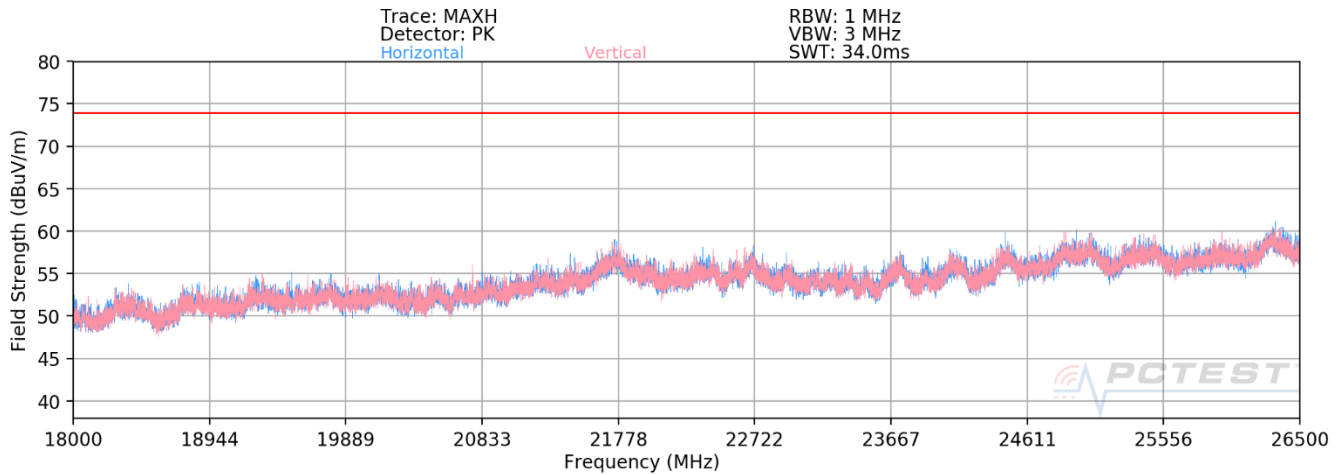
Plot 7-23. Radiated Spurious Plot above 18GHz MIMO (802.11ax OFDMA – 26 Tones)
