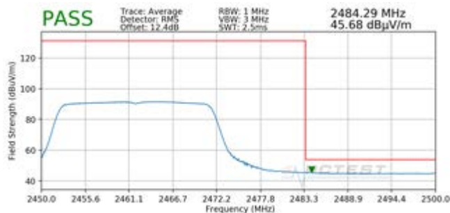
Plot 7-31. Radiated Restricted Upper Band Edge Measurement SISO ANT1 (Average – 242 Tones)
