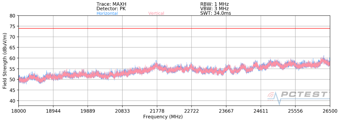
Plot 7-15. Radiated Spurious Plot above 18GHz SISO ANT2 (802.11ax OFDMA – 26 Tones)
