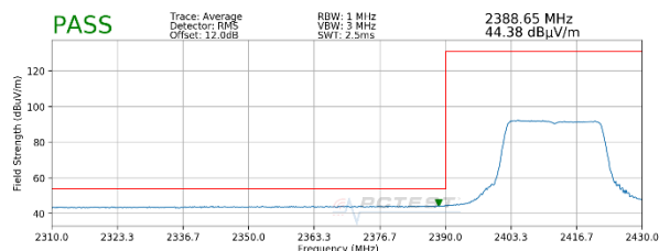
Plot 7-45. Radiated Restricted Lower Band Edge Measurement MIMO (Average – 242 Tones)
