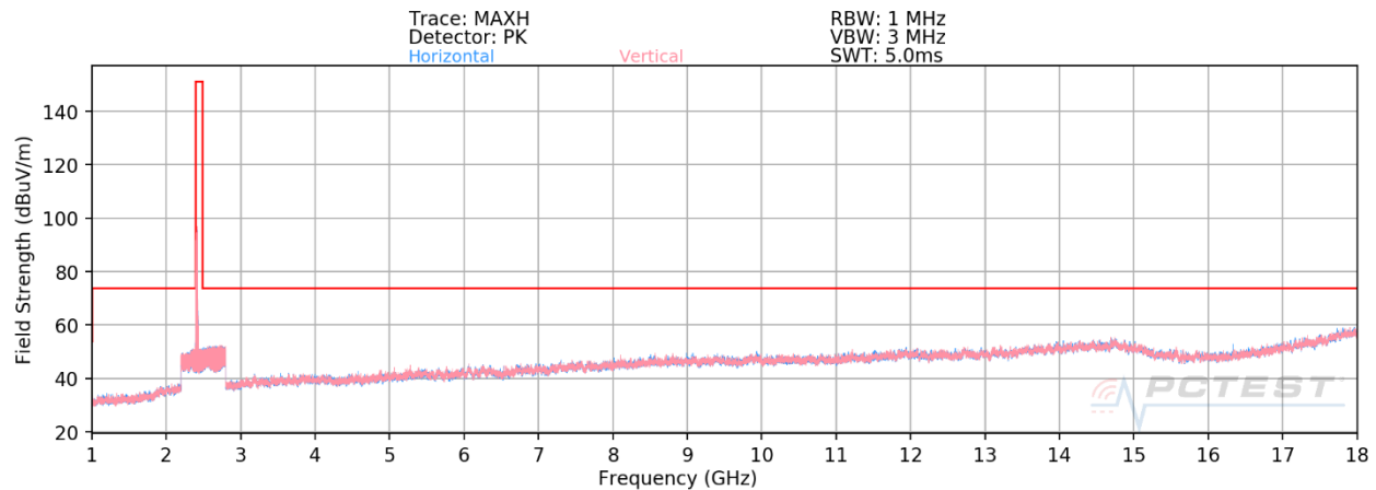
Plot 7-12. Radiated Spurious Plot above 1GHz SISO ANT2 (802.11ax OFDMA – 242 Tones – Ch. 1)
