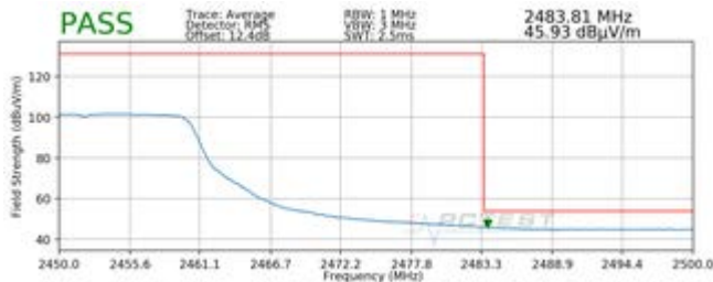
Plot 7-17. Radiated Restricted Upper Band Edge Measurement SISO ANT1 (Average)
