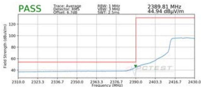
Plot 7-23. Radiated Restricted Lower Band Edge Measurement SISO ANT2 (Average)
