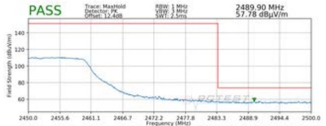
Plot 7-18. Radiated Restricted Upper Band Edge Measurement SISO ANT1 (Peak)
