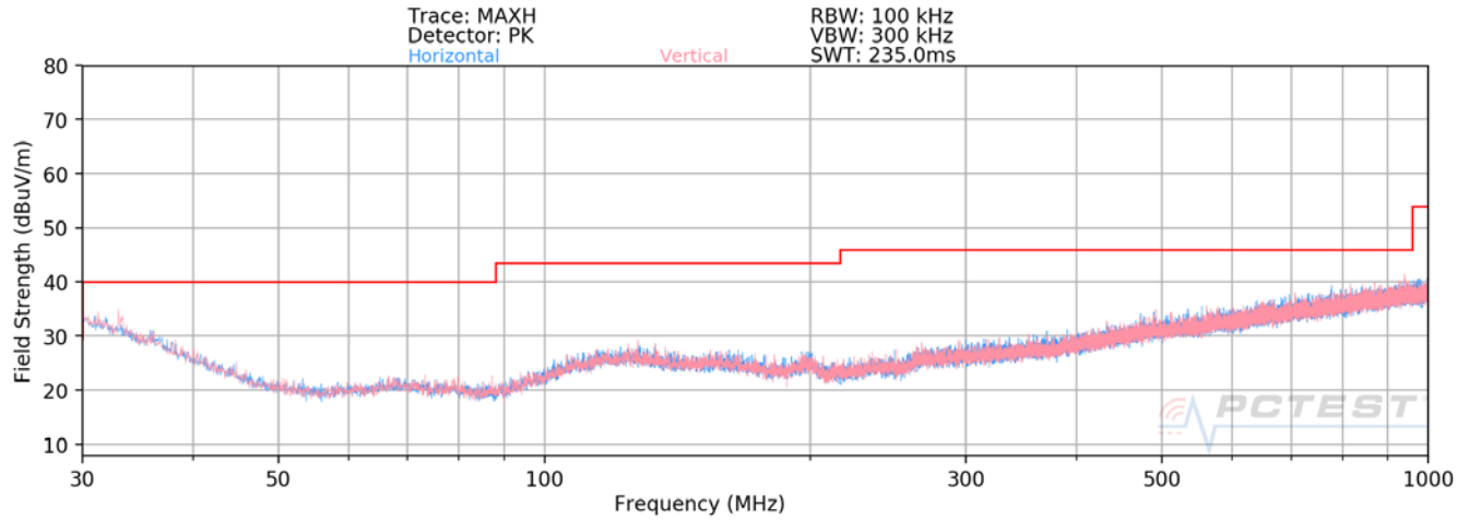
Plot 7-39. Radiated Spurious Plot below 1GHz MIMO
