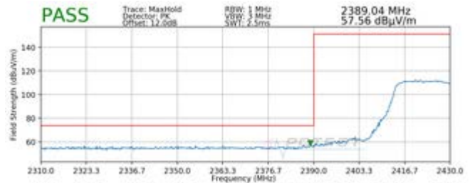
Plot 7-16. Radiated Restricted Lower Band Edge Measurement SISO ANT1 (Peak)
