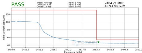
Plot 7-33. Radiated Restricted Upper Band Edge Measurement MIMO (Average)
