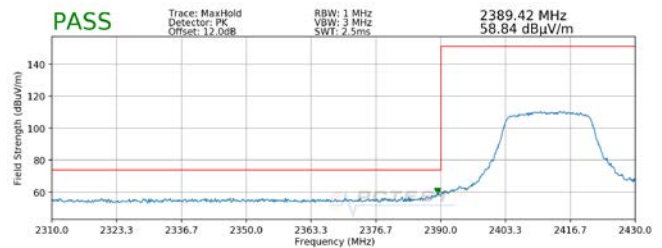
Plot 7-30. Radiated Restricted Lower Band Edge Measurement MIMO (Peak)
