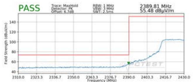
Plot 7-24. Radiated Restricted Lower Band Edge Measurement SISO ANT2 (Peak)
