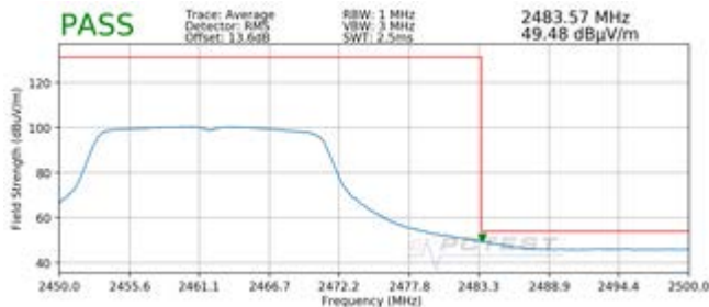
Plot 7-35. Radiated Restricted Upper Band Edge Measurement MIMO (Average)
