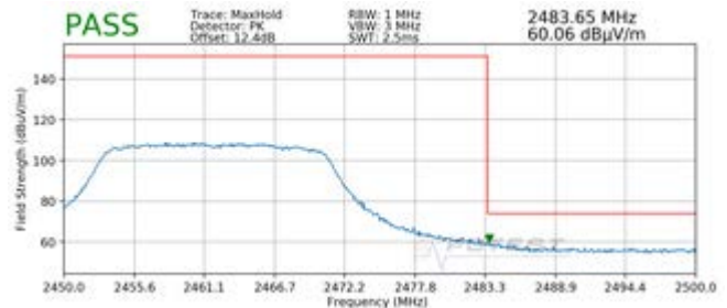
Plot 7-36. Radiated Restricted Upper Band Edge Measurement MIMO (Peak)
