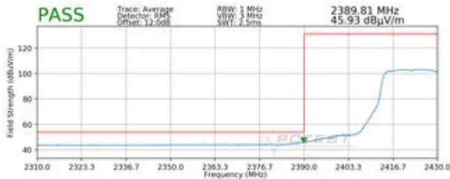
Plot 7-15. Radiated Restricted Lower Band Edge Measurement SISO ANT1 (Average)
