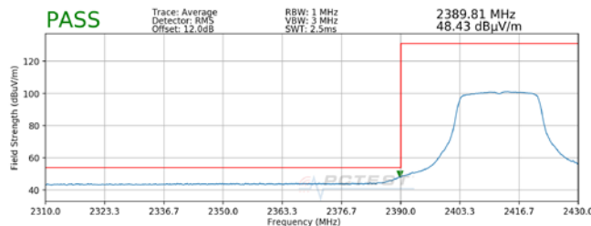
Plot 7-29. Radiated Restricted Lower Band Edge Measurement MIMO (Average)
