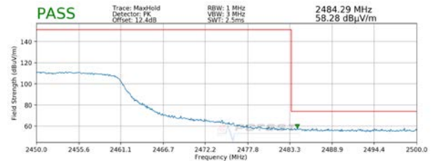
Plot 7-34. Radiated Restricted Upper Band Edge Measurement MIMO (Peak)
