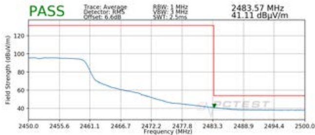
Plot 7-25. Radiated Restricted Upper Band Edge Measurement SISO ANT2 (Average)
