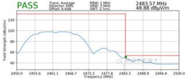
Plot 7-27. Radiated Restricted Upper Band Edge Measurement SISO ANT2 (Average)
