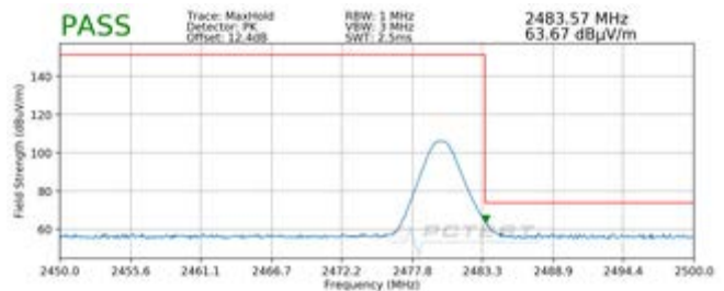
Plot 7-6. Radiated Restricted Upper Band Edge Measurement (Peak)
