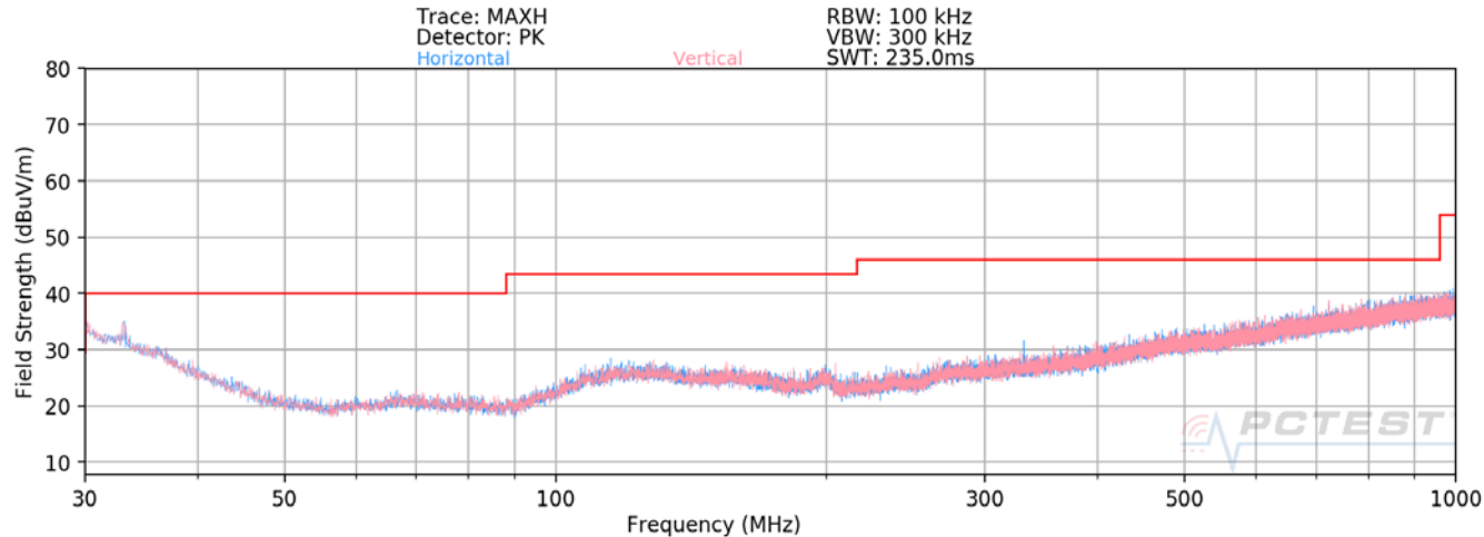
Plot 7-9. Radiated Spurious Plot below 1GHz
