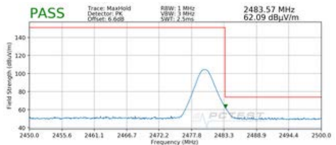
Plot 7-8. Radiated Restricted Upper Band Edge Measurement (Peak) with WCP+DD
