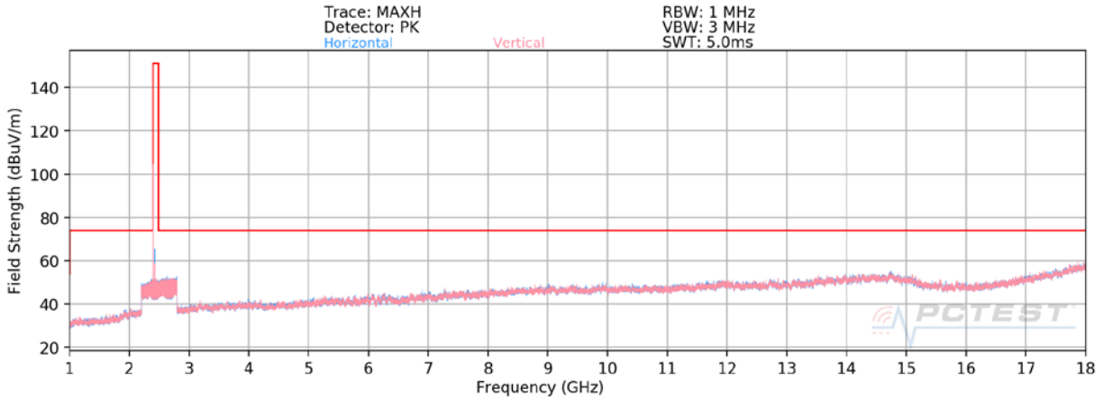
Plot 7-1. Radiated Spurious Plot above 1GHz (BT- Ch. 0)
