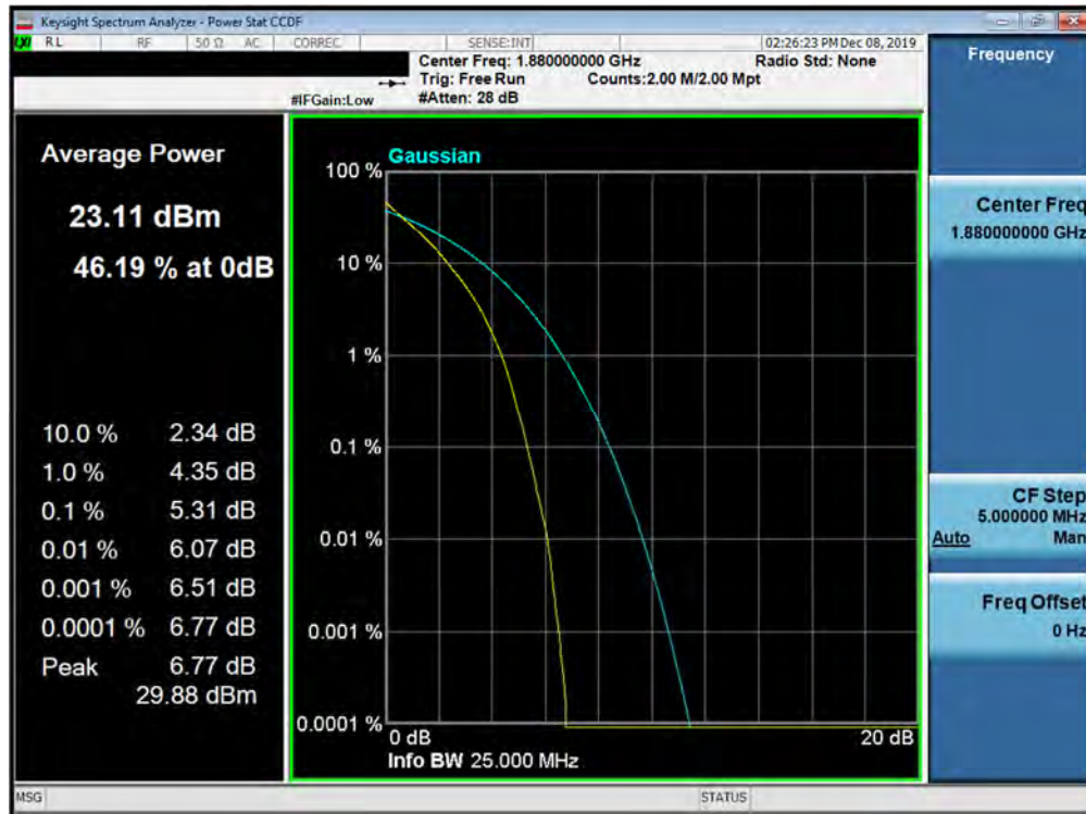
Plot 7-431. PAR Plot (Band 2 - 20.0MHz QPSK - Full RB Configuration)
