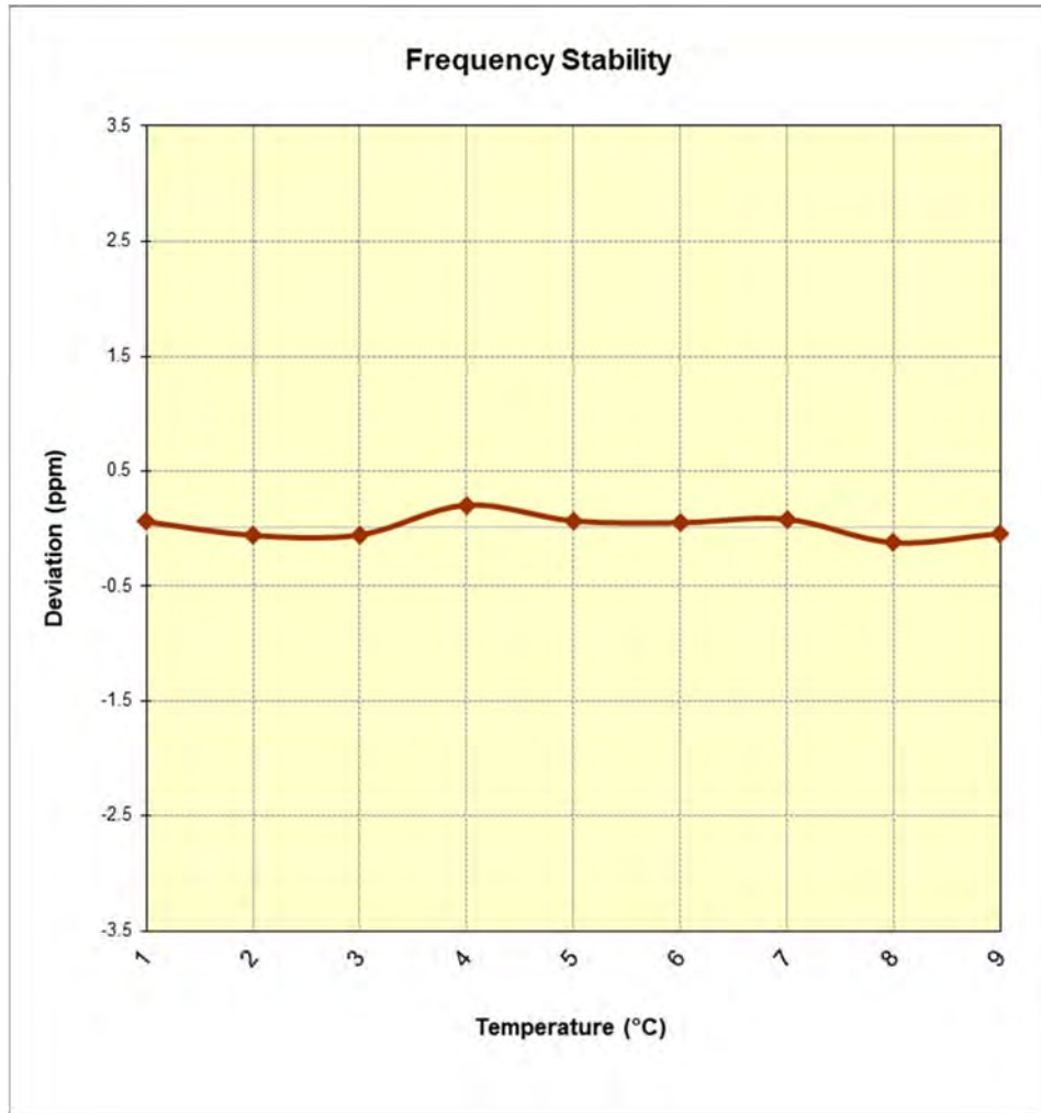
Figure 7-18. Frequency Stability Graph (5G NR n66)
