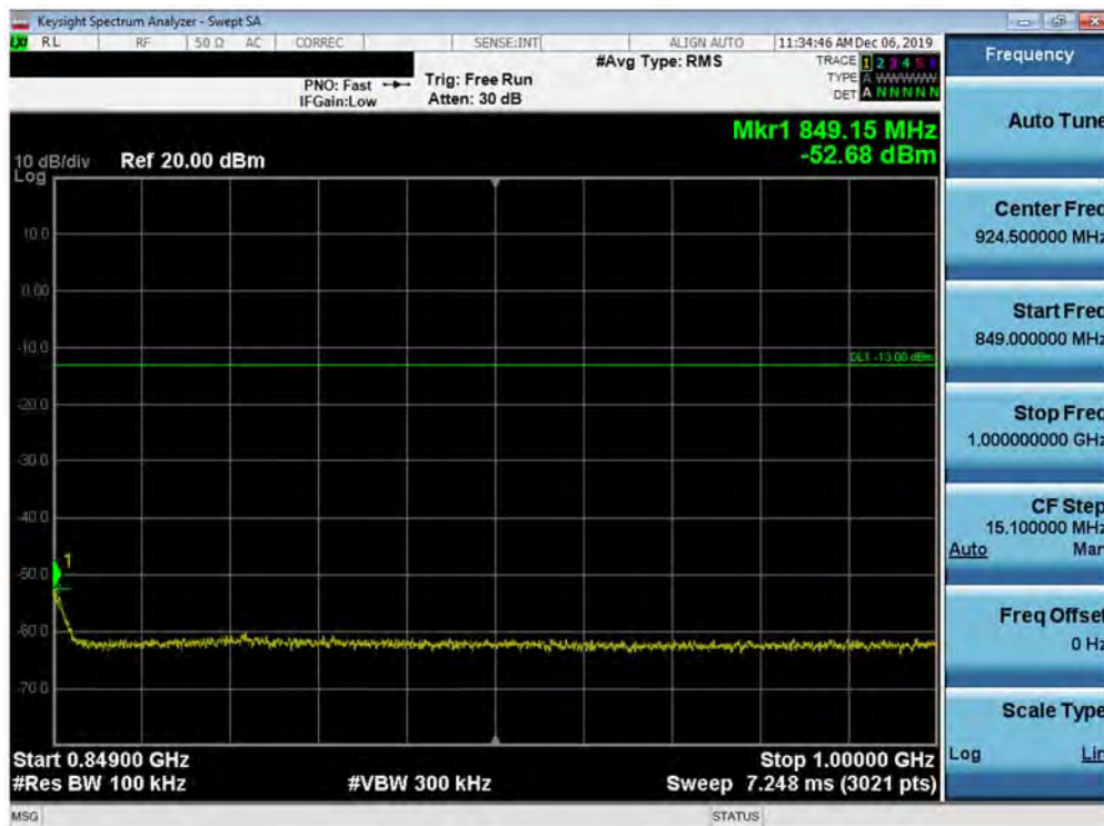
Plot 7-457. Conducted Spurious Plot (Band 5 - 10.0MHz QPSK - Left Carrier 1/49 Right Carrier 1/0 - Mid Channel)
