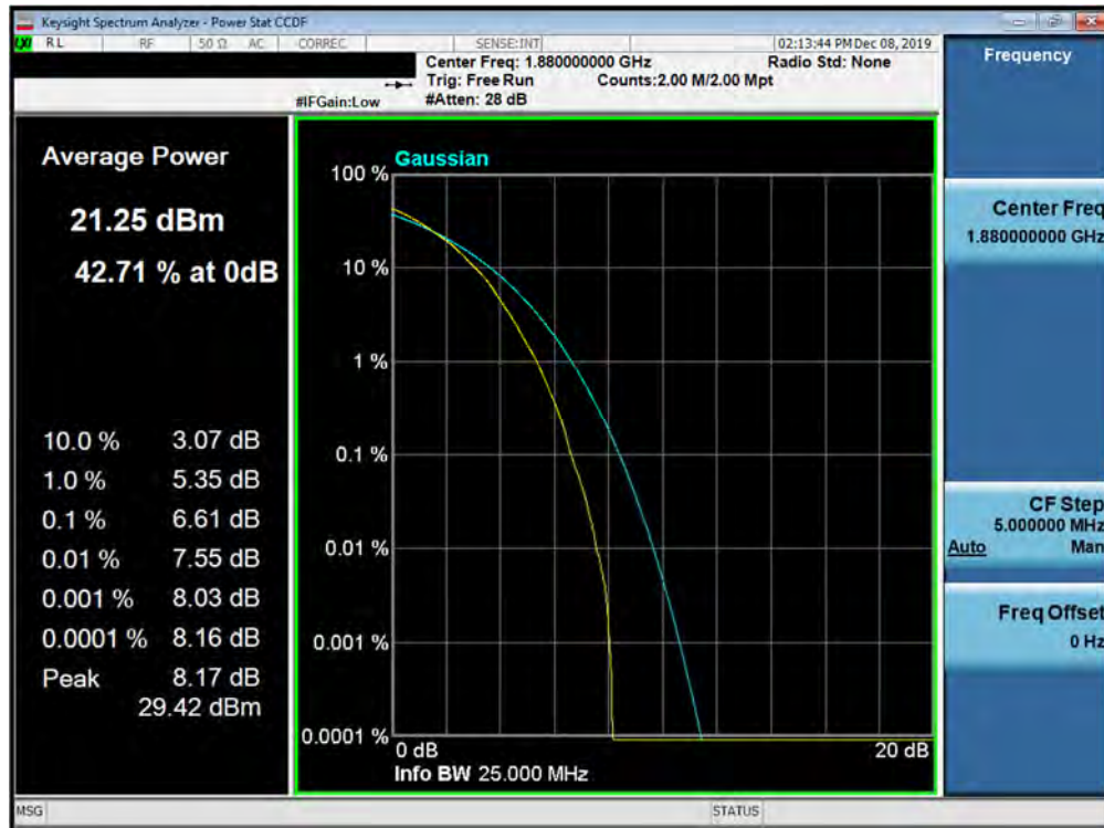
Plot 7-429. PAR Plot (Band 2 - 15.0MHz 64-QAM - Full RB Configuration)
