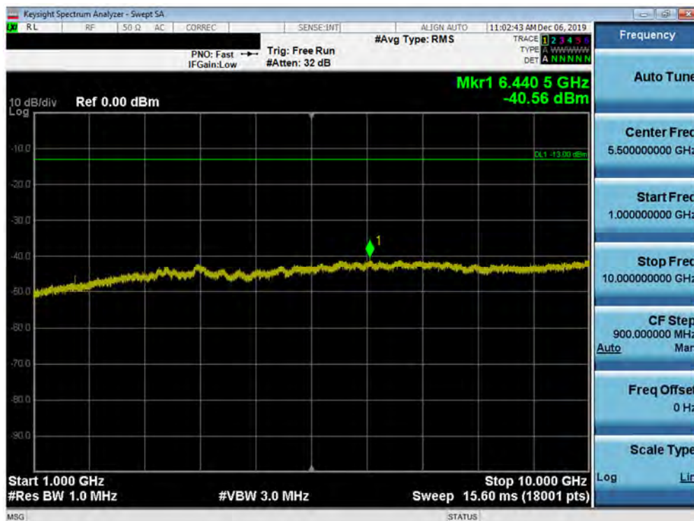
Plot 7-454. Conducted Spurious Plot (Band 5 - 10.0MHz QPSK - Left Carrier 1/49 Right Carrier 1/0 - Low Channel)
