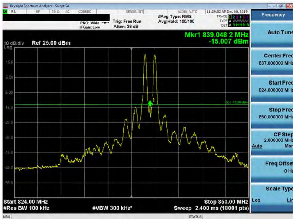
Plot 7-460. Conducted Spurious Plot (Band 5 - 10.0MHz QPSK - Left Carrier 1/49 Right Carrier 1/0 - High Channel)
