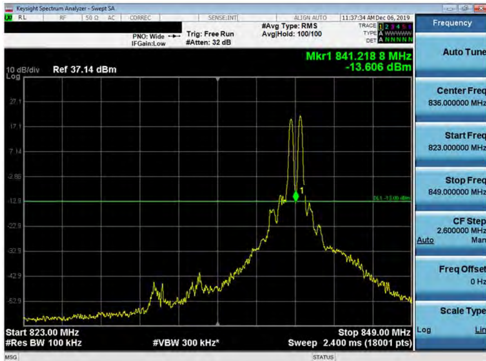
Plot 7-456. Conducted Spurious Plot (Band 5 - 10.0MHz QPSK - Left Carrier 1/49 Right Carrier 1/0 - Mid Channel)
