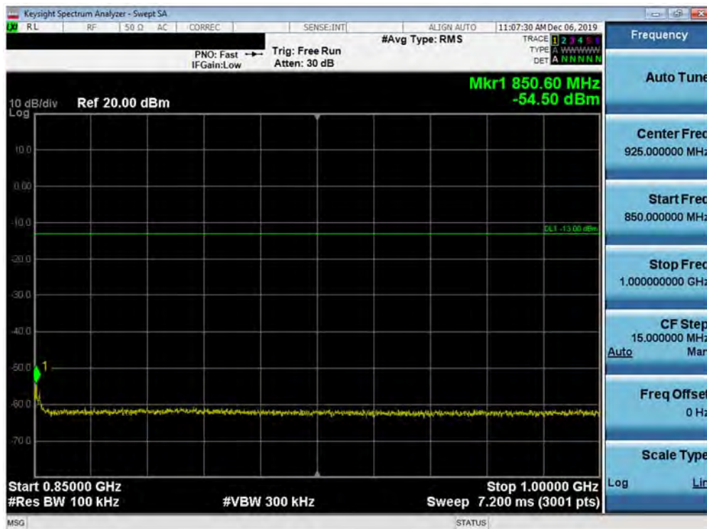
Plot 7-461. Conducted Spurious Plot (Band 5 - 10.0MHz QPSK - Left Carrier 1/49 Right Carrier 1/0 - High Channel)
