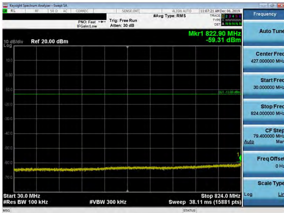
Plot 7-459. Conducted Spurious Plot (Band 5 - 10.0MHz QPSK - Left Carrier 1/49 Right Carrier 1/0 - High Channel)
