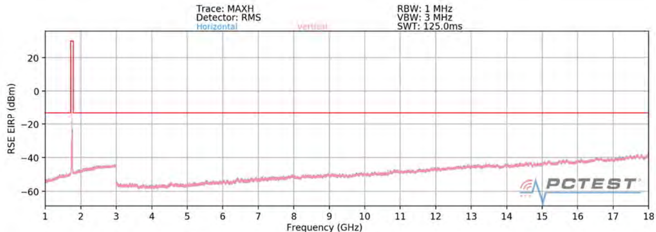
Plot 7-474. Radiated Spurious Plot above 1GHz (5G NR n66 + B66)
