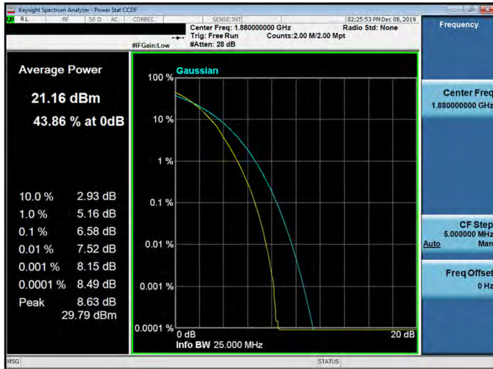
Plot 7-433. PAR Plot (Band 2 - 20.0MHz 64-QAM - Full RB Configuration)
