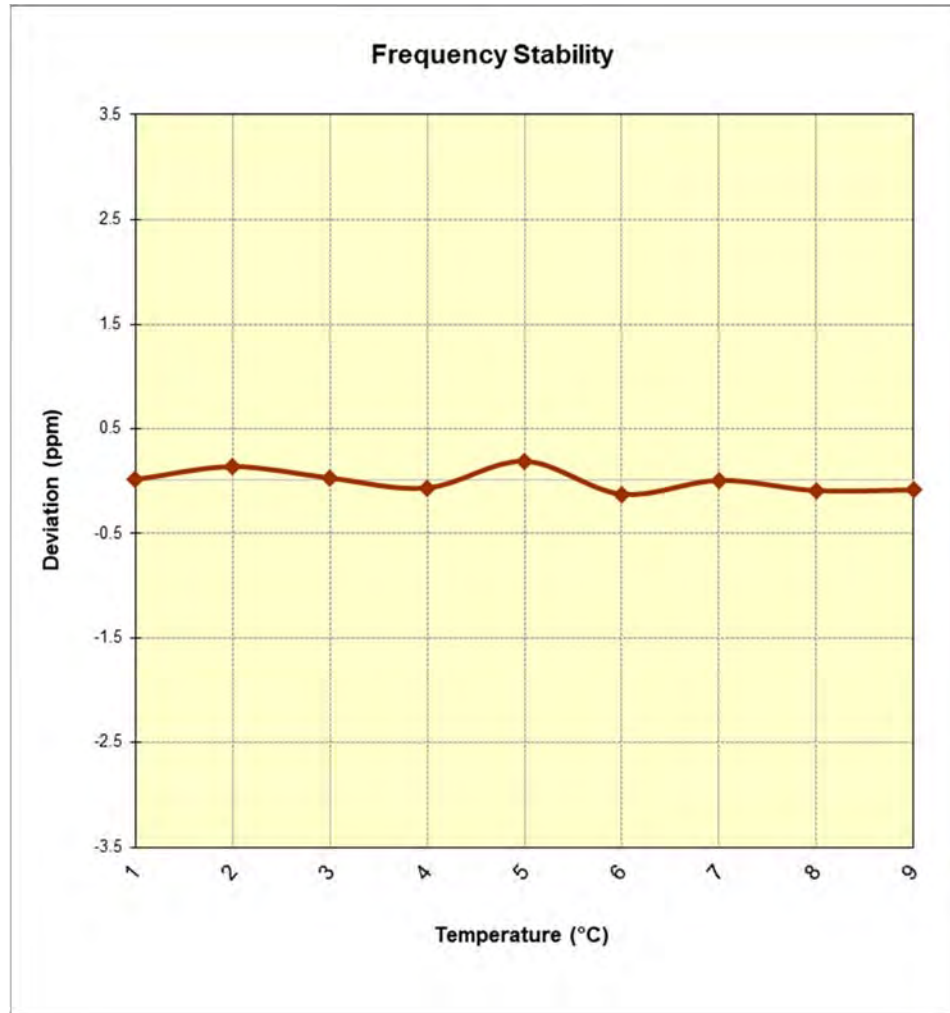
Figure 7-19. Frequency Stability Graph (5G NR n2)
