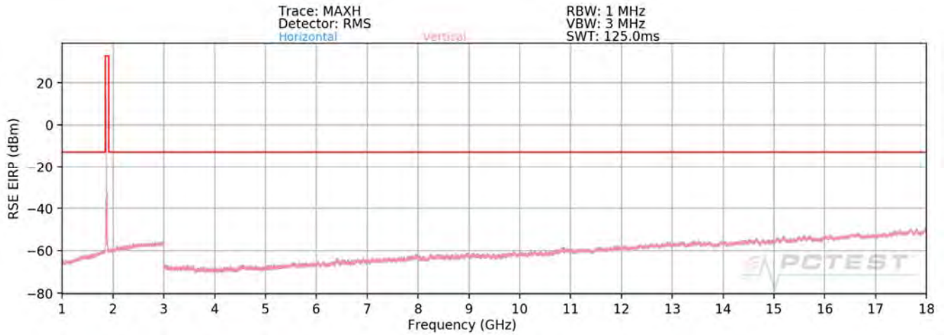
Plot 7-473. Radiated Spurious Plot above 1GHz (5G NR n5 + B2)
