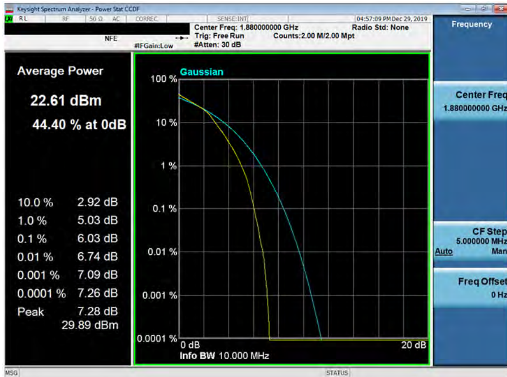
Plot 7-424. PAR Plot (Band 2 - 10.0MHz 16-QAM - Full RB Configuration)
