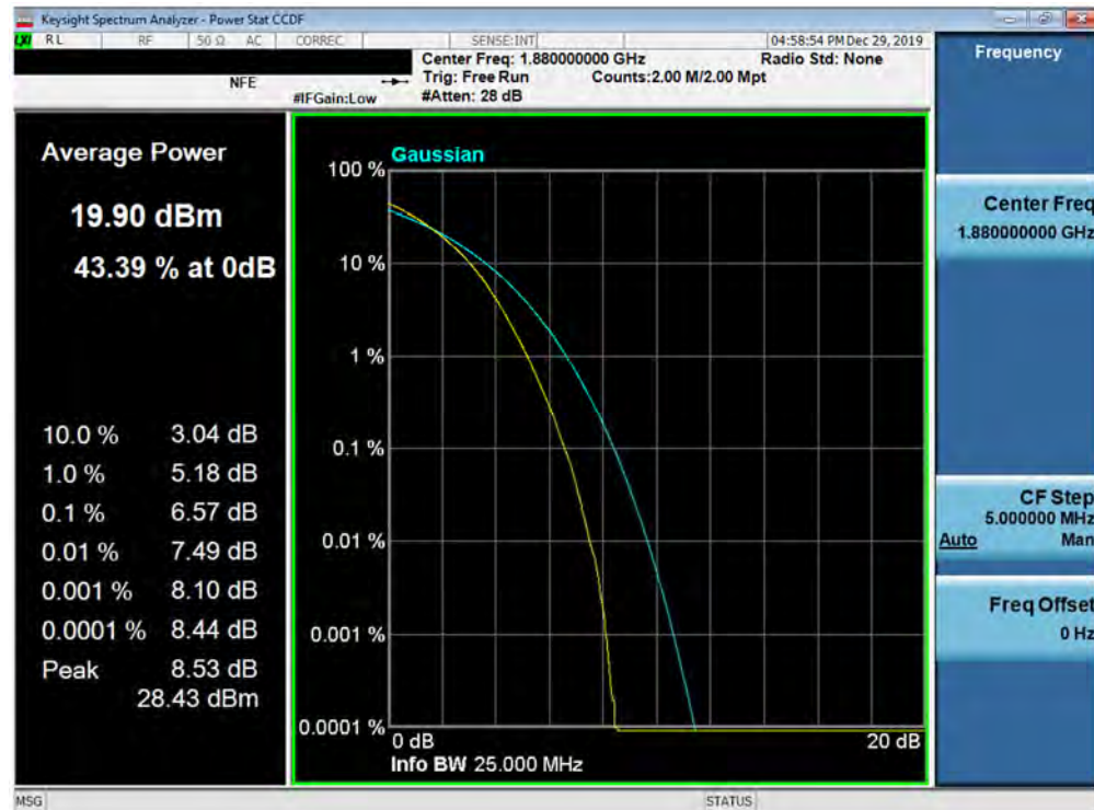
Plot 7-434. PAR Plot (Band 2 - 20.0MHz 256-QAM - Full RB Configuration)
