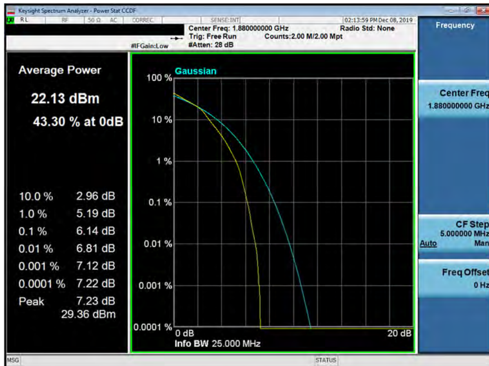
Plot 7-428. PAR Plot (Band 2 - 15.0MHz 16-QAM - Full RB Configuration)
