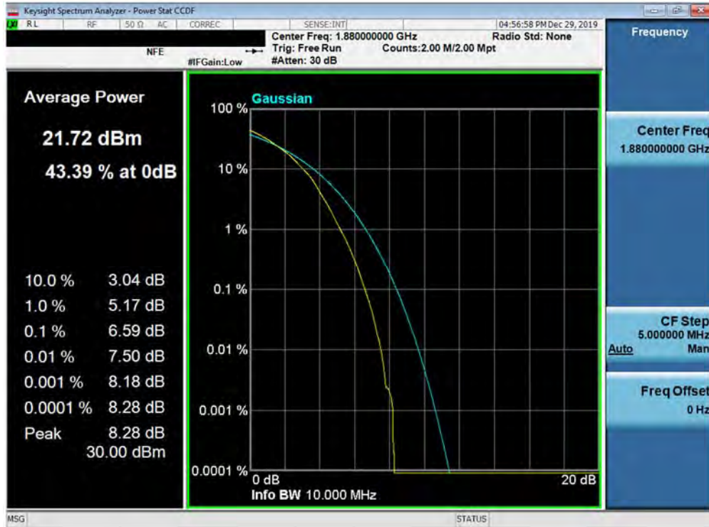
Plot 7-425. PAR Plot (Band 2 - 10.0MHz 64-QAM - Full RB Configuration)
