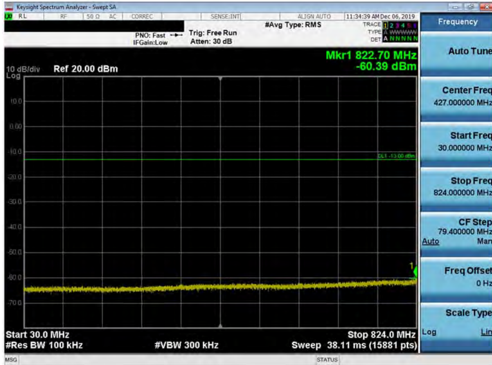
Plot 7-455. Conducted Spurious Plot (Band 5 - 10.0MHz QPSK - Left Carrier 1/49 Right Carrier 1/0 - Mid Channel)
