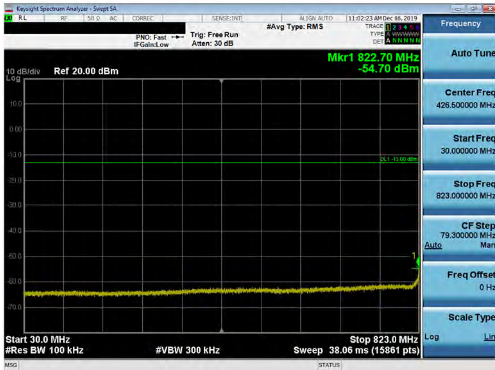
Plot 7-451. Conducted Spurious Plot (Band 5 - 10.0MHz QPSK - Left Carrier 1/49 Right Carrier 1/0 - Low Channel)
