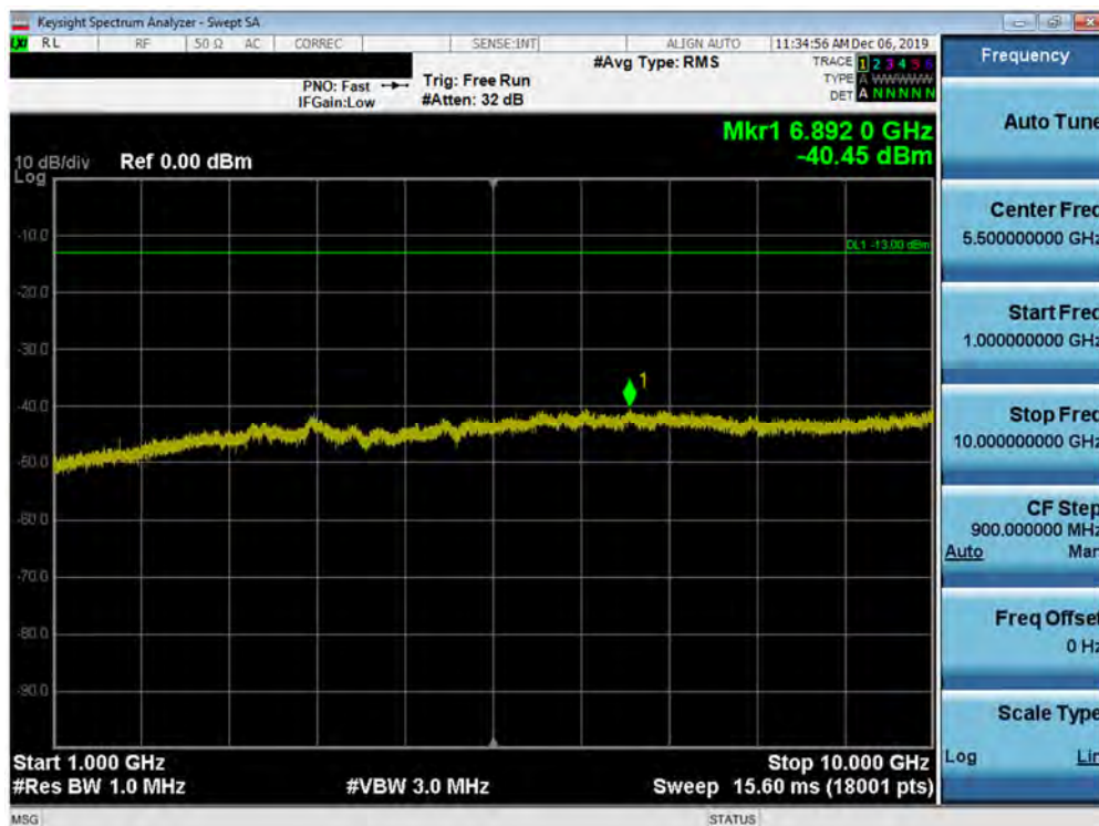
Plot 7-458. Conducted Spurious Plot (Band 5 - 10.0MHz QPSK - Left Carrier 1/49 Right Carrier 1/0 - Mid Channel)
