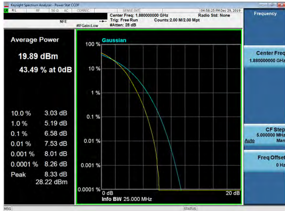
Plot 7-430. PAR Plot (Band 2 - 15.0MHz 256-QAM - Full RB Configuration)
