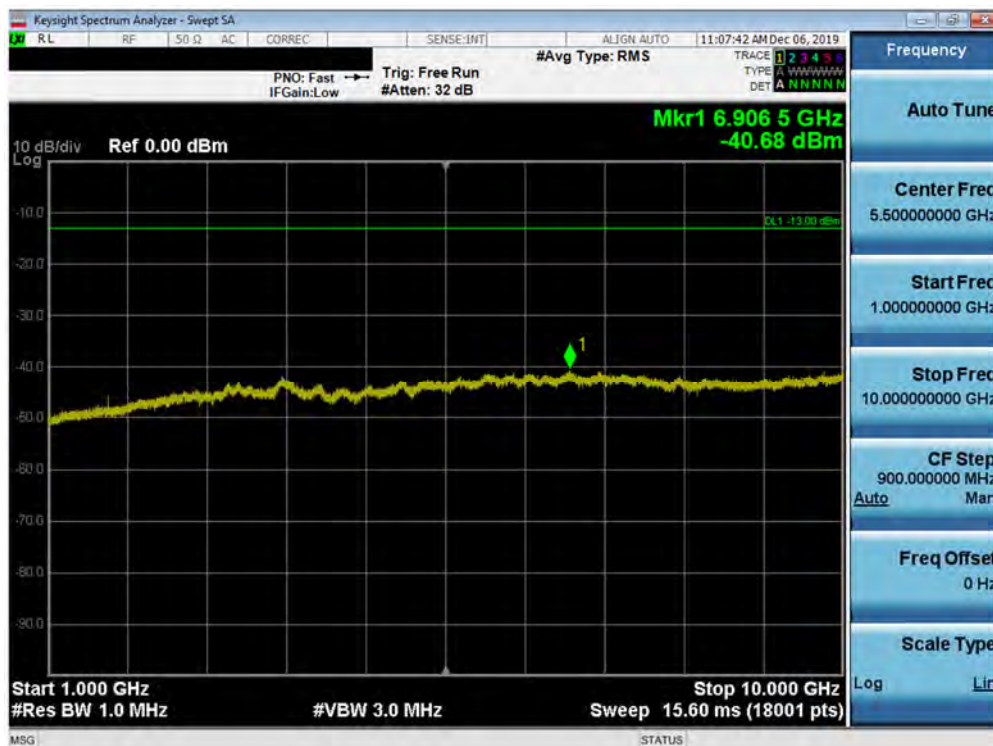
Plot 7-462. Conducted Spurious Plot (Band 5 - 10.0MHz QPSK - Left Carrier 1/49 Right Carrier 1/0 - High Channel)
