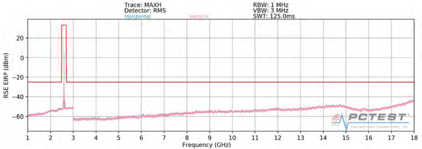
Plot 7-471. Radiated Spurious Plot 1GHz - 18GHz (Band 41)
