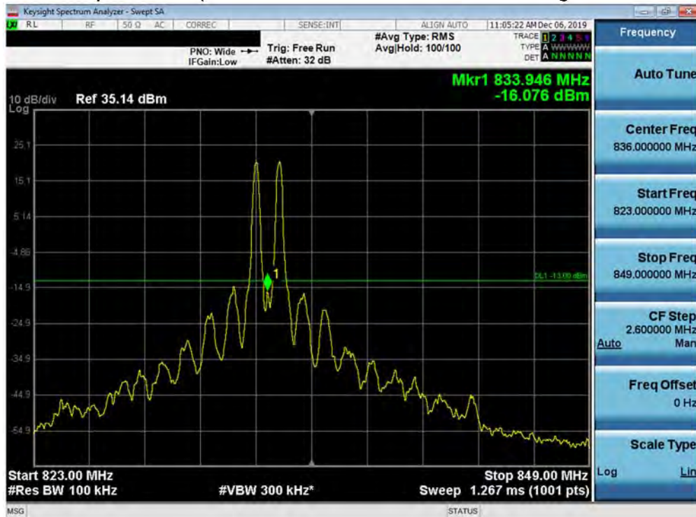
Plot 7-452. Conducted Spurious Plot (Band 5 - 10.0MHz QPSK - Left Carrier 1/49 Right Carrier 1/0 - Low Channel)
