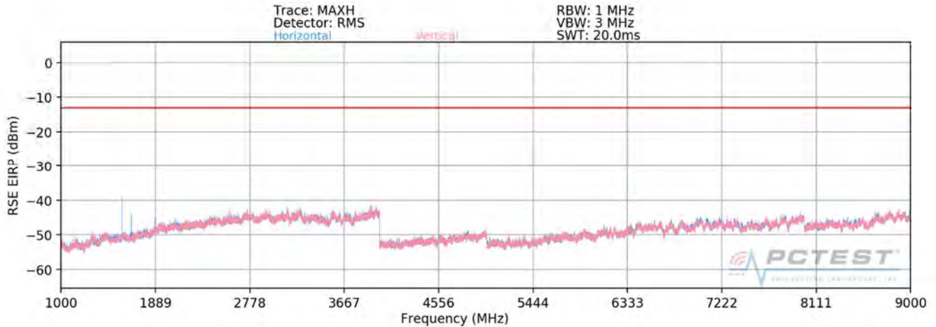
Plot 7-53. Radiated Spurious Plot (ULCA B5 Left Carrier: RB 1 Offset 49, Right Carrier: RB 1 Offset 0)
