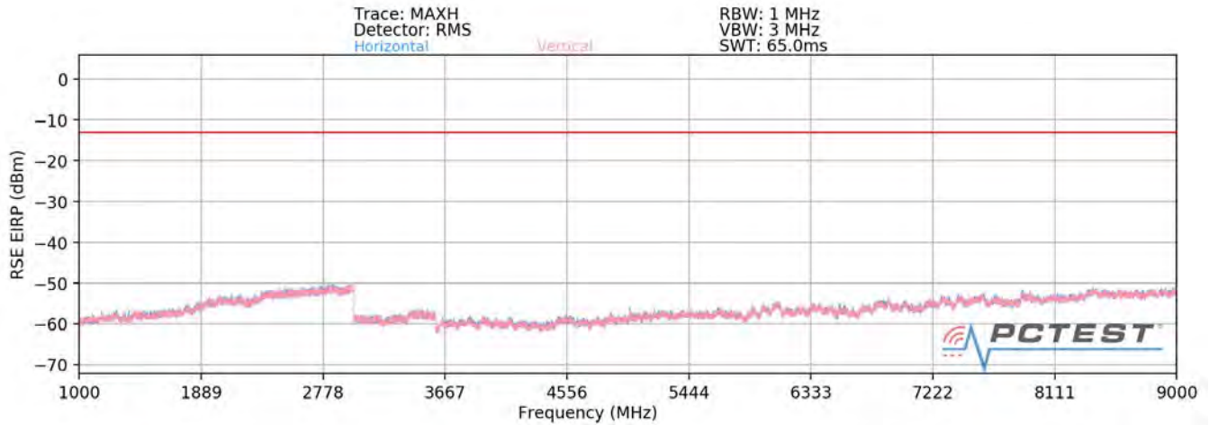
Plot 7-467. Radiated Spurious Plot above 1GHz (Band 5)
