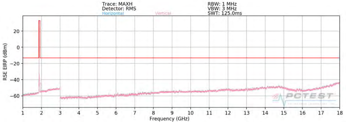
Plot 7-469. Radiated Spurious Plot above 1GHz (Band 2)
