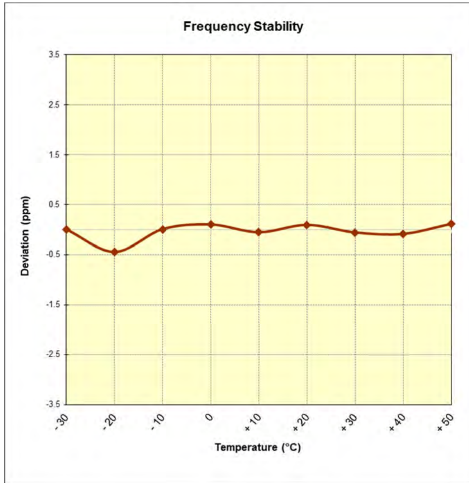
Figure 7-17. Frequency Stability Graph (5G NR n5)
