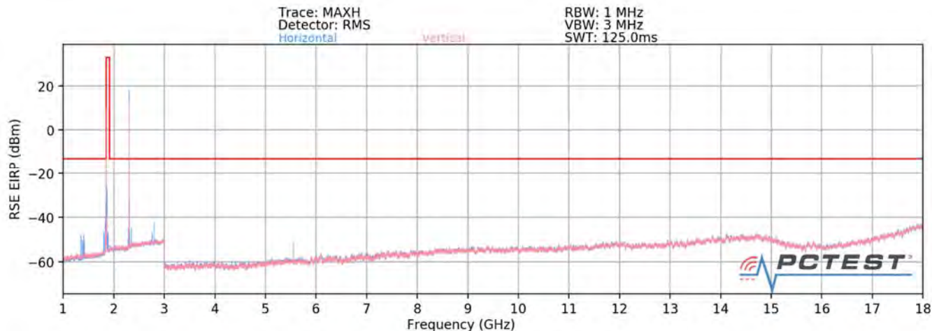
Plot 7-476. Radiated Spurious Plot above 1GHz (5G NR n2 + B30)
