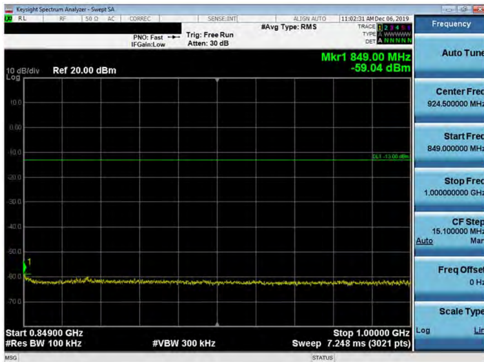
Plot 7-453. Conducted Spurious Plot (Band 5 - 10.0MHz QPSK - Left Carrier 1/49 Right Carrier 1/0 - Low Channel)
