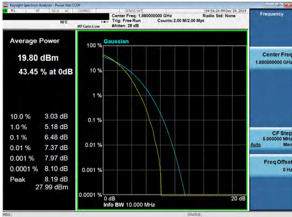
Plot 7-426. PAR Plot (Band 2 - 10.0MHz 256-QAM - Full RB Configuration)
