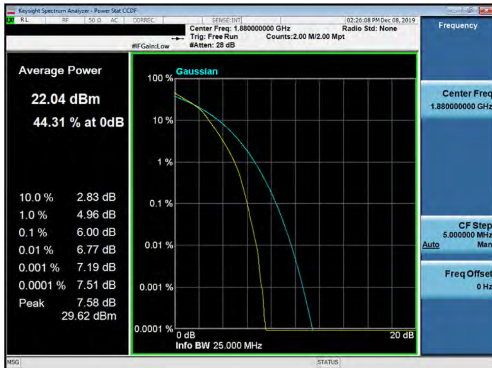
Plot 7-432. PAR Plot (Band 2 - 20.0MHz 16-QAM - Full RB Configuration)
