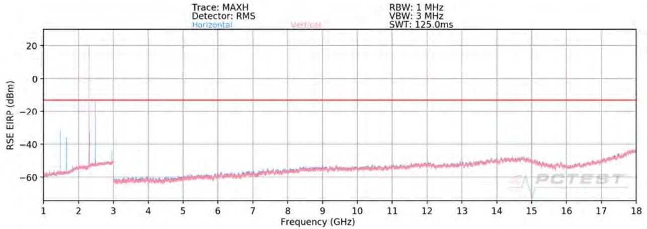
Plot 7-475. Radiated Spurious Plot above 1GHz (5G NR n5 + B30)
