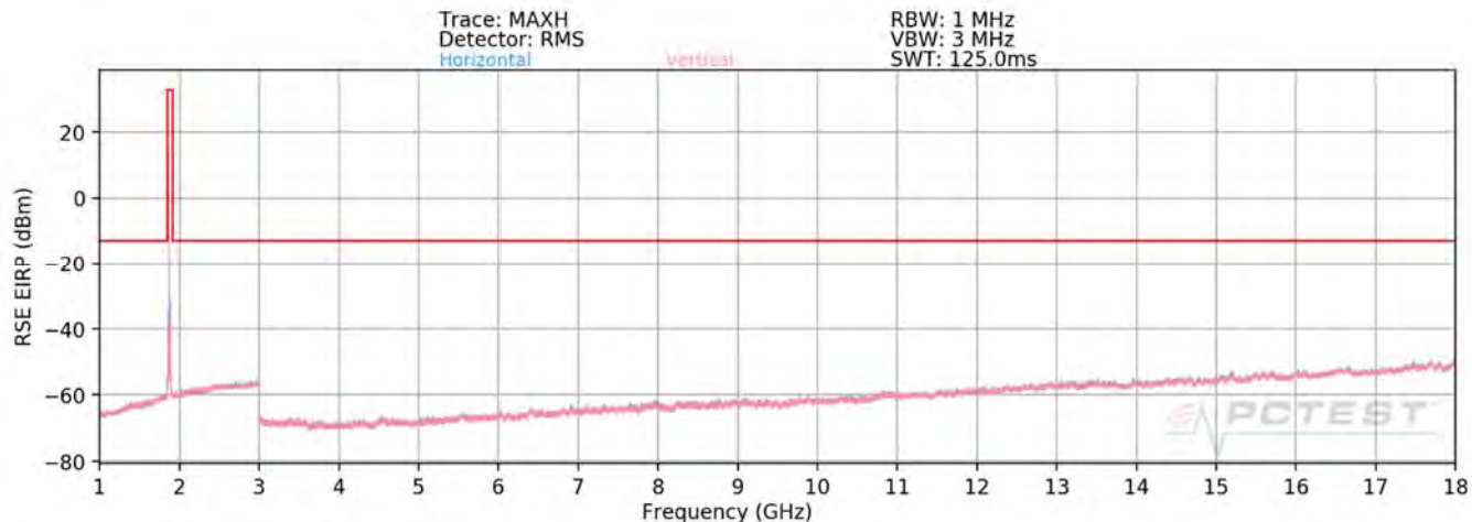
Plot 7-472. Radiated Spurious Plot above 1GHz (5G NR n2 + B5)
