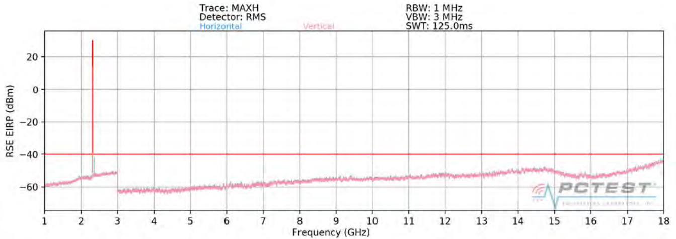
Plot 7-470. Radiated Spurious Plot 1GHz - 18GHz (Band 30)
