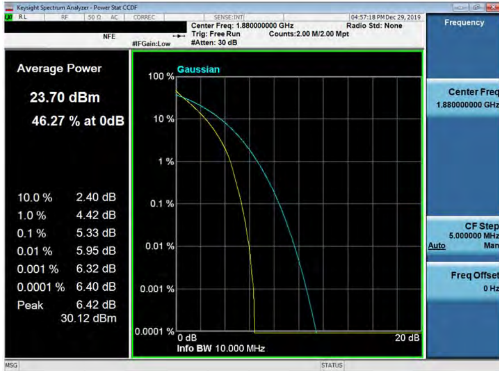
Plot 7-423. PAR Plot (Band 2 - 10.0MHz QPSK - Full RB Configuration)
