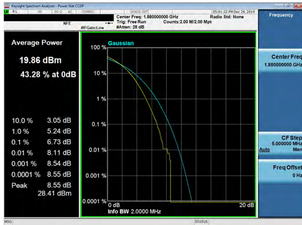
Plot 7-414. PAR Plot (Band 2 - 1.4MHz 256-QAM - Full RB Configuration)
