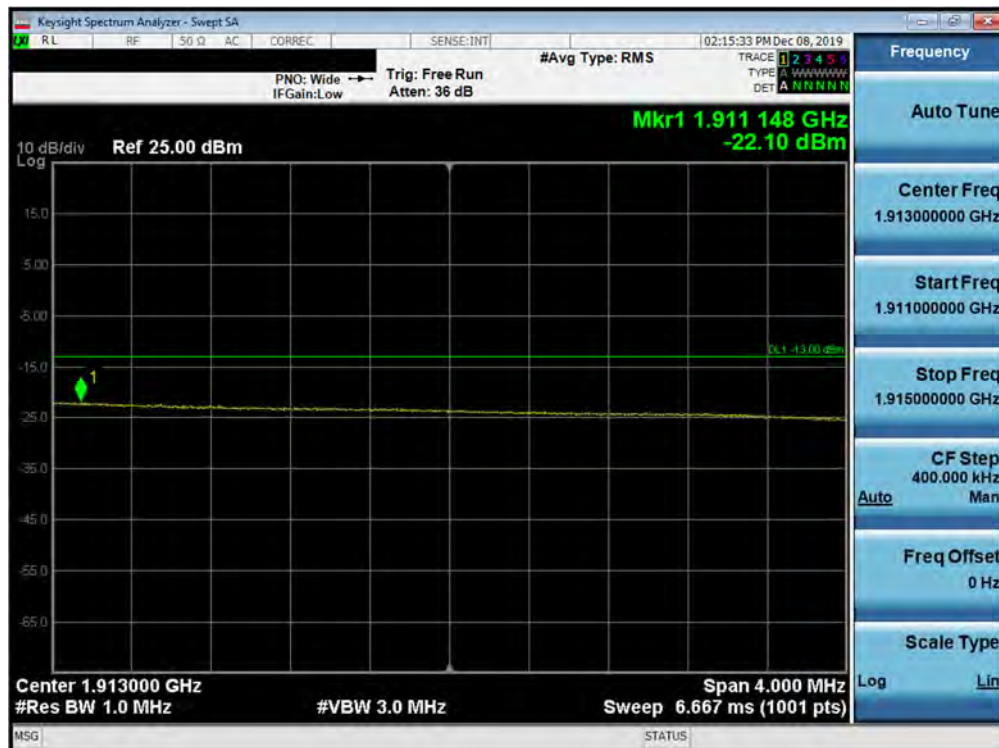
Plot 7-309. Upper Extended Band Edge Plot (Band 2 - 15.0MHz QPSK - Full RB Configuration)
