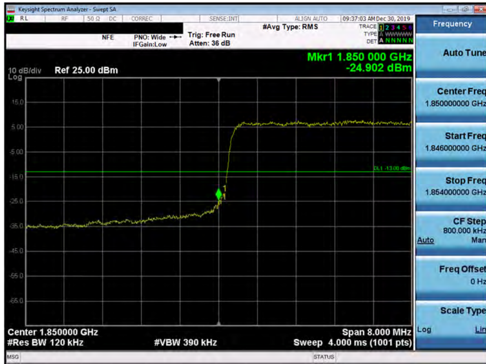
Plot 7-387. Lower Band Edge Plot (5G NR n2 - 10.0MHz QPSK - DFT-s - Full RB Configuration)
