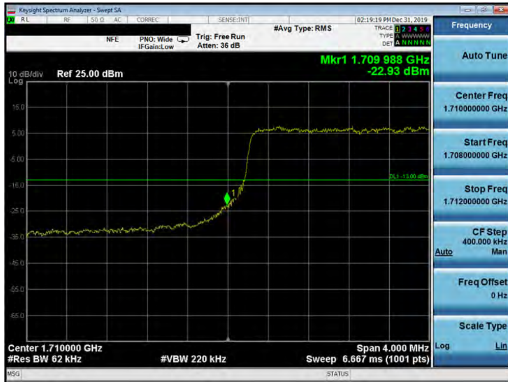
Plot 7-347. Lower Band Edge Plot (5G NR n66 - 5.0MHz QPSK - DFT-s - Full RB Configuration)
