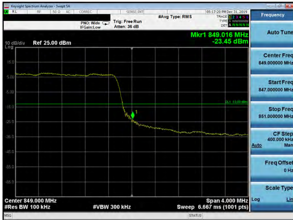
Plot 7-333. Upper Band Edge Plot (5G NR n5 - 5.0MHz QPSK - DFT-s - Full RB Configuration)
