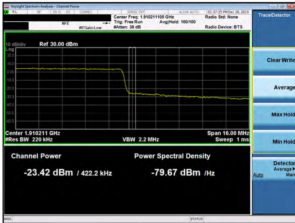
Plot 7-409. Upper Band Edge Plot (5G NR n2 - 20.0MHz QPSK - CP - Full RB Configuration)
