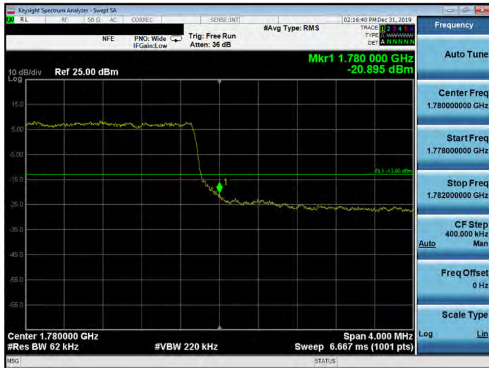
Plot 7-351. Upper Band Edge Plot (5G NR n66 - 5.0MHz QPSK - DFT-s - Full RB Configuration)
