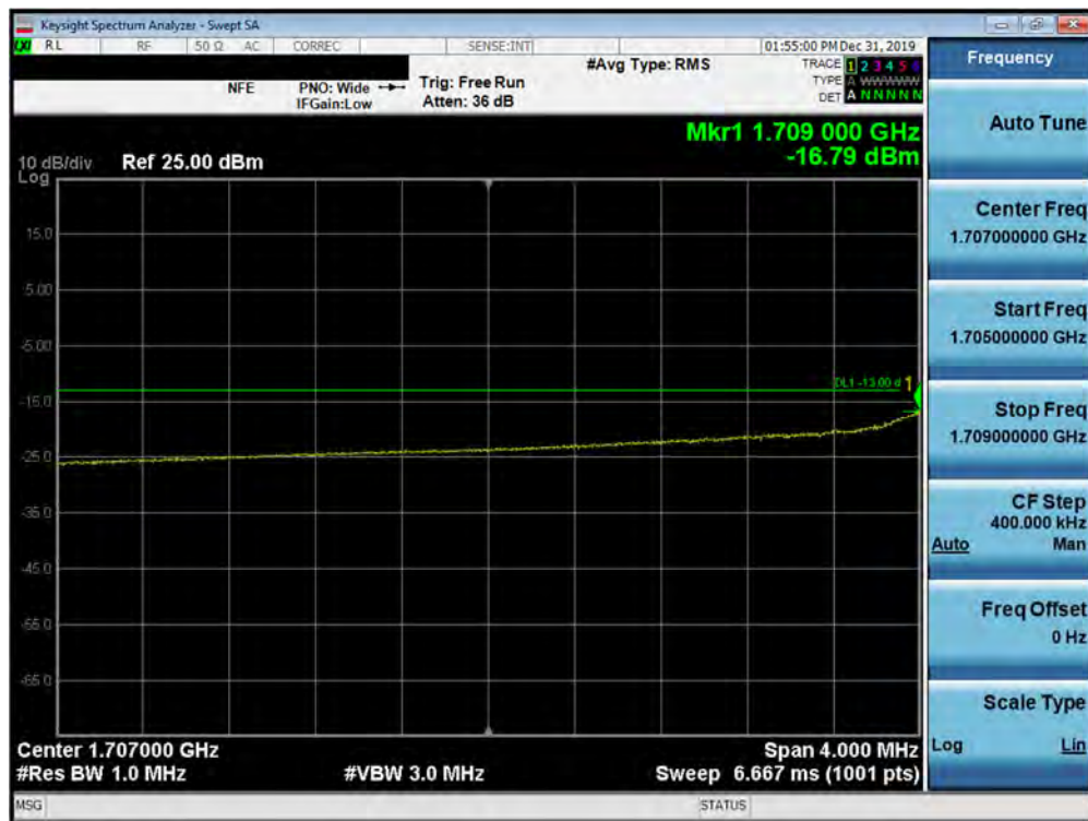
Plot 7-358. Lower Extended Band Edge Plot (5G NR n66 - 10.0MHz QPSK - CP - Full RB Configuration)
