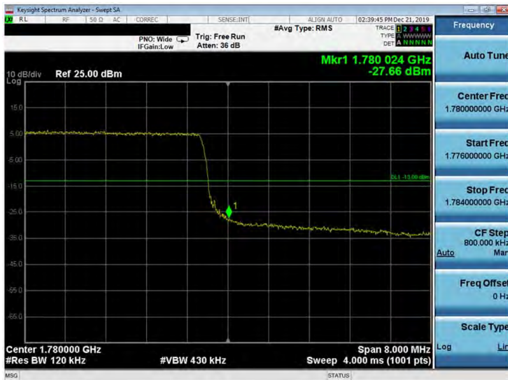
Plot 7-276. Upper Band Edge Plot (Band 66 - 10.0MHz QPSK - Full RB Configuration)
