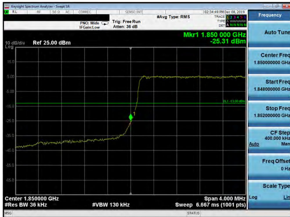
Plot 7-294. Lower Band Edge Plot (Band 2 - 3.0MHz QPSK - Full RB Configuration)
