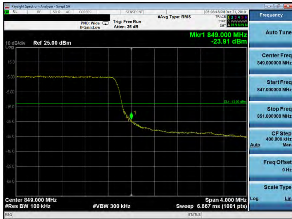
Plot 7-334. Upper Band Edge Plot (5G NR n5 - 5.0MHz QPSK - CP - Full RB Configuration)
