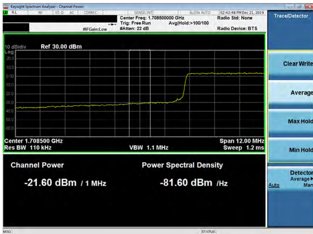
Plot 7-279. Lower Extended Band Edge Plot (Band 66/4 - 15.0MHz QPSK - Full RB Configuration)
