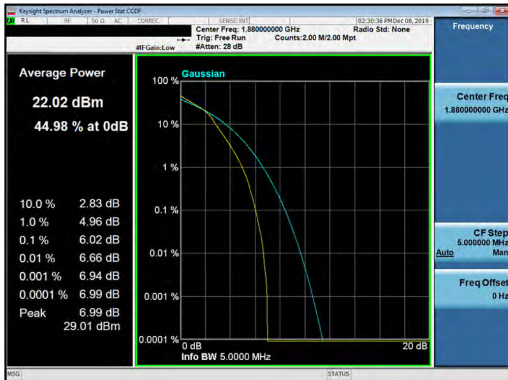
Plot 7-420. PAR Plot (Band 2 - 5.0MHz 16-QAM - Full RB Configuration)
