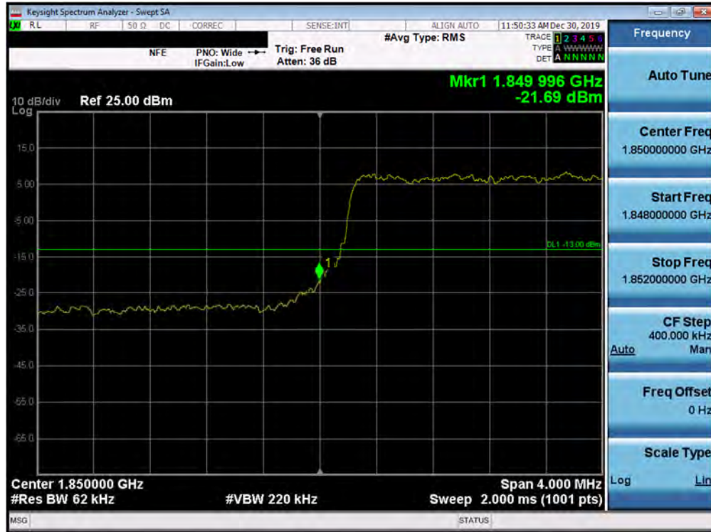
Plot 7-379. Lower Band Edge Plot (5G NR n2 - 5.0MHz QPSK - DFT-s - Full RB Configuration)
