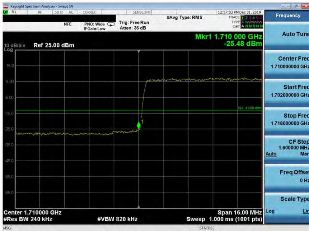
Plot 7-371. Lower Band Edge Plot (5G NR n66 - 20.0MHz QPSK - DFT-s - Full RB Configuration)
