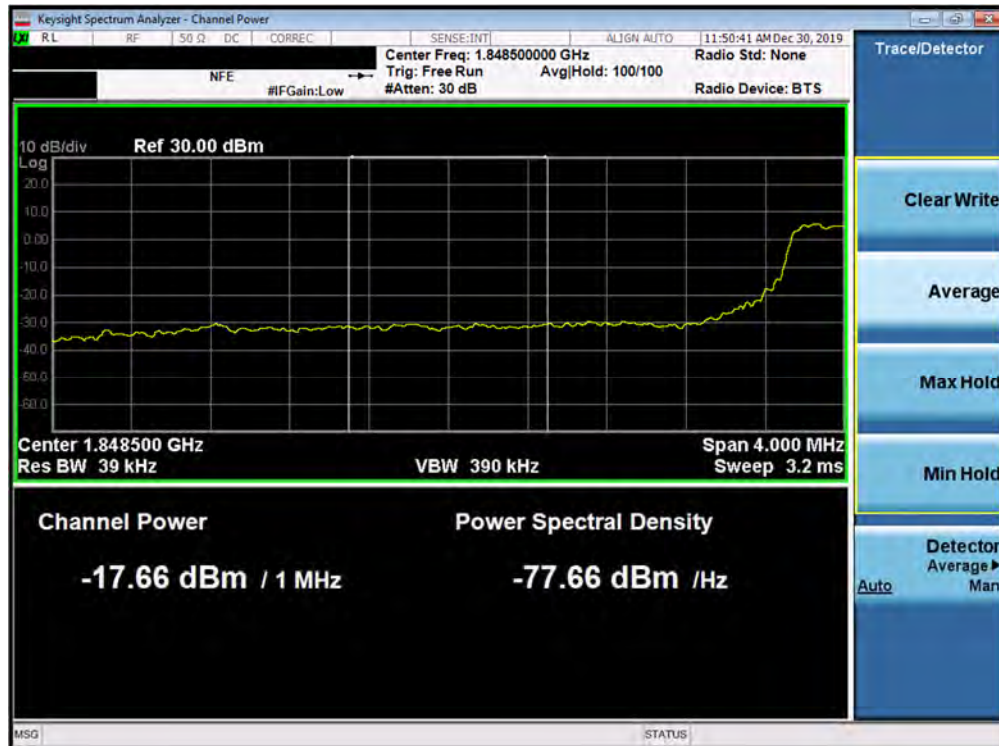
Plot 7-380. Lower Extended Band Edge Plot (5G NR n2 - 5.0MHz QPSK - DFT-s - Full RB Configuration)
