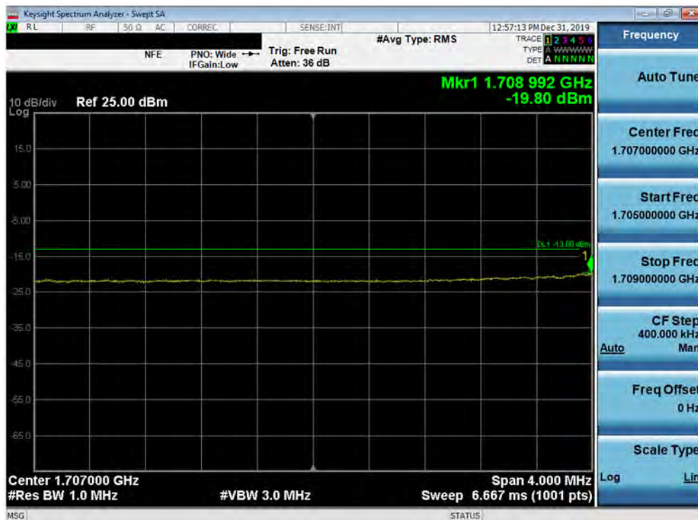
Plot 7-372. Lower Extended Band Edge Plot (5G NR n66 - 20.0MHz QPSK - DFT-s - Full RB Configuration)
