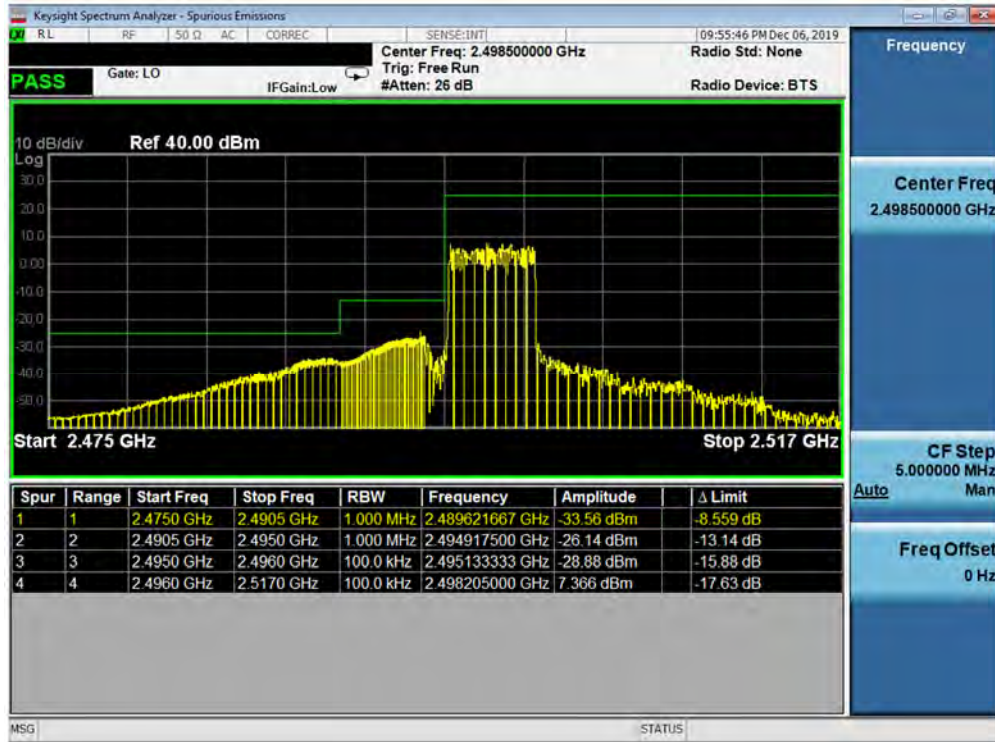
Plot 7-323. Lower ACP Plot at 2496 MHz (Band 41 - 5.0MHz QPSK - Full RB Configuration)
