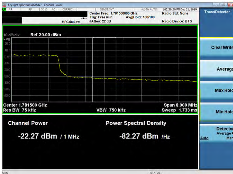
Plot 7-277. Upper Extended Band Edge Plot (Band 66 - 10.0MHz QPSK - Full RB Configuration)
