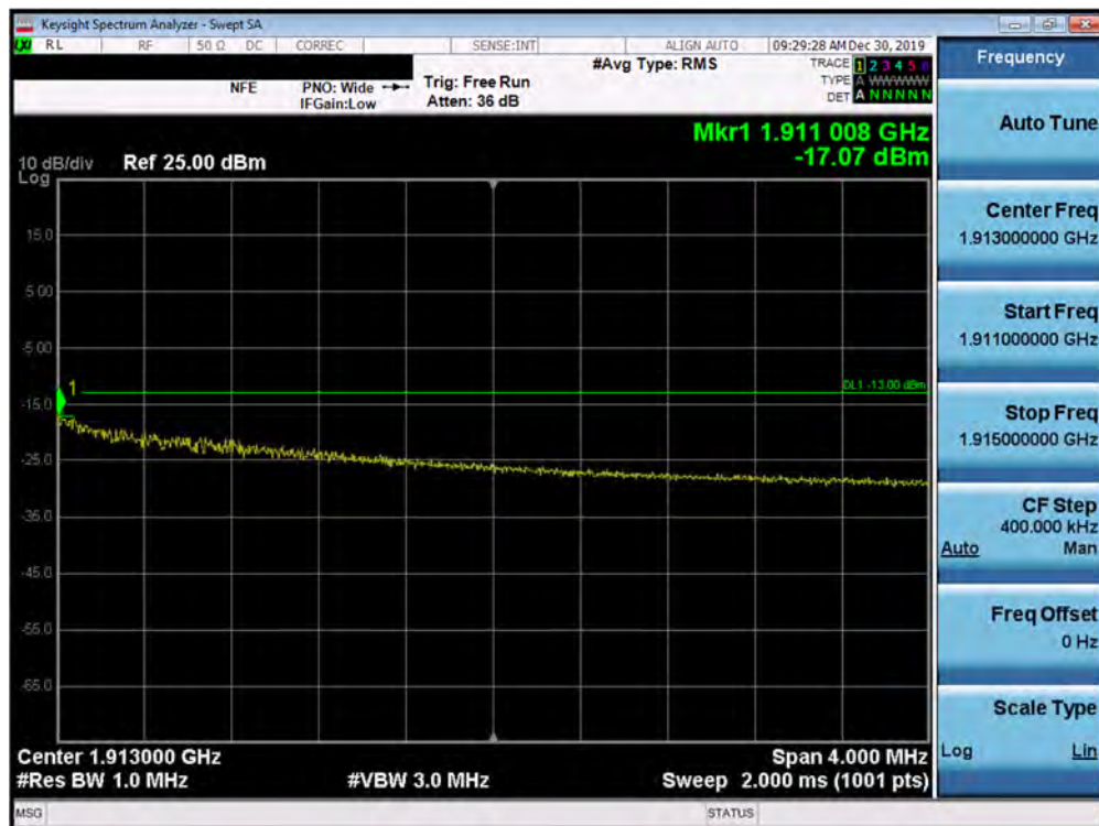
Plot 7-394. Upper Extended Band Edge Plot (5G NR n2 - 10.0MHz QPSK - CP - Full RB Configuration)
