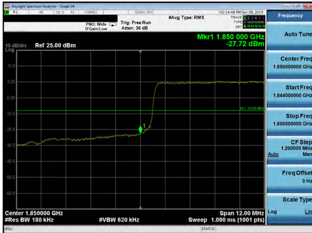
Plot 7-306. Lower Band Edge Plot (Band 2 - 15.0MHz QPSK - Full RB Configuration)
