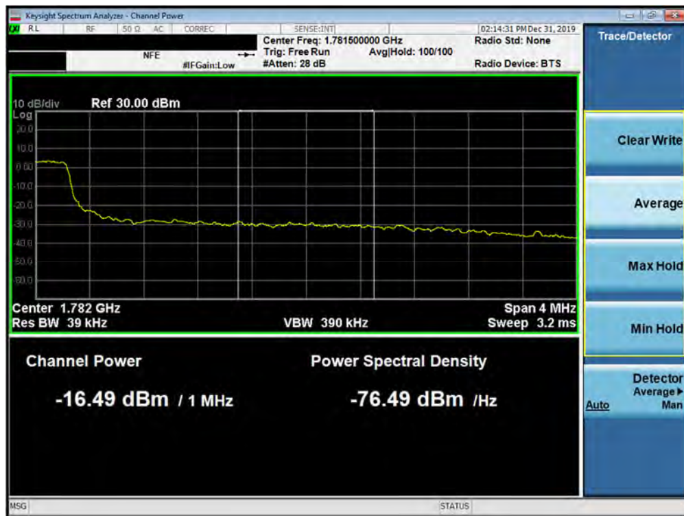
Plot 7-354. Upper Extended Band Edge Plot (5G NR n66 - 5.0MHz QPSK - CP - Full RB Configuration)
