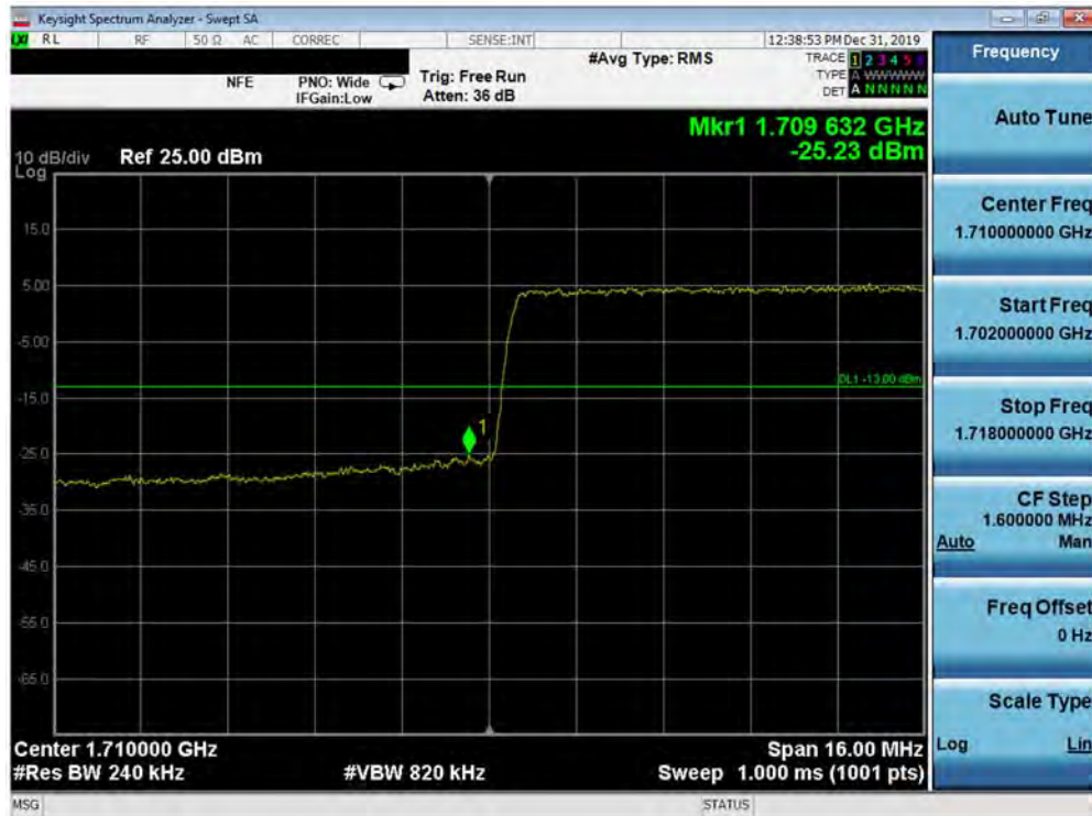
Plot 7-373. Lower Band Edge Plot (5G NR n66 - 20.0MHz QPSK - CP - Full RB Configuration)
