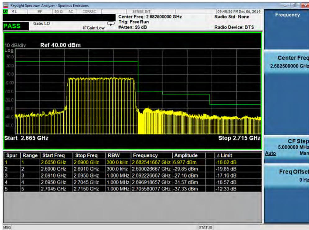
Plot 7-328. Upper ACP Plot (Band 41 - 15.0MHz QPSK - Full RB Configuration)
