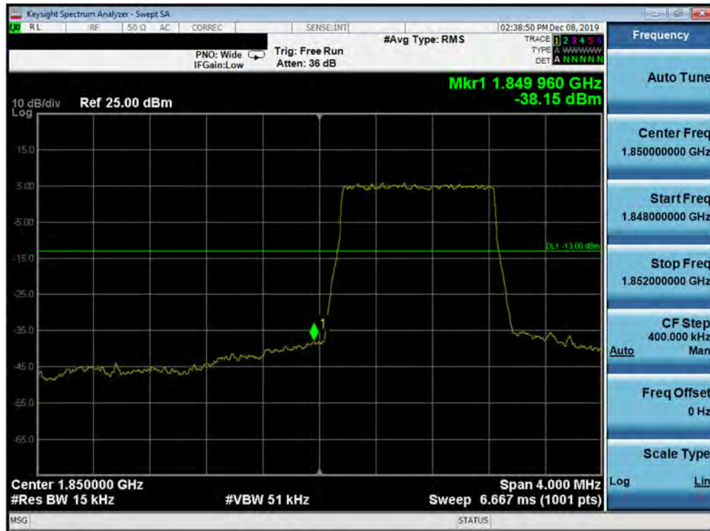
Plot 7-290. Lower Band Edge Plot (Band 2 - 1.4MHz QPSK - Full RB Configuration)
