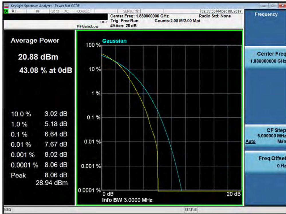
Plot 7-417. PAR Plot (Band 2 - 3.0MHz 64-QAM - Full RB Configuration)
