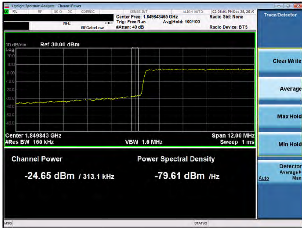
Plot 7-397. Lower Band Edge Plot (5G NR n2 - 15.0MHz QPSK - CP - Full RB Configuration)
