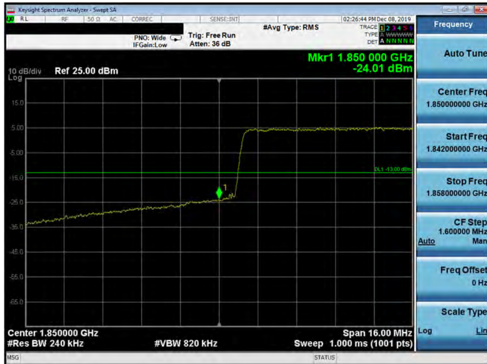
Plot 7-310. Lower Band Edge Plot (Band 2 - 20.0MHz QPSK - Full RB Configuration)
