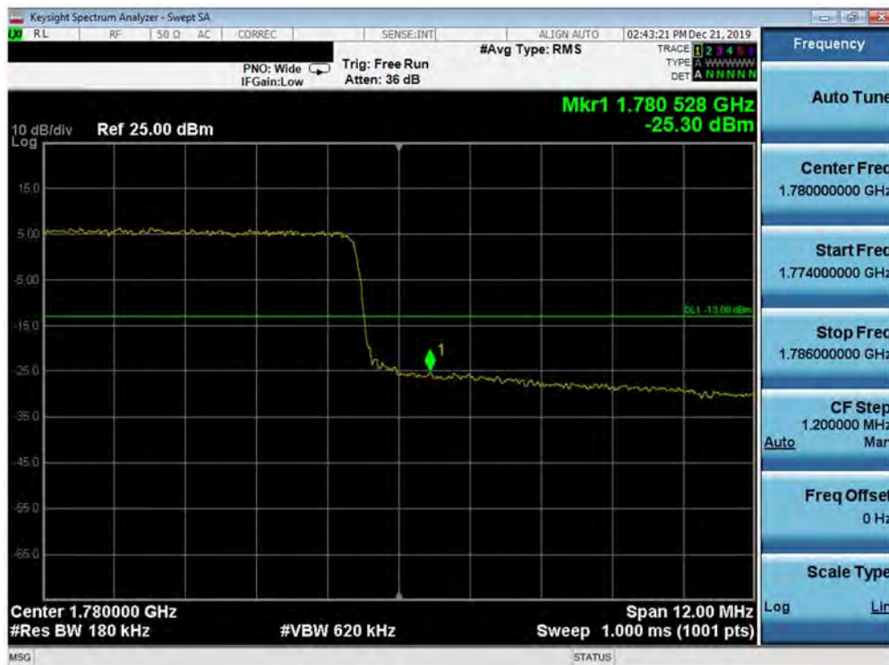
Plot 7-282. Upper Band Edge Plot (Band 66 - 15.0MHz QPSK - Full RB Configuration)
