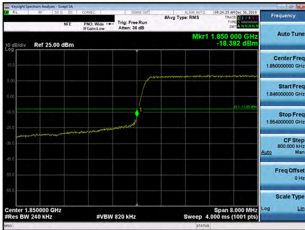
Plot 7-389. Lower Band Edge Plot (5G NR n2 - 10.0MHz QPSK - CP - Full RB Configuration)
