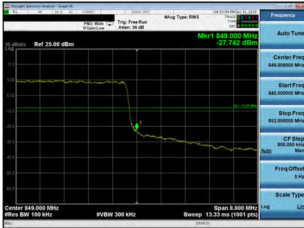
Plot 7-337. Upper Band Edge Plot (5G NR n5 - 10.0MHz QPSK - DFT-s - Full RB Configuration)
