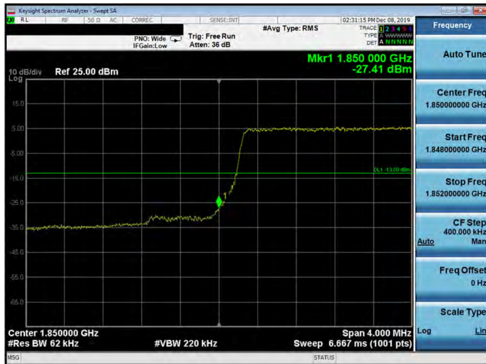
Plot 7-298. Lower Band Edge Plot (Band 2 - 5.0MHz QPSK - Full RB Configuration)
