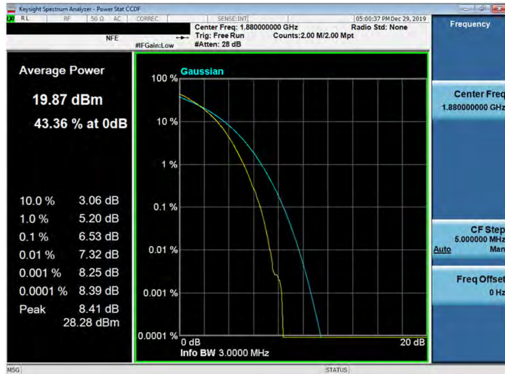
Plot 7-418. PAR Plot (Band 2 - 3.0MHz 256-QAM - Full RB Configuration)
