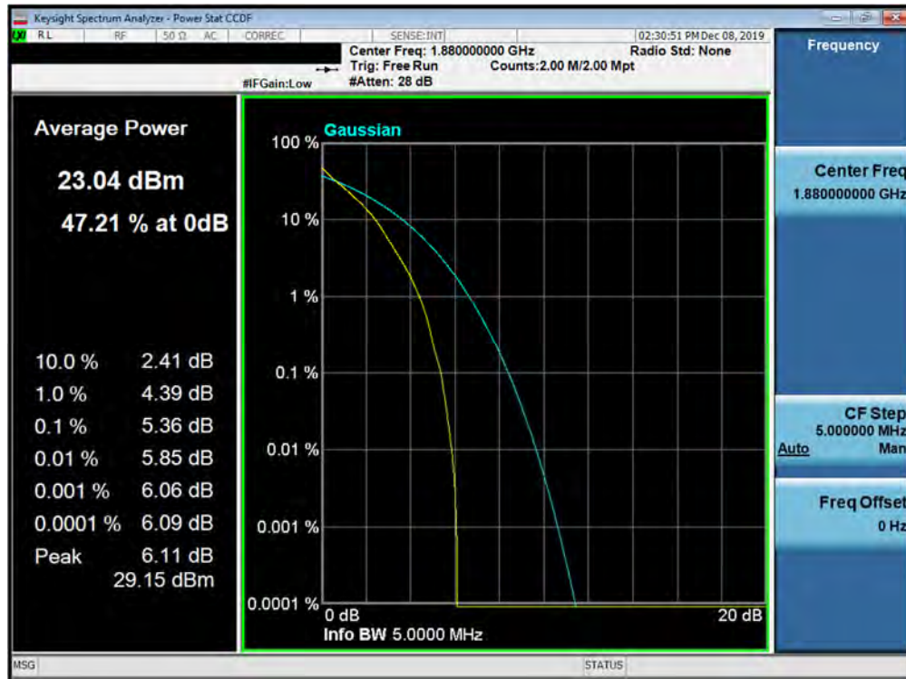
Plot 7-419. PAR Plot (Band 2 - 5.0MHz QPSK - Full RB Configuration)
