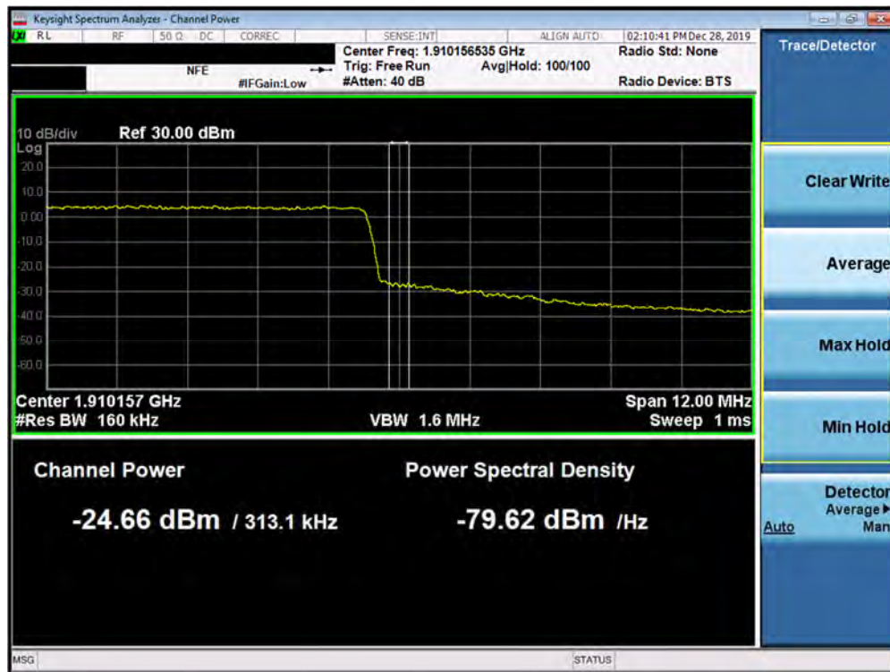
Plot 7-401. Upper Band Edge Plot (5G NR n2 - 15.0MHz QPSK - CP - Full RB Configuration)
