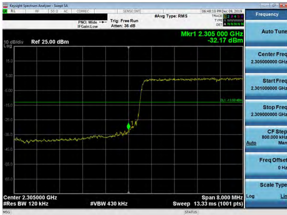
Plot 7-317. Lower Band Edge Plot (Band 30 - 10.0MHz QPSK - Full RB Configuration)
