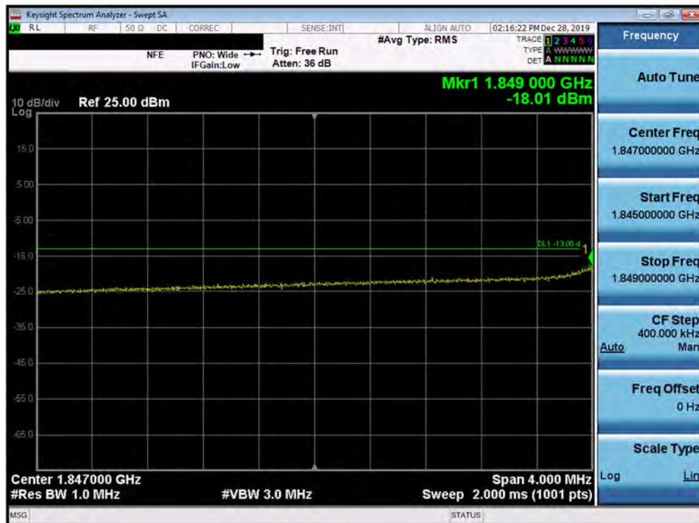
Plot 7-396. Lower Extended Band Edge Plot (5G NR n2 - 15.0MHz QPSK - DFT-s - Full RB Configuration)
