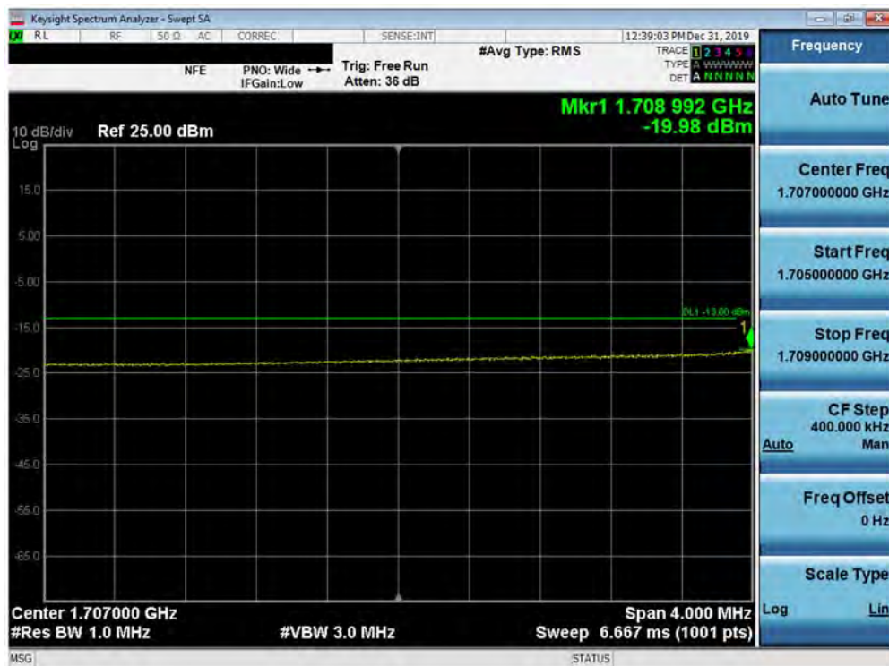
Plot 7-374. Lower Extended Band Edge Plot (5G NR n66 - 20.0MHz QPSK - CP - Full RB Configuration)
