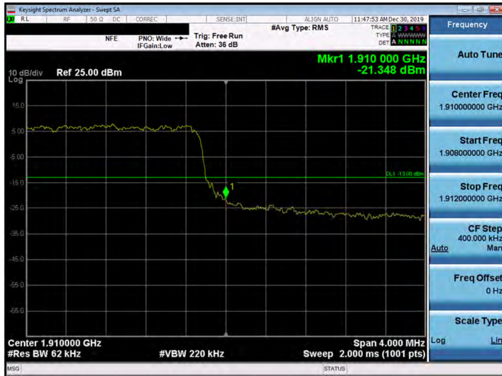
Plot 7-383. Upper Band Edge Plot (5G NR n2 - 5.0MHz QPSK - DFT-s - Full RB Configuration)
