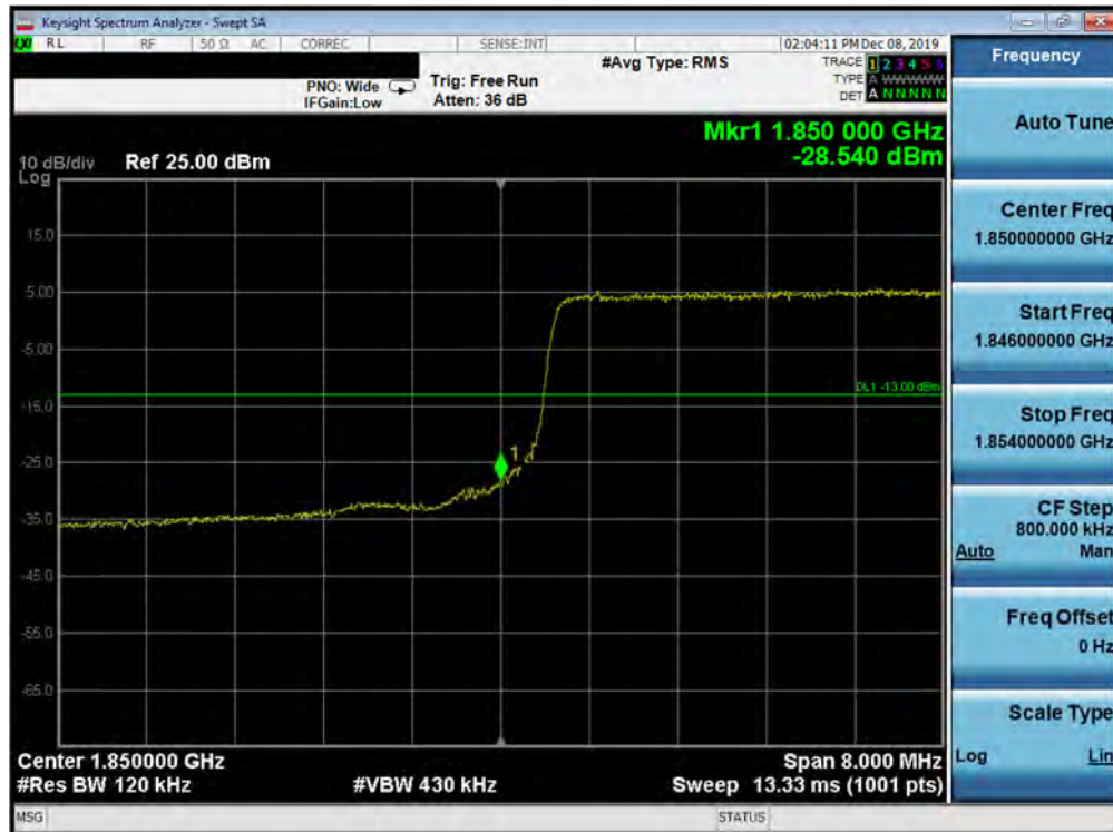
Plot 7-302. Lower Band Edge Plot (Band 2 - 10.0MHz QPSK - Full RB Configuration)
