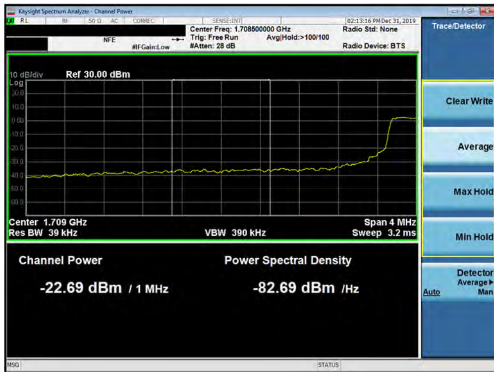
Plot 7-350. Lower Extended Band Edge Plot (5G NR n66 - 5.0MHz QPSK - CP - Full RB Configuration)
