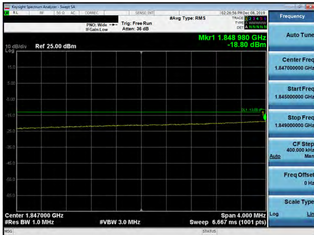
Plot 7-311. Lower Extended Band Edge Plot (Band 2 - 20.0MHz QPSK - Full RB Configuration)
