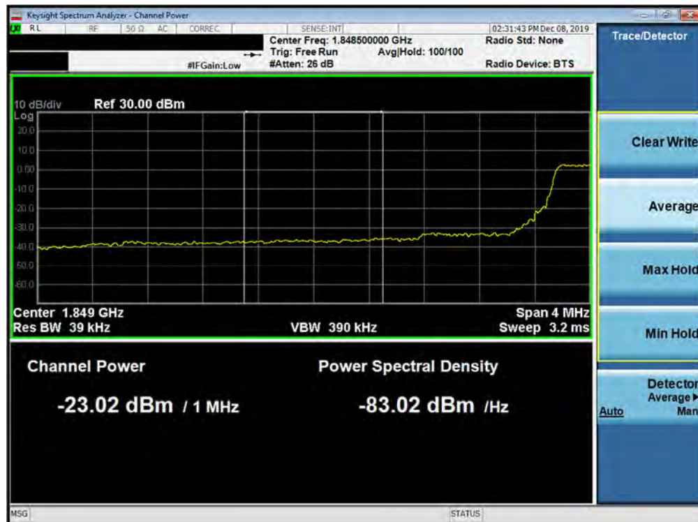
Plot 7-299. Lower Extended Band Edge Plot (Band 2 - 5.0MHz QPSK - Full RB Configuration)
