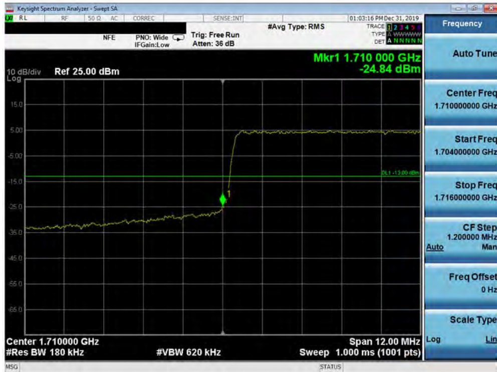
Plot 7-365. Lower Band Edge Plot (5G NR n66 - 15.0MHz QPSK - CP - Full RB Configuration)
