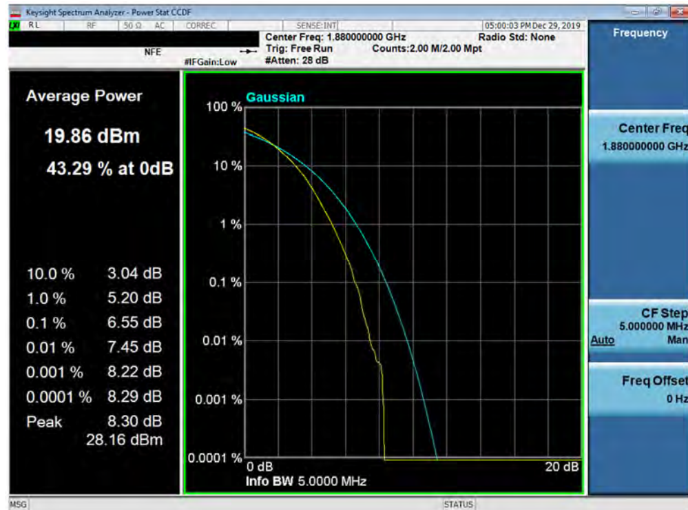
Plot 7-422. PAR Plot (Band 2 - 5.0MHz 256-QAM - Full RB Configuration)
