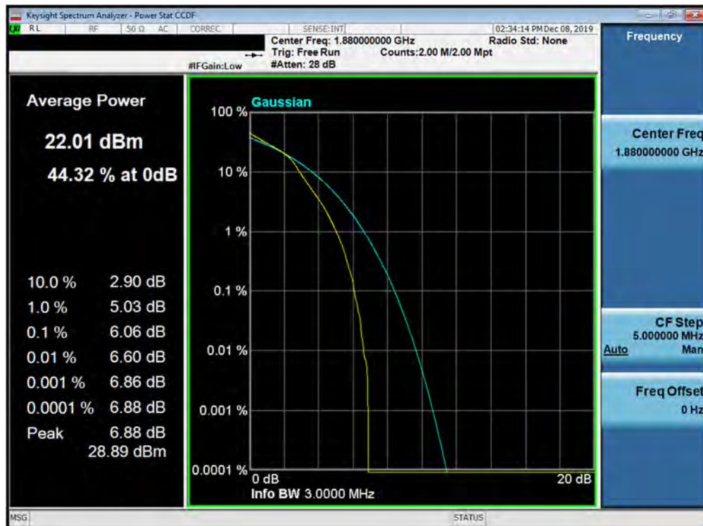
Plot 7-416. PAR Plot (Band 2 - 3.0MHz 16-QAM - Full RB Configuration)
