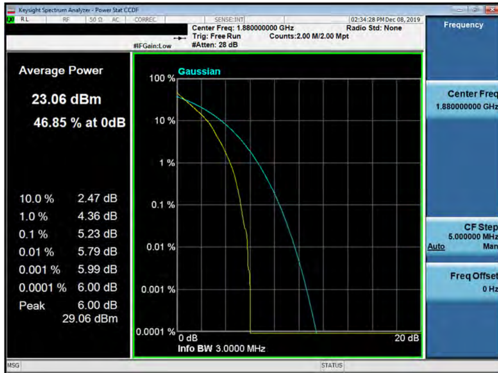
Plot 7-415. PAR Plot (Band 2 - 3.0MHz QPSK - Full RB Configuration)
