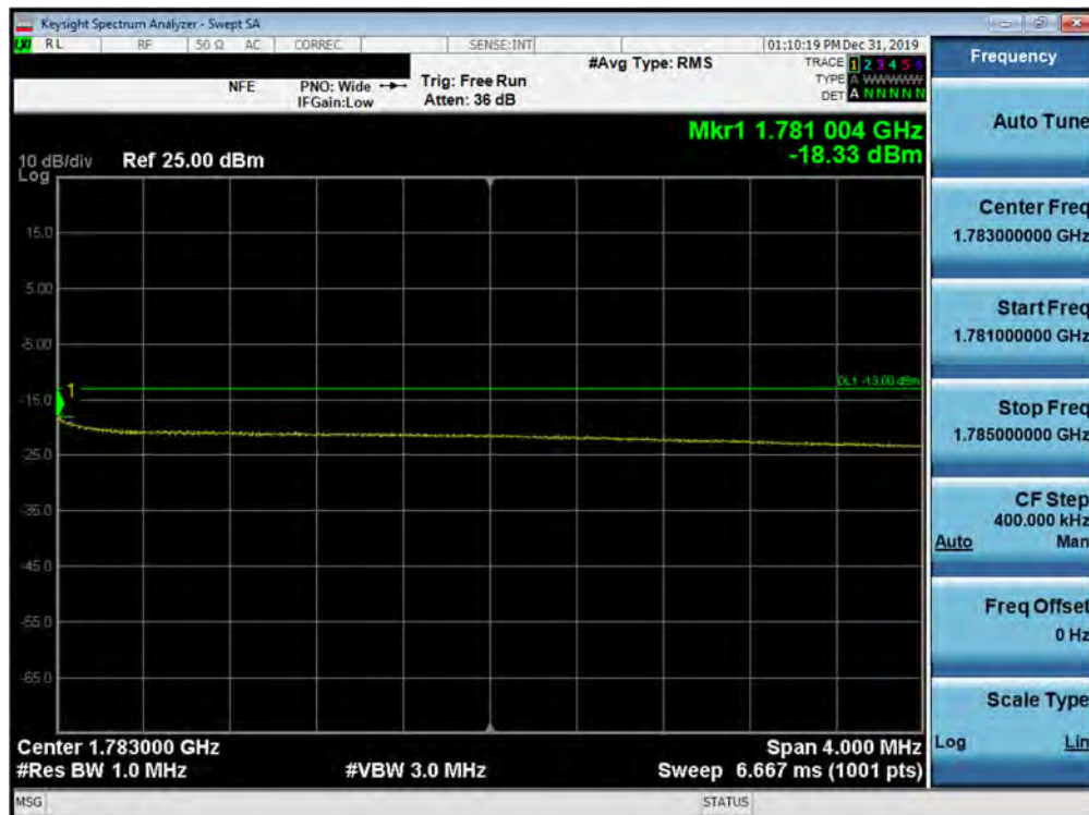
Plot 7-368. Upper Extended Band Edge Plot (5G NR n66 - 15.0MHz QPSK - DFT-s - Full RB Configuration)
