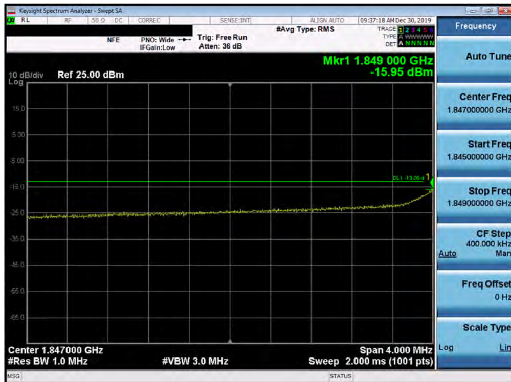
Plot 7-388. Lower Extended Band Edge Plot (5G NR n2 - 10.0MHz QPSK - DFT-s - Full RB Configuration)
