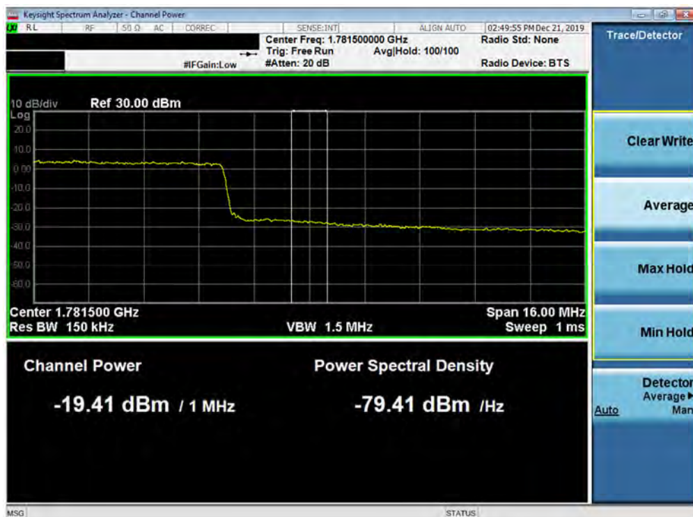
Plot 7-289. Upper Extended Band Edge Plot (Band 66 - 20.0MHz QPSK - Full RB Configuration)
