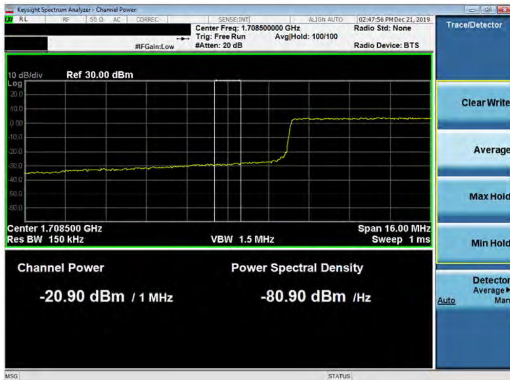
Plot 7-285. Lower Extended Band Edge Plot (Band 66/4 - 20.0MHz QPSK - Full RB Configuration)
