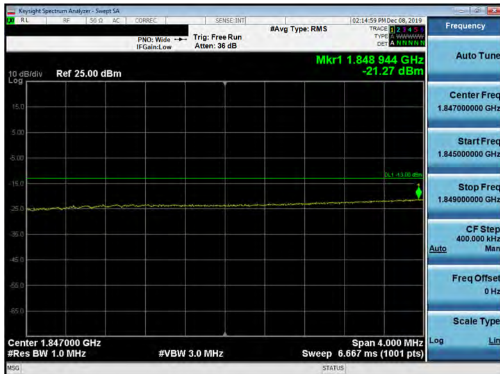
Plot 7-307. Lower Extended Band Edge Plot (Band 2 - 15.0MHz QPSK - Full RB Configuration)
