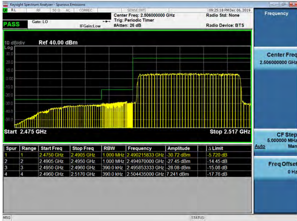
Plot 7-329. Lower ACP Plot at 2496 MHz (Band 41 - 20.0MHz QPSK - Full RB Configuration)
