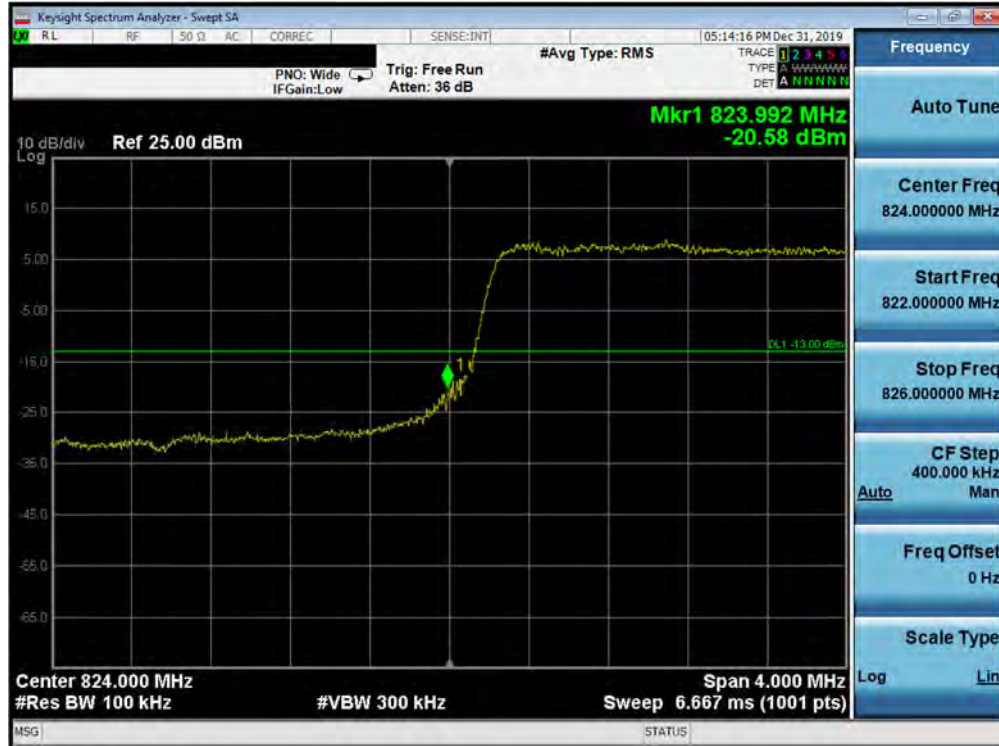
Plot 7-331. Lower Band Edge Plot (5G NR n5 - 5.0MHz QPSK - DFT-s - Full RB Configuration)
