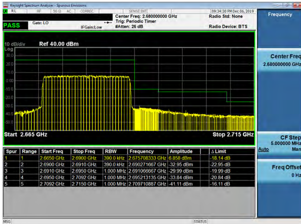
Plot 7-330. Upper ACP Plot (Band 41 - 20.0MHz QPSK - Full RB Configuration)
