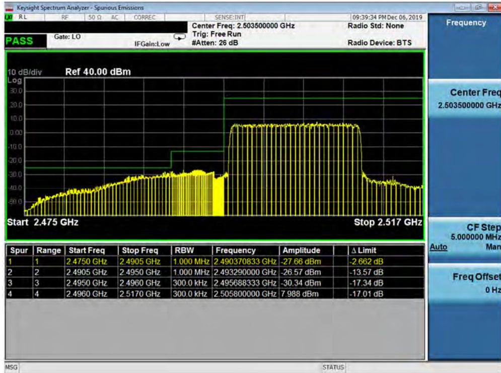
Plot 7-327. Lower ACP Plot at 2496 MHz (Band 41 - 15.0MHz QPSK - Full RB Configuration)
