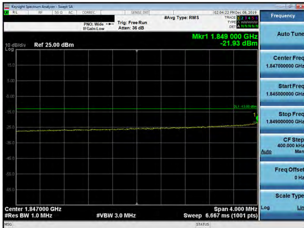
Plot 7-303. Lower Extended Band Edge Plot (Band 2 - 10.0MHz QPSK - Full RB Configuration)
