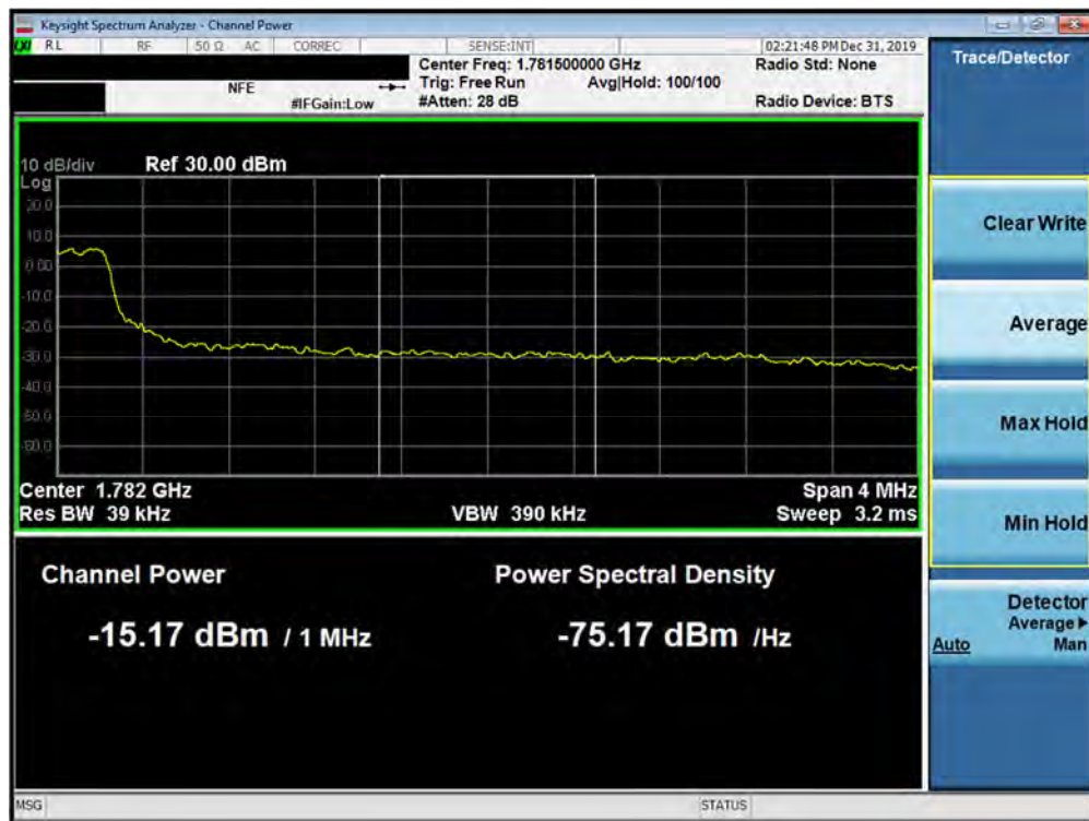
Plot 7-352. Upper Extended Band Edge Plot (5G NR n66 - 5.0MHz QPSK - DFT-s - Full RB Configuration)
