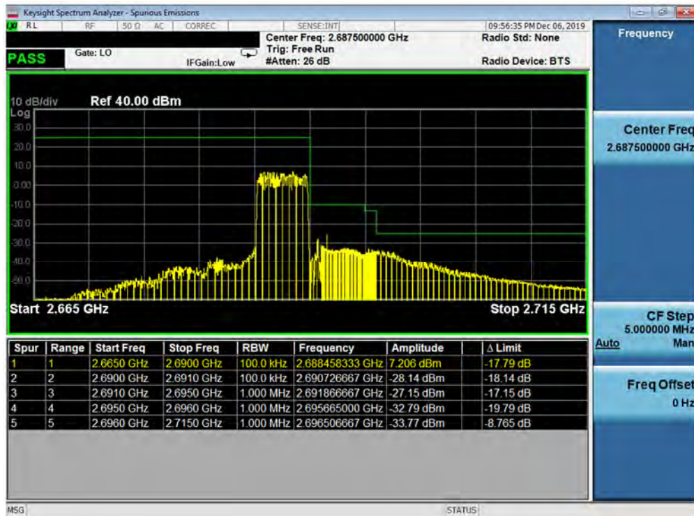
Plot 7-324. Upper ACP Plot (Band 41 - 5.0MHz QPSK - Full RB Configuration)
