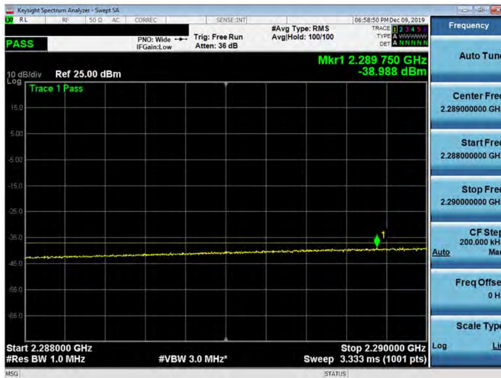
Plot 7-318. Lower Extended Band Edge Plot (Band 30 - 5.0MHz QPSK - Full RB Configuration)
