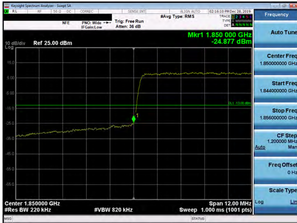
Plot 7-395. Lower Band Edge Plot (5G NR n2 - 15.0MHz QPSK - DFT-s - Full RB Configuration)
