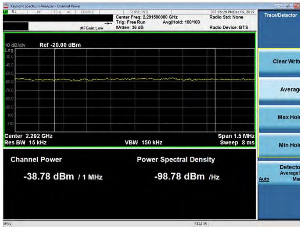
Plot 7-320. Lower Extended Band Edge Plot (Band 30 - 5.0MHz QPSK - Full RB Configuration)
