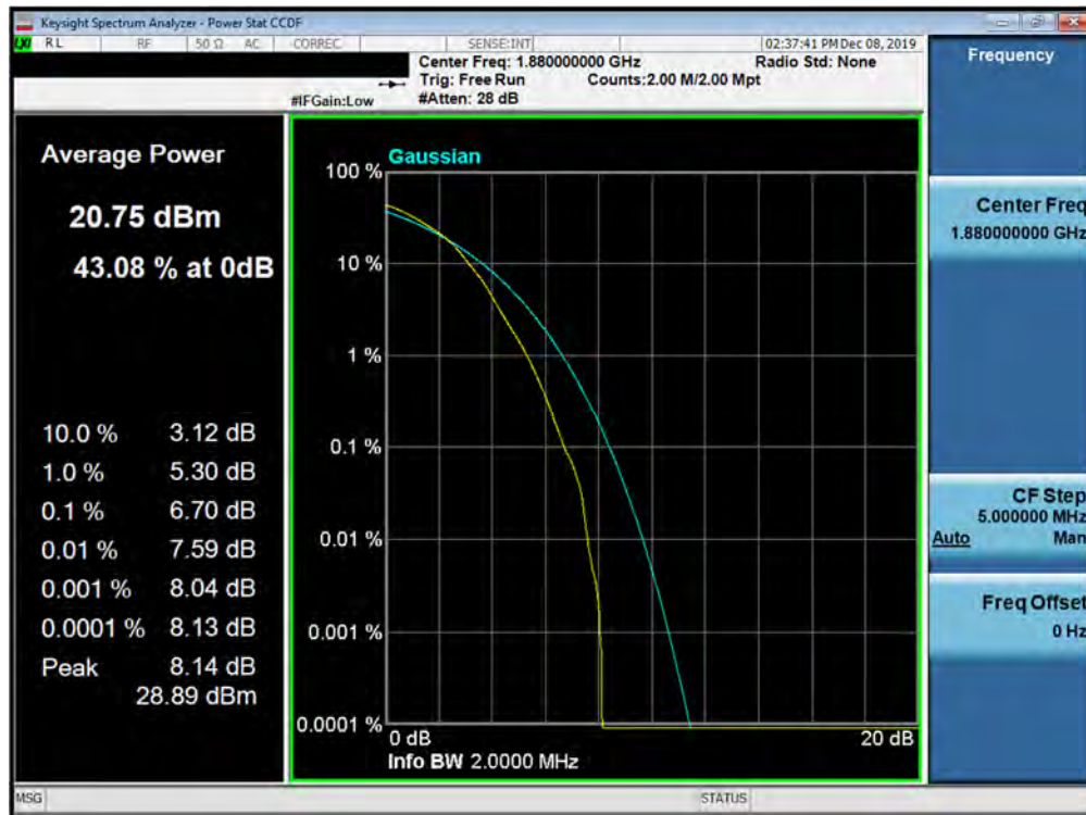
Plot 7-413. PAR Plot (Band 2 - 1.4MHz 64-QAM - Full RB Configuration)
