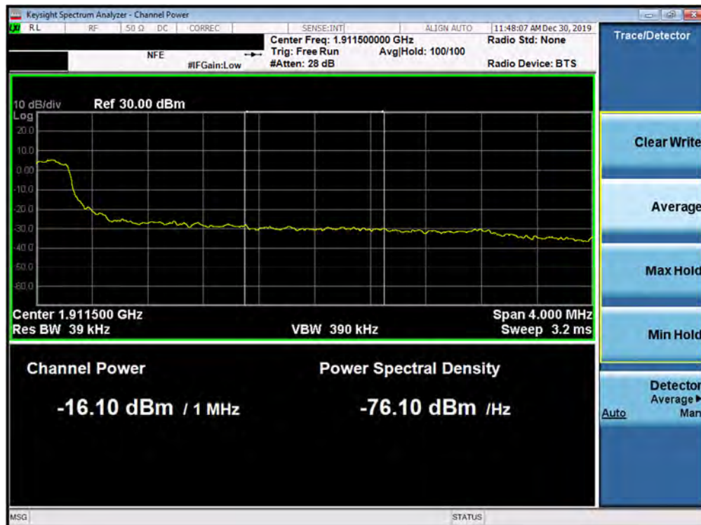
Plot 7-384. Upper Extended Band Edge Plot (5G NR n2 - 5.0MHz QPSK - DFT-s - Full RB Configuration)
