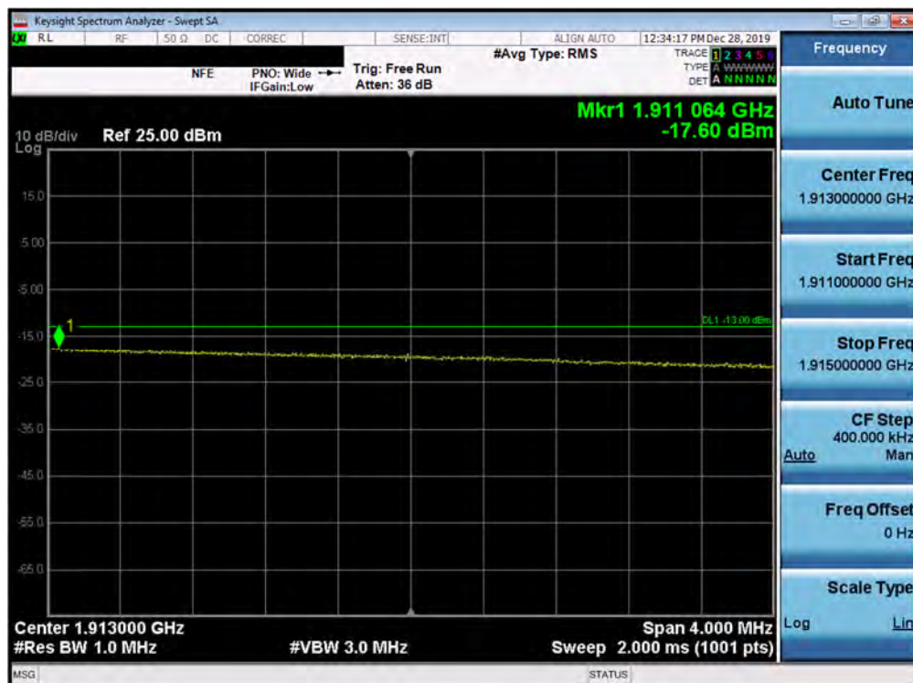
Plot 7-408. Upper Extended Band Edge Plot (5G NR n2 - 20.0MHz QPSK - DFT-s - Full RB Configuration)
