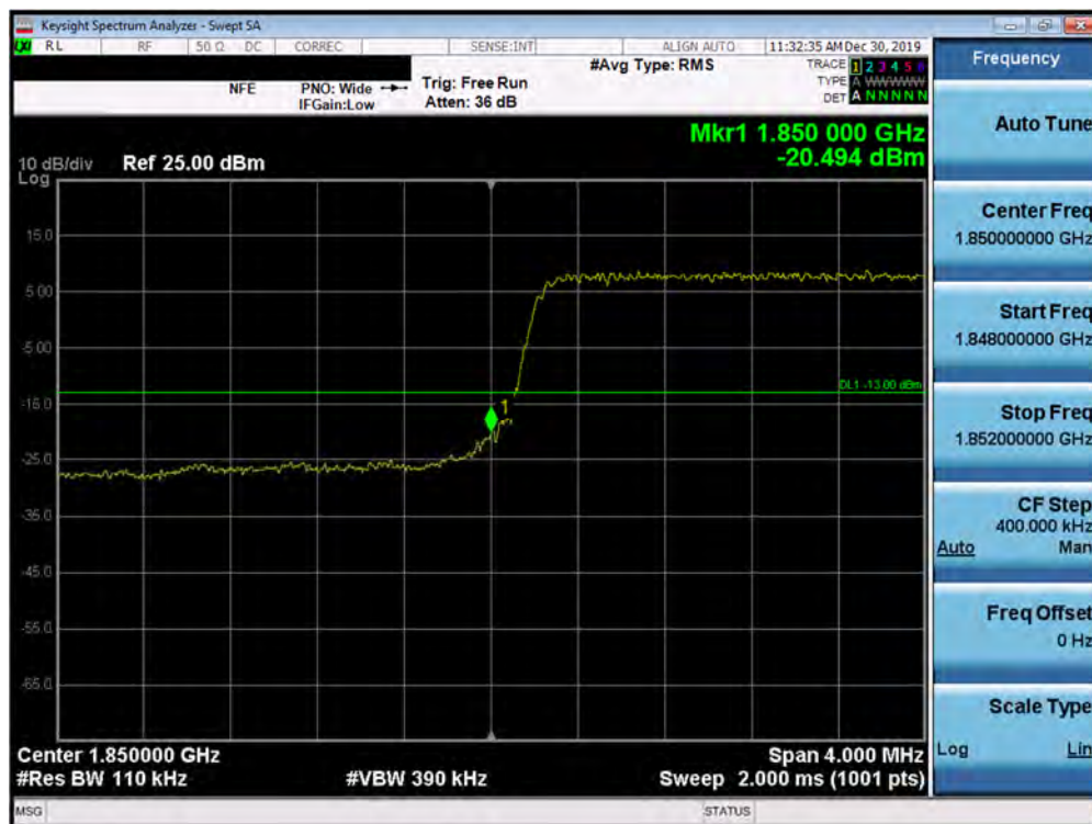
Plot 7-381. Lower Band Edge Plot (5G NR n2 - 5.0MHz QPSK - CP - Full RB Configuration)
