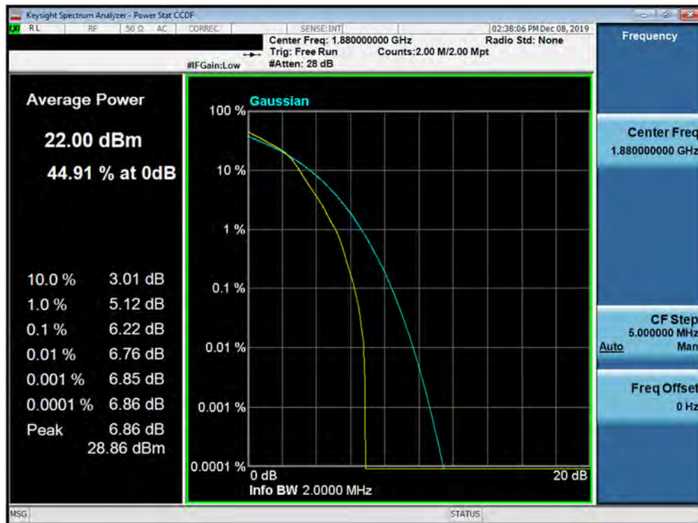
Plot 7-412. PAR Plot (Band 2 - 1.4MHz 16-QAM - Full RB Configuration)
