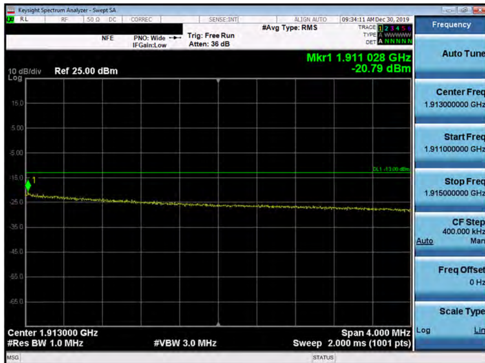
Plot 7-392. Upper Extended Band Edge Plot (5G NR n2 - 10.0MHz QPSK - DFT-s - Full RB Configuration)
