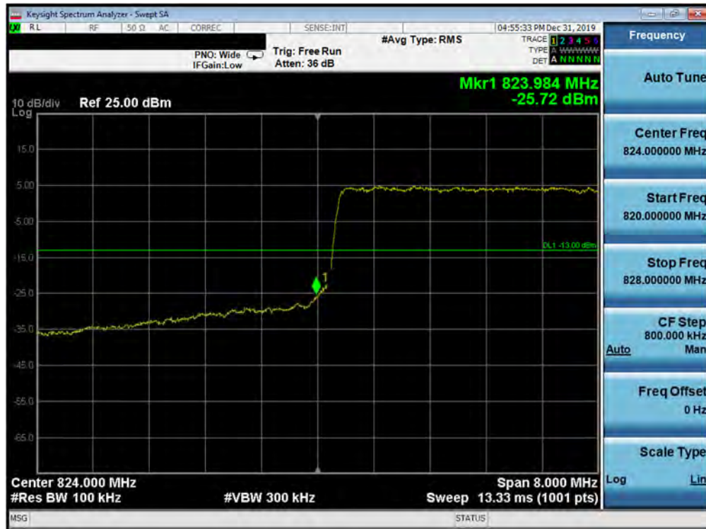
Plot 7-335. Lower Band Edge Plot (5G NR n5 - 10.0MHz QPSK - DFT-s - Full RB Configuration)
