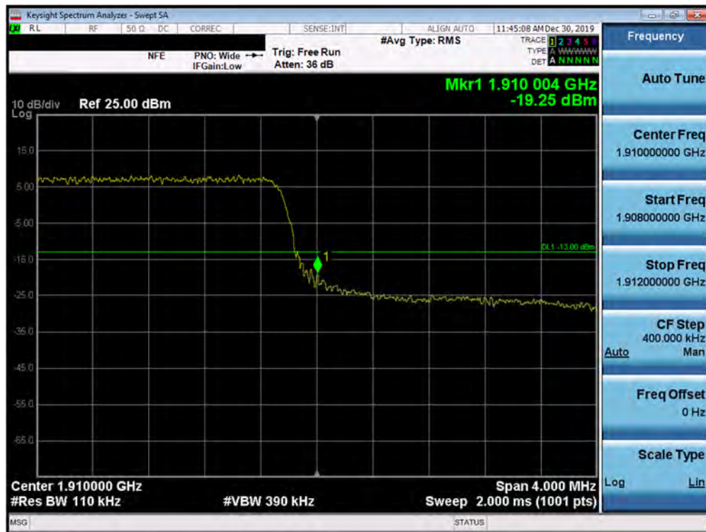
Plot 7-385. Upper Band Edge Plot (5G NR n2 - 5.0MHz QPSK - CP - Full RB Configuration)
