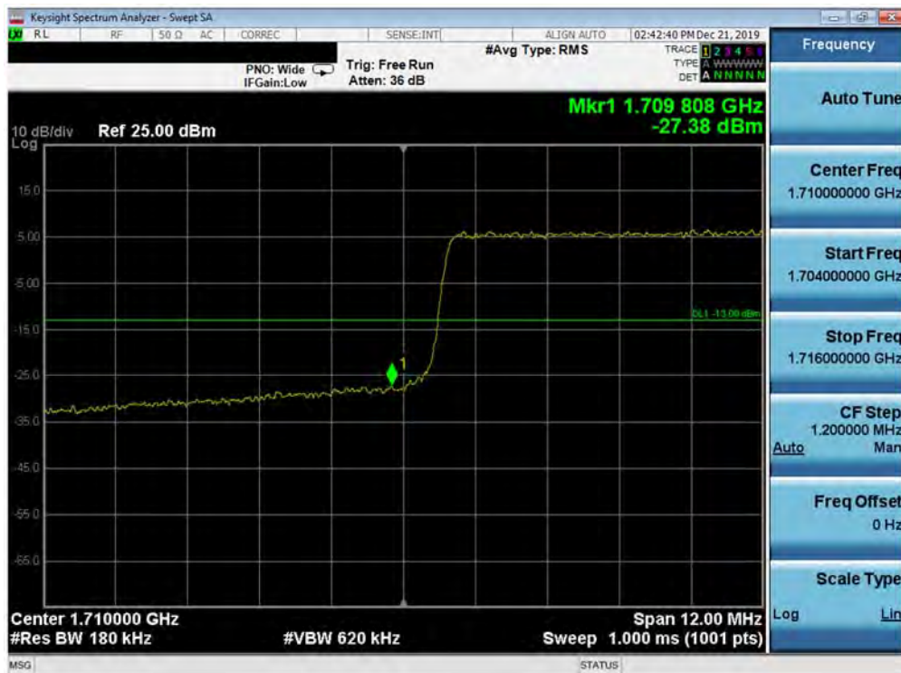
Plot 7-278. Lower Band Edge Plot (Band 66/4 - 15.0MHz QPSK - Full RB Configuration)
