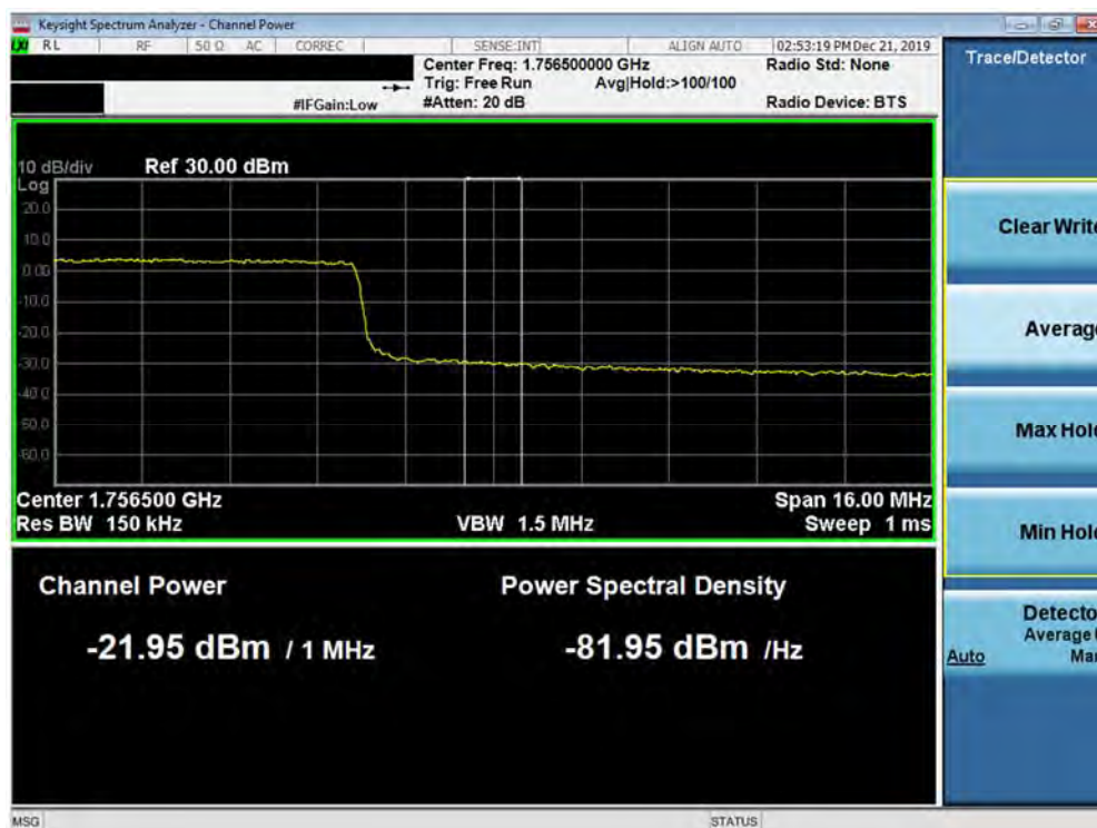
Plot 7-287. Upper Extended Band Edge Plot (Band 4 - 20.0MHz QPSK - Full RB Configuration)
