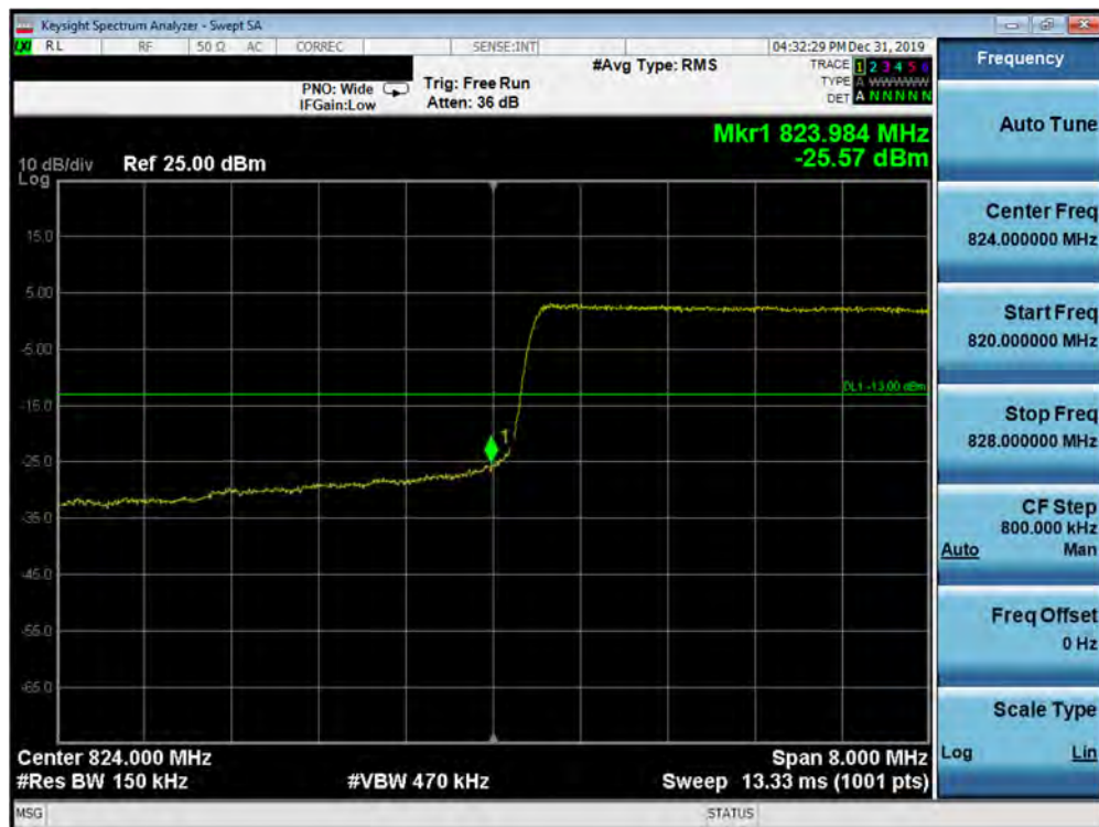
Plot 7-340. Lower Band Edge Plot (5G NR n5 - 15.0MHz QPSK - CP - Full RB Configuration)
