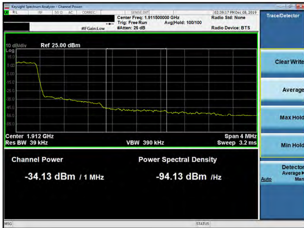
Plot 7-293. Upper Extended Band Edge Plot (Band 2 - 1.4MHz QPSK - Full RB Configuration)
