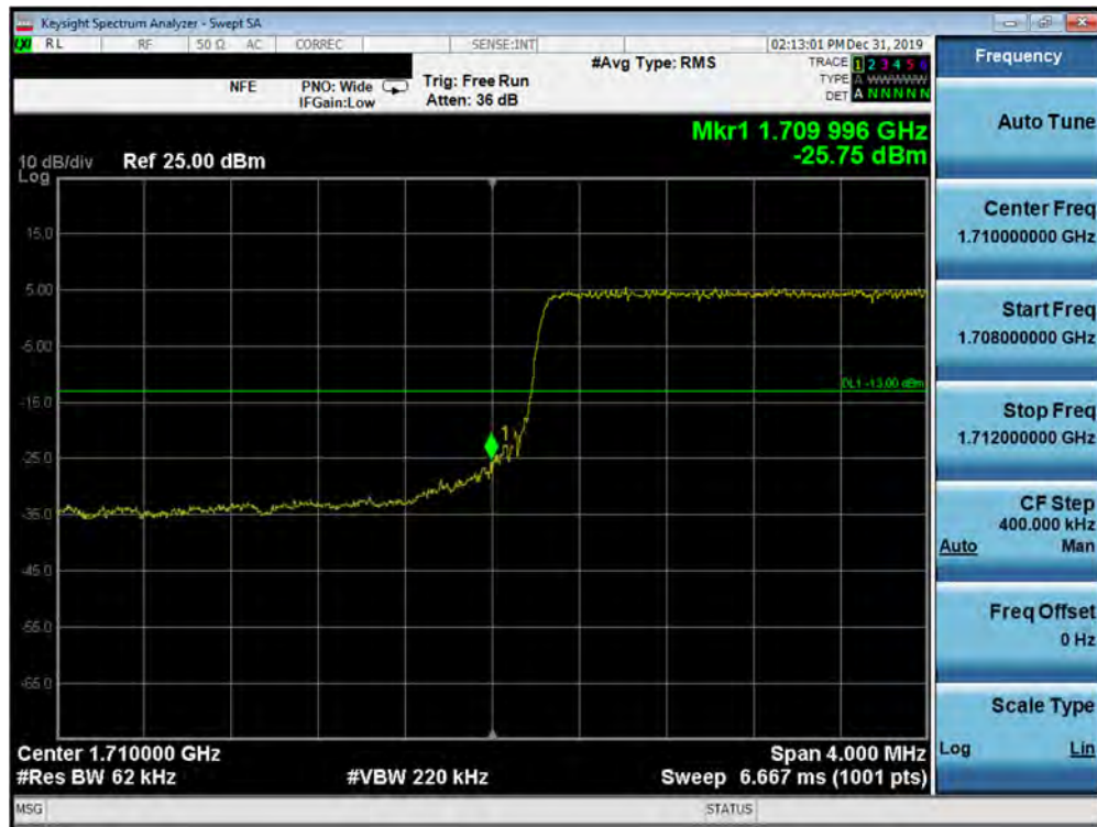
Plot 7-349. Lower Band Edge Plot (5G NR n66 - 5.0MHz QPSK - CP - Full RB Configuration)
