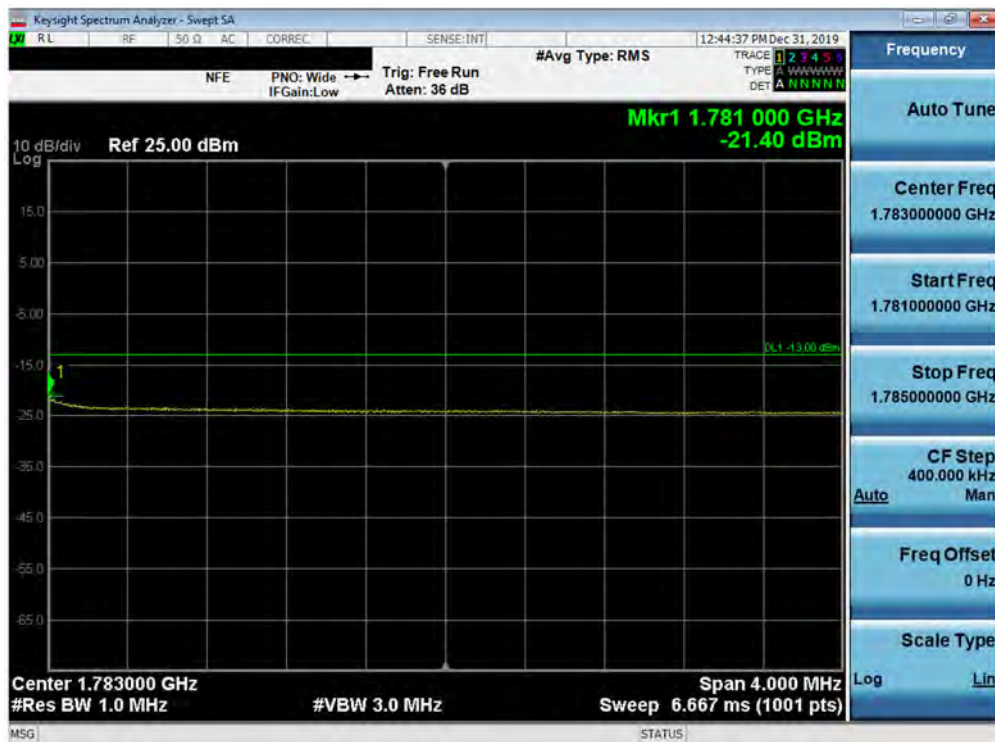
Plot 7-376. Upper Extended Band Edge Plot (5G NR n66 - 20.0MHz QPSK - DFT-s - Full RB Configuration)
