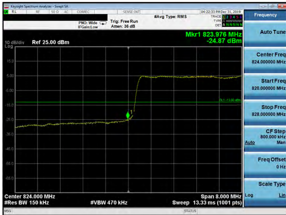
Plot 7-339. Lower Band Edge Plot (5G NR n5 - 15.0MHz QPSK - DFT-s - Full RB Configuration)
