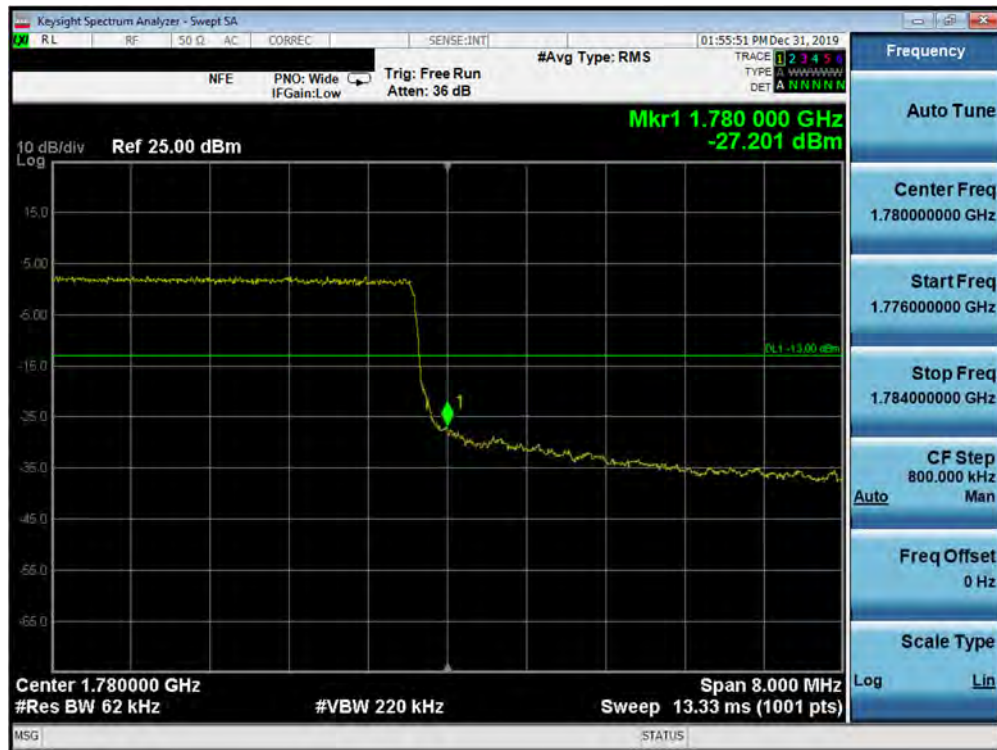
Plot 7-361. Upper Band Edge Plot (5G NR n66 - 10.0MHz QPSK - CP - Full RB Configuration)
