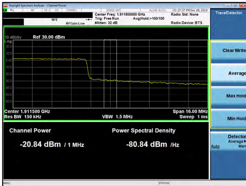
Plot 7-410. Upper Extended Band Edge Plot (5G NR n2 - 20.0MHz QPSK - CP - Full RB Configuration)
