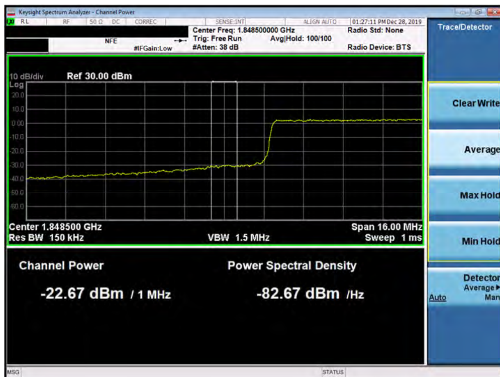
Plot 7-406. Lower Extended Band Edge Plot (5G NR n2 - 20.0MHz QPSK - CP - Full RB Configuration)
