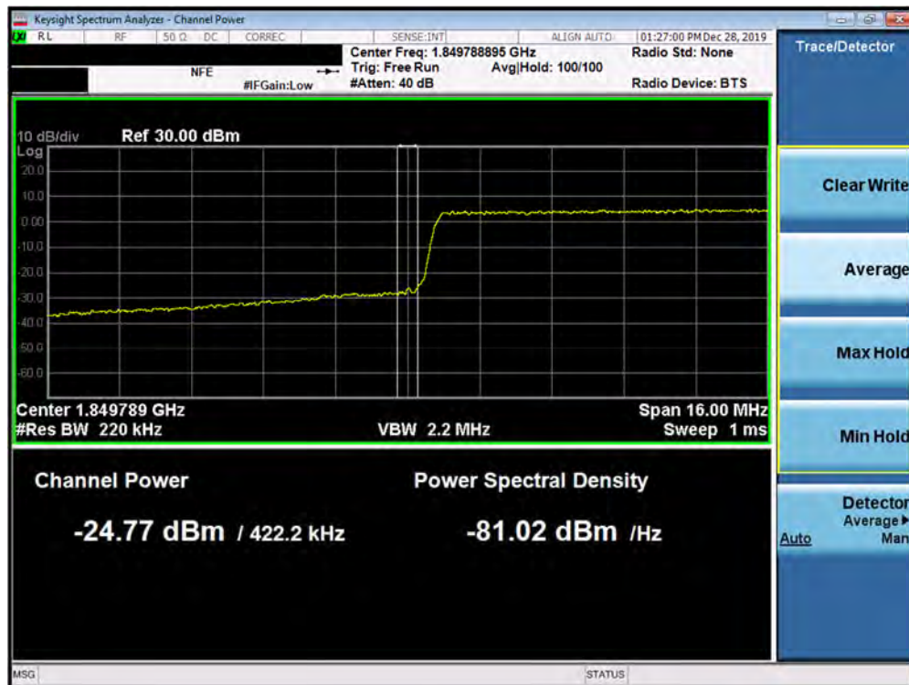
Plot 7-405. Lower Band Edge Plot (5G NR n2 - 20.0MHz QPSK - CP - Full RB Configuration)
