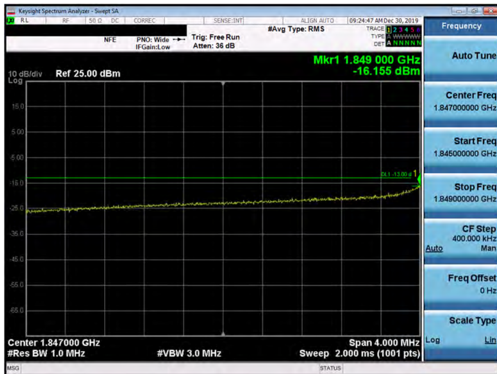
Plot 7-390. Lower Extended Band Edge Plot (5G NR n2 - 10.0MHz QPSK - CP - Full RB Configuration)
