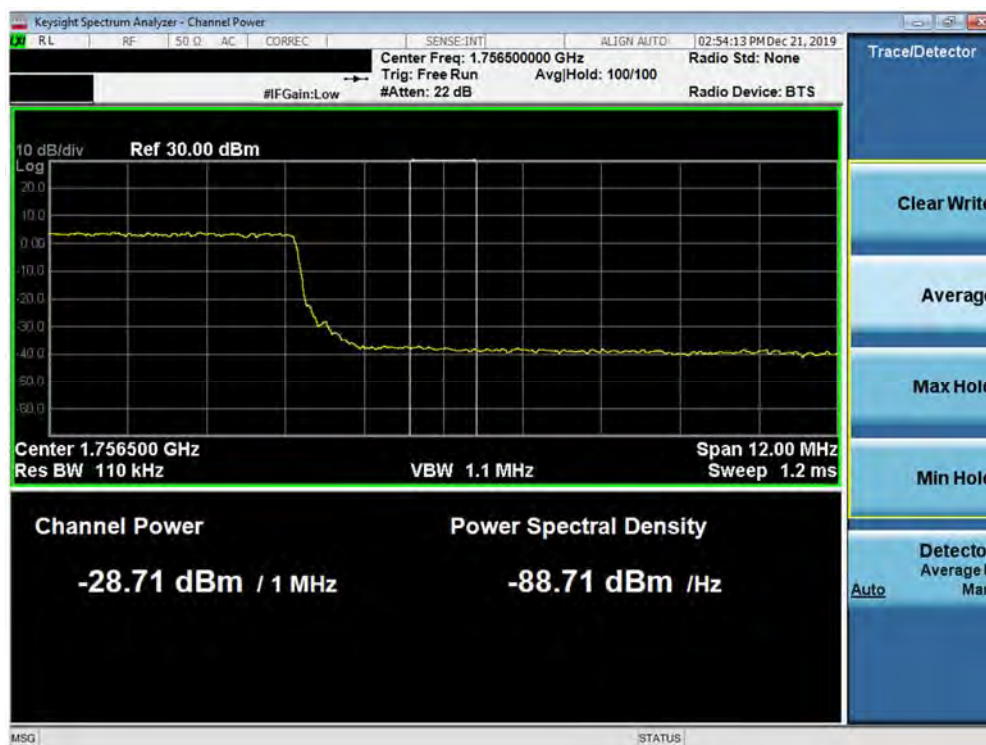
Plot 7-281. Upper Extended Band Edge Plot (Band 4 - 15.0MHz QPSK - Full RB Configuration)
