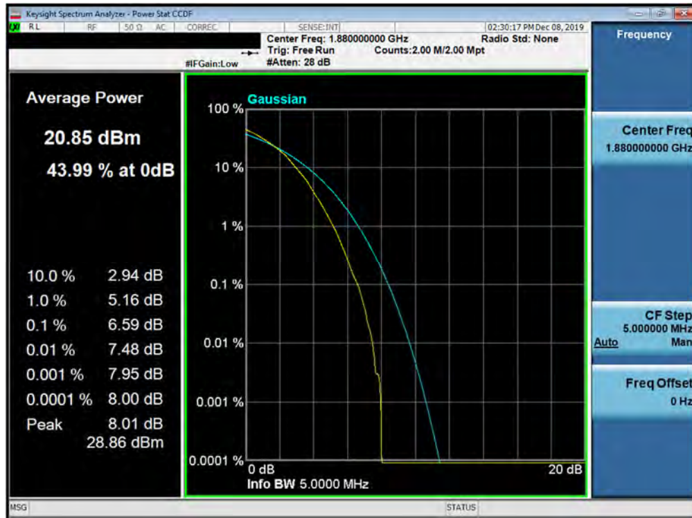
Plot 7-421. PAR Plot (Band 2 - 5.0MHz 64-QAM - Full RB Configuration)
