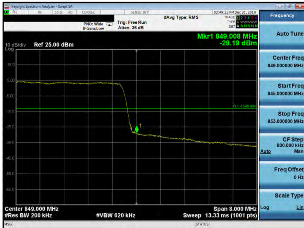
Plot 7-346. Upper Band Edge Plot (5G NR n5 - 20.0MHz QPSK - CP - Full RB Configuration)
