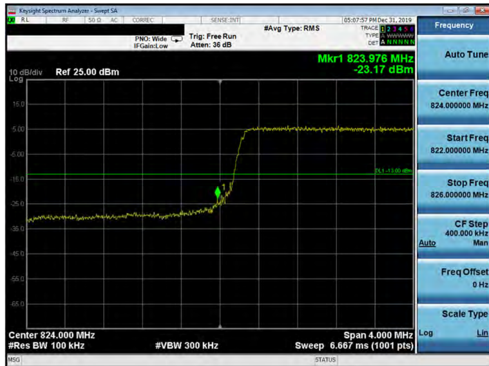
Plot 7-332. Lower Band Edge Plot (5G NR n5 - 5.0MHz QPSK - CP - Full RB Configuration)
