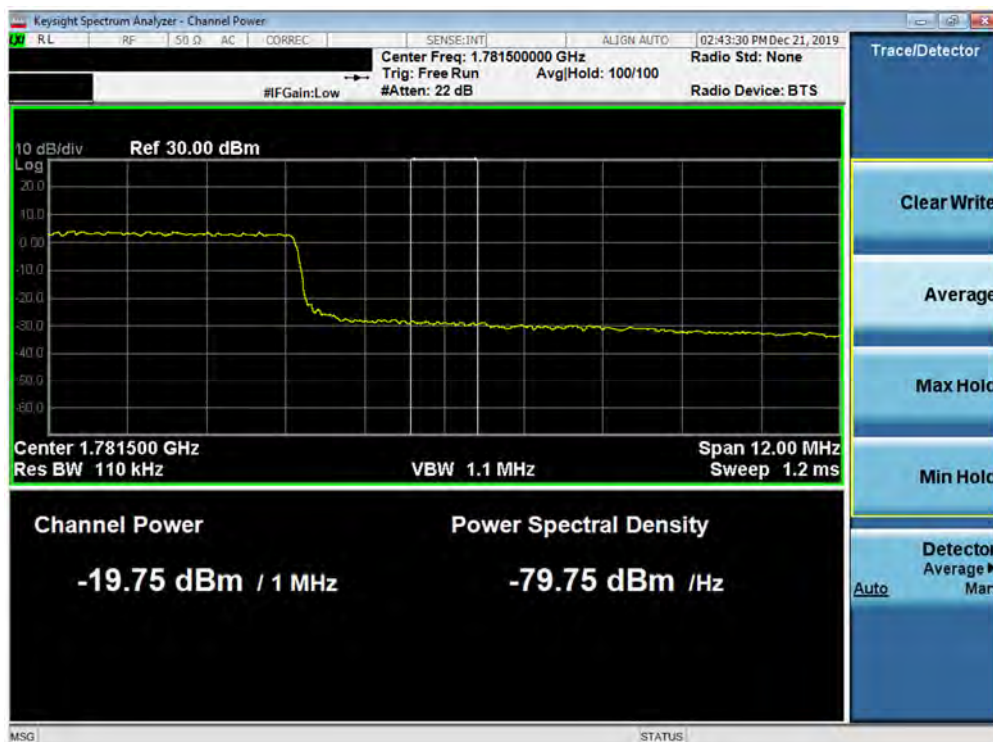
Plot 7-283. Upper Extended Band Edge Plot (Band 66 - 15.0MHz QPSK - Full RB Configuration)
