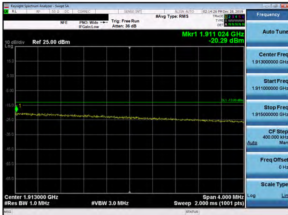
Plot 7-400. Upper Extended Band Edge Plot (5G NR n2 - 15.0MHz QPSK - DFT-s - Full RB Configuration)
