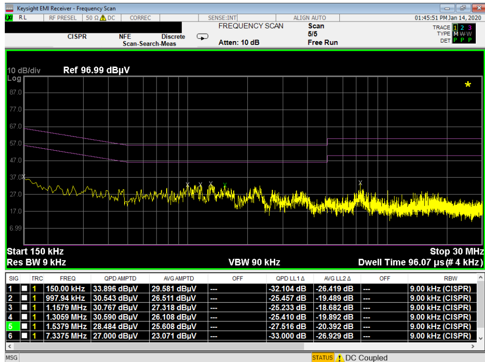
Plot 7-7. Line-Conducted Test Plot with Antenna Terminated in 50Ω (N)
