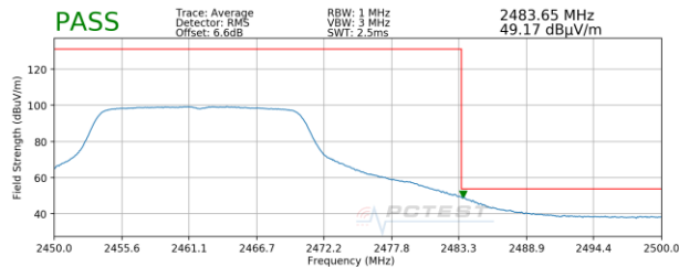
Plot 7-19. Radiated Restricted Upper Band Edge Measurement SISO ANT1 (Average)
