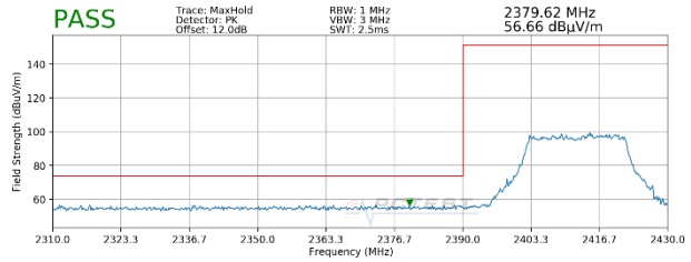
Plot 7-38. Radiated Restricted Lower Band Edge Measurement SISO ANT2 (Peak – 242 Tones)
