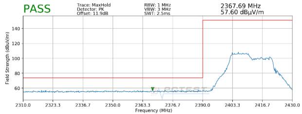
Plot 7-26. Radiated Restricted Lower Band Edge Measurement SISO ANT1 (Peak – 106 Tones)
