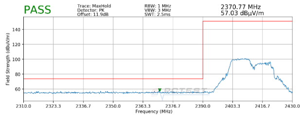
Plot 7-34. Radiated Restricted Lower Band Edge Measurement SISO ANT2 (Peak – 106 Tones)
