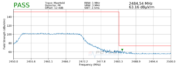
Plot 7-32. Radiated Restricted Upper Band Edge Measurement SISO ANT1 (Peak – 242 Tones)
