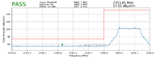
Plot 7-30. Radiated Restricted Lower Band Edge Measurement SISO ANT1 (Peak – 242 Tones)
