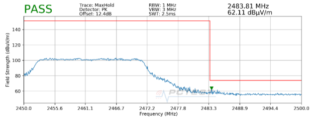
Plot 7-48. Radiated Restricted Upper Band Edge Measurement MIMO (Peak – 242 Tones)
