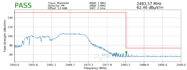
Plot 7-44. Radiated Restricted Upper Band Edge Measurement MIMO (Peak – 106 Tones)
