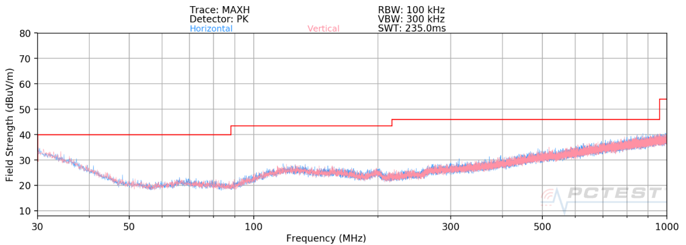
Plot 7-50. Radiated Spurious Plot below 1GHz MIMO (242 Tones)
