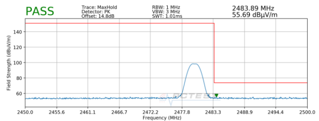
Plot 7-2. Radiated Restricted Upper Band Edge Measurement (Peak)
