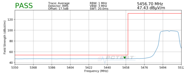
Plot 7-53. Radiated Lower Band Edge Plot SISO ANT2 (Average – UNII Band 2C)
