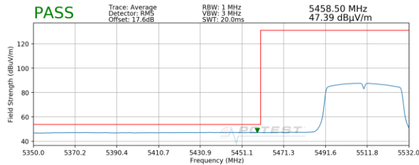
Plot 7-39. Radiated Lower Band Edge Plot SISO ANT1 (Average – UNII Band 2C)
