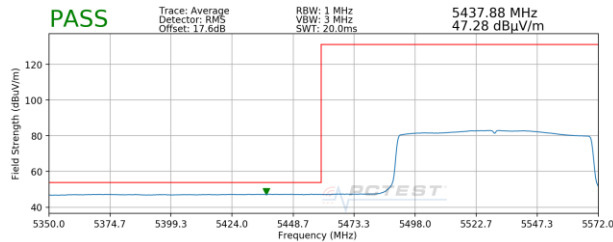
Plot 7-46. Radiated Lower Band Edge Plot SISO ANT1 (Average – UNII Band 2C)
