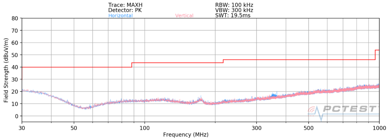
Plot 7-99. Radiated Spurious Plot below 1GHz (5GHz – 2.4 GHz)
