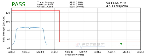
Plot 7-37. Radiated Upper Band Edge Plot SISO ANT1 (Average - UNII Band 2A)
