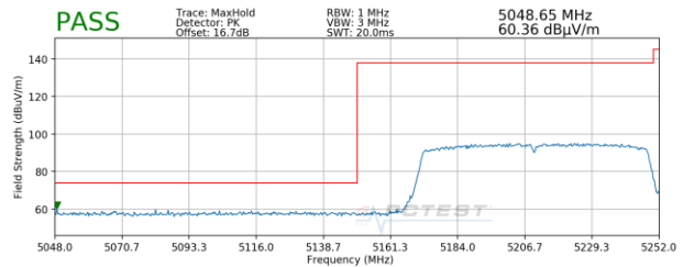
Plot 7-64. Radiated Lower Band Edge Plot SISO ANT2 (Peak - UNII Band 1)
