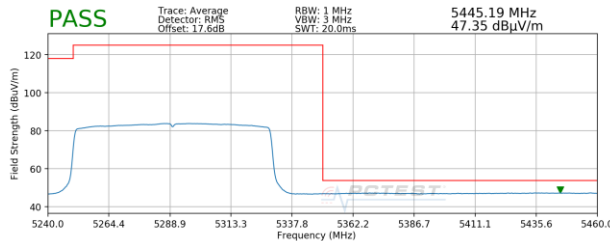
Plot 7-65. Radiated Upper Band Edge Plot SISO ANT2 (Average - UNII Band 2A)
