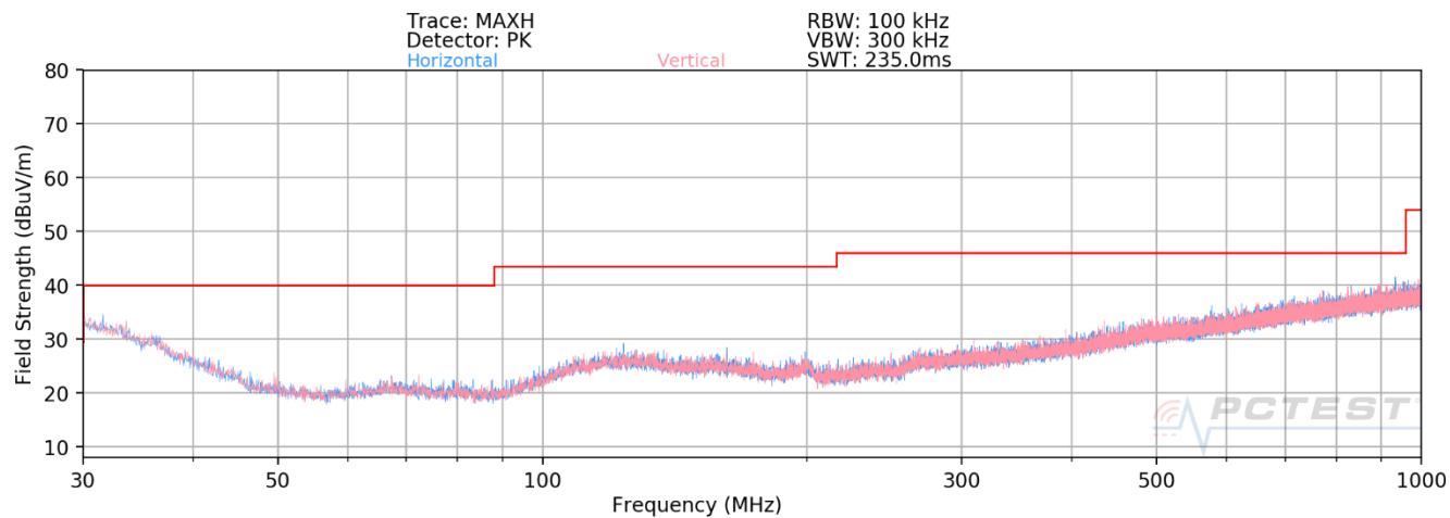
Plot 7-97. Radiated Spurious Plot below 1GHz SISO ANT2 (802.11a – U3 Ch. 157)
