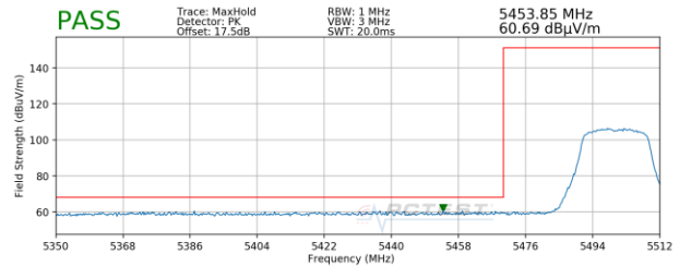
Plot 7-33. Radiated Lower Band Edge Plot SISO ANT1 (Peak – UNII Band 2C)
