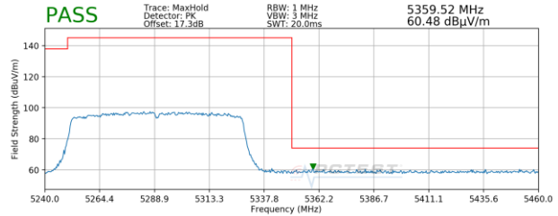
Plot 7-91. Radiated Upper Band Edge Plot MIMO (Peak – UNII Band 2A)
