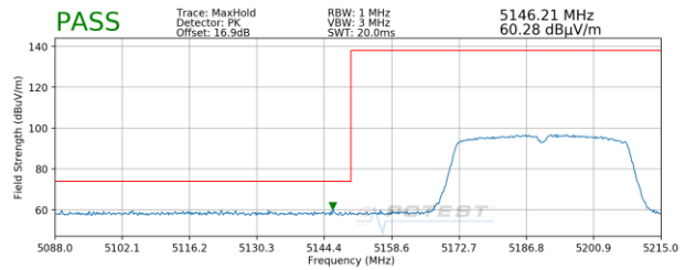
Plot 7-36. Radiated Lower Band Edge Plot SISO ANT1 (Peak - UNII Band 1)
