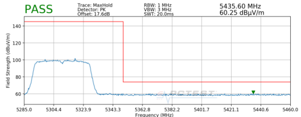
Plot 7-82. Radiated Upper Band Edge Plot MIMO (Peak – UNII Band 2A)
