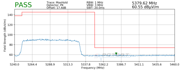
Plot 7-45. Radiated Upper Band Edge Plot SISO ANT1 (Peak - UNII Band 2A)
