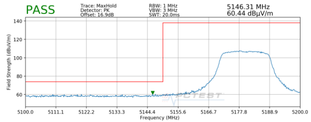
Plot 7-50. Radiated Lower Band Edge Plot SISO ANT2 (Peak - UNII Band 1)
