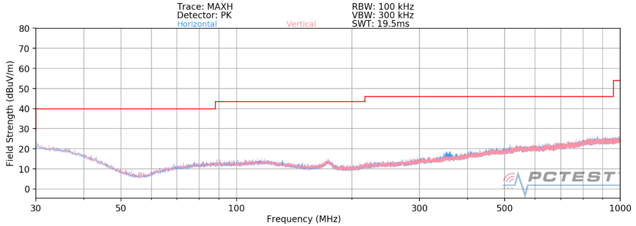
Plot 7-98. Radiated Spurious Plot below 1GHz (2.4GHz – 5GHz)
