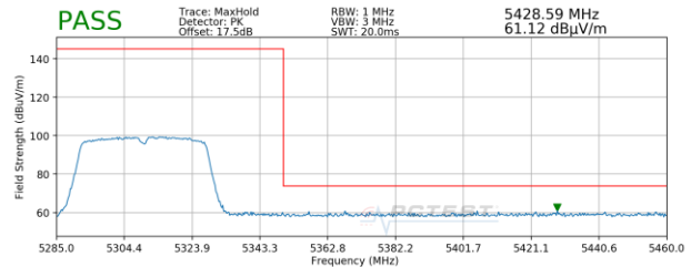
Plot 7-59. Radiated Upper Band Edge Plot SISO ANT2 (Peak - UNII Band 2A)
