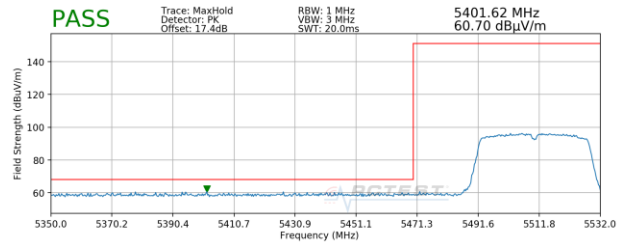
Plot 7-61. Radiated Lower Band Edge Plot SISO ANT2 (Peak – UNII Band 2C)
