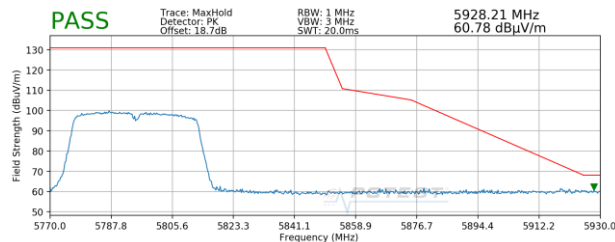
Plot 7-62. Radiated Upper Band Edge Plot SISO ANT2 (Peak – UNII Band 3)
