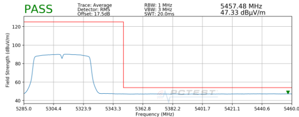
Plot 7-58. Radiated Upper Band Edge Plot SISO ANT2 (Average - UNII Band 2A)
