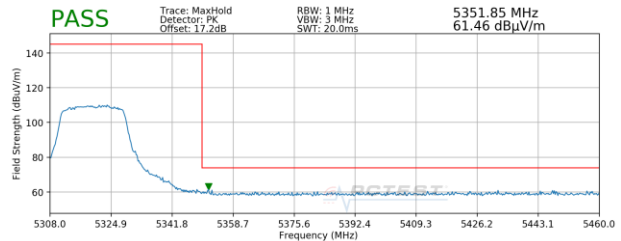
Plot 7-73. Radiated Upper Band Edge Plot MIMO (Peak – UNII Band 2A)
