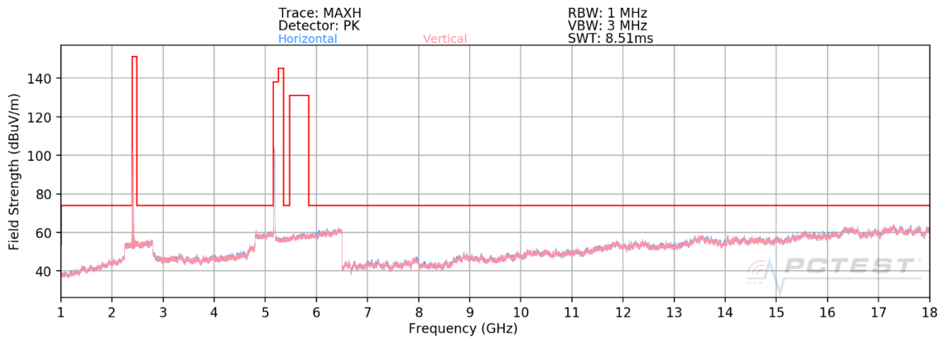
Plot 7-22. Radiated Spurious Plot above 1GHz (5GHz - 2.4 GHz)
