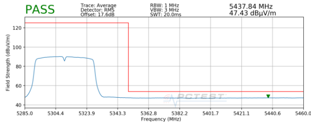
Plot 7-81. Radiated Upper Band Edge Plot MIMO (Average – UNII Band 2A)
