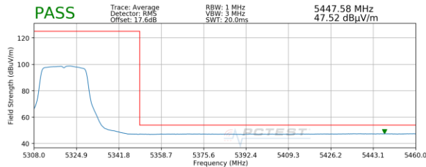
Plot 7-51. Radiated Upper Band Edge Plot SISO ANT2 (Average - UNII Band 2A)
