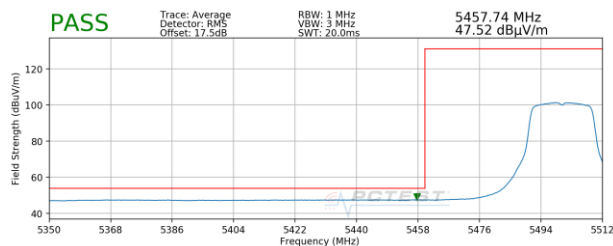
Plot 7-74. Radiated Lower Band Edge Plot MIMO (Average – UNII Band 2C)
