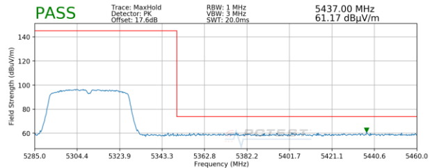
Plot 7-38. Radiated Upper Band Edge Plot SISO ANT1 (Peak - UNII Band 2A)
