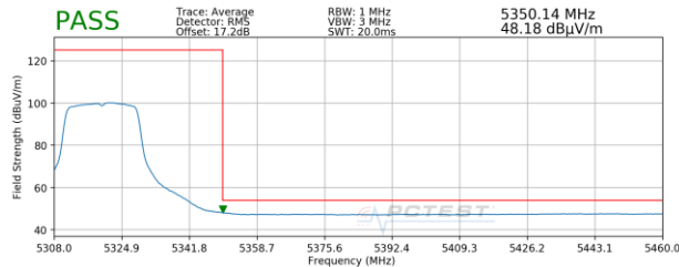
Plot 7-72. Radiated Upper Band Edge Plot MIMO (Average – UNII Band 2A)
