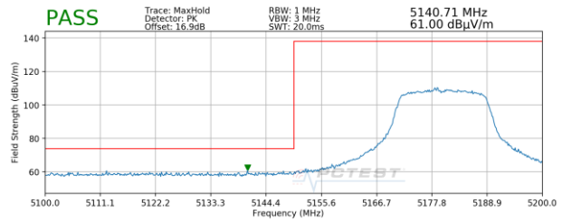
Plot 7-71. Radiated Lower Band Edge Plot MIMO (Peak – UNII Band 1)
