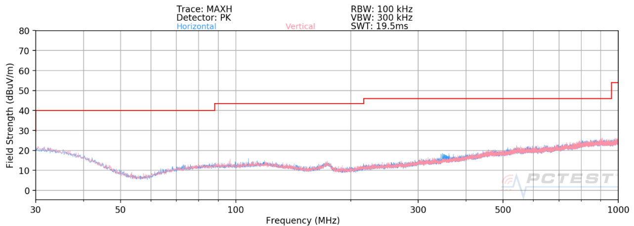
Plot 7-100. Radiated Spurious Plot below 1GHz (Dual Band Simult. Tx)
