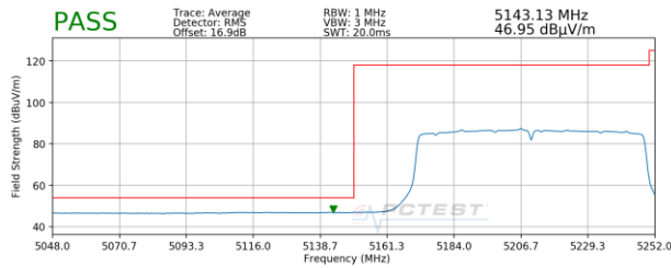
Plot 7-88. Radiated Lower Band Edge Plot MIMO (Average – UNII Band 1)
