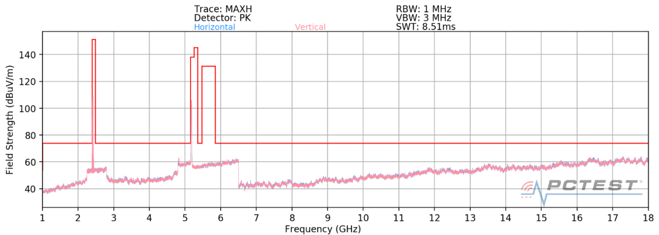
Plot 7-25. Radiated Spurious Plot above 1GHz (Dual Band Simult. Tx)
