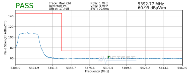
Plot 7-52. Radiated Upper Band Edge Plot SISO ANT2 (Peak - UNII Band 2A)
