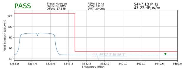
Plot 7-86. Radiated Band Edge Plot MIMO (Average – WCP + DD)
