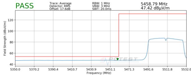
Plot 7-83. Radiated Lower Band Edge Plot MIMO (Average – UNII Band 2C)
