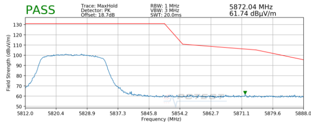
Plot 7-34. Radiated Upper Band Edge Plot SISO ANT1 (Peak – UNII Band 3)
