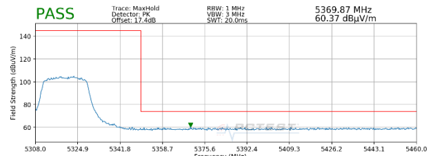
Plot 7-78. Radiated Band Edge Plot SISO ANT2 (Peak – WCP + DD)
