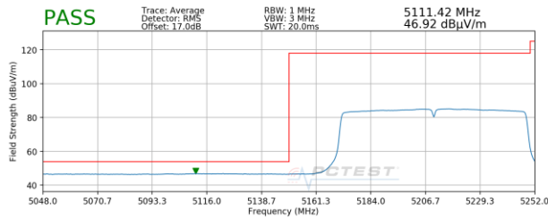
Plot 7-42. Radiated Lower Band Edge Plot SISO ANT1 (Average - UNII Band 1)
