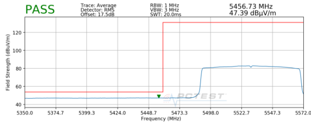
Plot 7-67. Radiated Lower Band Edge Plot SISO ANT2 (Average – UNII Band 2C)
