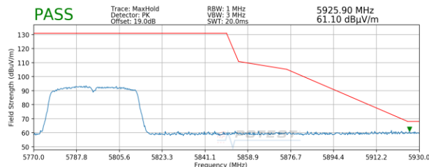
Plot 7-41. Radiated Upper Band Edge Plot SISO ANT1 (Peak – UNII Band 3)
