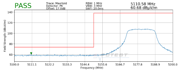
Plot 7-29. Radiated Lower Band Edge Plot SISO ANT1 (Peak - UNII Band 1)
