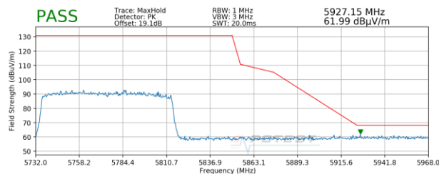
Plot 7-69. Radiated Upper Band Edge Plot SISO ANT2 (Peak – UNII Band 3)
