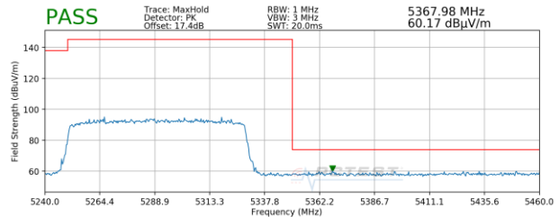
Plot 7-66. Radiated Upper Band Edge Plot SISO ANT2 (Peak - UNII Band 2A)
