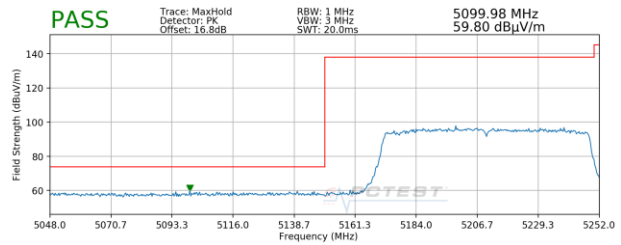
Plot 7-89. Radiated Lower Band Edge Plot MIMO (Peak – UNII Band 1)
