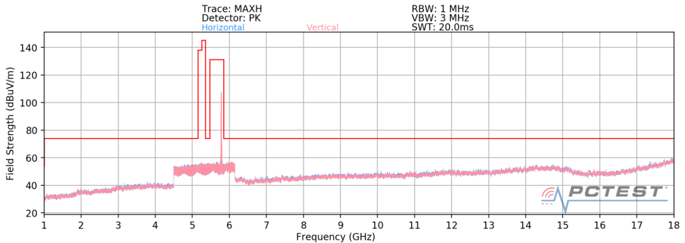
Plot 7-16. Radiated Spurious Plot above 1GHz MIMO/CDD (802.11a – U3 Ch. 157)
