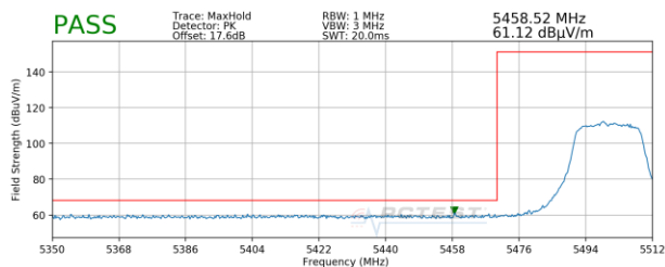
Plot 7-75. Radiated Lower Band Edge Plot MIMO (Peak – UNII Band 2C)
