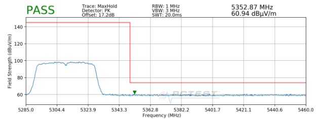
Plot 7-87. Radiated Band Edge Plot MIMO (Peak – WCP + DD)
