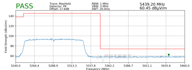
Plot 7-96. Radiated Band Edge Plot MIMO (Peak – WCP)
