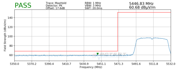
Plot 7-40. Radiated Lower Band Edge Plot SISO ANT1 (Peak – UNII Band 2C)
