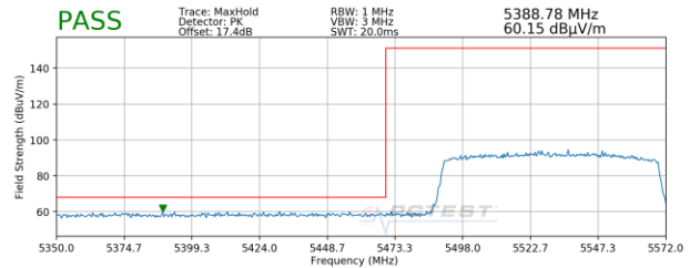
Plot 7-68. Radiated Lower Band Edge Plot SISO ANT2 (Peak – UNII Band 2C)
