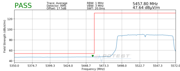
Plot 7-92. Radiated Lower Band Edge Plot MIMO (Average – UNII Band 2C)
