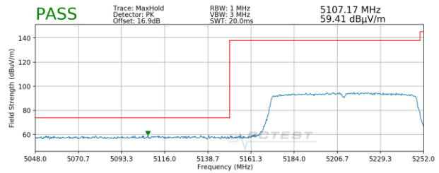
Plot 7-43. Radiated Lower Band Edge Plot SISO ANT1 (Peak - UNII Band 1)
