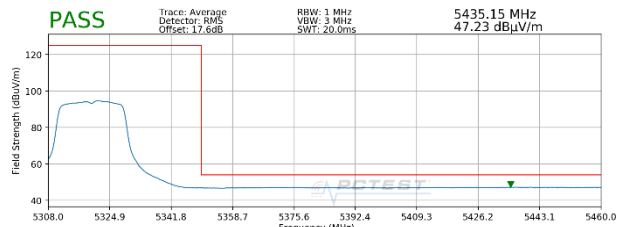
Plot 7-77. Radiated Band Edge Plot SISO ANT2 (Average – WCP + DD)
