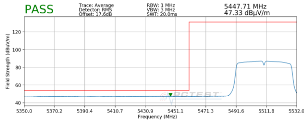
Plot 7-60. Radiated Lower Band Edge Plot SISO ANT2 (Average – UNII Band 2C)
