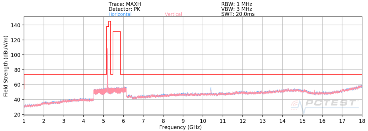
Plot 7-13. Radiated Spurious Plot above 1GHz MIMO/CDD (802.11a – U1 Ch. 40)
