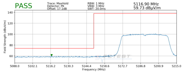
Plot 7-80. Radiated Lower Band Edge Plot MIMO (Peak – UNII Band 1)
