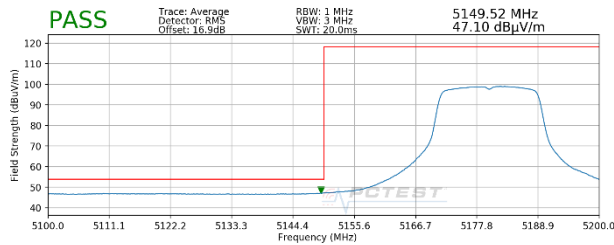
Plot 7-28. Radiated Lower Band Edge Plot SISO ANT1 (Average - UNII Band 1)
