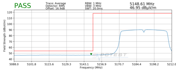
Plot 7-79. Radiated Lower Band Edge Plot MIMO (Average – UNII Band 1)
