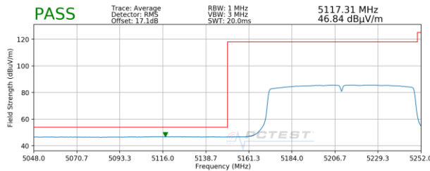
Plot 7-63. Radiated Lower Band Edge Plot SISO ANT2 (Average - UNII Band 1)
