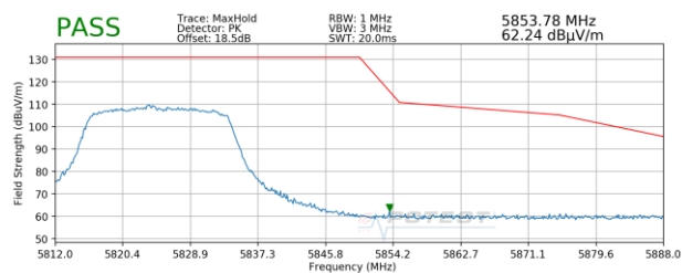
Plot 7-76. Radiated Upper Band Edge Plot MIMO (Peak – UNII Band 3)
