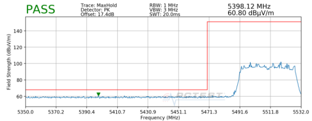
Plot 7-84. Radiated Lower Band Edge Plot MIMO (Peak – UNII Band 2C)
