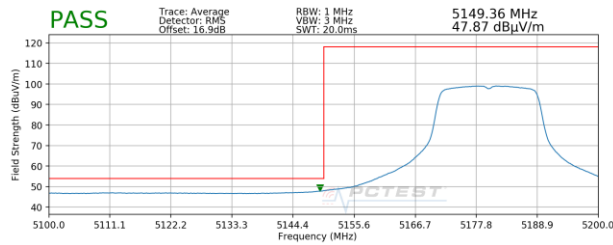
Plot 7-70. Radiated Lower Band Edge Plot MIMO (Average – UNII Band 1)
