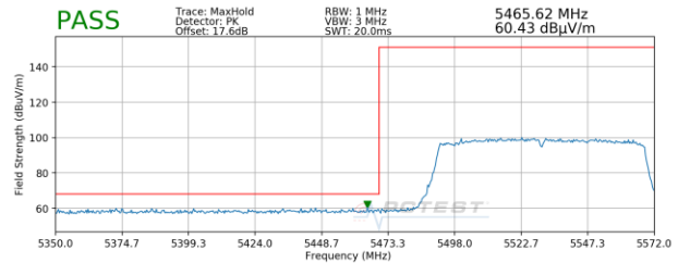
Plot 7-93. Radiated Lower Band Edge Plot MIMO (Peak – UNII Band 2C)
