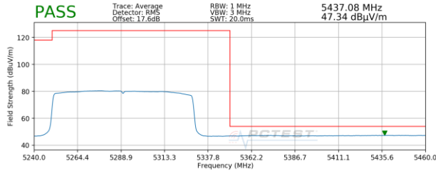
Plot 7-44. Radiated Upper Band Edge Plot SISO ANT1 (Average - UNII Band 2A)
