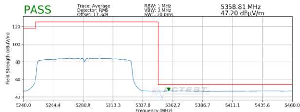
Plot 7-95. Radiated Band Edge Plot MIMO (Average – WCP)
