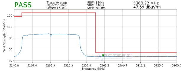
Plot 7-90. Radiated Upper Band Edge Plot MIMO (Average – UNII Band 2A)
