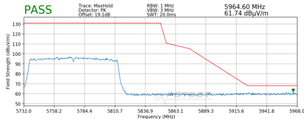
Plot 7-94. Radiated Upper Band Edge Plot MIMO (Peak – UNII Band 3)
