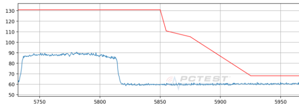
Plot 7-48. Radiated Upper Band Edge Plot SISO ANT1 (Peak – UNII Band 3)
