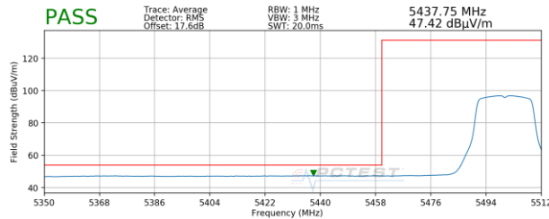
Plot 7-32. Radiated Lower Band Edge Plot SISO ANT1 (Average – UNII Band 2C)
