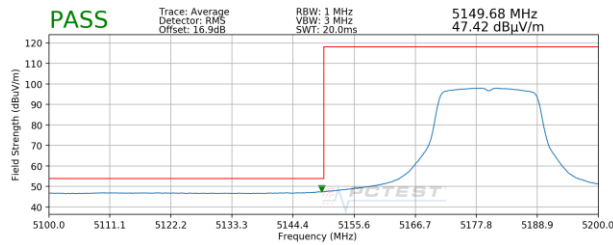
Plot 7-49. Radiated Lower Band Edge Plot SISO ANT2 (Average - UNII Band 1)
