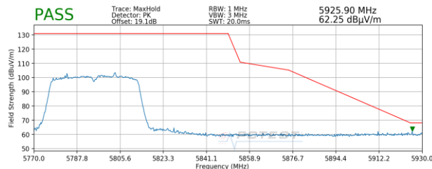
Plot 7-85. Radiated Upper Band Edge Plot MIMO (Peak – UNII Band 3)
