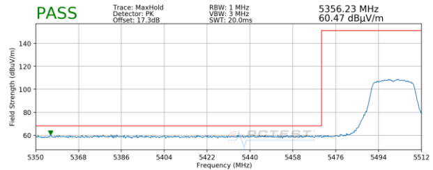
Plot 7-54. Radiated Lower Band Edge Plot SISO ANT2 (Peak – UNII Band 2C)
