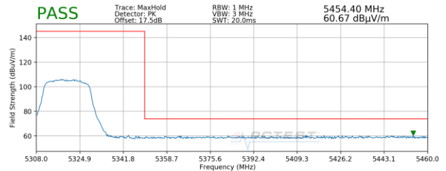
Plot 7-31. Radiated Upper Band Edge Plot SISO ANT1 (Peak - UNII Band 2A)
