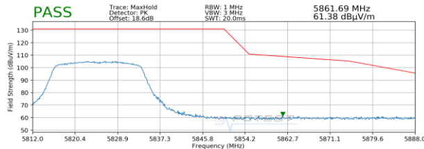
Plot 7-55. Radiated Upper Band Edge Plot SISO ANT2 (Peak – UNII Band 3)
