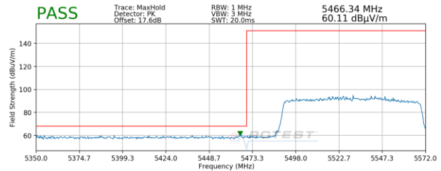
Plot 7-47. Radiated Lower Band Edge Plot SISO ANT1 (Peak – UNII Band 2C)
