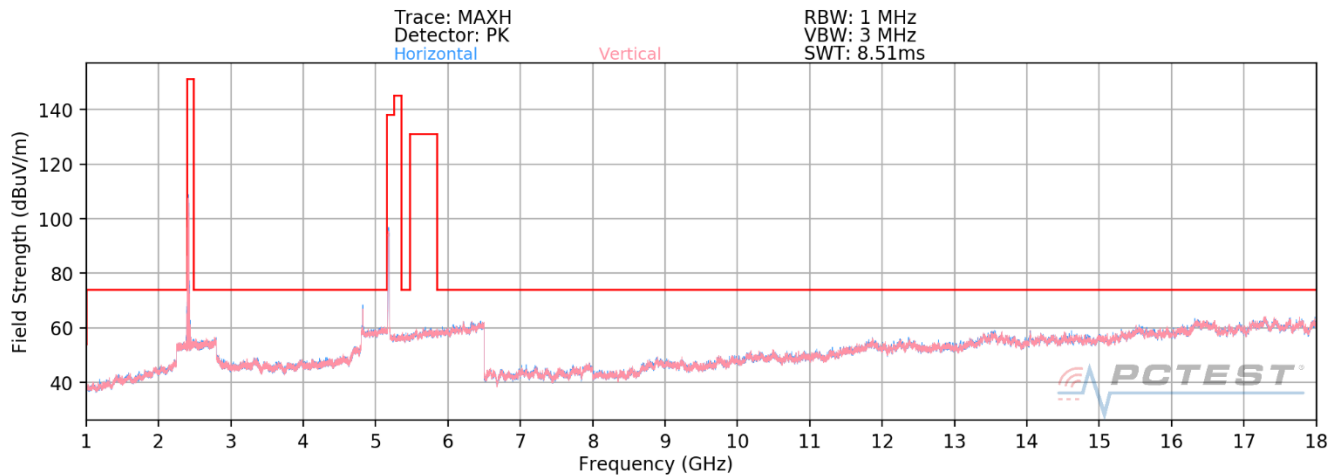
Plot 7-19. Radiated Spurious Plot above 1GHz (2.4GHz – 5GHz)
