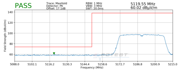
Plot 7-57. Radiated Lower Band Edge Plot SISO ANT2 (Peak - UNII Band 1)
