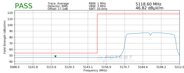
Plot 7-35. Radiated Lower Band Edge Plot SISO ANT1 (Average - UNII Band 1)
