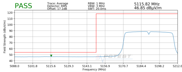
Plot 7-56. Radiated Lower Band Edge Plot SISO ANT2 (Average - UNII Band 1)
