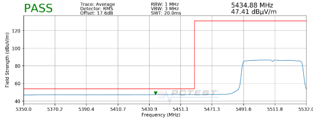
Plot 7-69. Radiated Lower Band Edge Plot SISO ANT2 (Average – UNII Band 2C – 484 Tones)
