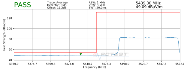
Plot 7-97. Radiated Lower Band Edge Plot MIMO (Average - UNII Band 2C - 996 Tones)
