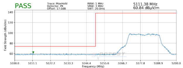
Plot 7-38. Radiated Lower Band Edge Plot SISO ANT1 (Peak – UNII Band 1 – 242 Tones)
