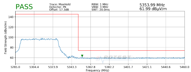
Plot 7-68. Radiated Upper Band Edge Plot SISO ANT2 (Peak – UNII Band 2A – 484 Tones)
