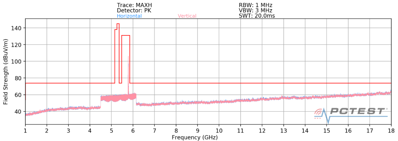
Plot 7-28. Radiated Spurious Plot above 1GHz MIMO (802.11ax – U3 Ch. 157 – 26 Tones)
