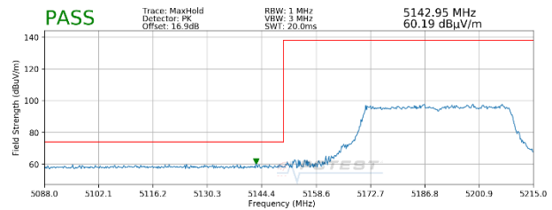
Plot 7-66. Radiated Lower Band Edge Plot SISO ANT2 (Peak – UNII Band 1 – 484 Tones)
