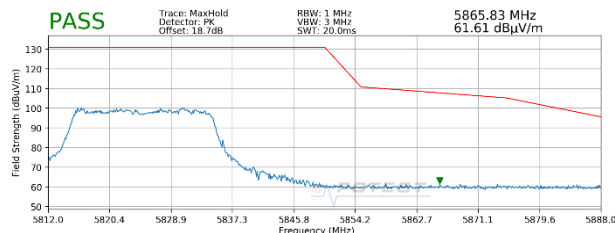
Plot 7-64. Radiated Upper Band Edge Plot SISO ANT2 (Peak - UNII Band 3 - 242 Tones)
