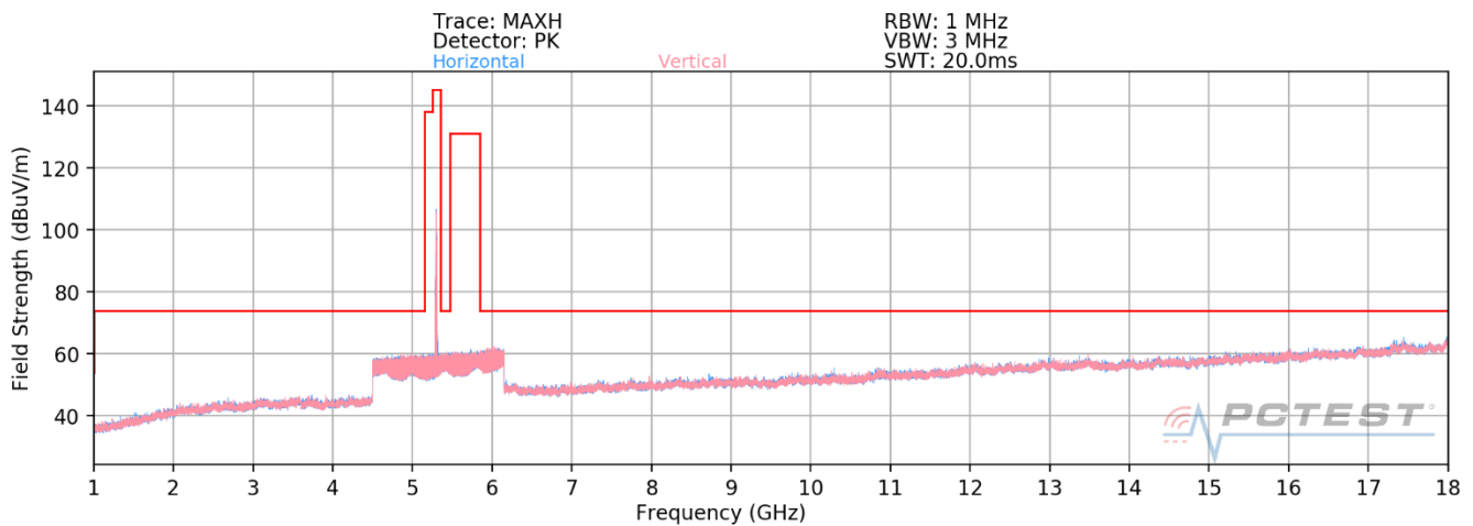
Plot 7-26. Radiated Spurious Plot above 1GHz MIMO (802.11ax – U2A Ch. 56 – 26 Tones)
