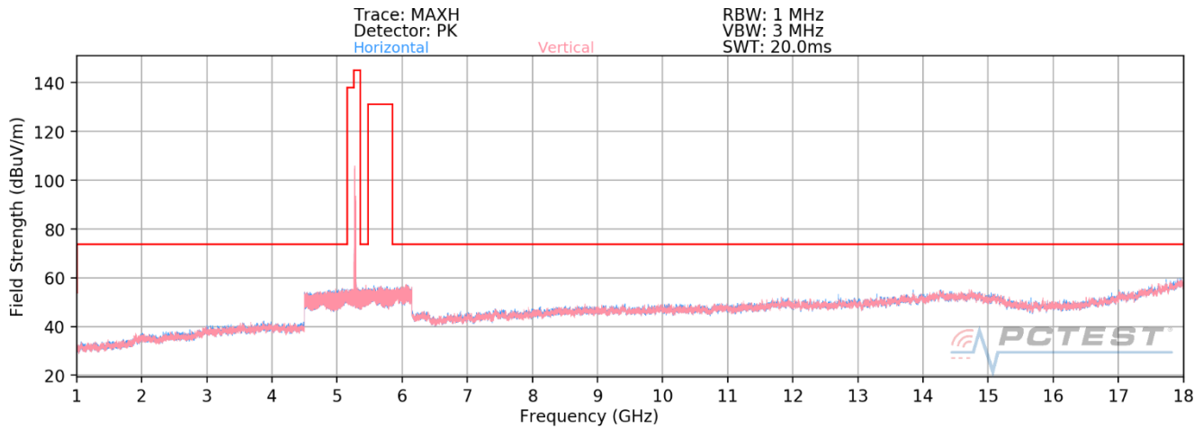
Plot 7-2. Radiated Spurious Plot above 1GHz SISO ANT1 (802.11ax – U2A Ch. 56 – 26 Tones)
