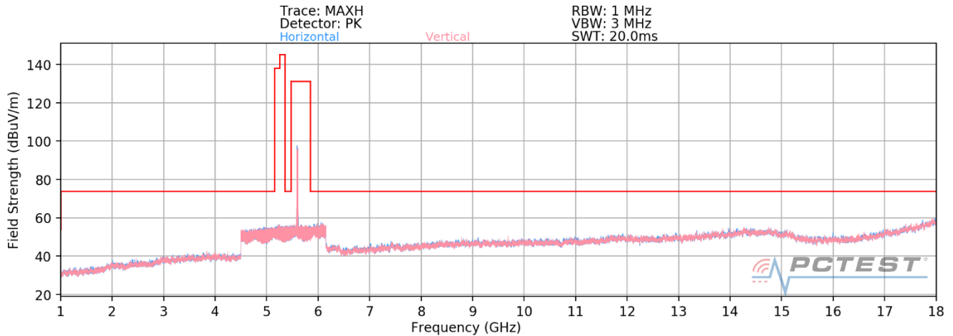
Plot 7-9. Radiated Spurious Plot above 1GHz SISO ANT1 (802.11ax – U2C Ch. 120 – 242 Tones)
