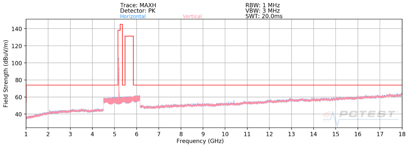
Plot 7-25. Radiated Spurious Plot above 1GHz MIMO (802.11ax – U1 Ch. 40 – 26 Tones)
