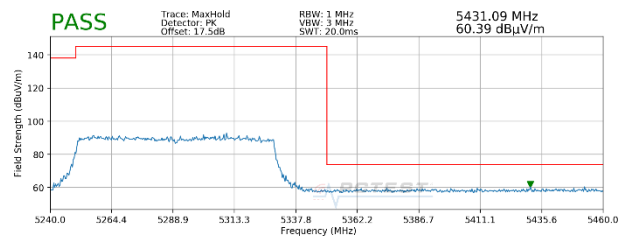
Plot 7-54. Radiated Upper Band Edge Plot SISO ANT1 (Peak – UNII Band 2A – 996 Tones)
