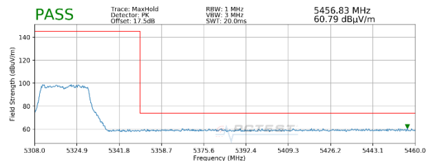
Plot 7-40. Radiated Upper Band Edge Plot SISO ANT1 (Peak – UNII Band 2A – 242 Tones)
