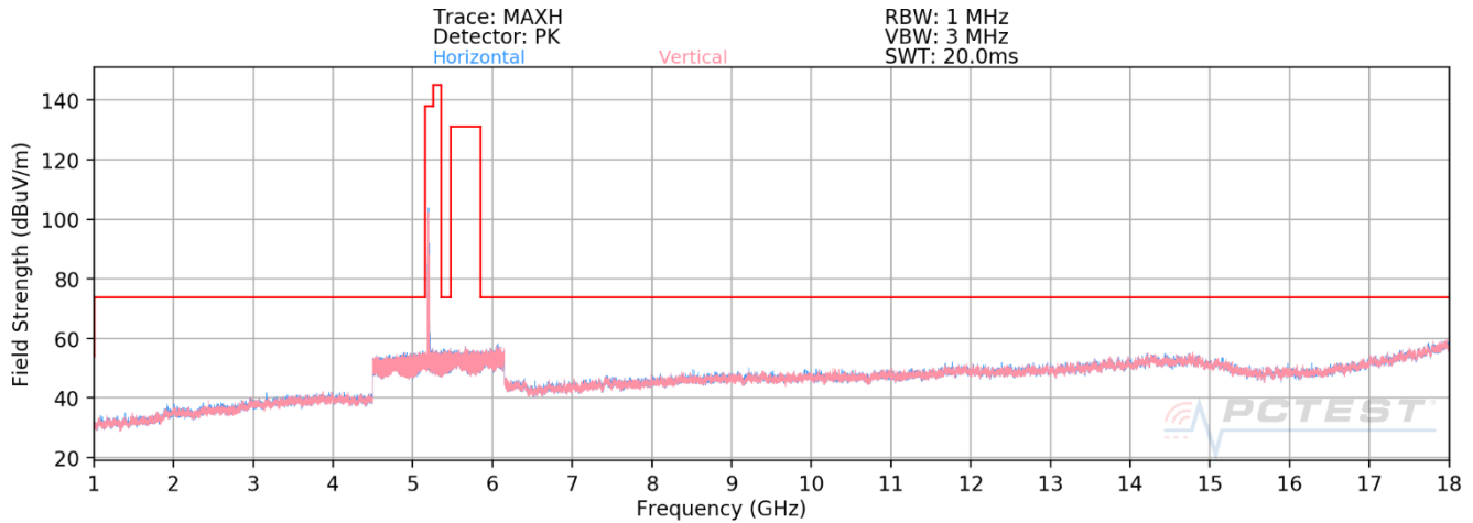
Plot 7-1. Radiated Spurious Plot above 1GHz SISO ANT1 (802.11ax – U1 Ch. 40 – 26 Tones)
