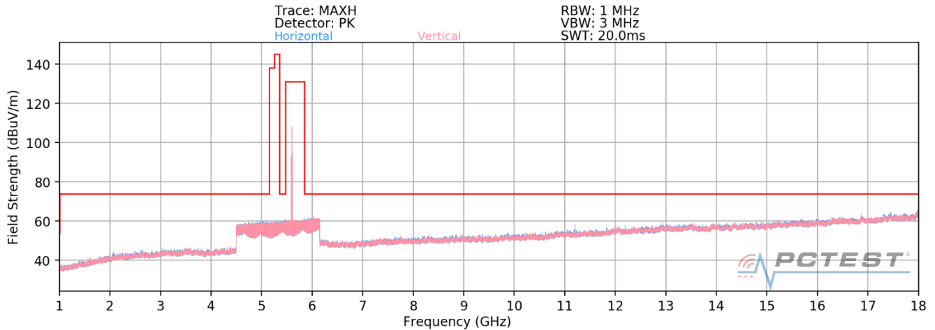
Plot 7-15. Radiated Spurious Plot above 1GHz SISO ANT2 (802.11ax – U2C Ch. 120 – 26 Tones)
