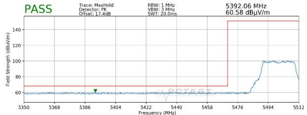
Plot 7-63. Radiated Lower Band Edge Plot SISO ANT2 (Peak - UNII Band 2C - 242 Tones)
