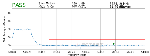
Plot 7-61. Radiated Upper Band Edge Plot SISO ANT2 (Peak – UNII Band 2A – 242 Tones)
