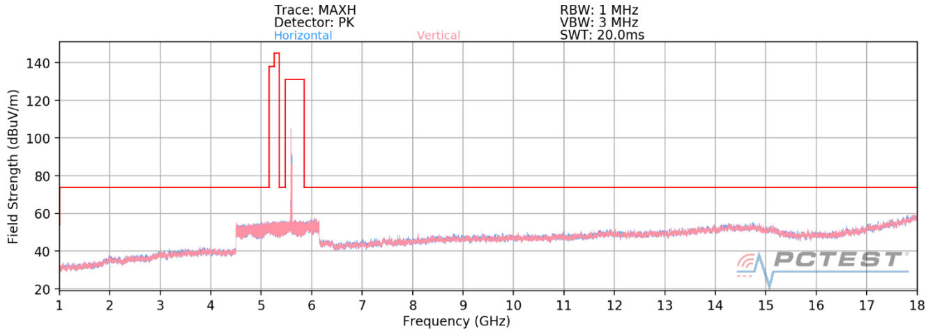
Plot 7-3. Radiated Spurious Plot above 1GHz SISO ANT1 (802.11ax – U2C Ch. 120 – 26 Tones)
