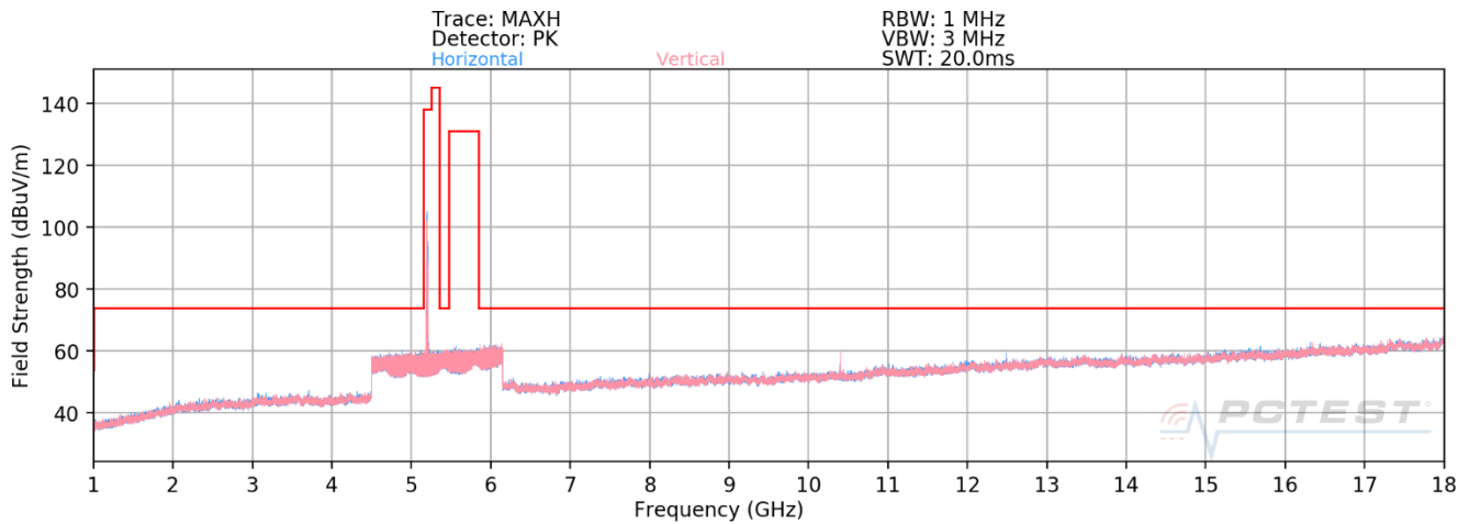
Plot 7-13. Radiated Spurious Plot above 1GHz SISO ANT2 (802.11ax – U1 Ch. 40 – 26 Tones)
