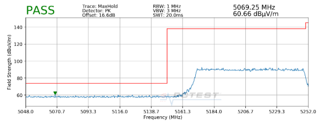
Plot 7-52. Radiated Lower Band Edge Plot SISO ANT1 (Peak – UNII Band 1 – 996 Tones)
