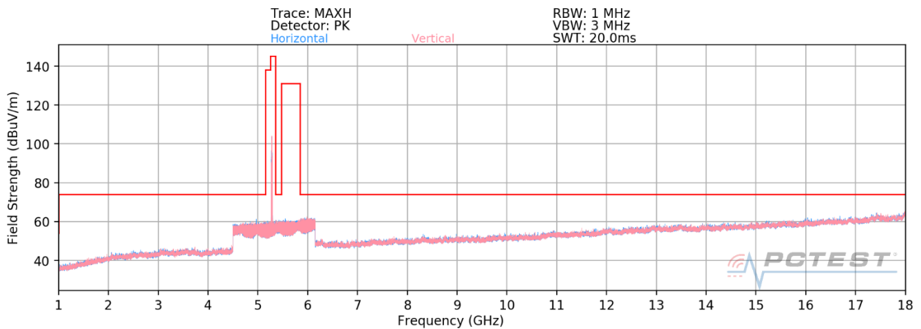
Plot 7-14. Radiated Spurious Plot above 1GHz SISO ANT2 (802.11ax – U2A Ch. 56 – 26 Tones)
