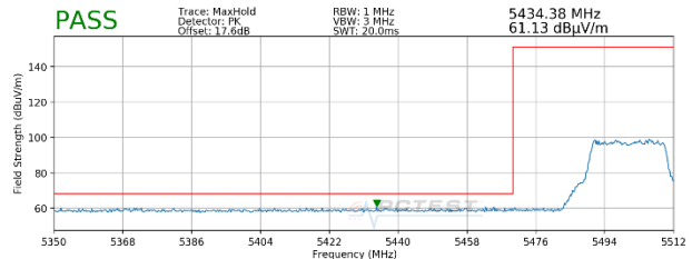
Plot 7-42. Radiated Lower Band Edge Plot SISO ANT1 (Peak - UNII Band 2C - 242 Tones)
