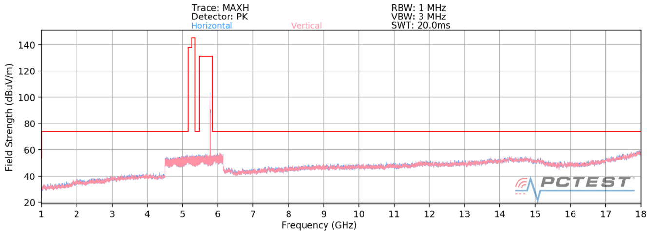
Plot 7-4. Radiated Spurious Plot above 1GHz SISO ANT1 (802.11ax – U3 Ch. 157 – 26 Tones)
