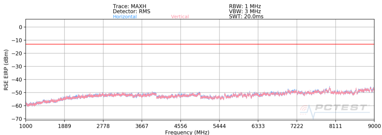
Plot 7-3. Radiated Spurious Plot (Band 26)
