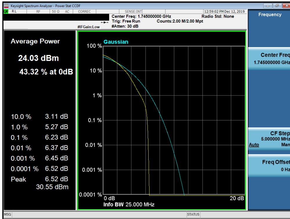
Plot 7-763. PAR Plot (Band n66 - 15.0MHz 64-QAM - Full RB Configuration)
