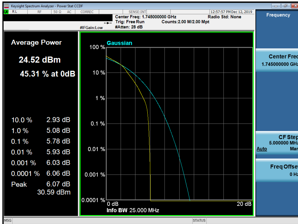
Plot 7-762. PAR Plot (Band n66 - 15.0MHz 16-QAM - Full RB Configuration)
