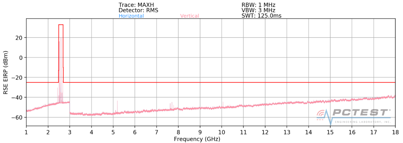
Plot 7-777. Radiated Spurious Plot above 1GHz (Intra-Band Contiguous (B41+n41))
