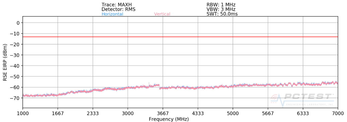
Plot 7-769. Radiated Spurious Plot above 1GHz (n71 Standalone)
