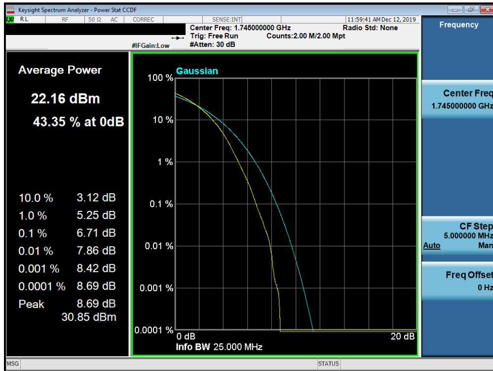
Plot 7-768. PAR Plot (Band n66 - 20.0MHz 256-QAM - Full RB Configuration)
