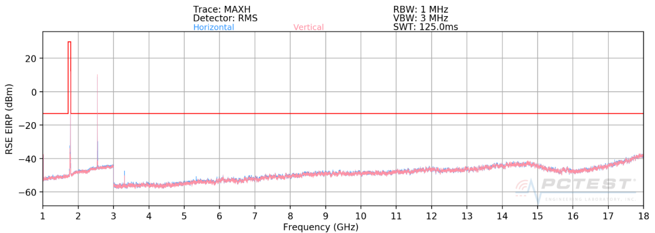
Plot 7-774. Radiated Spurious Plot above 1GHz (n66 ENDC - ANCHOR B7)
