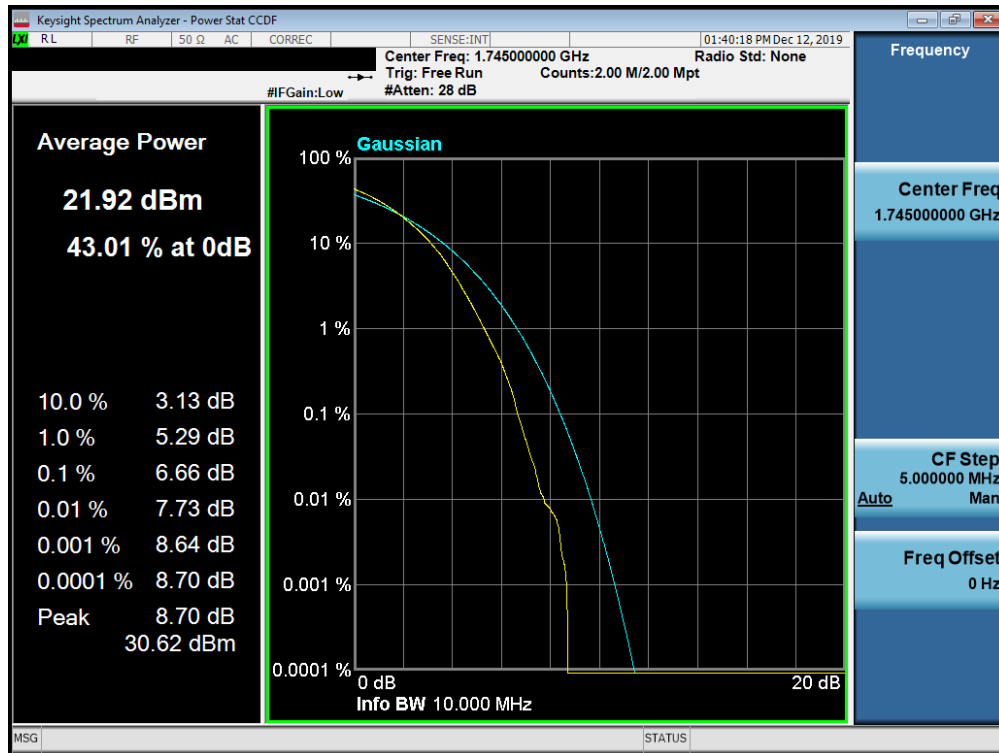
Plot 7-760. PAR Plot (Band n66 - 10.0MHz 256-QAM - Full RB Configuration)
