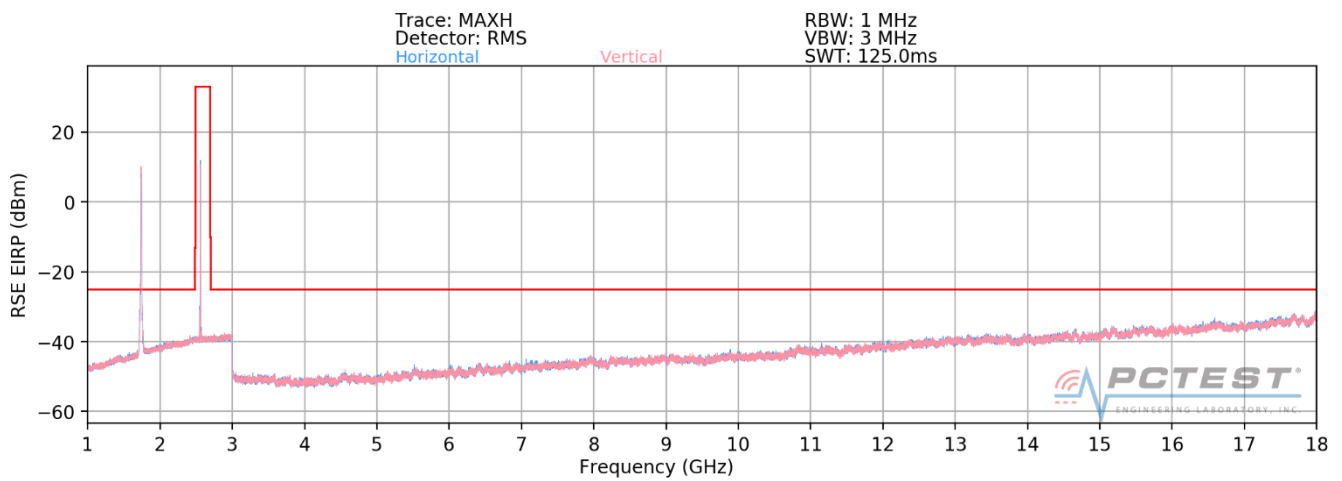
Plot 7-779. Radiated Spurious Plot above 1GHz (n41 ENDC - ANCHOR B66)
