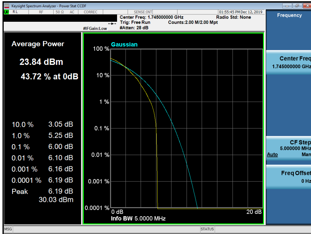
Plot 7-755. PAR Plot (Band n66 - 5.0MHz 64-QAM - Full RB Configuration)
