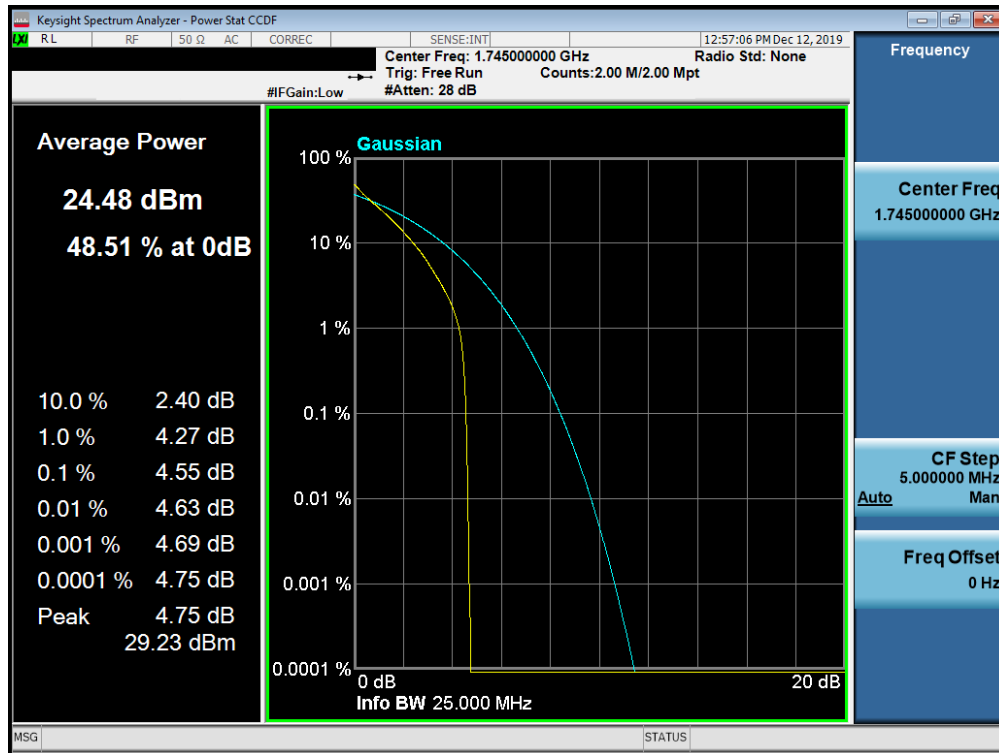
Plot 7-761. PAR Plot (Band n66 - 15.0MHz QPSK - Full RB Configuration)
