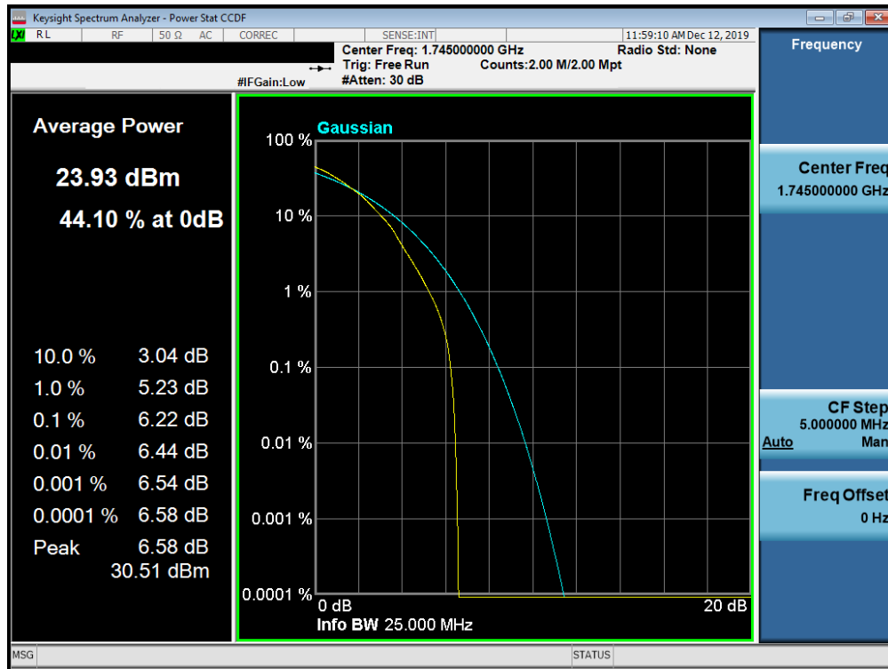
Plot 7-767. PAR Plot (Band n66 - 20.0MHz 64-QAM - Full RB Configuration)
