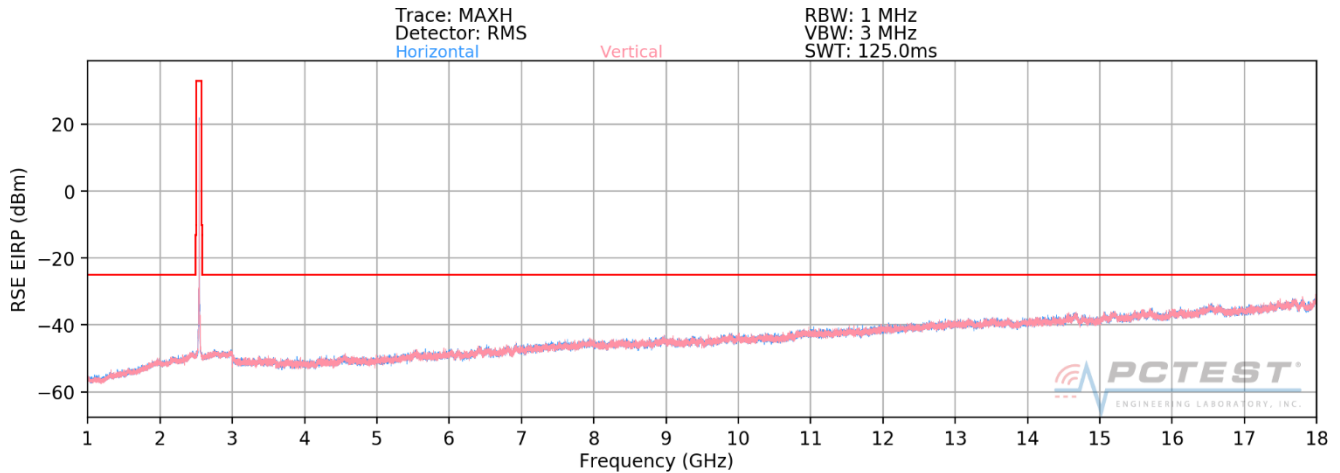
Plot 7-771. Radiated Spurious Plot above 1GHz (n71 ENDC – ANCHOR B7)
