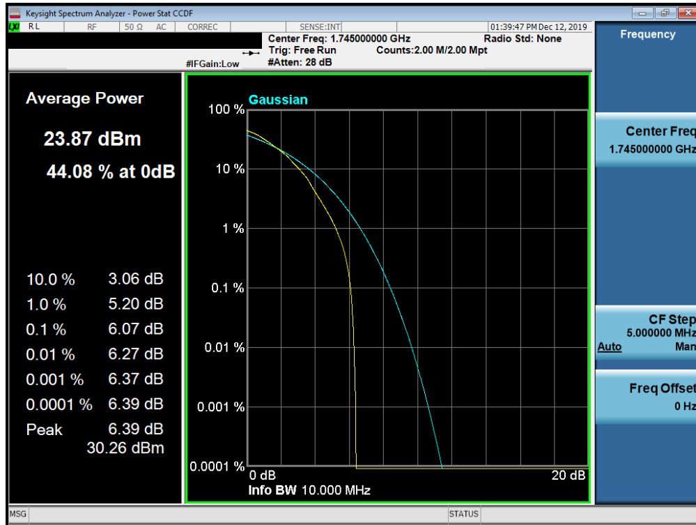
Plot 7-759. PAR Plot (Band n66 - 10.0MHz 64-QAM - Full RB Configuration)
