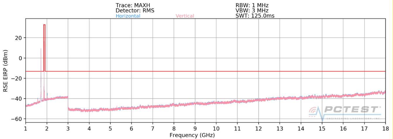
Plot 7-776. Radiated Spurious Plot above 1GHz (n25 END C – ANCHOR B66)
