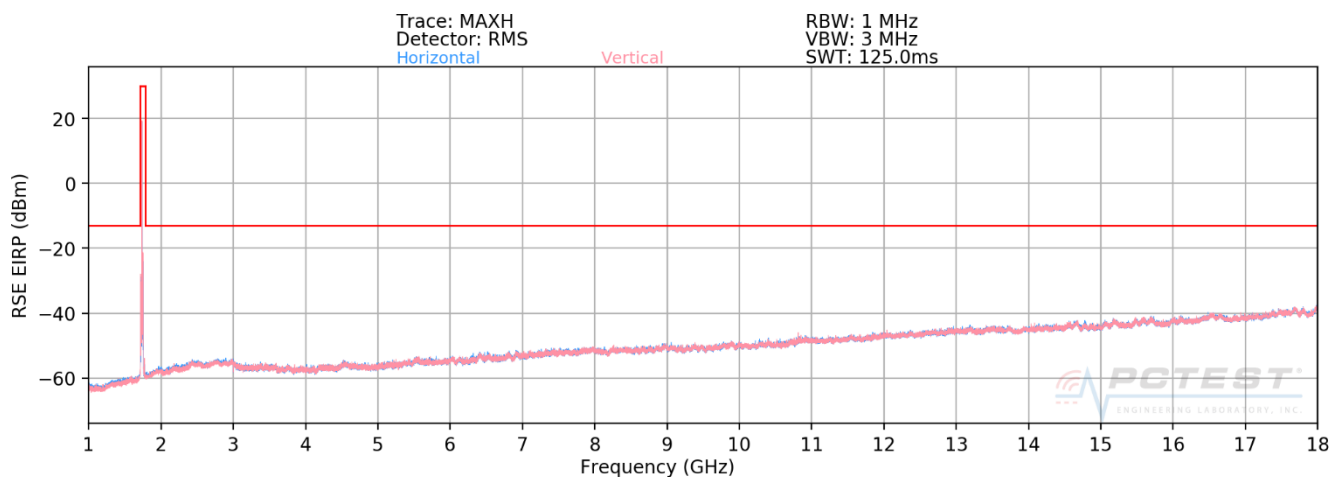
Plot 7-770. Radiated Spurious Plot above 1GHz (n71 ENDC - ANCHOR B66)
