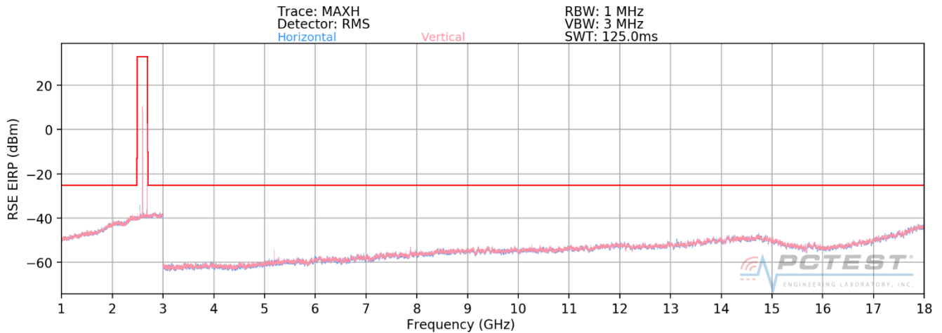
Plot 7-778. Radiated Spurious Plot above 1GHz (Intra-Band Non-Contiguous (B41+n41))
