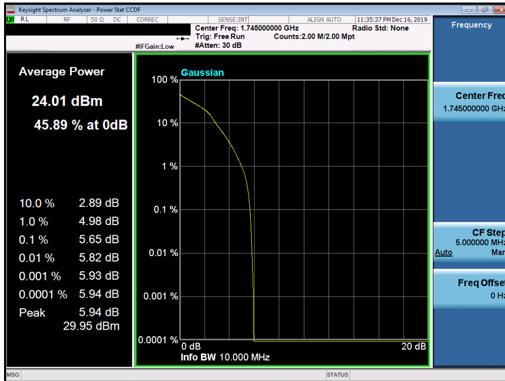
Plot 7-758. PAR Plot (Band n66 - 10.0MHz 16-QAM - Full RB Configuration)
