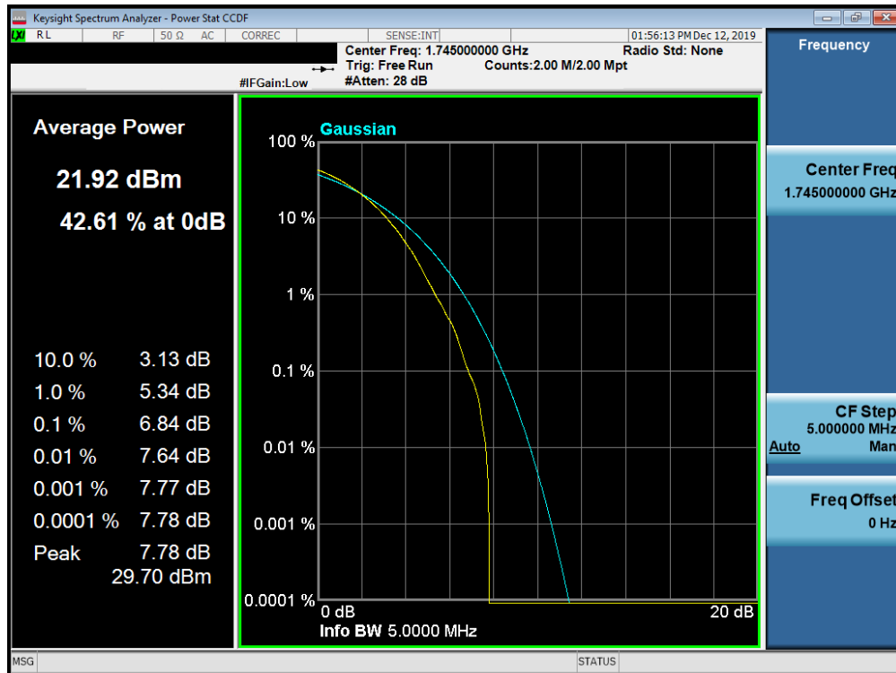
Plot 7-756. PAR Plot (Band n66 - 5.0MHz 256-QAM - Full RB Configuration)
