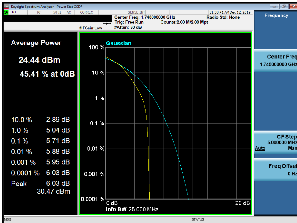
Plot 7-766. PAR Plot (Band n66 - 20.0MHz 16-QAM - Full RB Configuration)
