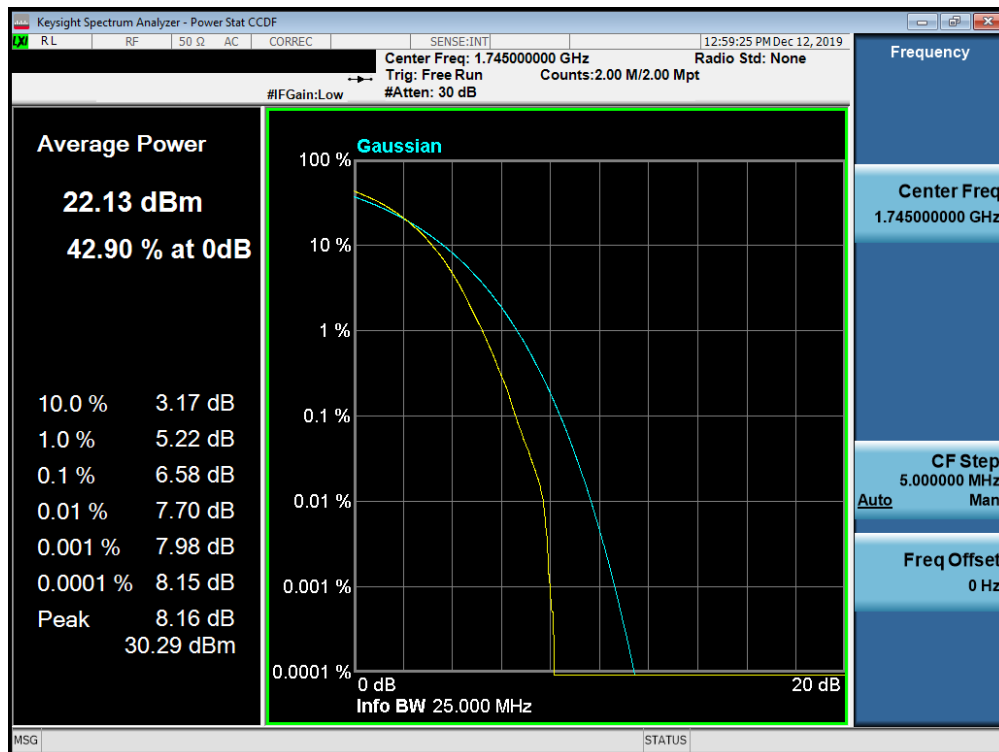
Plot 7-764. PAR Plot (Band n66 - 15.0MHz 56-QAM - Full RB Configuration)
