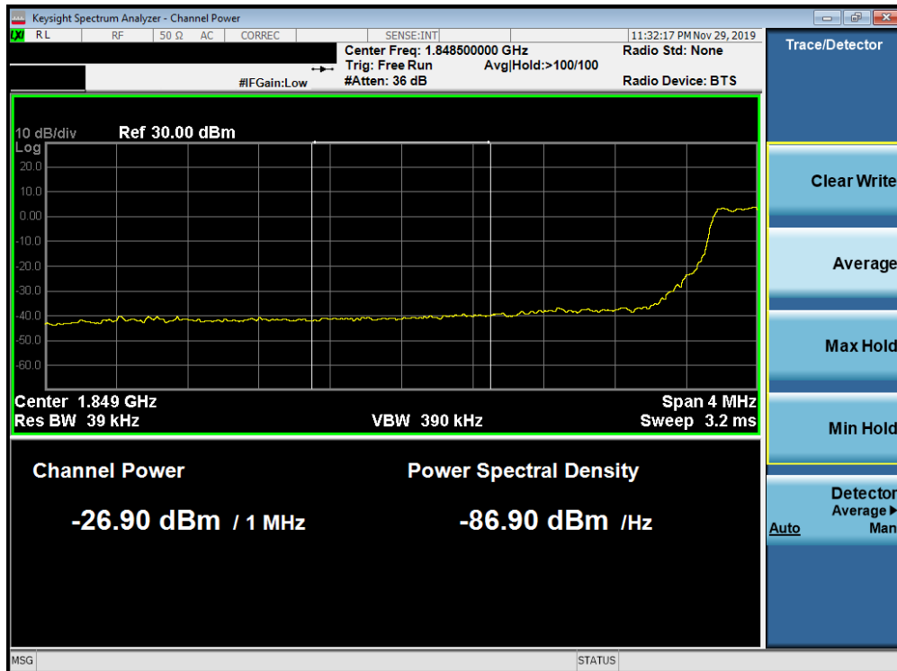
Plot 7-321. Lower Extended Band Edge Plot (Band 25/2 - 5.0MHz QPSK - Full RB Configuration)
