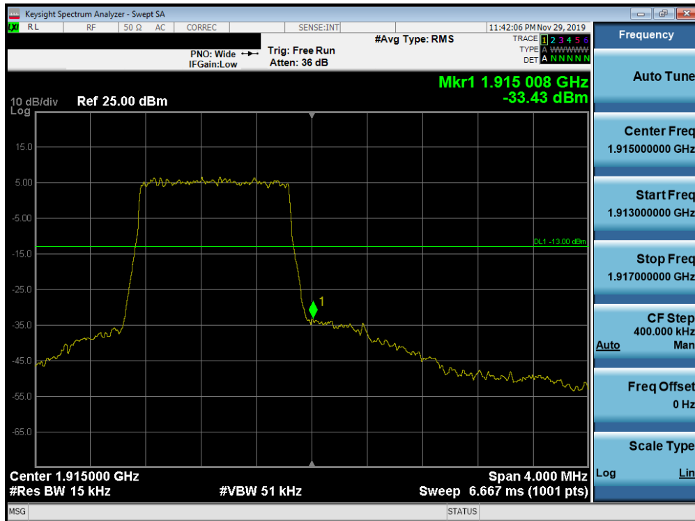
Plot 7-312. Upper Band Edge Plot (Band 25 - 1.4MHz QPSK - Full RB Configuration)
