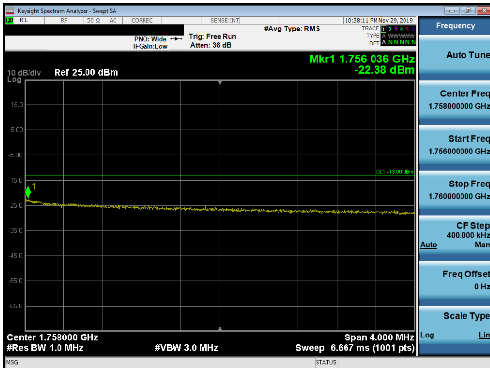
Plot 7-293. Upper Extended Band Edge Plot (Band 4 - 10.0MHz QPSK - Full RB Configuration)
