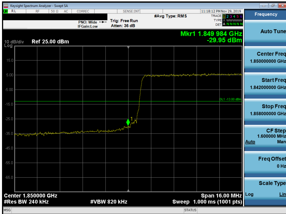
Plot 7-338. Lower Band Edge Plot (Band 25/2 - 20.0MHz QPSK - Full RB Configuration)
