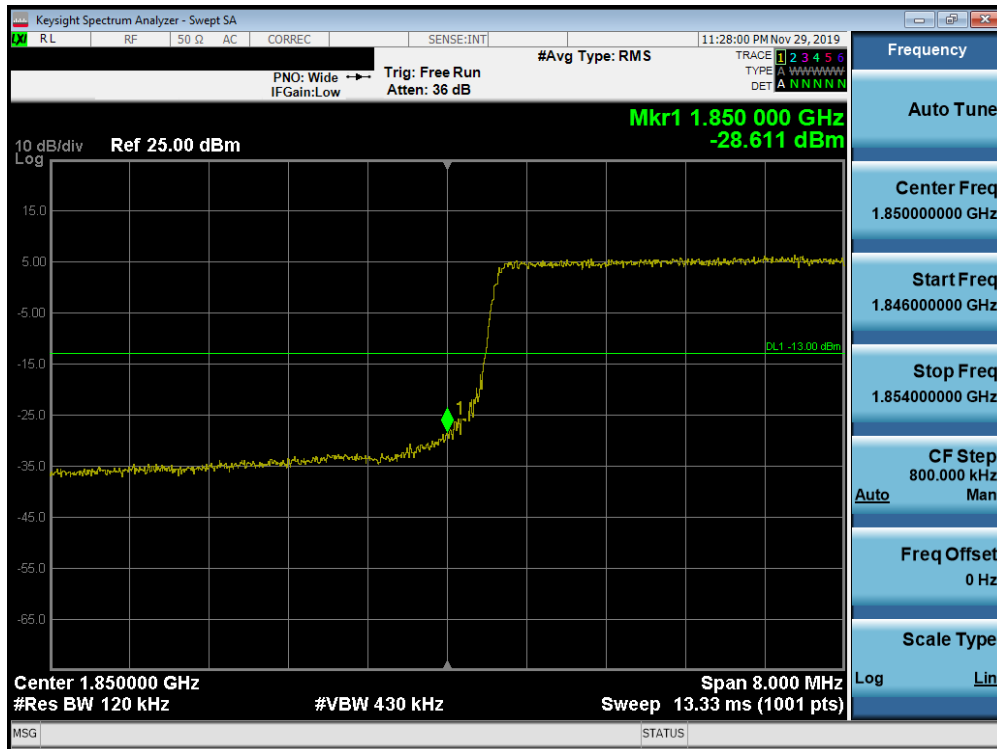
Plot 7-326. Lower Band Edge Plot (Band 25/2 - 10.0MHz QPSK - Full RB Configuration)
