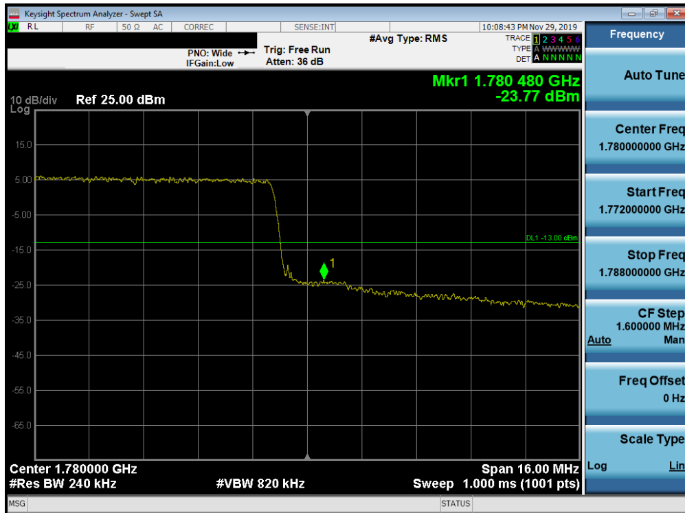
Plot 7-306. Upper Band Edge Plot (Band 66 - 20.0MHz QPSK - Full RB Configuration)
