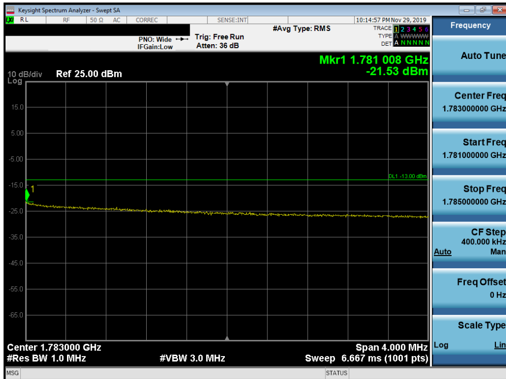
Plot 7-295. Upper Extended Band Edge Plot (Band 66 - 10.0MHz QPSK - Full RB Configuration)
