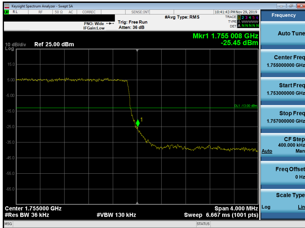
Plot 7-280. Upper Band Edge Plot (Band 4 - 3.0MHz QPSK - Full RB Configuration)
