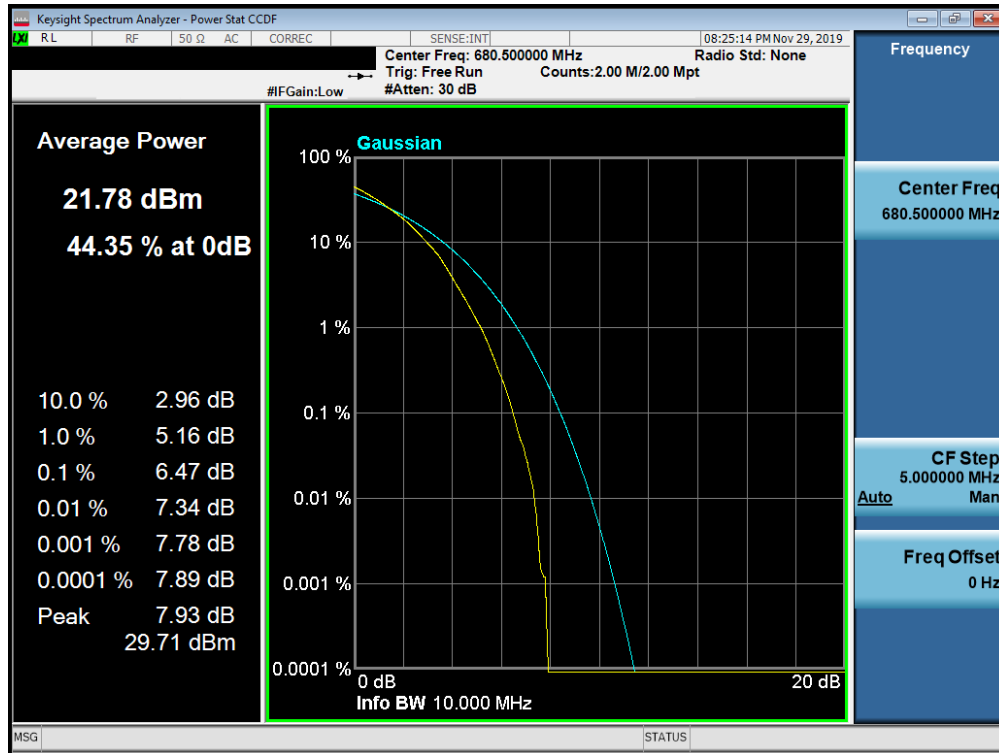
Plot 7-385. PAR Plot (Band 71 - 10.0MHz 64-QAM - Full RB Configuration)
