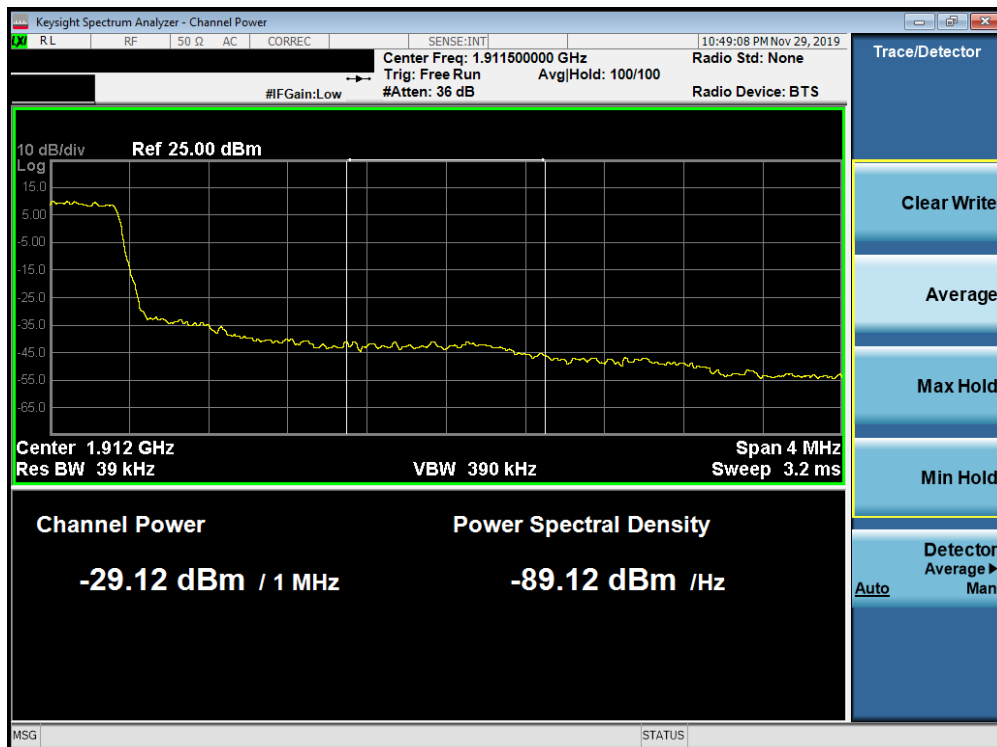
Plot 7-311. Upper Extended Band Edge Plot (Band 2 - 1.4MHz QPSK - Full RB Configuration)
