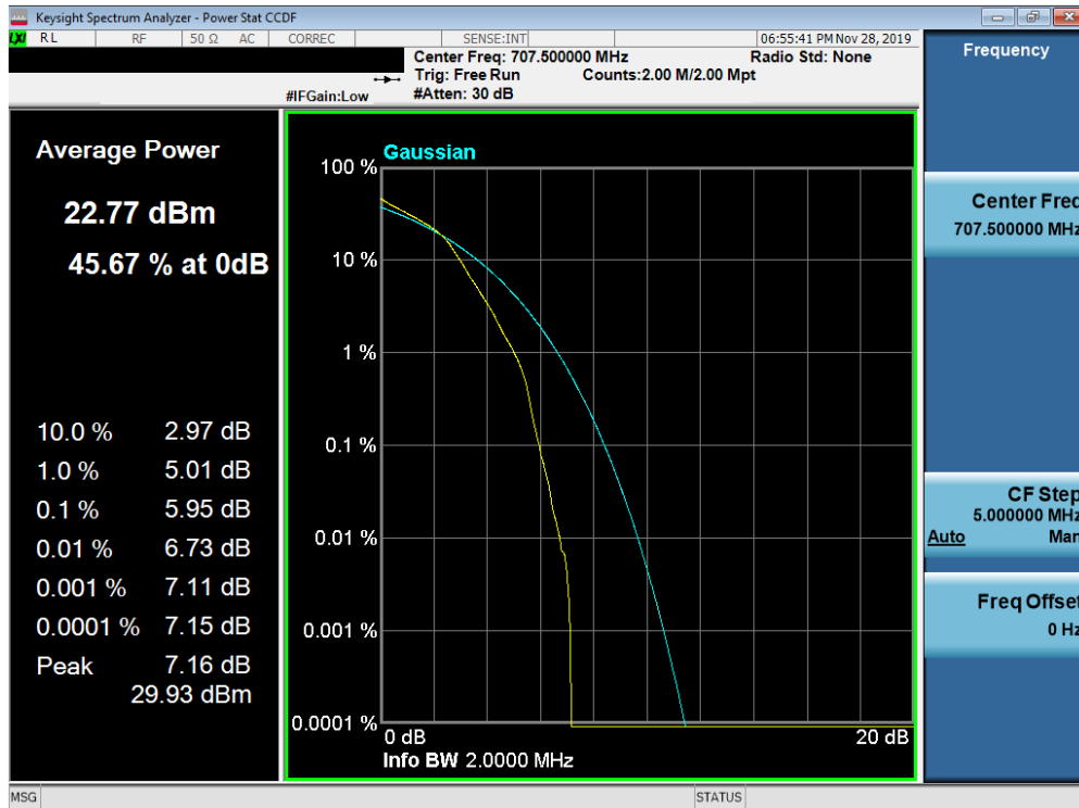
Plot 7-396. PAR Plot (Band 12 - 1.4MHz 16-QAM - Full RB Configuration)
