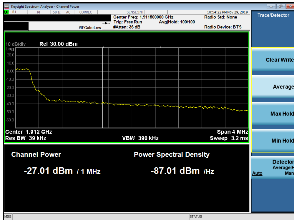
Plot 7-323. Upper Extended Band Edge Plot (Band 2 - 5.0MHz QPSK - Full RB Configuration)
