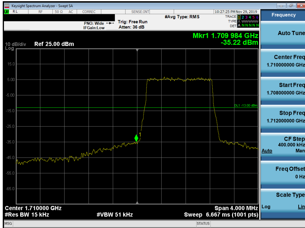
Plot 7-272. Lower Band Edge Plot (Band 66/4 - 1.4MHz QPSK - Full RB Configuration)
