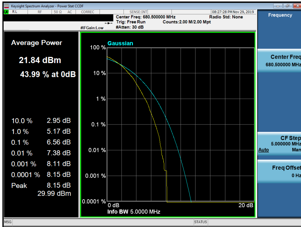
Plot 7-381. PAR Plot (Band 71 – 5.0MHz 64-QAM - Full RB Configuration)
