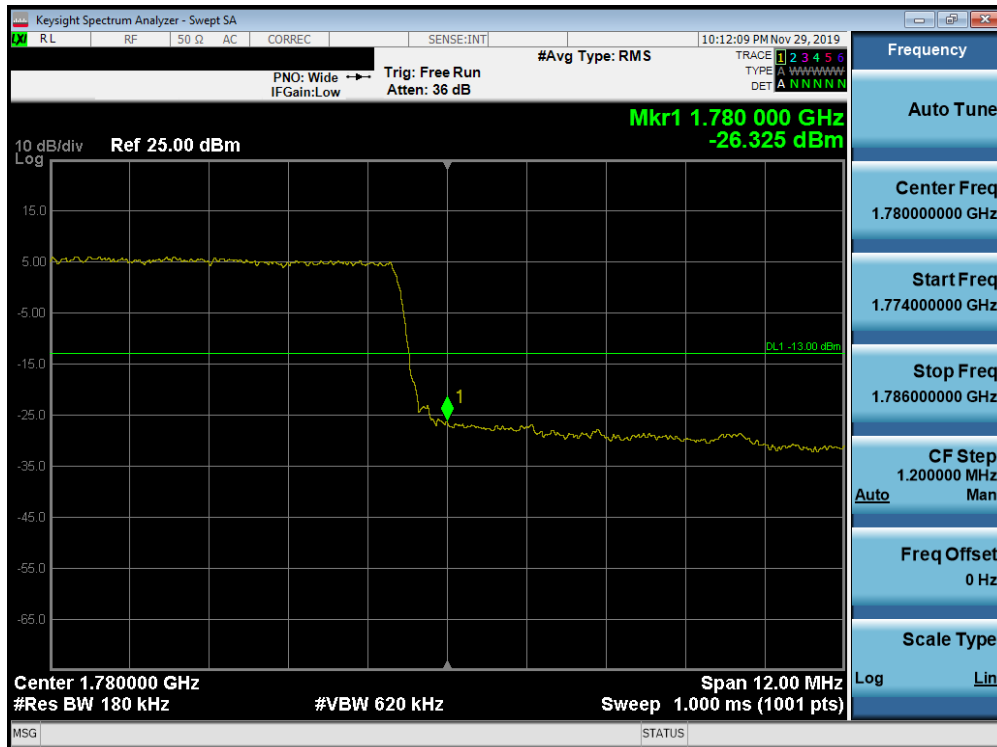
Plot 7-300. Upper Band Edge Plot (Band 66 - 15.0MHz QPSK - Full RB Configuration)
