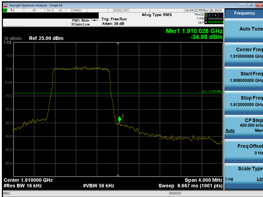
Plot 7-310. Upper Band Edge Plot (Band 2 - 1.4MHz QPSK - Full RB Configuration)
