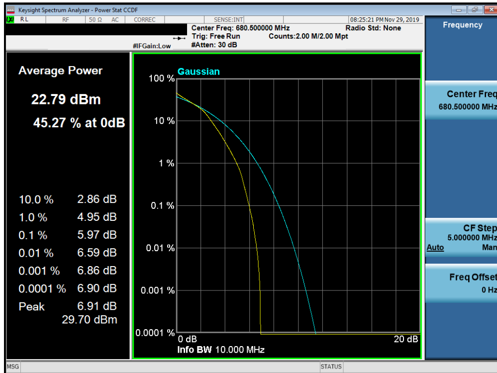
Plot 7-384. PAR Plot (Band 71 - 10.0MHz 16-QAM - Full RB Configuration)
