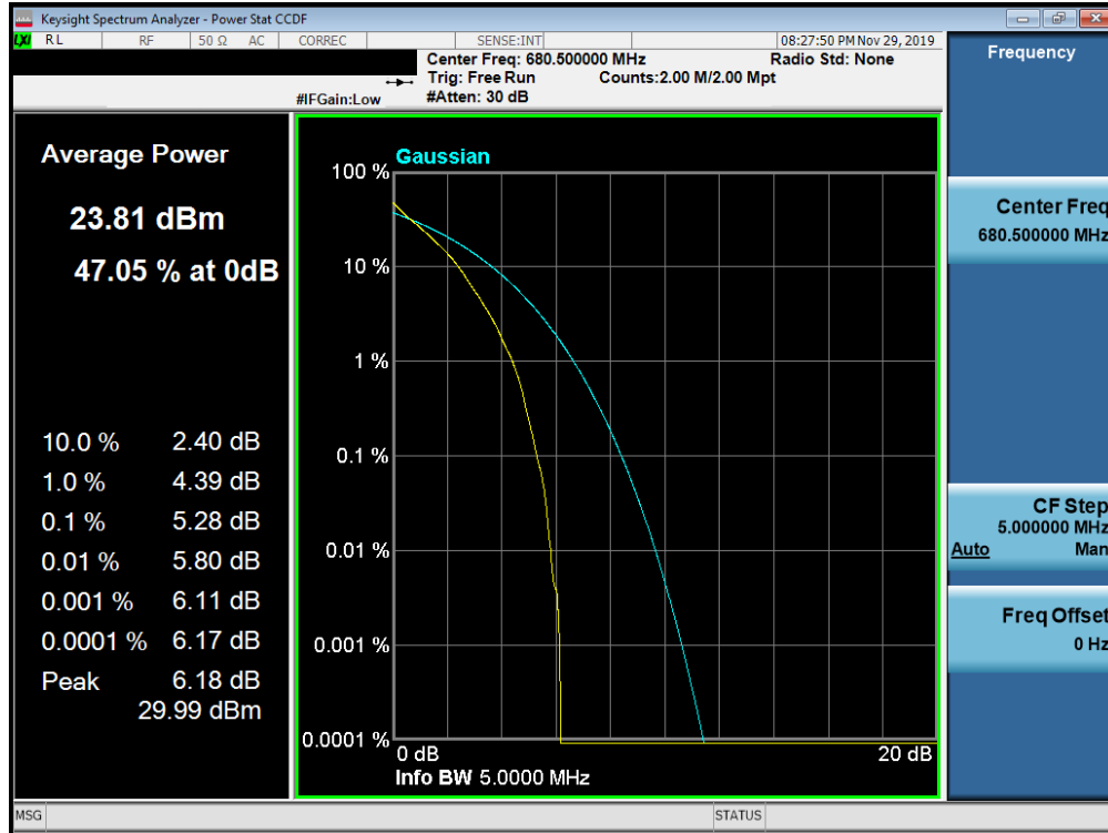
Plot 7-379. PAR Plot (Band 71 – 5.0MHz QPSK - Full RB Configuration)
