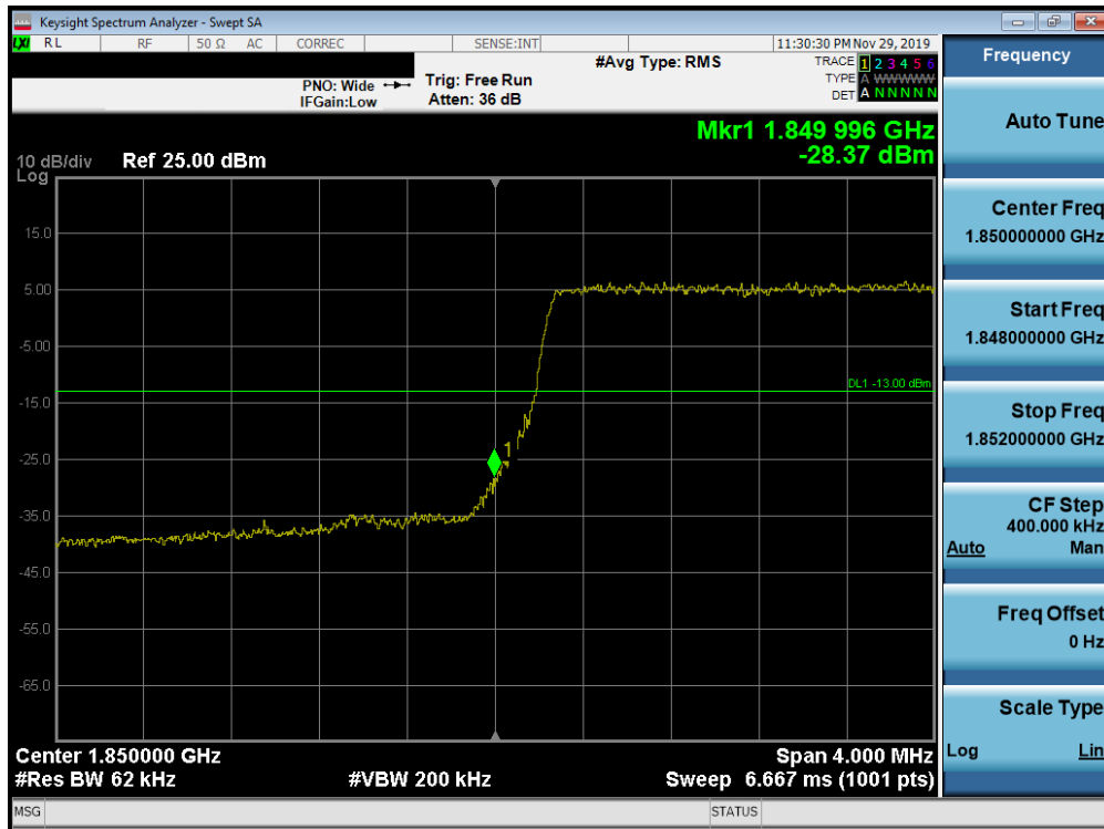
Plot 7-320. Lower Band Edge Plot (Band 25/2 - 5.0MHz QPSK - Full RB Configuration)
