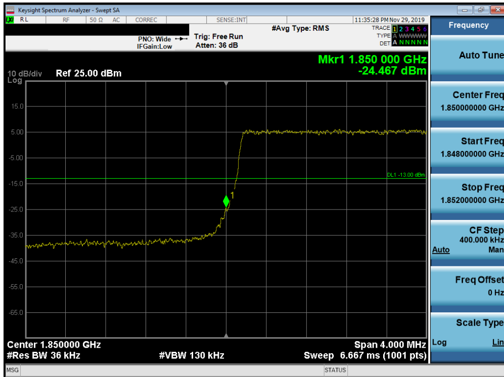
Plot 7-314. Lower Band Edge Plot (Band 25/2 - 3.0MHz QPSK - Full RB Configuration)
