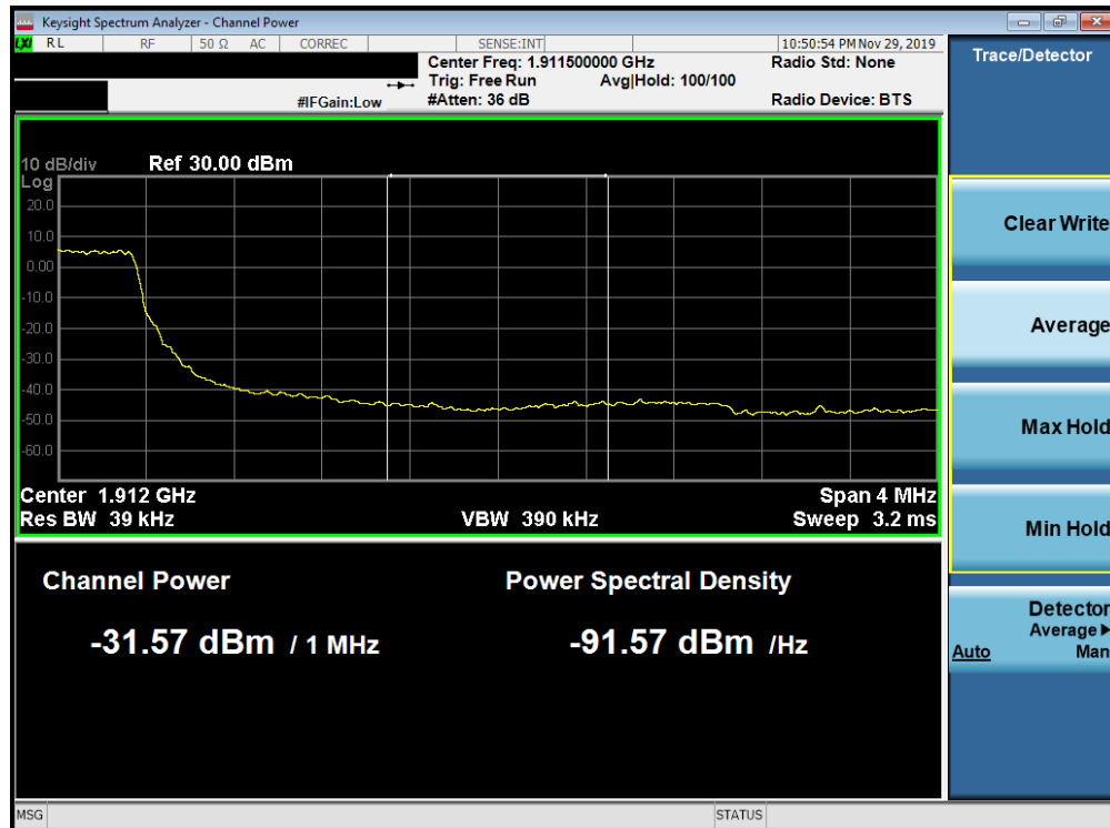
Plot 7-317. Upper Extended Band Edge Plot (Band 2 - 3.0MHz QPSK - Full RB Configuration)
