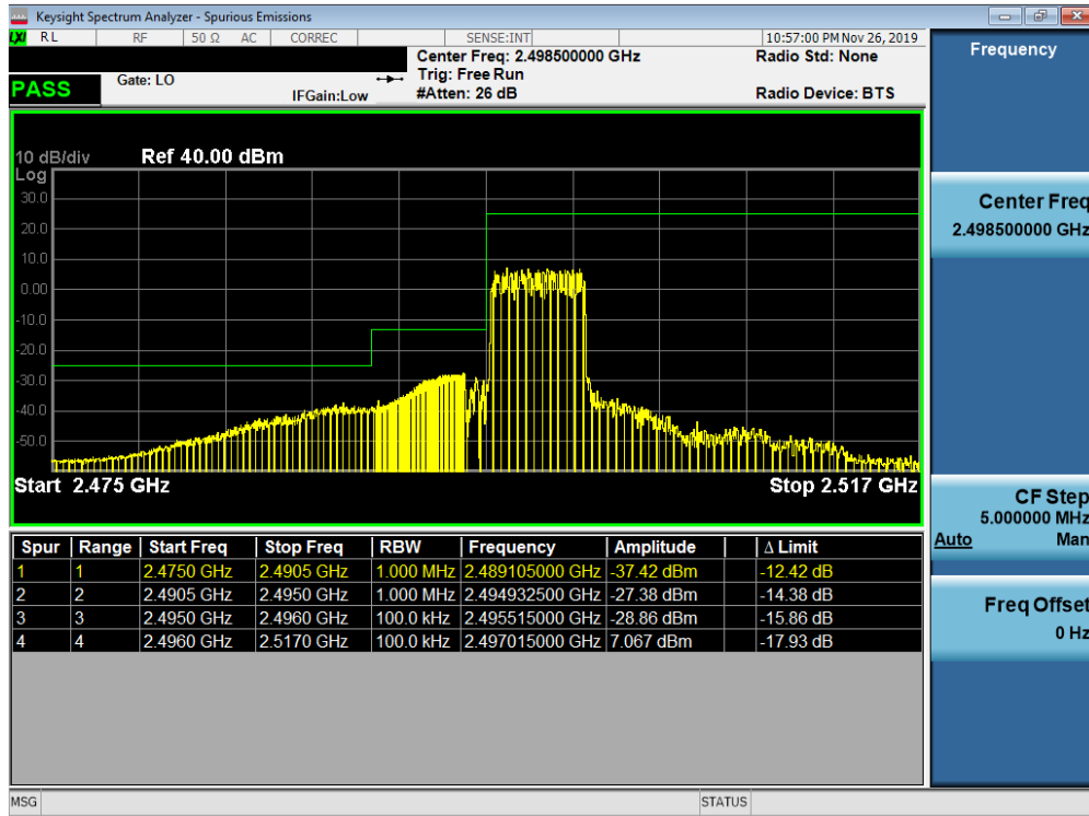
Plot 7-371. Lower ACP Plot at 2496 MHz (Band 41 PC3 - 5.0MHz QPSK - Full RB Configuration)
