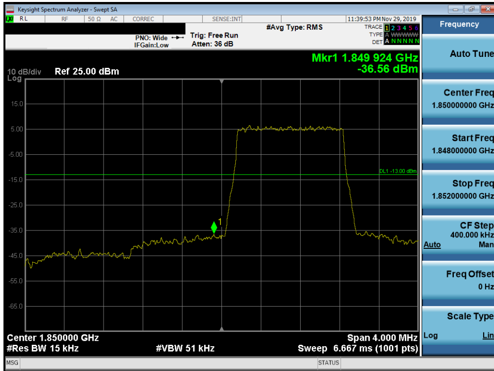
Plot 7-308. Lower Band Edge Plot (Band 25/2 - 1.4MHz QPSK - Full RB Configuration)
