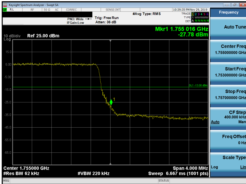
Plot 7-286. Upper Band Edge Plot (Band 4 - 5.0MHz QPSK - Full RB Configuration)
