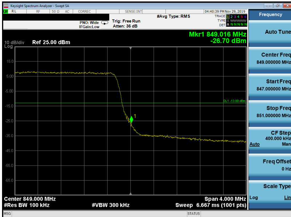
Plot 7-267. Upper Band Edge Plot (Band 26/5 - 5.0MHz QPSK - Full RB Configuration)
