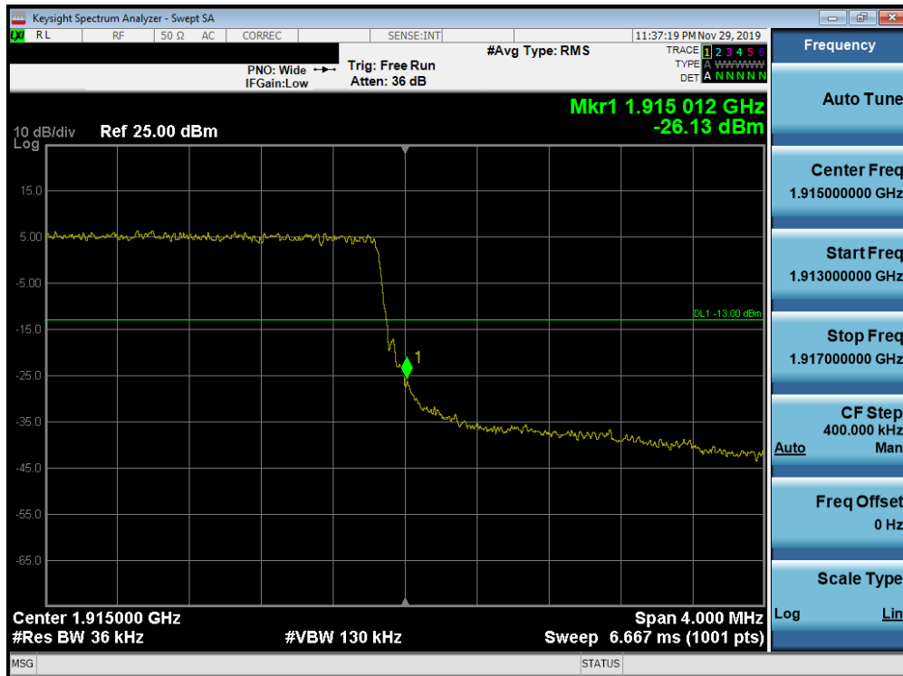
Plot 7-318. Upper Band Edge Plot (Band 25 - 3.0MHz QPSK - Full RB Configuration)
