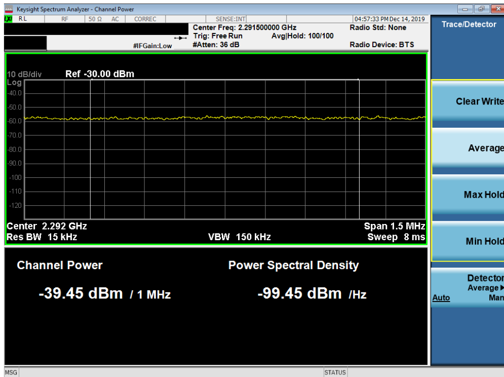
Plot 7-351. Lower Extended Band Edge Plot (Band 30 - 10.0MHz QPSK - Full RB Configuration)
