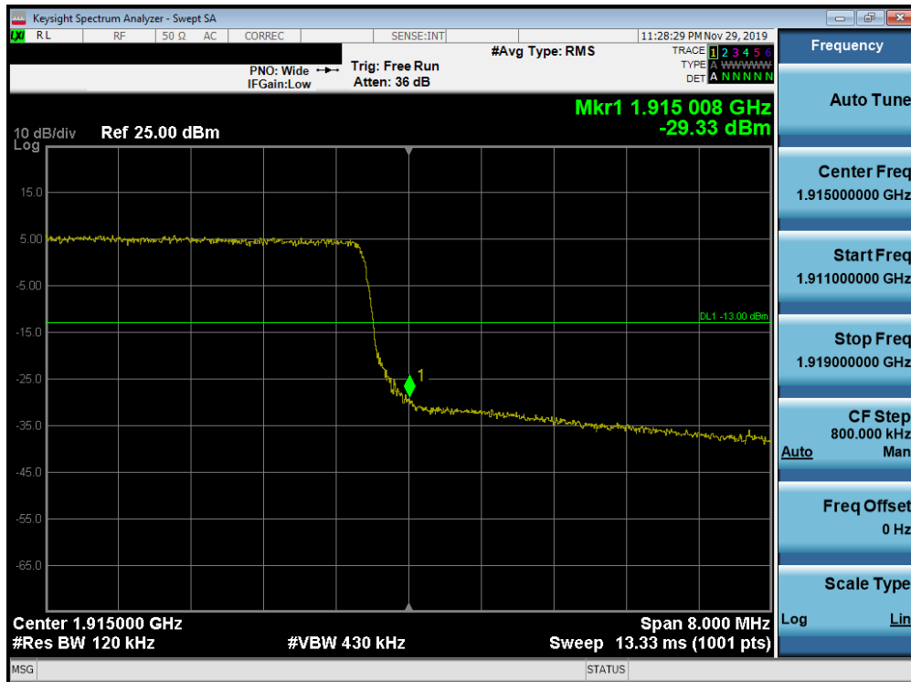
Plot 7-330. Upper Band Edge Plot (Band 25 - 10.0MHz QPSK - Full RB Configuration)
