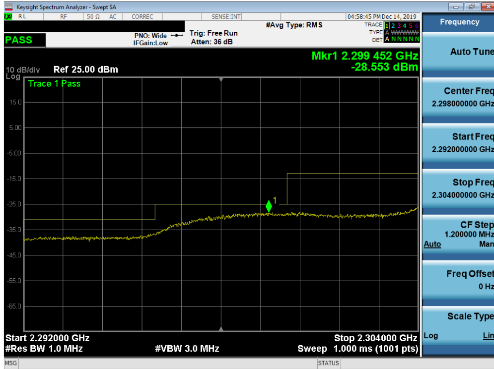
Plot 7-352. Lower Extended Band Edge Plot (Band 30 - 10.0MHz QPSK - Full RB Configuration)
