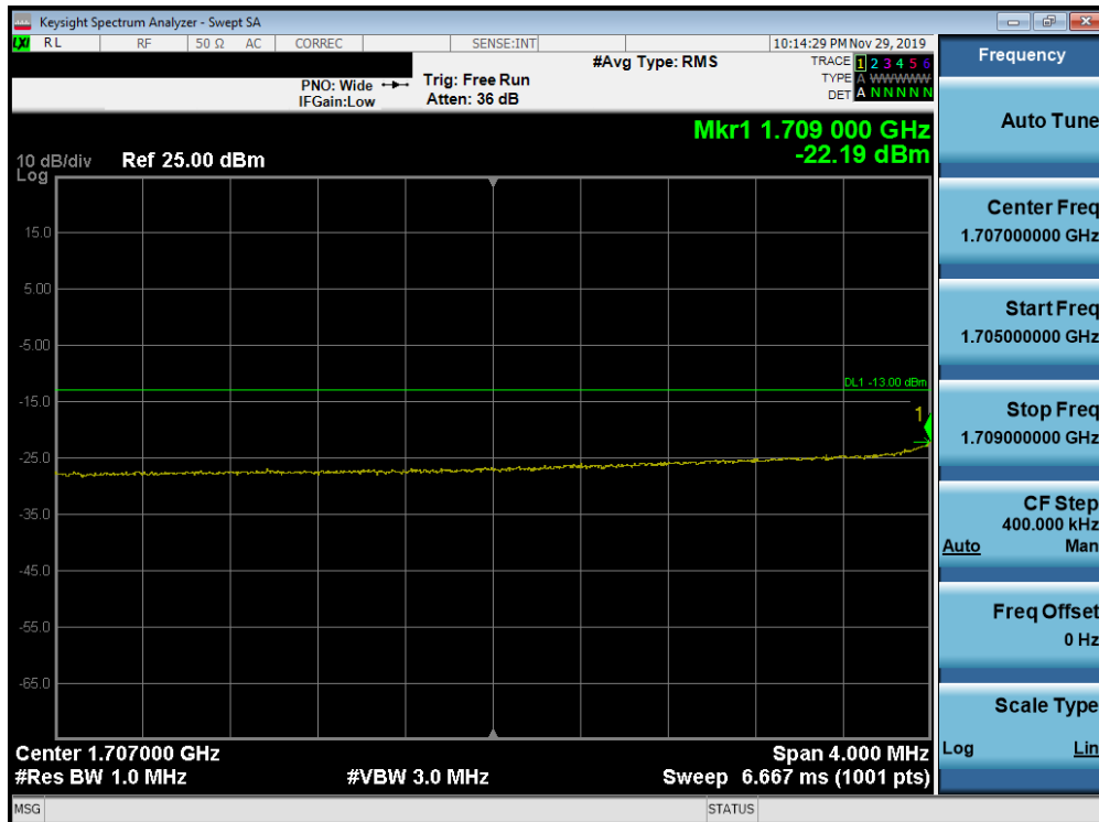
Plot 7-291. Lower Extended Band Edge Plot (Band 66/4 - 10.0MHz QPSK - Full RB Configuration)
