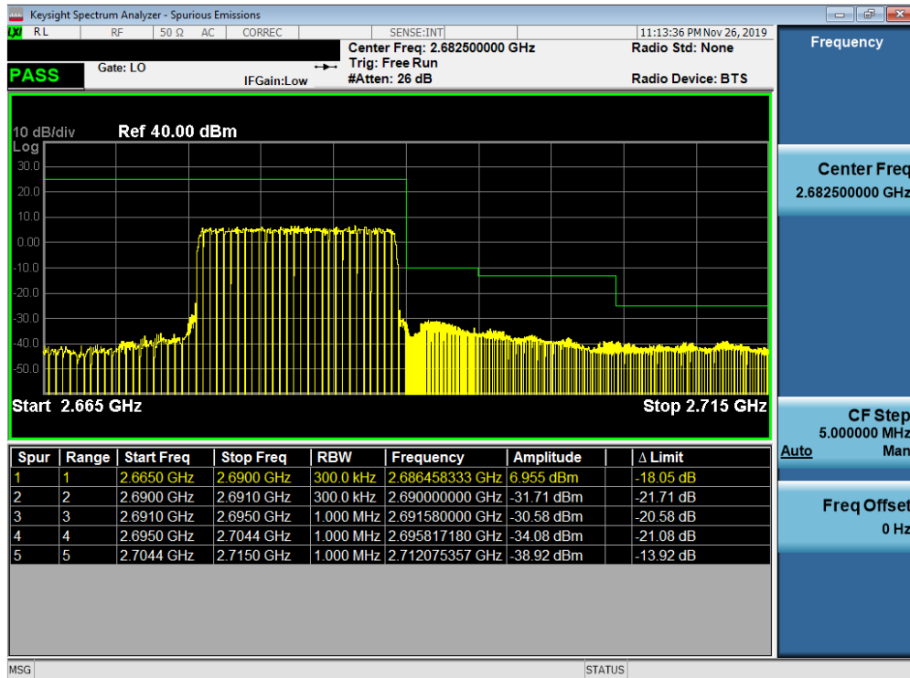
Plot 7-376. Upper ACP Plot (Band 41 PC3 - 15.0MHz QPSK - Full RB Configuration)
