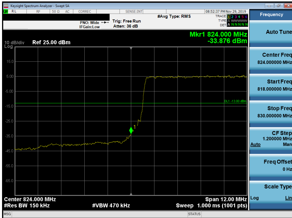
Plot 7-270. Lower Band Edge Plot (Band 26 - 15.0MHz QPSK - Full RB Configuration)
