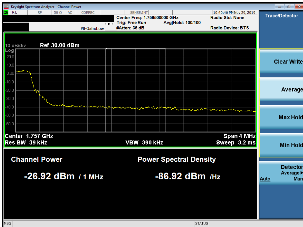
Plot 7-287. Upper Extended Band Edge Plot (Band 4 - 5.0MHz QPSK - Full RB Configuration)
