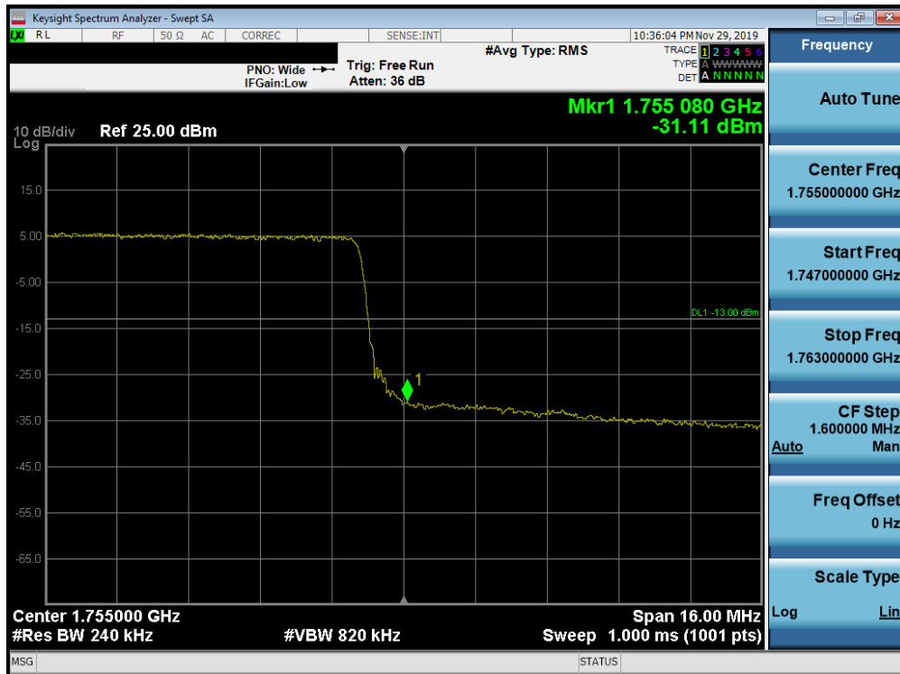
Plot 7-304. Upper Band Edge Plot (Band 4 - 20.0MHz QPSK - Full RB Configuration)
