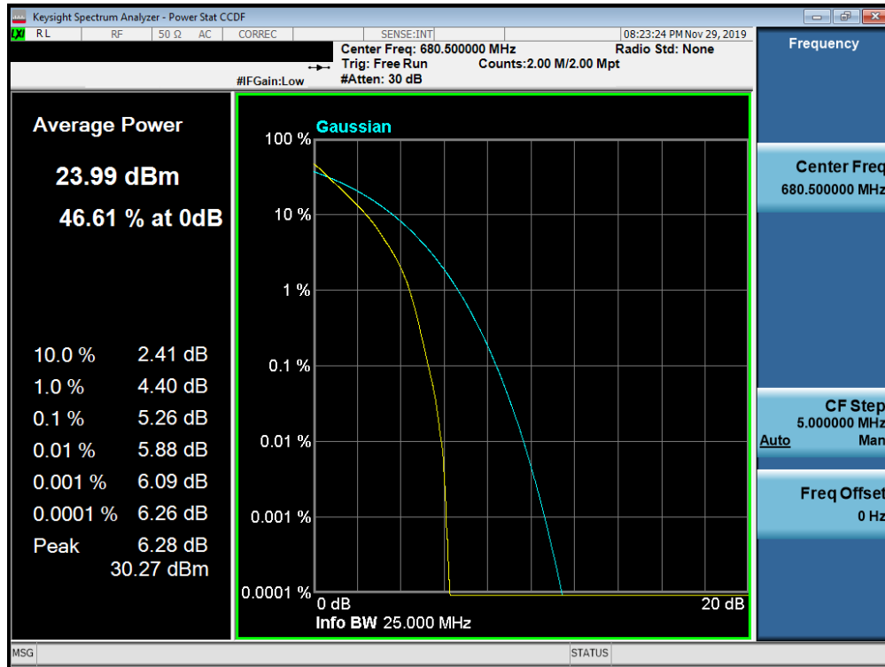
Plot 7-387. PAR Plot (Band 71 - 15.0MHz QPSK - Full RB Configuration)
