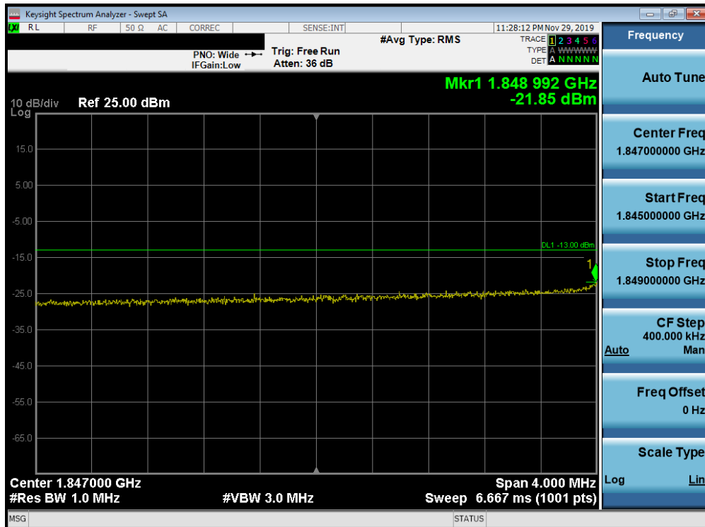
Plot 7-327. Lower Extended Band Edge Plot (Band 25/2 - 10.0MHz QPSK - Full RB Configuration)
