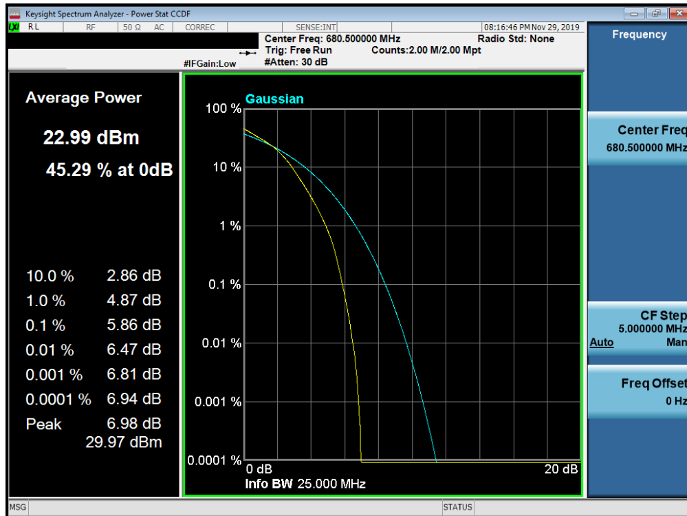
Plot 7-392. PAR Plot (Band 71 - 20.0MHz 16-QAM - Full RB Configuration)
