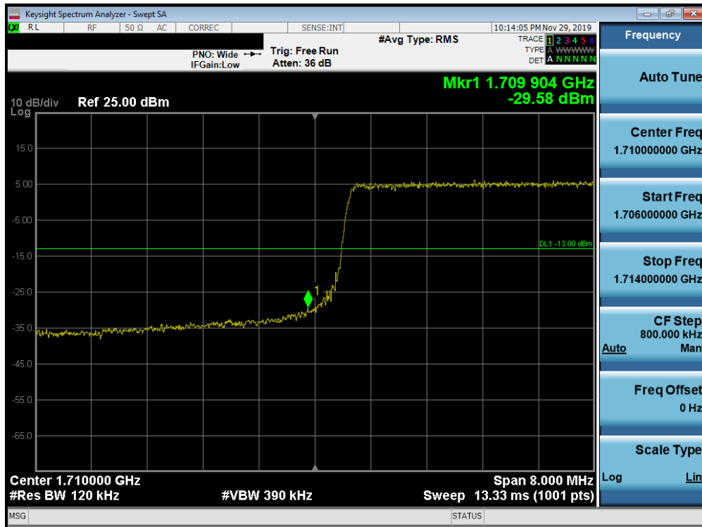
Plot 7-290. Lower Band Edge Plot (Band 66/4 - 10.0MHz QPSK - Full RB Configuration)
