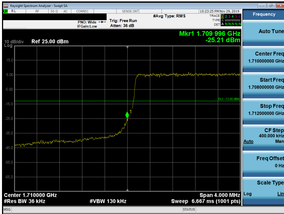
Plot 7-278. Lower Band Edge Plot (Band 66/4 - 3.0MHz QPSK - Full RB Configuration)
