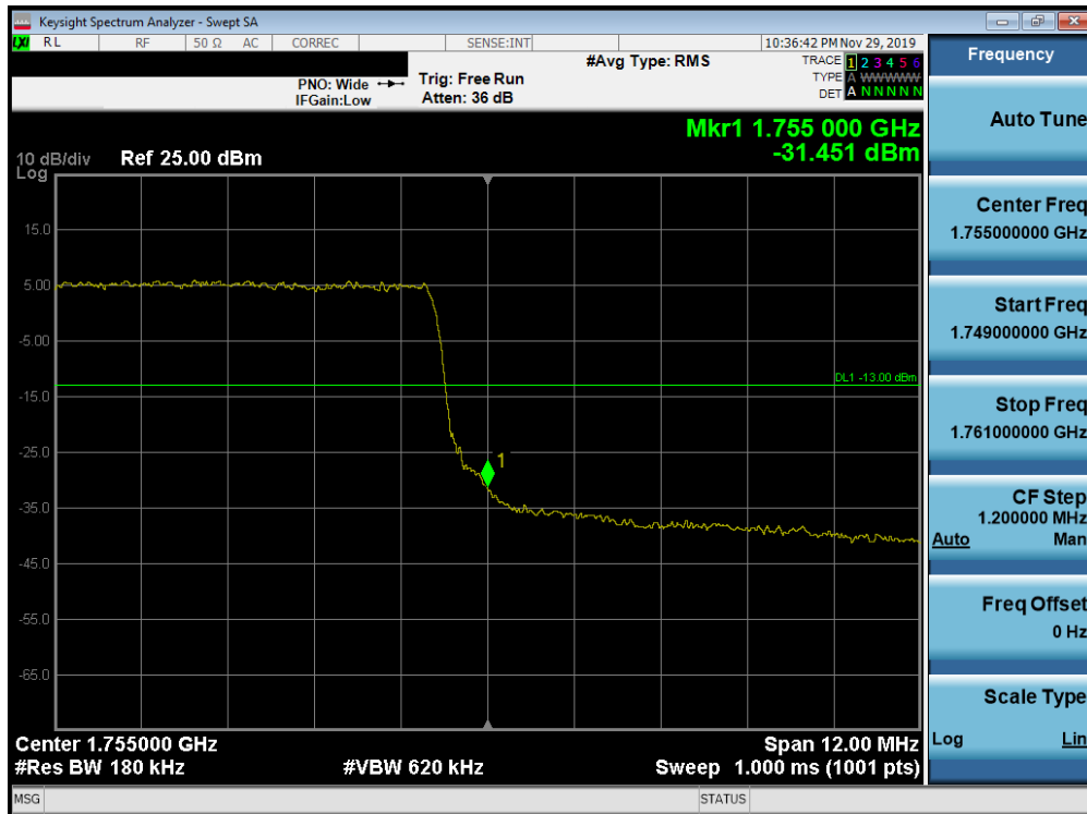
Plot 7-298. Upper Band Edge Plot (Band 4 - 15.0MHz QPSK - Full RB Configuration)
