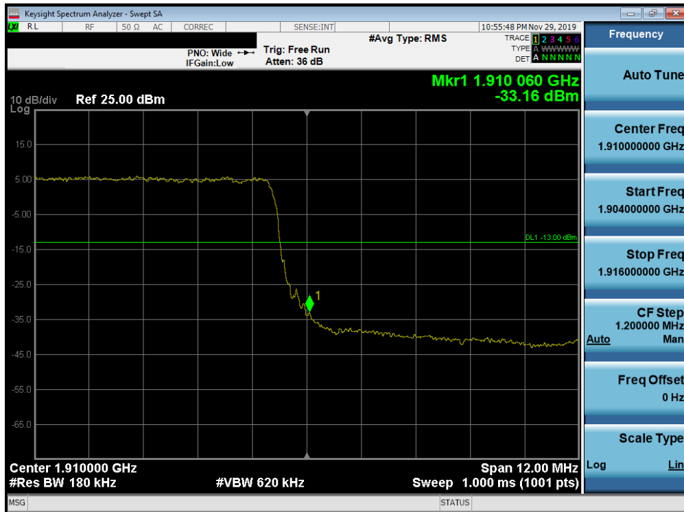
Plot 7-334. Upper Band Edge Plot (Band 2 - 15.0MHz QPSK - Full RB Configuration)
