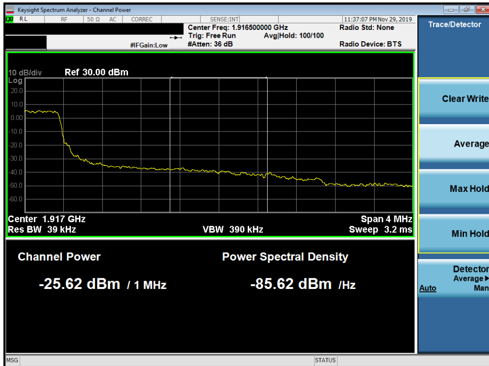
Plot 7-319. Upper Extended Band Edge Plot (Band 25 - 3.0MHz QPSK - Full RB Configuration)
