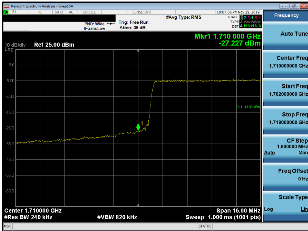
Plot 7-302. Lower Band Edge Plot (Band 66/4 - 20.0MHz QPSK - Full RB Configuration)
