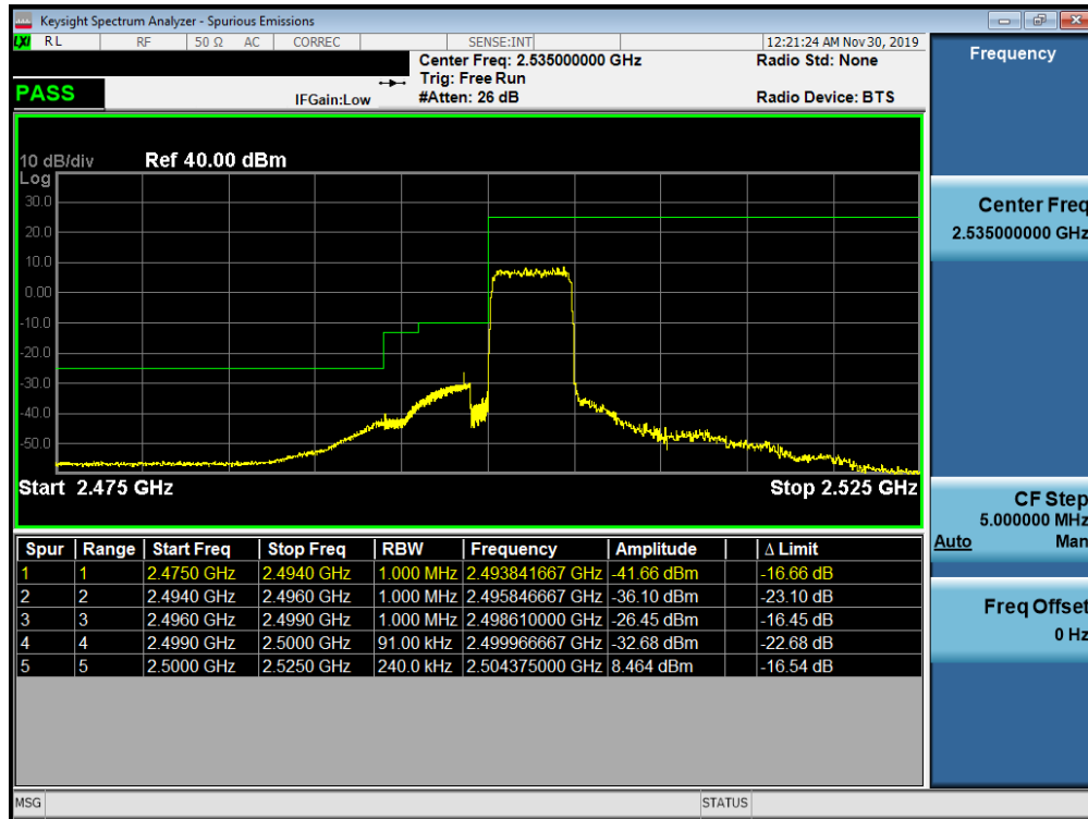
Plot 7-355. Lower ACP Plot (Band 7 - 5.0MHz QPSK - Full RB Configuration)
