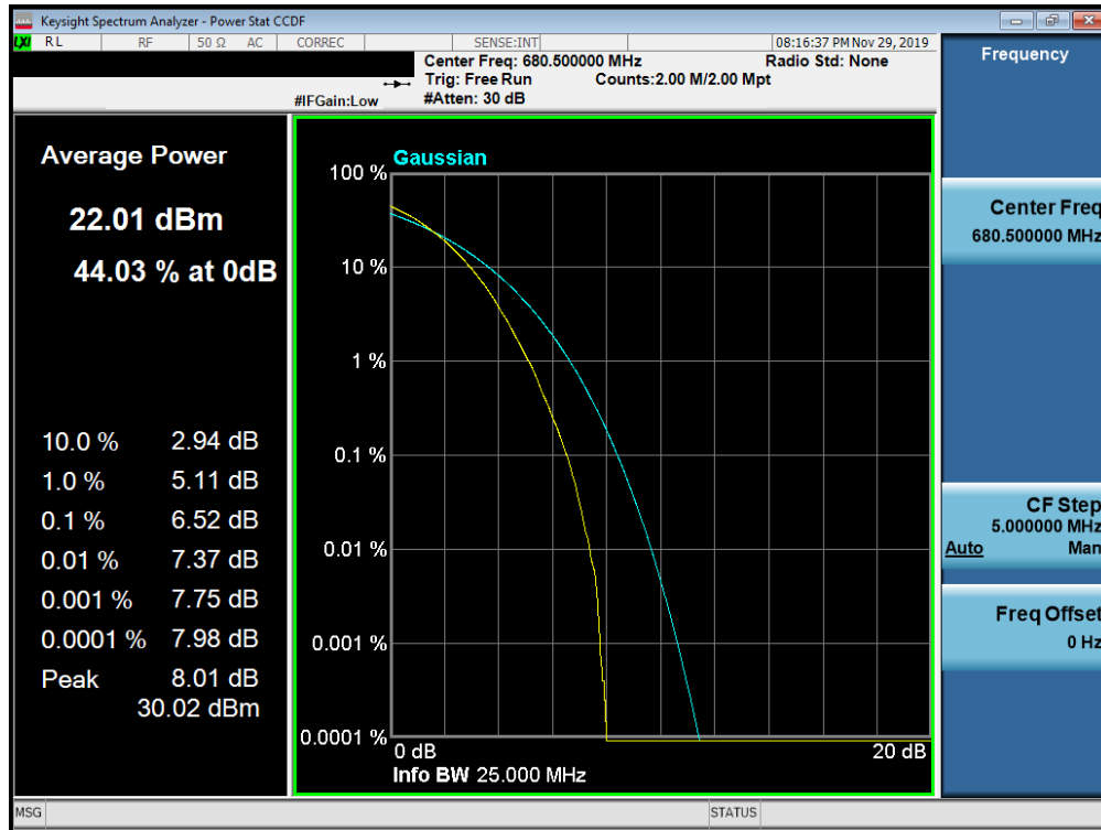
Plot 7-393. PAR Plot (Band 71 - 20.0MHz 64-QAM - Full RB Configuration)
