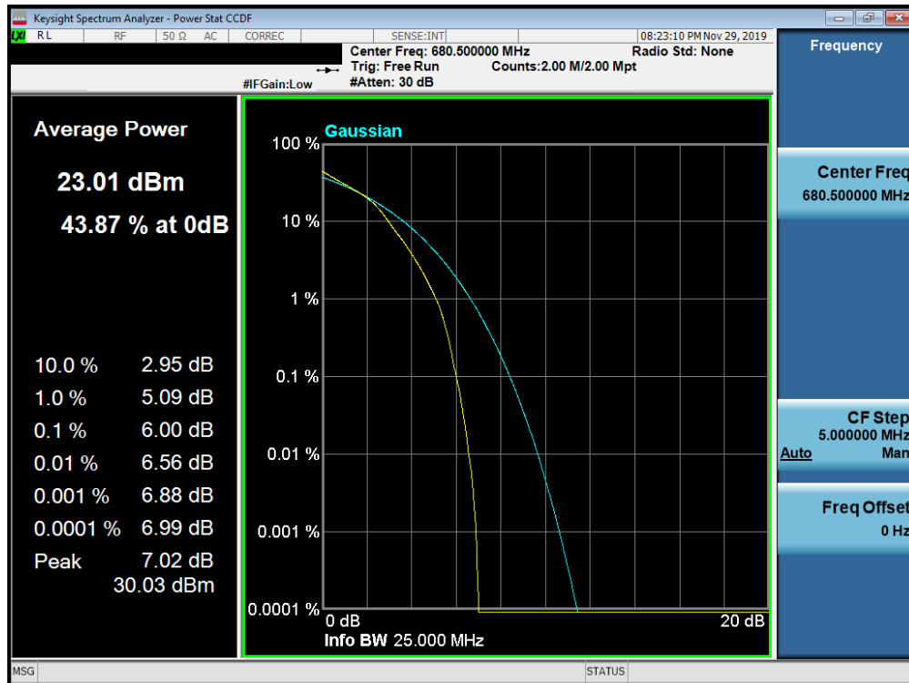
Plot 7-388. PAR Plot (Band 71 - 15.0MHz 16-QAM - Full RB Configuration)
