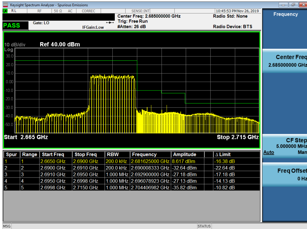
Plot 7-366. Upper ACP Plot (Band 41 PC2- 10.0MHz QPSK - Full RB Configuration)
