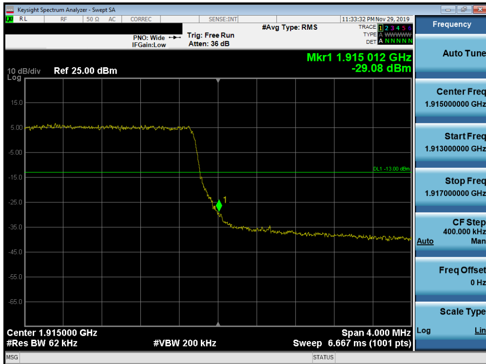
Plot 7-324. Upper Band Edge Plot (Band 25 - 5.0MHz QPSK - Full RB Configuration)
