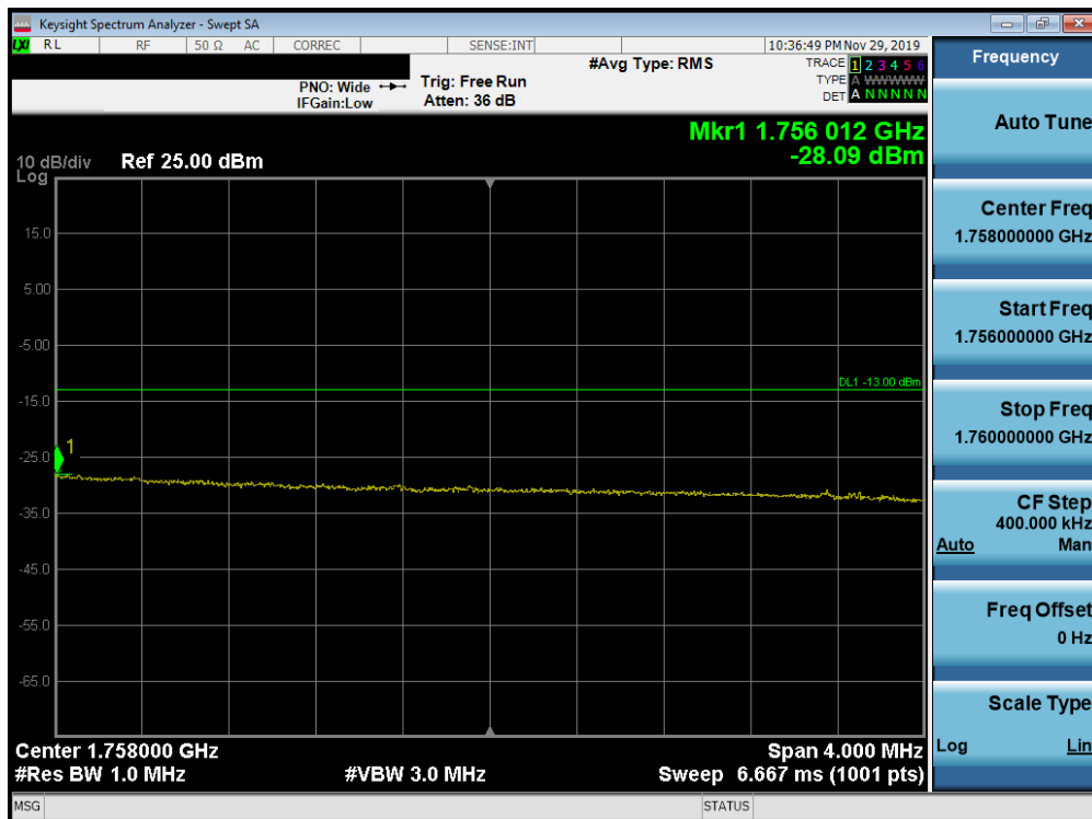
Plot 7-299. Upper Extended Band Edge Plot (Band 4 - 15.0MHz QPSK - Full RB Configuration)
