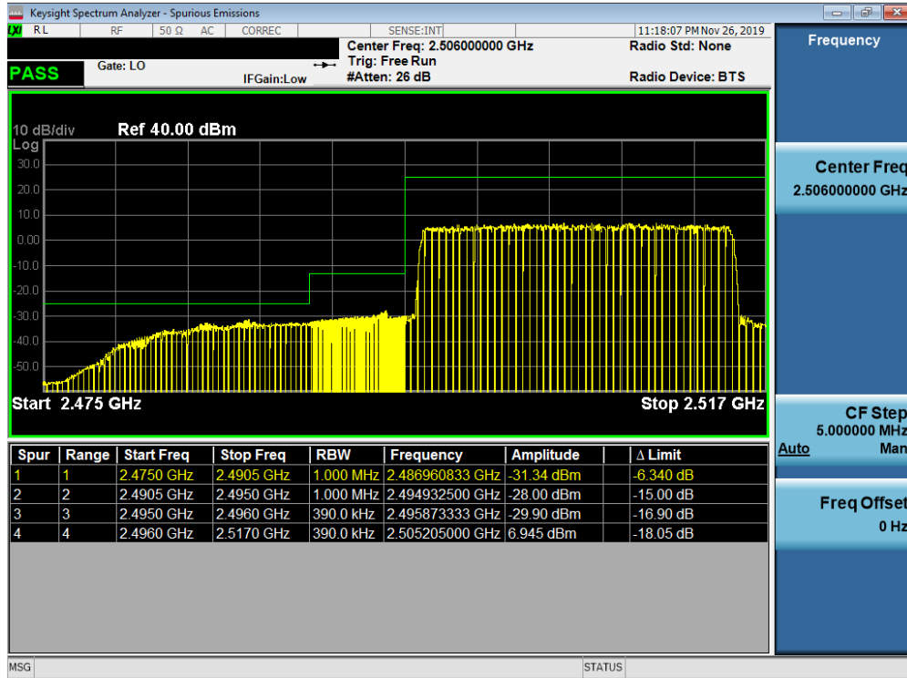
Plot 7-377. Lower ACP Plot at 2496 MHz (Band 41 PC3 - 20.0MHz QPSK - Full RB Configuration)
