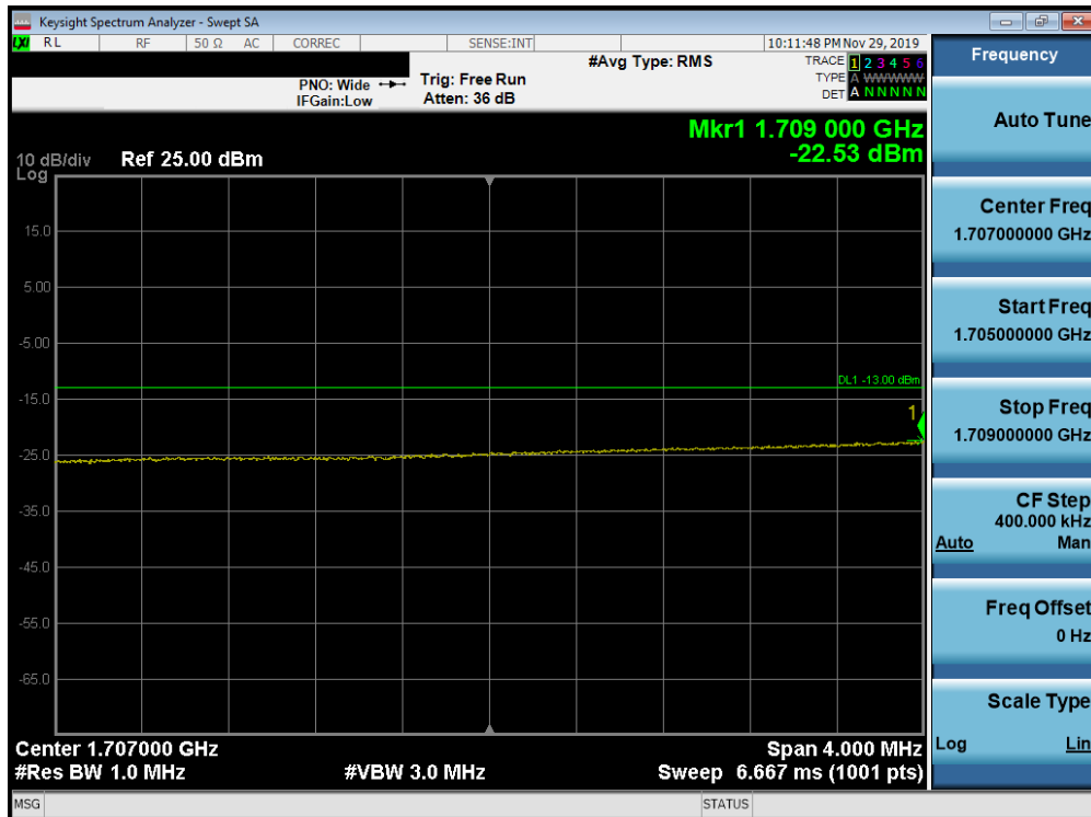
Plot 7-297. Lower Extended Band Edge Plot (Band 66/4 - 15.0MHz QPSK - Full RB Configuration)
