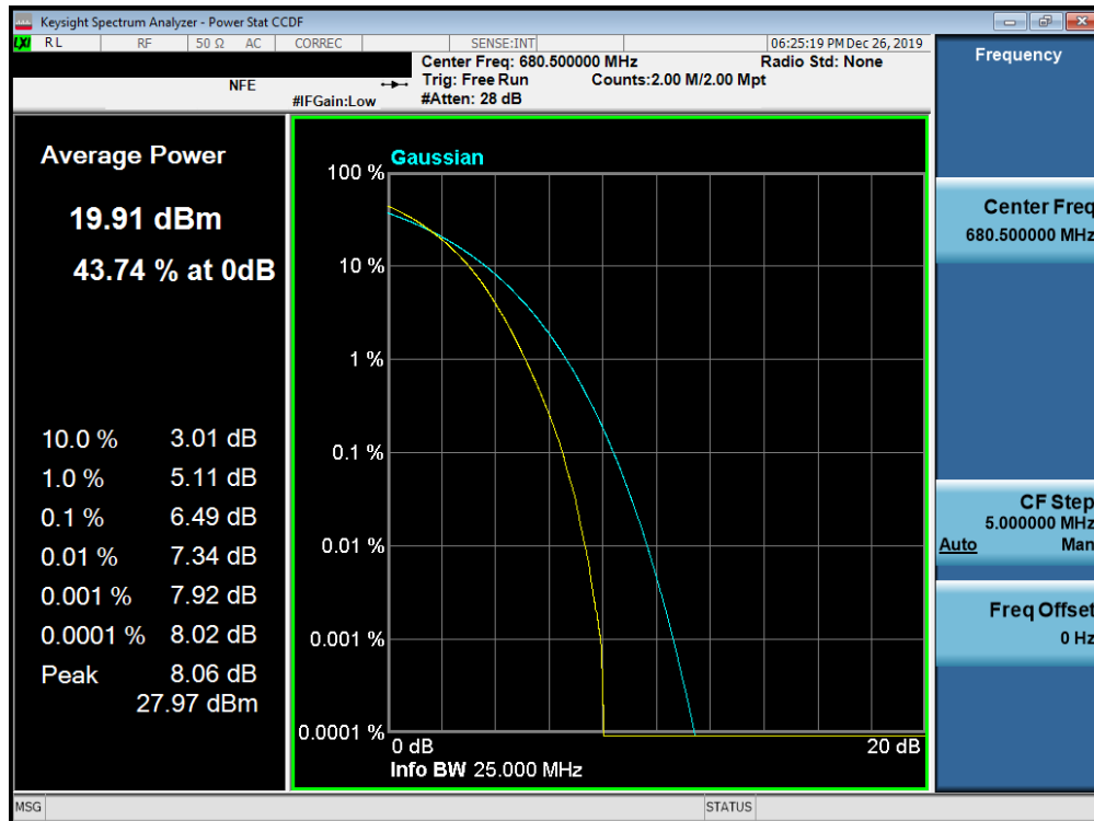
Plot 7-394. PAR Plot (Band 71 - 20.0MHz 256-QAM - Full RB Configuration)
