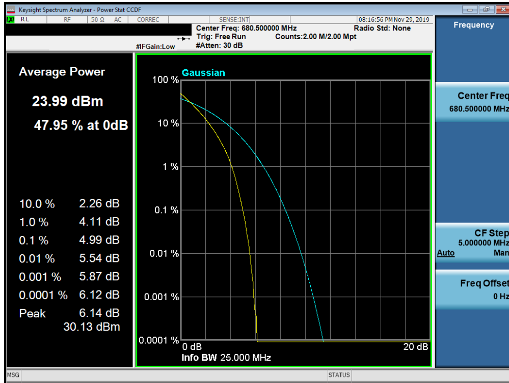
Plot 7-391. PAR Plot (Band 71 - 20.0MHz QPSK - Full RB Configuration)
