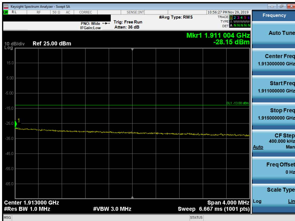
Plot 7-341. Upper Extended Band Edge Plot (Band 2 - 20.0MHz QPSK - Full RB Configuration)
