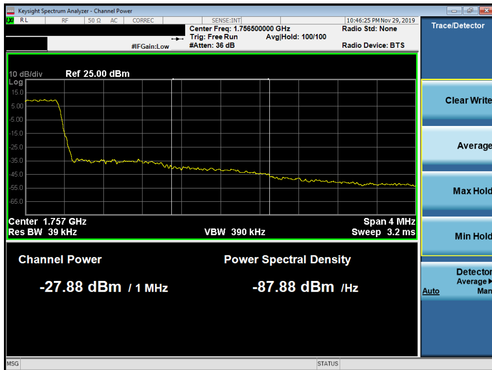
Plot 7-275. Upper Extended Band Edge Plot (Band 4 - 1.4MHz QPSK - Full RB Configuration)
