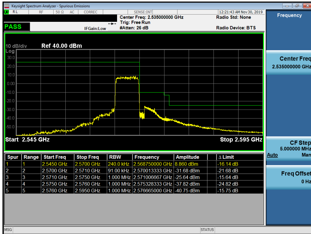
Plot 7-356. Higher ACP Plot (Band 7 - 5.0MHz QPSK - Full RB Configuration)
