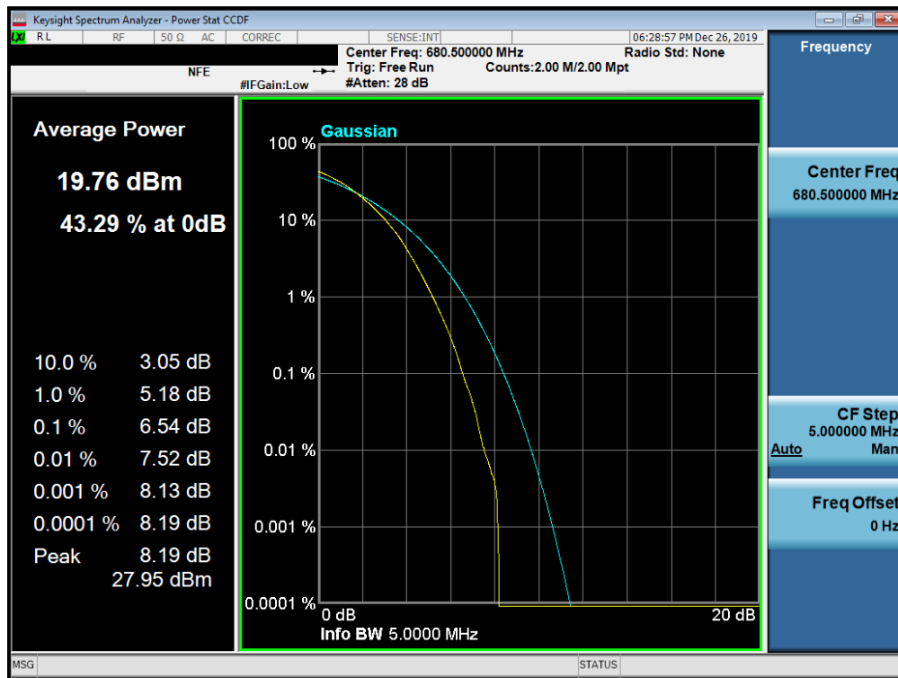
Plot 7-382. PAR Plot (Band 71 – 5.0MHz 256-QAM - Full RB Configuration)
