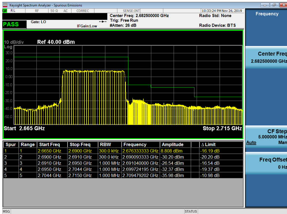
Plot 7-368. Upper ACP Plot (Band 41 PC2- 15.0MHz QPSK - Full RB Configuration)
