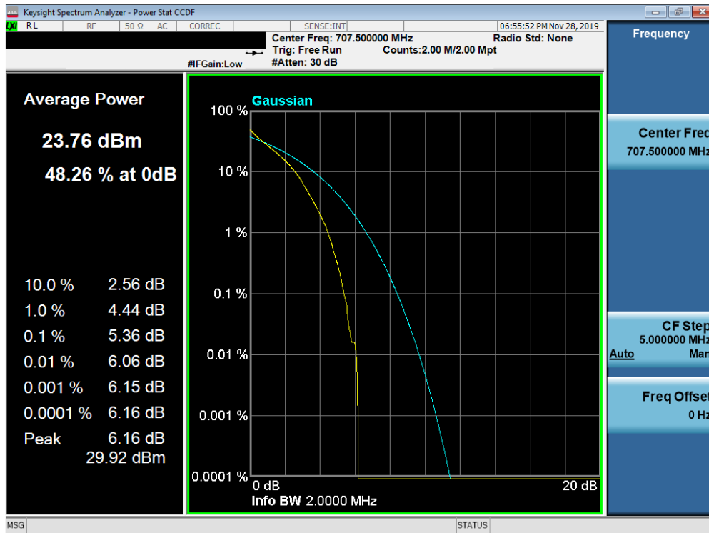
Plot 7-395. PAR Plot (Band 12 - 1.4MHz QPSK - Full RB Configuration)
