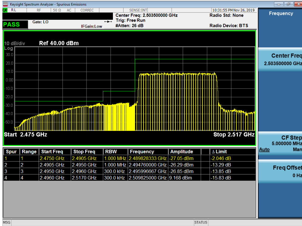
Plot 7-367. Lower ACP Plot at 2496 MHz (Band 41 PC2- 15.0MHz QPSK - Full RB Configuration)
