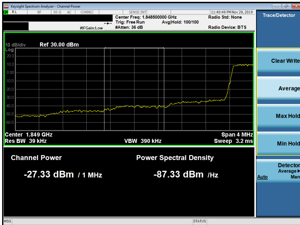
Plot 7-309. Lower Extended Band Edge Plot (Band 25/2 - 1.4MHz QPSK - Full RB Configuration)
