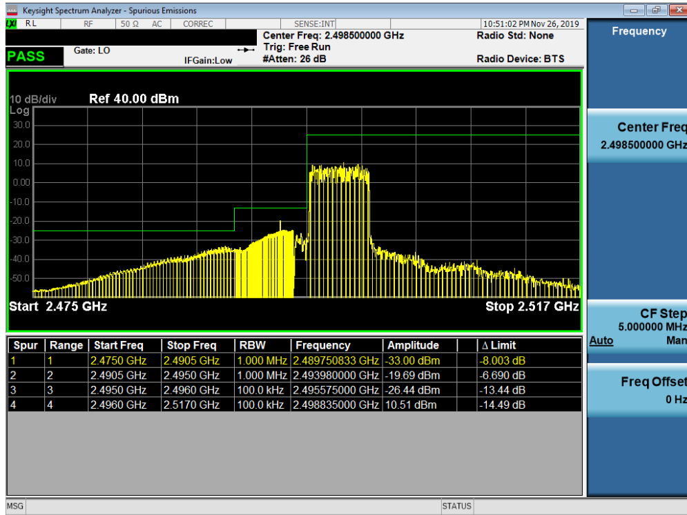
Plot 7-363. Lower ACP Plot at 2496 MHz (Band 41 PC2- 5.0MHz QPSK - Full RB Configuration)
