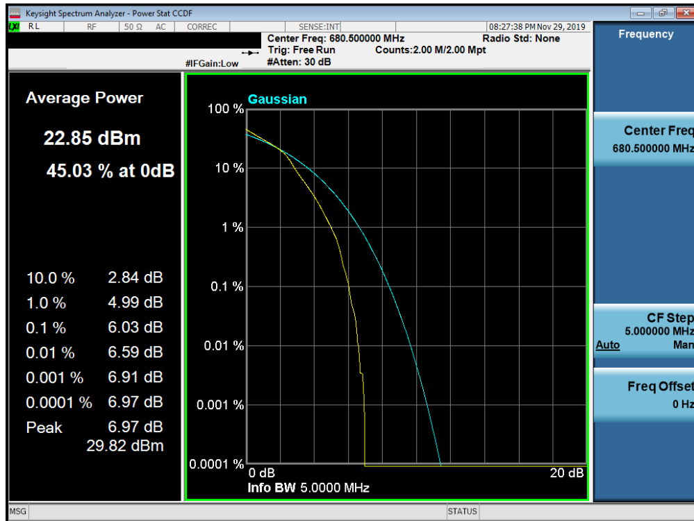
Plot 7-380. PAR Plot (Band 71 – 5.0MHz 16-QAM - Full RB Configuration)
