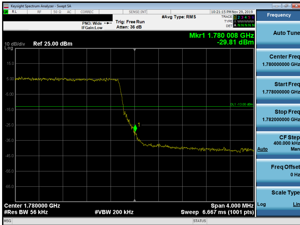
Plot 7-288. Upper Band Edge Plot (Band 66 - 5.0MHz QPSK - Full RB Configuration)
