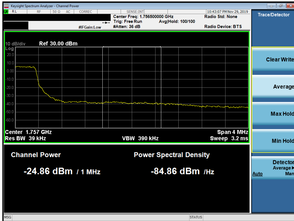
Plot 7-281. Upper Extended Band Edge Plot (Band 4 - 3.0MHz QPSK - Full RB Configuration)
