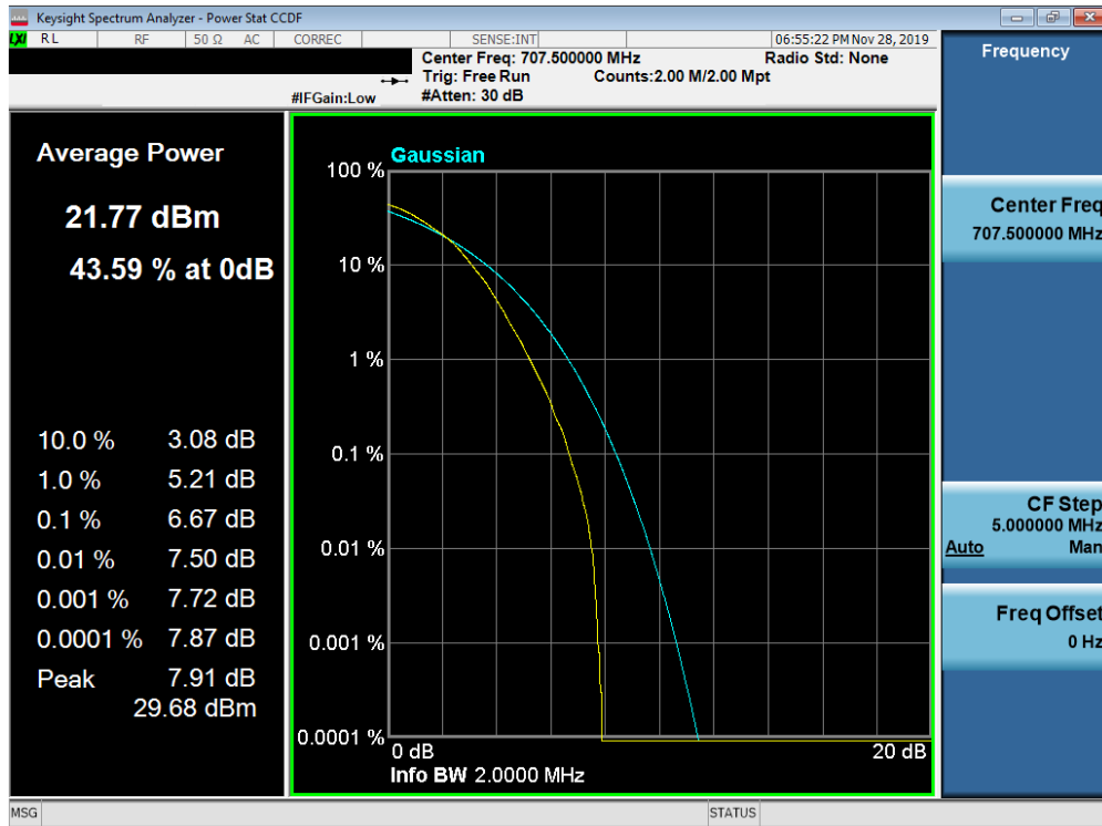
Plot 7-397. PAR Plot (Band 12 - 1.4MHz 64-QAM - Full RB Configuration)
