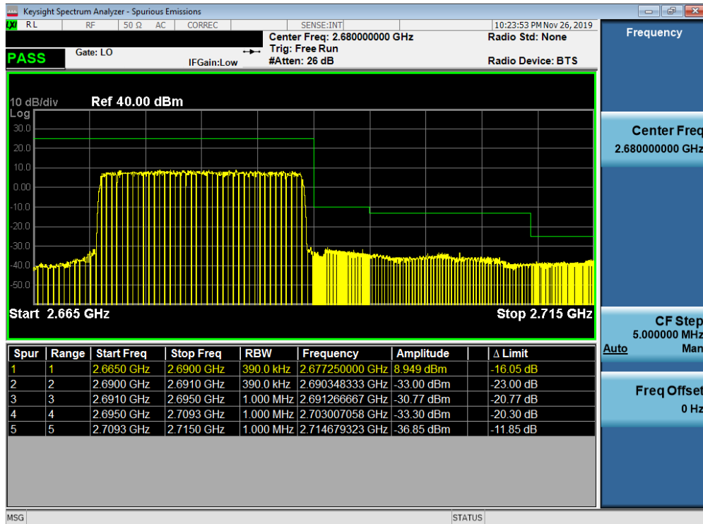
Plot 7-370. Upper ACP Plot (Band 41 PC2 - 20.0MHz QPSK - Full RB Configuration)
