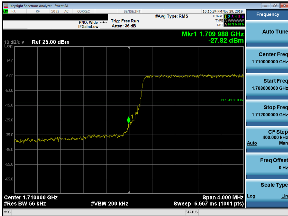
Plot 7-284. Lower Band Edge Plot (Band 66/4 - 5.0MHz QPSK - Full RB Configuration)
