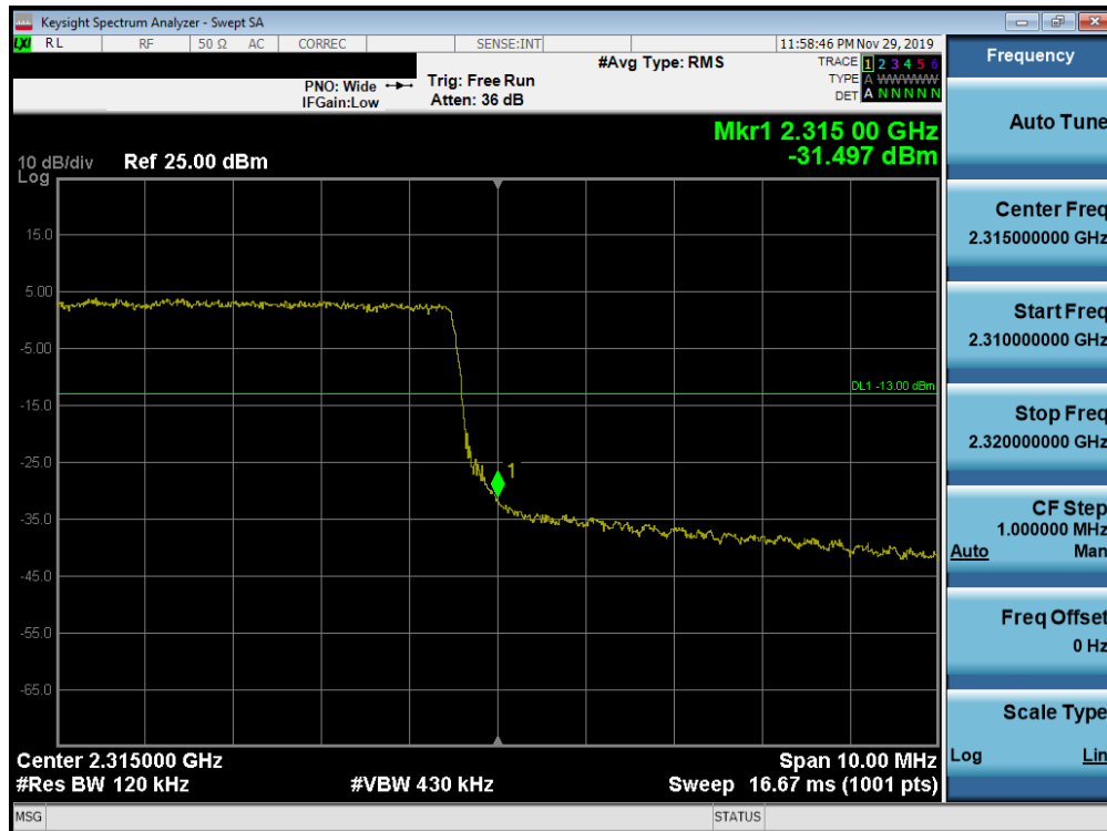
Plot 7-353. Upper Band Edge Plot (Band 30 - 10.0MHz QPSK - Full RB Configuration)
