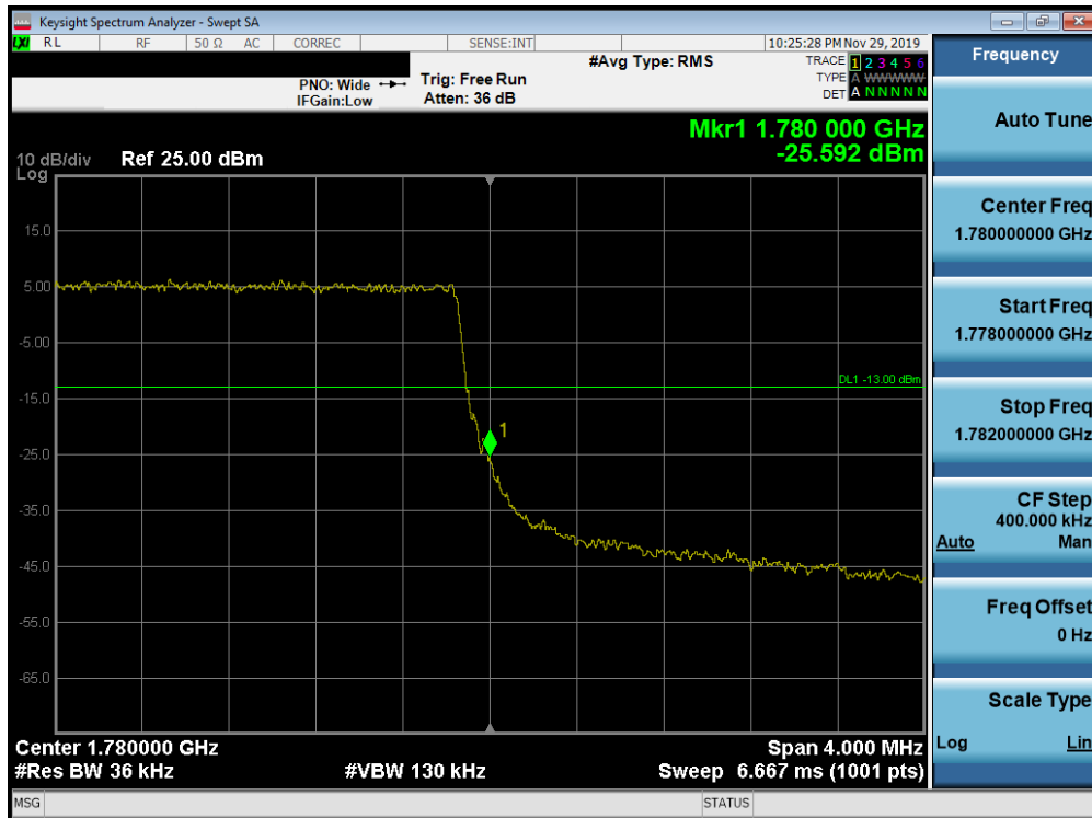
Plot 7-282. Upper Band Edge Plot (Band 66 - 3.0MHz QPSK - Full RB Configuration)
