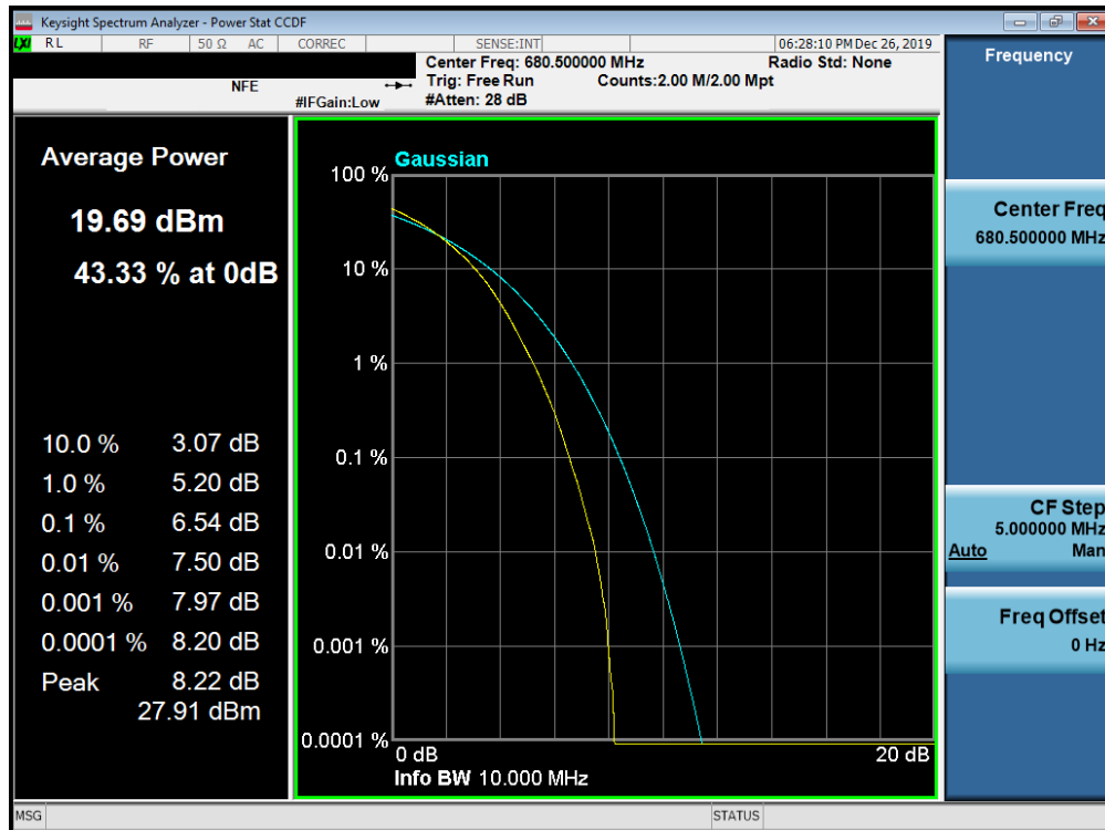
Plot 7-386. PAR Plot (Band 71 - 10.0MHz 256-QAM - Full RB Configuration)
