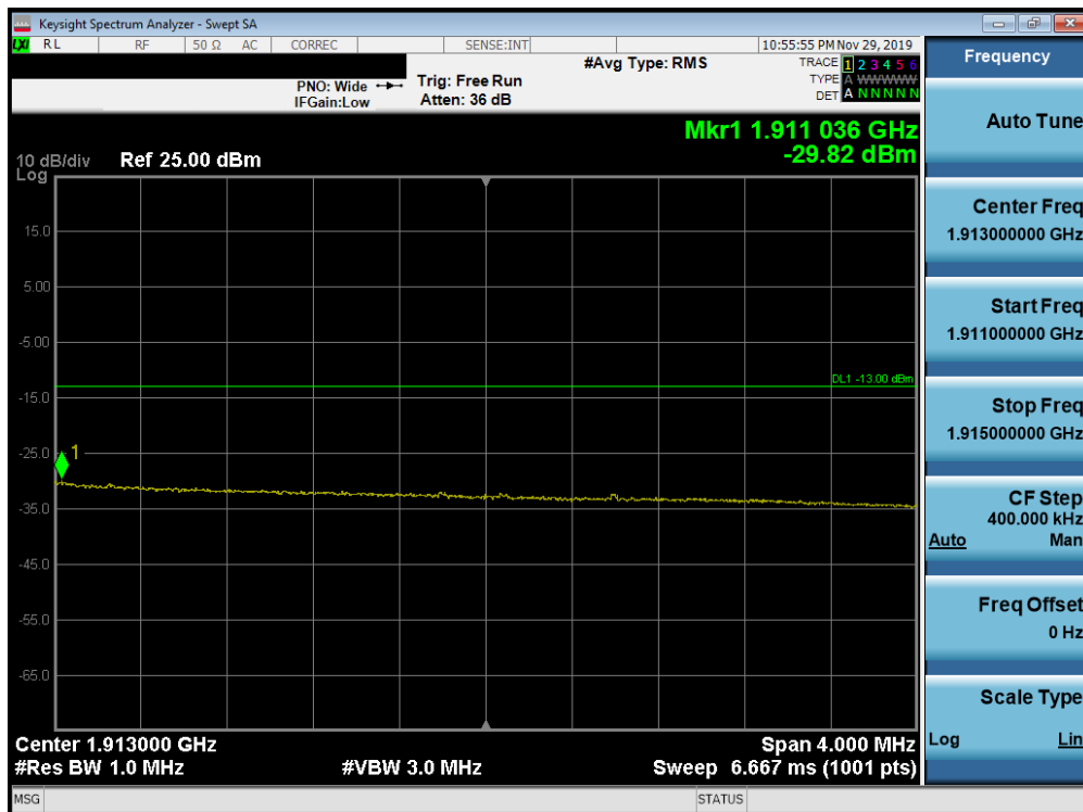
Plot 7-335. Upper Extended Band Edge Plot (Band 2 - 15.0MHz QPSK - Full RB Configuration)
