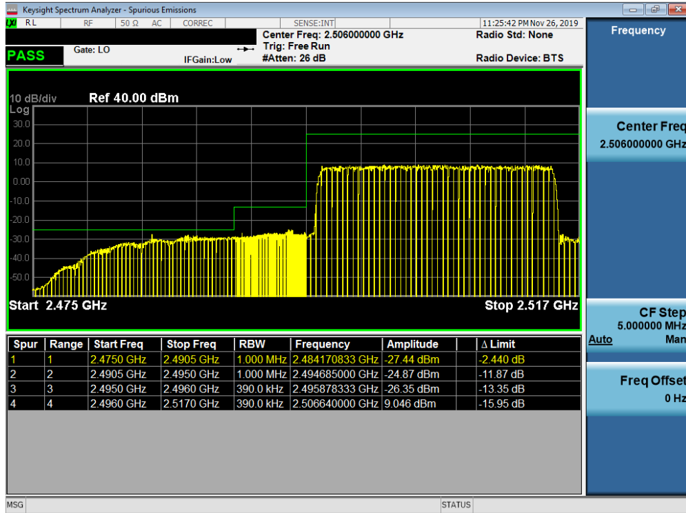
Plot 7-369. Lower ACP Plot at 2496 MHz (Band 41 PC2 - 20.0MHz QPSK - Full RB Configuration)
