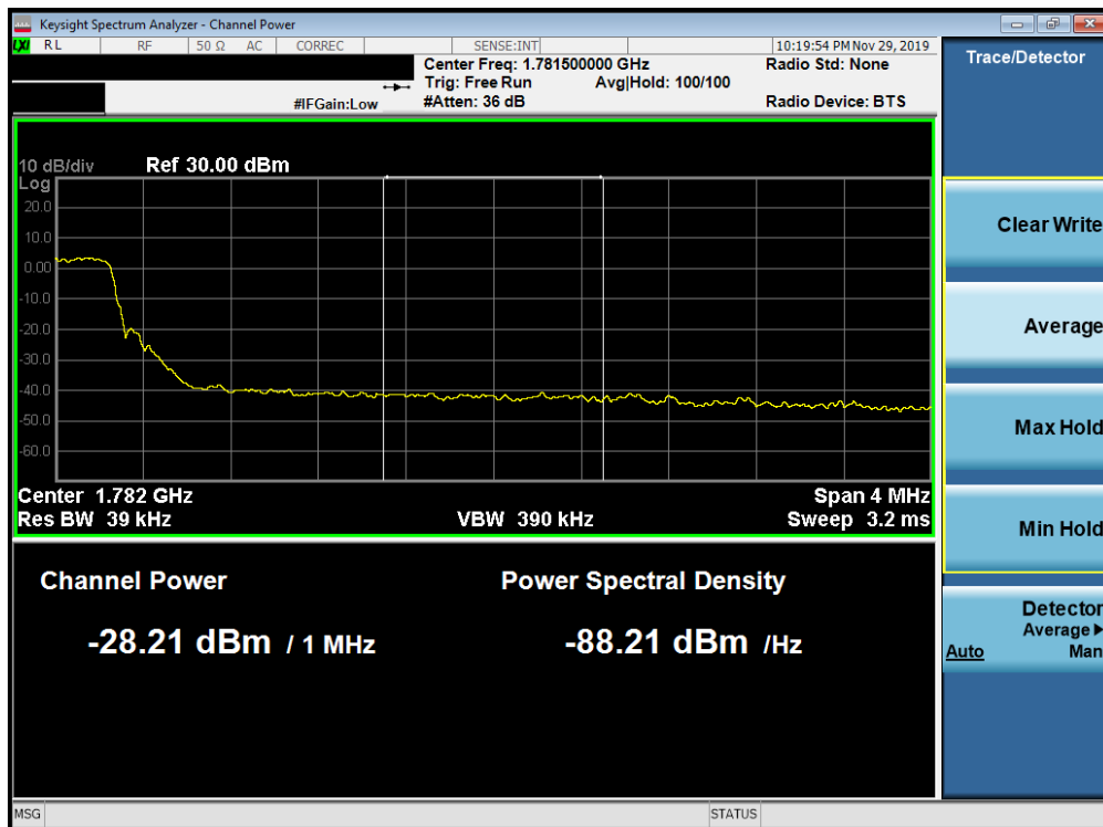
Plot 7-289. Upper Extended Band Edge Plot (Band 66 - 5.0MHz QPSK - Full RB Configuration)
