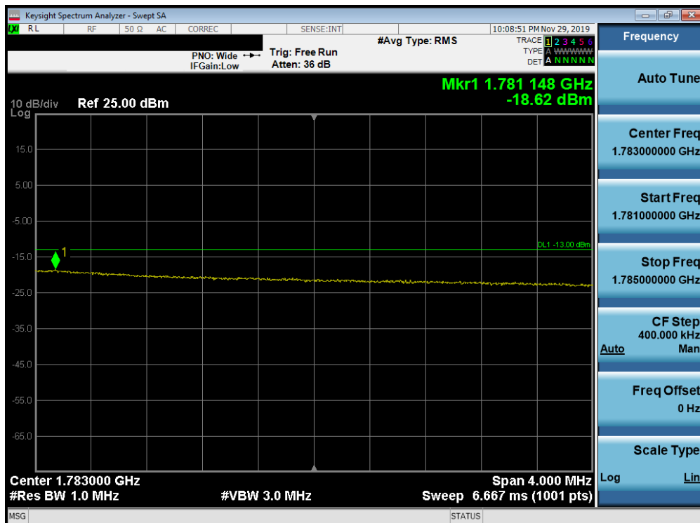
Plot 7-307. Upper Extended Band Edge Plot (Band 66 - 20.0MHz QPSK - Full RB Configuration)
