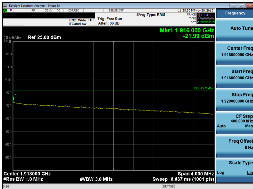
Plot 7-331. Upper Extended Band Edge Plot (Band 25 - 10.0MHz QPSK - Full RB Configuration)
