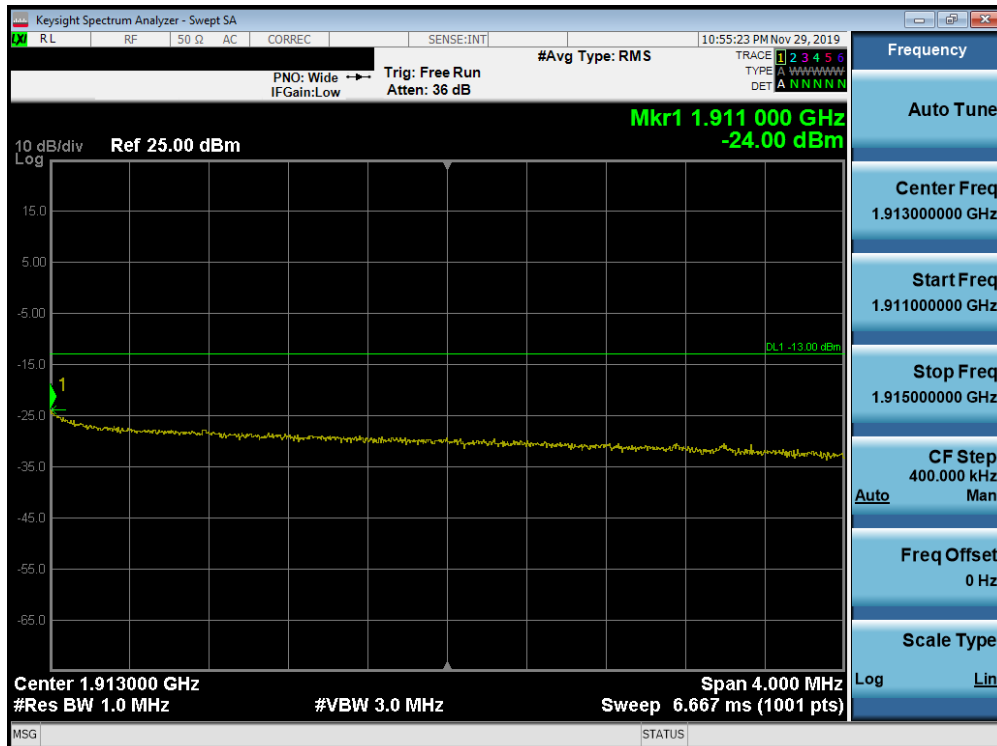
Plot 7-329. Upper Extended Band Edge Plot (Band 2 - 10.0MHz QPSK - Full RB Configuration)
