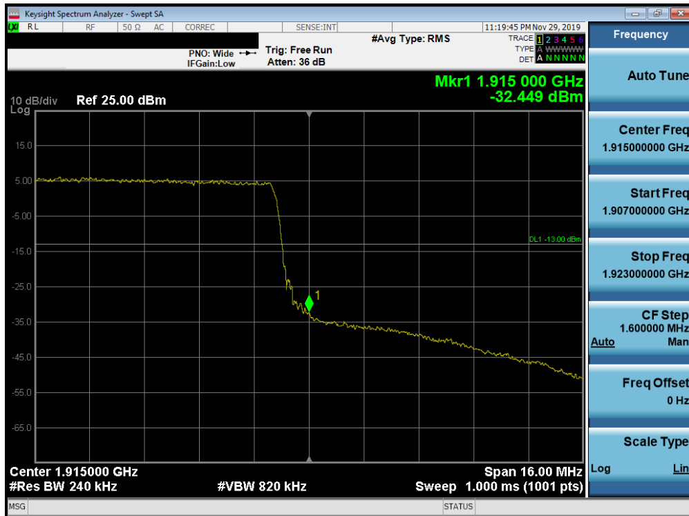
Plot 7-342. Upper Band Edge Plot (Band 25 - 20.0MHz QPSK - Full RB Configuration)
