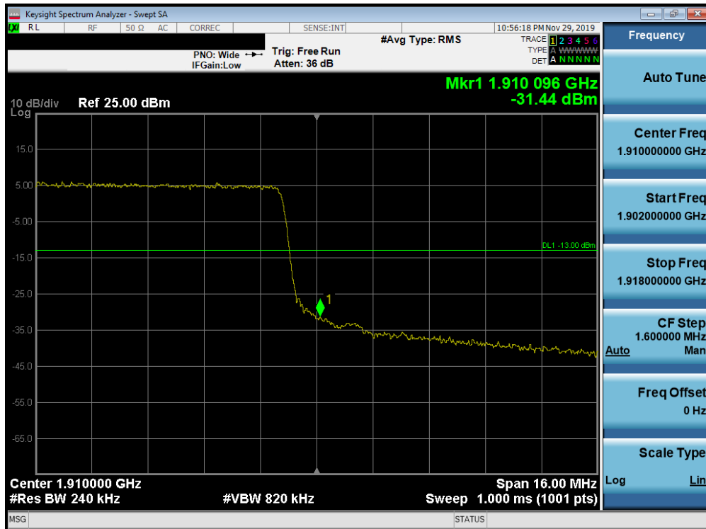
Plot 7-340. Upper Band Edge Plot (Band 2 - 20.0MHz QPSK - Full RB Configuration)
