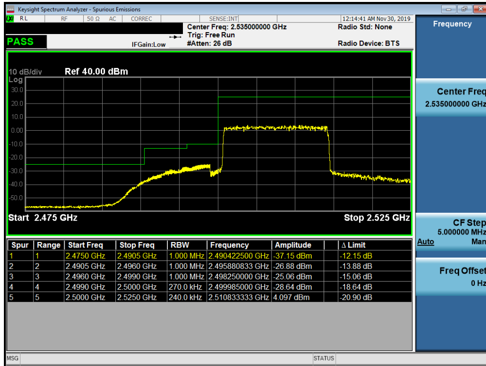
Plot 7-359. Lower ACP Plot (Band 7 - 15.0MHz QPSK - Full RB Configuration)
