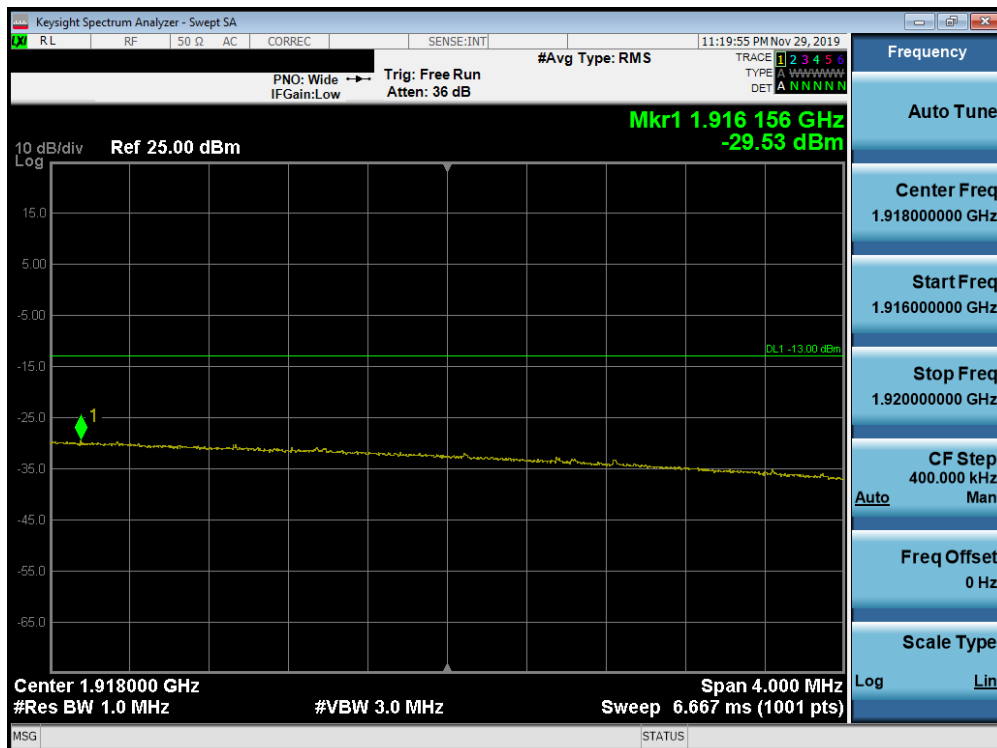
Plot 7-343. Upper Extended Band Edge Plot (Band 25 - 20.0MHz QPSK - Full RB Configuration)
