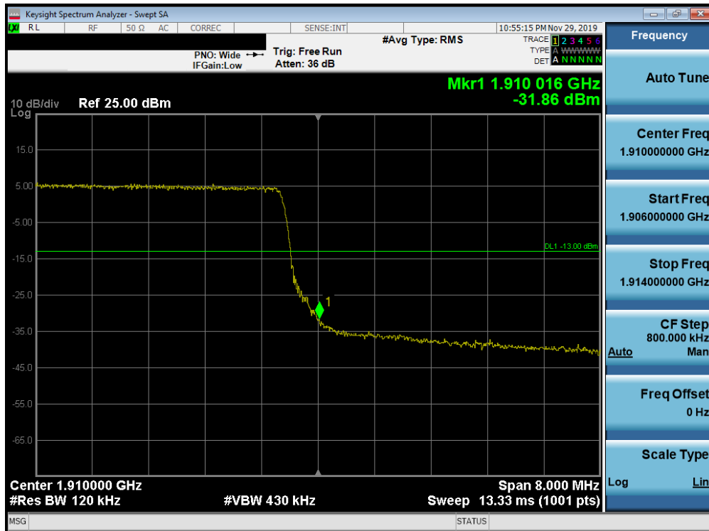
Plot 7-328. Upper Band Edge Plot (Band 2 - 10.0MHz QPSK - Full RB Configuration)
