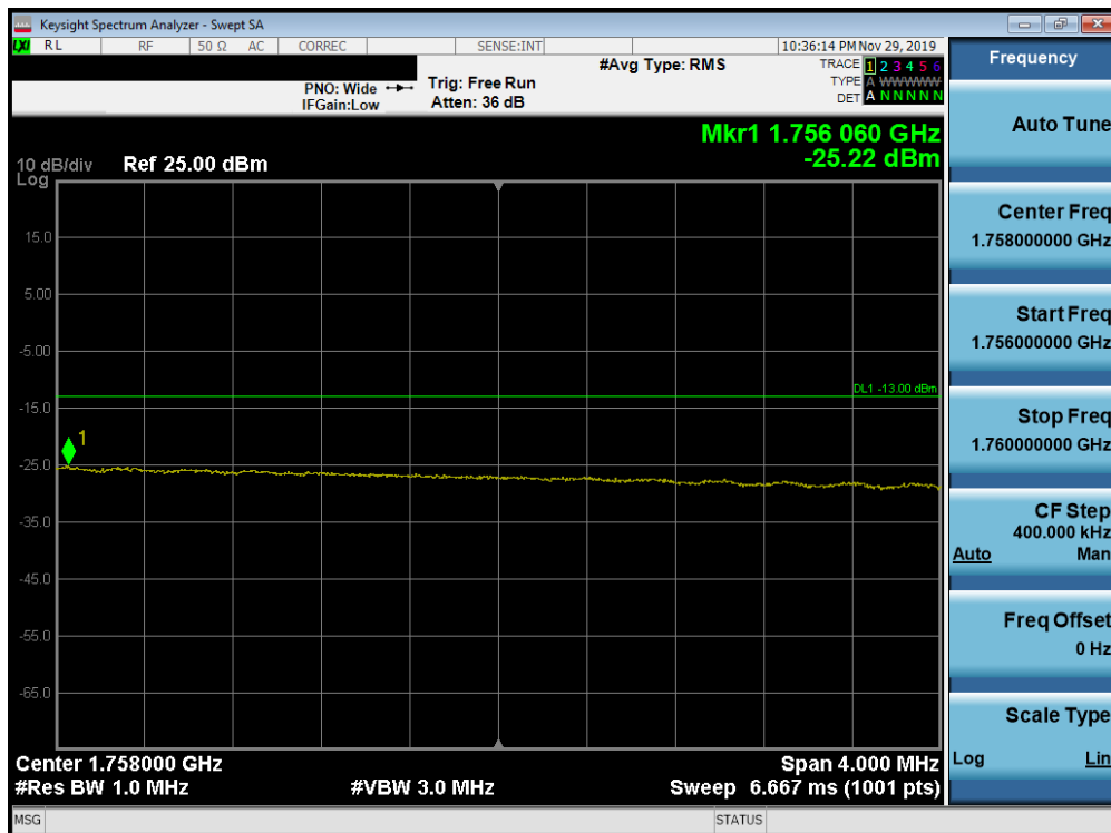
Plot 7-305. Upper Extended Band Edge Plot (Band 4 - 20.0MHz QPSK - Full RB Configuration)
