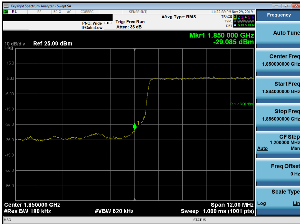
Plot 7-332. Lower Band Edge Plot (Band 25/2 - 15.0MHz QPSK - Full RB Configuration)
