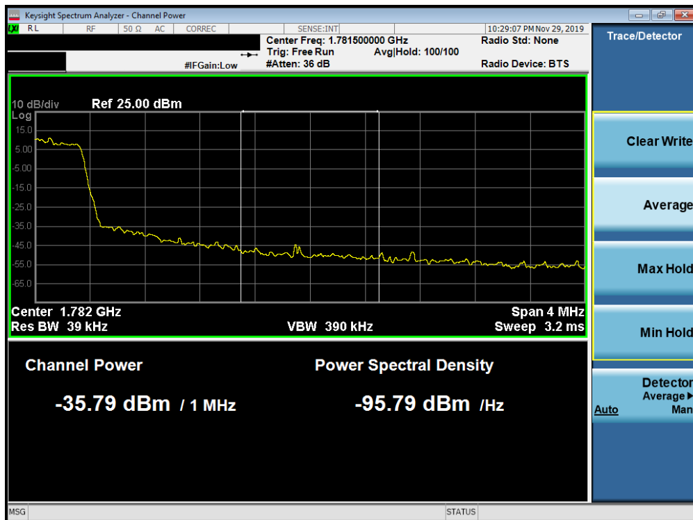
Plot 7-277. Upper Extended Band Edge Plot (Band 66 - 1.4MHz QPSK - Full RB Configuration)
