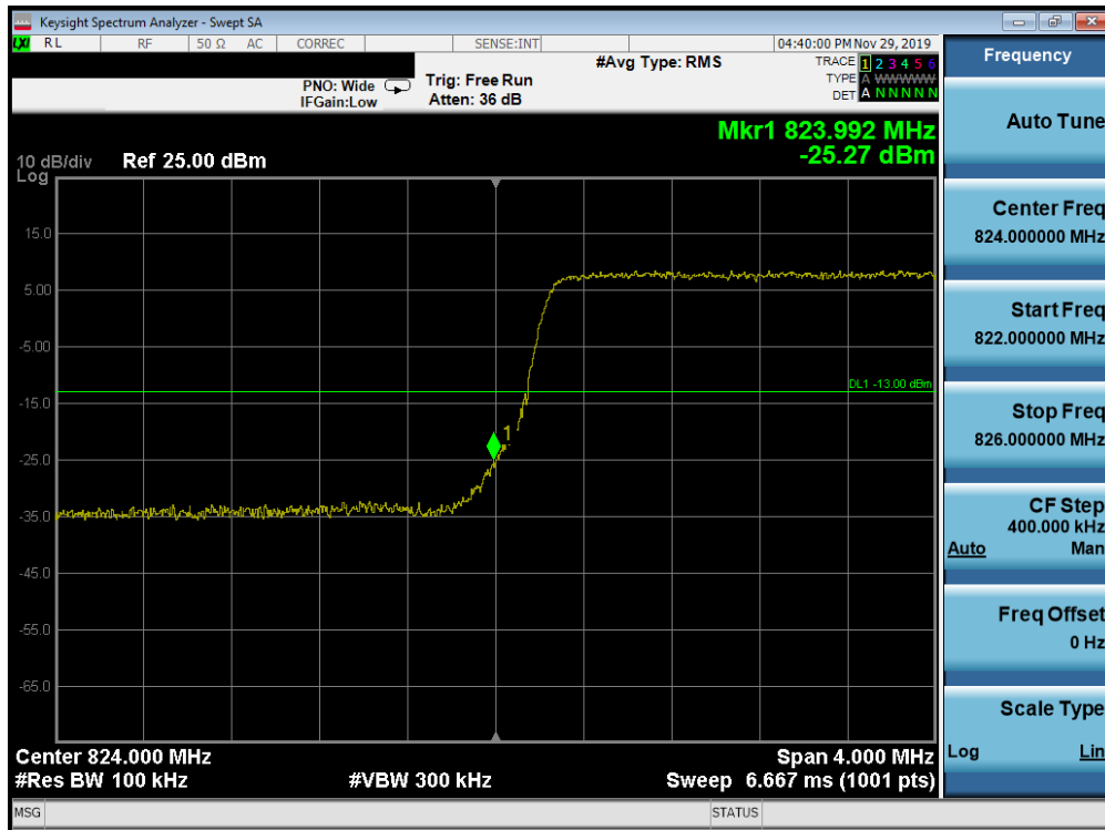
Plot 7-266. Lower Band Edge Plot (Band 26/5 - 5.0MHz QPSK - Full RB Configuration)
