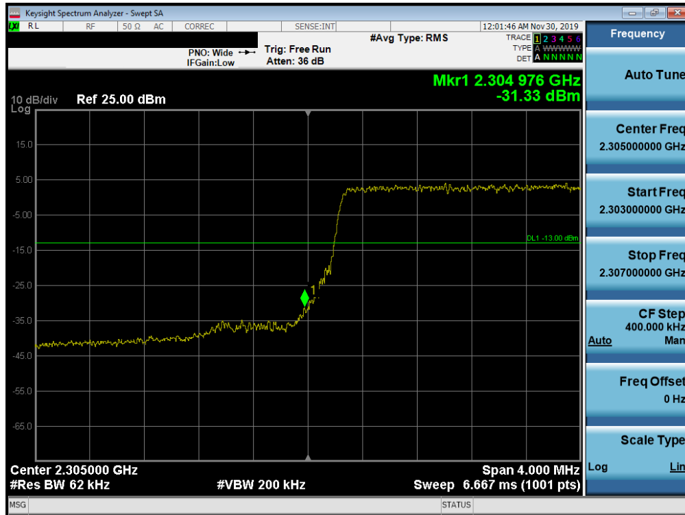
Plot 7-344. Lower Band Edge Plot (Band 30 - 5.0MHz QPSK - Full RB Configuration)
