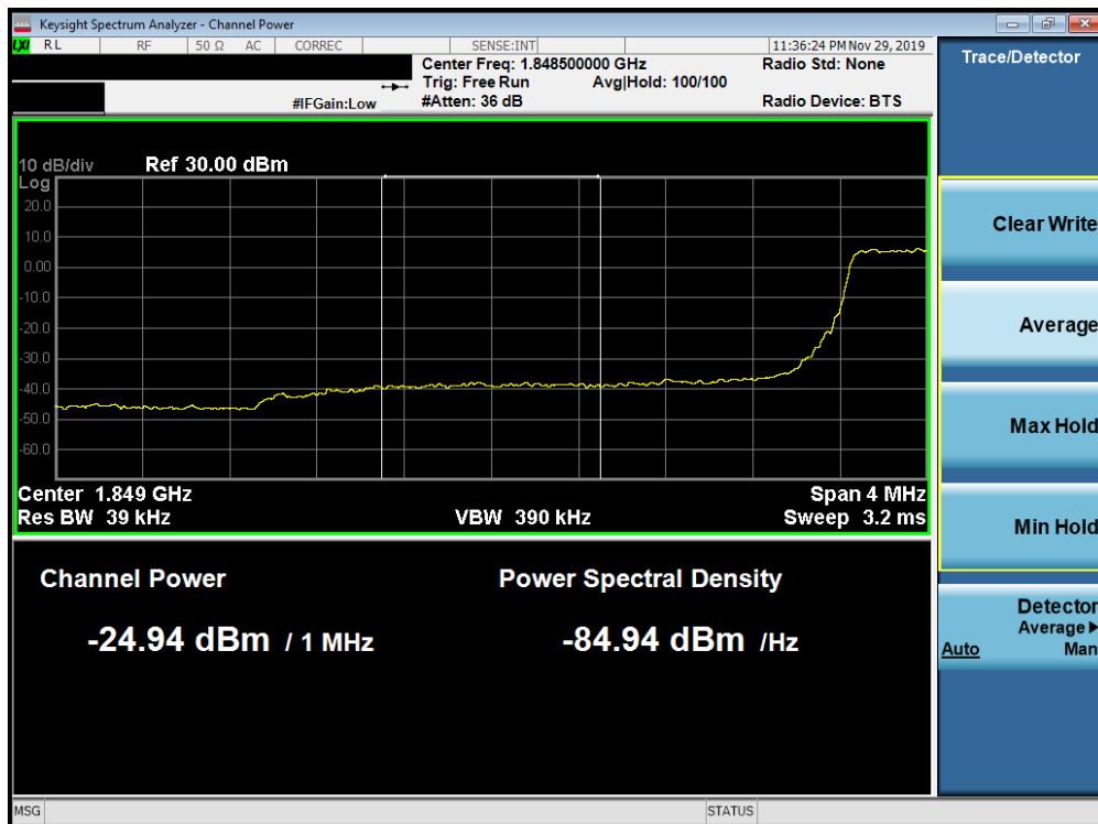
Plot 7-315. Lower Extended Band Edge Plot (Band 25/2 - 3.0MHz QPSK - Full RB Configuration)
