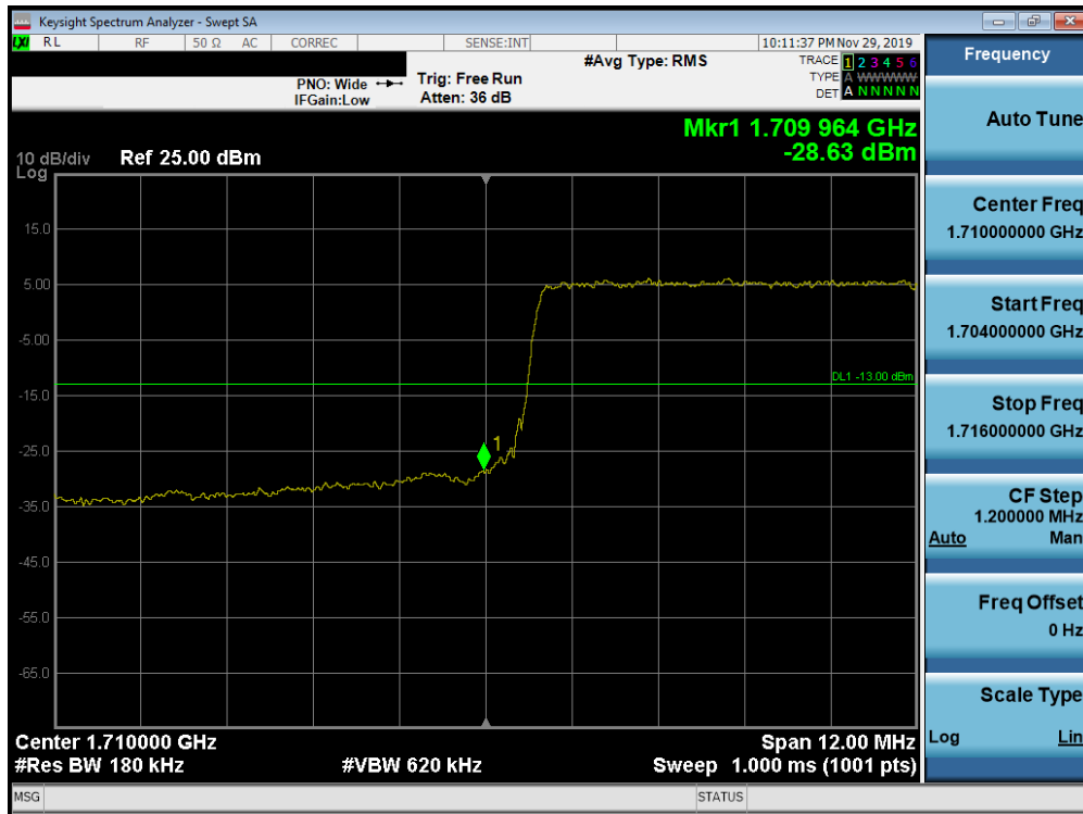
Plot 7-296. Lower Band Edge Plot (Band 66/4 - 15.0MHz QPSK - Full RB Configuration)
