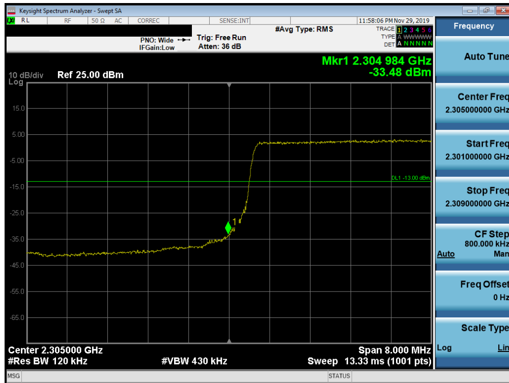
Plot 7-348. Lower Band Edge Plot (Band 30 - 10.0MHz QPSK - Full RB Configuration)
