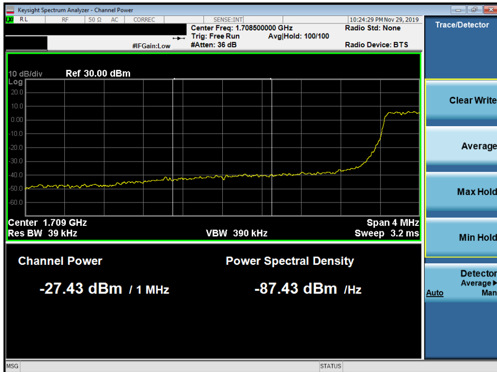
Plot 7-279. Lower Extended Band Edge Plot (Band 66/4 - 3.0MHz QPSK - Full RB Configuration)
