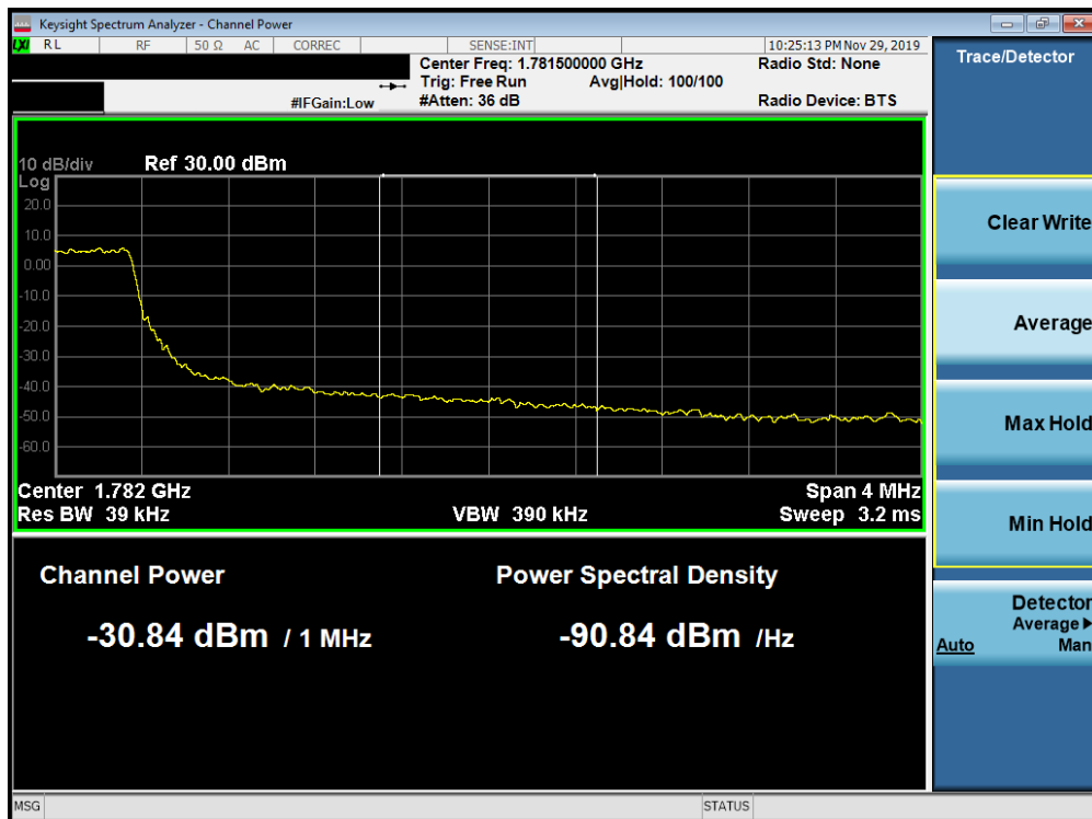
Plot 7-283. Upper Extended Band Edge Plot (Band 66 - 3.0MHz QPSK - Full RB Configuration)
