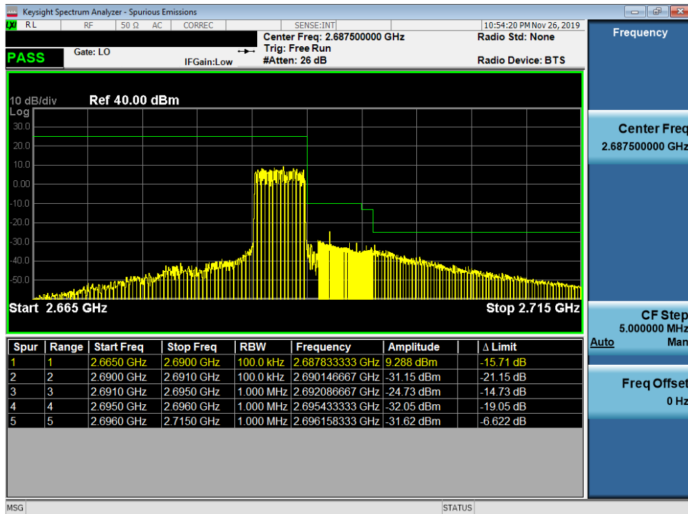
Plot 7-364. Upper ACP Plot (Band 41 PC2- 5.0MHz QPSK - Full RB Configuration)
