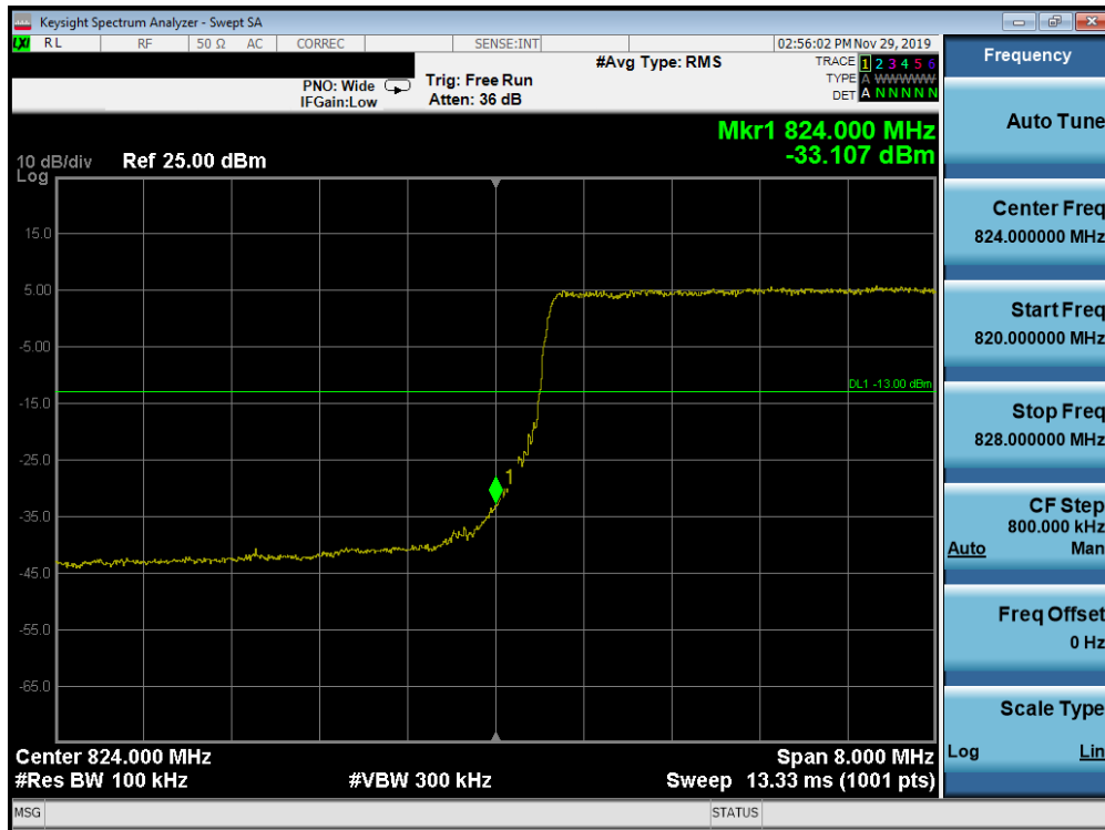
Plot 7-268. Lower Band Edge Plot (Band 26/5 - 10.0MHz QPSK - Full RB Configuration)
