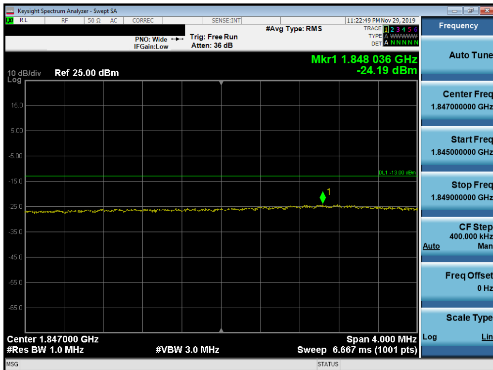
Plot 7-333. Lower Extended Band Edge Plot (Band 25/2 - 15.0MHz QPSK - Full RB Configuration)
