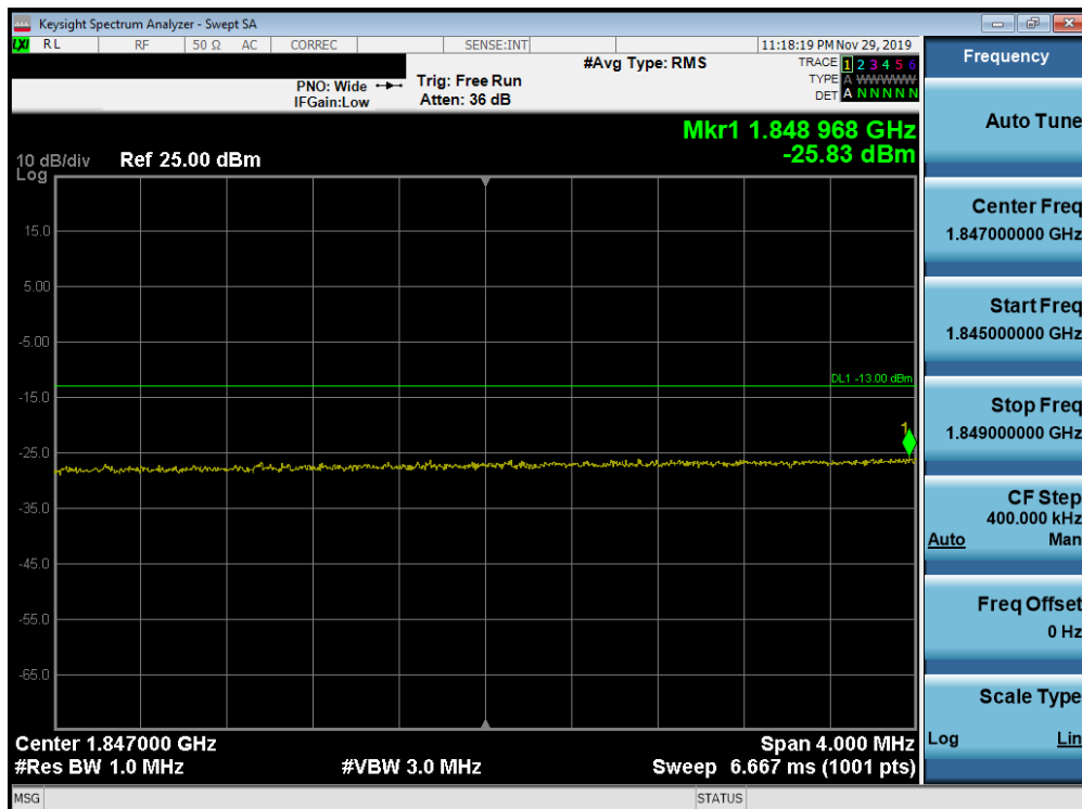
Plot 7-339. Lower Extended Band Edge Plot (Band 25/2 - 20.0MHz QPSK - Full RB Configuration)
