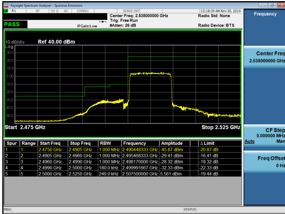
Plot 7-357. Lower ACP Plot (Band 7 - 10.0MHz QPSK - Full RB Configuration)
