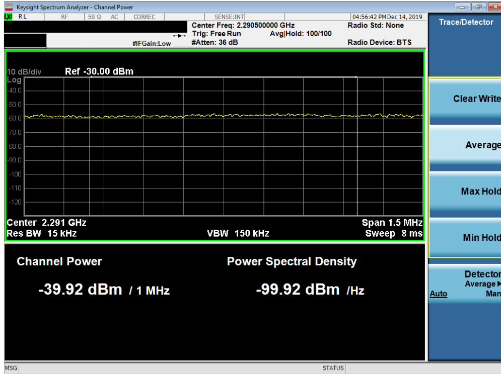
Plot 7-350. Lower Extended Band Edge Plot (Band 30 - 10.0MHz QPSK - Full RB Configuration)
