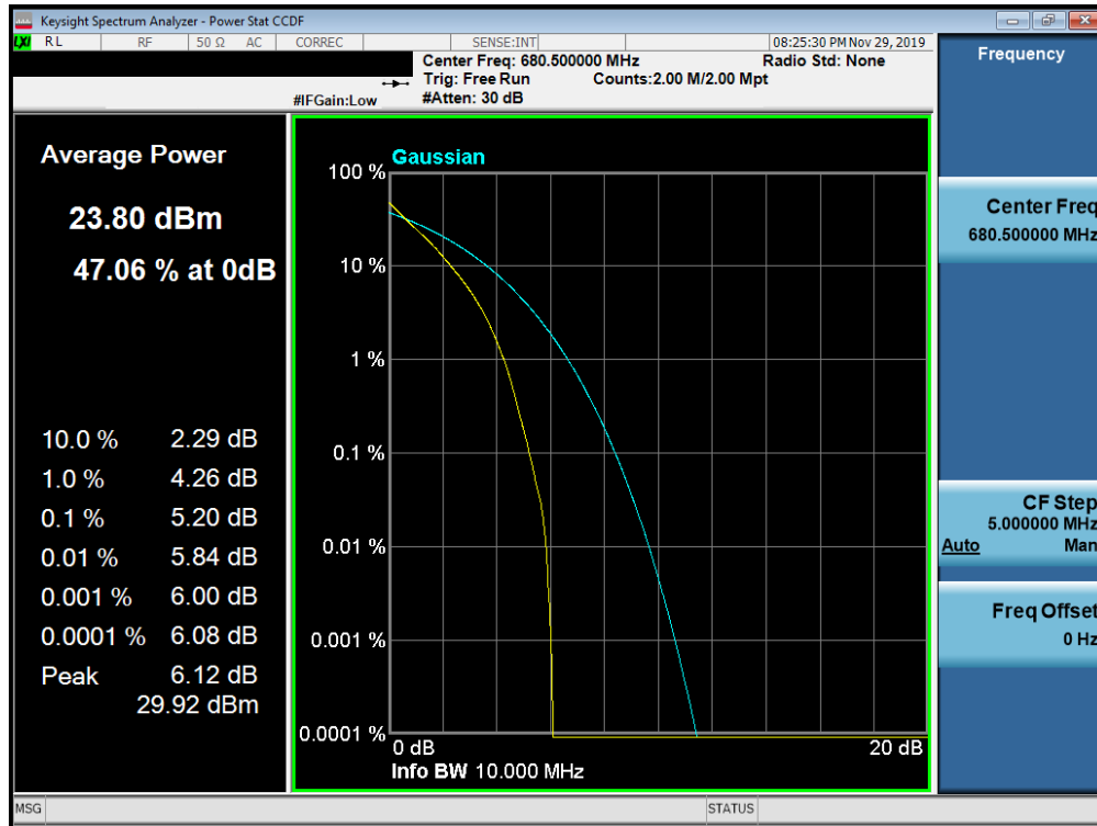
Plot 7-383. PAR Plot (Band 71 - 10.0MHz QPSK - Full RB Configuration)
