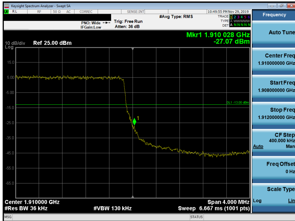
Plot 7-316. Upper Band Edge Plot (Band 2 - 3.0MHz QPSK - Full RB Configuration)
