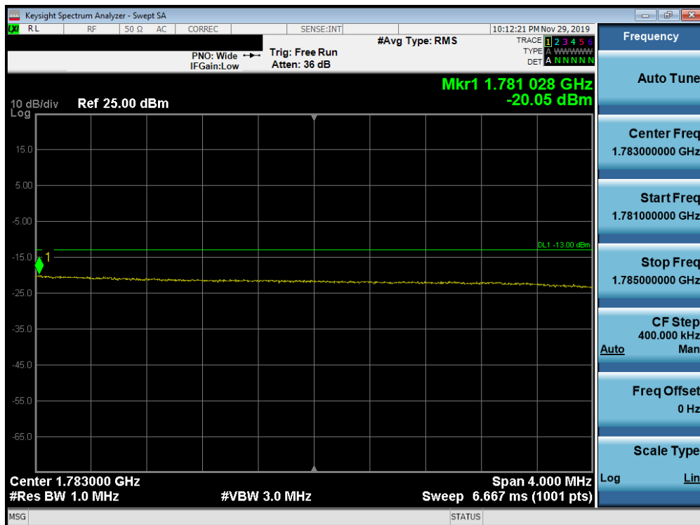
Plot 7-301. Upper Extended Band Edge Plot (Band 66 - 15.0MHz QPSK - Full RB Configuration)
