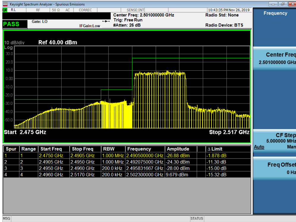
Plot 7-365. Lower ACP Plot at 2496 MHz (Band 41 PC2- 10.0MHz QPSK - Full RB Configuration)
