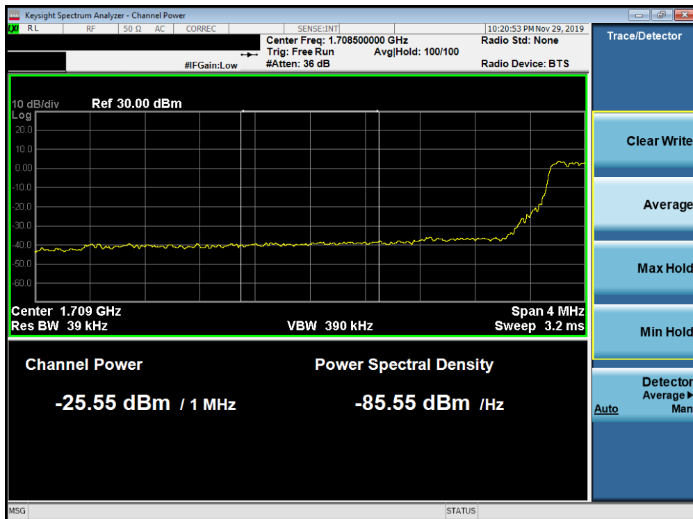
Plot 7-285. Lower Extended Band Edge Plot (Band 66/4 - 5.0MHz QPSK - Full RB Configuration)
