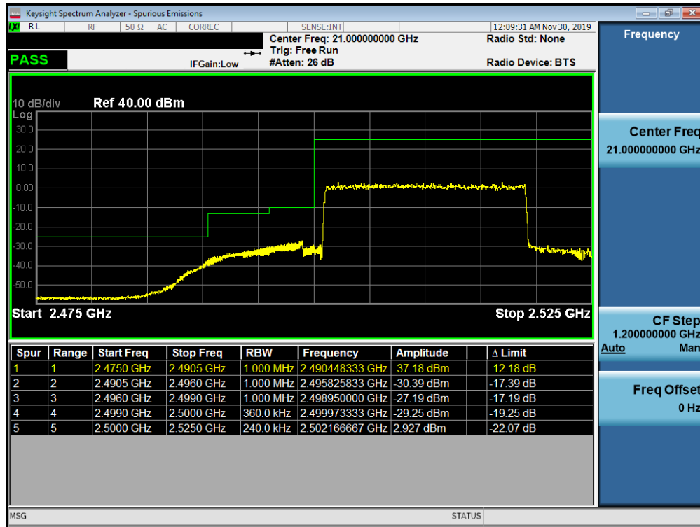
Plot 7-361. Lower ACP Plot (Band 7 - 20.0MHz QPSK - Full RB Configuration)
