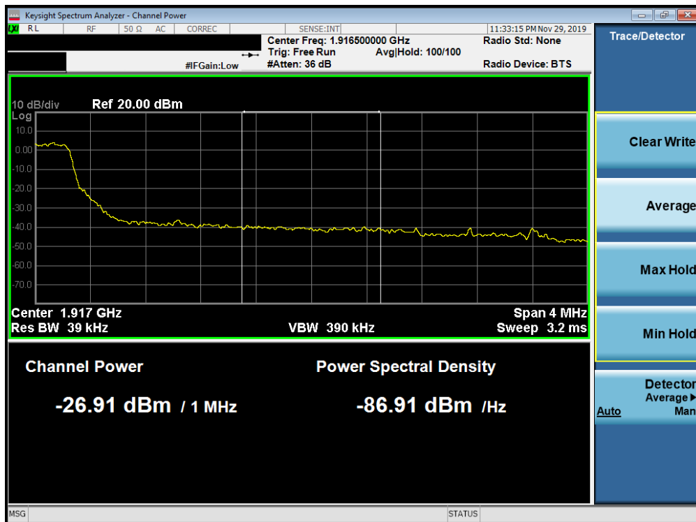
Plot 7-325. Upper Extended Band Edge Plot (Band 25 - 5.0MHz QPSK - Full RB Configuration)
