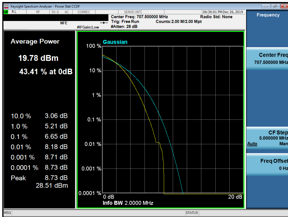
Plot 7-398. PAR Plot (Band 12 - 1.4MHz 256-QAM - Full RB Configuration)
