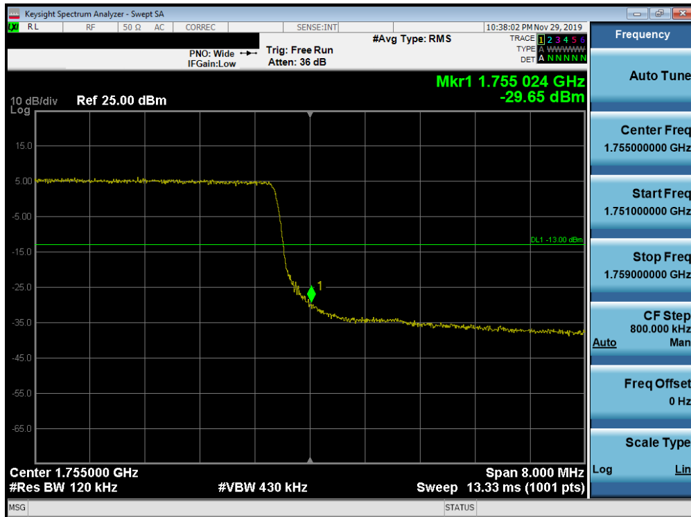
Plot 7-292. Upper Band Edge Plot (Band 4 - 10.0MHz QPSK - Full RB Configuration)
