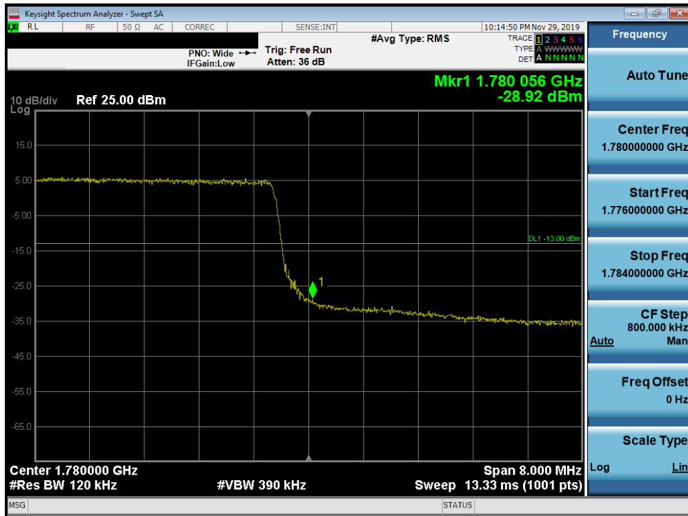
Plot 7-294. Upper Band Edge Plot (Band 66 - 10.0MHz QPSK - Full RB Configuration)
