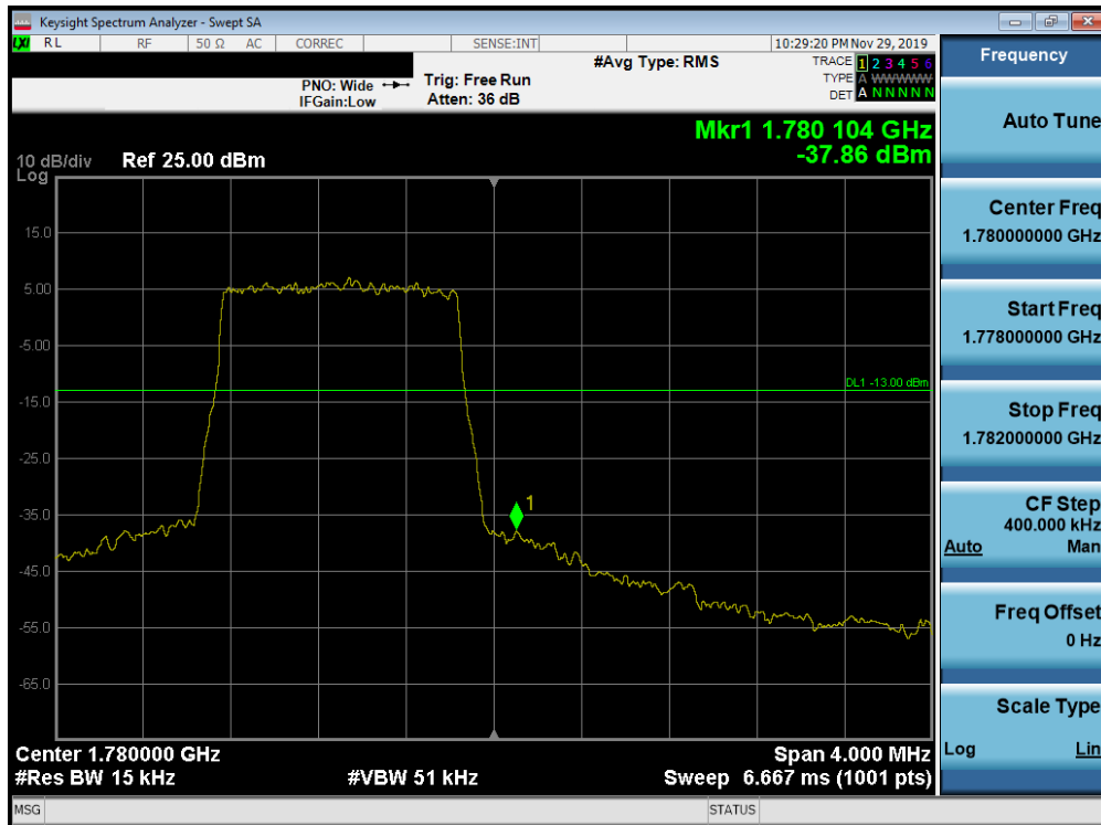
Plot 7-276. Upper Band Edge Plot (Band 66 - 1.4MHz QPSK - Full RB Configuration)
