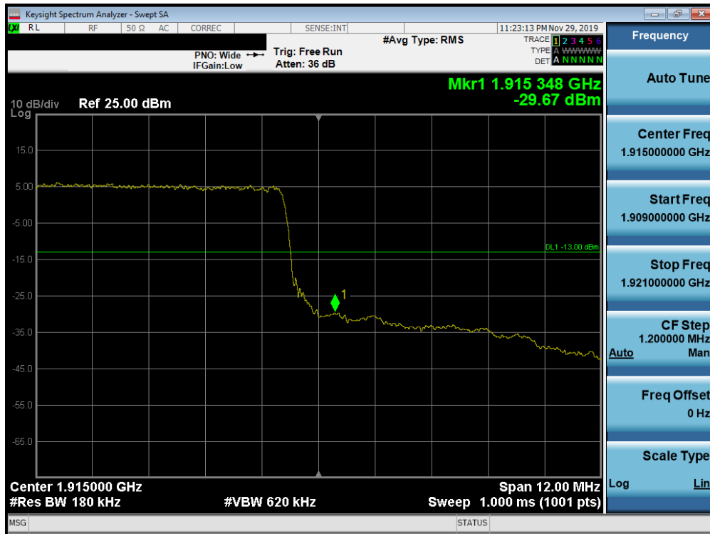
Plot 7-336. Upper Band Edge Plot (Band 25 - 15.0MHz QPSK - Full RB Configuration)
