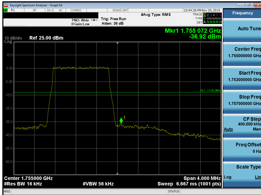
Plot 7-274. Upper Band Edge Plot (Band 4 - 1.4MHz QPSK - Full RB Configuration)
