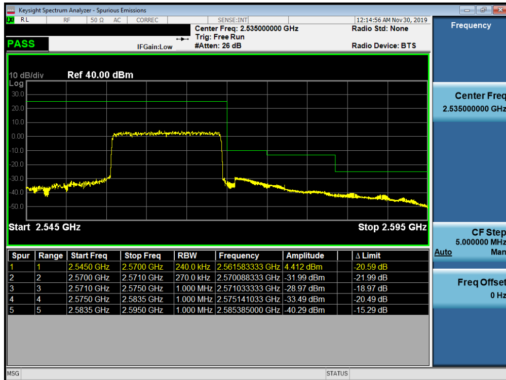
Plot 7-360. Higher ACP Plot (Band 7 - 15.0MHz QPSK - Full RB Configuration)
