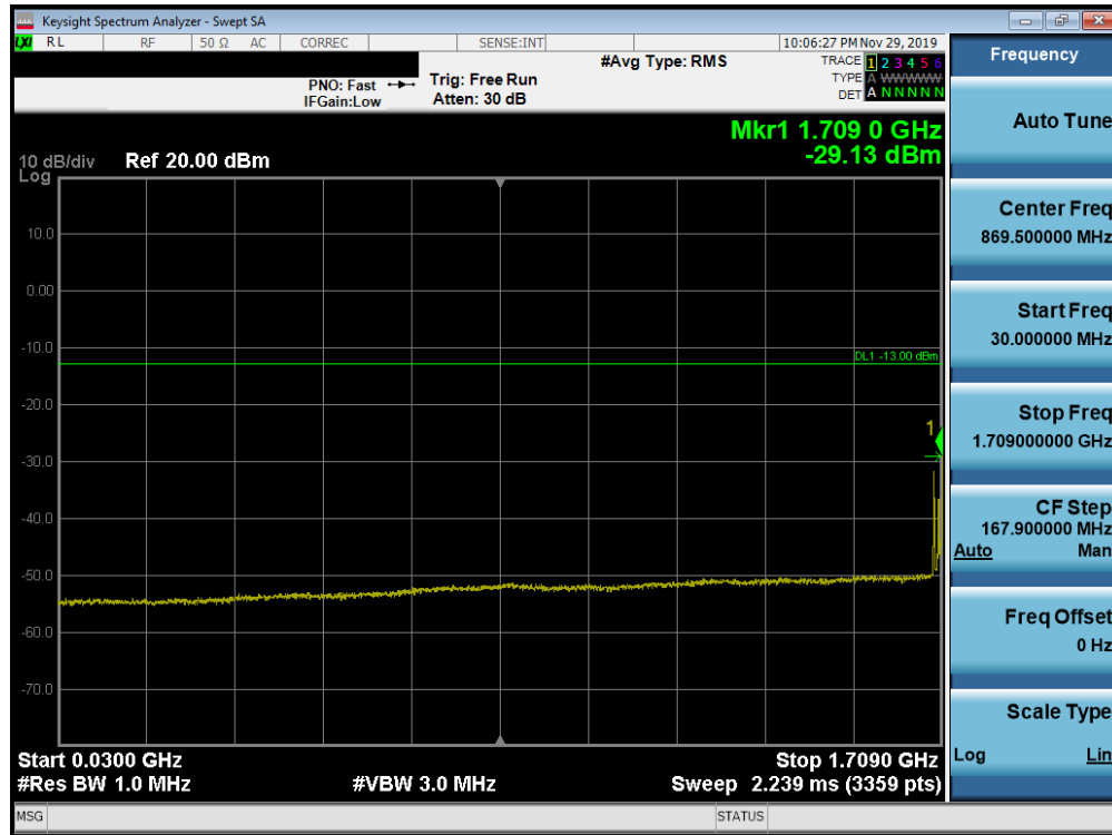
Plot 7-188. Conducted Spurious Plot (Band 66/4 - 20.0MHz QPSK - RB Size 1, RB Offset 0 - Low Channel)
