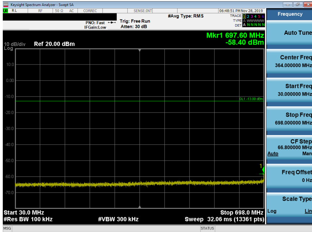
Plot 7-164. Conducted Spurious Plot (Band 12/17 - 10.0MHz QPSK - RB Size 1, RB Offset 0 - High Channel)
