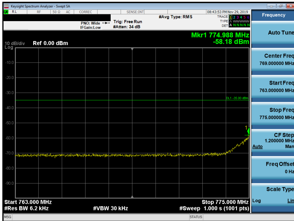
Plot 7-255. Lower Emission Mask Plot (Band 13 - 5.0MHz QPSK - Full RB Configuration)
