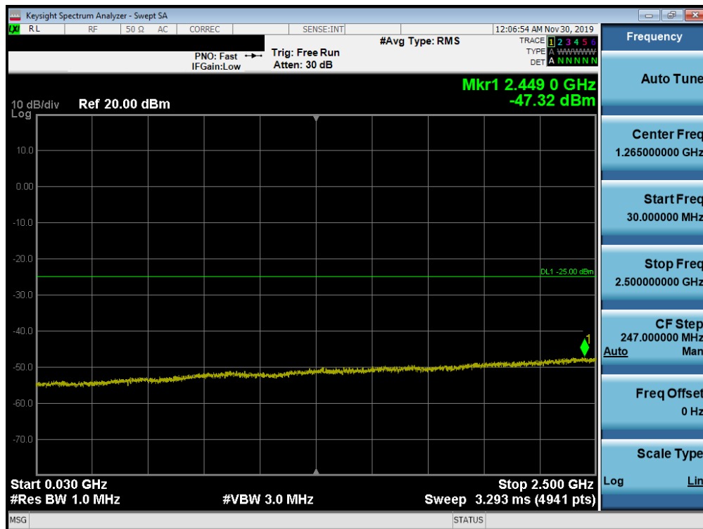
Plot 7-212. Conducted Spurious Plot (Band 7 - 20.0MHz QPSK - RB Size 1, RB Offset 0 - Mid Channel)
