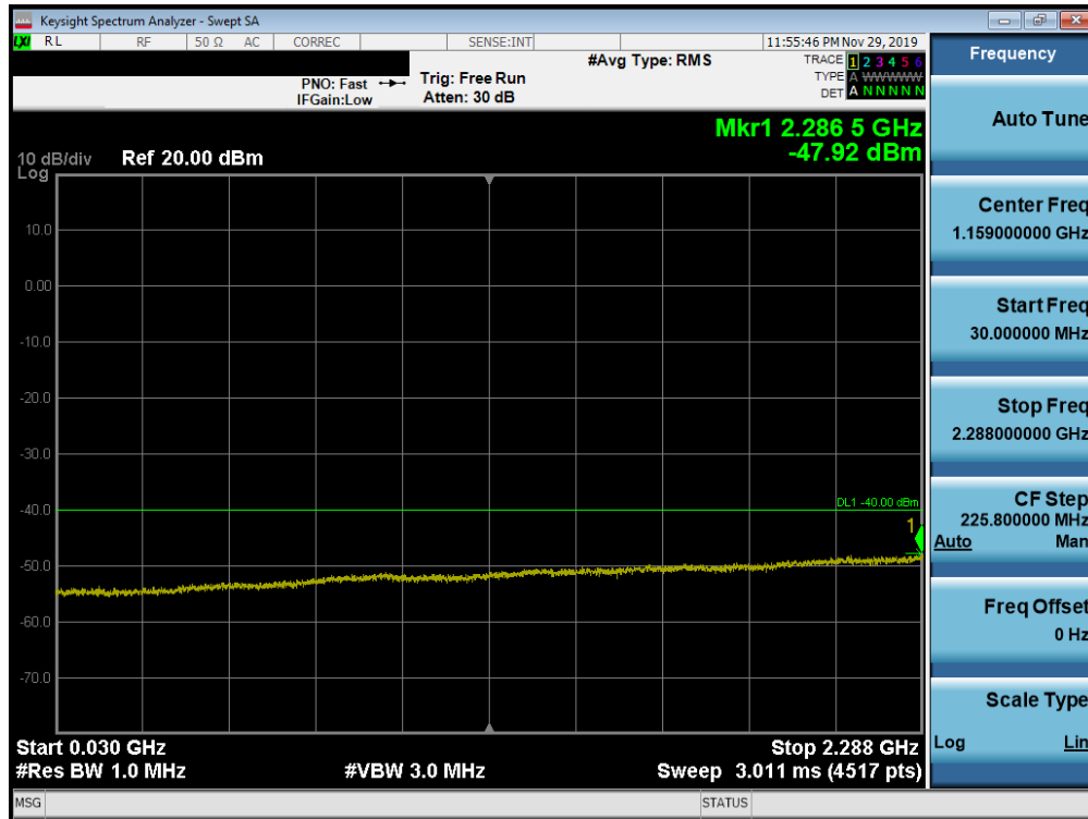
Plot 7-206. Conducted Spurious Plot (Band 30 - 10.0MHz QPSK - RB Size 1, RB Offset 0 – Mid Channel)
