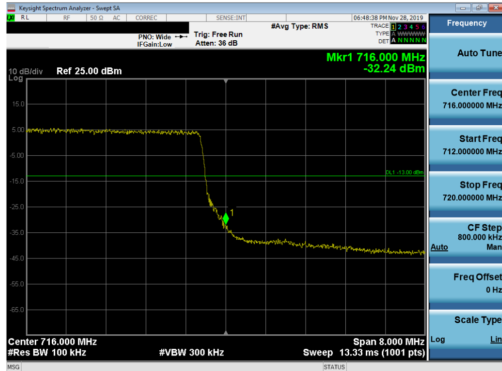
Plot 7-253. Upper Band Edge Plot (Band 12/17 - 10.0MHz QPSK - Full RB Configuration)
