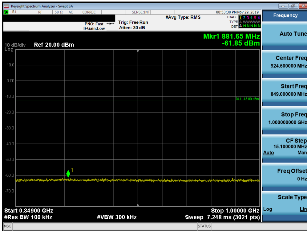
Plot 7-180. Conducted Spurious Plot (Band 26 - 15.0MHz QPSK - RB Size 1, RB Offset 0 - Low Channel)
