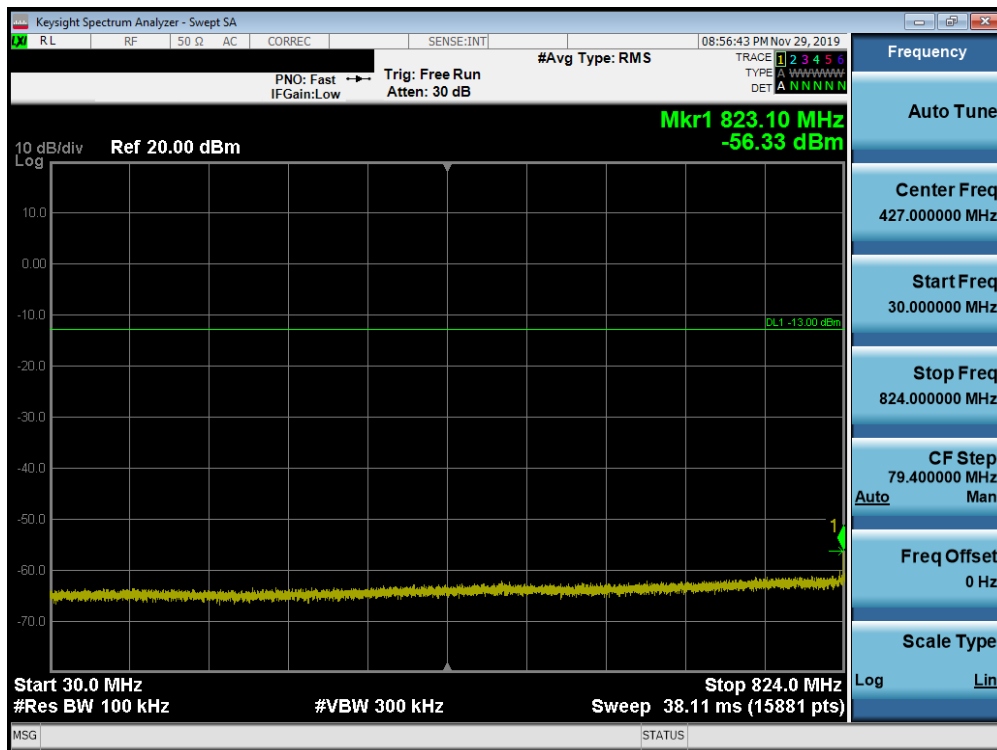
Plot 7-173. Conducted Spurious Plot (Band 26/5 - 10.0MHz QPSK - RB Size 1, RB Offset 0 - Mid Channel)
