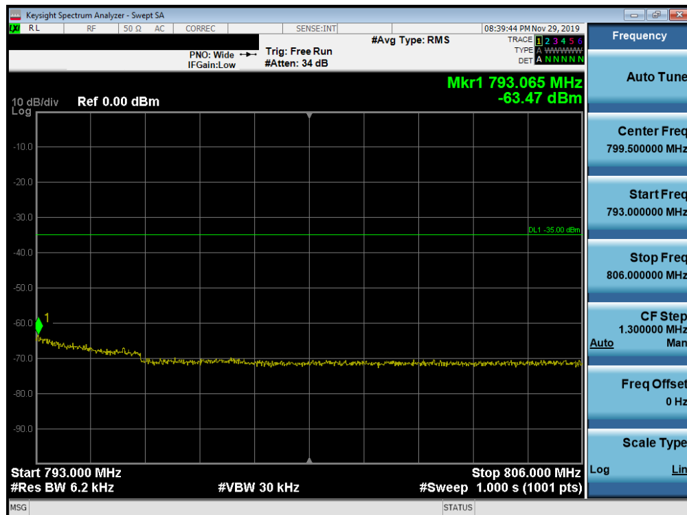
Plot 7-261. Upper Emission Mask Plot (Band 13 - 10.0MHz QPSK - Full RB Configuration)
