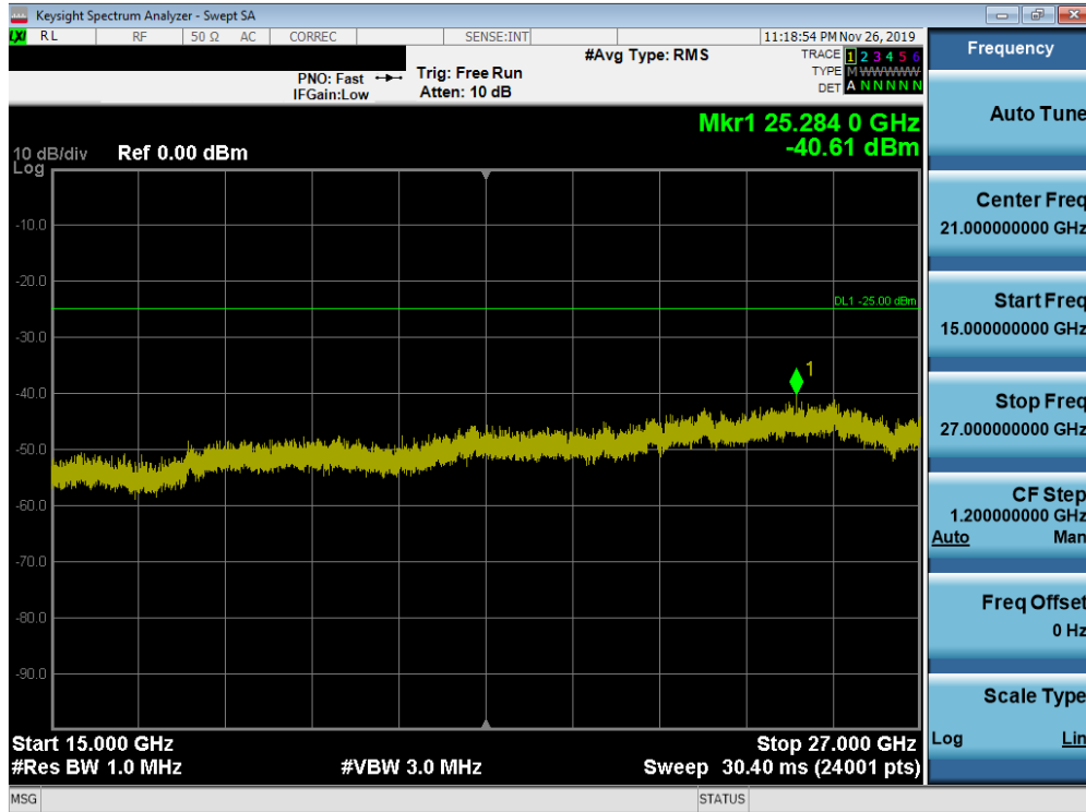
Plot 7-235. Conducted Spurious Plot (Band 41 (PC3) - 20.0MHz QPSK - RB Size 1, RB Offset 0 – High Channel)
