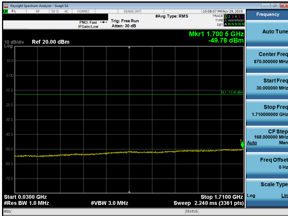
Plot 7-194. Conducted Spurious Plot (Band 66/4 - 20.0MHz QPSK - RB Size 1, RB Offset 0 - High Channel)
