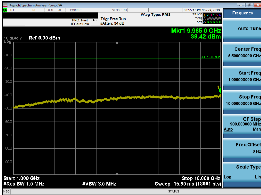
Plot 7-184. Conducted Spurious Plot (Band 26 - 15.0MHz QPSK - RB Size 1, RB Offset 0 - Mid Channel)
