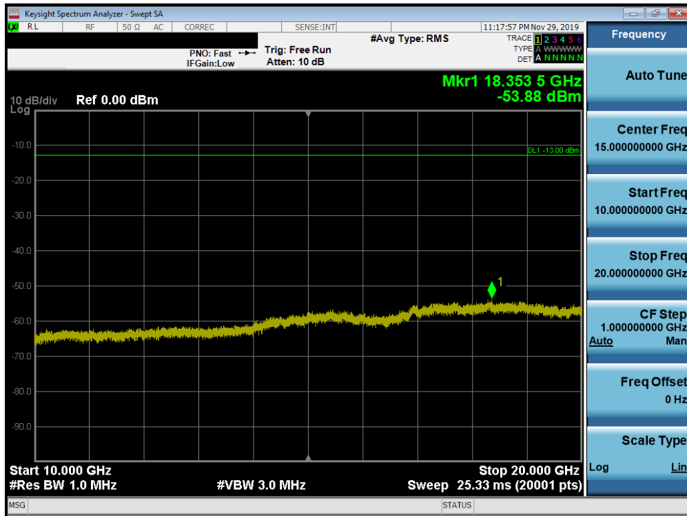
Plot 7-199. Conducted Spurious Plot (Band 25/2 - 20.0MHz QPSK - RB Size 1, RB Offset 0 - Low Channel)
