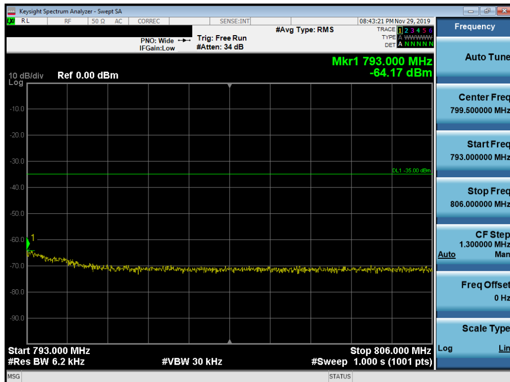
Plot 7-257. Upper Emission Mask Plot (Band 13 - 5.0MHz QPSK - Full RB Configuration)
