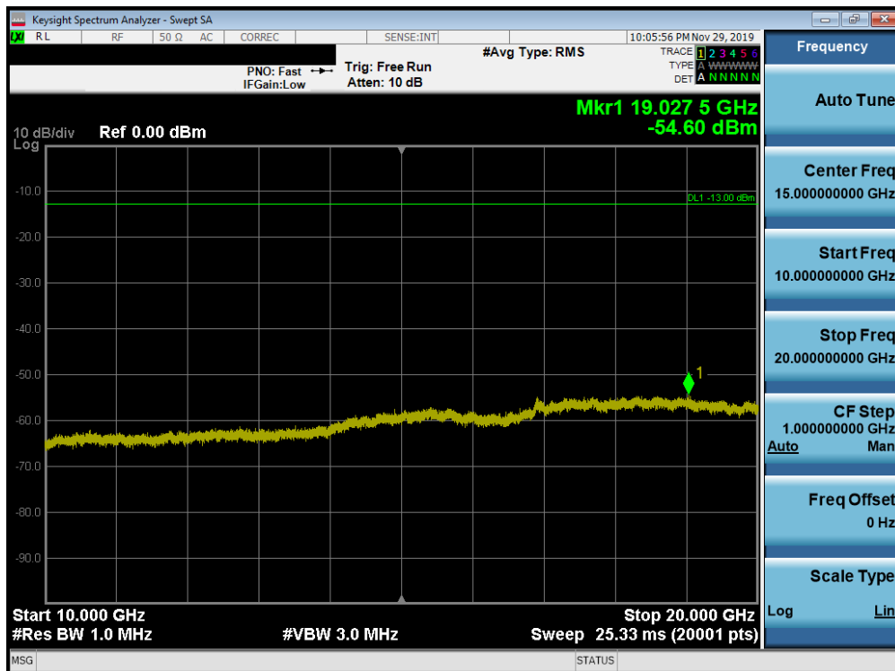
Plot 7-193. Conducted Spurious Plot (Band 66/4 - 20.0MHz QPSK - RB Size 1, RB Offset 0 - Mid Channel)
