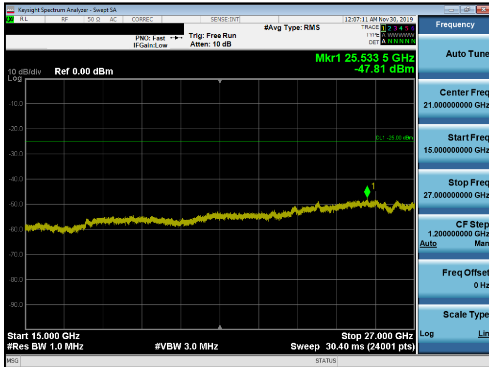
Plot 7-214. Conducted Spurious Plot (Band 7 - 20.0MHz QPSK - RB Size 1, RB Offset 0 – Mid Channel)
