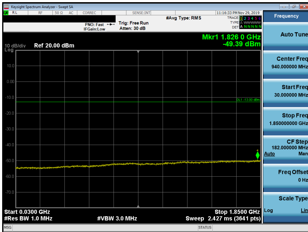
Plot 7-200. Conducted Spurious Plot (Band 25/2 - 20.0MHz QPSK - RB Size 1, RB Offset 0 - Mid Channel)
