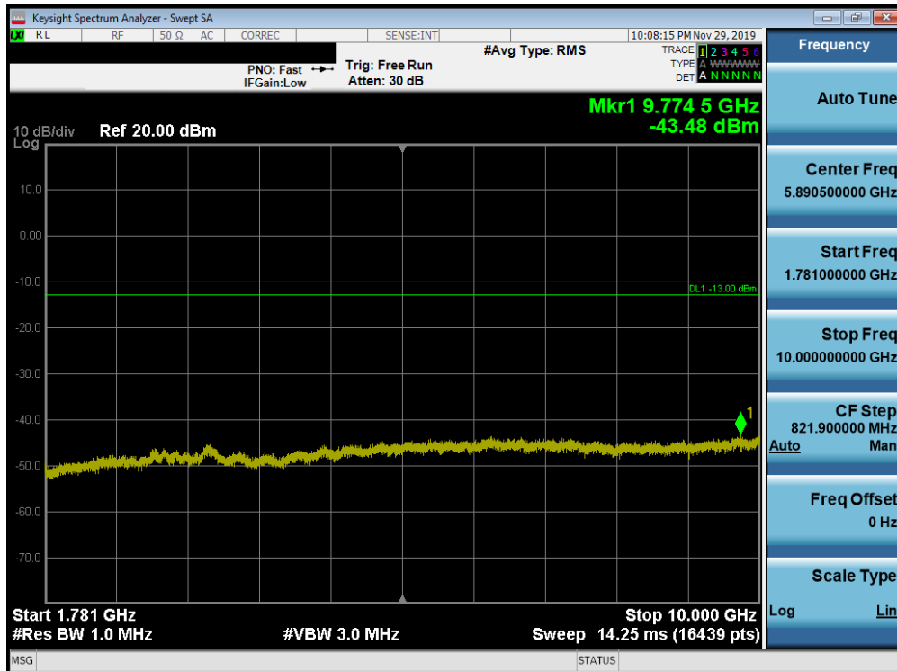
Plot 7-195. Conducted Spurious Plot (Band 66/4 - 20.0MHz QPSK - RB Size 1, RB Offset 0 - High Channel)
