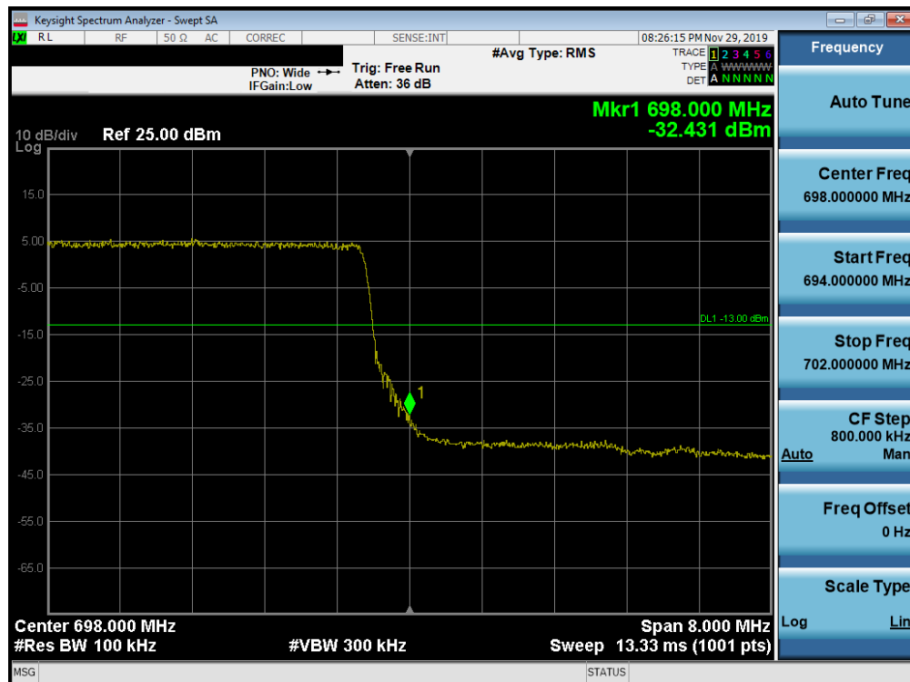
Plot 7-239. Upper Band Edge Plot (Band 71 - 10.0MHz QPSK - Full RB Configuration)
