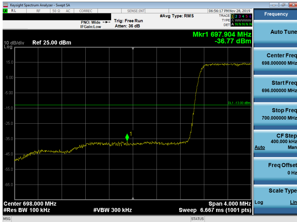
Plot 7-244. Lower Band Edge Plot (Band 12 - 1.4MHz QPSK - Full RB Configuration)
