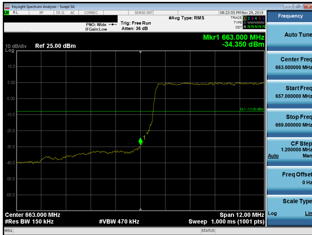
Plot 7-240. Lower Band Edge Plot (Band 71 - 15.0MHz QPSK - Full RB Configuration)
