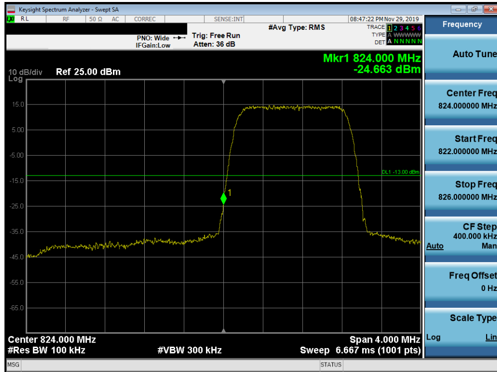
Plot 7-262. Lower Band Edge Plot (Band 26/5 - 1.4MHz QPSK - Full RB Configuration)
