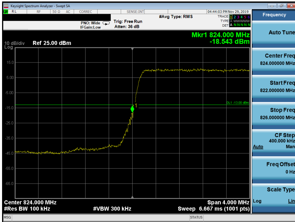
Plot 7-264. Lower Band Edge Plot (Band 26/5 - 3.0MHz QPSK - Full RB Configuration)
