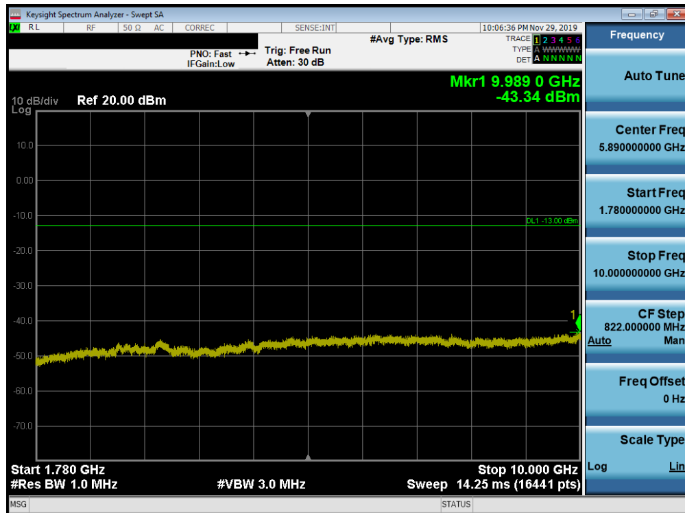
Plot 7-189. Conducted Spurious Plot (Band 66/4 - 20.0MHz QPSK - RB Size 1, RB Offset 0 - Low Channel)
