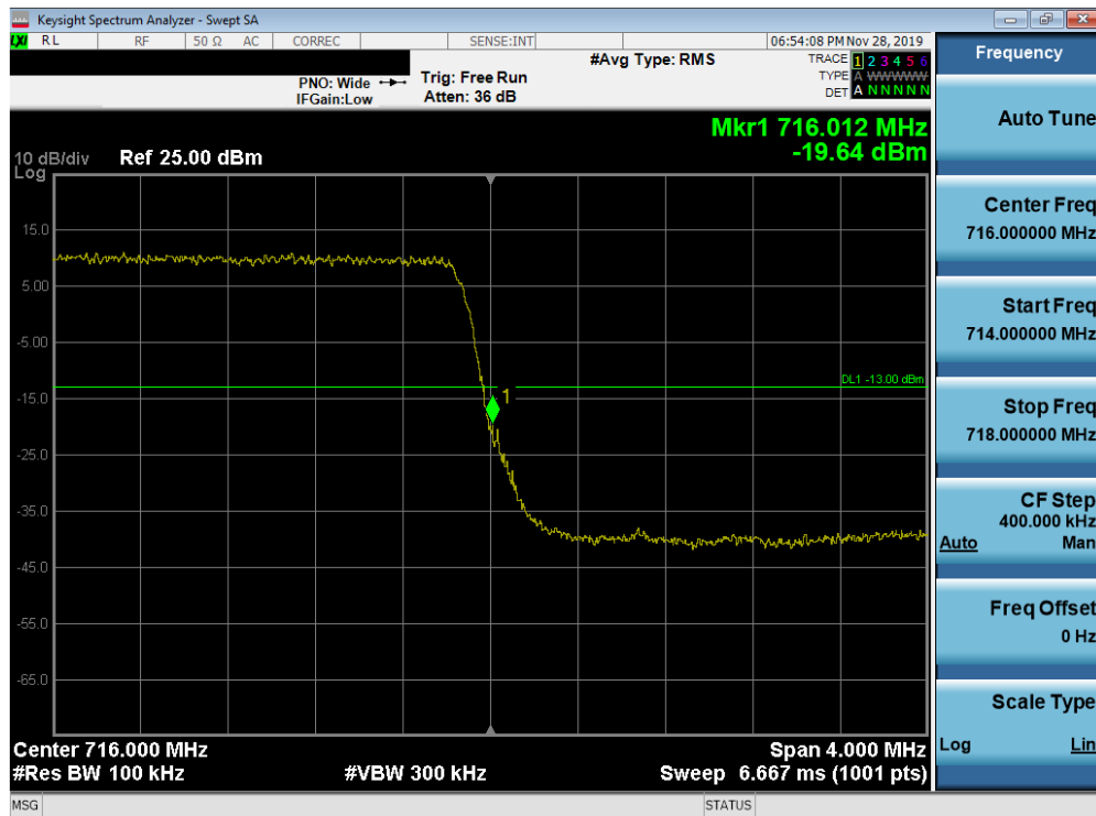
Plot 7-247. Upper Band Edge Plot (Band 12 - 3.0MHz QPSK - Full RB Configuration)
