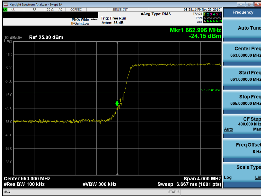
Plot 7-236. Lower Band Edge Plot (Band 71 - 5.0MHz QPSK - Full RB Configuration)
