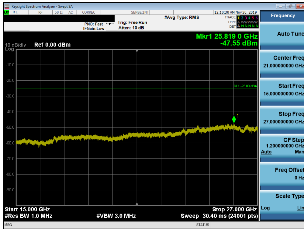
Plot 7-217. Conducted Spurious Plot (Band 7 - 20.0MHz QPSK - RB Size 1, RB Offset 0 – High Channel)
