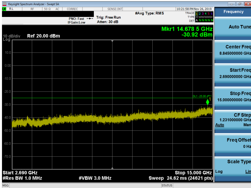
Plot 7-219. Conducted Spurious Plot (Band 41 (PC2) - 20.0MHz QPSK - RB Size 1, RB Offset 0 - Low Channel)
