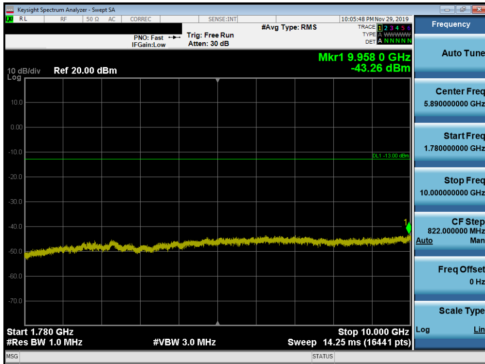
Plot 7-192. Conducted Spurious Plot (Band 66/4 - 20.0MHz QPSK - RB Size 1, RB Offset 0 - Mid Channel)
