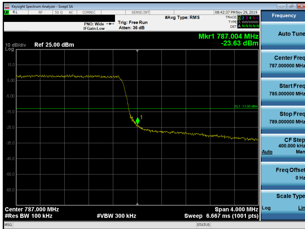
Plot 7-256. Upper Band Edge Plot (Band 13 - 5.0MHz QPSK - Full RB Configuration)
