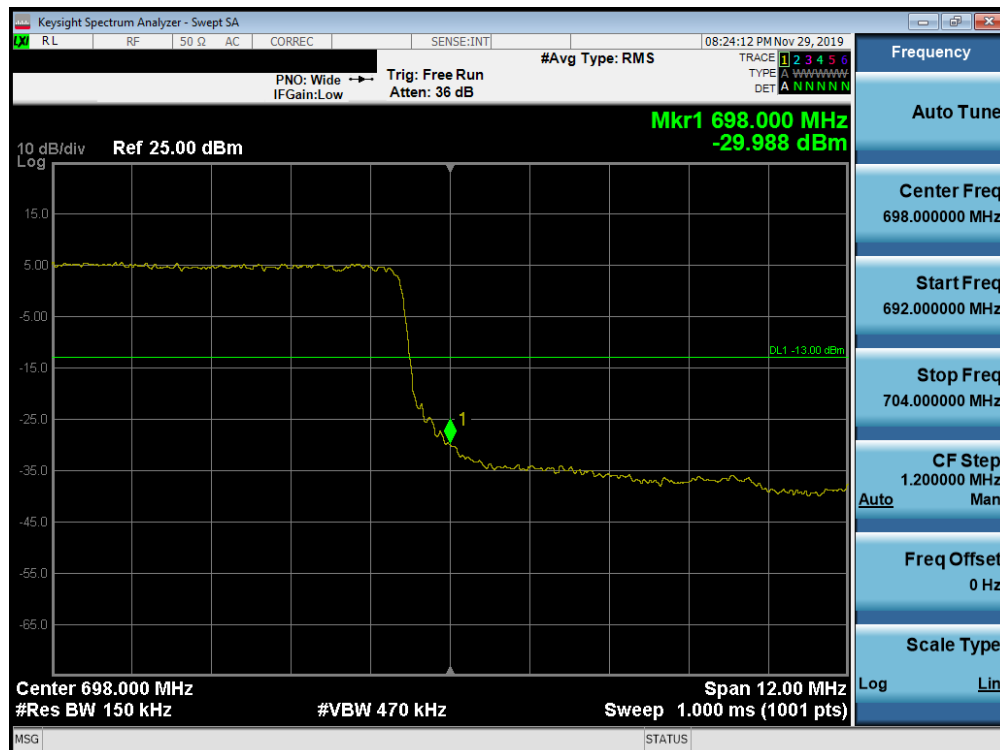
Plot 7-241. Upper Band Edge Plot (Band 71 - 15.0MHz QPSK - Full RB Configuration)
