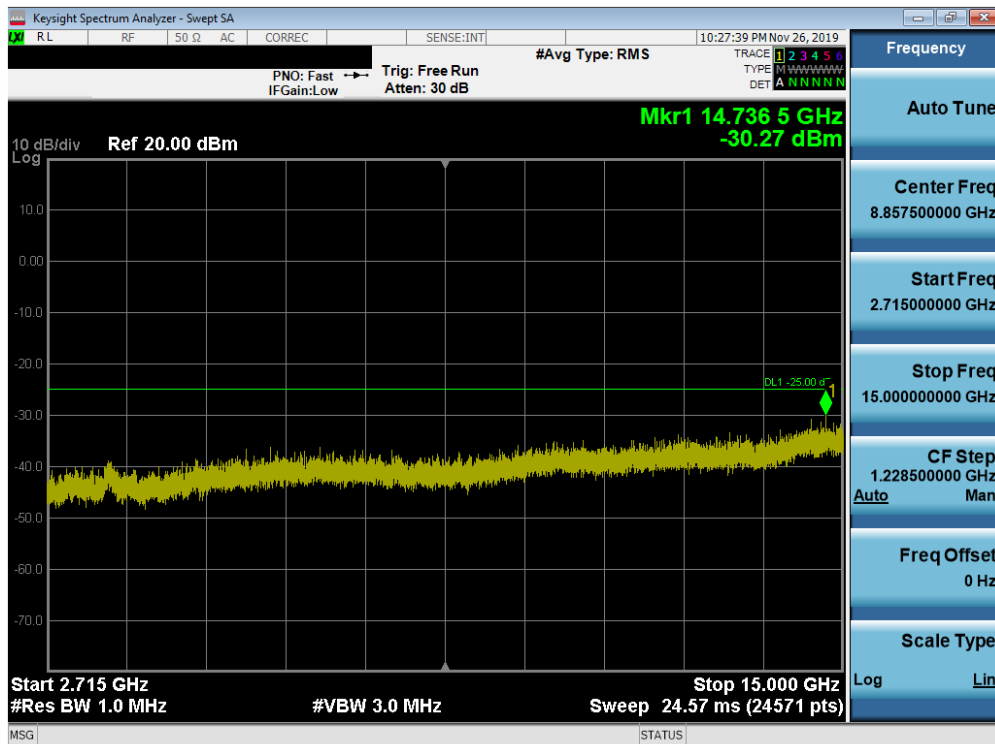
Plot 7-225. Conducted Spurious Plot (Band 41 (PC2) - 20.0MHz QPSK - RB Size 1, RB Offset 0 – High Channel)
