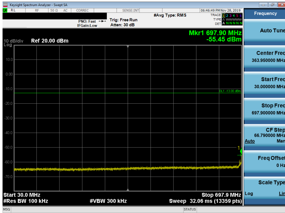
Plot 7-158. Conducted Spurious Plot (Band 12/17 - 10.0MHz QPSK - RB Size 1, RB Offset 0 - Low Channel)
