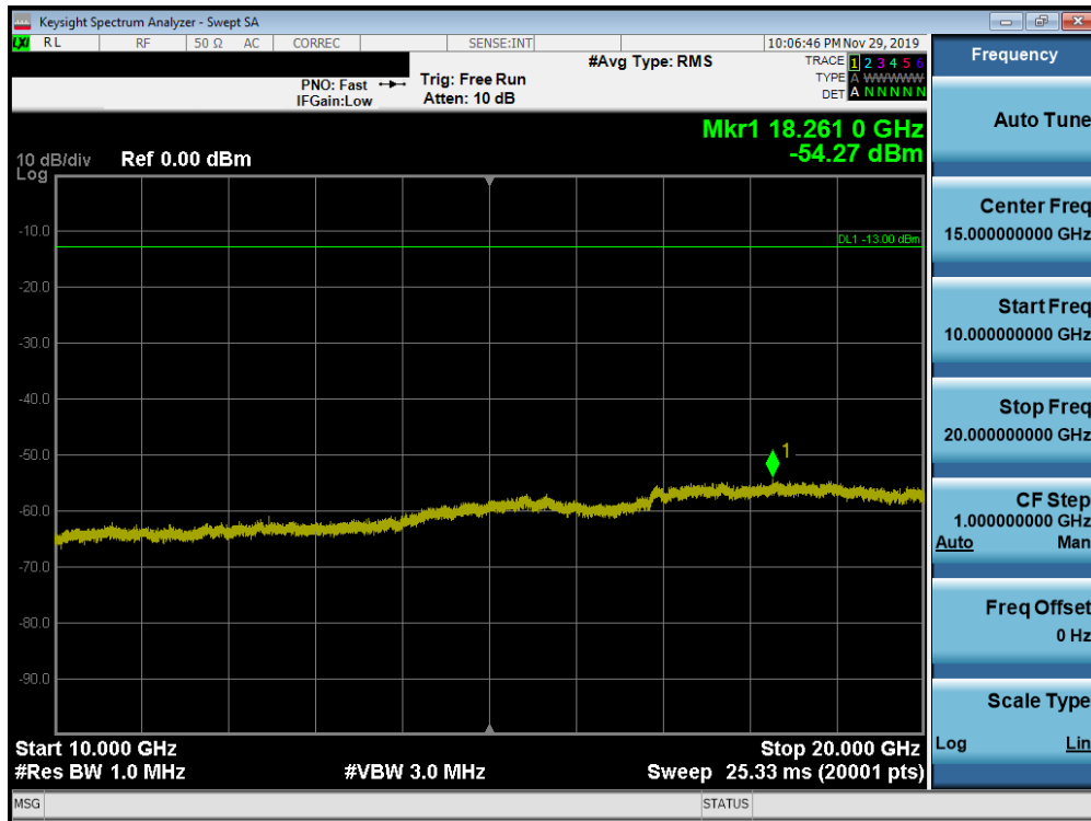
Plot 7-190. Conducted Spurious Plot (Band 66/4 - 20.0MHz QPSK - RB Size 1, RB Offset 0 - Low Channel)
