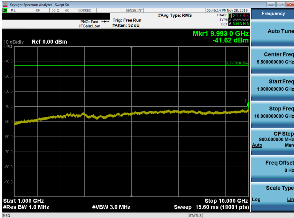
Plot 7-163. Conducted Spurious Plot (Band 12/17 - 10.0MHz QPSK - RB Size 1, RB Offset 0 - Mid Channel)
