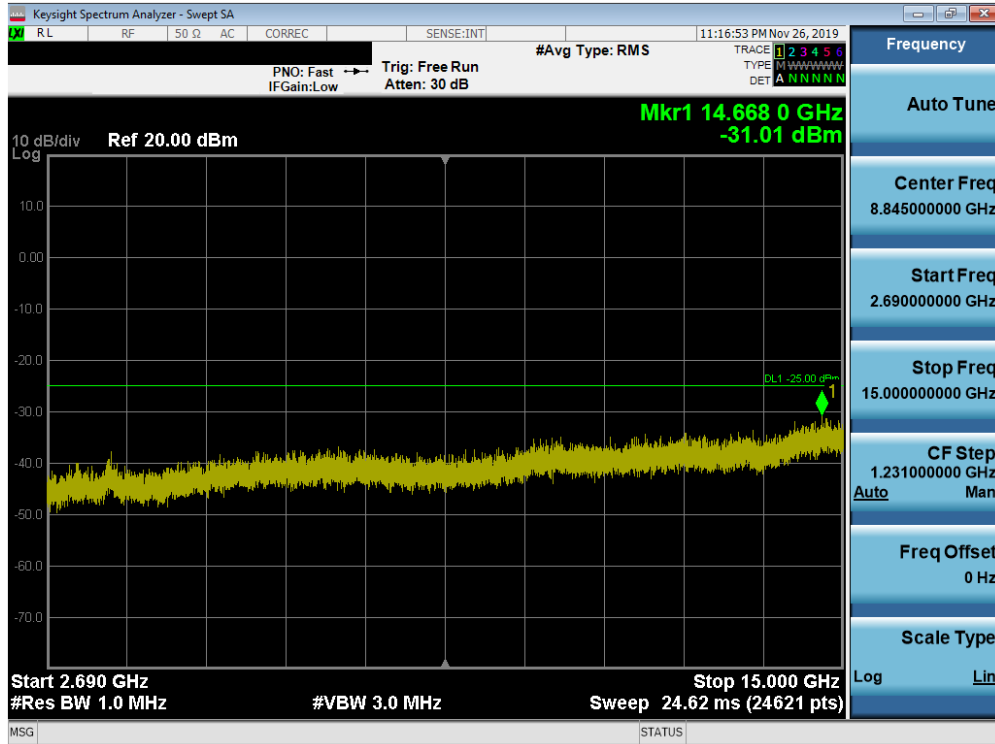
Plot 7-231. Conducted Spurious Plot (Band 41 (PC3) - 20.0MHz QPSK - RB Size 1, RB Offset 0 – Mid Channel)
