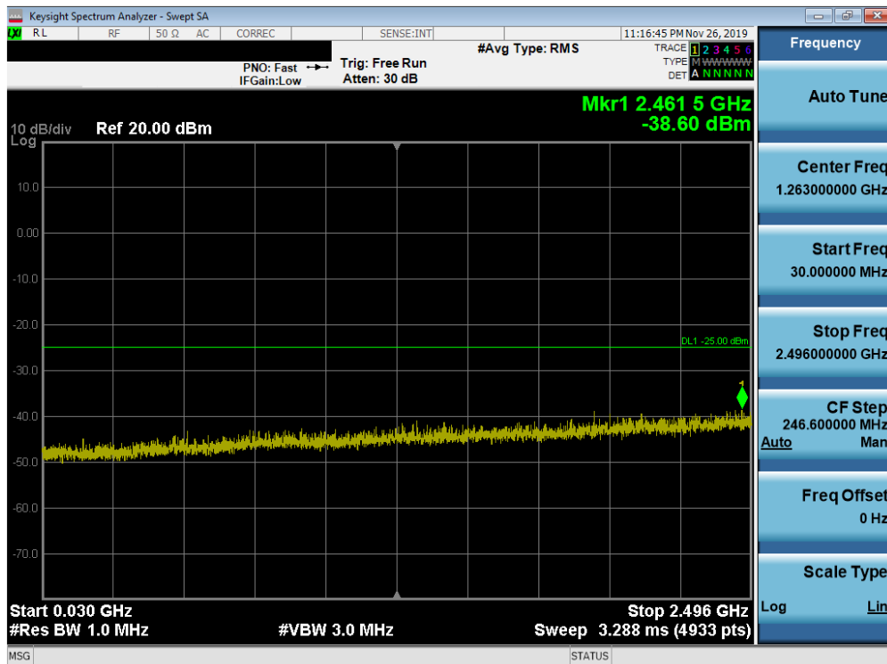
Plot 7-230. Conducted Spurious Plot (Band 41 (PC3) - 20.0MHz QPSK - RB Size 1, RB Offset 0 - Mid Channel)
