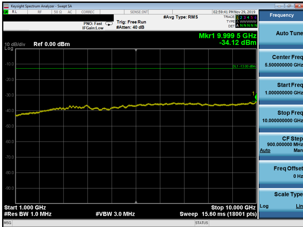
Plot 7-178. Conducted Spurious Plot (Band 26/5 - 10.0MHz QPSK - RB Size 1, RB Offset 0 - High Channel)
