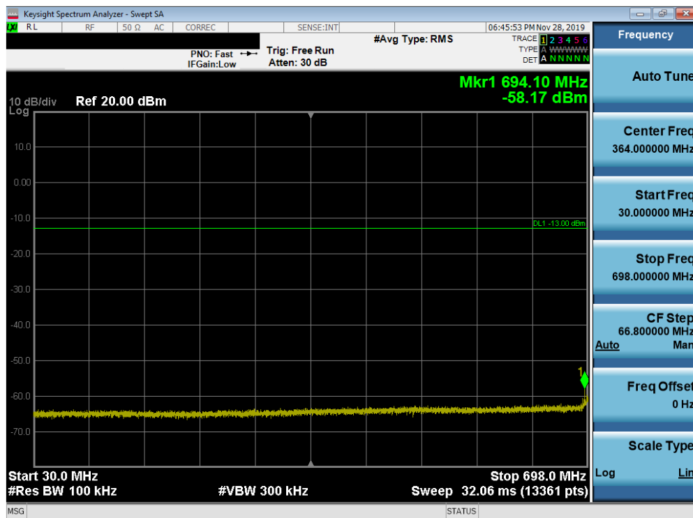
Plot 7-161. Conducted Spurious Plot (Band 12/17 - 10.0MHz QPSK - RB Size 1, RB Offset 0 - Mid Channel)
