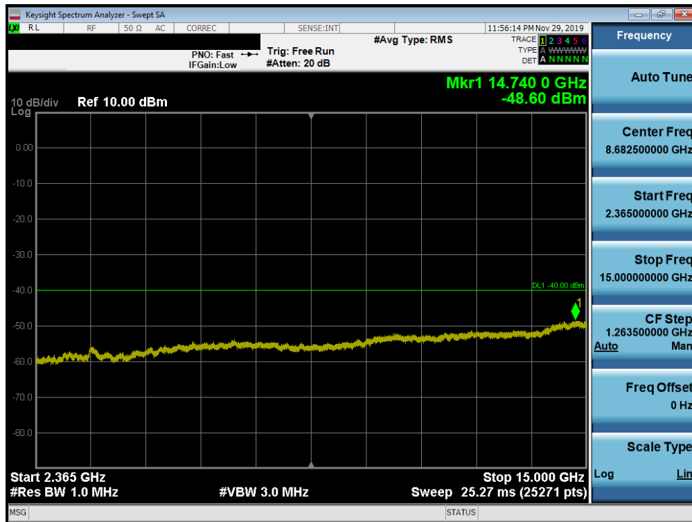
Plot 7-207. Conducted Spurious Plot (Band 30 - 10.0MHz QPSK - RB Size 1, RB Offset 0 – Mid Channel)
