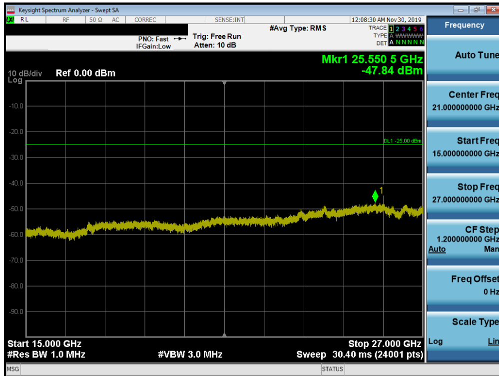
Plot 7-211. Conducted Spurious Plot (Band 7 - 20.0MHz QPSK - RB Size 1, RB Offset 0 - Low Channel)
