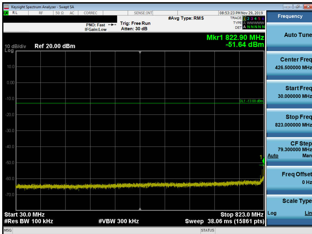
Plot 7-179. Conducted Spurious Plot (Band 26 - 15.0MHz QPSK - RB Size 1, RB Offset 0 - Low Channel)
