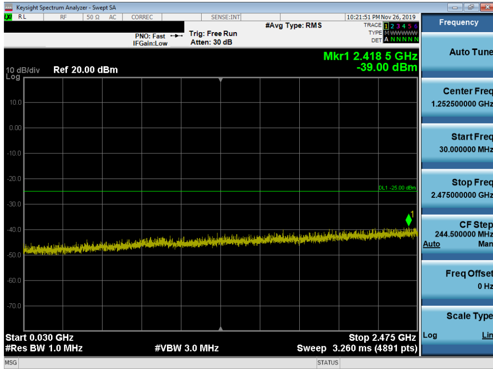
Plot 7-218. Conducted Spurious Plot (Band 41 (PC2) - 20.0MHz QPSK - RB Size 1, RB Offset 0 - Low Channel)
