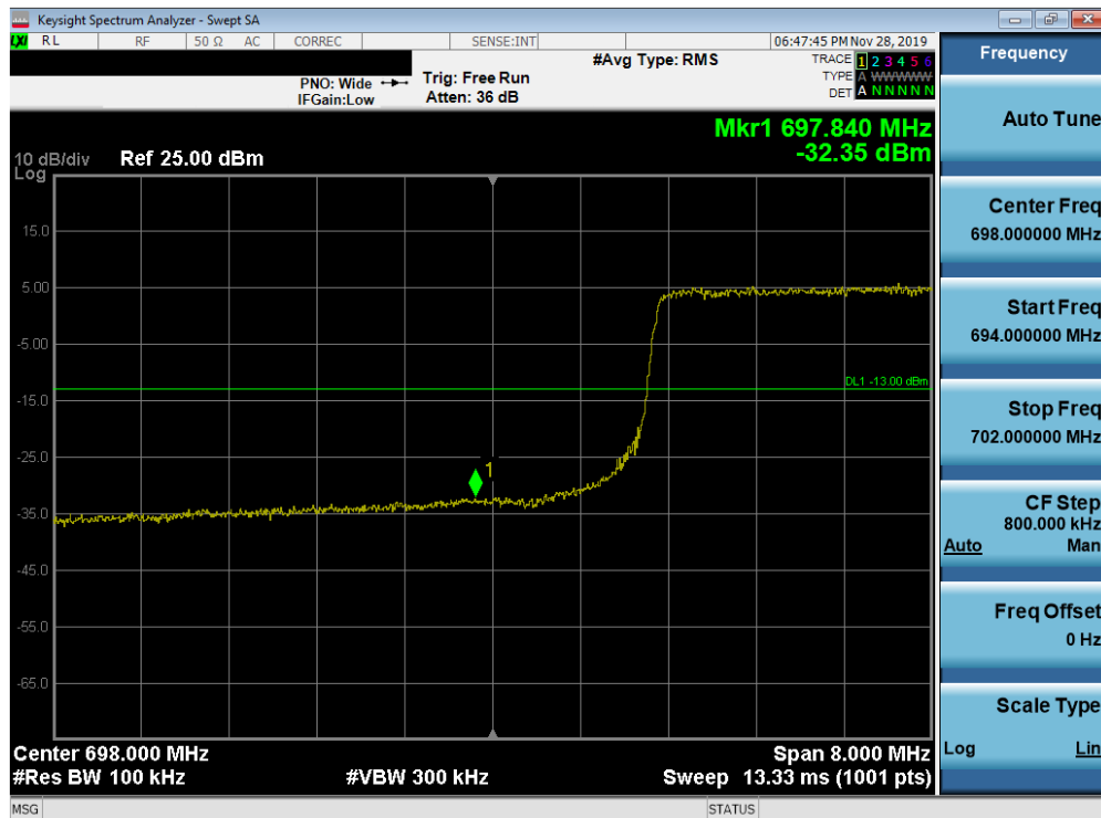
Plot 7-251. Lower Band Edge Plot (Band 12 - 10.0MHz QPSK - Full RB Configuration)
