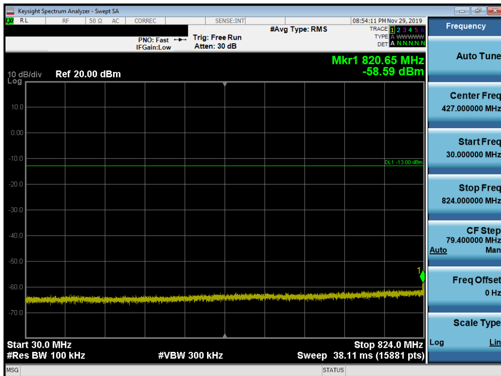
Plot 7-185. Conducted Spurious Plot (Band 26 - 15.0MHz QPSK - RB Size 1, RB Offset 0 - High Channel)
