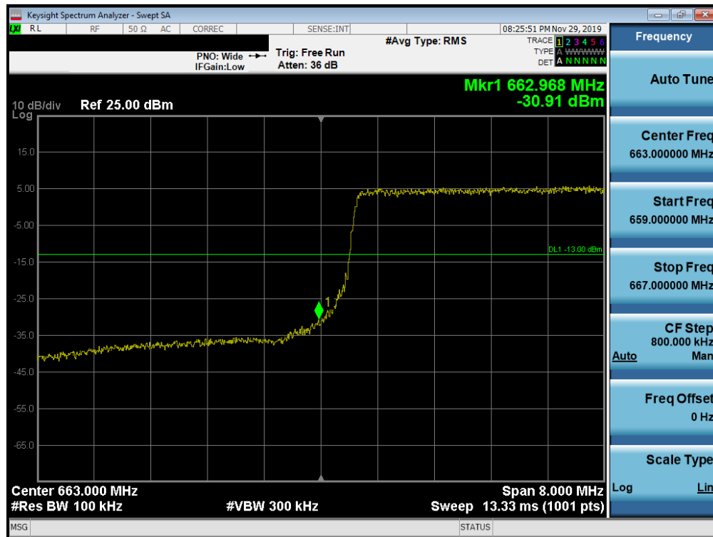
Plot 7-238. Lower Band Edge Plot (Band 71 - 10.0MHz QPSK - Full RB Configuration)
