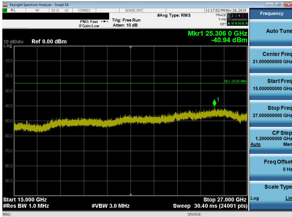
Plot 7-232. Conducted Spurious Plot (Band 41 (PC3) - 20.0MHz QPSK - RB Size 1, RB Offset 0 – Mid Channel)
