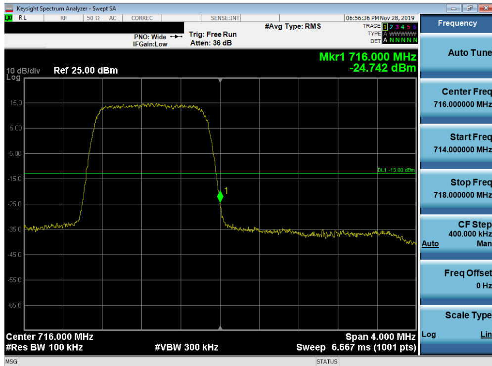
Plot 7-245. Upper Band Edge Plot (Band 12 - 1.4MHz QPSK - Full RB Configuration)
