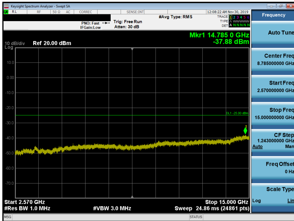
Plot 7-210. Conducted Spurious Plot (Band 7 - 20.0MHz QPSK - RB Size 1, RB Offset 0 - Low Channel)
