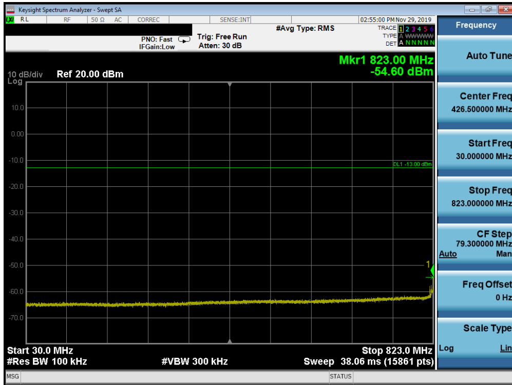
Plot 7-170. Conducted Spurious Plot (Band 26/5 - 10.0MHz QPSK - RB Size 1, RB Offset 0 - Low Channel)
