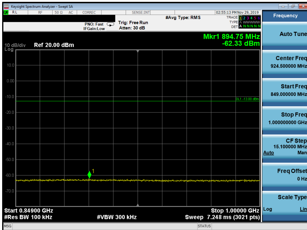
Plot 7-171. Conducted Spurious Plot (Band 26/5 - 10.0MHz QPSK - RB Size 1, RB Offset 0 - Low Channel)
