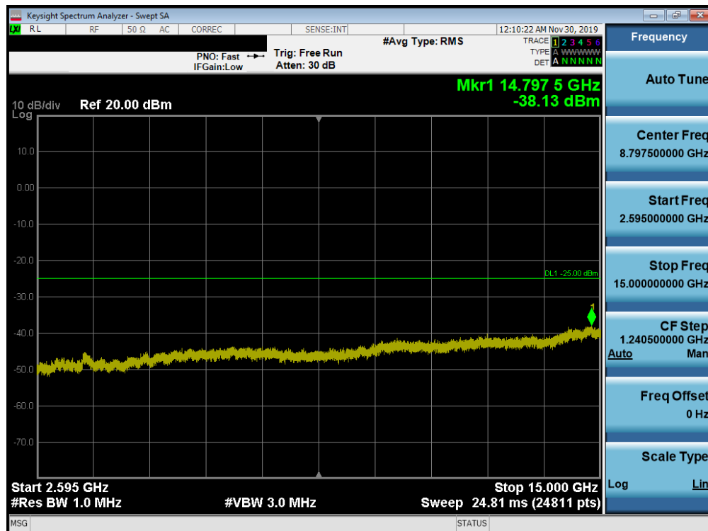
Plot 7-216. Conducted Spurious Plot (Band 7 - 20.0MHz QPSK - RB Size 1, RB Offset 0 – High Channel)
