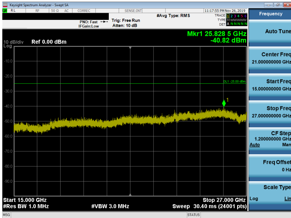
Plot 7-229. Conducted Spurious Plot (Band 41 (PC3) - 20.0MHz QPSK - RB Size 1, RB Offset 0 - Low Channel)
