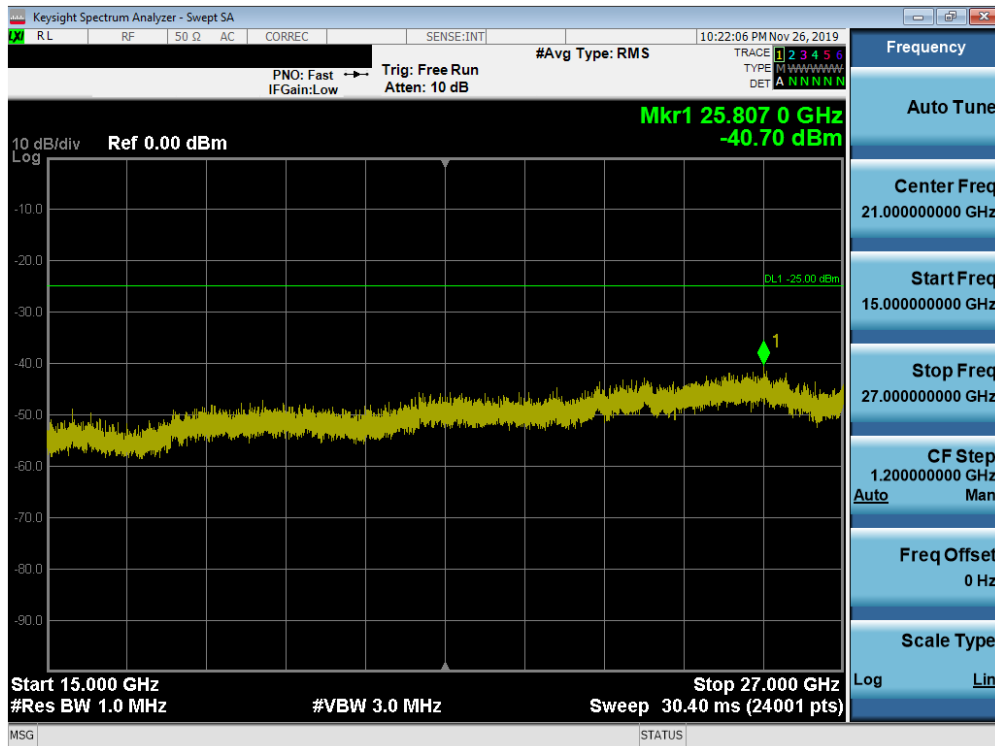
Plot 7-220. Conducted Spurious Plot (Band 41 (PC2) - 20.0MHz QPSK - RB Size 1, RB Offset 0 - Low Channel)
