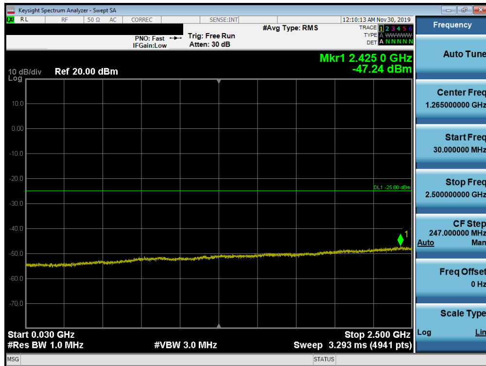
Plot 7-215. Conducted Spurious Plot (Band 7 - 20.0MHz QPSK - RB Size 1, RB Offset 0 – High Channel)
