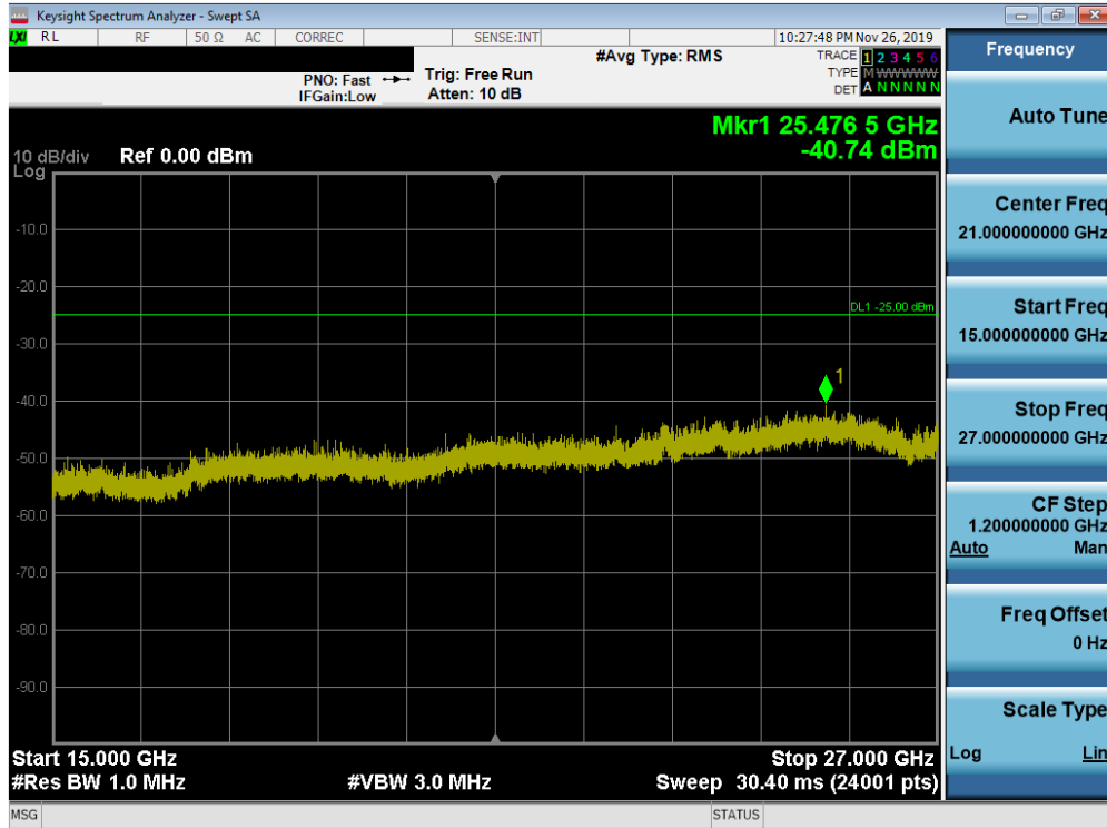
Plot 7-226. Conducted Spurious Plot (Band 41 (PC2) - 20.0MHz QPSK - RB Size 1, RB Offset 0 – High Channel)
