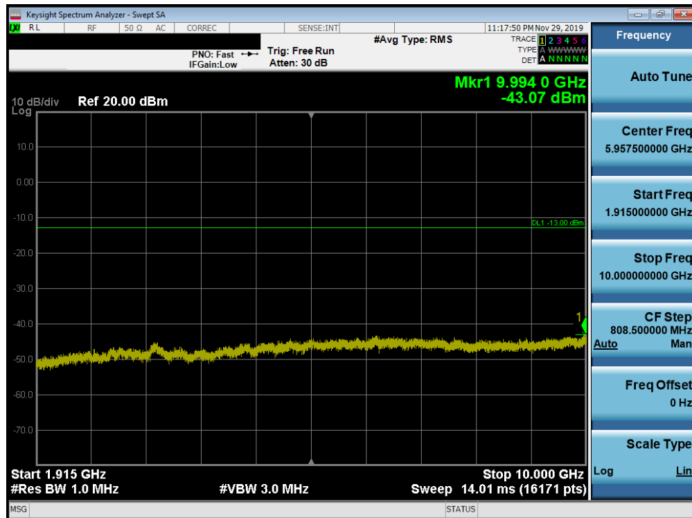
Plot 7-198. Conducted Spurious Plot (Band 25/2 - 20.0MHz QPSK - RB Size 1, RB Offset 0 - Low Channel)
