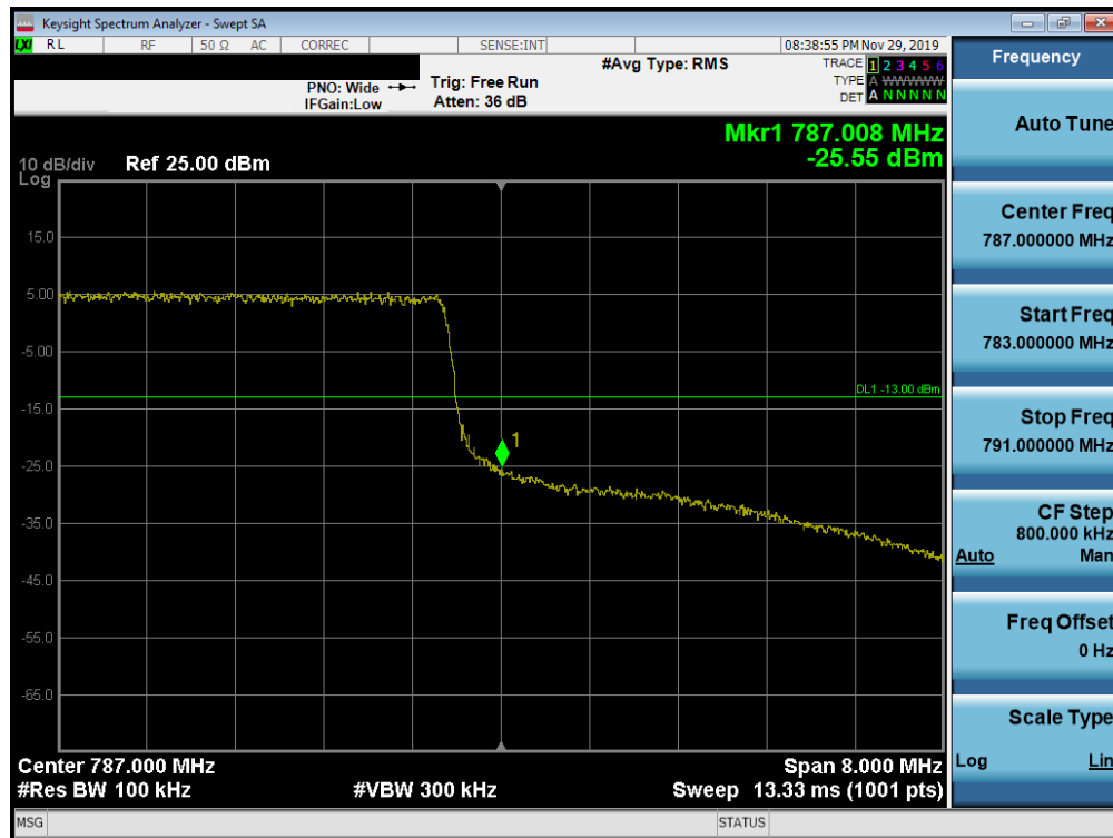
Plot 7-260. Upper Band Edge Plot (Band 13 - 10.0MHz QPSK - Full RB Configuration)
