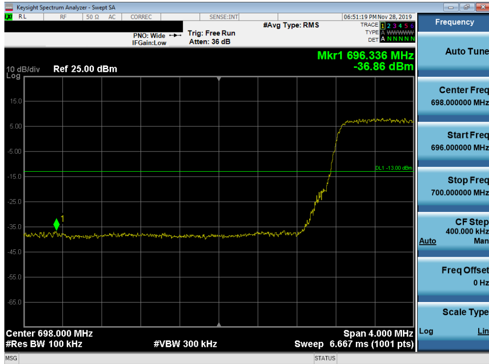
Plot 7-248. Lower Band Edge Plot (Band 12 - 5.0MHz QPSK - Full RB Configuration)
