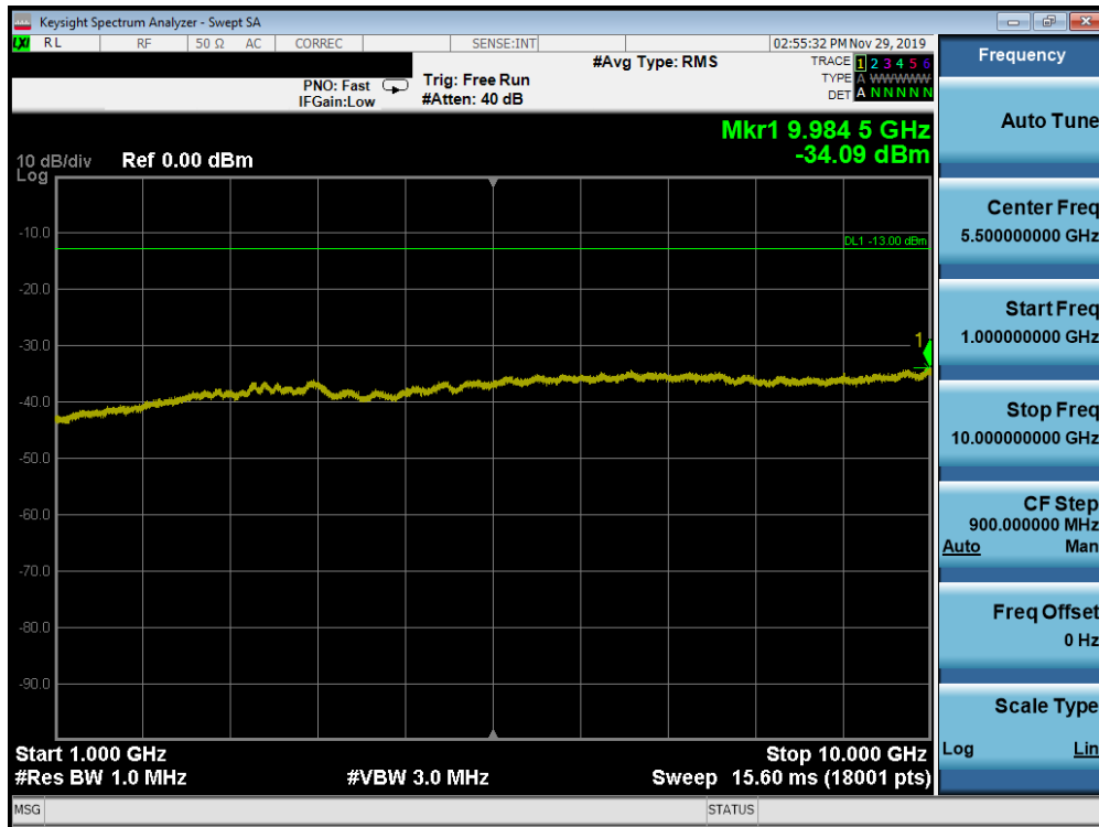
Plot 7-172. Conducted Spurious Plot (Band 26/5 - 10.0MHz QPSK - RB Size 1, RB Offset 0 - Low Channel)
