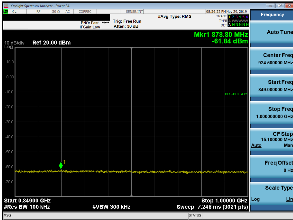
Plot 7-174. Conducted Spurious Plot (Band 26/5 - 10.0MHz QPSK - RB Size 1, RB Offset 0 - Mid Channel)
