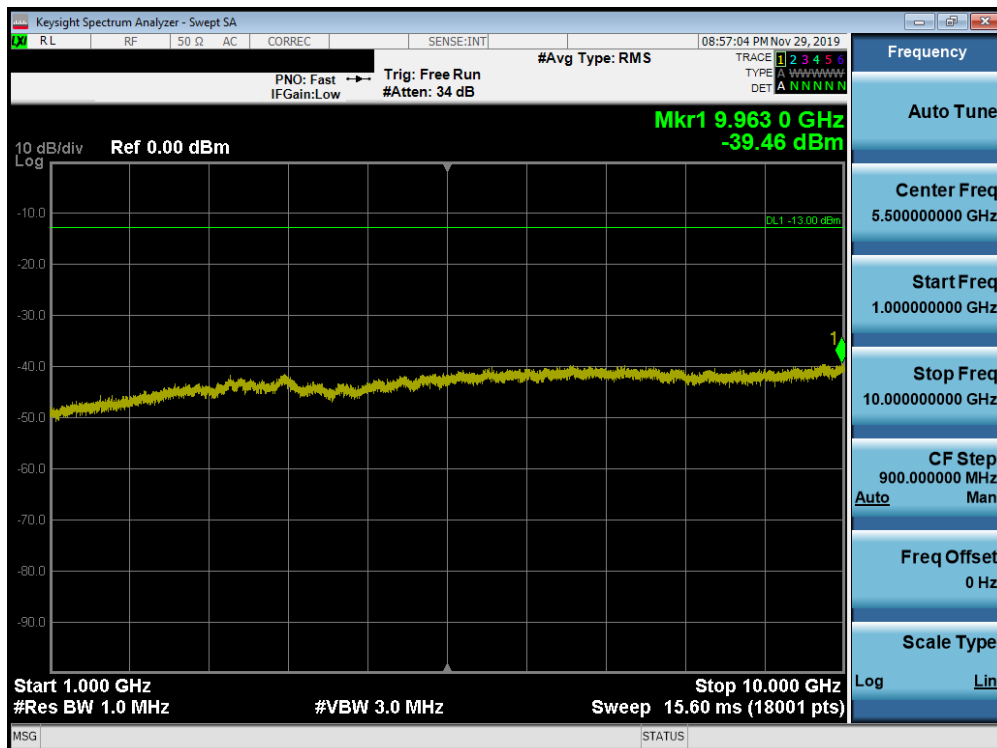
Plot 7-175. Conducted Spurious Plot (Band 26/5 - 10.0MHz QPSK - RB Size 1, RB Offset 0 - Mid Channel)
