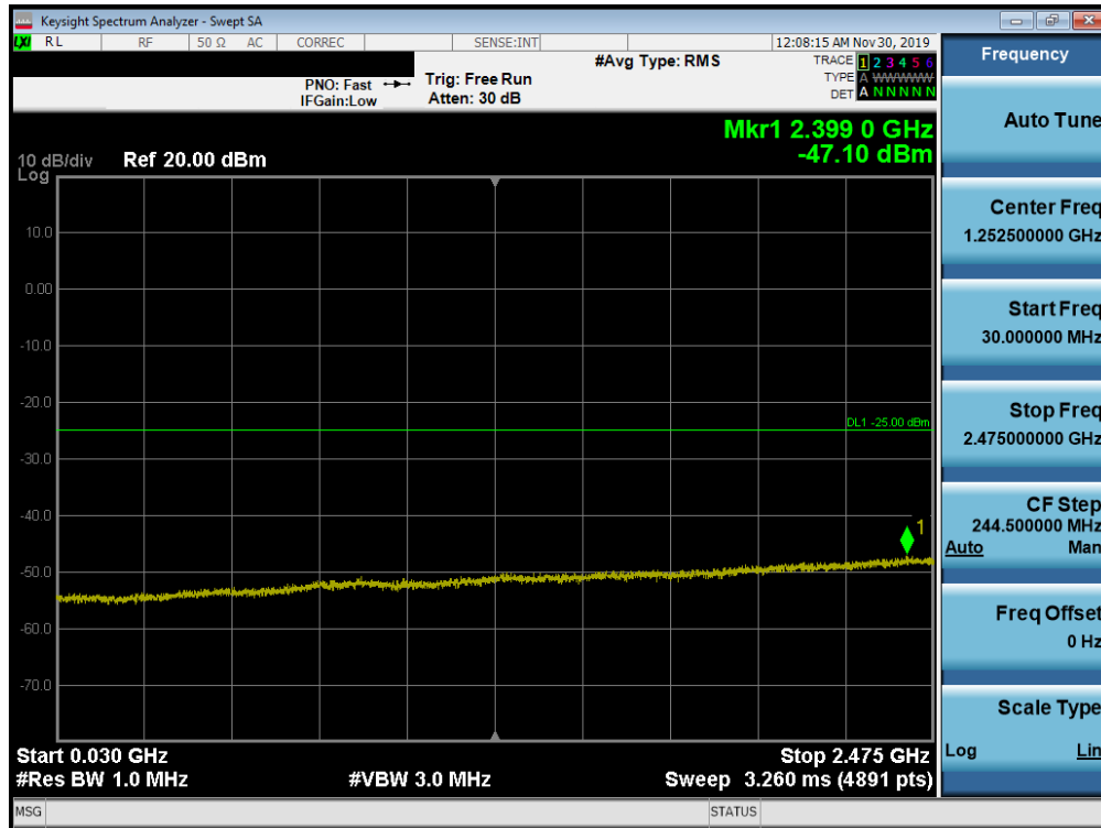
Plot 7-209. Conducted Spurious Plot (Band 7 - 20.0MHz QPSK - RB Size 1, RB Offset 0 - Low Channel)
