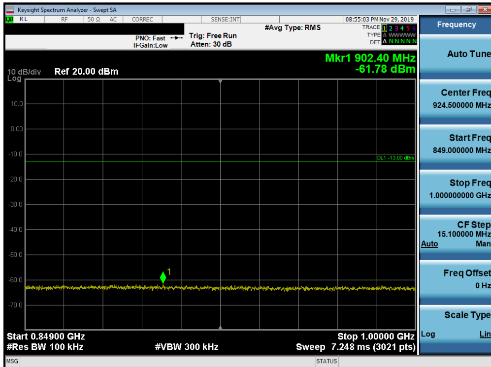
Plot 7-183. Conducted Spurious Plot (Band 26 - 15.0MHz QPSK - RB Size 1, RB Offset 0 - Mid Channel)
