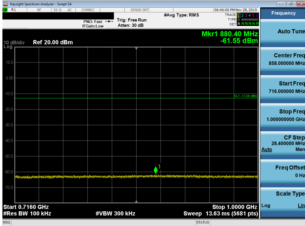
Plot 7-162. Conducted Spurious Plot (Band 12/17 - 10.0MHz QPSK - RB Size 1, RB Offset 0 - Mid Channel)
