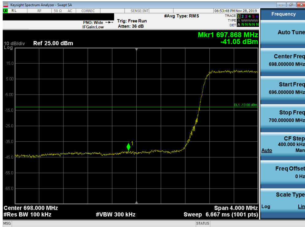
Plot 7-246. Lower Band Edge Plot (Band 12 - 3.0MHz QPSK - Full RB Configuration)
