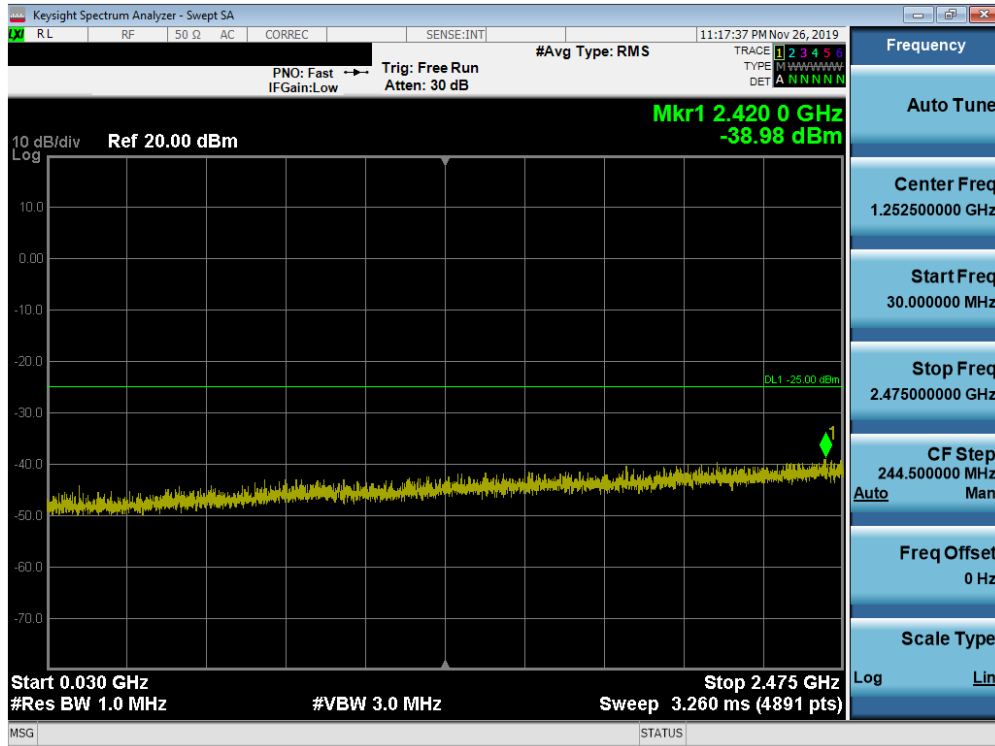
Plot 7-227. Conducted Spurious Plot (Band 41 (PC3) - 20.0MHz QPSK - RB Size 1, RB Offset 0 - Low Channel)
