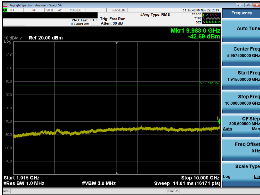
Plot 7-201. Conducted Spurious Plot (Band 25/2 - 20.0MHz QPSK - RB Size 1, RB Offset 0 - Mid Channel)
