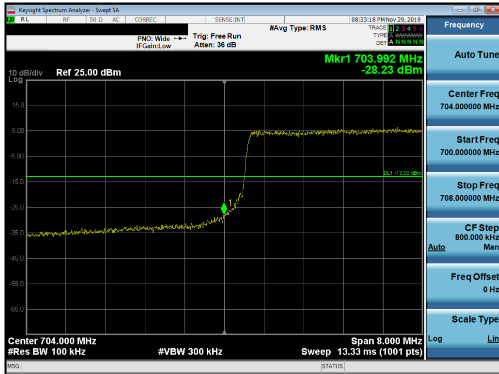
Plot 7-252. Lower Band Edge Plot (Band 17 - 10.0MHz QPSK - Full RB Configuration)
