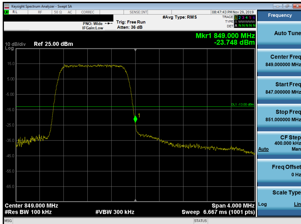
Plot 7-263. Upper Band Edge Plot (Band 26/5 - 1.4MHz QPSK - Full RB Configuration)
