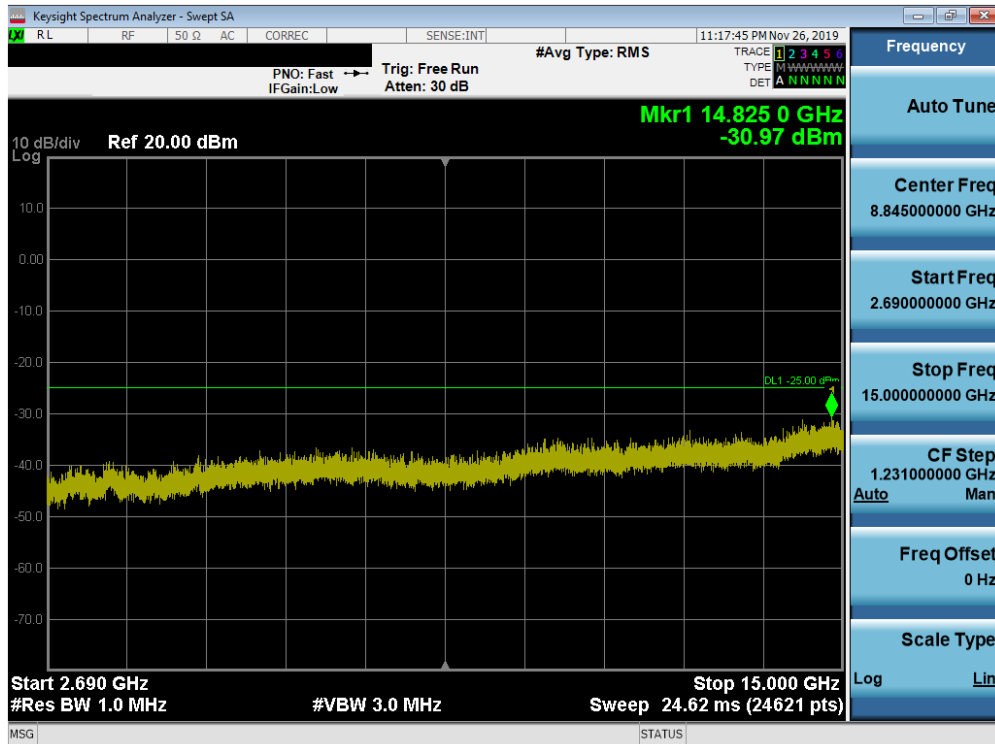
Plot 7-228. Conducted Spurious Plot (Band 41 (PC3) - 20.0MHz QPSK - RB Size 1, RB Offset 0 - Low Channel)
