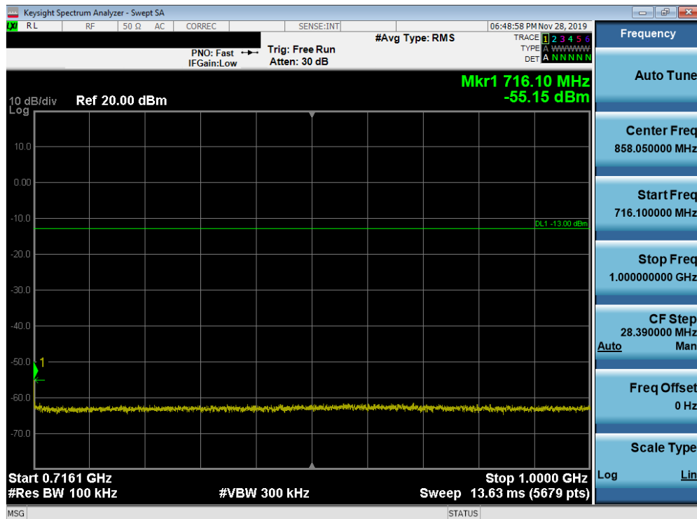
Plot 7-165. Conducted Spurious Plot (Band 12/17 - 10.0MHz QPSK - RB Size 1, RB Offset 0 - High Channel)
