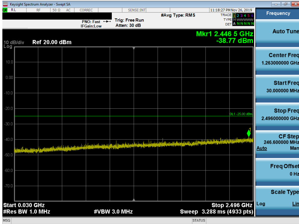
Plot 7-233. Conducted Spurious Plot (Band 41 (PC3) - 20.0MHz QPSK - RB Size 1, RB Offset 0 – High Channel)
