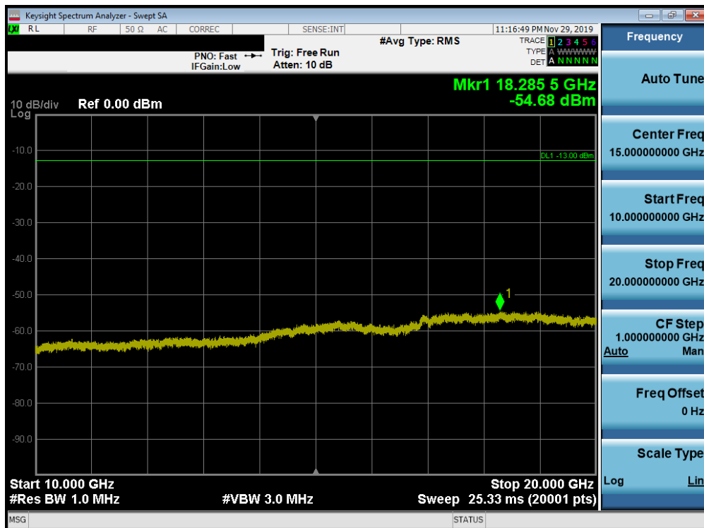
Plot 7-202. Conducted Spurious Plot (Band 25/2 - 20.0MHz QPSK - RB Size 1, RB Offset 0 - Mid Channel)
