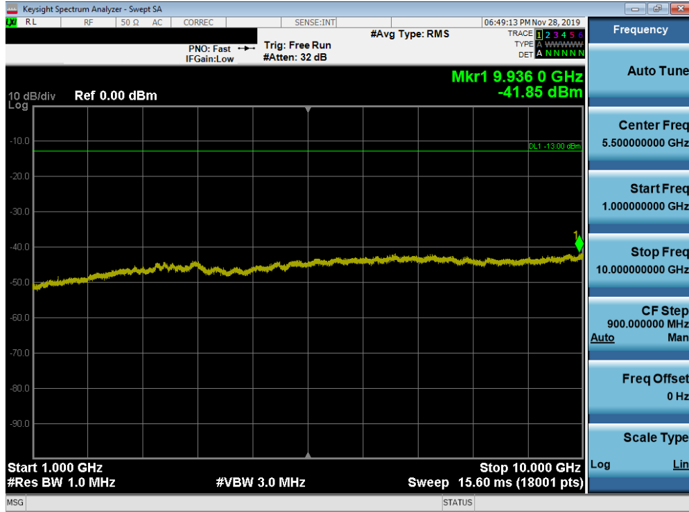
Plot 7-166. Conducted Spurious Plot (Band 12/17 - 10.0MHz QPSK - RB Size 1, RB Offset 0 - High Channel)
