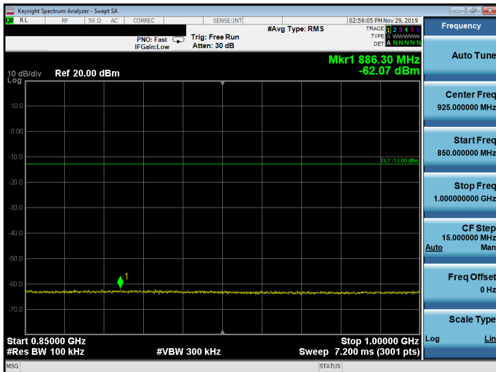
Plot 7-177. Conducted Spurious Plot (Band 26/5 - 10.0MHz QPSK - RB Size 1, RB Offset 0 - High Channel)
