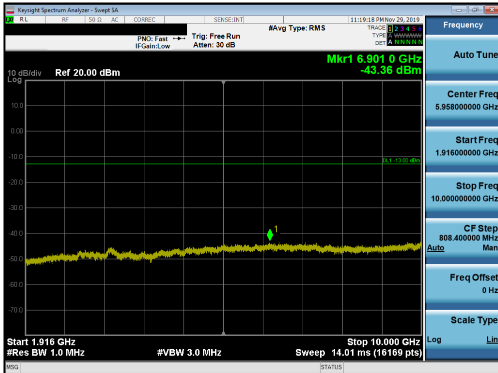
Plot 7-204. Conducted Spurious Plot (Band 25/2 - 20.0MHz QPSK - RB Size 1, RB Offset 0 - High Channel)
