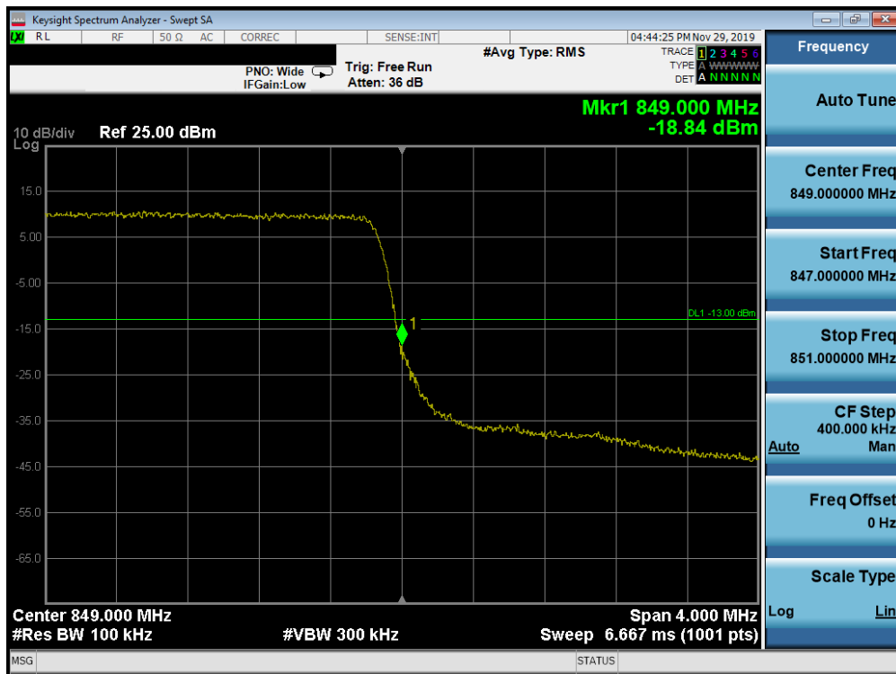
Plot 7-265. Upper Band Edge Plot (Band 26/5 - 3.0MHz QPSK - Full RB Configuration)
