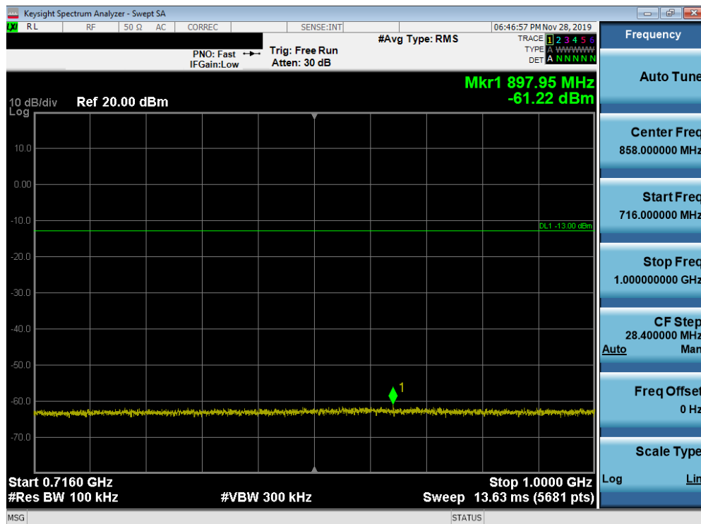
Plot 7-159. Conducted Spurious Plot (Band 12/17 - 10.0MHz QPSK - RB Size 1, RB Offset 0 - Low Channel)
