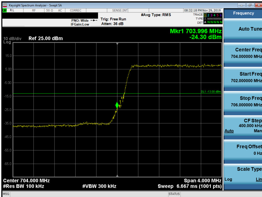
Plot 7-249. Lower Band Edge Plot (Band 17 - 5.0MHz QPSK - Full RB Configuration)
