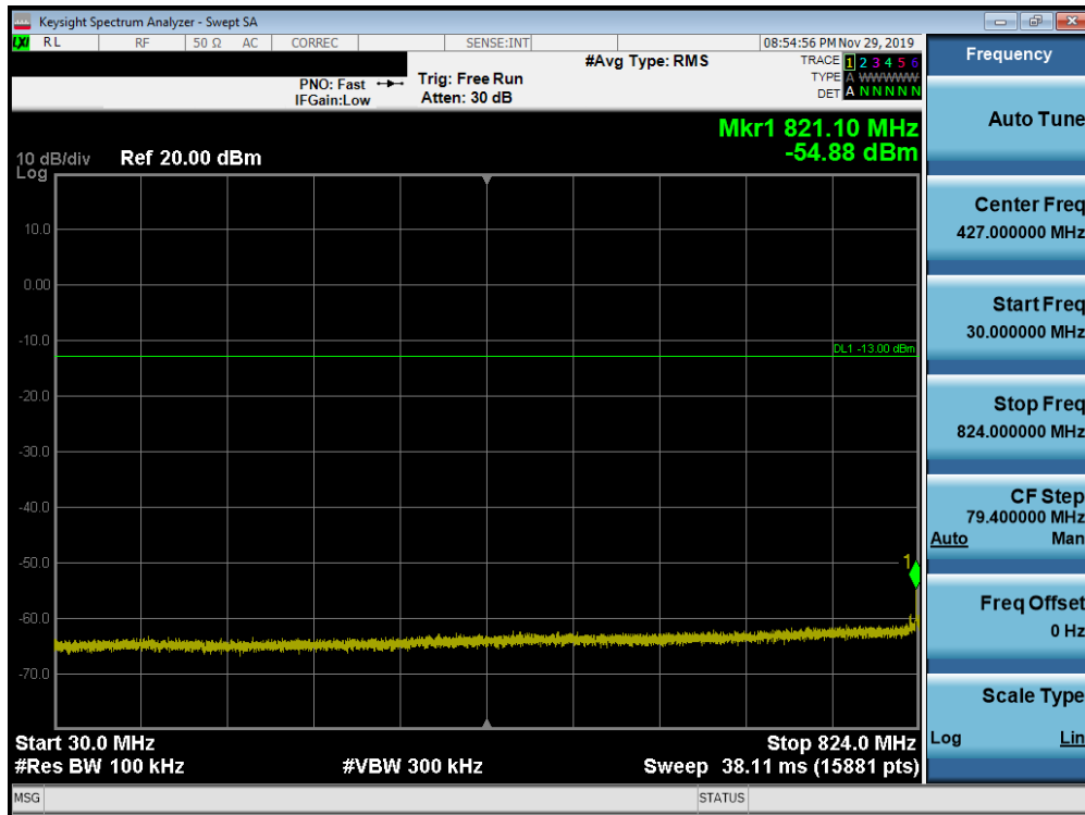
Plot 7-182. Conducted Spurious Plot (Band 26 - 15.0MHz QPSK - RB Size 1, RB Offset 0 - Mid Channel)
