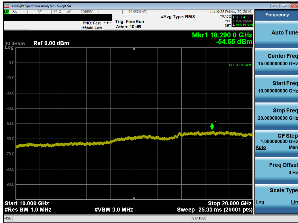
Plot 7-205. Conducted Spurious Plot (Band 25/2 - 20.0MHz QPSK - RB Size 1, RB Offset 0 - High Channel)
