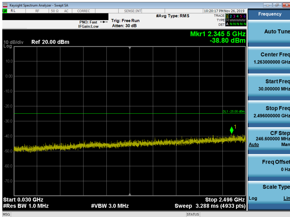
Plot 7-221. Conducted Spurious Plot (Band 41 (PC2) - 20.0MHz QPSK - RB Size 1, RB Offset 0 - Mid Channel)
