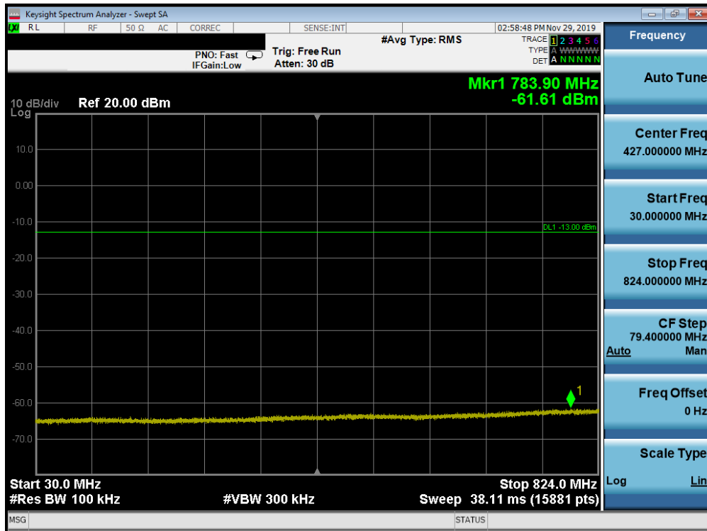
Plot 7-176. Conducted Spurious Plot (Band 26/5 - 10.0MHz QPSK - RB Size 1, RB Offset 0 - High Channel)
