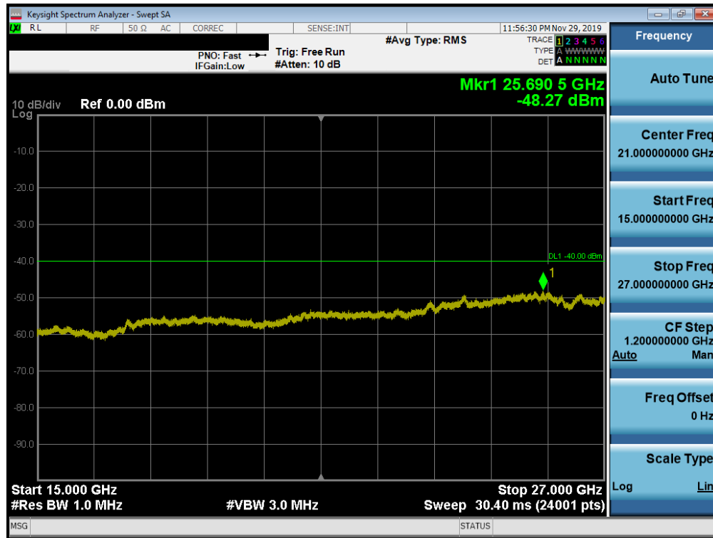
Plot 7-208. Conducted Spurious Plot (Band 30 - 10.0MHz QPSK - RB Size 1, RB Offset 0 – Mid Channel)
