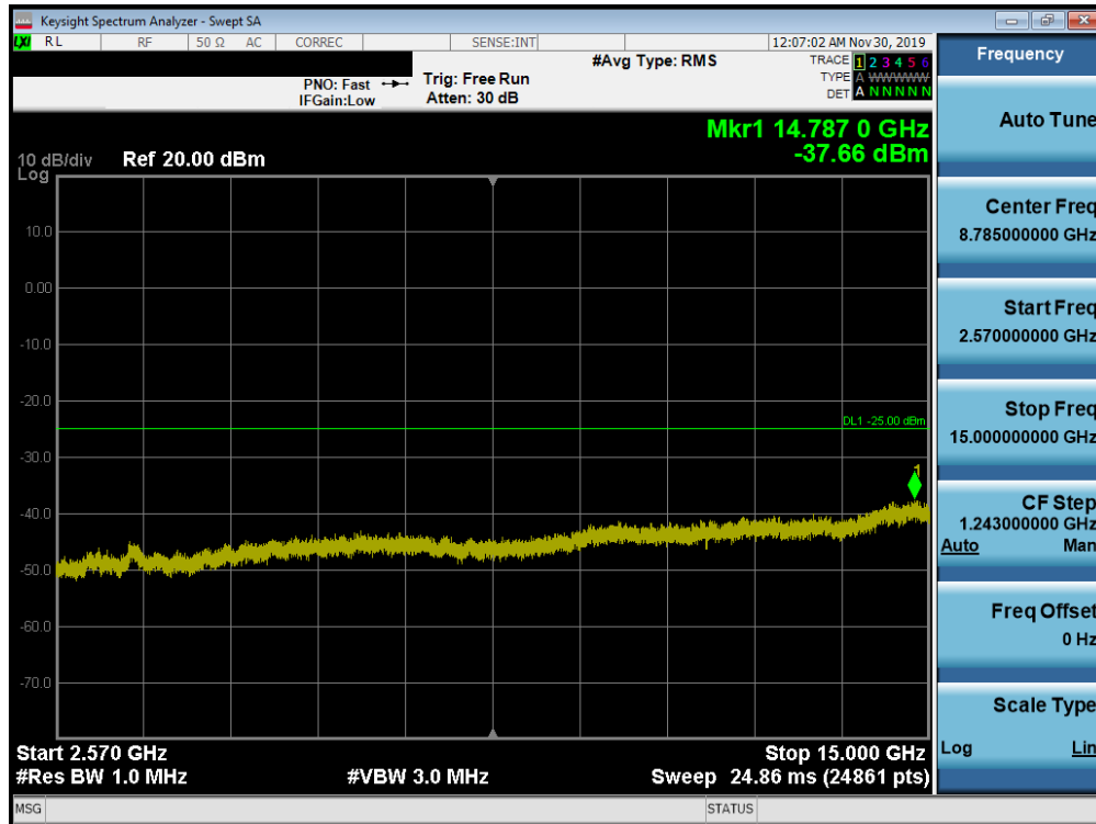
Plot 7-213. Conducted Spurious Plot (Band 7 - 20.0MHz QPSK - RB Size 1, RB Offset 0 – Mid Channel)
