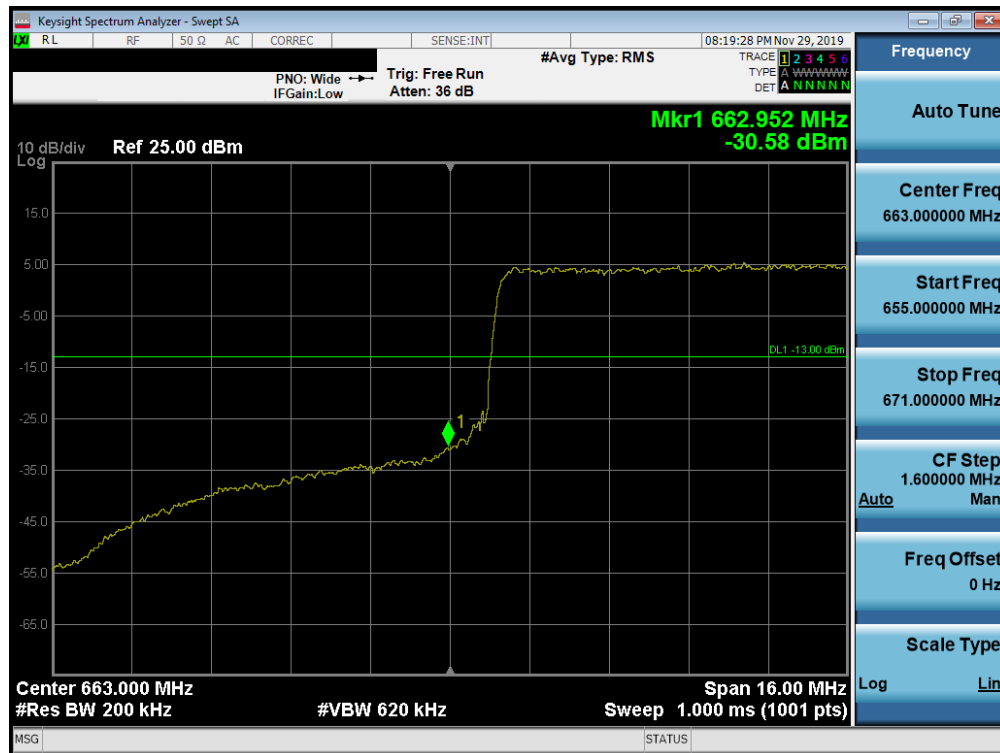
Plot 7-242. Lower Band Edge Plot (Band 71 - 20.0MHz QPSK - Full RB Configuration)
