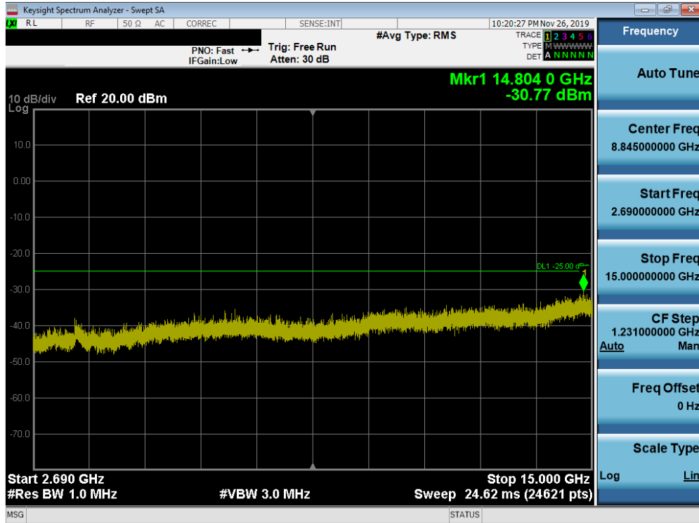
Plot 7-222. Conducted Spurious Plot (Band 41 (PC2) - 20.0MHz QPSK - RB Size 1, RB Offset 0 – Mid Channel)
