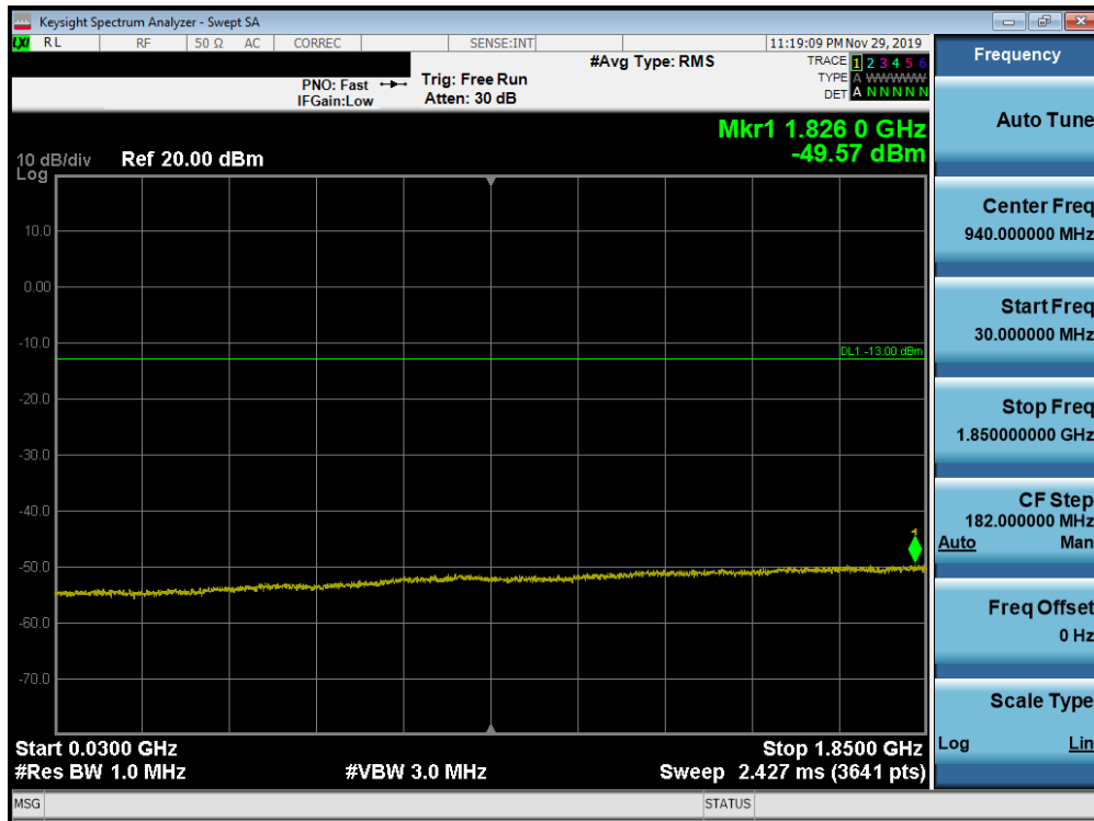
Plot 7-203. Conducted Spurious Plot (Band 25/2 - 20.0MHz QPSK - RB Size 1, RB Offset 0 - High Channel)
