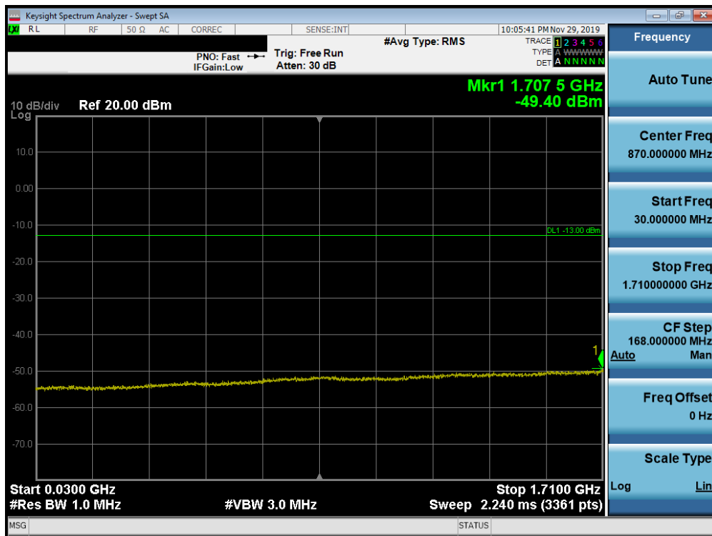
Plot 7-191. Conducted Spurious Plot (Band 66/4 - 20.0MHz QPSK - RB Size 1, RB Offset 0 - Mid Channel)
