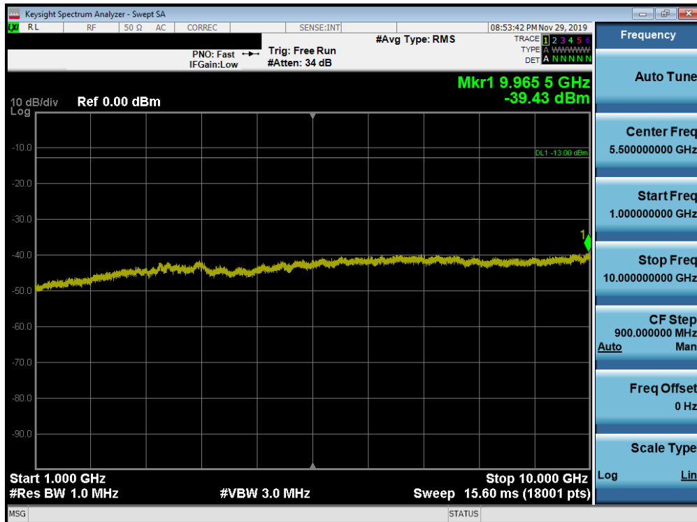
Plot 7-181. Conducted Spurious Plot (Band 26 - 15.0MHz QPSK - RB Size 1, RB Offset 0 - Low Channel)
