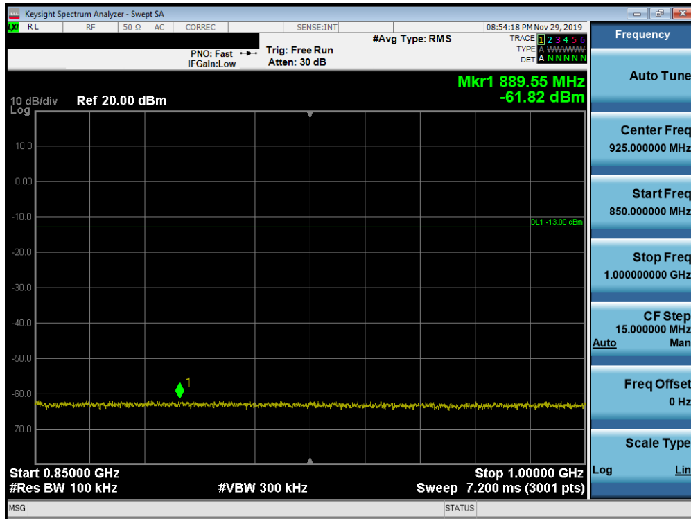
Plot 7-186. Conducted Spurious Plot (Band 26 - 15.0MHz QPSK - RB Size 1, RB Offset 0 - High Channel)
