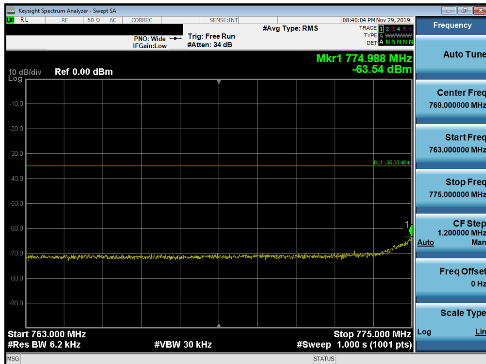
Plot 7-259. Lower Emission Mask Plot (Band 13 - 10.0MHz QPSK - Full RB Configuration)
