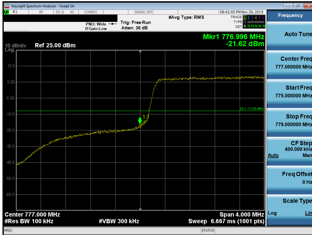
Plot 7-254. Lower Band Edge Plot (Band 13 - 5.0MHz QPSK - Full RB Configuration)
