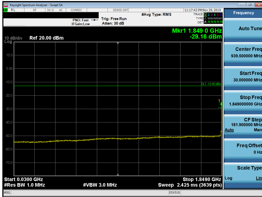
Plot 7-197. Conducted Spurious Plot (Band 25/2 - 20.0MHz QPSK - RB Size 1, RB Offset 0 - Low Channel)
