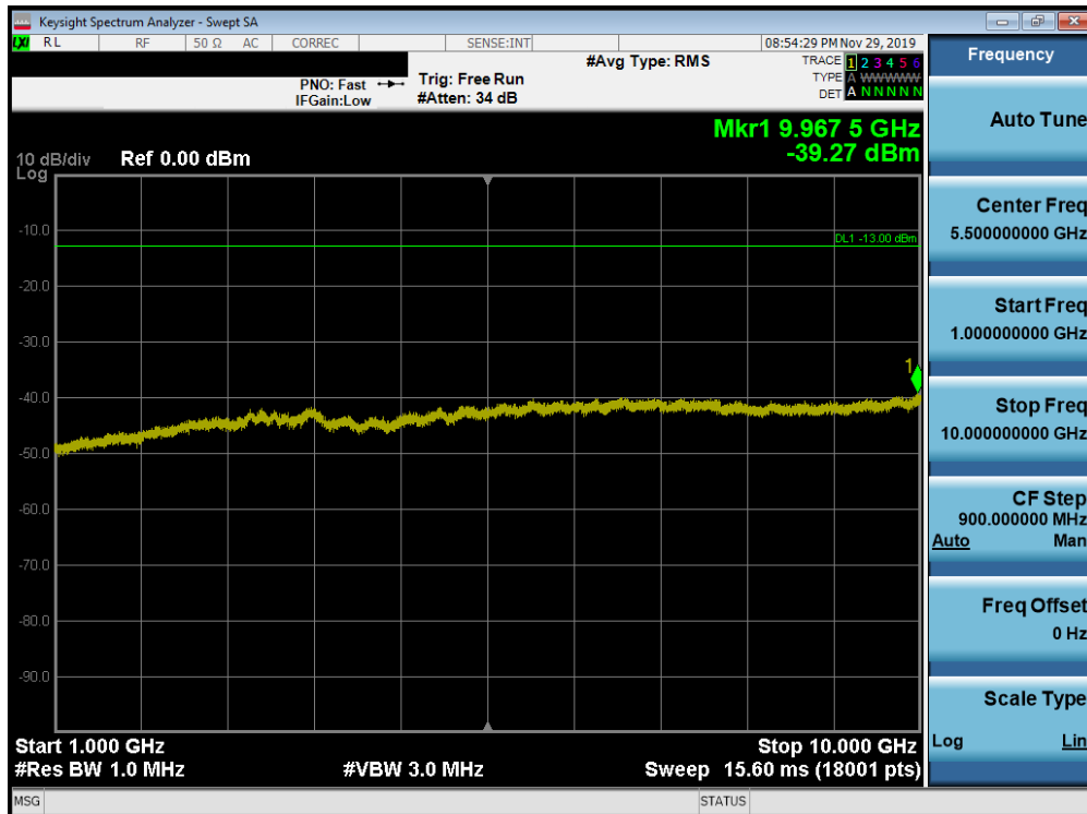
Plot 7-187. Conducted Spurious Plot (Band 26 - 15.0MHz QPSK - RB Size 1, RB Offset 0 - High Channel)
