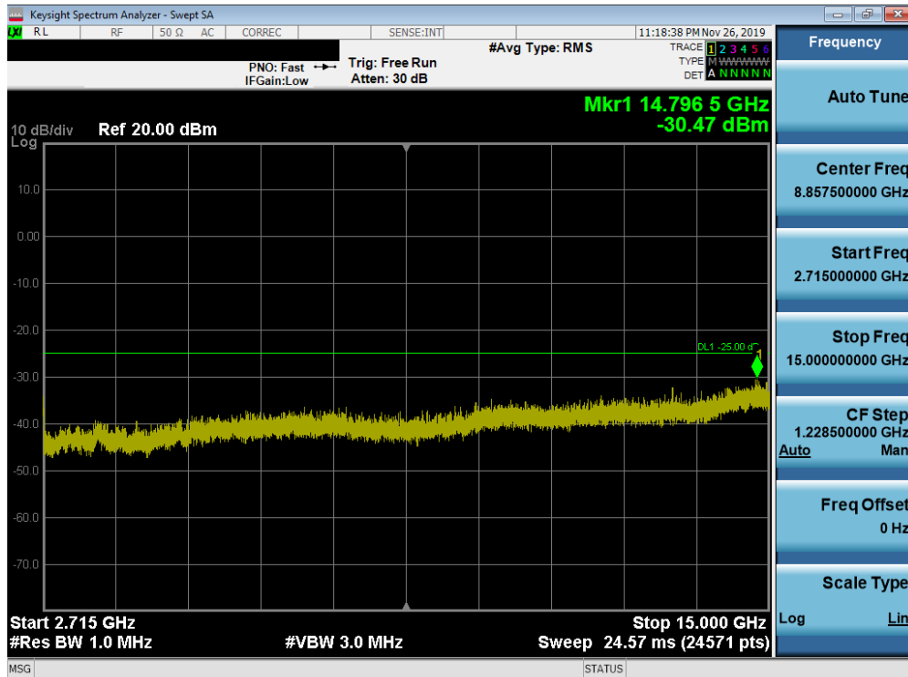
Plot 7-234. Conducted Spurious Plot (Band 41 (PC3) - 20.0MHz QPSK - RB Size 1, RB Offset 0 – High Channel)
