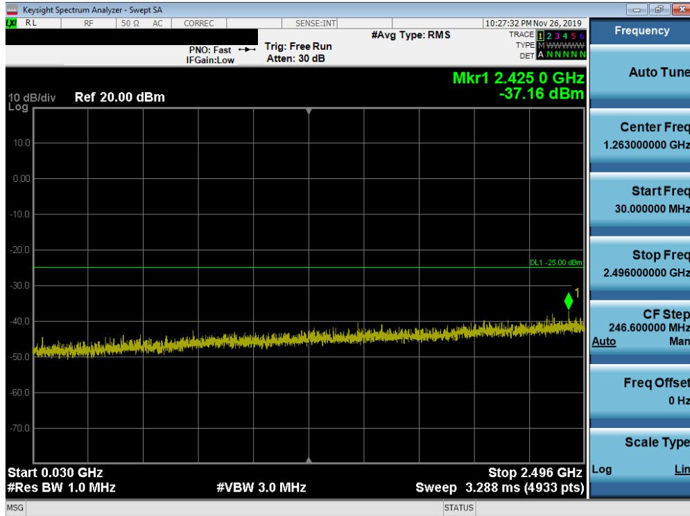
Plot 7-224. Conducted Spurious Plot (Band 41 (PC2) - 20.0MHz QPSK - RB Size 1, RB Offset 0 – High Channel)
