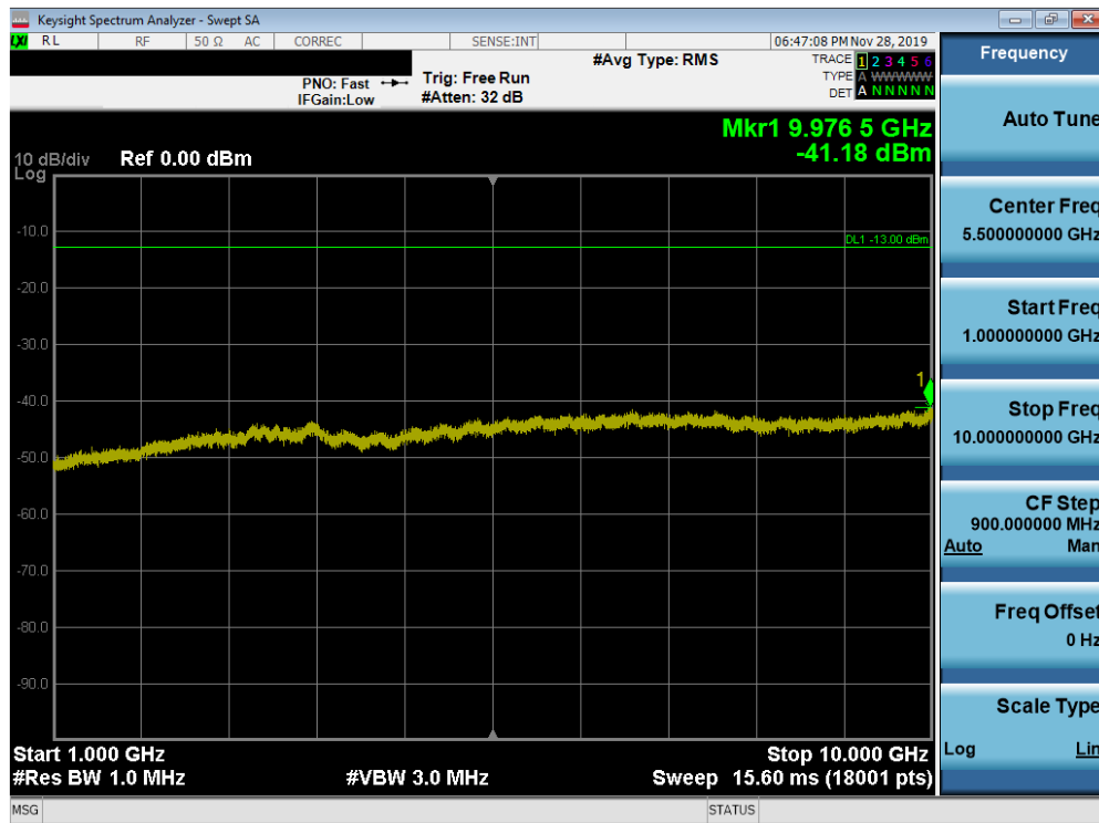
Plot 7-160. Conducted Spurious Plot (Band 12/17 - 10.0MHz QPSK - RB Size 1, RB Offset 0 - Low Channel)
