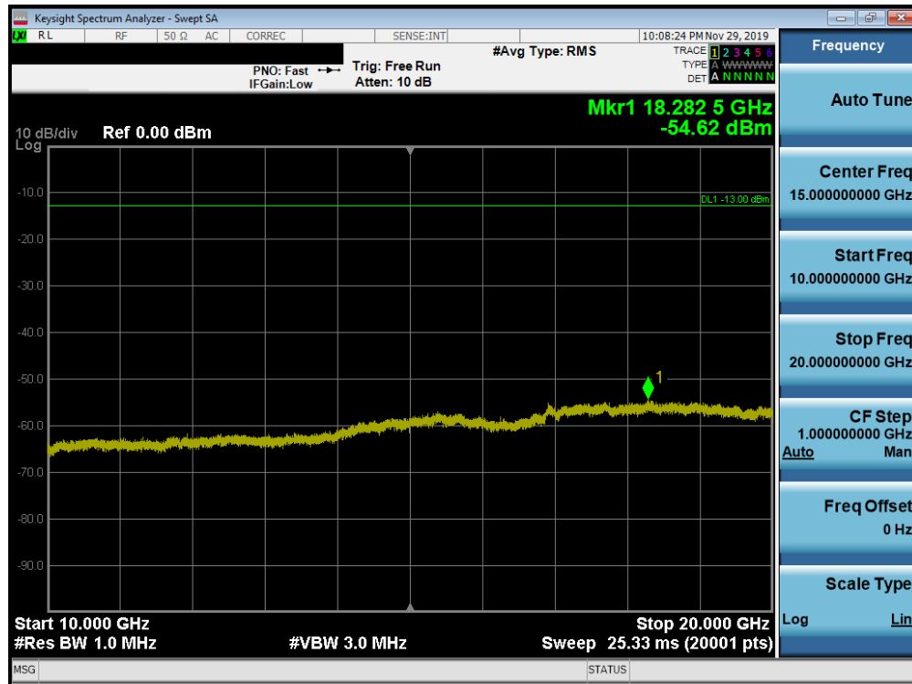
Plot 7-196. Conducted Spurious Plot (Band 66/4 - 20.0MHz QPSK - RB Size 1, RB Offset 0 - High Channel)
