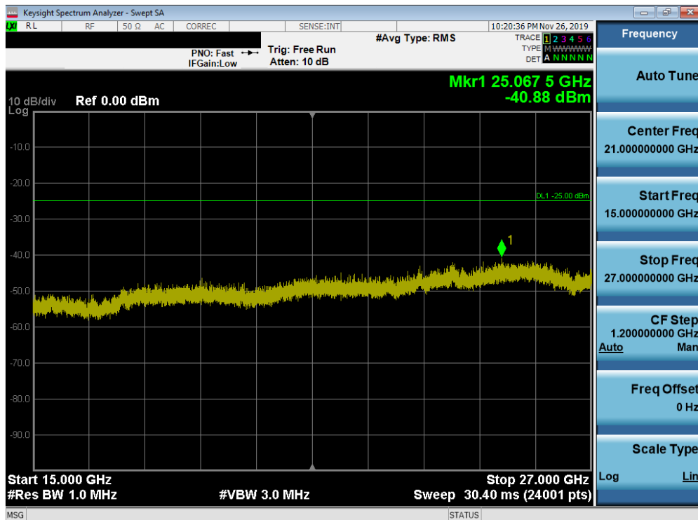
Plot 7-223. Conducted Spurious Plot (Band 41 (PC2) - 20.0MHz QPSK - RB Size 1, RB Offset 0 – Mid Channel)
