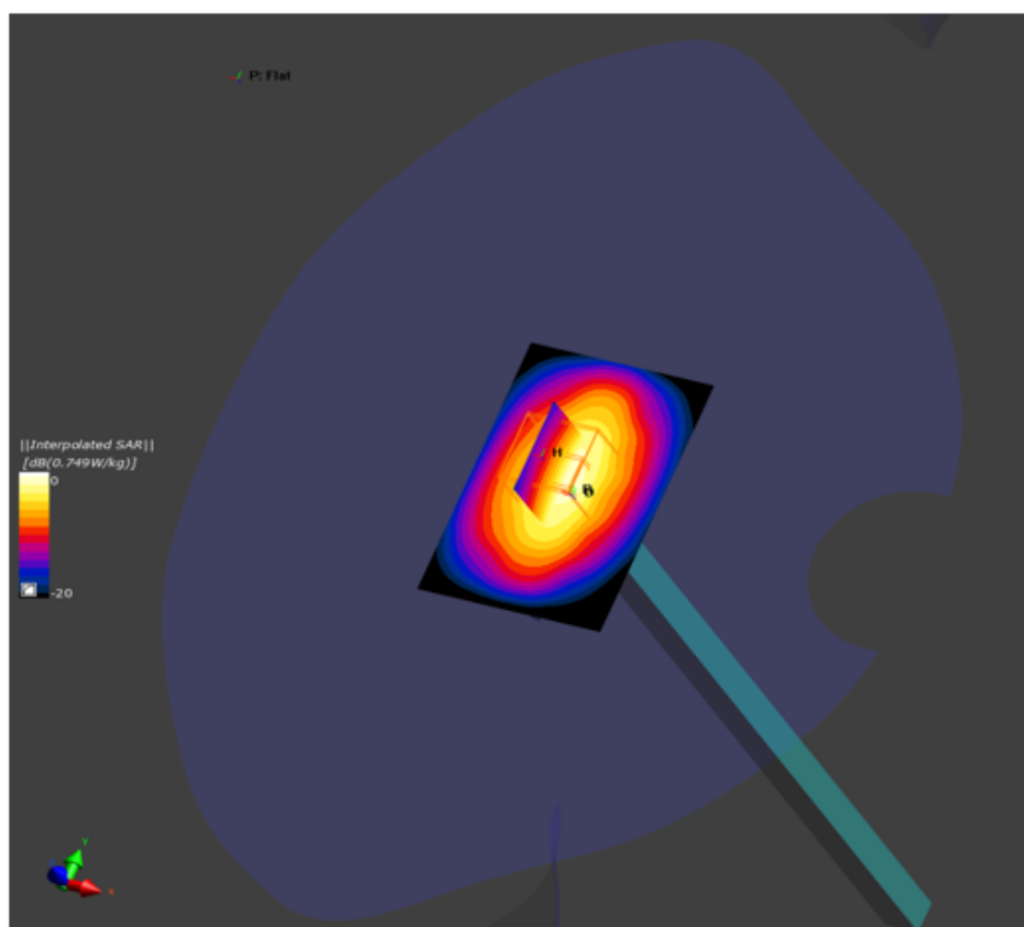
Figure C-2 SAR measurement system verification plot for 1800MHz performed on 1/19/2020. Input power = 10.0mW.
