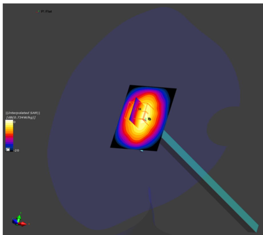
Figure C-3 SAR measurement system verification plot for 1800MHz performed on 1/20/2020. Input power = 10.0mW.
