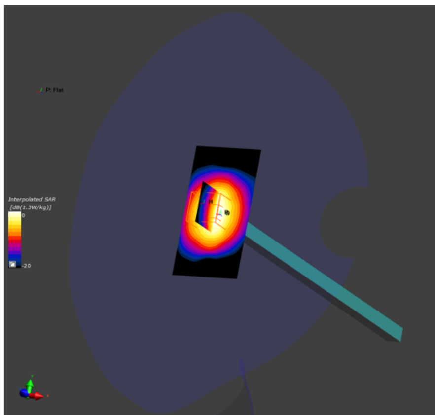
Figure C-1 SAR measurement system verification plot for 2600MHz performed on 1/18/2020. Input power = 10.0mW.
