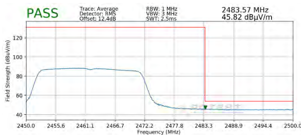
Plot 7-95. Radiated Restricted Upper Band Edge Measurement SISO ANT2 (Average – 242 Tones)
