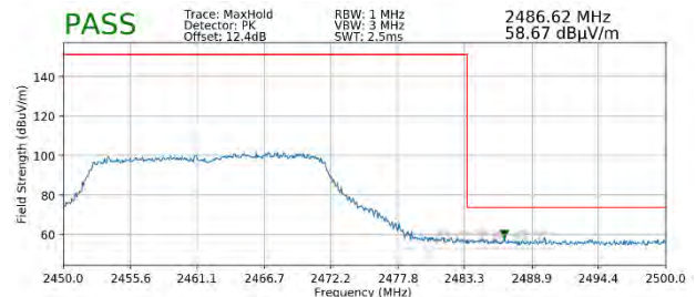
Plot 7-88. Radiated Restricted Upper Band Edge Measurement SISO ANT1 (Peak – 242 Tones)
