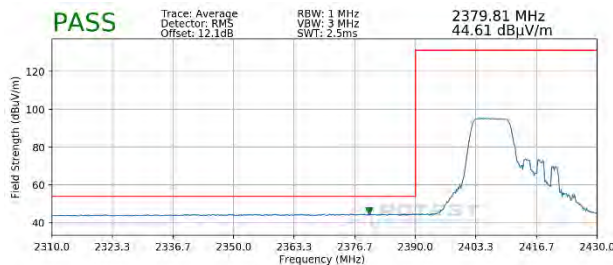
Plot 7-81. Radiated Restricted Lower Band Edge Measurement SISO ANT1 (Average – 106 Tones)
