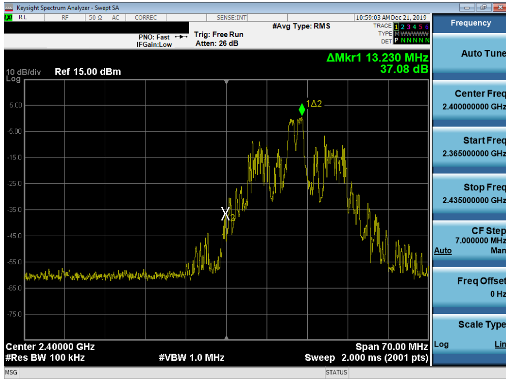
Plot 7-29. Band Edge Plot SISO ANT2 (802.11ax OFDMA - 26 Tones - Ch. 1)
