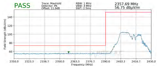
Plot 7-98. Radiated Restricted Lower Band Edge Measurement MIMO (Peak – 106 Tones)
