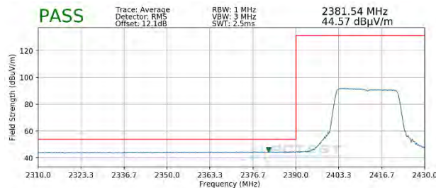
Plot 7-85. Radiated Restricted Lower Band Edge Measurement SISO ANT1 (Average – 242 Tones)
