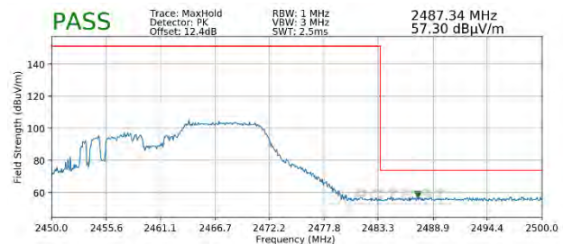
Plot 7-84. Radiated Restricted Upper Band Edge Measurement SISO ANT1 (Peak – 106 Tones)
