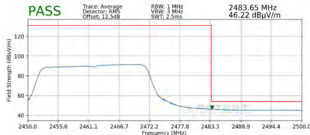
Plot 7-87. Radiated Restricted Upper Band Edge Measurement SISO ANT1 (Average – 242 Tones)
