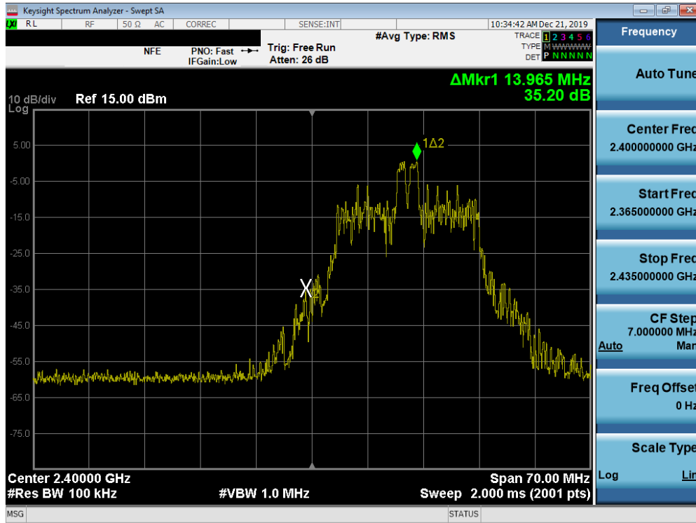
Plot 7-25. Band Edge Plot SISO ANT1 (802.11ax OFDMA - 26 Tones - Ch. 1)
