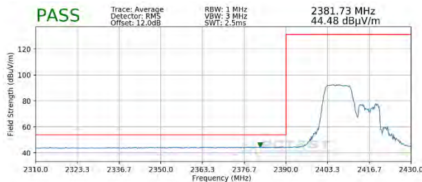
Plot 7-97. Radiated Restricted Lower Band Edge Measurement MIMO (Average – 106 Tones)
