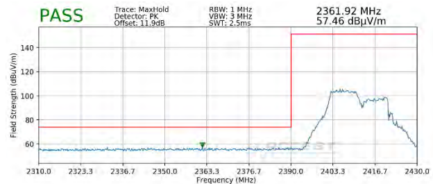
Plot 7-82. Radiated Restricted Lower Band Edge Measurement SISO ANT1 (Peak – 106 Tones)
