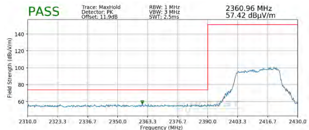
Plot 7-94. Radiated Restricted Lower Band Edge Measurement SISO ANT2 (Peak – 242 Tones)
