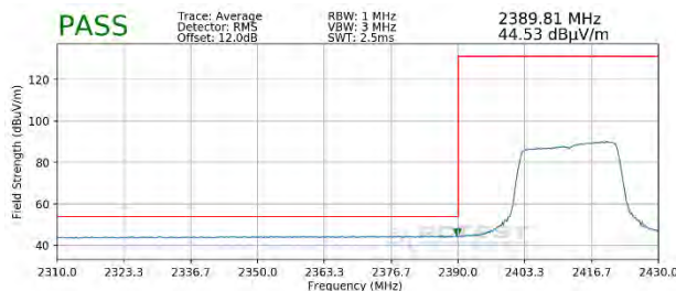
Plot 7-93. Radiated Restricted Lower Band Edge Measurement SISO ANT2 (Average – 242 Tones)
