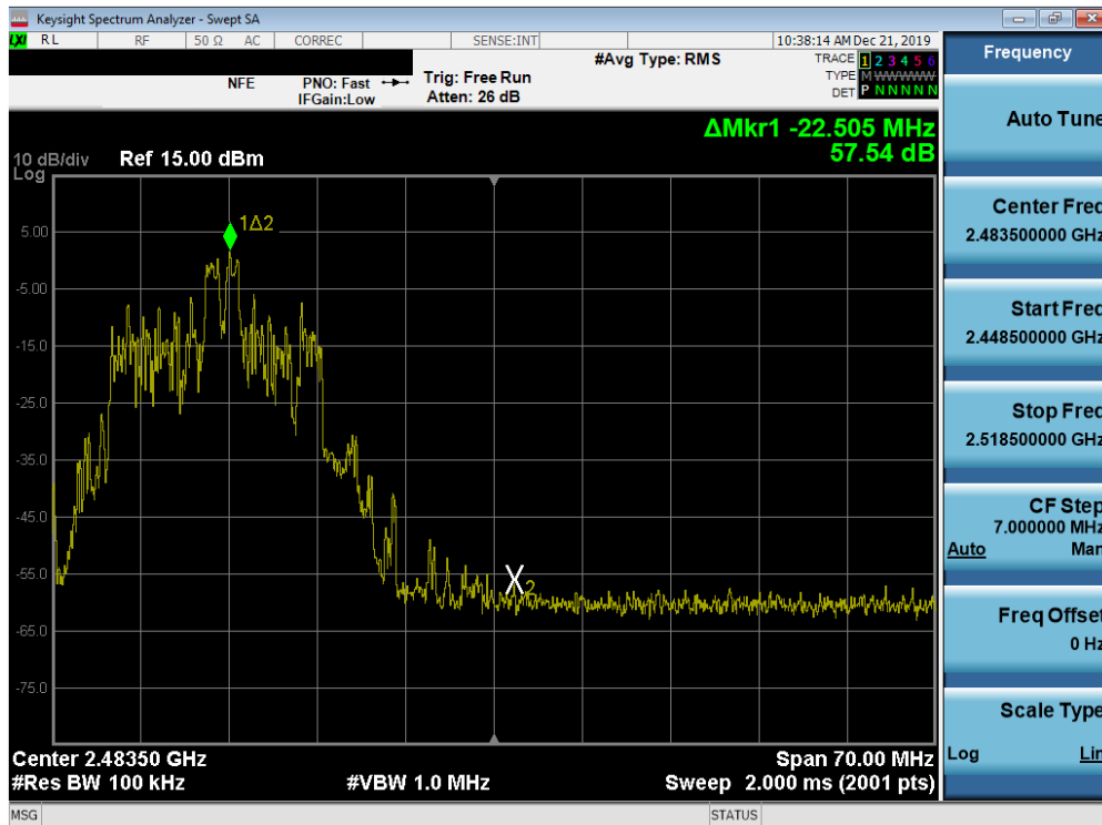
Plot 7-26. Band Edge Plot SISO ANT1 (802.11ax OFDMA - 26 Tones - Ch. 11)
