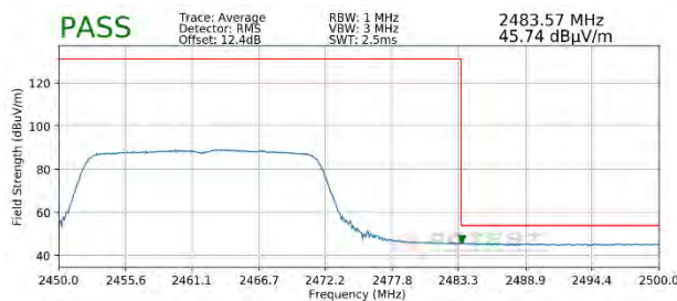
Plot 7-103. Radiated Restricted Upper Band Edge Measurement MIMO (Average – 242 Tones)
