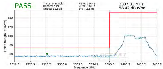
Plot 7-90. Radiated Restricted Lower Band Edge Measurement SISO ANT2 (Peak – 106 Tones)
