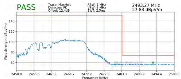
Plot 7-100. Radiated Restricted Upper Band Edge Measurement MIMO (Peak – 106 Tones)
