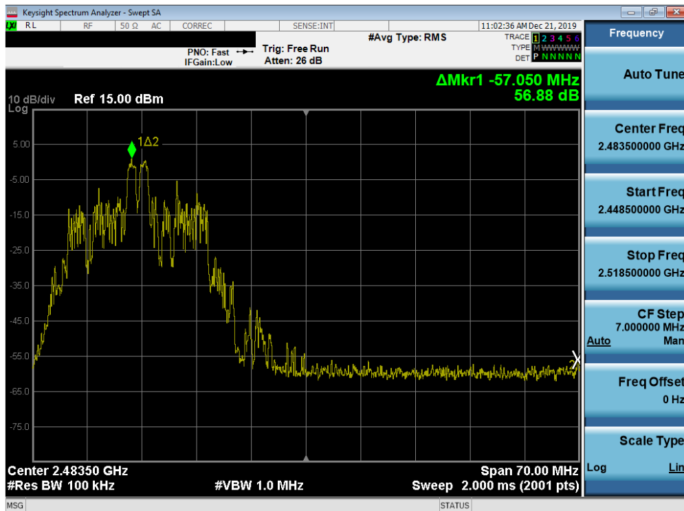
Plot 7-30. Band Edge Plot SISO ANT2 (802.11ax OFDMA - 26 Tones - Ch. 11)
