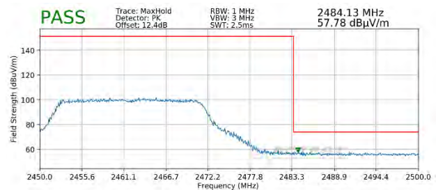
Plot 7-104. Radiated Restricted Upper Band Edge Measurement MIMO (Peak – 242 Tones)
