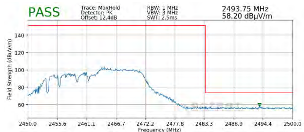
Plot 7-92. Radiated Restricted Upper Band Edge Measurement SISO ANT2 (Peak – 106 Tones)
