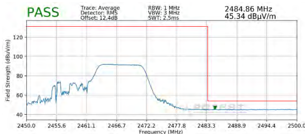
Plot 7-99. Radiated Restricted Upper Band Edge Measurement MIMO (Average – 106 Tones)
