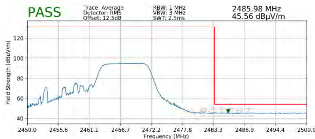
Plot 7-83. Radiated Restricted Upper Band Edge Measurement SISO ANT1 (Average – 106 Tones)
