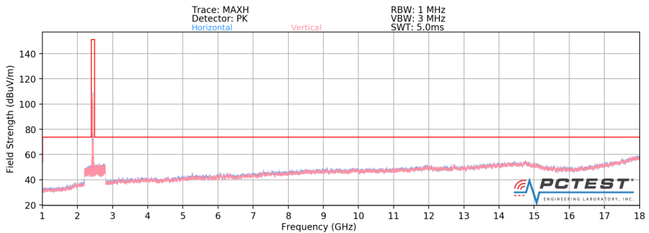
Plot 7-110. Radiated Spurious Plot above 1GHz SISO ANT1 (802.11b – Ch. 6)
