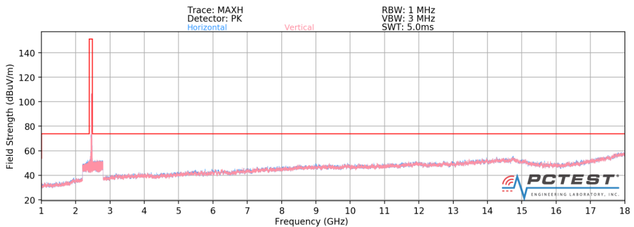
Plot 7-111. Radiated Spurious Plot above 1GHz SISO ANT1 (802.11b – Ch. 11)
