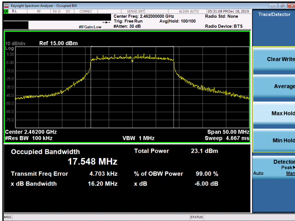
Plot 7-24. 6dB Bandwidth Plot SISO ANT2 (802.11n (2.4GHz) – Ch. 11)
