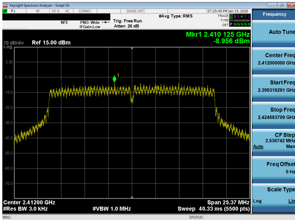
Plot 7-55. Power Spectral Density Plot SISO ANT2 (802.11ac (2.4GHz) – Ch. 1)
