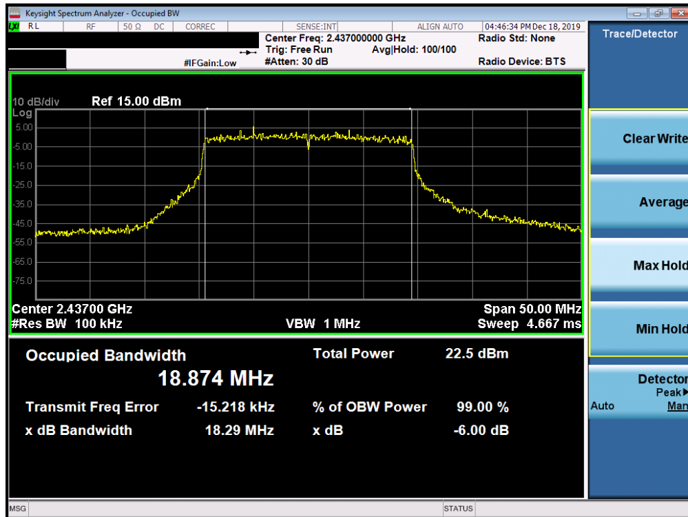
Plot 7-14. 6dB Bandwidth Plot SISO ANT1 (802.11ax (2.4GHz) – Ch. 6)
