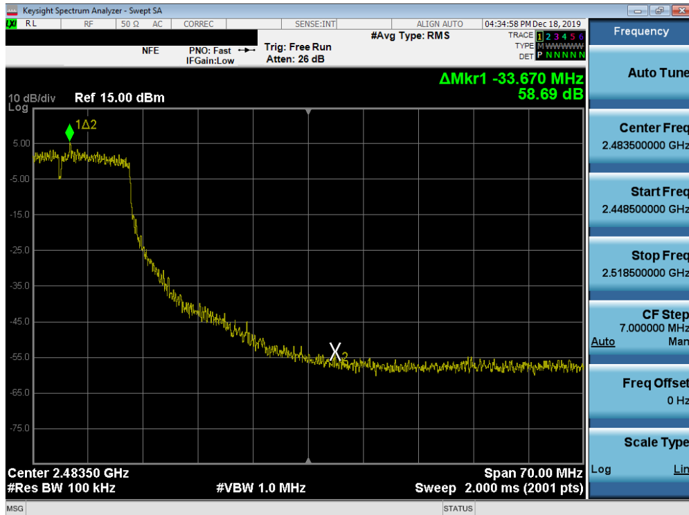
Plot 7-69. Band Edge Plot SISO ANT1 (802.11n – Ch. 9)
