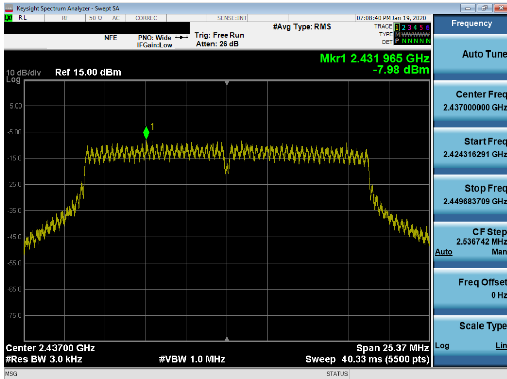
Plot 7-41. Power Spectral Density Plot SISO ANT1 (802.11ac (2.4GHz) – Ch. 6)
