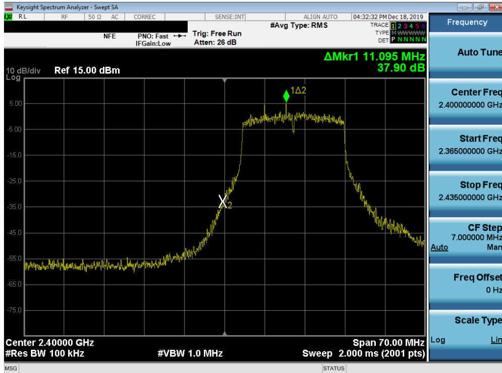
Plot 7-67. Band Edge Plot SISO ANT1 (802.11n (2.4GHz) – Ch. 1)
