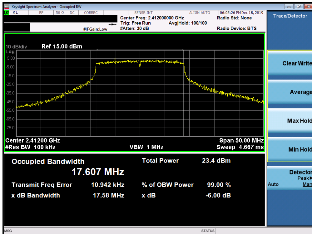
Plot 7-25. 6dB Bandwidth Plot SISO ANT2 (802.11ac (2.4GHz) – Ch. 1)
