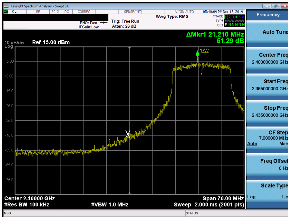
Plot 7-94. Band Edge Plot SISO ANT2 (802.11ax – Ch. 3)
