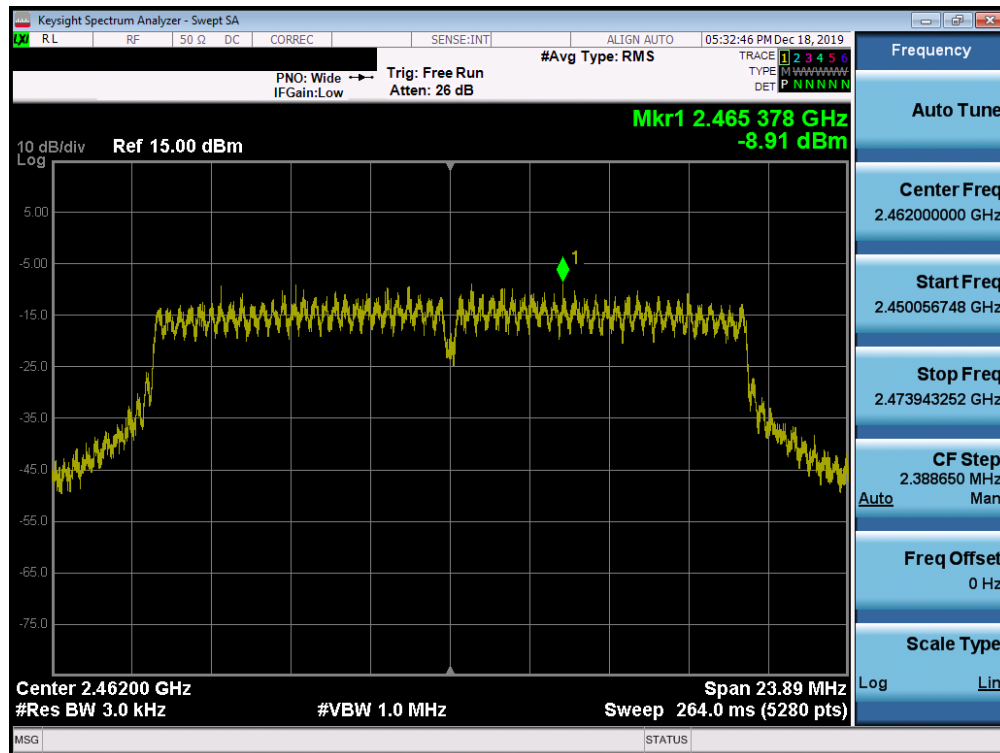
Plot 7-60. Power Spectral Density Plot SISO ANT2 (802.11ax (2.4GHz) – Ch. 11)
