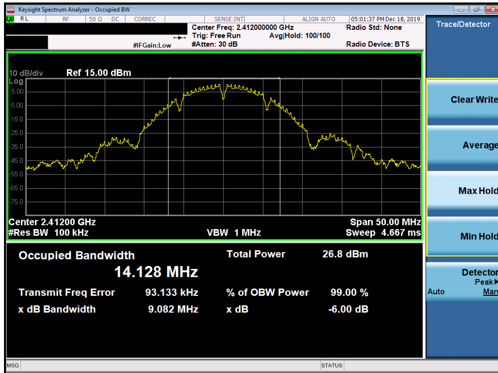
Plot 7-16. 6dB Bandwidth Plot SISO ANT2 (802.11b – Ch. 1)
