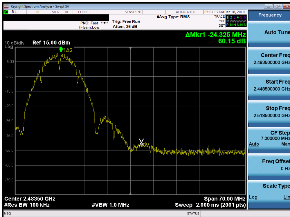
Plot 7-80. Band Edge Plot SISO ANT2 (802.11b – Ch. 11)
