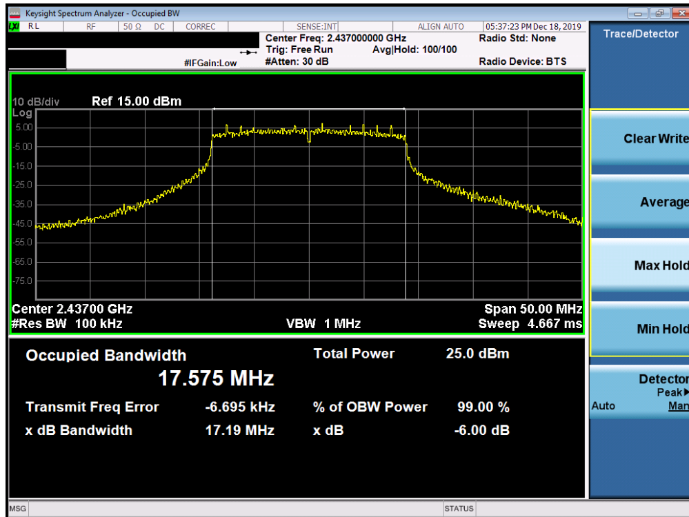
Plot 7-29. 6dB Bandwidth Plot SISO ANT2 (802.11ax (2.4GHz) – Ch. 6)
