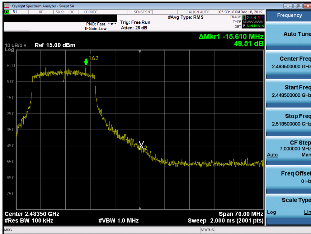
Plot 7-96. Band Edge Plot SISO ANT2 (802.11ax (2.4GHz) – Ch. 11)
