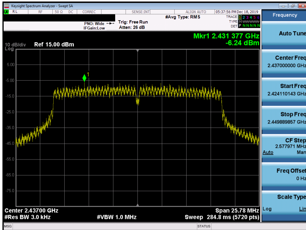
Plot 7-59. Power Spectral Density Plot SISO ANT2 (802.11ax (2.4GHz) - Ch. 6)
