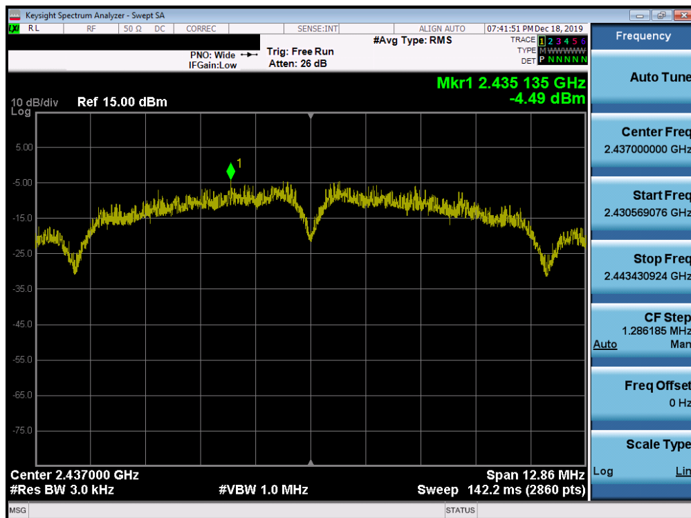
Plot 7-32. Power Spectral Density Plot SISO ANT1 (802.11b – Ch. 6)
