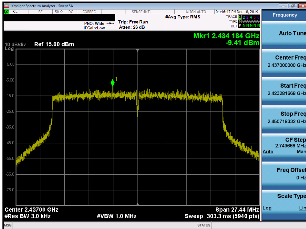
Plot 7-44. Power Spectral Density Plot SISO ANT1 (802.11ax (2.4GHz) – Ch. 6)
