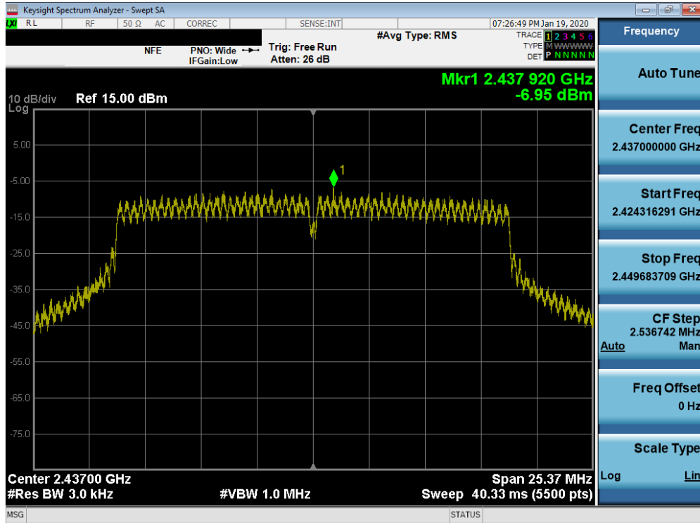
Plot 7-56. Power Spectral Density Plot SISO ANT2 (802.11ac (2.4GHz) – Ch. 6)
