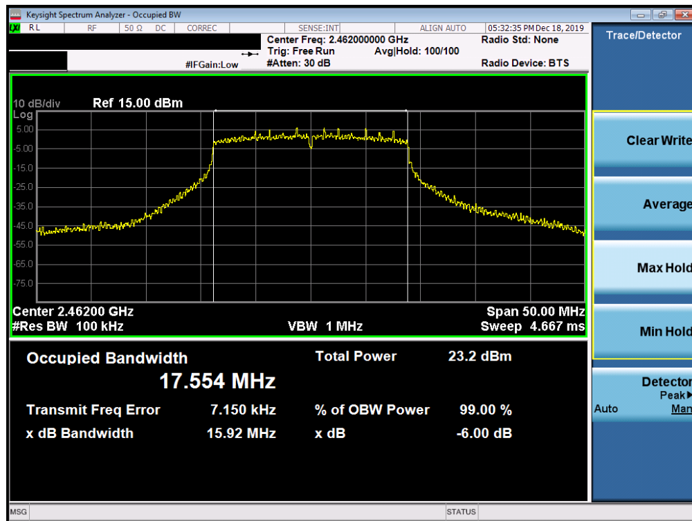
Plot 7-30. 6dB Bandwidth Plot SISO ANT2 (802.11ax (2.4GHz) – Ch. 11)
