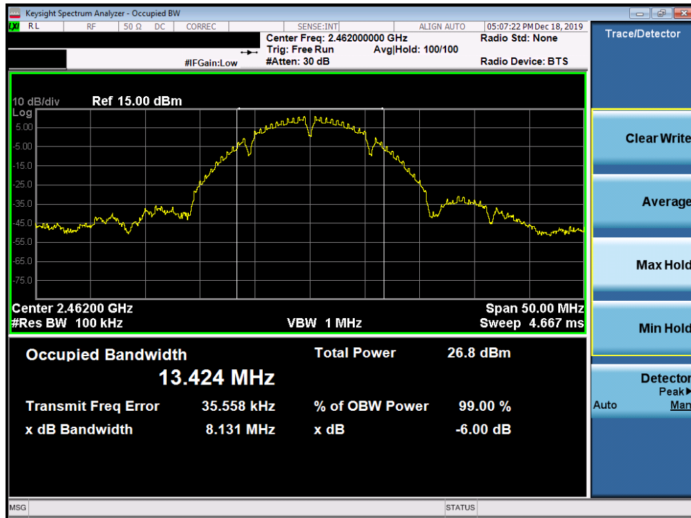
Plot 7-18. 6dB Bandwidth Plot SISO ANT2 (802.11b – Ch. 11)
