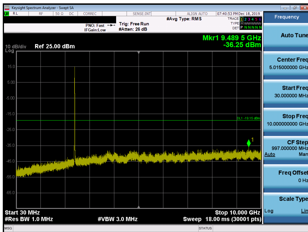
Plot 7-97. Conducted Spurious Plot SISO ANT1 (802.11b – Ch. 1)
