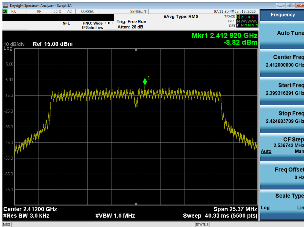
Plot 7-40. Power Spectral Density Plot SISO ANT1 (802.11ac (2.4GHz) – Ch. 1)
