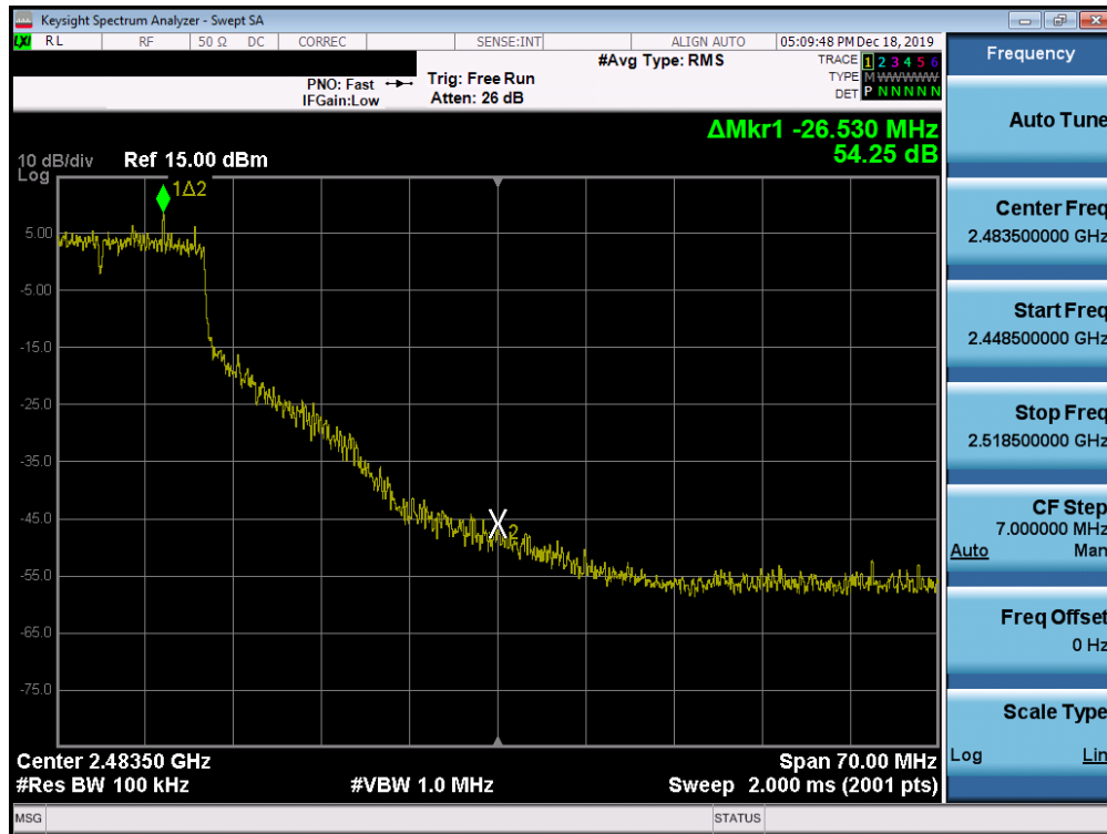
Plot 7-83. Band Edge Plot SISO ANT2 (802.11g- Ch. 9)
