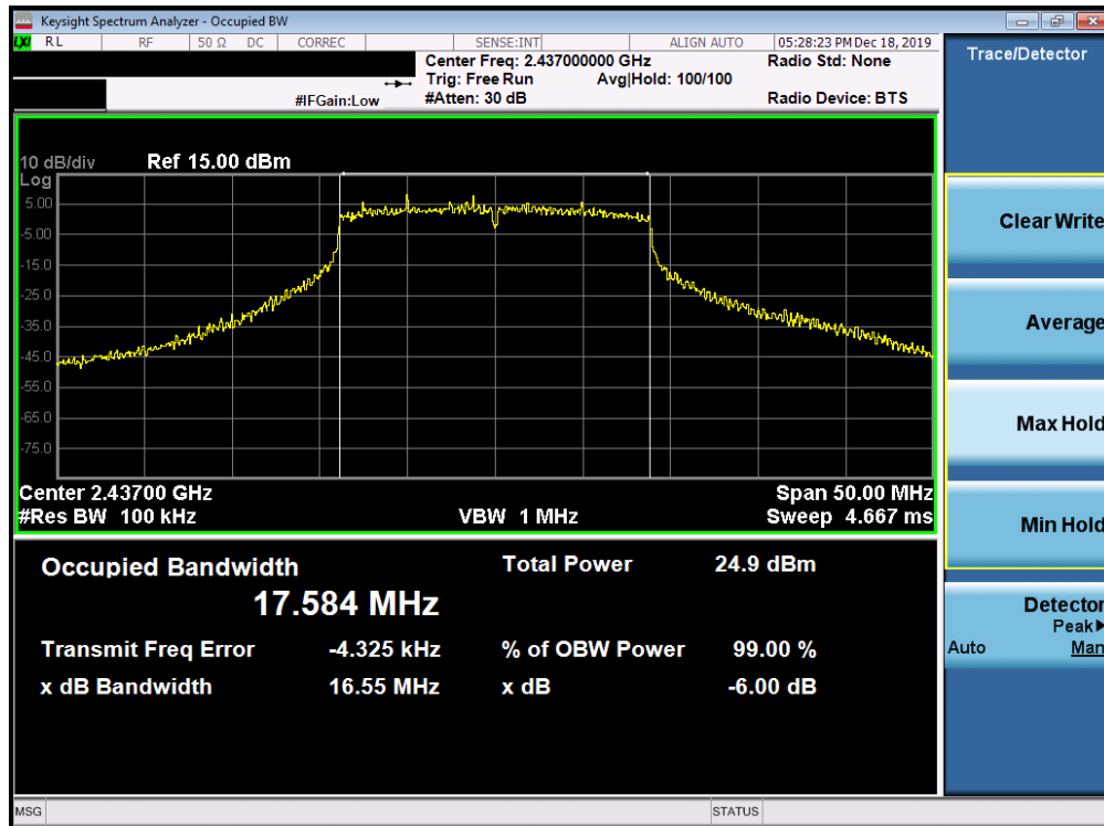
Plot 7-23. 6dB Bandwidth Plot SISO ANT2 (802.11n (2.4GHz) – Ch. 6)
