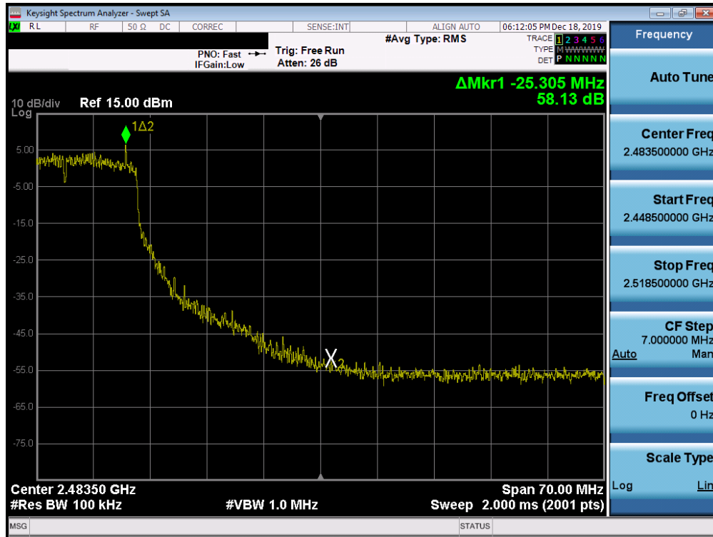
Plot 7-73. Band Edge Plot SISO ANT1 (802.11ac - Ch. 9)
