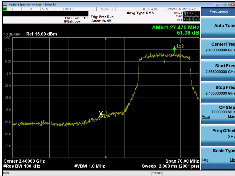
Plot 7-76. Band Edge Plot SISO ANT1 (802.11ax– Ch. 3)
