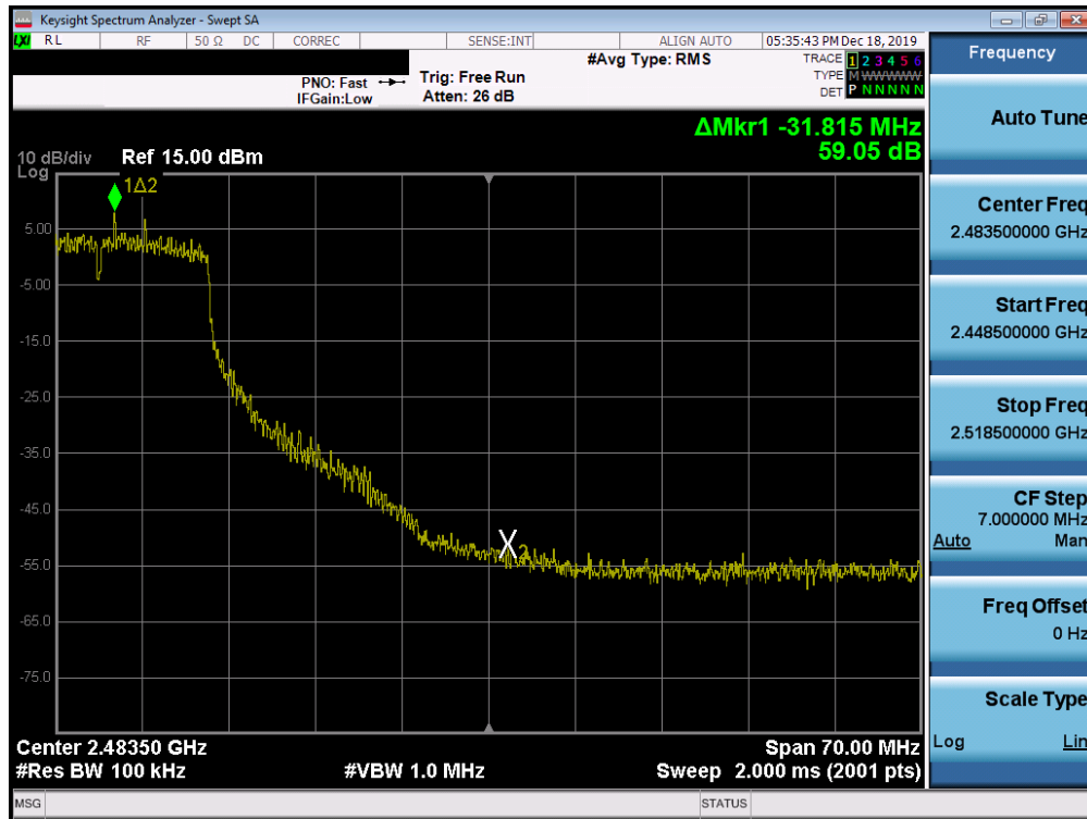
Plot 7-95. Band Edge Plot SISO ANT2 (802.11ax – Ch. 9)
