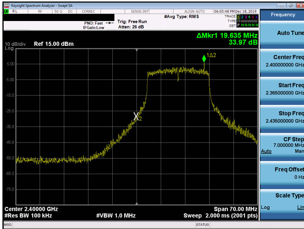
Plot 7-89. Band Edge Plot SISO ANT2 (802.11ac (2.4GHz) – Ch. 1)
