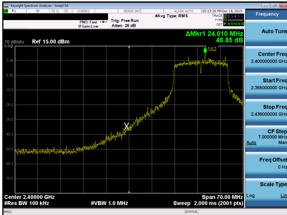
Plot 7-82. Band Edge Plot SISO ANT2 (802.11g- Ch. 3)
