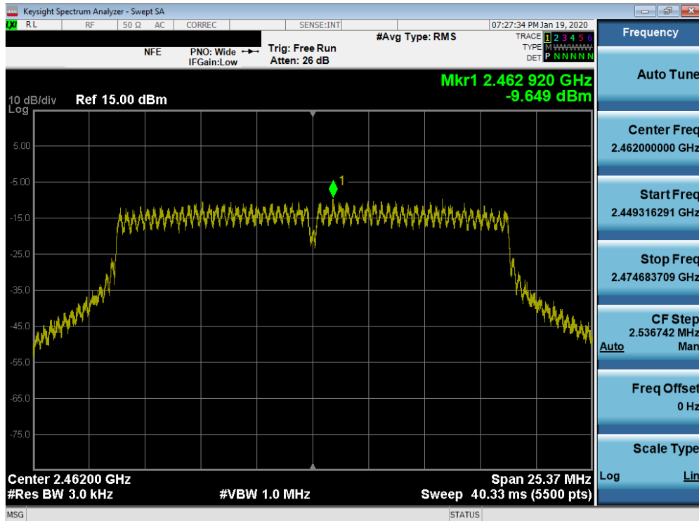
Plot 7-57. Power Spectral Density Plot SISO ANT2 (802.11ac (2.4GHz) – Ch. 11)
