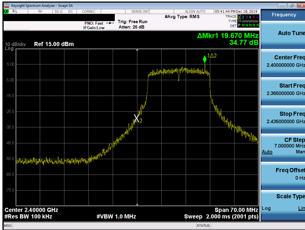
Plot 7-93. Band Edge Plot SISO ANT2 (802.11ax (2.4GHz) – Ch. 1)
