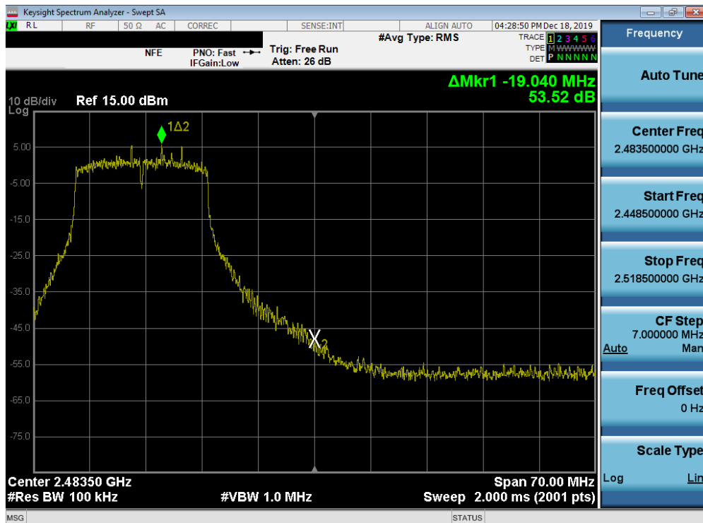
Plot 7-66. Band Edge Plot SISO ANT1 (802.11g - Ch. 11)
