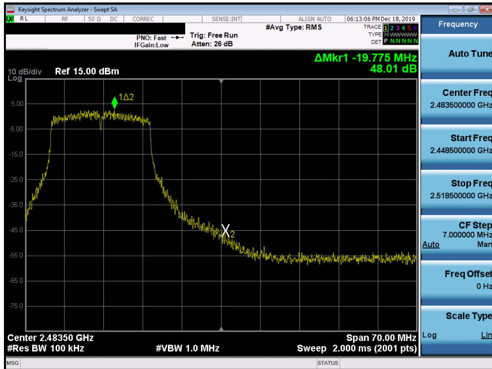
Plot 7-74. Band Edge Plot SISO ANT1 (802.11ac (2.4GHz) - Ch. 11)
