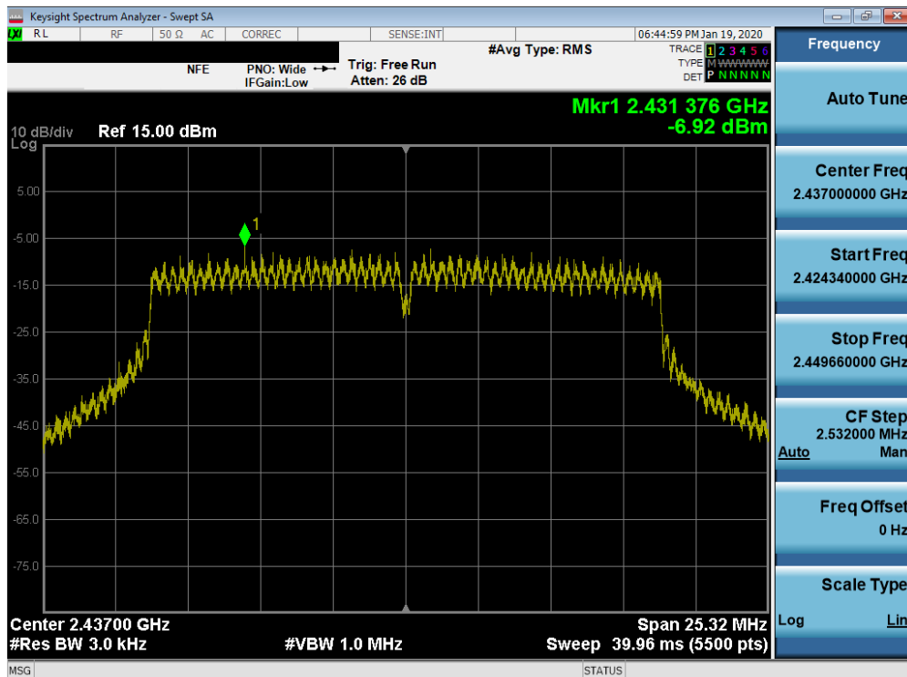
Plot 7-38. Power Spectral Density Plot SISO ANT1 (802.11n (2.4GHz) – Ch. 6)
