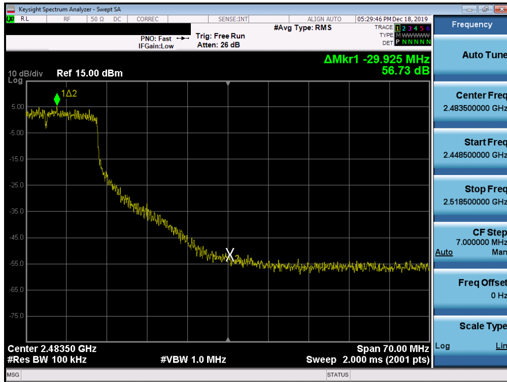
Plot 7-87. Band Edge Plot SISO ANT2 (802.11n- Ch. 9)
