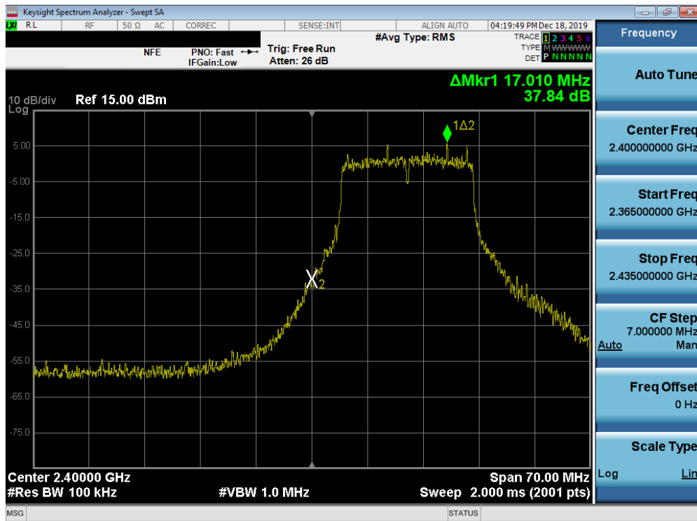
Plot 7-63. Band Edge Plot SISO ANT1 (802.11g- Ch. 1)
