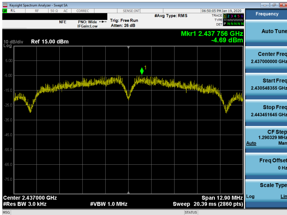
Plot 7-47. Power Spectral Density Plot SISO ANT2 (802.11b – Ch. 6)
