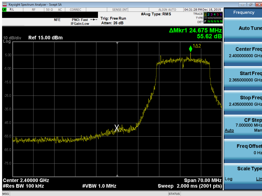
Plot 7-68. Band Edge Plot SISO ANT1 (802.11n– Ch. 3)
