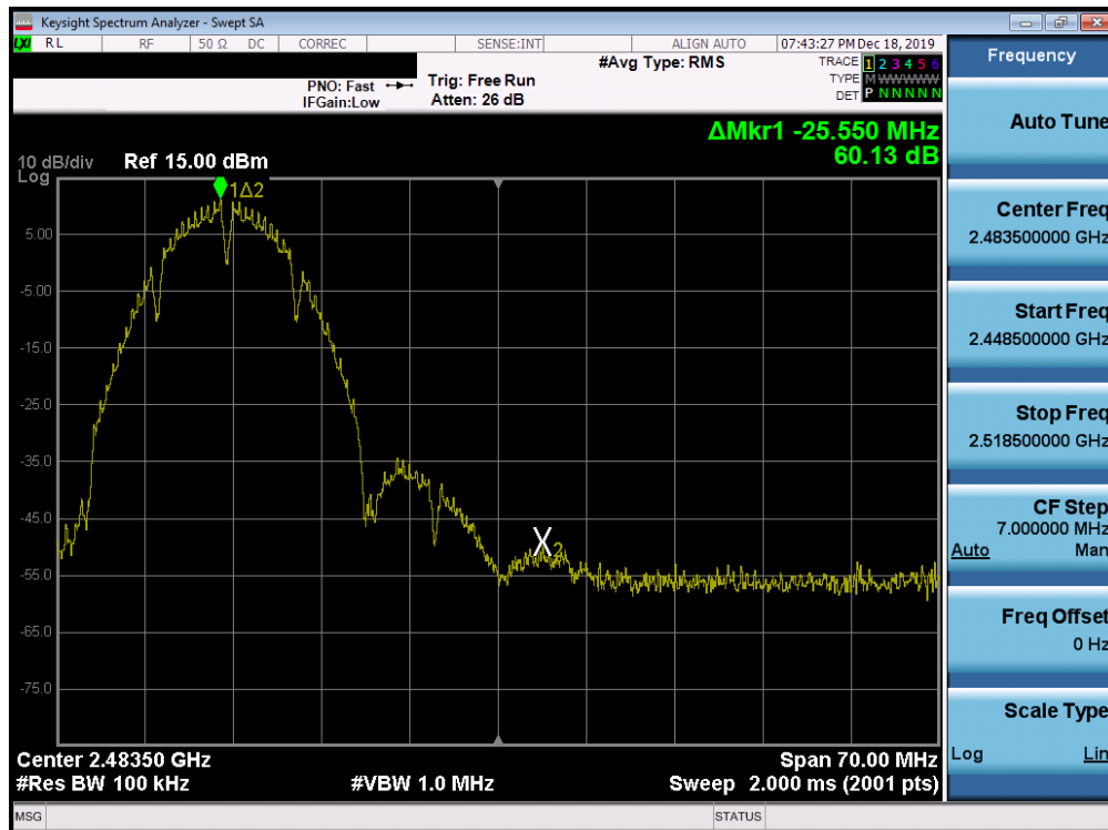
Plot 7-62. Band Edge Plot SISO ANT1 (802.11b – Ch. 11)
