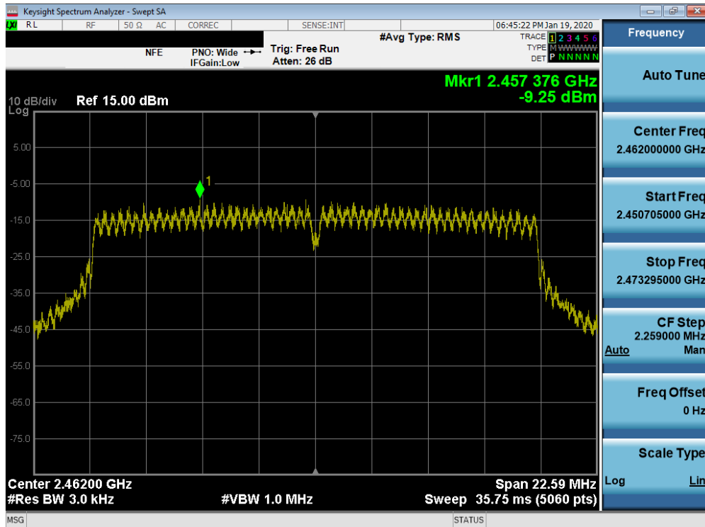
Plot 7-39. Power Spectral Density Plot SISO ANT1 (802.11n (2.4GHz) – Ch. 11)
