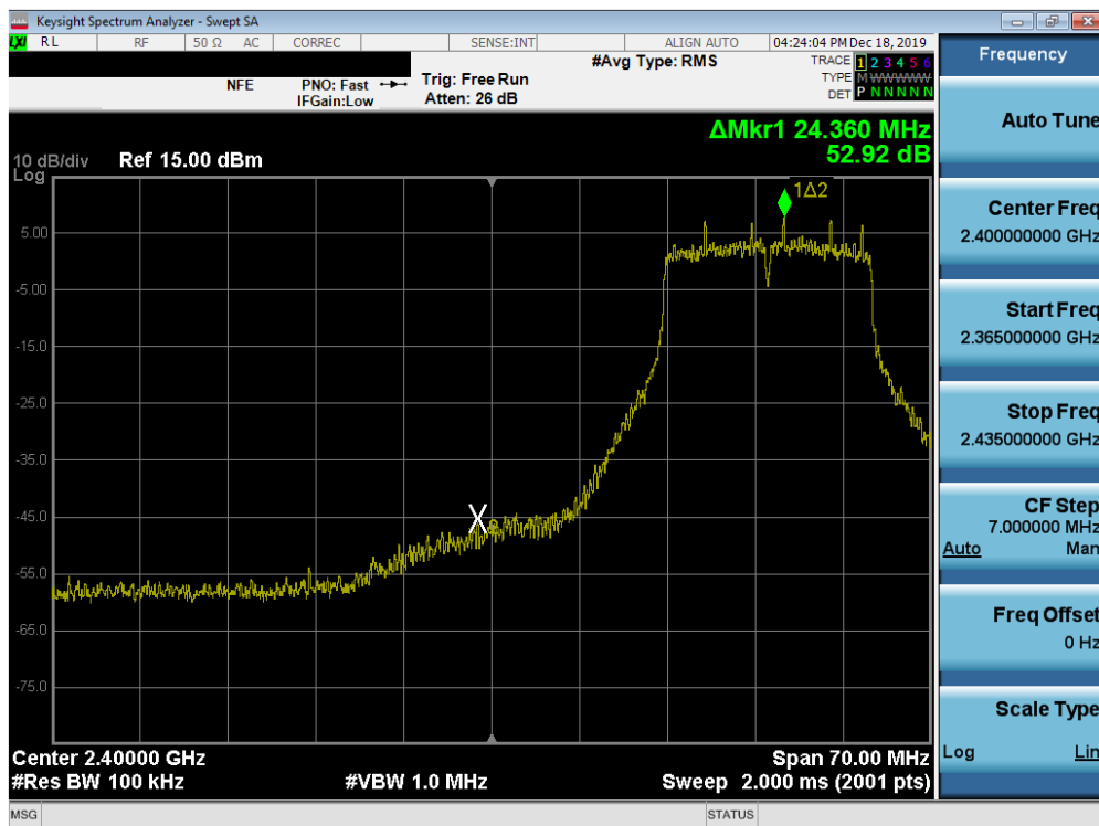
Plot 7-64. Band Edge Plot SISO ANT1 (802.11g- Ch. 3)
