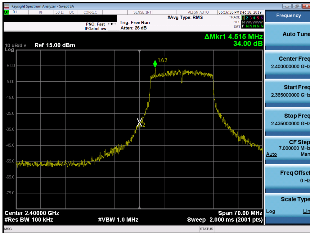
Plot 7-71. Band Edge Plot SISO ANT1 (802.11ac (2.4GHz) – Ch. 1)
