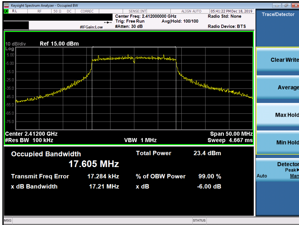
Plot 7-28. 6dB Bandwidth Plot SISO ANT2 (802.11ax (2.4GHz) – Ch. 1)
