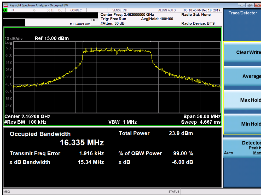
Plot 7-21. 6dB Bandwidth Plot SISO ANT2 (802.11g – Ch. 11)
