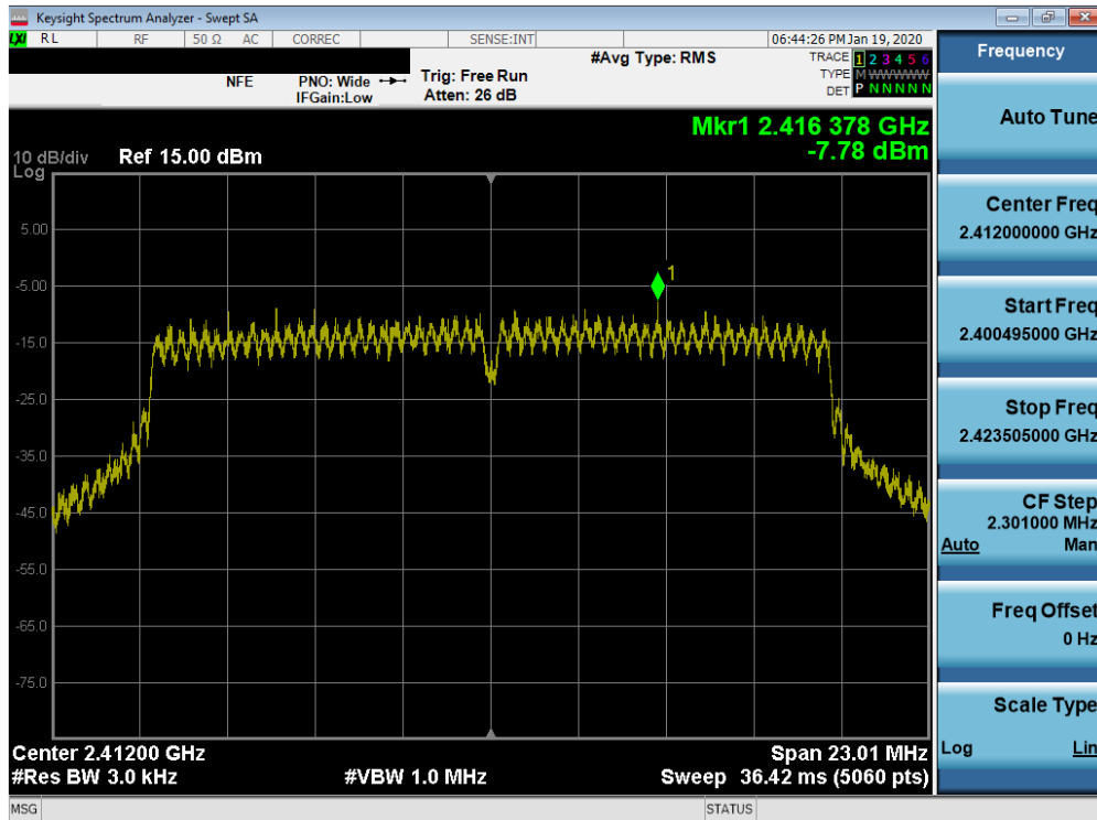
Plot 7-37. Power Spectral Density Plot SISO ANT1 (802.11n (2.4GHz) – Ch. 1)
