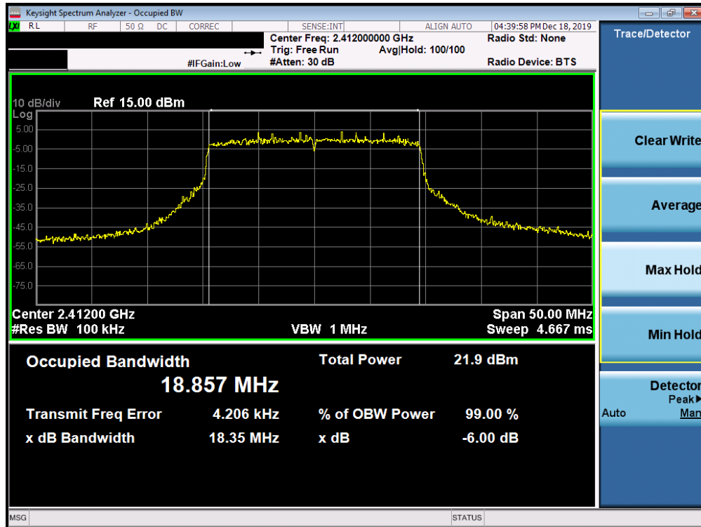
Plot 7-13. 6dB Bandwidth Plot SISO ANT1 (802.11ax (2.4GHz) – Ch. 1)
