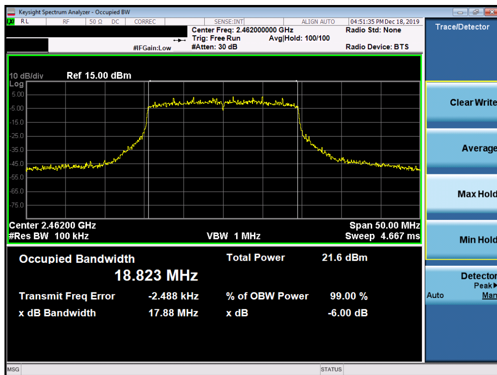
Plot 7-15. 6dB Bandwidth Plot SISO ANT1 (802.11ax (2.4GHz) – Ch. 11)
