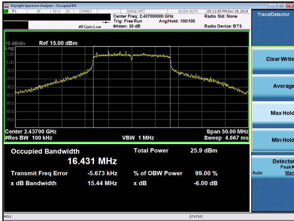
Plot 7-20. 6dB Bandwidth Plot SISO ANT2 (802.11g – Ch. 6)
