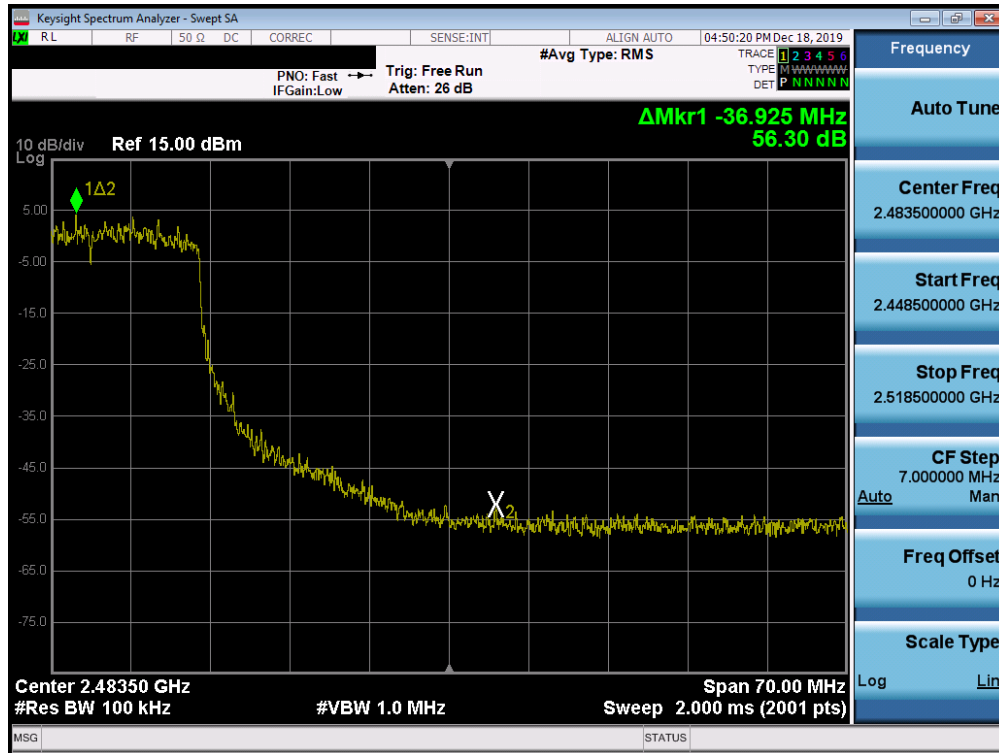
Plot 7-77. Band Edge Plot SISO ANT1 (802.11ax - Ch. 9)
