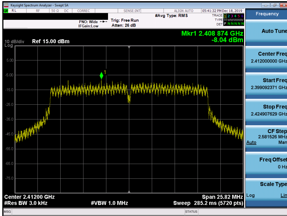
Plot 7-58. Power Spectral Density Plot SISO ANT2 (802.11ax (2.4GHz) - Ch. 1)
