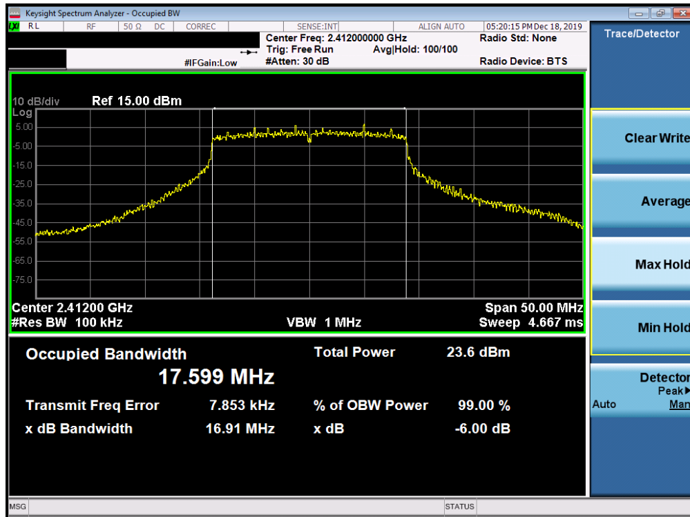
Plot 7-22. 6dB Bandwidth Plot SISO ANT2 (802.11n (2.4GHz) – Ch. 1)
