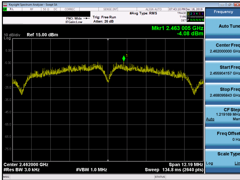
Plot 7-33. Power Spectral Density Plot SISO ANT1 (802.11b – Ch. 11)
