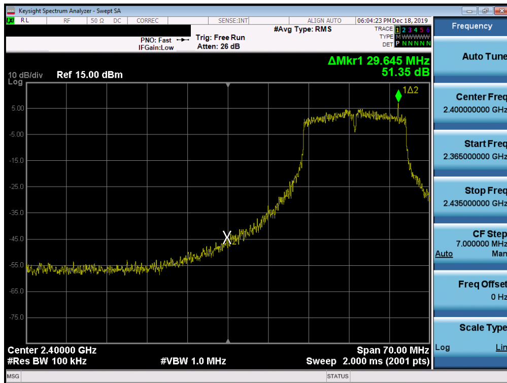
Plot 7-90. Band Edge Plot SISO ANT2 (802.11ac – Ch. 3)
