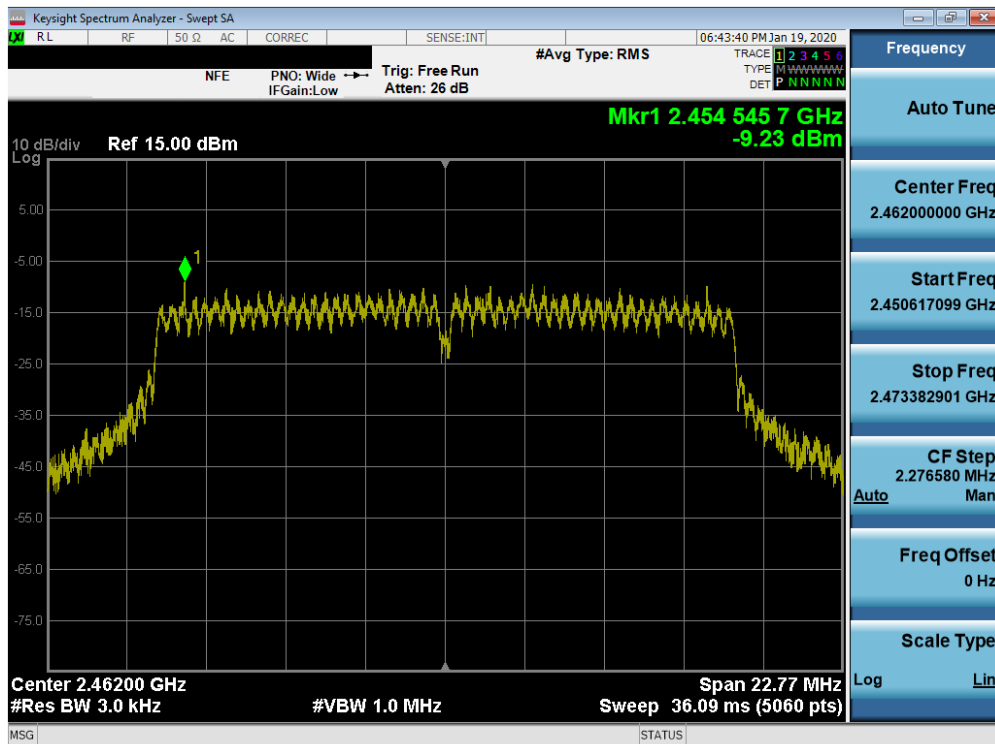
Plot 7-36. Power Spectral Density Plot SISO ANT1 (802.11g – Ch. 11)
