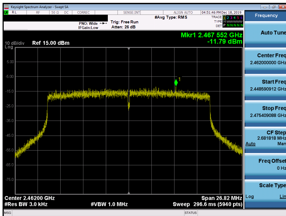
Plot 7-45. Power Spectral Density Plot SISO ANT1 (802.11ax (2.4GHz) – Ch. 11)
