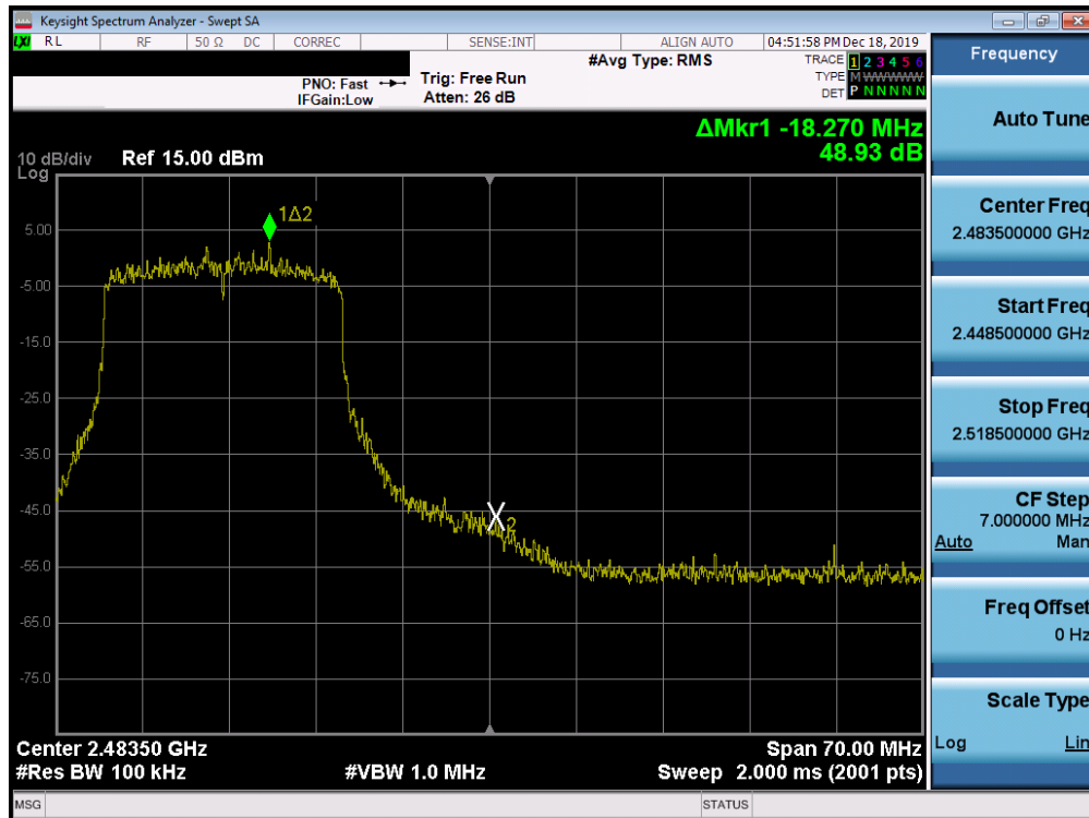
Plot 7-78. Band Edge Plot SISO ANT1 (802.11ax (2.4GHz) - Ch. 11)
