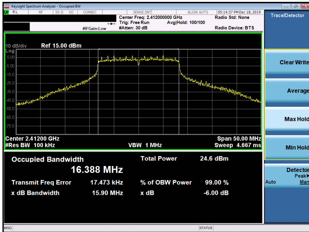
Plot 7-19. 6dB Bandwidth Plot SISO ANT2 (802.11g – Ch. 1)
