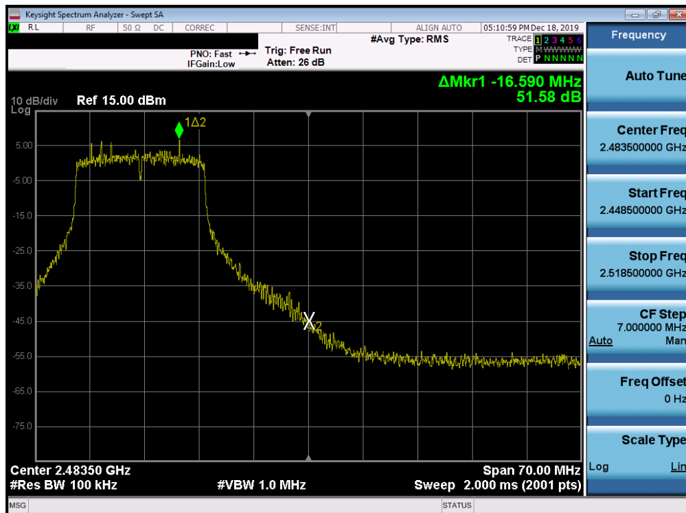
Plot 7-84. Band Edge Plot SISO ANT2 (802.11g - Ch. 11)
