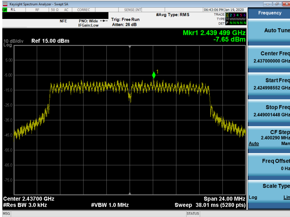
Plot 7-35. Power Spectral Density Plot SISO ANT1 (802.11g – Ch. 6)
