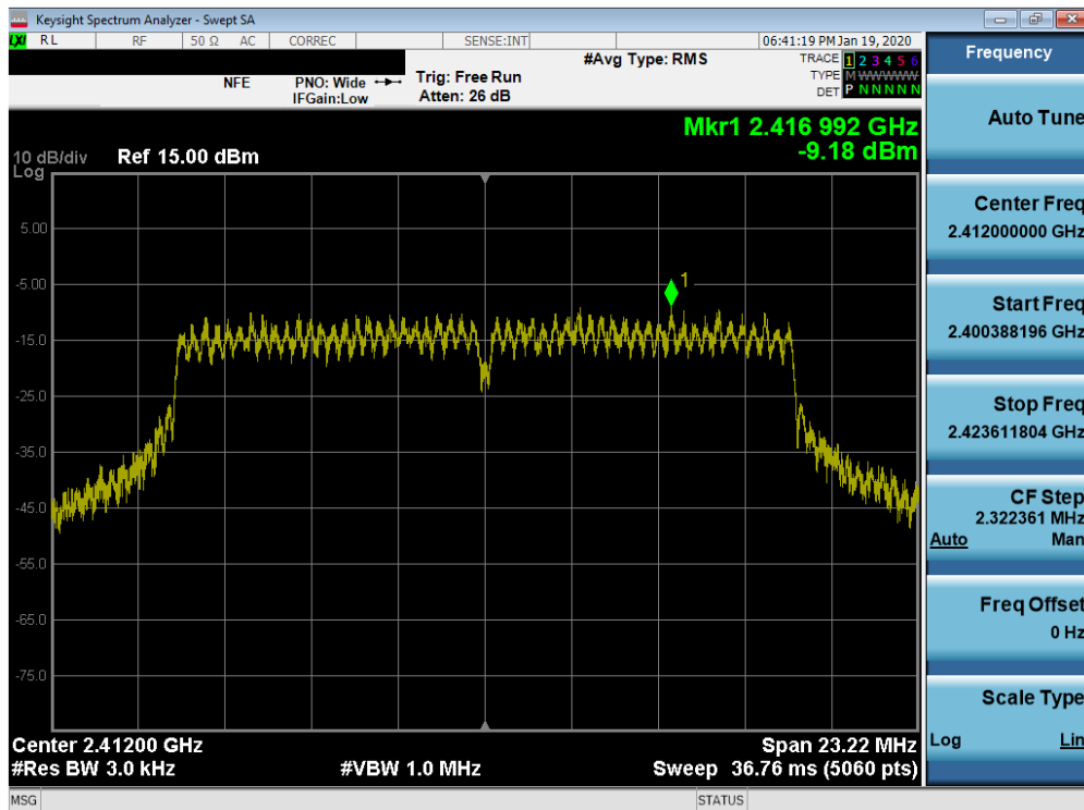
Plot 7-34. Power Spectral Density Plot SISO ANT1 (802.11g – Ch. 1)
