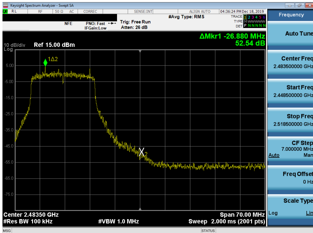
Plot 7-70. Band Edge Plot SISO ANT1 (802.11n (2.4GHz) – Ch. 11)
