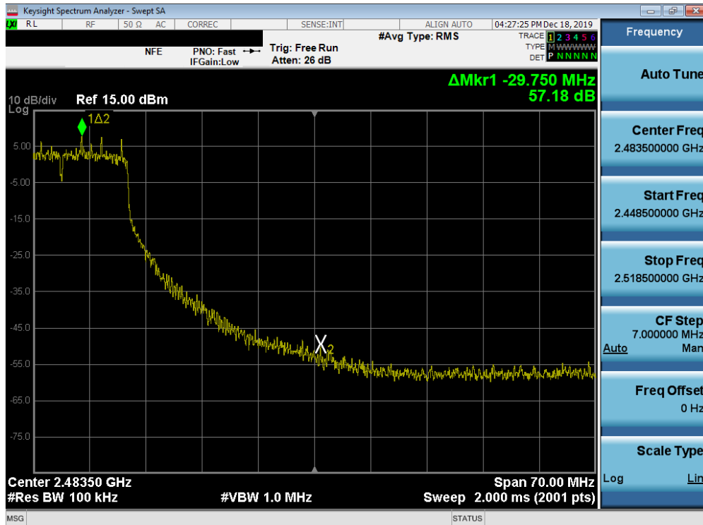
Plot 7-65. Band Edge Plot SISO ANT1 (802.11g - Ch. 9)
