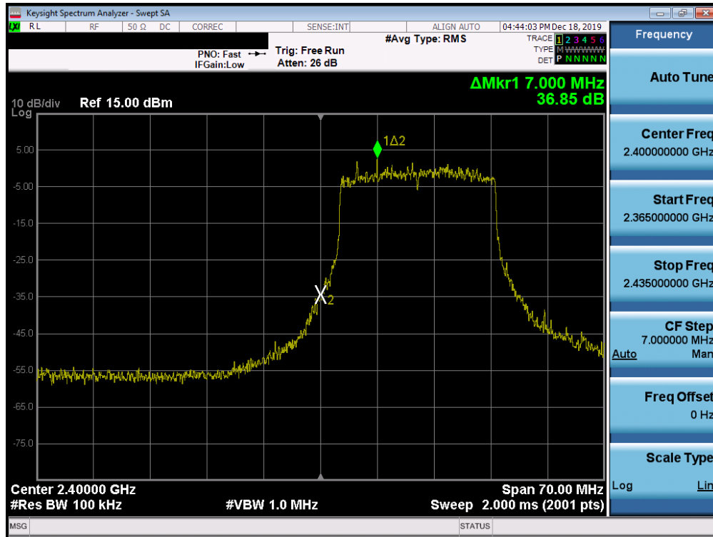
Plot 7-75. Band Edge Plot SISO ANT1 (802.11ax (2.4GHz) – Ch. 1)
