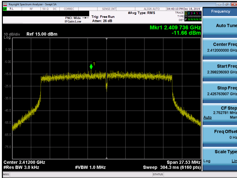
Plot 7-43. Power Spectral Density Plot SISO ANT1 (802.11ax (2.4GHz) – Ch. 1)
