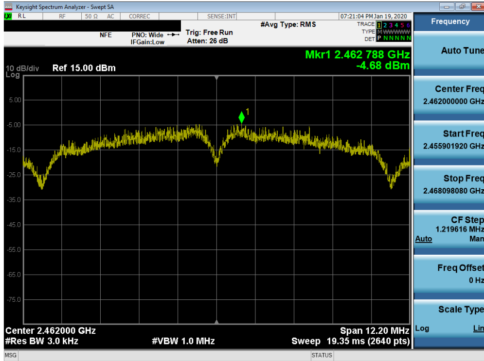
Plot 7-48. Power Spectral Density Plot SISO ANT2 (802.11b – Ch. 11)
