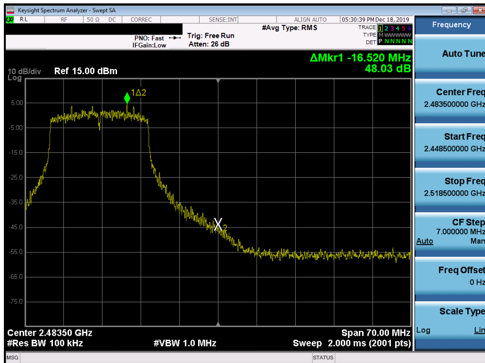
Plot 7-88. Band Edge Plot SISO ANT2 (802.11n (2.4GHz) - Ch. 11)
