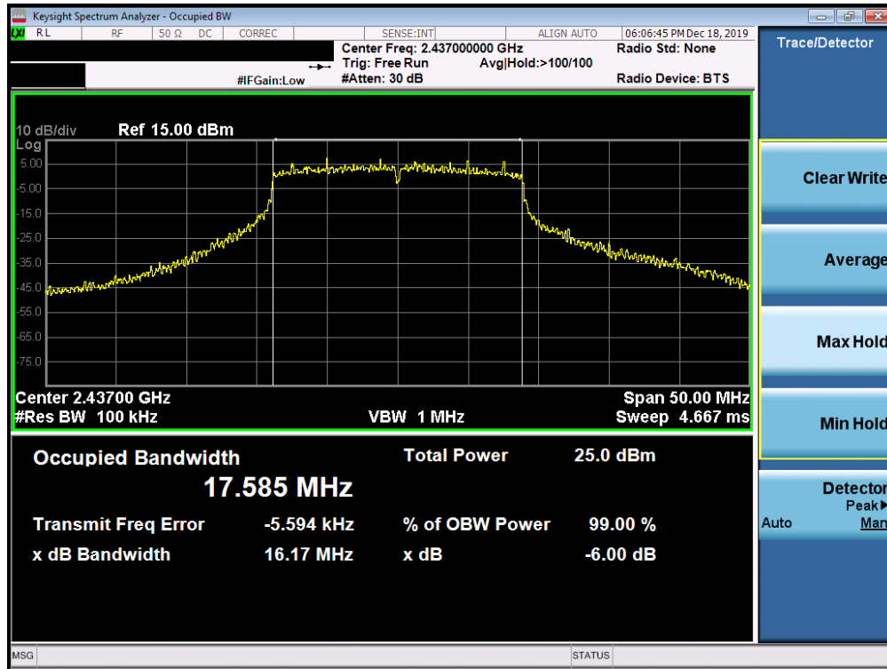
Plot 7-26. 6dB Bandwidth Plot SISO ANT2 (802.11ac (2.4GHz) – Ch. 6)
