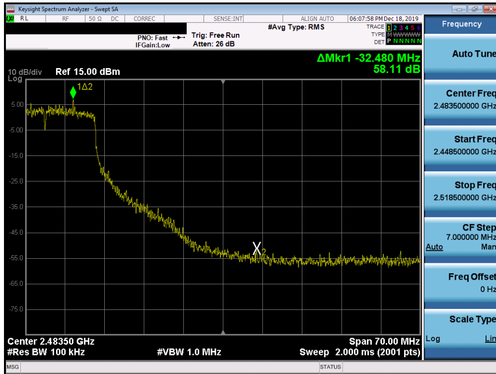
Plot 7-91. Band Edge Plot SISO ANT2 (802.11ac - Ch. 9)
