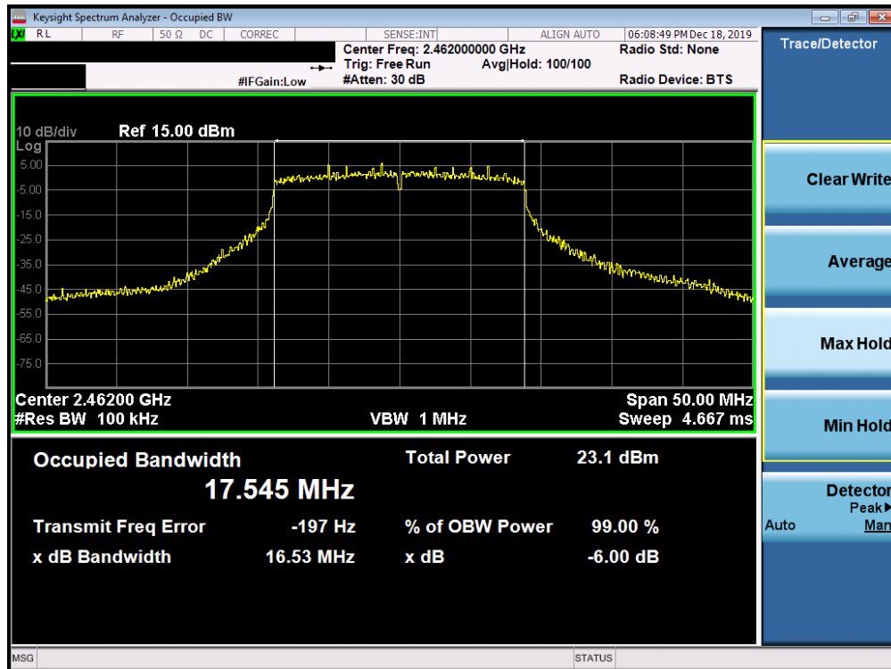
Plot 7-27. 6dB Bandwidth Plot SISO ANT2 (802.11ac (2.4GHz) – Ch. 11)
