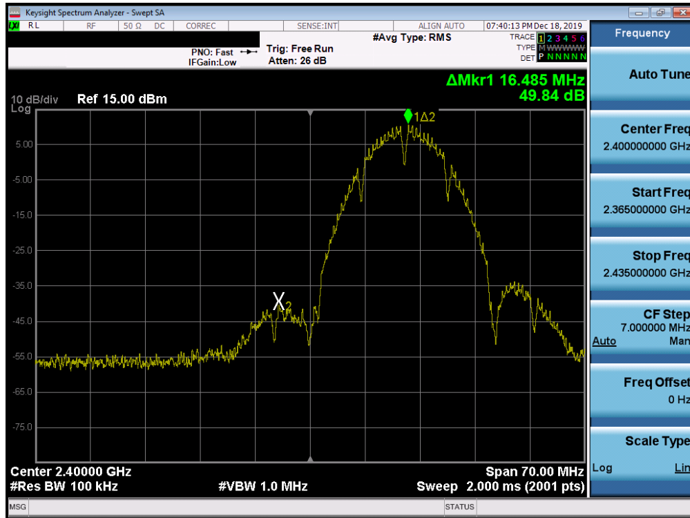
Plot 7-61. Band Edge Plot SISO ANT1 (802.11b – Ch. 1)
