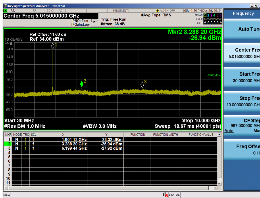
LTE Band 2 / 15MHz / 64QAM - RB Size/Offset (36/18) – High Channel
