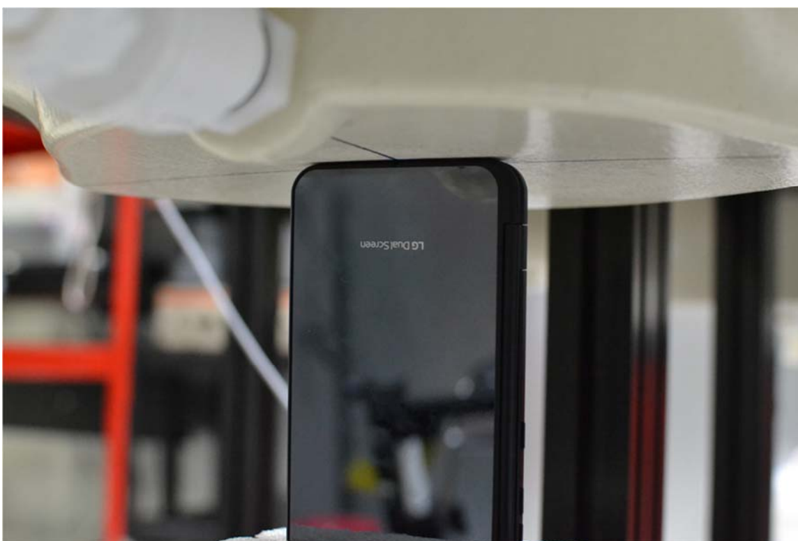
SAR Test Setup Photo 24 – Bottom Side at 0 mm with Dual Display Cover Position #1 (0 degrees)
