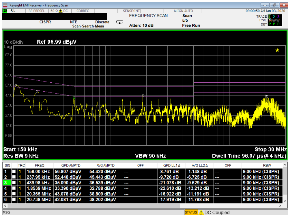
Plot 7-7. Line-Conducted Test Plot (N) with Antenna Terminated at 50Ω
