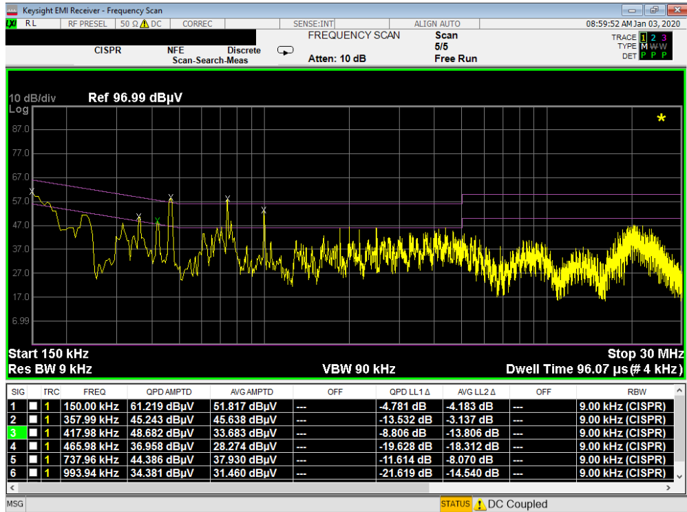
Plot 7-6. Line-Conducted Test Plot (L1) with Antenna Terminated at 50Ω
