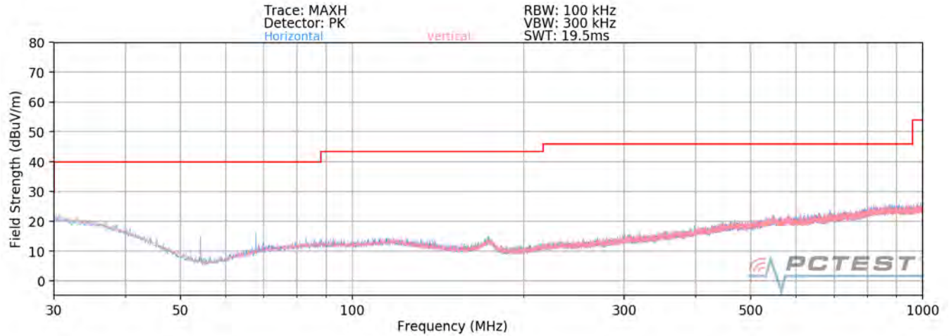
Plot 7-140. Radiated Spurious Plot below 1GHz SISO ANT2
