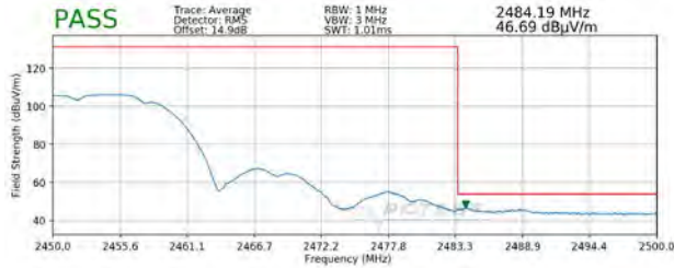
Plot 7-111. Radiated Restricted Upper Band Edge Measurement SISO ANT1 (Average)
