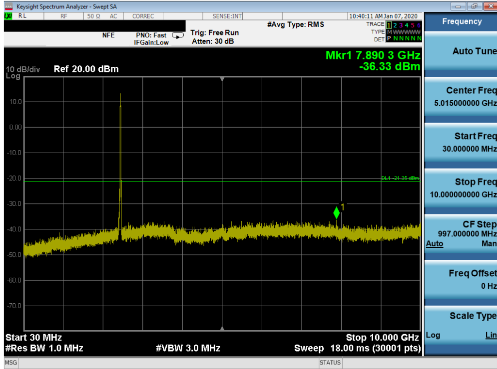
Plot 7-93. Conducted Spurious Plot SISO ANT2 (802.11b – Ch. 11)
