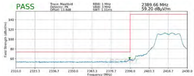
Plot 7-130. Radiated Restricted Lower Band Edge Measurement MIMO/CDD (Peak)
