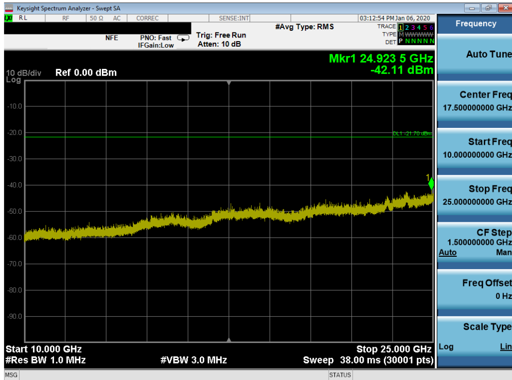
Plot 7-86. Conducted Spurious Plot SISO ANT1 (802.11b – Ch. 6)
