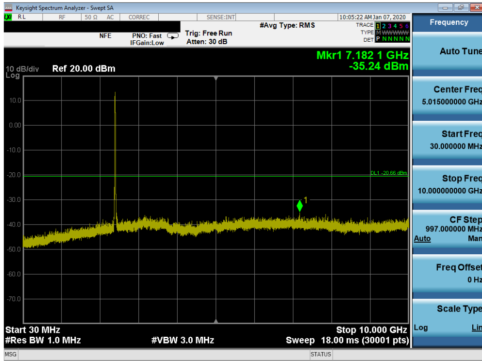
Plot 7-89. Conducted Spurious Plot SISO ANT2 (802.11b – Ch. 1)
