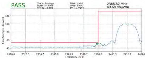
Plot 7-119. Radiated Restricted Lower Band Edge Measurement SISO ANT2 (Average)
