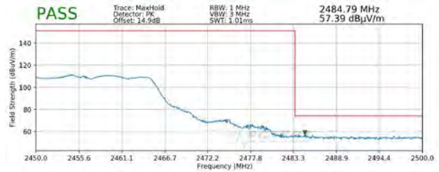
Plot 7-134. Radiated Restricted Upper Band Edge Measurement MIMO/CDD (Peak)
