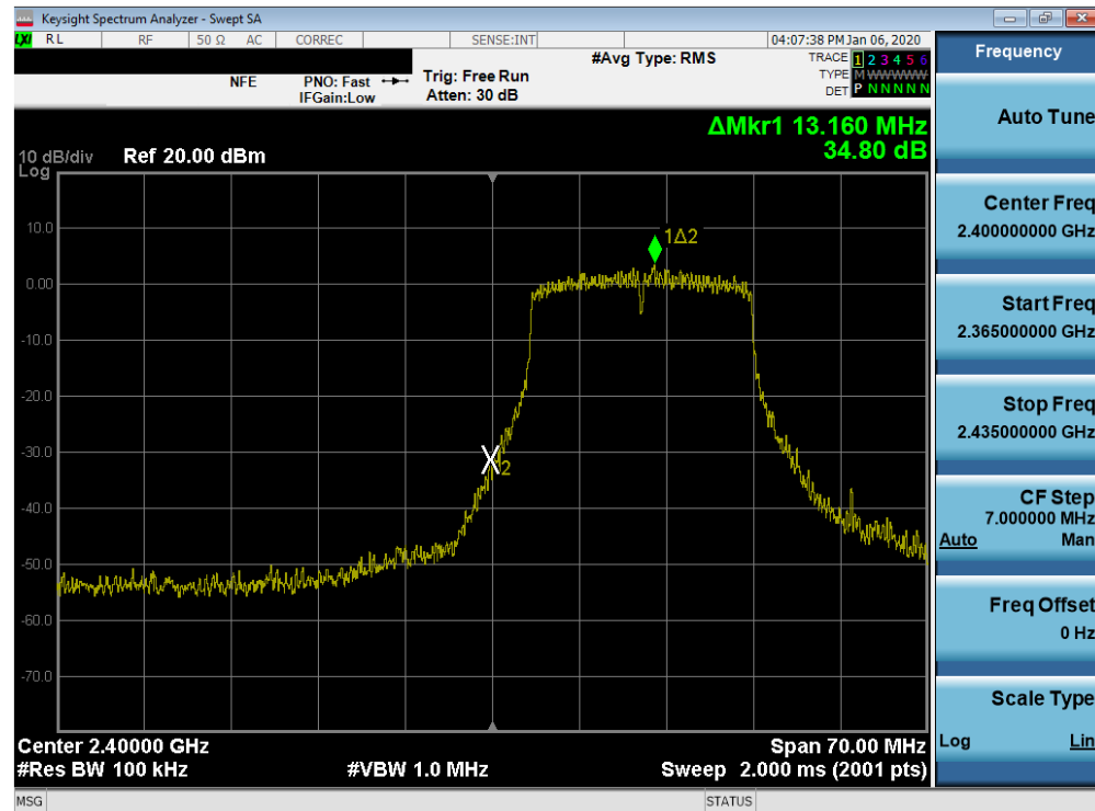
Plot 7-56. Band Edge Plot SISO ANT1 (802.11n (2.4GHz) - Ch. 1)
