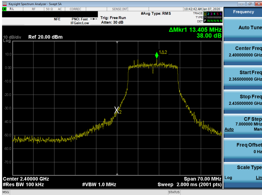
Plot 7-68. Band Edge Plot SISO ANT2 (802.11g- Ch. 1)
