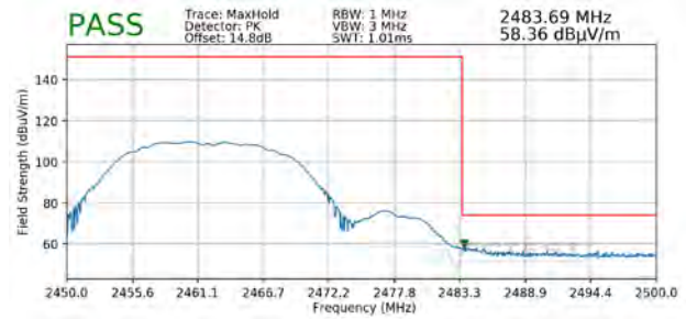
Plot 7-116. Radiated Restricted Upper Band Edge Measurement SISO ANT1 (Peak)
