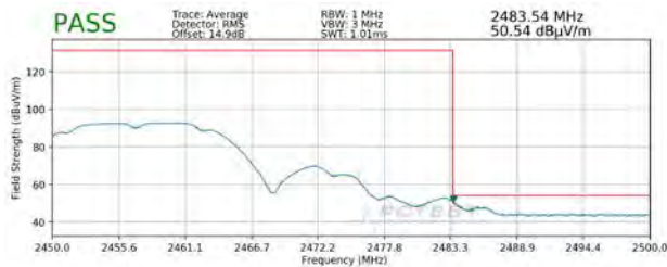
Plot 7-123. Radiated Restricted Upper Band Edge Measurement SISO ANT2 (Average)
