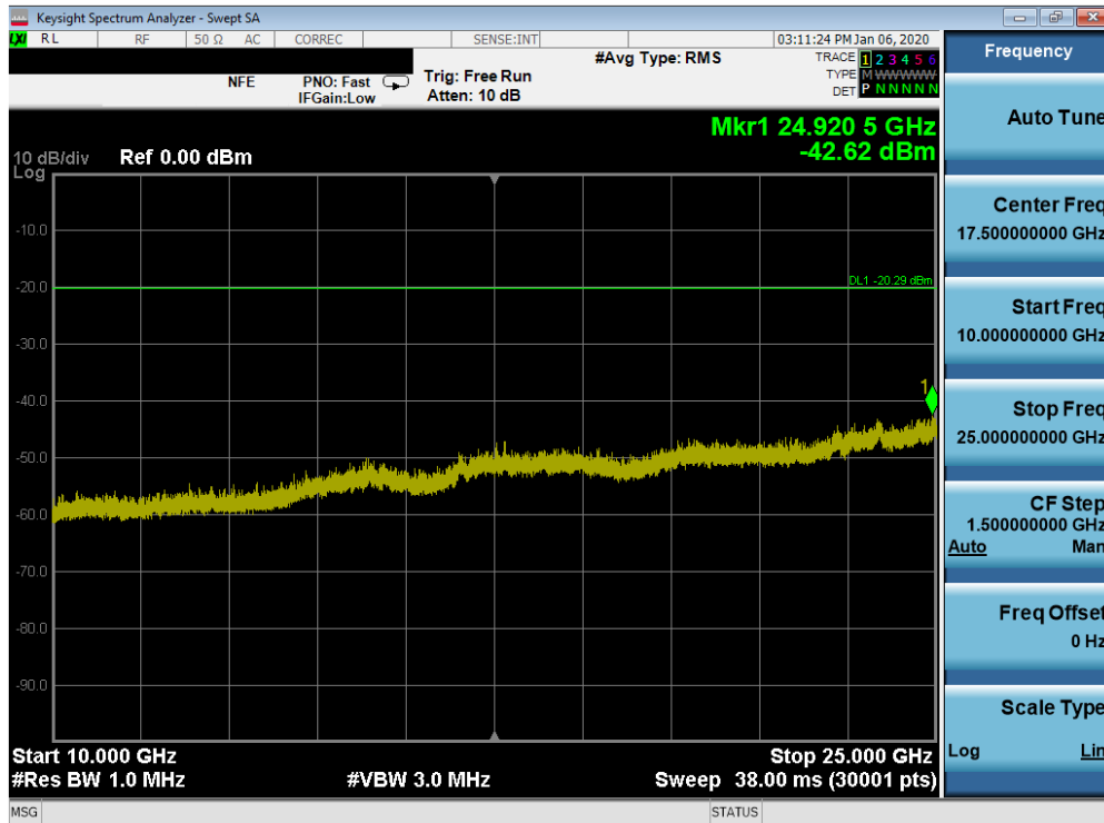
Plot 7-84. Conducted Spurious Plot SISO ANT1 (802.11b – Ch. 1)
