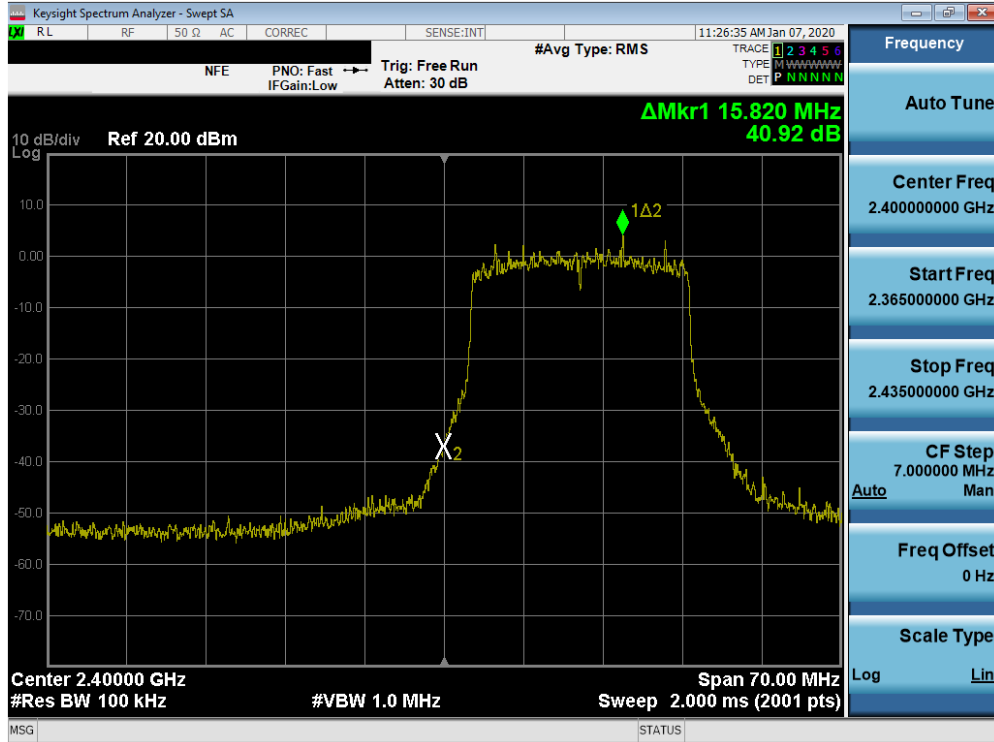
Plot 7-78. Band Edge Plot SISO ANT2 (802.11ax (2.4GHz) – Ch. 1)
