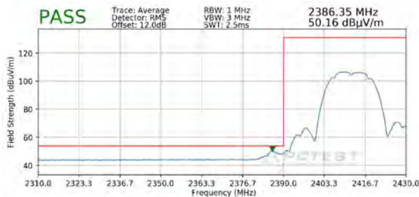
Plot 7-107. Radiated Restricted Lower Band Edge Measurement SISO ANT1 (Average)
