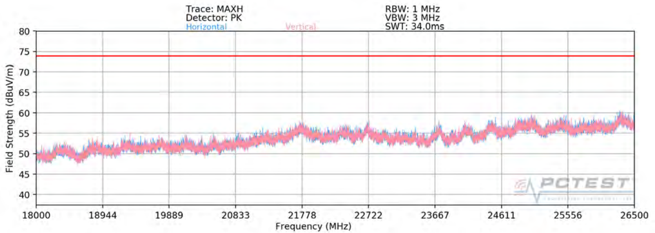
Plot 7-106. Radiated Spurious Plot above 18GHz MIMO/CDD
