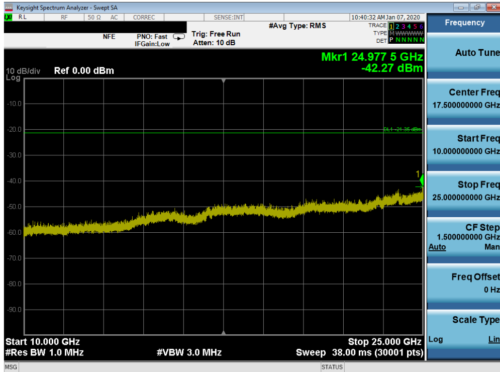
Plot 7-94. Conducted Spurious Plot SISO ANT2 (802.11b – Ch. 11)
