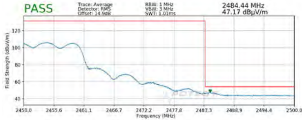
Plot 7-131. Radiated Restricted Upper Band Edge Measurement MIMO/CDD (Average)
