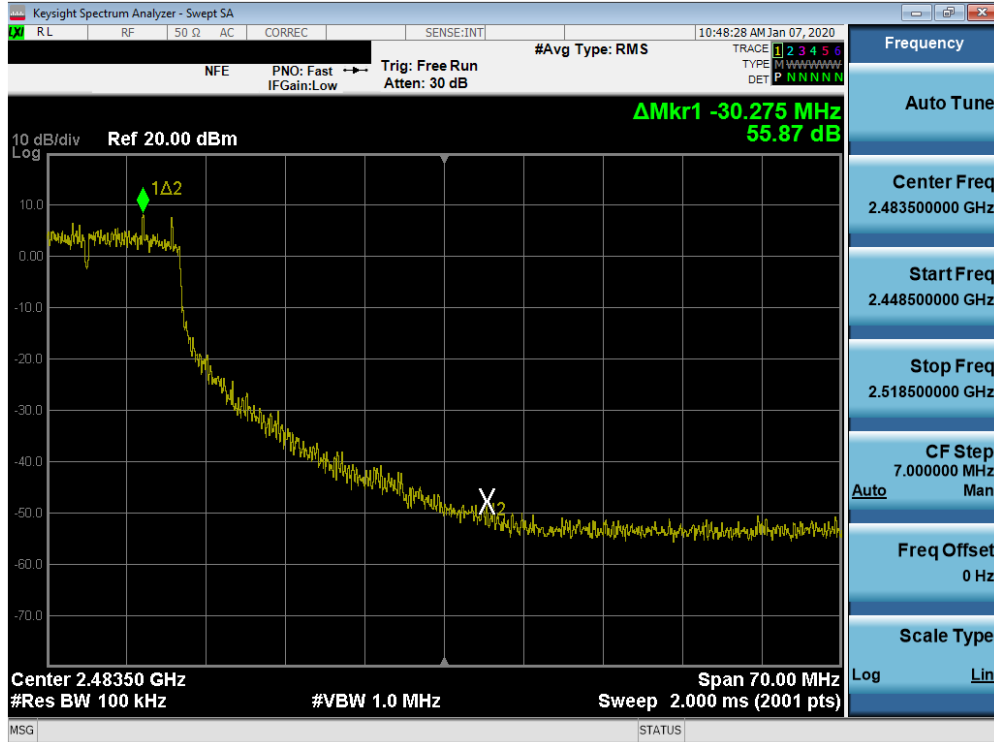
Plot 7-70. Band Edge Plot SISO ANT2 (802.11g – Ch. 9)
