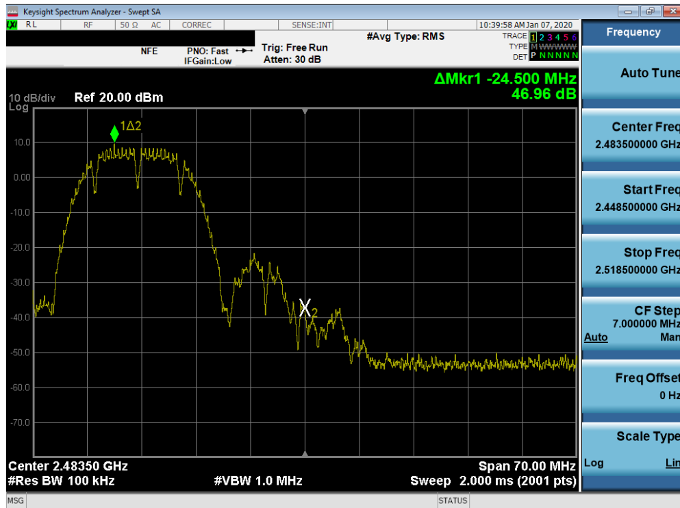
Plot 7-67. Band Edge Plot SISO ANT2 (802.11b - Ch. 11)
