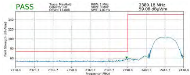
Plot 7-120. Radiated Restricted Lower Band Edge Measurement SISO ANT2 (Peak)
