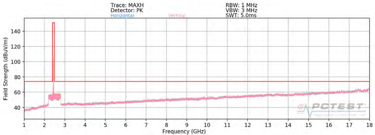
Plot 7-96. Radiated Spurious Plot above 1GHz SISO ANT1 (802.11b – Ch. 6)
