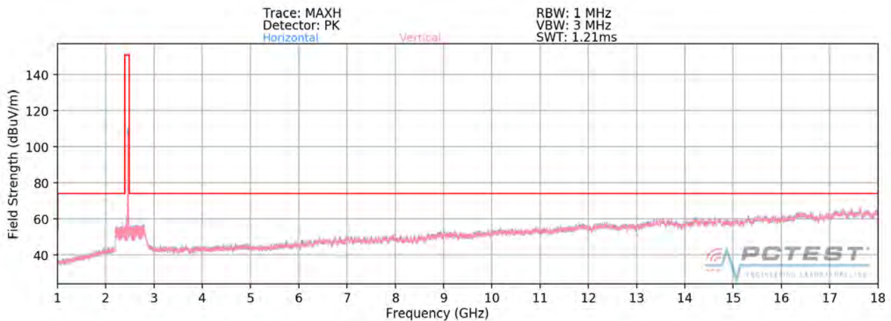
Plot 7-97. Radiated Spurious Plot above 1GHz SISO ANT1 (802.11b – Ch. 11)
