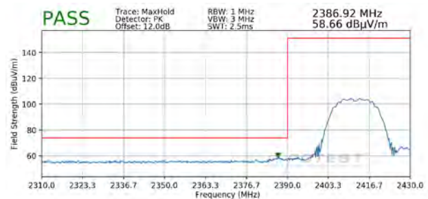
Plot 7-118. Radiated Restricted Lower Band Edge Measurement SISO ANT2 (Peak)
