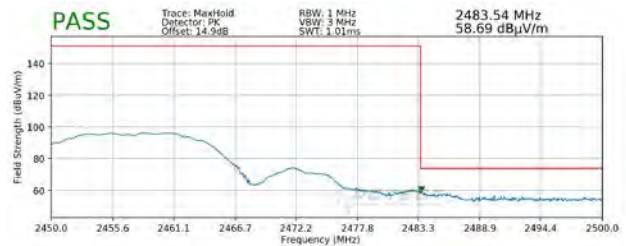
Plot 7-124. Radiated Restricted Upper Band Edge Measurement SISO ANT2 (Peak)
