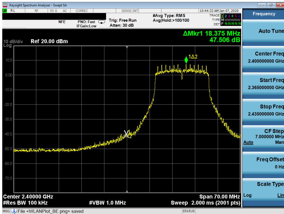
Plot 7-69. Band Edge Plot SISO ANT2 (802.11g - Ch. 2)
