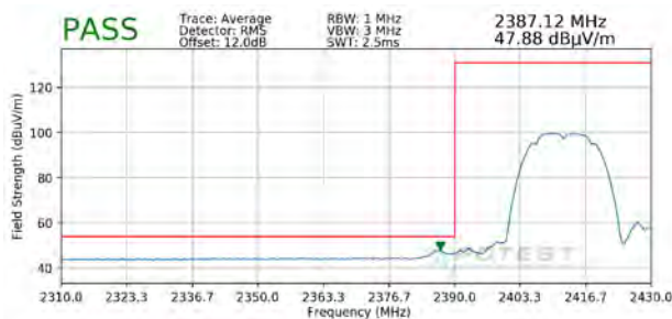
Plot 7-117. Radiated Restricted Lower Band Edge Measurement SISO ANT2 (Average)
