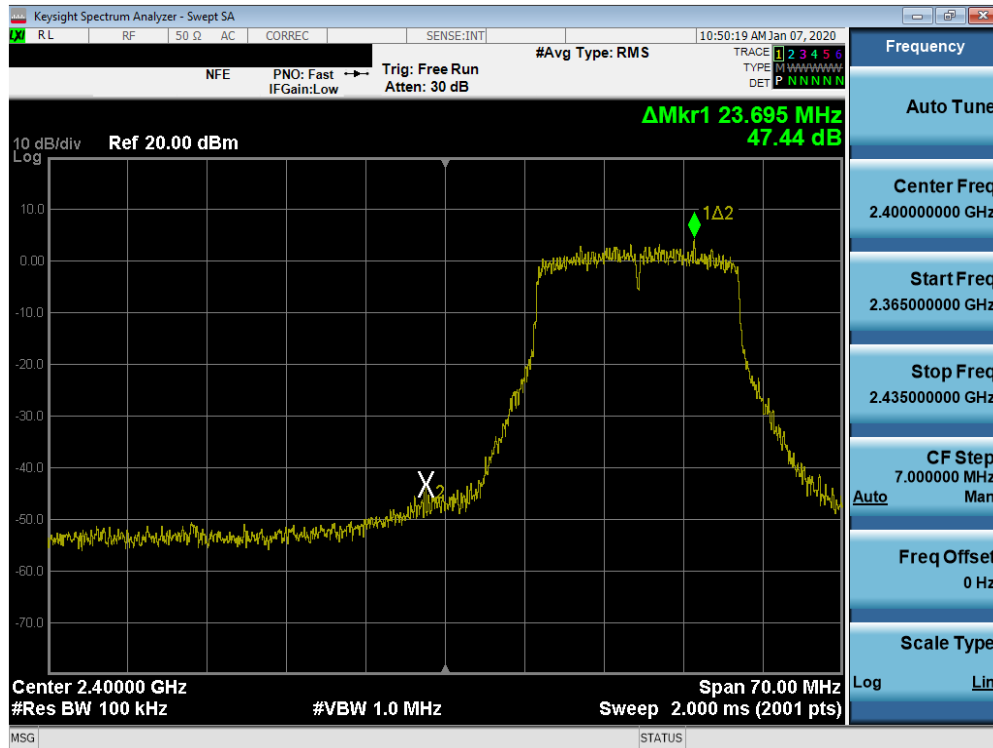
Plot 7-74. Band Edge Plot SISO ANT2 (802.11n – Ch. 2)
