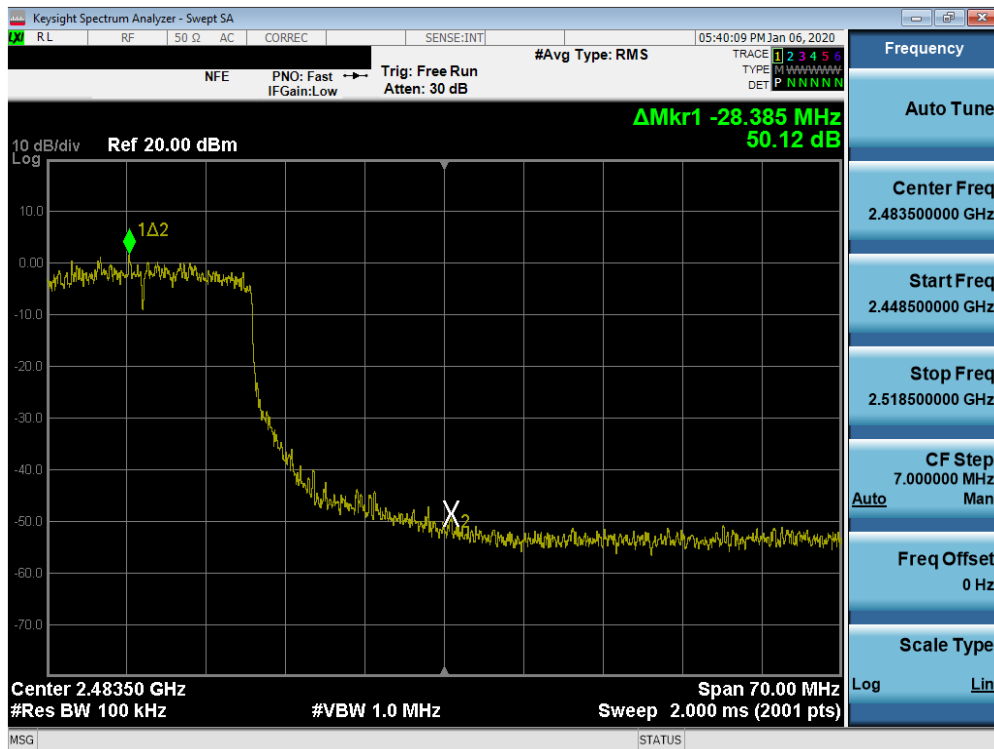
Plot 7-64. Band Edge Plot SISO ANT1 (802.11ax (2.4GHz) – Ch. 10)
