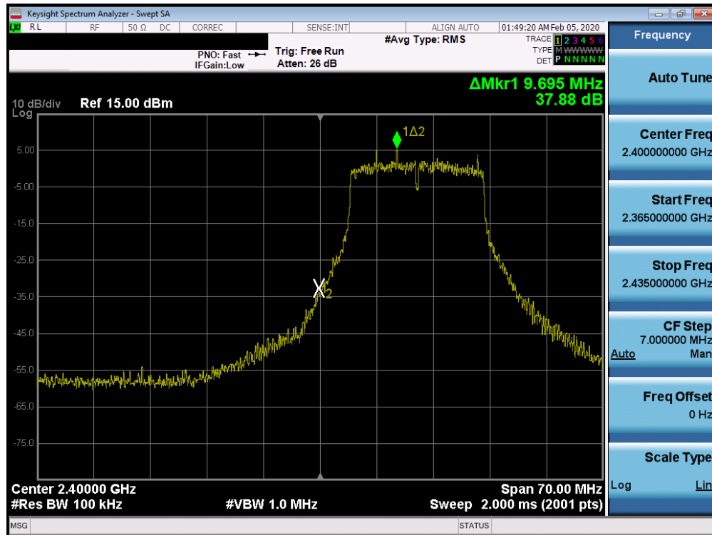
Plot 7-51. Band Edge Plot SISO ANT1 (802.11g- Ch. 1)
