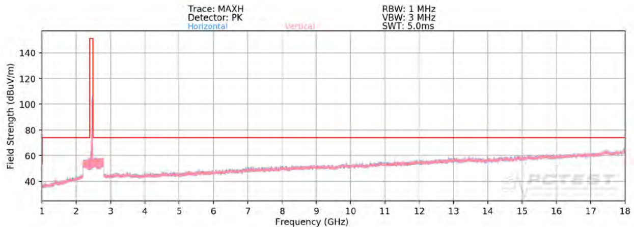
Plot 7-101. Radiated Spurious Plot above 1GHz SISO ANT2 (802.11b – Ch. 11)
