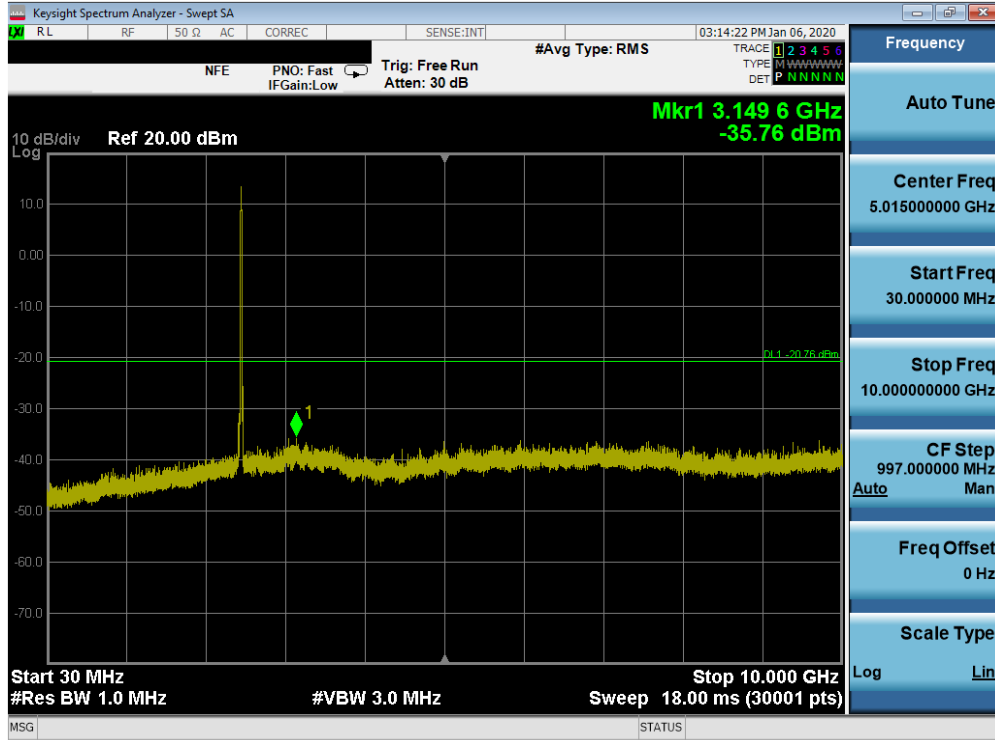
Plot 7-87. Conducted Spurious Plot SISO ANT1 (802.11b – Ch. 11)
