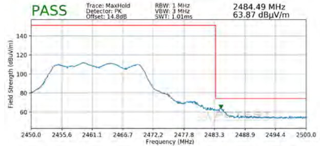
Plot 7-136. Radiated Restricted Upper Band Edge Measurement MIMO/CDD (Peak)
