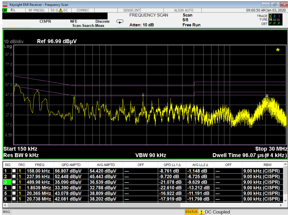
Plot 7-142. Line Conducted Plot with 802.11b (N)
