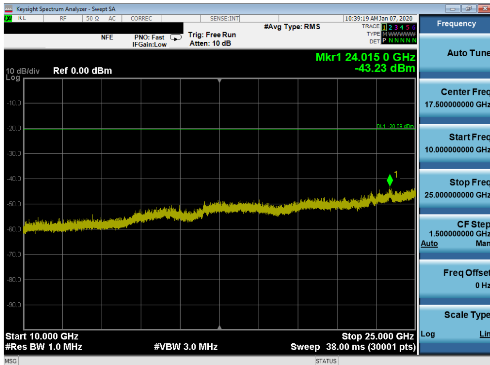
Plot 7-92. Conducted Spurious Plot SISO ANT2 (802.11b – Ch. 6)
