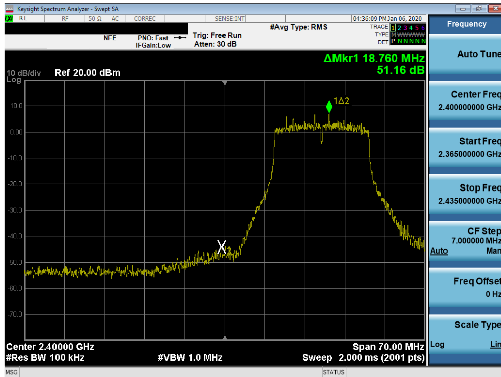
Plot 7-52. Band Edge Plot SISO ANT1 (802.11g- Ch. 2)
