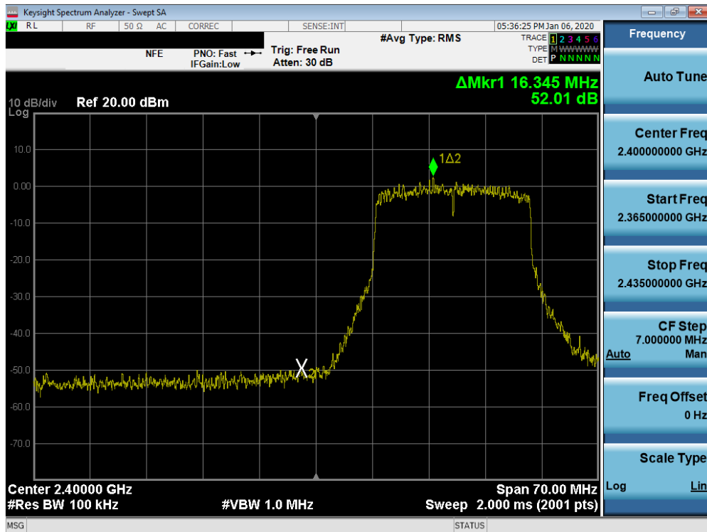
Plot 7-62. Band Edge Plot SISO ANT1 (802.11ax (2.4GHz) – Ch. 2)
