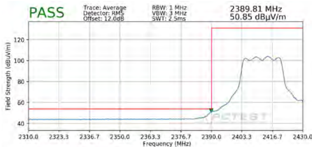
Plot 7-127. Radiated Restricted Lower Band Edge Measurement MIMO/CDD (Average)
