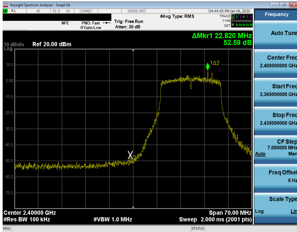
Plot 7-57. Band Edge Plot SISO ANT1 (802.11n (2.4GHz) – Ch. 2)
