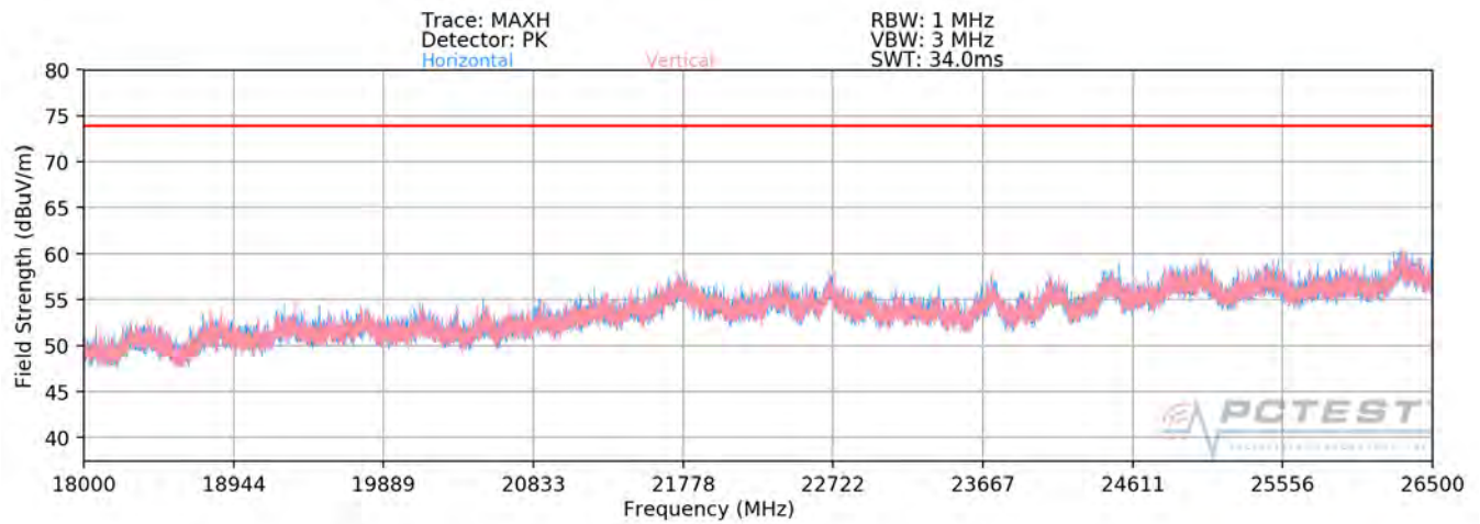
Plot 7-102. Radiated Spurious Plot above 18GHz SISO ANT2
