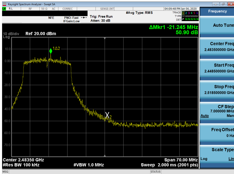
Plot 7-60. Band Edge Plot SISO ANT1 (802.11n (2.4GHz) – Ch. 11)
