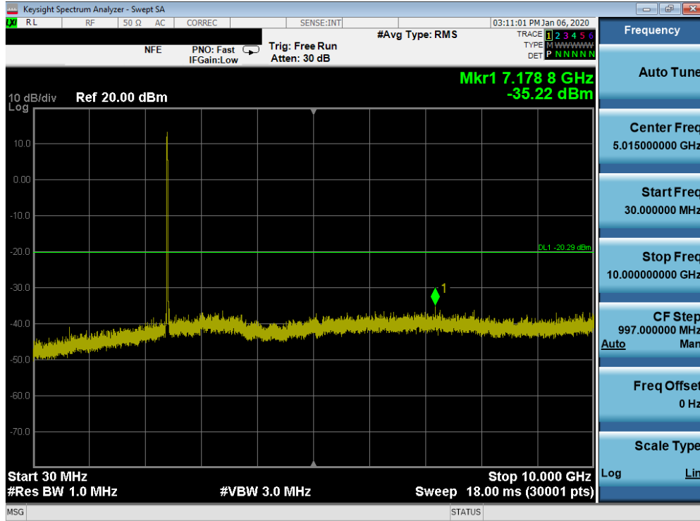
Plot 7-83. Conducted Spurious Plot SISO ANT1 (802.11b – Ch. 1)
