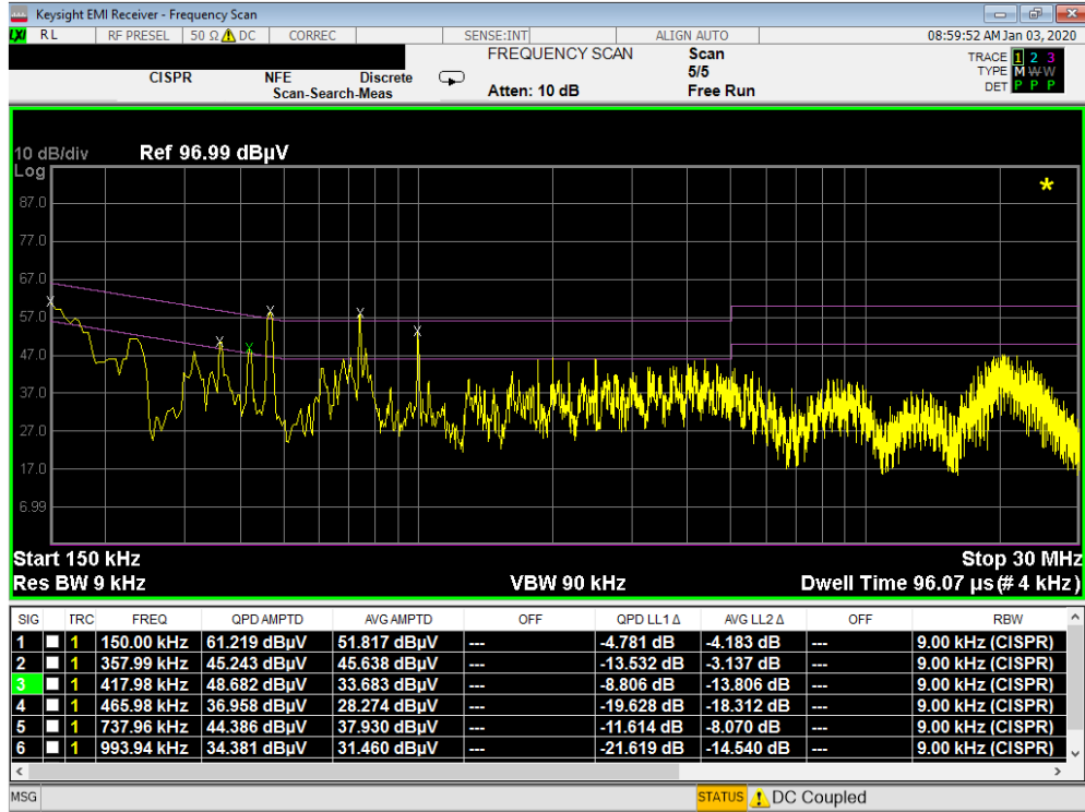
Plot 7-141. Line Conducted Plot with 802.11b (L1)
