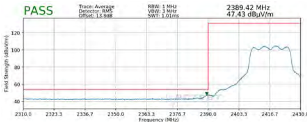
Plot 7-129. Radiated Restricted Lower Band Edge Measurement MIMO/CDD (Average)
