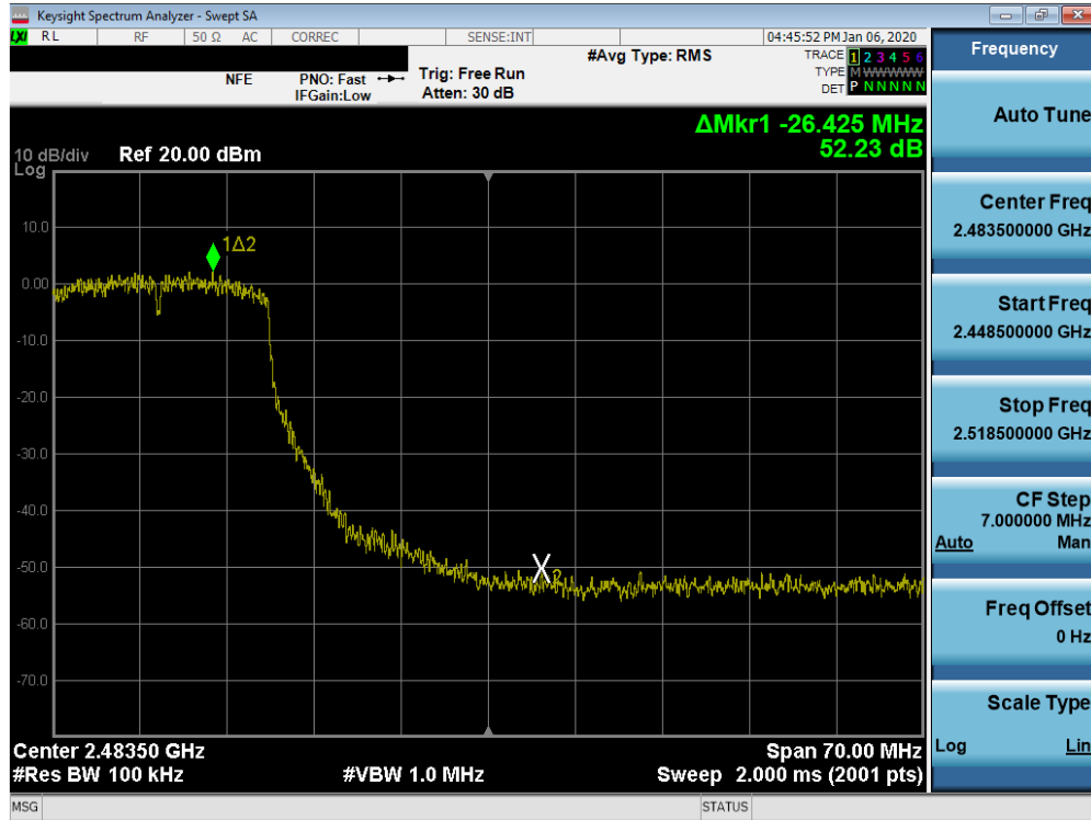
Plot 7-59. Band Edge Plot SISO ANT1 (802.11n (2.4GHz) – Ch. 10)
