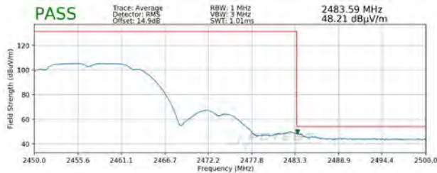
Plot 7-113. Radiated Restricted Upper Band Edge Measurement SISO ANT1 (Average)
