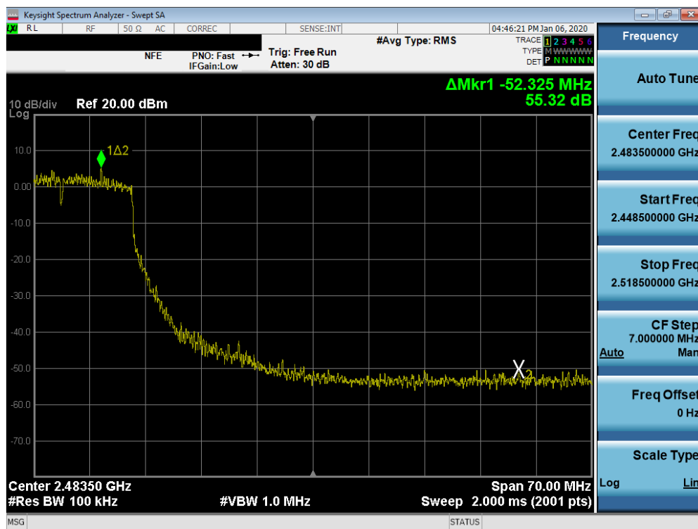
Plot 7-58. Band Edge Plot SISO ANT1 (802.11n (2.4GHz) – Ch. 9)
