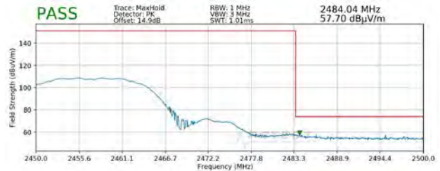
Plot 7-114. Radiated Restricted Upper Band Edge Measurement SISO ANT1 (Peak)
