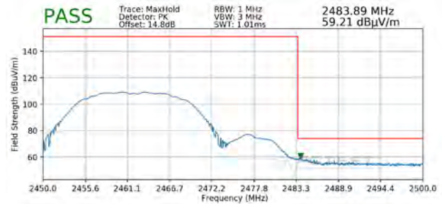
Plot 7-126. Radiated Restricted Upper Band Edge Measurement SISO ANT2 (Peak)
