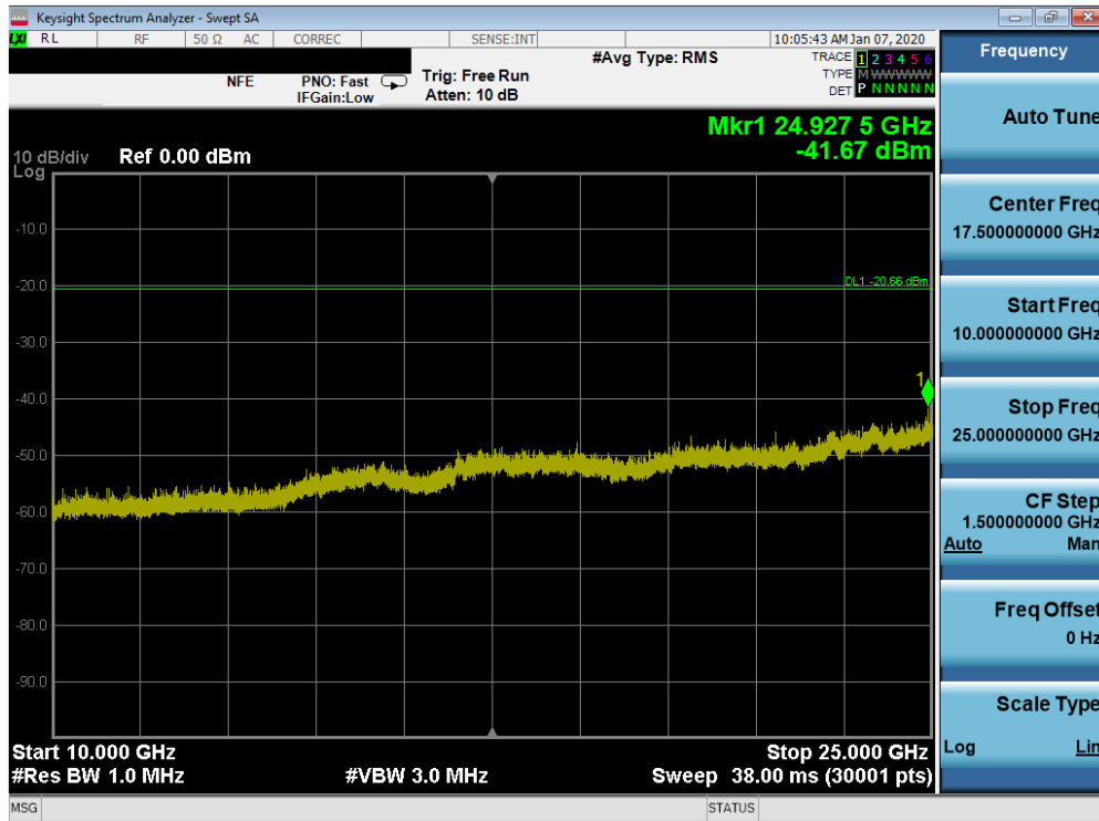
Plot 7-90. Conducted Spurious Plot SISO ANT2 (802.11b – Ch. 1)
