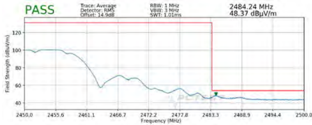
Plot 7-121. Radiated Restricted Upper Band Edge Measurement SISO ANT2 (Average)
