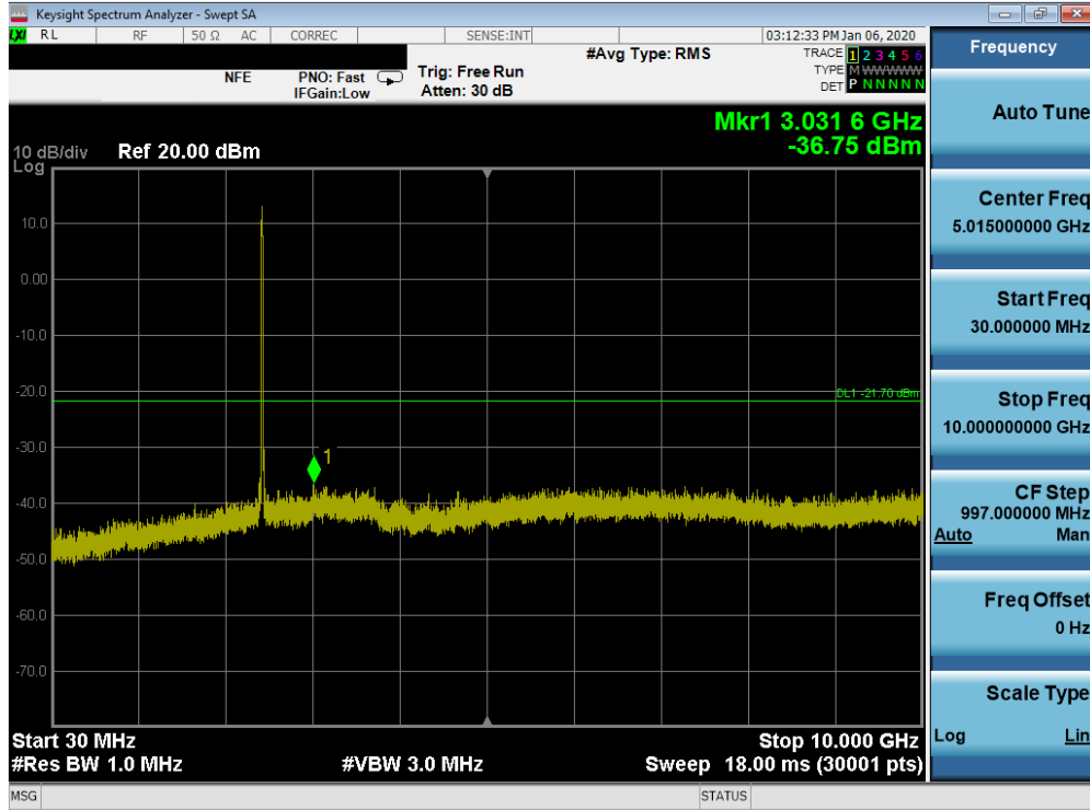
Plot 7-85. Conducted Spurious Plot SISO ANT1 (802.11b – Ch. 6)
