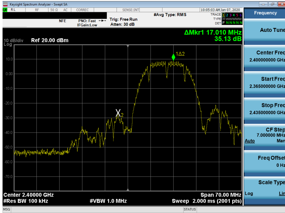
Plot 7-66. Band Edge Plot SISO ANT2 (802.11b - Ch. 1)
