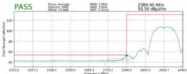
Plot 7-109. Radiated Restricted Lower Band Edge Measurement SISO ANT1 (Average)
