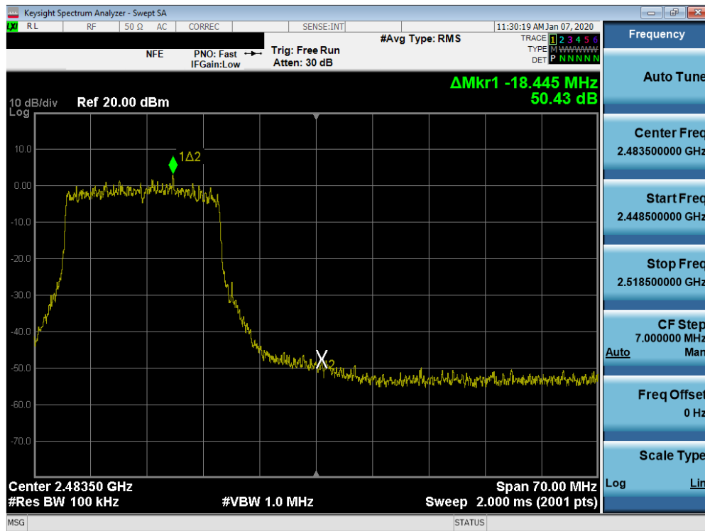
Plot 7-82. Band Edge Plot SISO ANT2 (802.11ax (2.4GHz) – Ch. 11)
