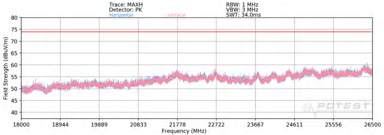
Plot 7-98. Radiated Spurious Plot above 18GHz SISO ANT1
