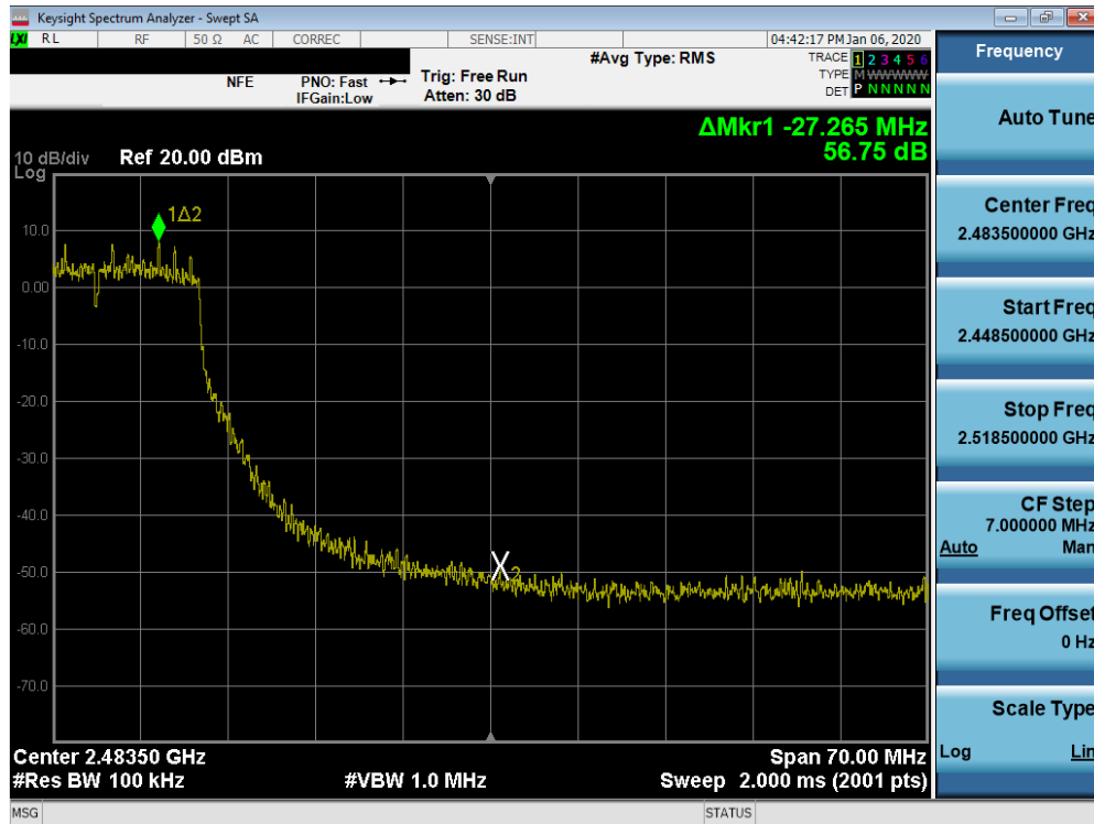
Plot 7-53. Band Edge Plot SISO ANT1 (802.11g – Ch. 9)
