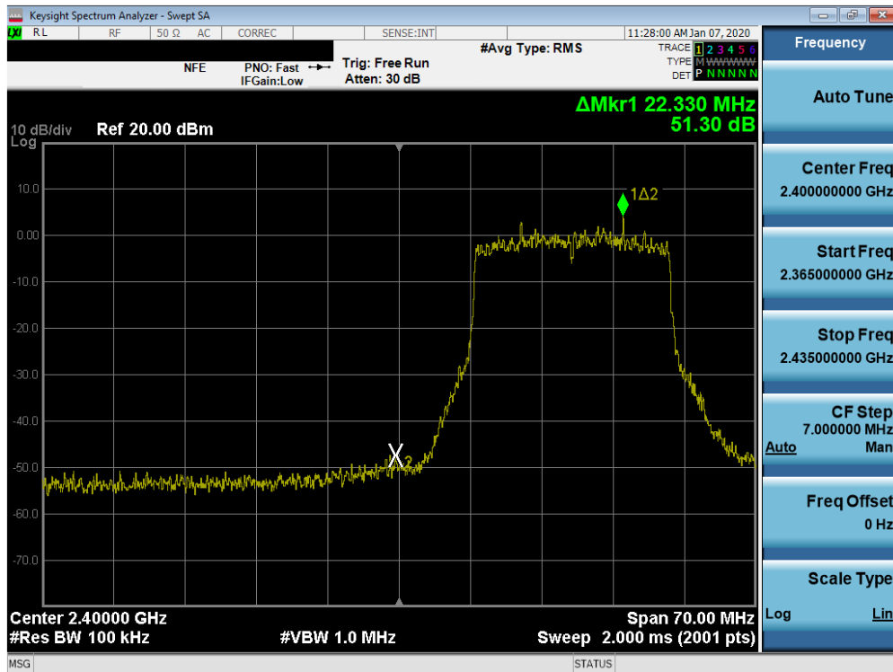
Plot 7-79. Band Edge Plot SISO ANT2 (802.11ax – Ch. 2)
