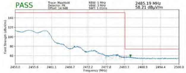
Plot 7-132. Radiated Restricted Upper Band Edge Measurement MIMO/CDD (Peak)
