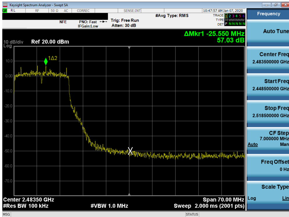
Plot 7-71. Band Edge Plot SISO ANT2 (802.11g – Ch. 10)
