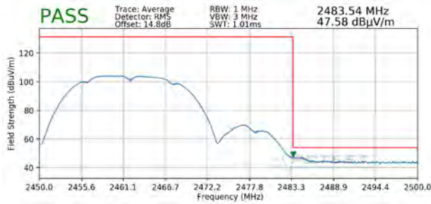
Plot 7-115. Radiated Restricted Upper Band Edge Measurement SISO ANT1 (Average)
