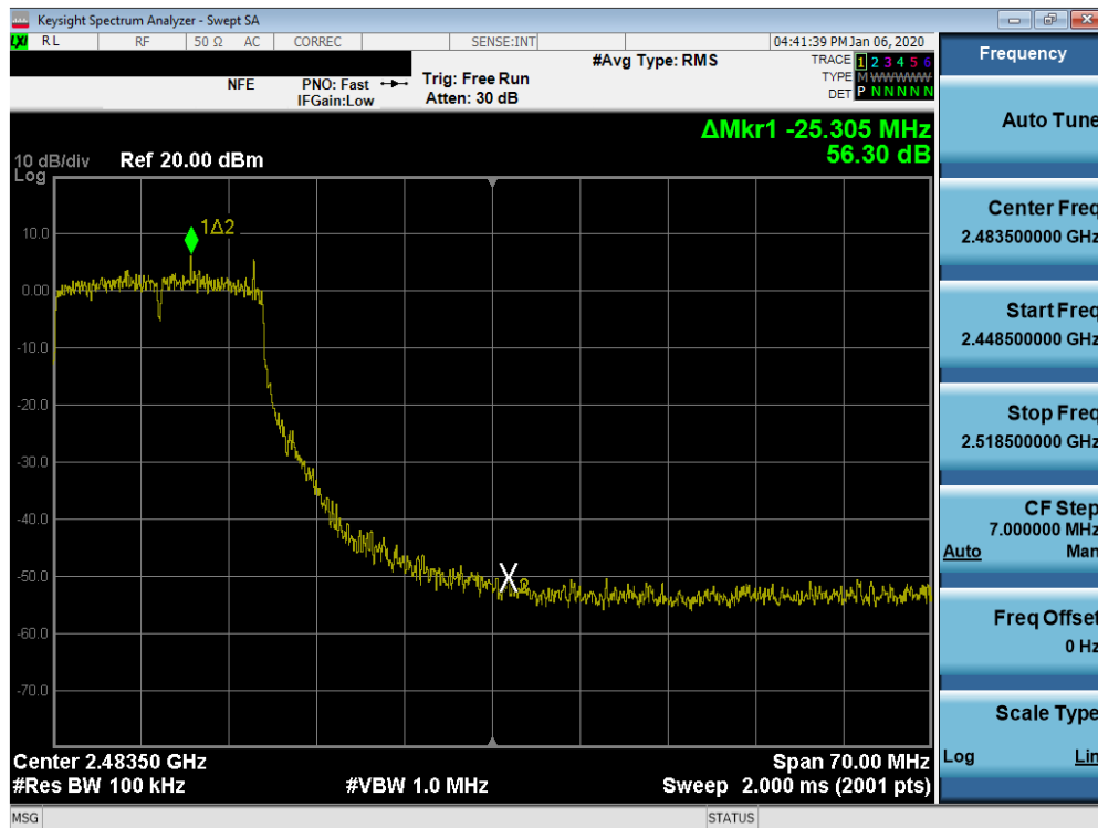
Plot 7-54. Band Edge Plot SISO ANT1 (802.11g – Ch. 10)
