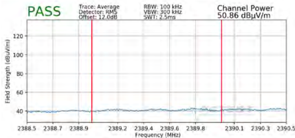
Plot 7-137. Radiated Restricted Band Edge Measurement MIMO/CDD with WCP + DD (Average)
