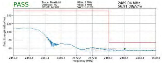
Plot 7-112. Radiated Restricted Upper Band Edge Measurement SISO ANT1 (Peak)
