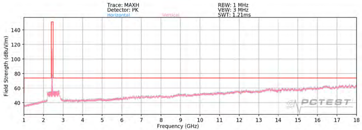
Plot 7-104. Radiated Spurious Plot above 1GHz MIMO/CDD (802.11g – Ch. 6)
