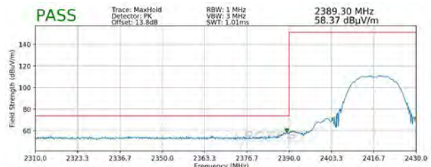
Plot 7-110. Radiated Restricted Lower Band Edge Measurement SISO ANT1 (Peak)
