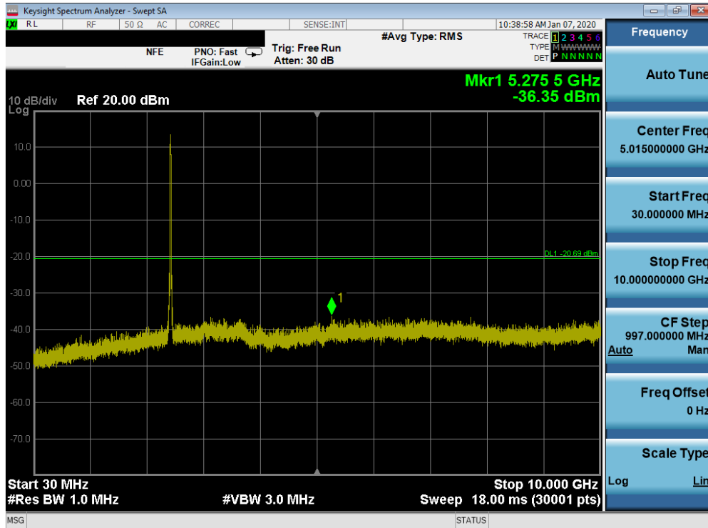
Plot 7-91. Conducted Spurious Plot SISO ANT2 (802.11b – Ch. 6)
