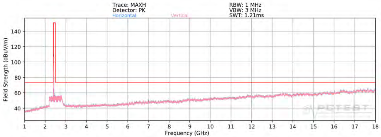
Plot 7-95. Radiated Spurious Plot above 1GHz SISO ANT1 (802.11b – Ch. 1)
