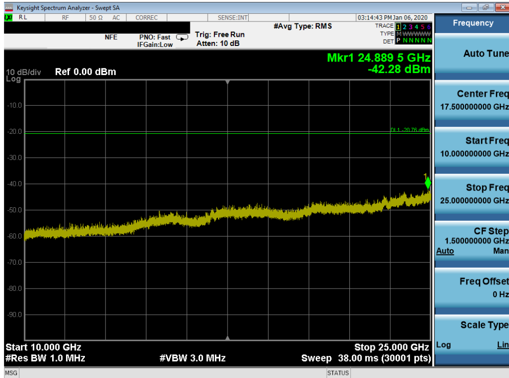
Plot 7-88. Conducted Spurious Plot SISO ANT1 (802.11b – Ch. 11)
