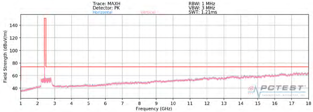
Plot 7-99. Radiated Spurious Plot above 1GHz SISO ANT2 (802.11b – Ch. 1)
