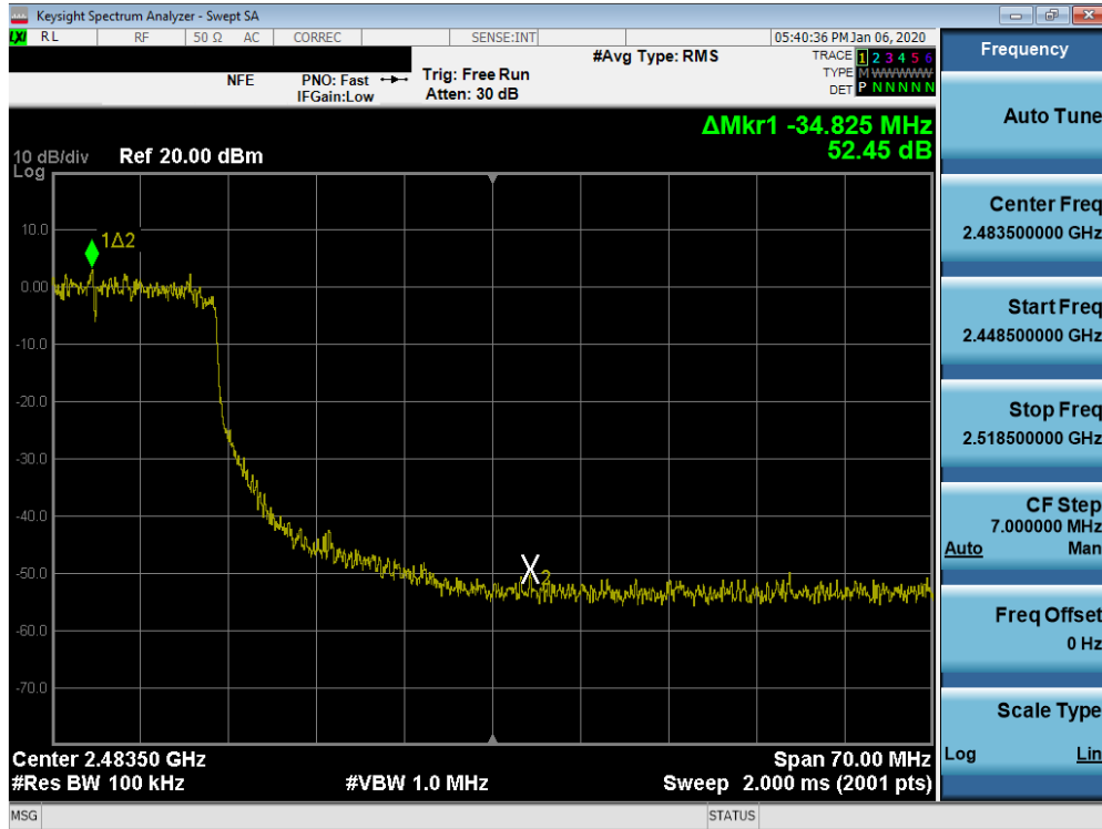
Plot 7-63. Band Edge Plot SISO ANT1 (802.11ax (2.4GHz) – Ch. 9)
