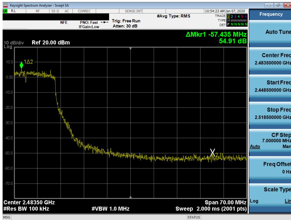
Plot 7-75. Band Edge Plot SISO ANT2 (802.11n – Ch. 9)
