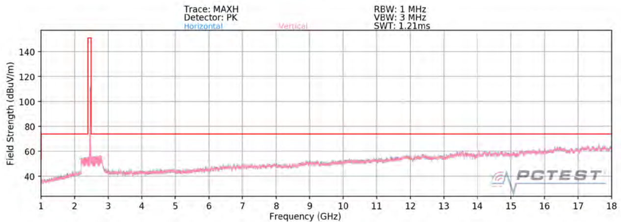
Plot 7-105. Radiated Spurious Plot above 1GHz MIMO/CDD (802.11g – Ch. 11)
