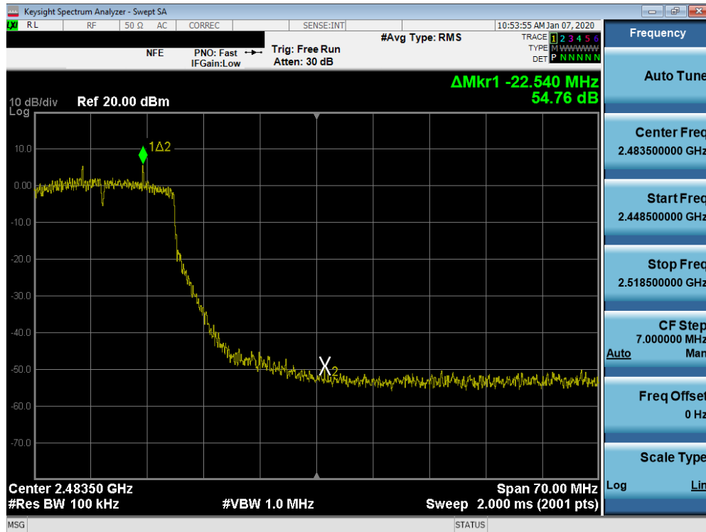
Plot 7-76. Band Edge Plot SISO ANT2 (802.11n - Ch. 10)
