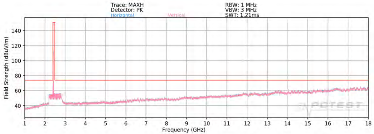
Plot 7-103. Radiated Spurious Plot above 1GHz MIMO/CDD (802.11g – Ch. 1)
