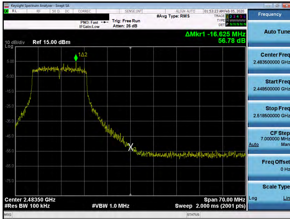
Plot 7-55. Band Edge Plot SISO ANT1 (802.11g - Ch. 11)
