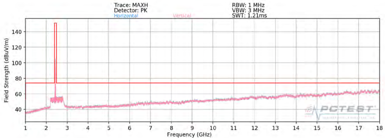
Plot 7-100. Radiated Spurious Plot above 1GHz SISO ANT2 (802.11b – Ch. 6)
