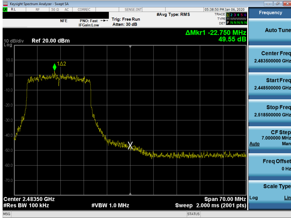
Plot 7-65. Band Edge Plot SISO ANT1 (802.11ax (2.4GHz) – Ch. 11)
