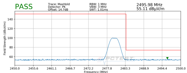
Plot 7-54. Radiated Restricted Upper Band Edge Measurement with WCP + DD (Peak)
