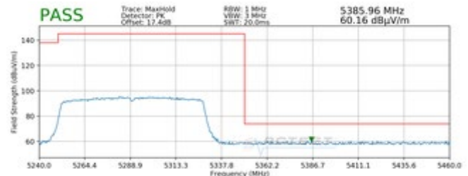
Plot 7-301. Radiated Upper Band Edge Plot SISO ANT1 (Peak – UNII Band 2A)
