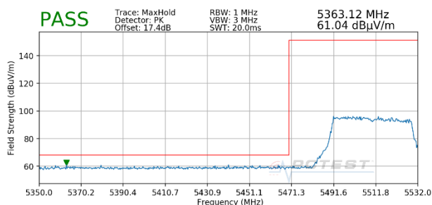
Plot 7-265. Radiated Lower Band Edge Plot SISO ANT1 (Peak – UNII Band 2C – 484 Tones)
