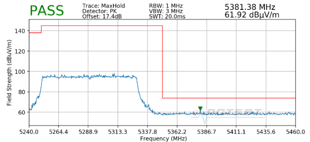
Plot 7-291. Radiated Upper Band Edge Plot SISO ANT2 (Peak – UNII Band 2A – 996 Tones)
