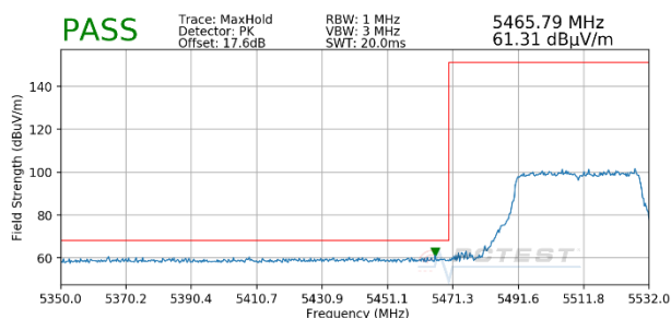
Plot 7-286. Radiated Lower Band Edge Plot SISO ANT2 (Peak – UNII Band 2C – 484 Tones)
