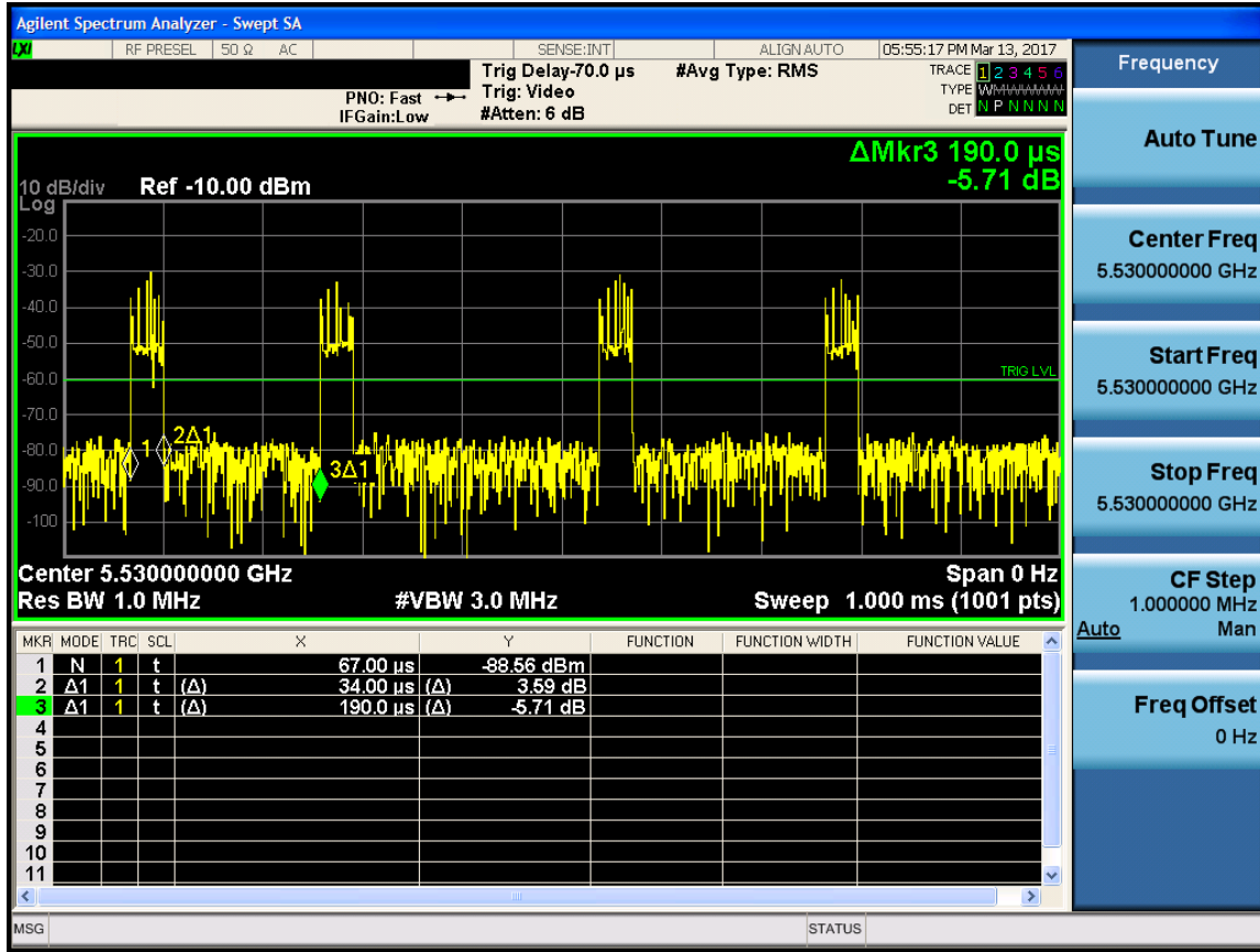
Figure 5-2. Band 2C Channel Loading Plot
