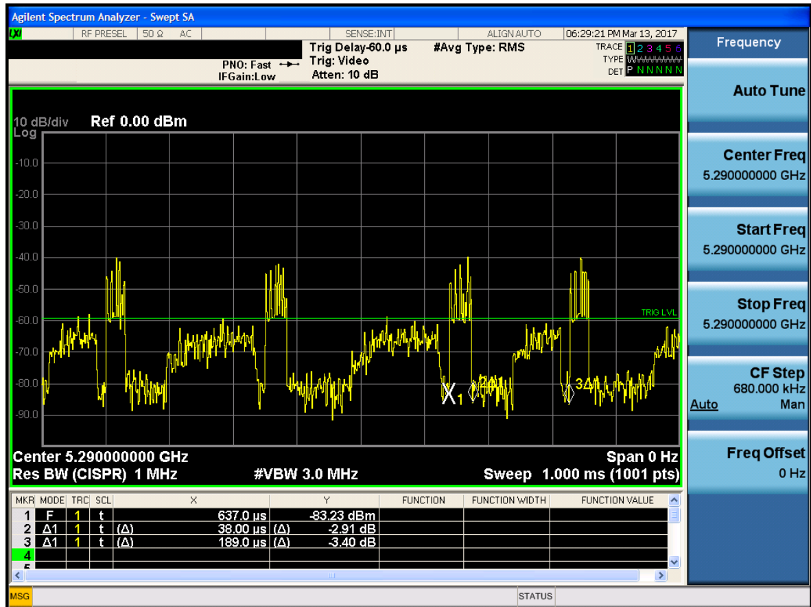
Figure 5-1. Band 2A Channel Loading Plot
