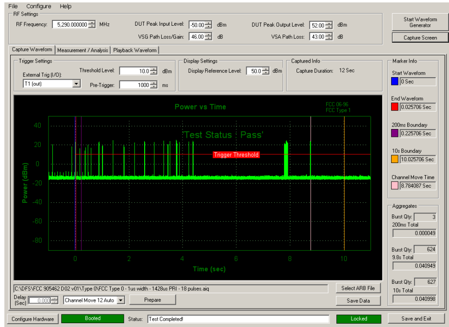
Figure 5-3. Band 2A Move Time and Aggregate Time
