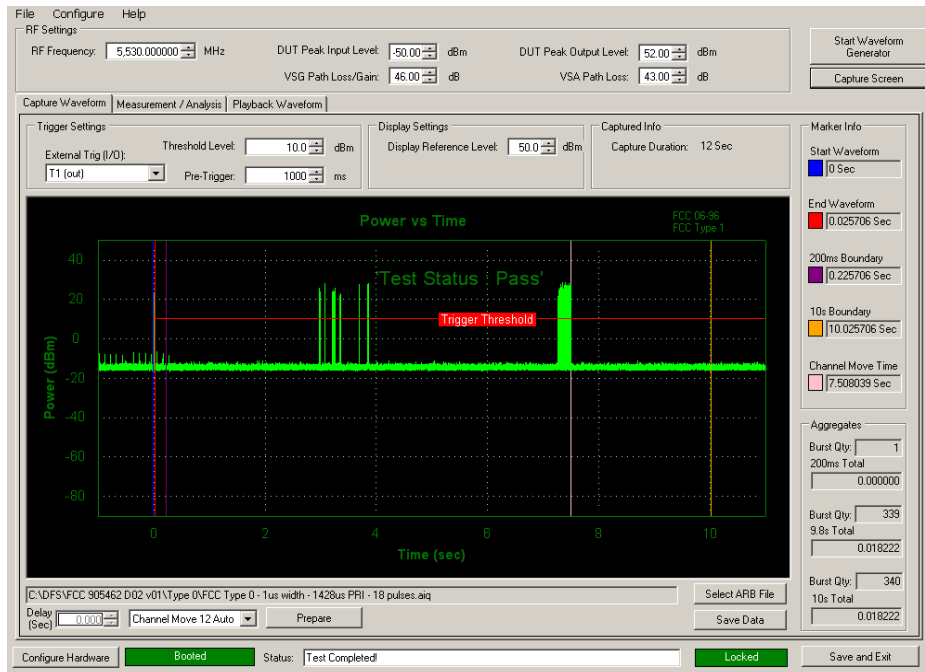
Figure 5-4. Band 2C Move Time and Aggregate Time
