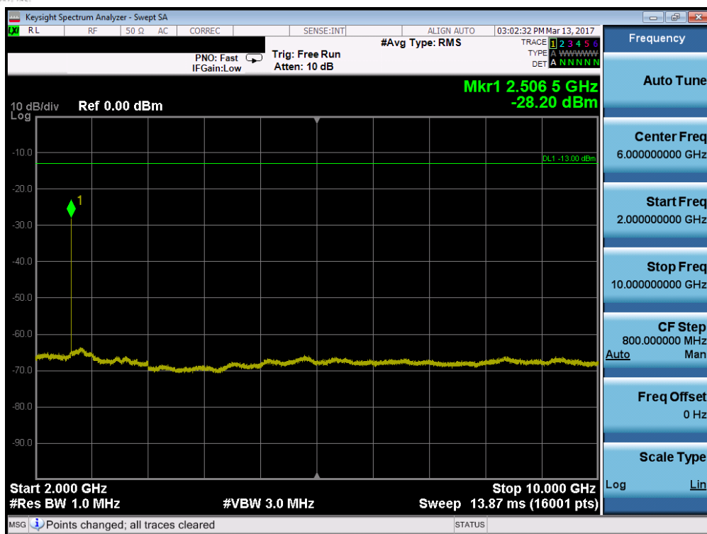
Plot 7-63. Conducted Spurious Plot (Band 5 – 3.0MHz QPSK – RB Size 1, RB Offset 0 – Mid Channel)
