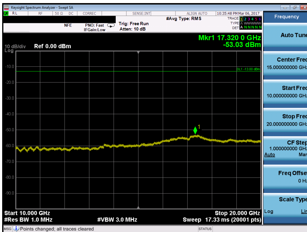
Plot 7-78. Conducted Spurious Plot (Band 66 – 5.0MHz QPSK – RB Size 1, RB Offset 0 – Low Channel)
