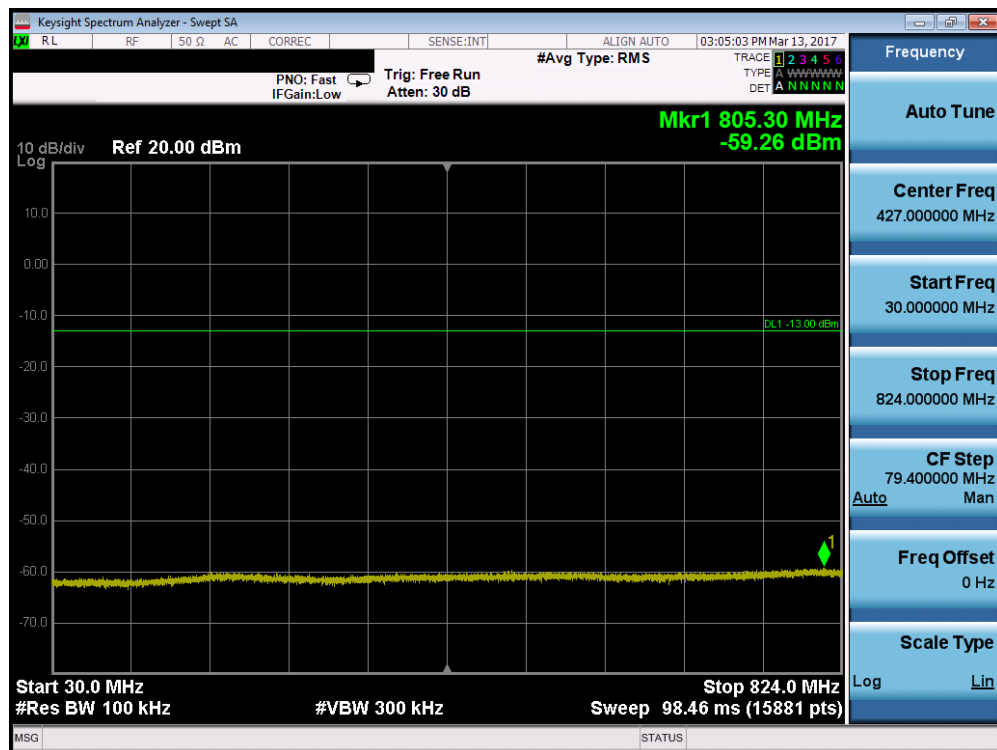
Plot 7-64. Conducted Spurious Plot (Band 5 – 3.0MHz QPSK – RB Size 1, RB Offset 0 – High Channel)
