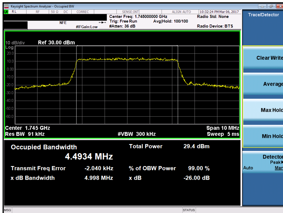
Plot 7-34. Occupied Bandwidth Plot (Band 66 – 5.0MHz 16-QAM – RB Size 25)
