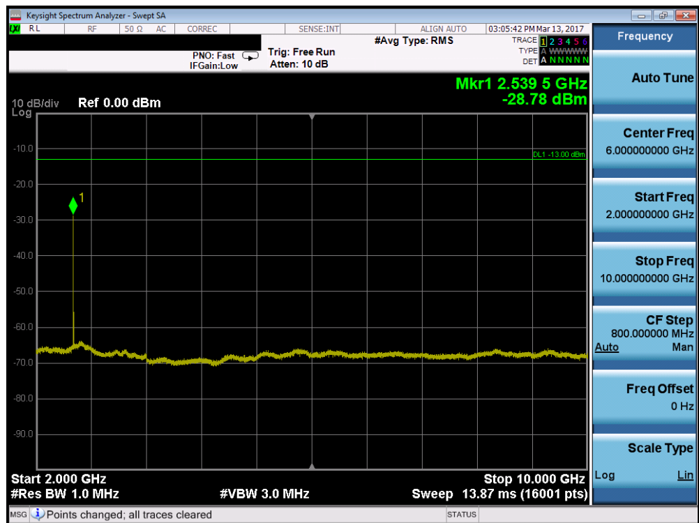
Plot 7-66. Conducted Spurious Plot (Band 5 – 3.0MHz QPSK – RB Size 1, RB Offset 0 – High Channel)
