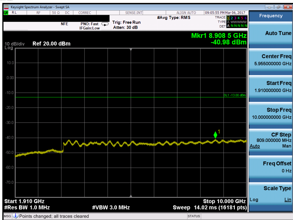
Plot 7-71. Conducted Spurious Plot (Band 2 – 15MHz QPSK – RB Size 1, RB Offset 0 – Mid Channel)
