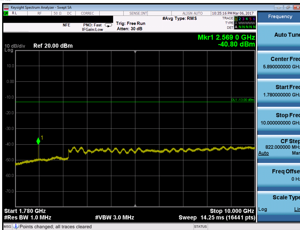
Plot 7-77. Conducted Spurious Plot (Band 66 – 5.0MHz QPSK – RB Size 1, RB Offset 0 – Low Channel)
