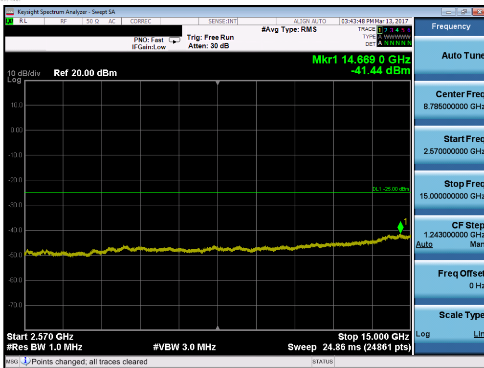
Plot 7-89. Conducted Spurious Plot (Band 7 – 10.0MHz QPSK – RB Size 1, RB Offset 0 – Mid Channel)
