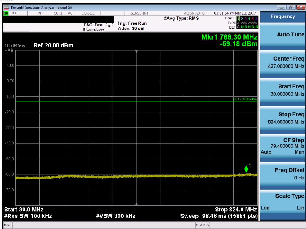
Plot 7-61. Conducted Spurious Plot (Band 5 – 3.0MHz QPSK – RB Size 1, RB Offset 0 – Mid Channel)
