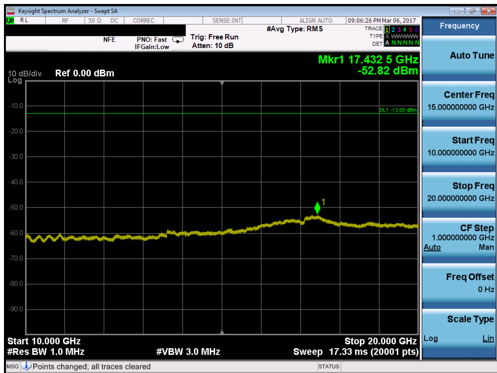
Plot 7-72. Conducted Spurious Plot (Band 2 – 15MHz QPSK – RB Size 1, RB Offset 0 – Mid Channel)
