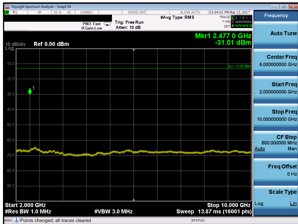
Plot 7-60. Conducted Spurious Plot (Band 5 – 3.0MHz QPSK – RB Size 1, RB Offset 0 – Low Channel)
