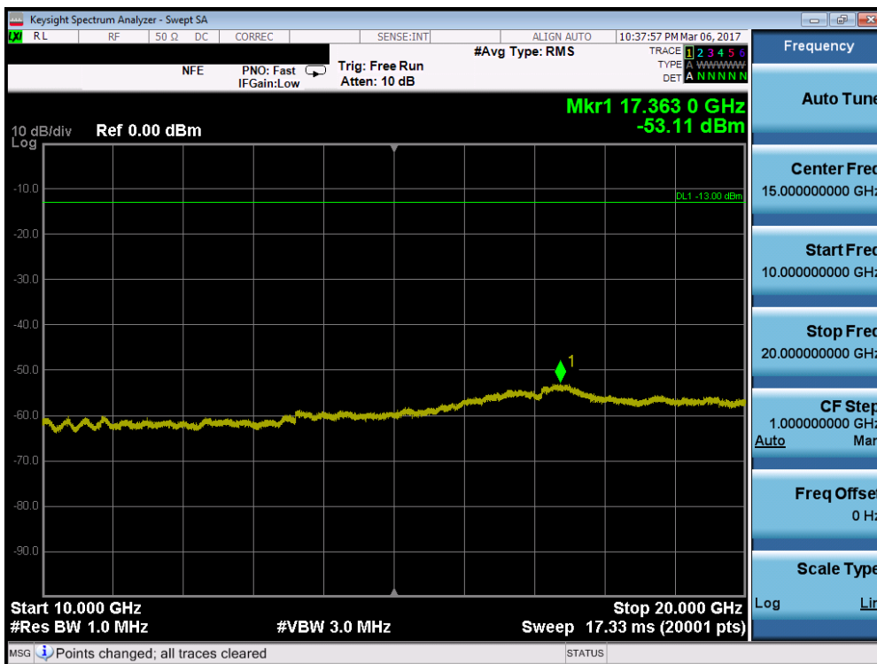
Plot 7-84. Conducted Spurious Plot (Band 66 – 5.0MHz QPSK – RB Size 1, RB Offset 0 – High Channel)
