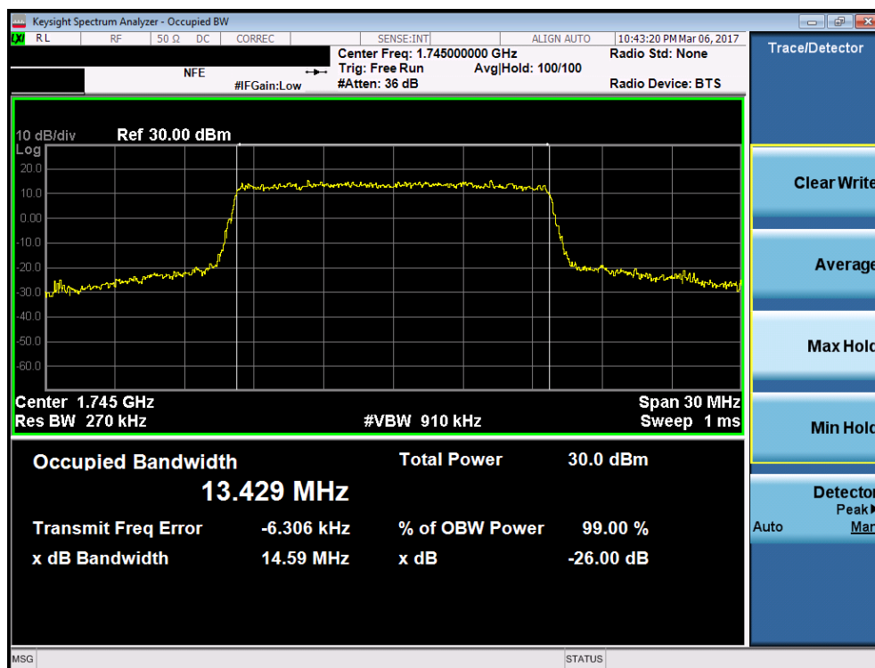
Plot 7-38. Occupied Bandwidth Plot (Band 66 – 15.0MHz 16-QAM – RB Size 75)
