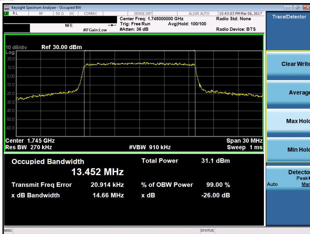
Plot 7-37. Occupied Bandwidth Plot (Band 66 – 15.0MHz QPSK – RB Size 75)
