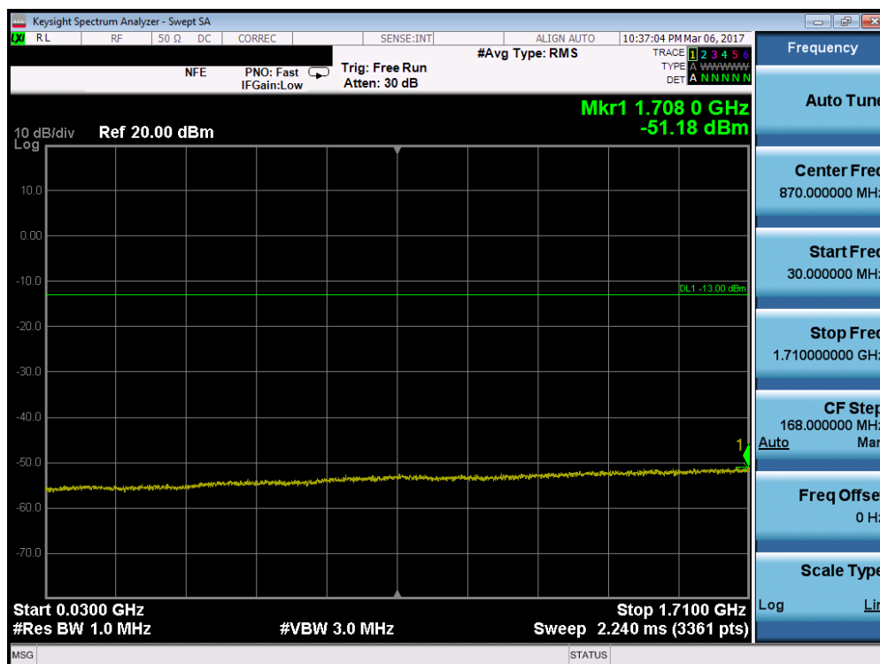
Plot 7-82. Conducted Spurious Plot (Band 66 – 5.0MHz QPSK – RB Size 1, RB Offset 0 – High Channel)
