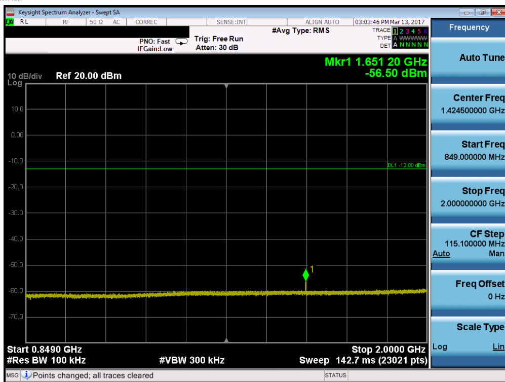
Plot 7-59. Conducted Spurious Plot (Band 5 – 3.0MHz QPSK – RB Size 1, RB Offset 0 – Low Channel)
