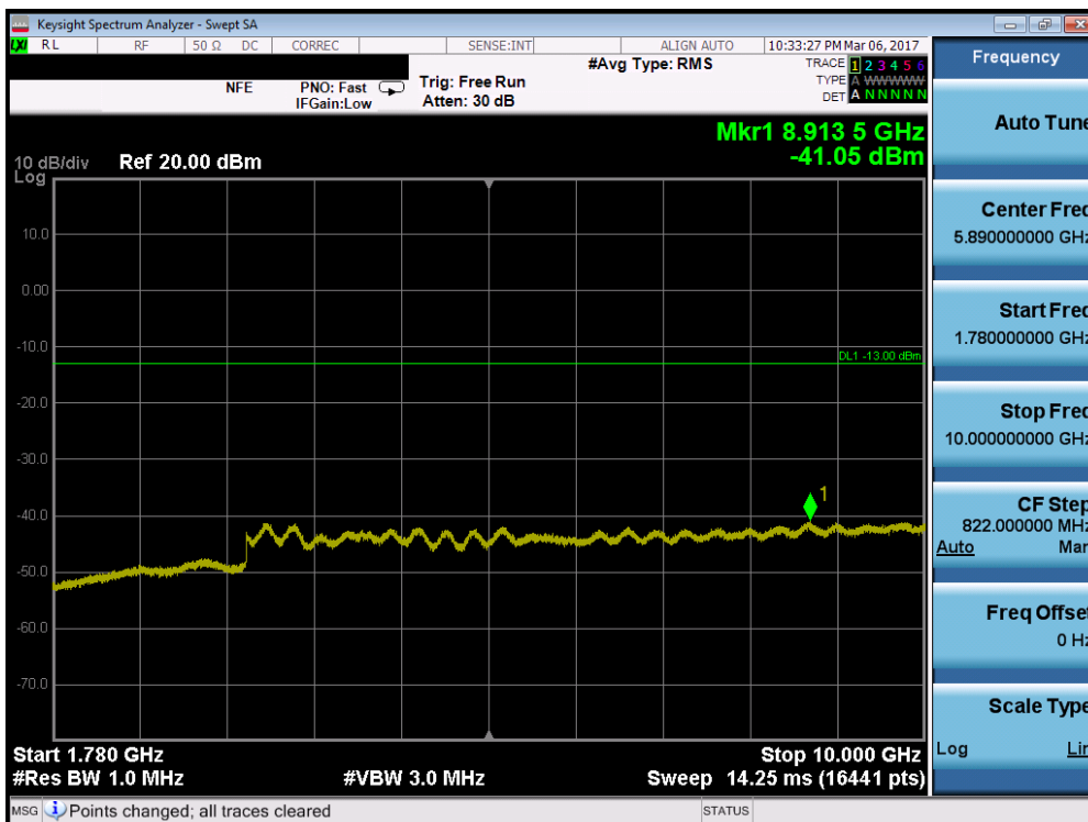
Plot 7-80. Conducted Spurious Plot (Band 66 – 5.0MHz QPSK – RB Size 1, RB Offset 0 – Mid Channel)
