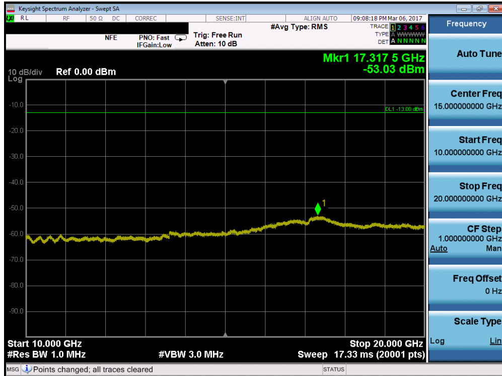
Plot 7-69. Conducted Spurious Plot (Band 2 – 15MHz QPSK – RB Size 1, RB Offset 0 – Low Channel)
