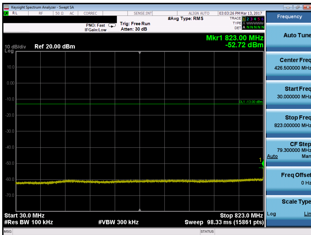
Plot 7-58. Conducted Spurious Plot (Band 5 – 3.0MHz QPSK – RB Size 1, RB Offset 0 – Low Channel)
