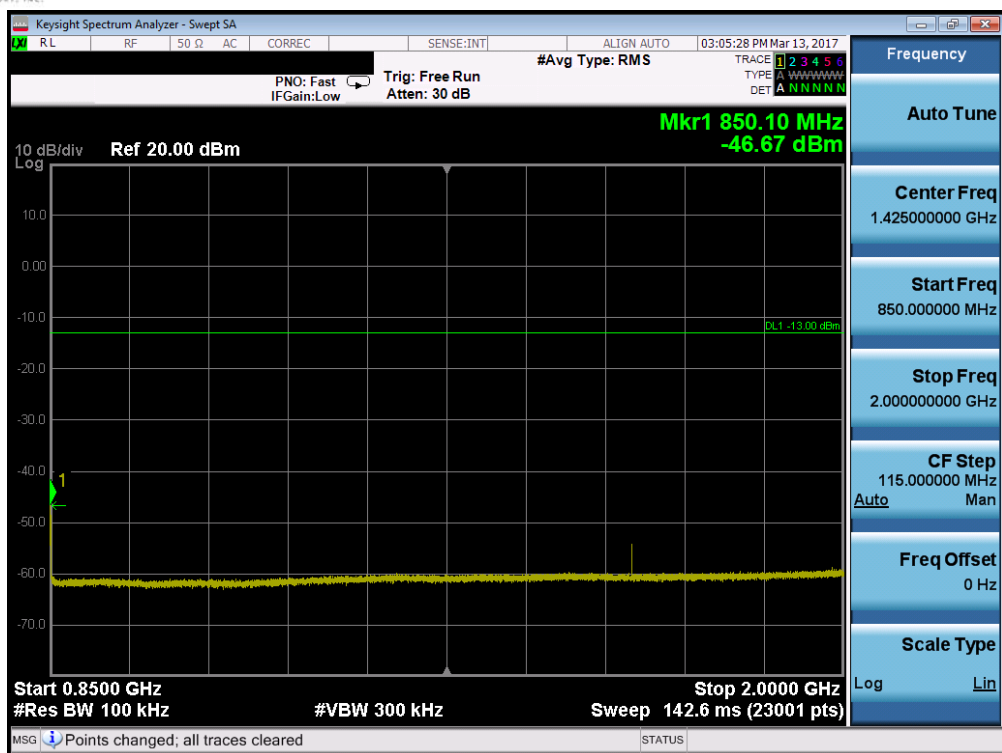
Plot 7-65. Conducted Spurious Plot (Band 5 – 3.0MHz QPSK – RB Size 1, RB Offset 0 – High Channel)
