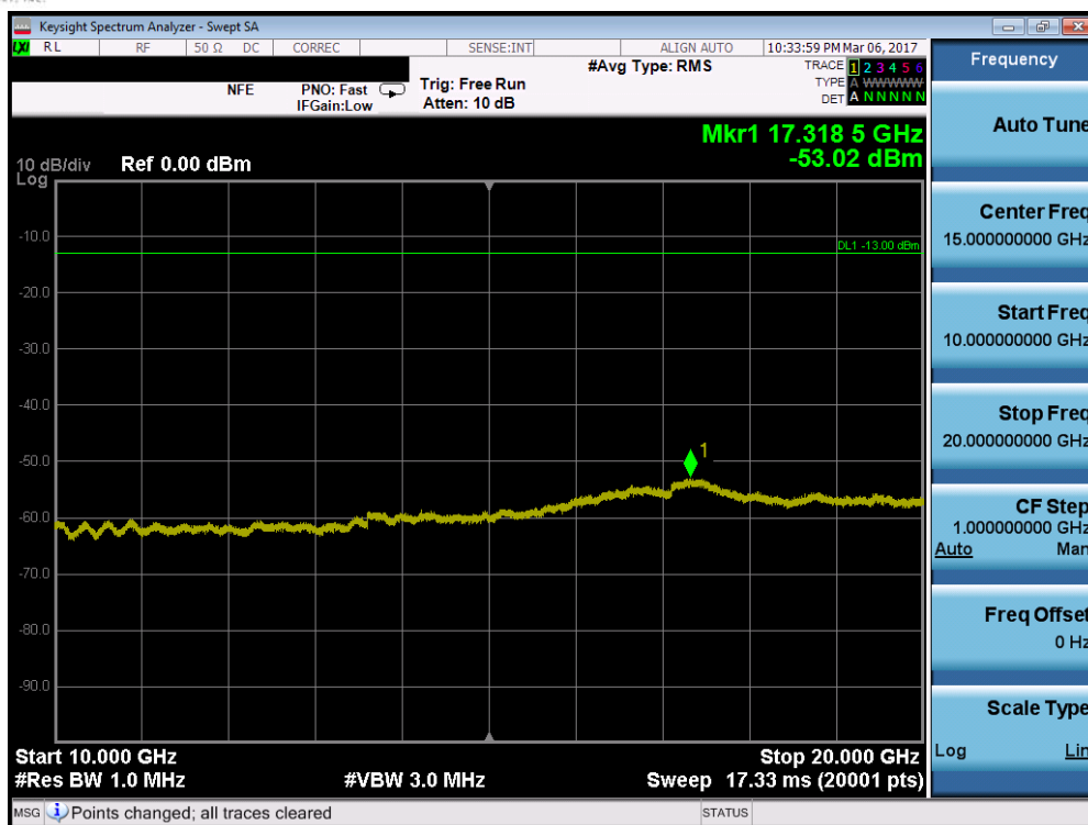
Plot 7-81. Conducted Spurious Plot (Band 66 – 5.0MHz QPSK – RB Size 1, RB Offset 0 – Mid Channel)
