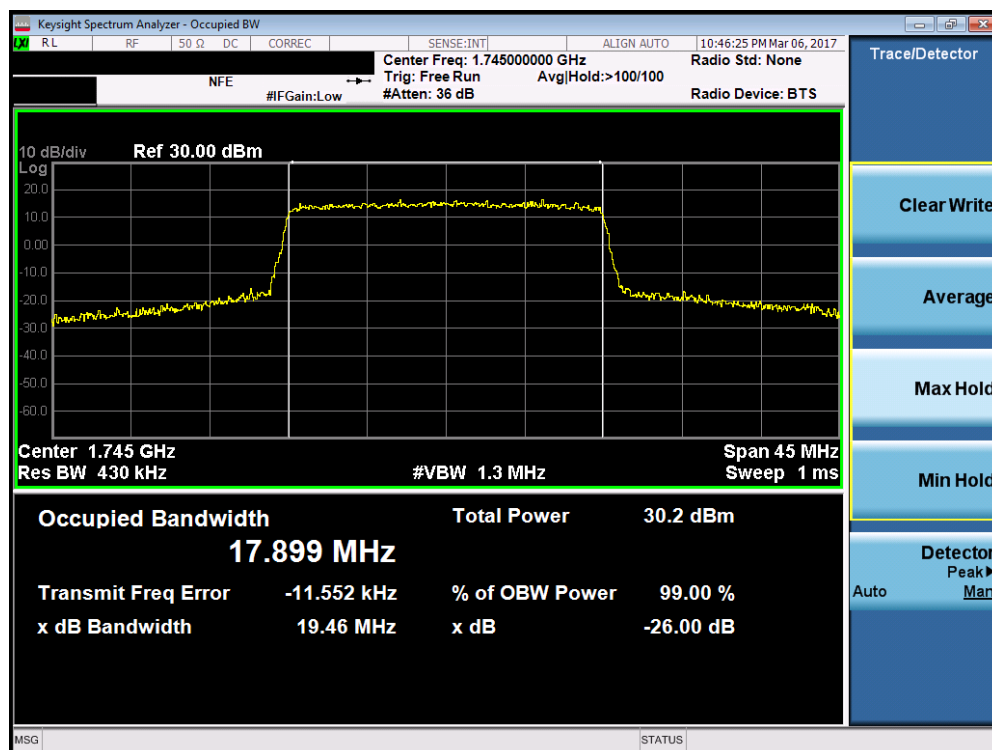
Plot 7-40. Occupied Bandwidth Plot (Band 66 – 20.0MHz 16-QAM – RB Size 100)
