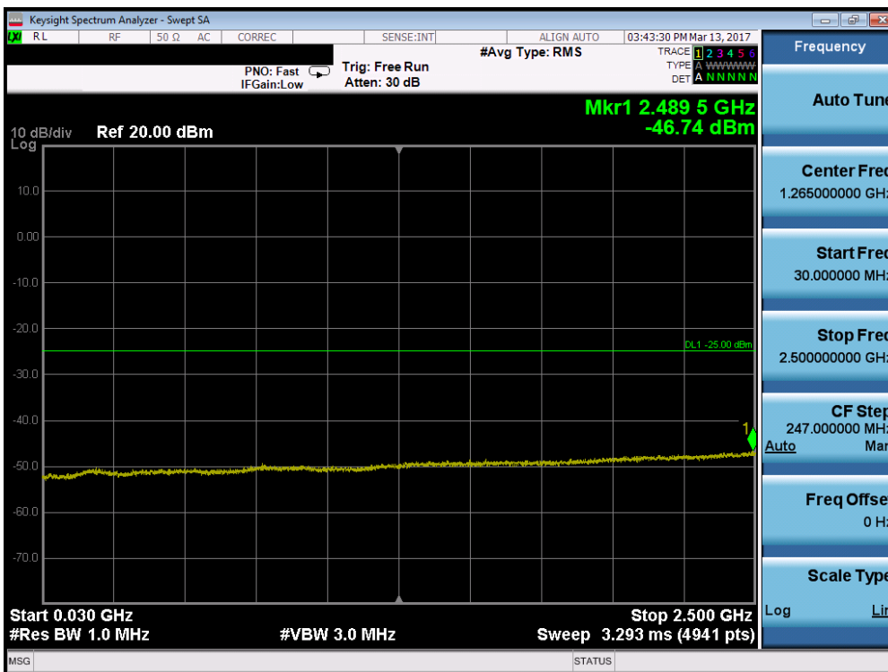
Plot 7-88. Conducted Spurious Plot (Band 7 – 10.0MHz QPSK – RB Size 1, RB Offset 0 – Mid Channel)
