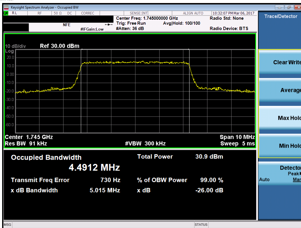
Plot 7-33. Occupied Bandwidth Plot (Band 66 – 5.0MHz QPSK – RB Size 25)
