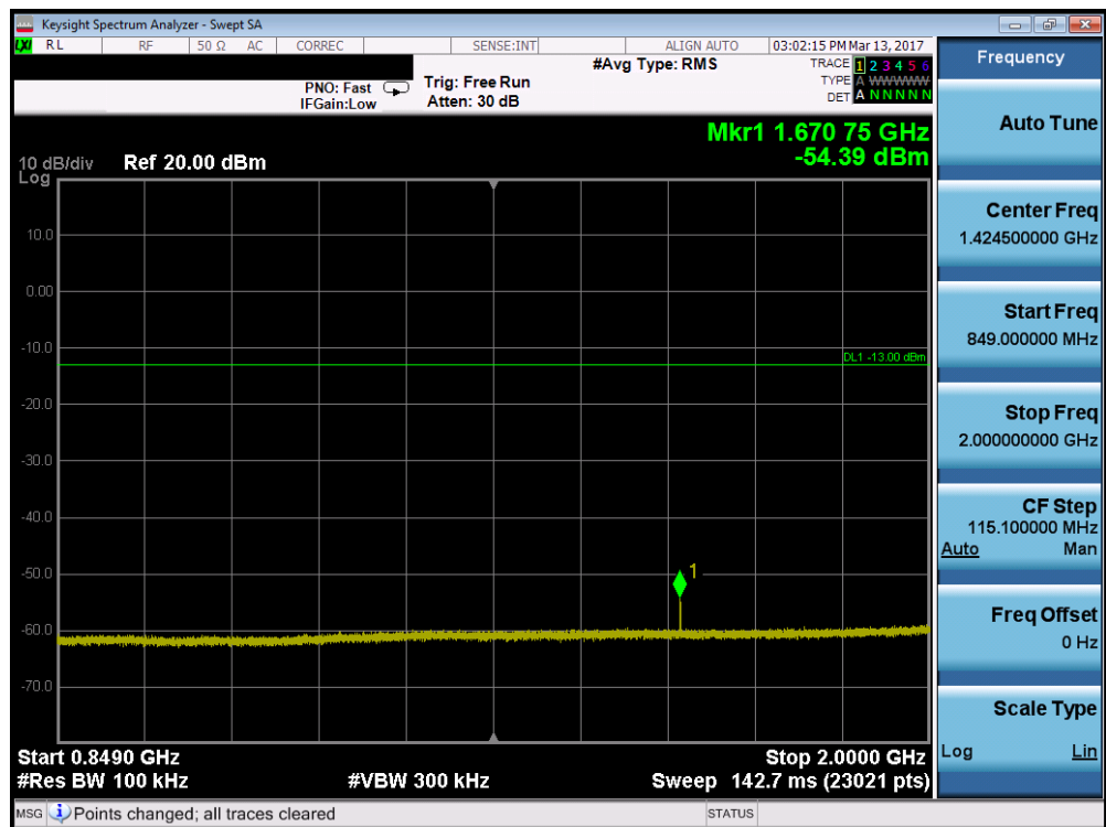
Plot 7-62. Conducted Spurious Plot (Band 5 – 3.0MHz QPSK – RB Size 1, RB Offset 0 – Mid Channel)
