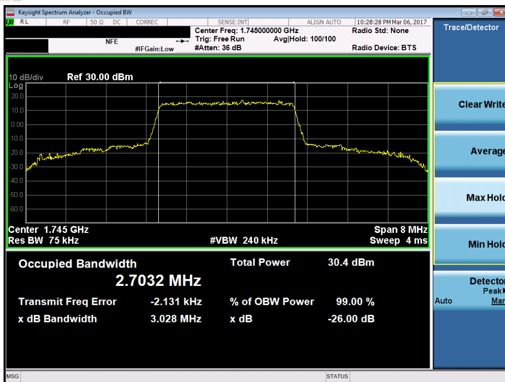
Plot 7-31. Occupied Bandwidth Plot (Band 66 – 3.0MHz QPSK – RB Size 15)
