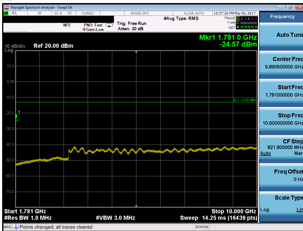
Plot 7-83. Conducted Spurious Plot (Band 66 – 5.0MHz QPSK – RB Size 1, RB Offset 0 – High Channel)
