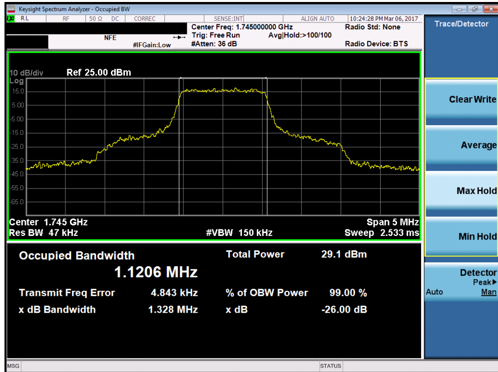
Plot 7-30. Occupied Bandwidth Plot (Band 66 – 1.4MHz 16-QAM – RB Size 6)
