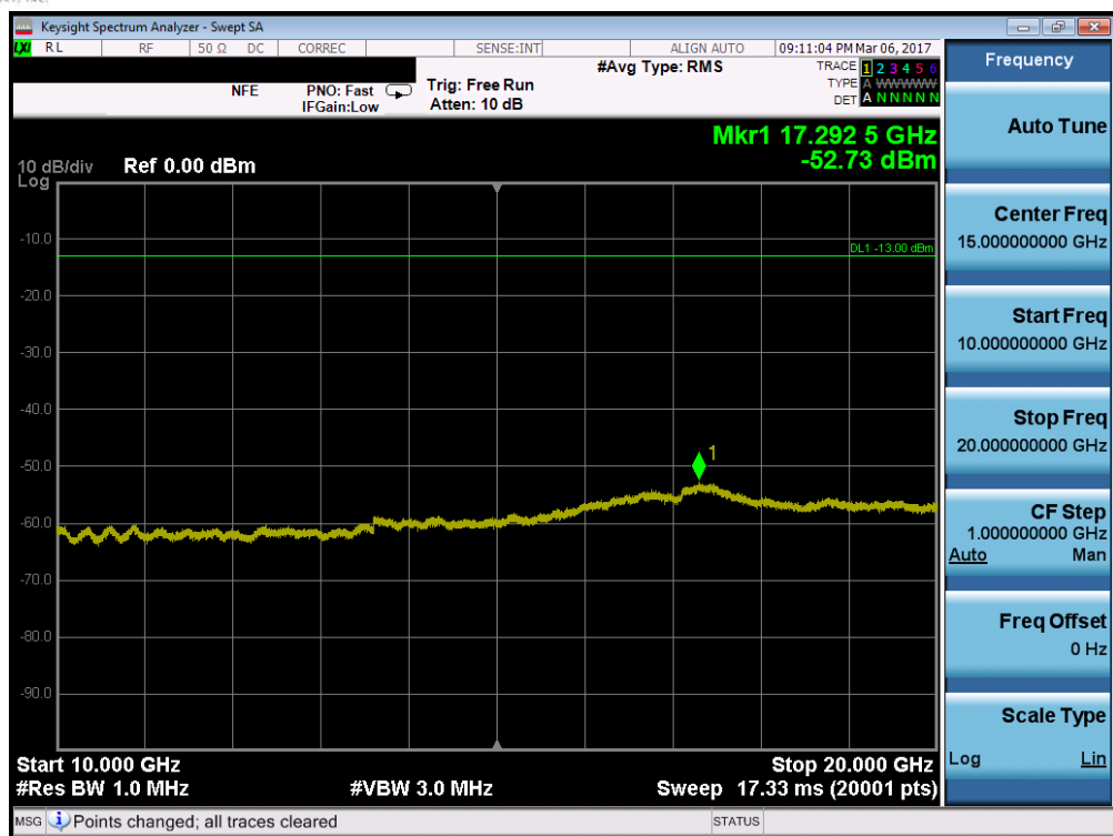
Plot 7-75. Conducted Spurious Plot (Band 2 – 15MHz QPSK – RB Size 1, RB Offset 0 – High Channel)
