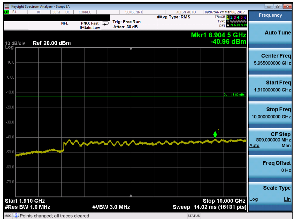
Plot 7-68. Conducted Spurious Plot (Band 2 – 15MHz QPSK – RB Size 1, RB Offset 0 – Low Channel)
