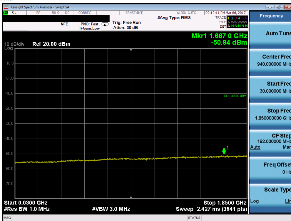
Plot 7-73. Conducted Spurious Plot (Band 2 – 15MHz QPSK – RB Size 1, RB Offset 0 – High Channel)
