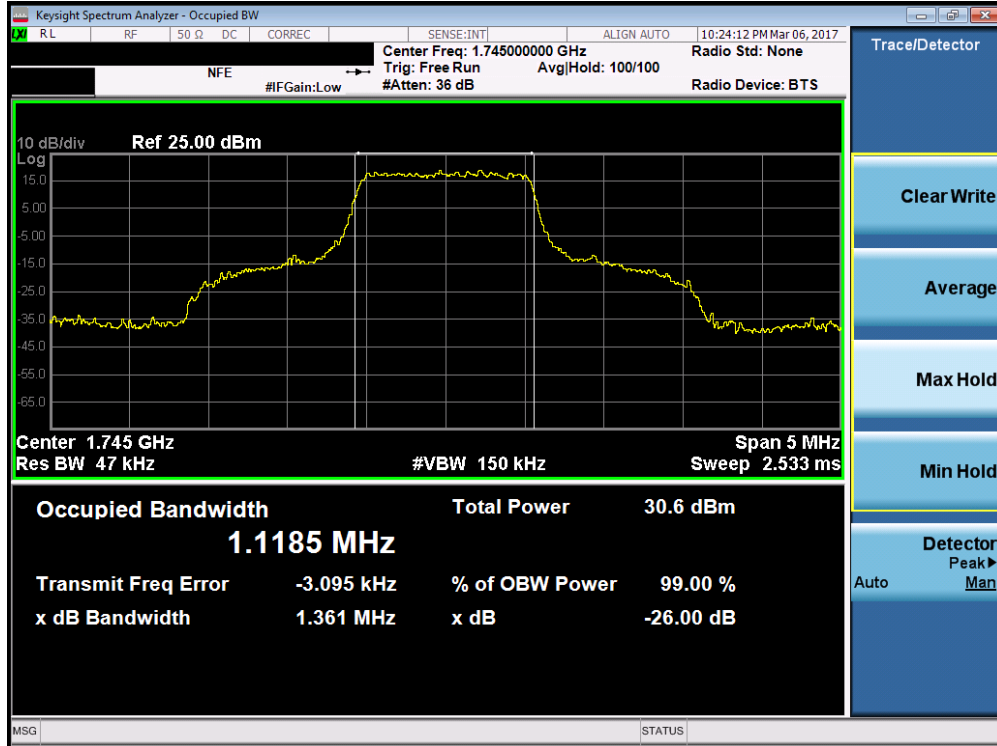
Plot 7-29. Occupied Bandwidth Plot (Band 66 – 1.4MHz QPSK – RB Size 6)
