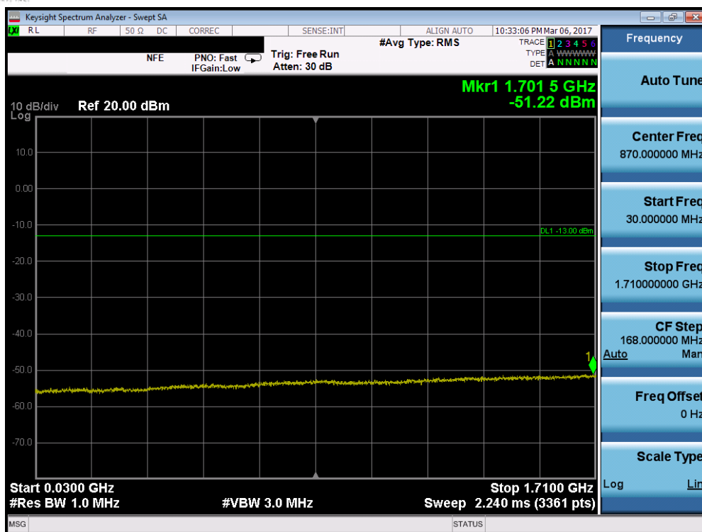
Plot 7-79. Conducted Spurious Plot (Band 66 – 5.0MHz QPSK – RB Size 1, RB Offset 0 – Mid Channel)
