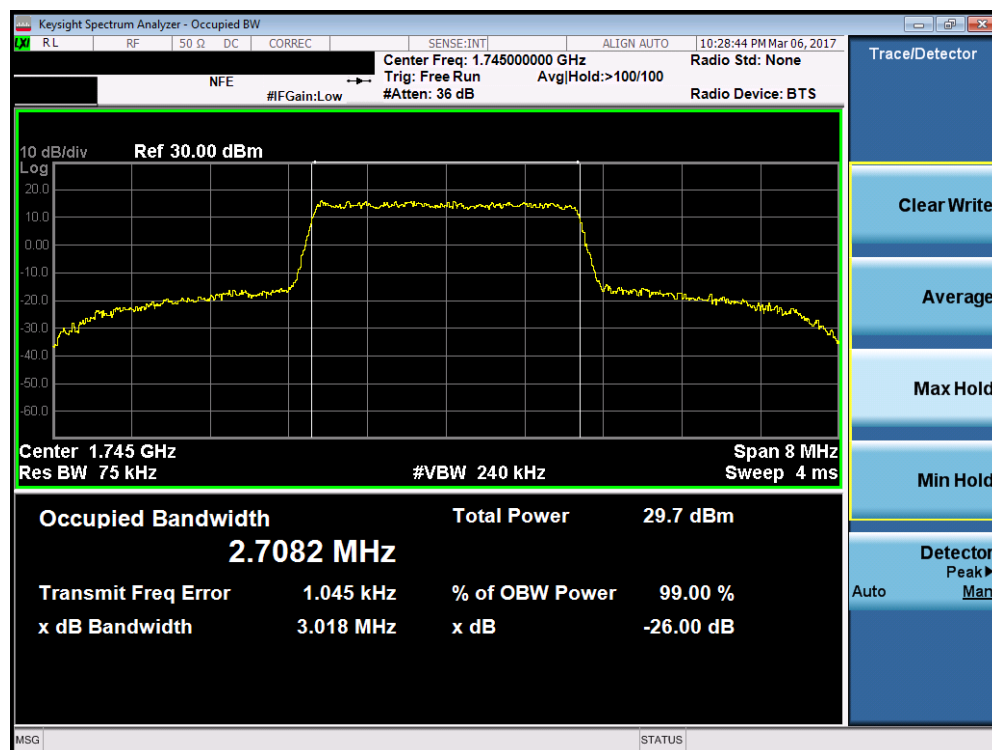
Plot 7-32. Occupied Bandwidth Plot (Band 66 – 3.0MHz 16-QAM – RB Size 15)
