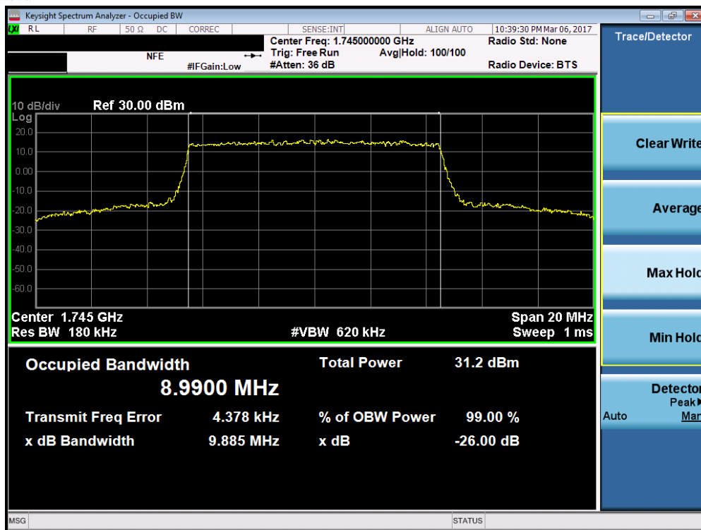
Plot 7-35. Occupied Bandwidth Plot (Band 66 – 10.0MHz QPSK – RB Size 50)
