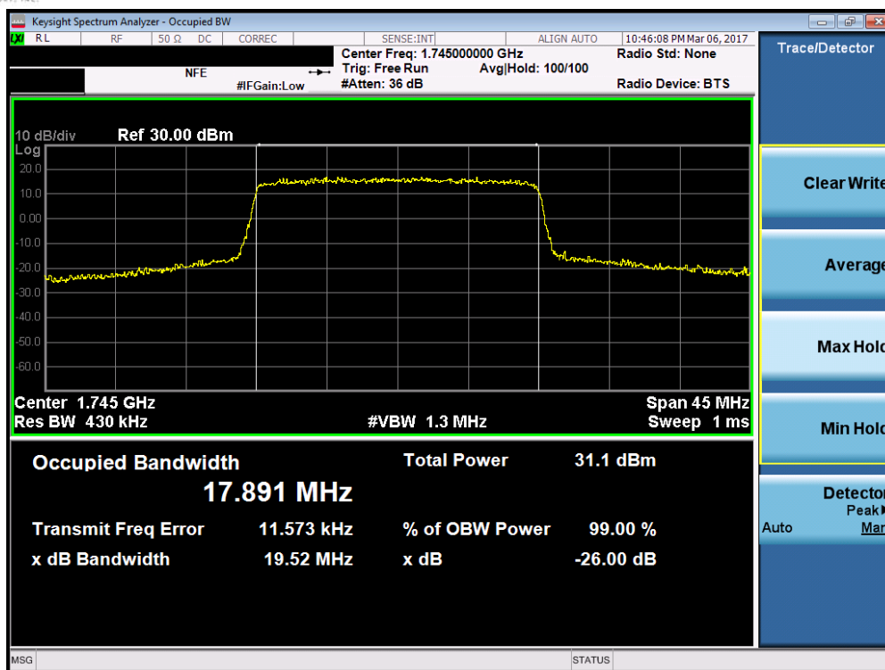
Plot 7-39. Occupied Bandwidth Plot (Band 66 – 20.0MHz QPSK – RB Size 100)
