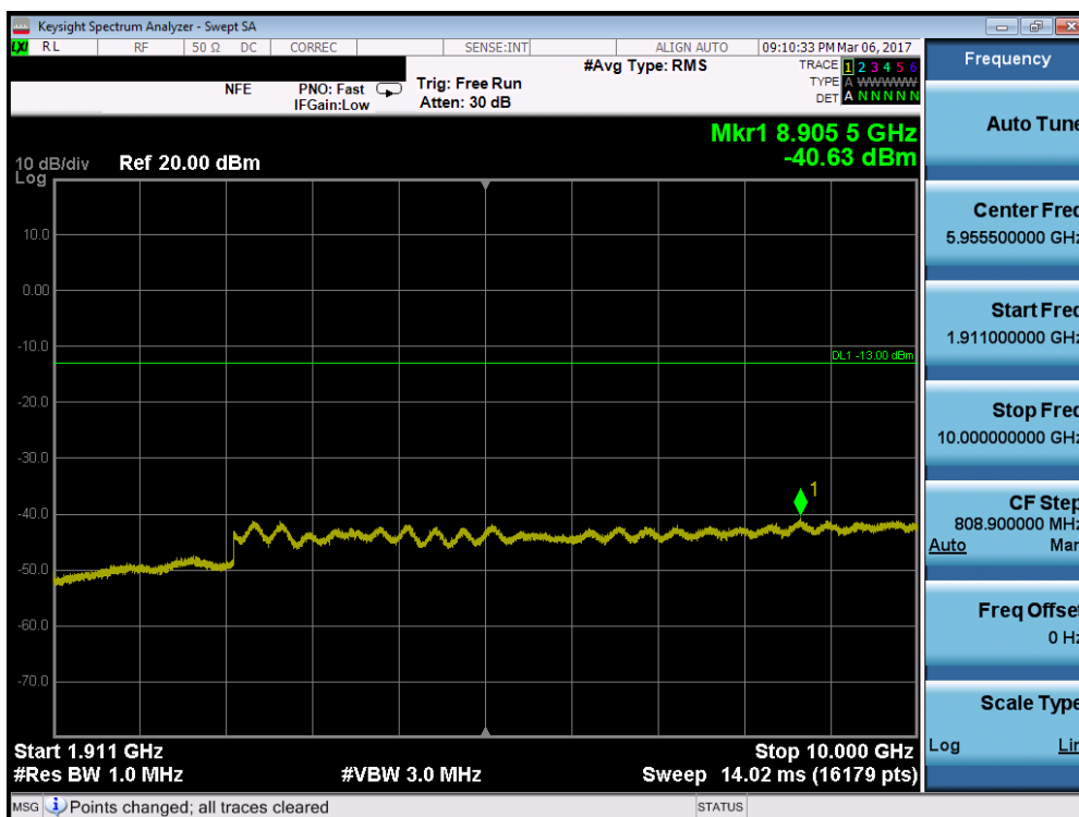
Plot 7-74. Conducted Spurious Plot (Band 2 – 15MHz QPSK – RB Size 1, RB Offset 0 – High Channel)
