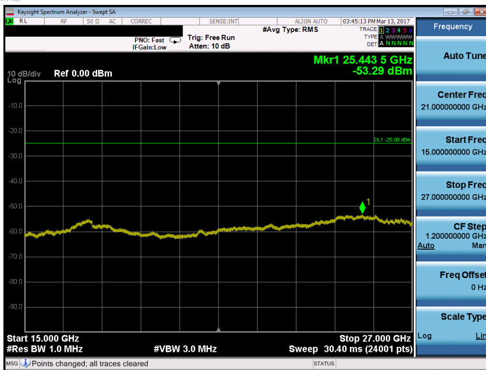
Plot 7-87. Conducted Spurious Plot (Band 7 – 10.0MHz QPSK – RB Size 1, RB Offset 0 – Low Channel)
