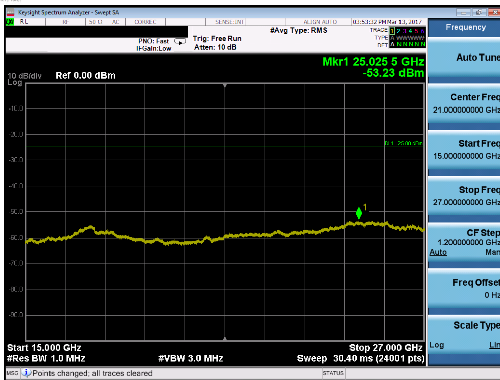
Plot 7-93. Conducted Spurious Plot (Band 7 – 10.0MHz QPSK – RB Size 1, RB Offset 0 – High Channel)
