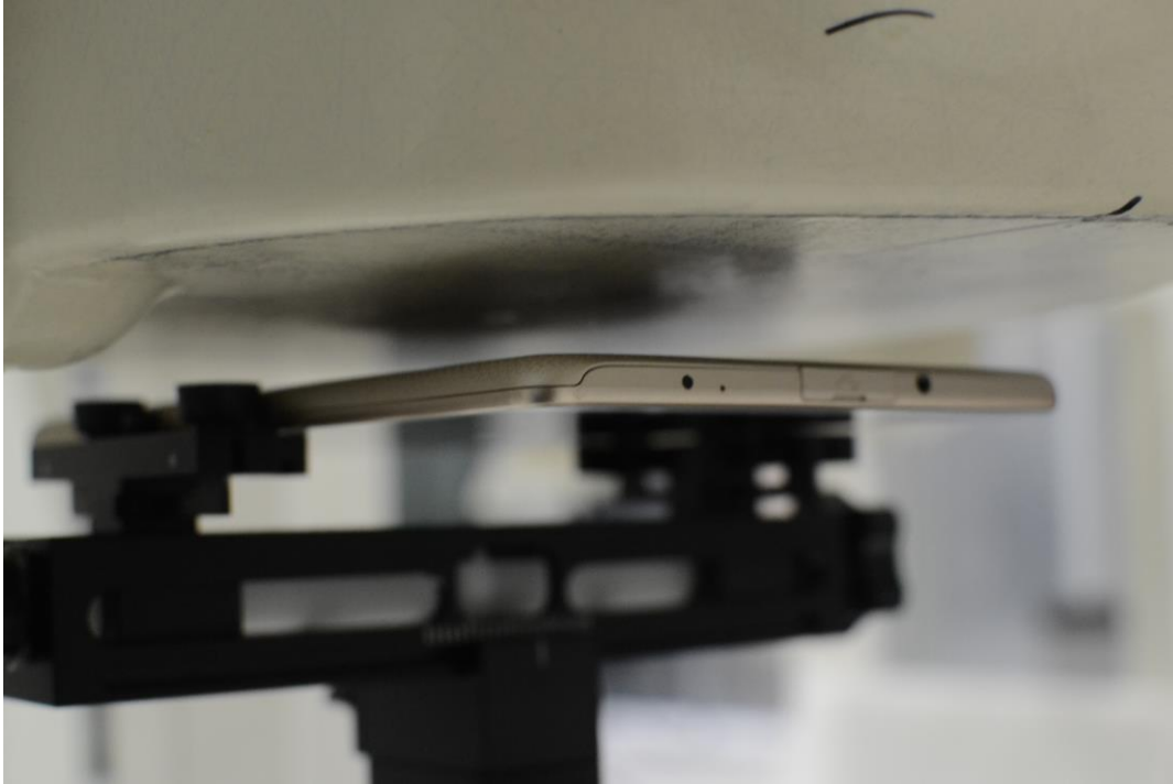
SAR Test Setup Photo 3: Back Side at 1.8 cm
