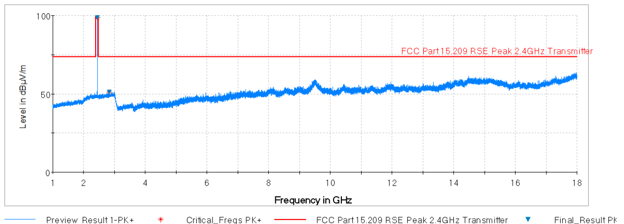
Plot 7-20. Radiated Spurious Plot above 1GHz (BT – Ch. 39, Ant. Pol. H)
