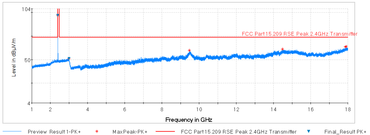
Plot 7-18. Radiated Spurious Plot above 1GHz (BT – Ch. 0, Ant. Pol. H)
