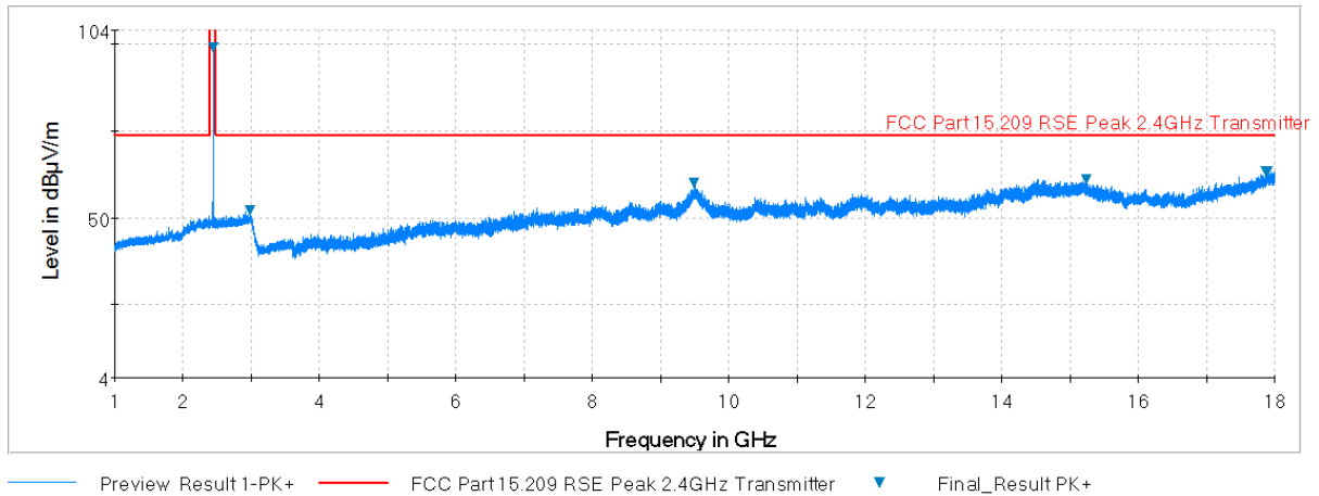
Plot 7-21. Radiated Spurious Plot above 1GHz (BT – Ch. 39, Ant. Pol. V)
