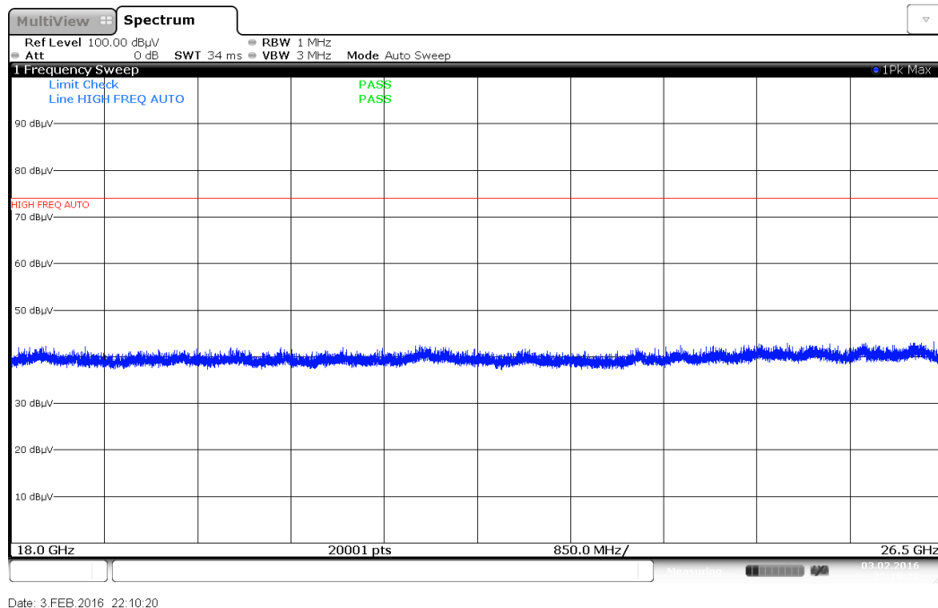
Plot 7-25. Radiated Spurious Plot above 18GHz (Pol. V)
