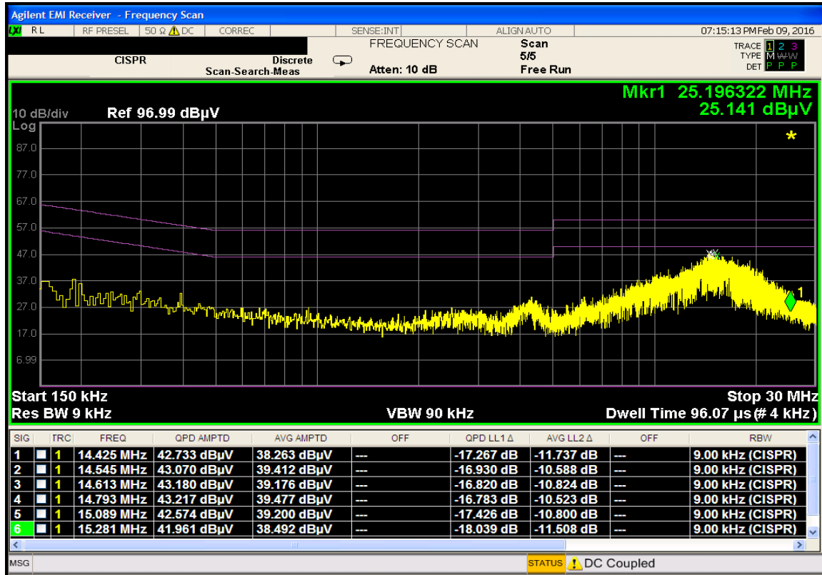
Plot 7-31. Line Conducted Plot with Bluetooth LE (N)
