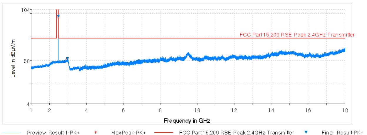
Plot 7-23. Radiated Spurious Plot above 1GHz (BT – Ch. 78, Ant. Pol. V)
