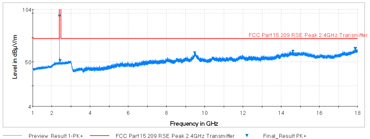
Plot 7-19. Radiated Spurious Plot above 1GHz (BT – Ch. 0, Ant. Pol. V)
