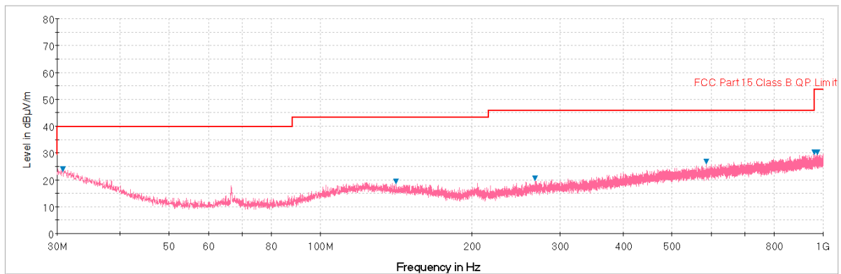
Plot 7-29. Radiated Spurious Plot below 1GHz (Pol. V)
