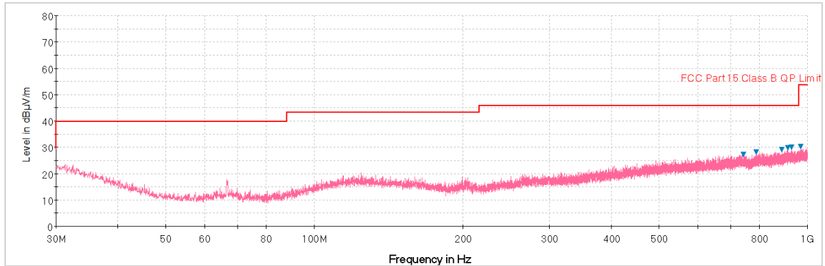
Plot 7-28. Radiated Spurious Plot below 1GHz (Pol. H)
