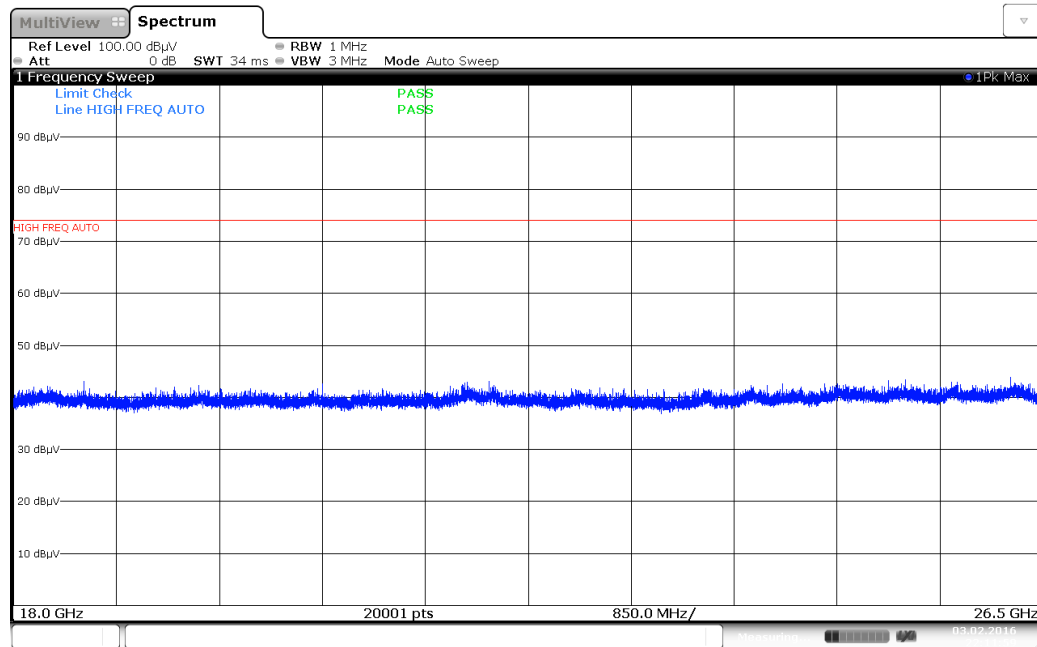
Plot 7-24. Radiated Spurious Plot above 18GHz (Pol. H)
