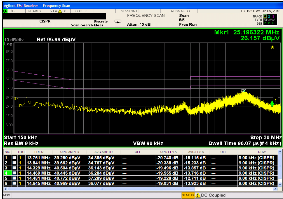
Plot 7-30. Line Conducted Plot with Bluetooth LE (L1)
