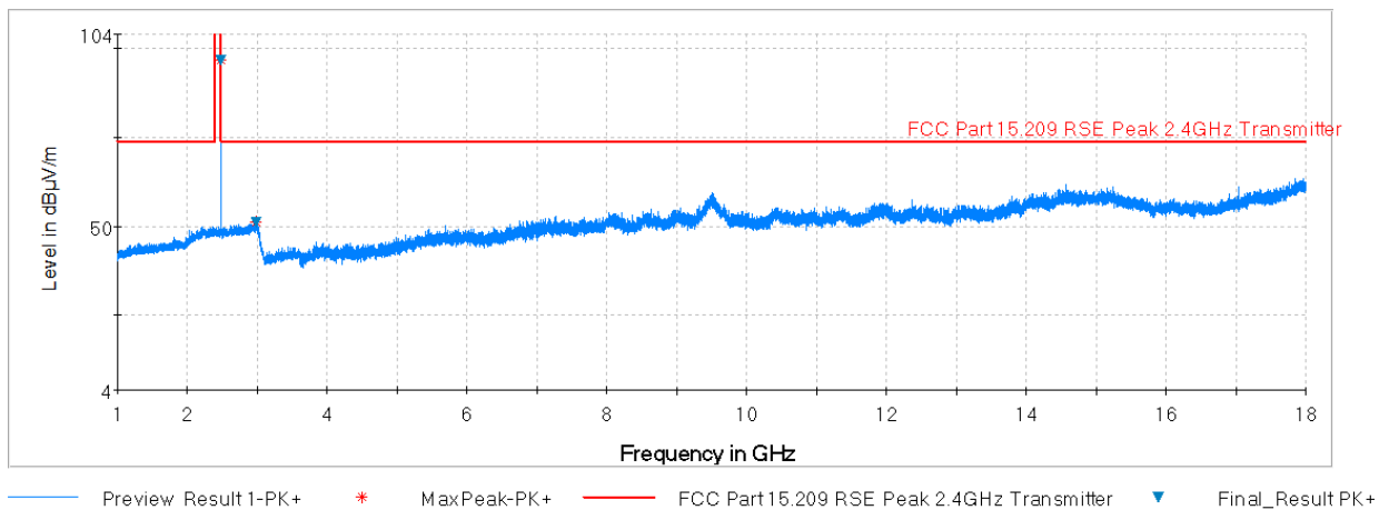
Plot 7-22. Radiated Spurious Plot above 1GHz (BT – Ch. 78, Ant. Pol. H)
