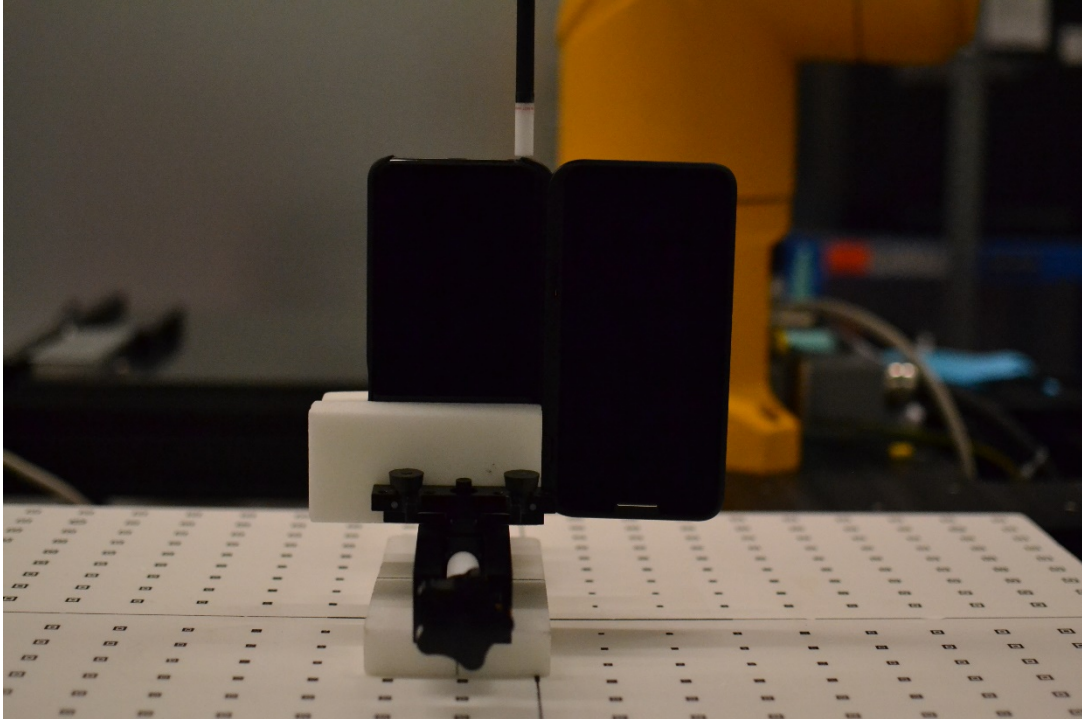
Near-Field Power Density Test Setup Photo 3 – Bottom Edge at 2 mm
