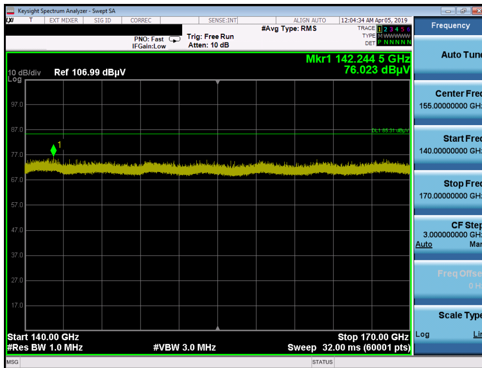
Plot 6-14. Radiated Spurious Plot 140-170 GHz
