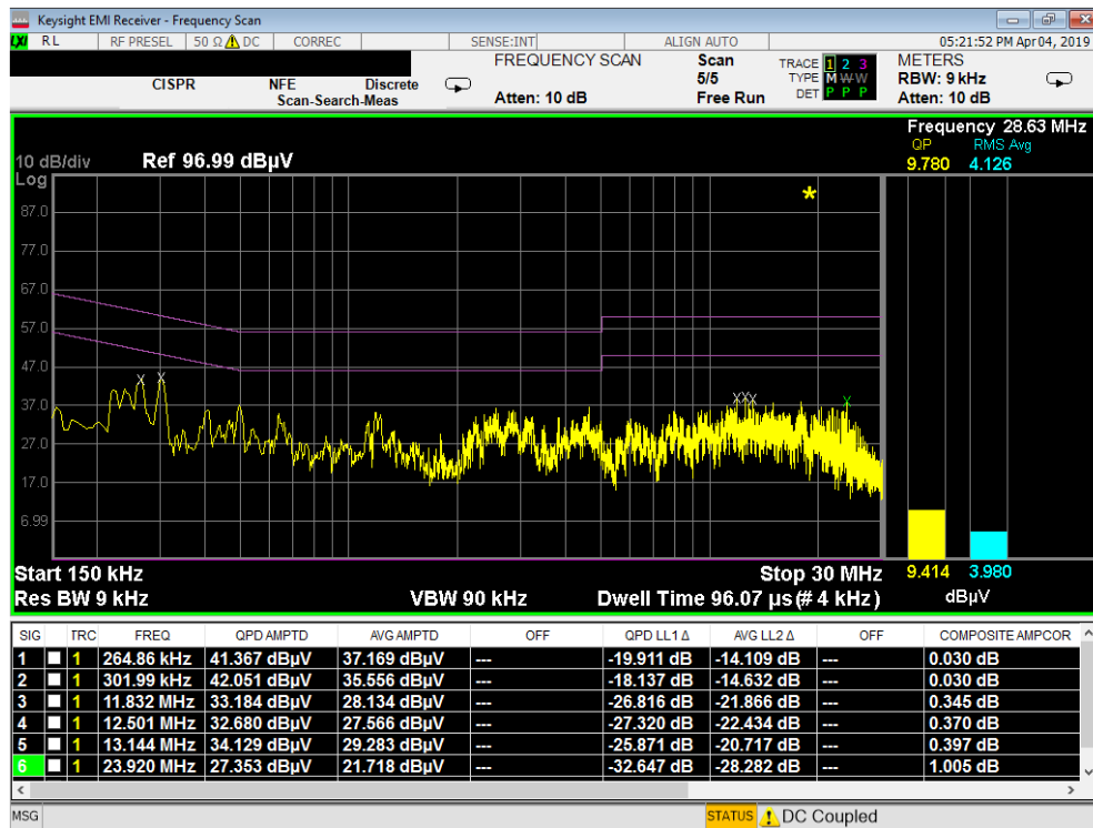
Plot 6-16. Line Conducted Plot (L1)
