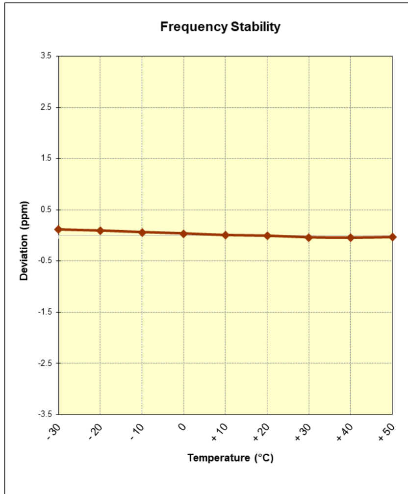
Figure 6-2. Frequency Stability Graph
