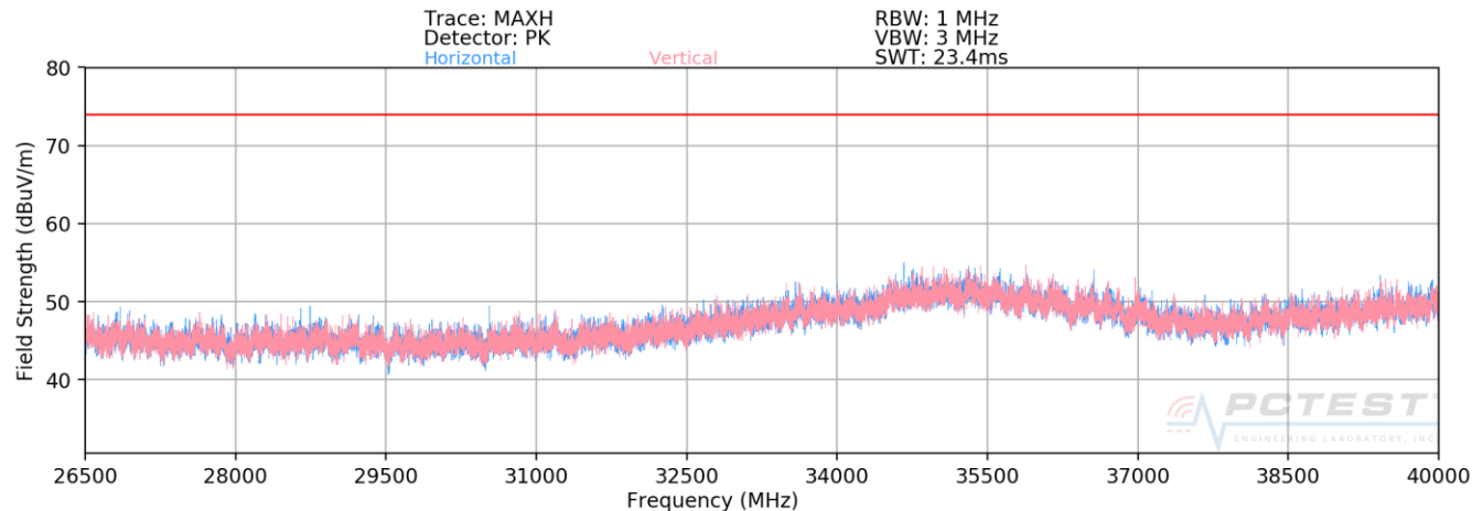
Plot 6-8. Radiated Spurious Plot 26.5-40 GHz
