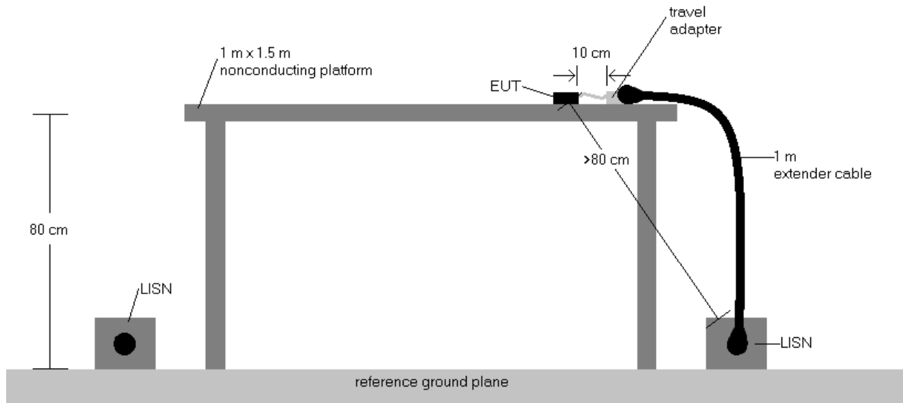
Figure 6-1. Test Instrument & Measurement Setup
