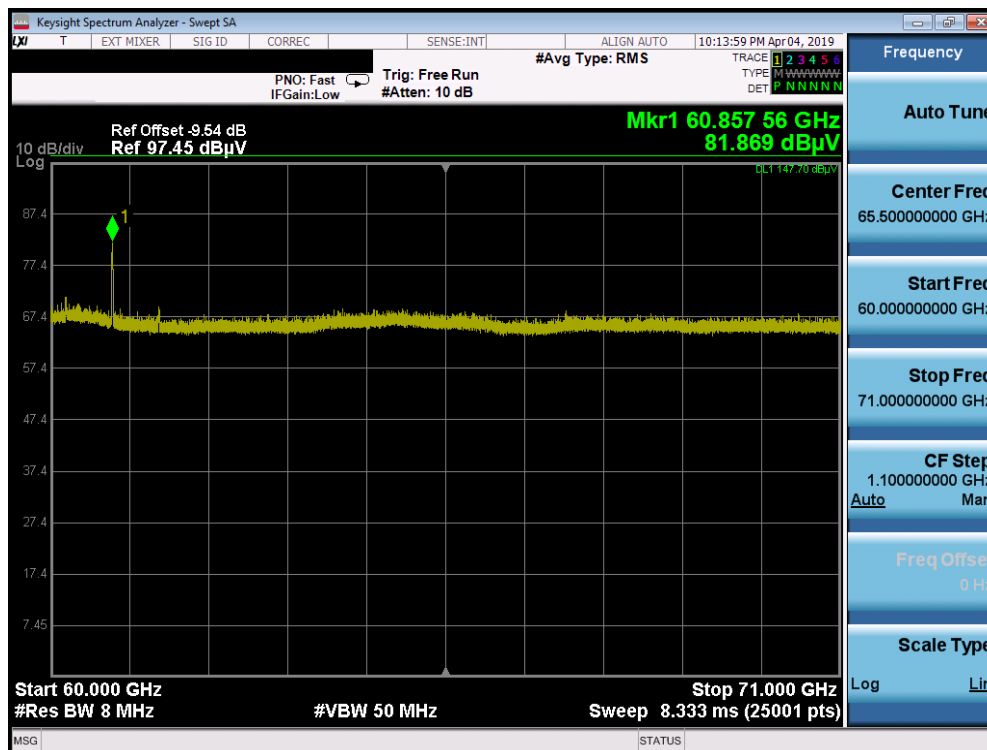
Plot 6-11. Spectrum Emission Mask 60-71 GHz
