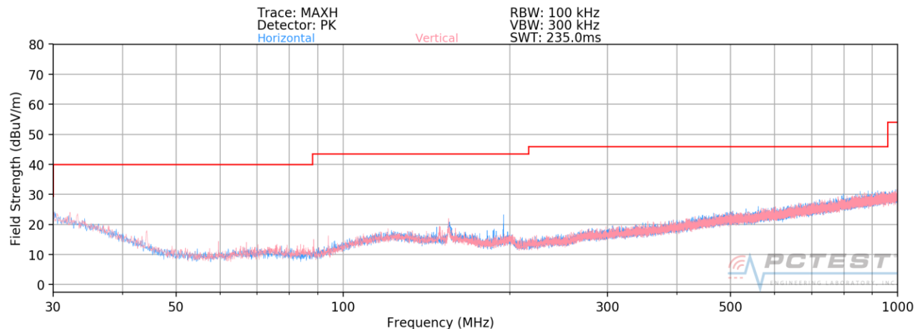
Plot 6-5. Radiated Spurious Plot 30 MHz - 1 GHz
