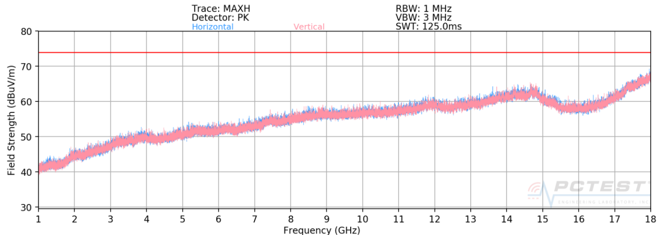
Plot 6-6. Radiated Spurious Plot 1-18 GHz
