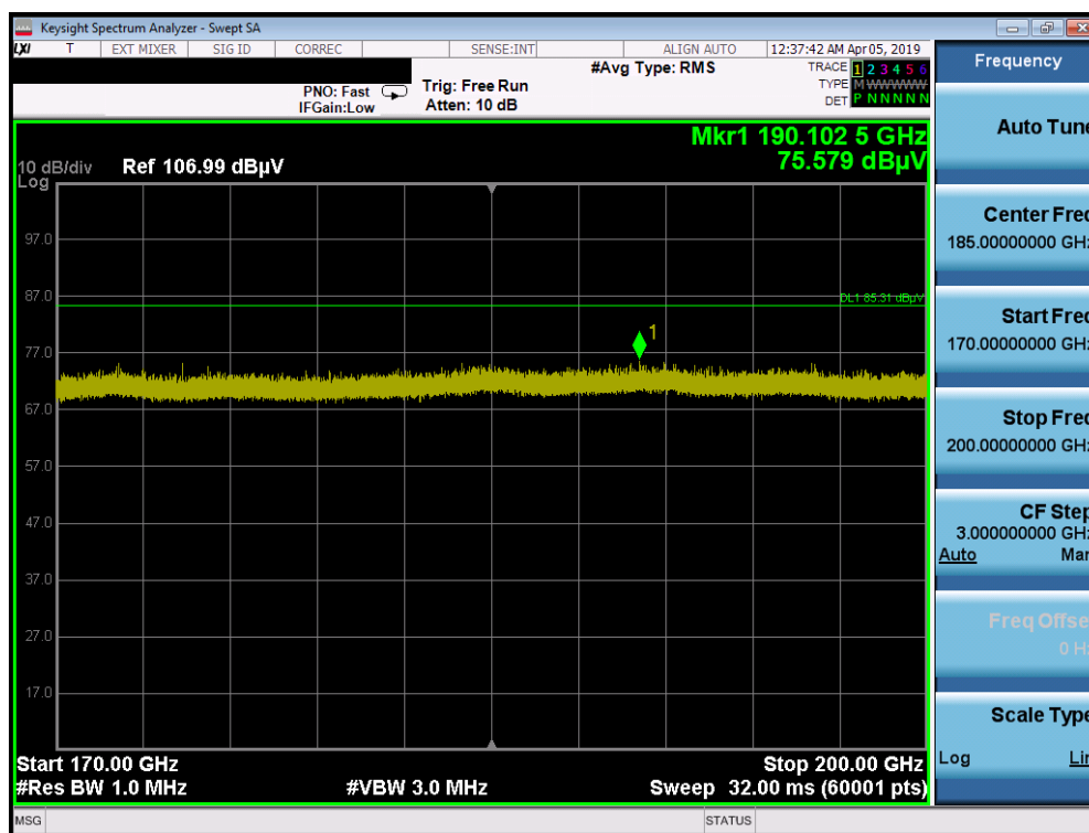
Plot 6-15. Radiated Spurious Plot 170-200 GHz
