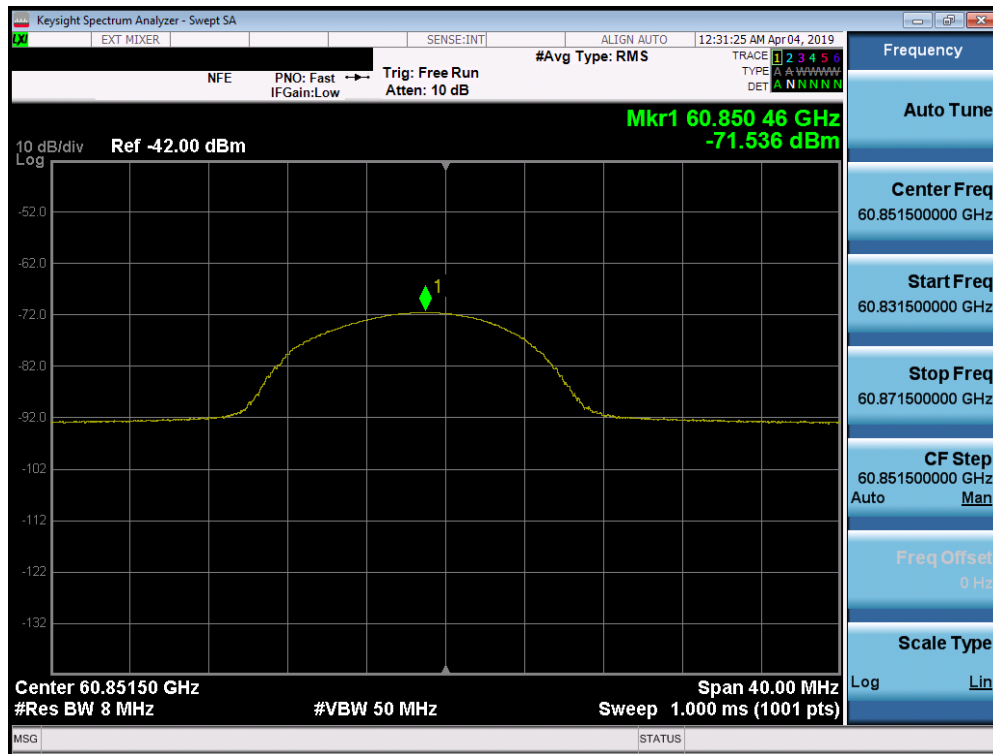
Plot 6-4. Swept mode EIRP Average
