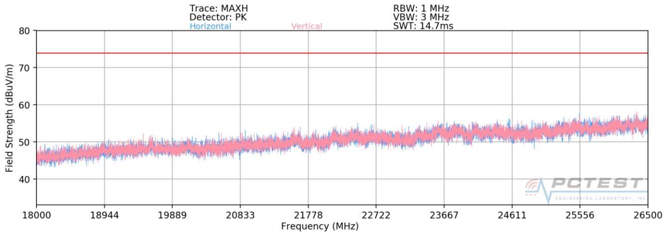
Plot 6-7. Radiated Spurious Plot 18-26.5 GHz
