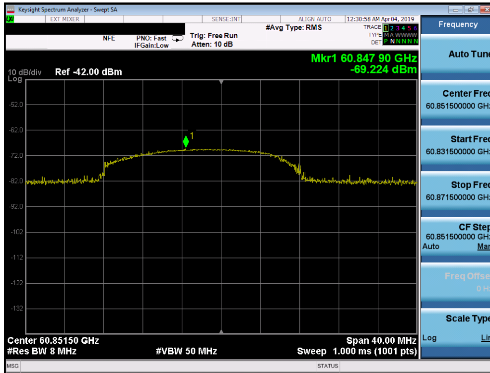
Plot 6-3. Swept mode EIRP Peak
