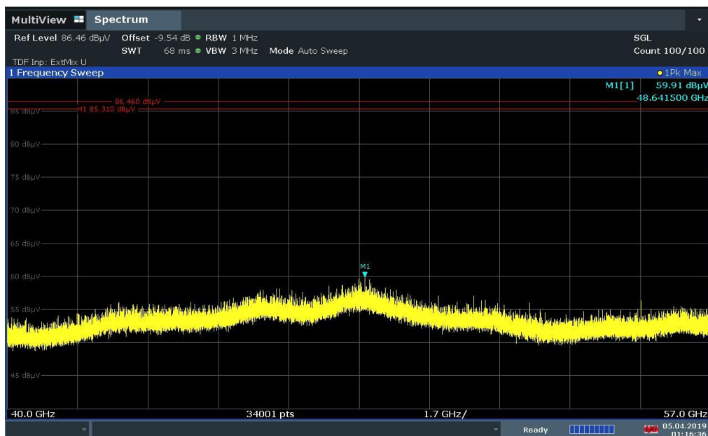
Plot 6-9. Radiated Spurious Plot 40-57 GHz
