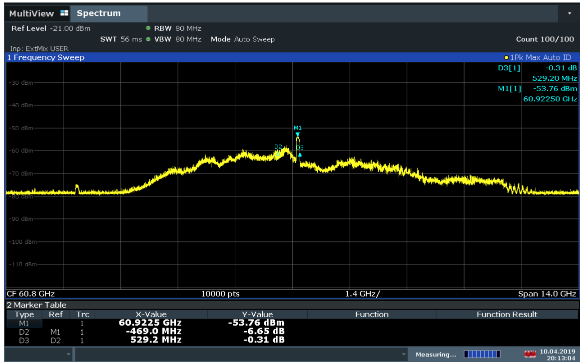
Plot 6-2. 6 dB Bandwidth Plot
