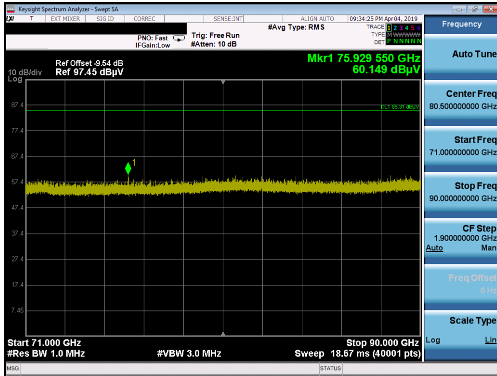
Plot 6-12. Radiated Spurious Plot 71-90 GHz
