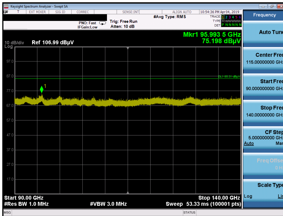
Plot 6-13. Radiated Spurious Plot 90-140 GHz
