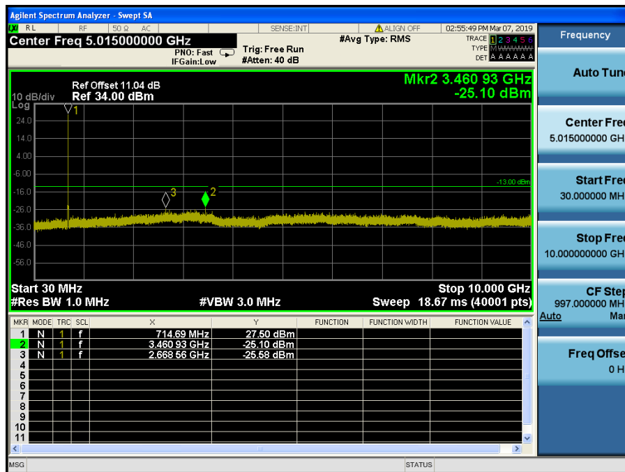
LTE Band 12,17 / 5MHz / 64QAM - RB Size/Offset (12/13) – High Channel
