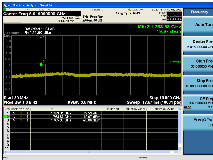
LTE Band 4 / 3MHz / QPSK - RB Size/Offset (8/4) – High Channel
