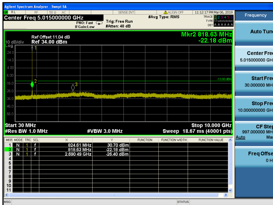
LTE Band 5 / 1.4MHz / 64QAM - RB Size/Offset (6/0) – Low Channel
