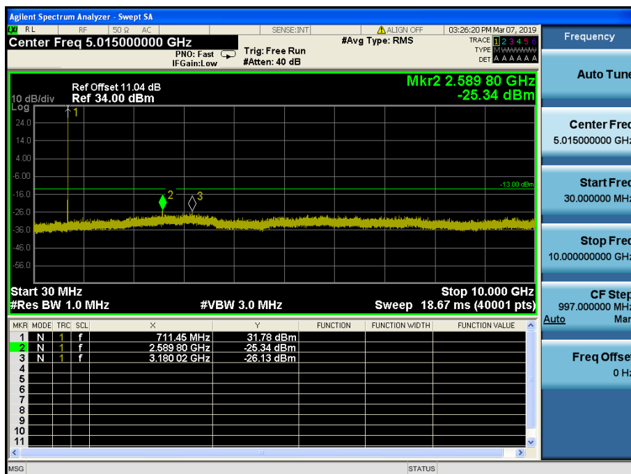
LTE Band 12,17 / 10MHz / 64QAM - RB Size/Offset (1/25) – High Channel
