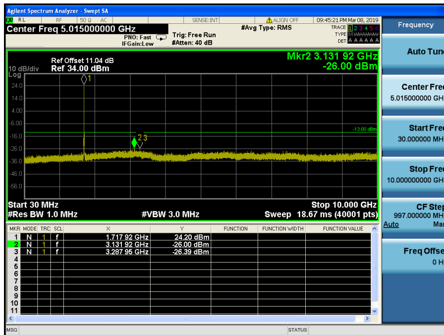
LTE Band 4 / 10MHz / 64QAM - RB Size/Offset (25/25) – Low Channel
