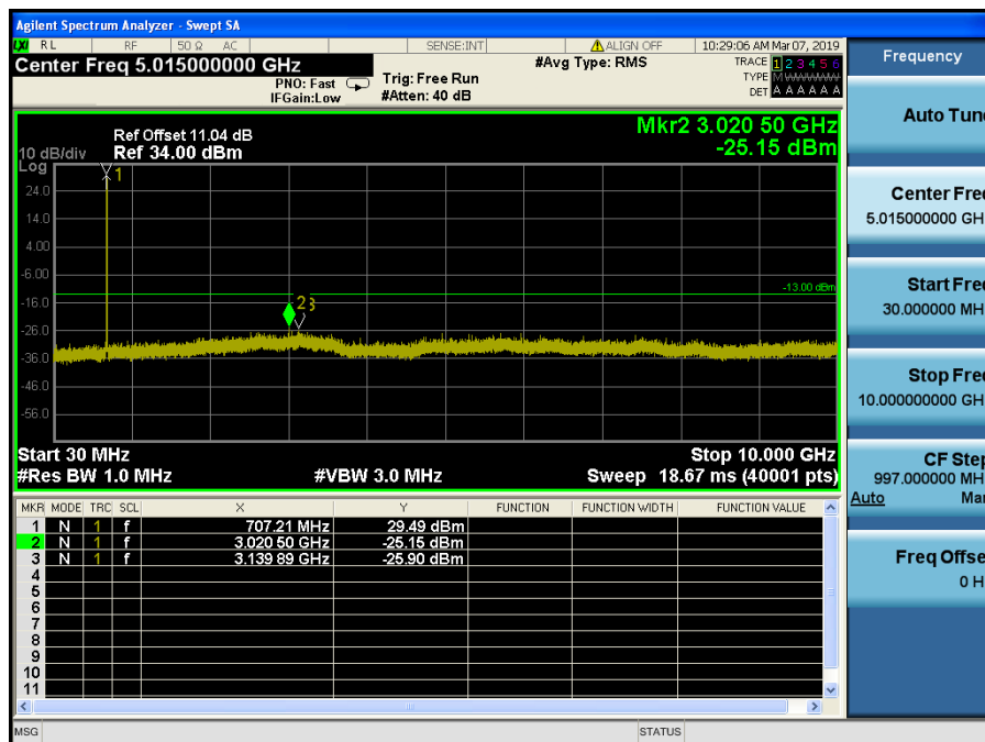
LTE Band 12,17 / 5MHz / 16QAM - RB Size/Offset (12/6) – Mid Channel
