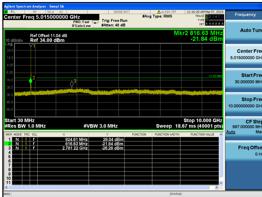
LTE Band 5 / 3MHz / 64QAM - RB Size/Offset (15/0) – Low Channel
