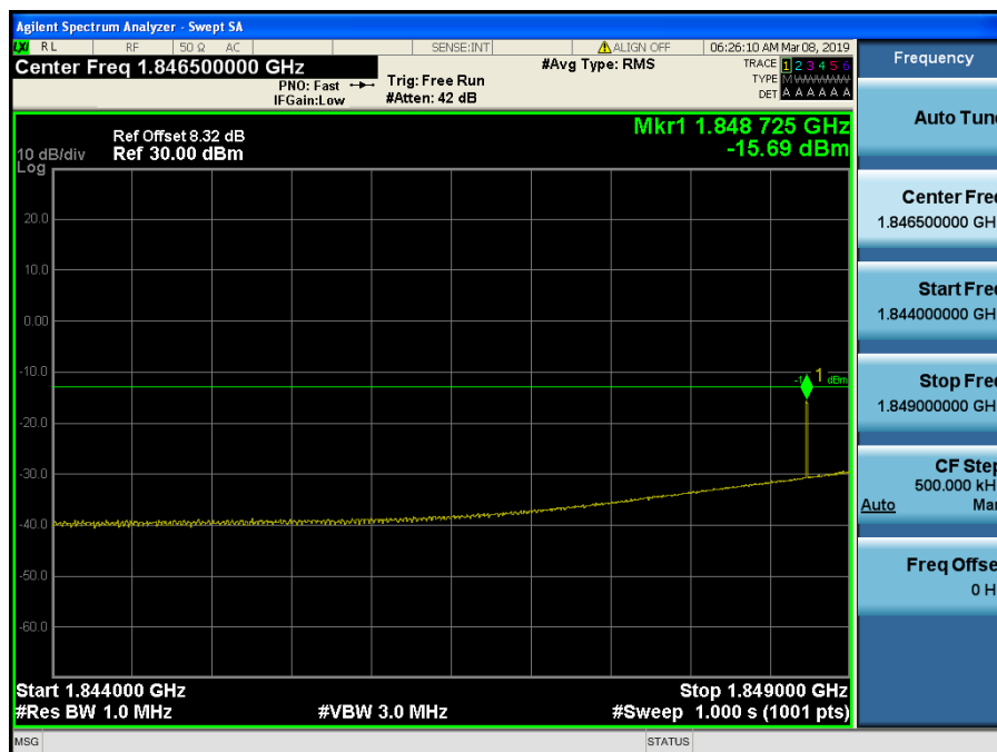
LTE Band 2 / 3MHz / 64QAM - RB Size/Offset (8/7)
