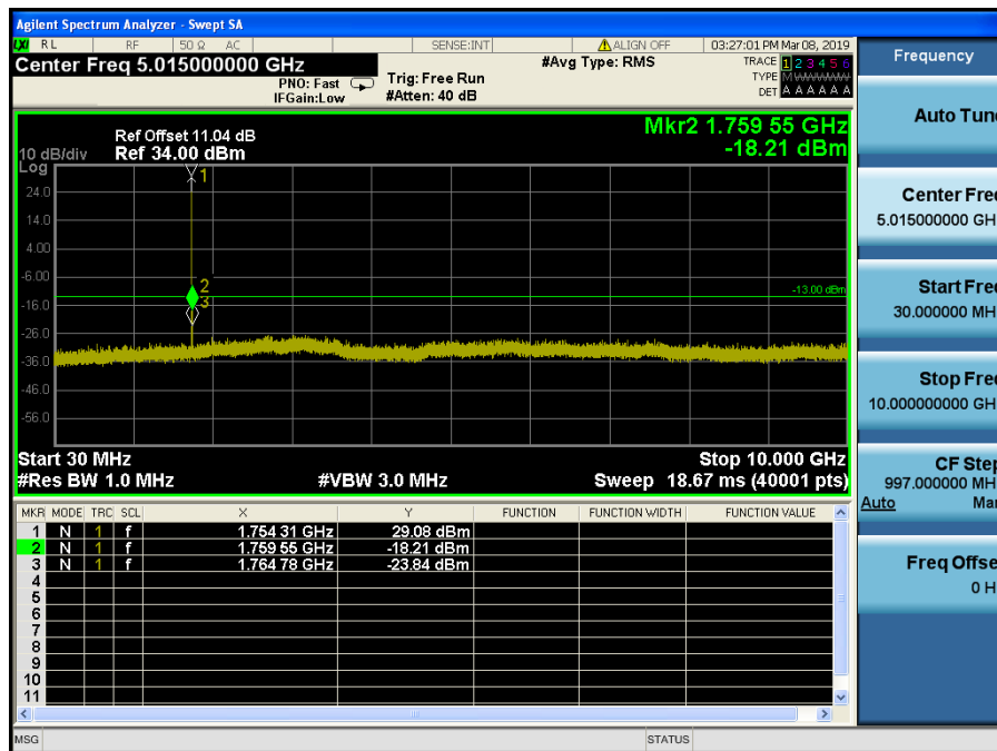
LTE Band 4 / 1.4MHz / 16QAM - RB Size/Offset (3/0) – High Channel
