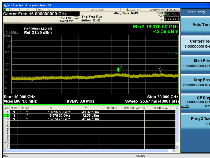
LTE Band 2 / 15MHz / 64QAM - RB Size/Offset (1/74) – Mid Channel
