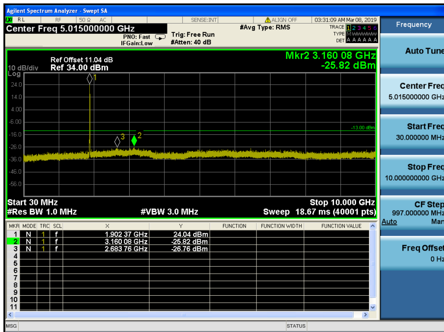
LTE Band 2 / 10MHz / 16QAM - RB Size/Offset (25/0) – High Channel
