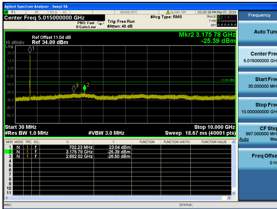
LTE Band 12,17 / 10MHz / 64QAM - RB Size/Offset (50/0) – Low Channel
