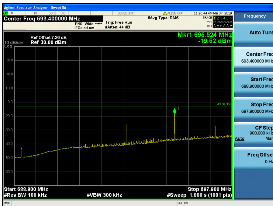
LTE Band 12,17 / 10MHz / 16QAM - RB Size/Offset (50/0)
