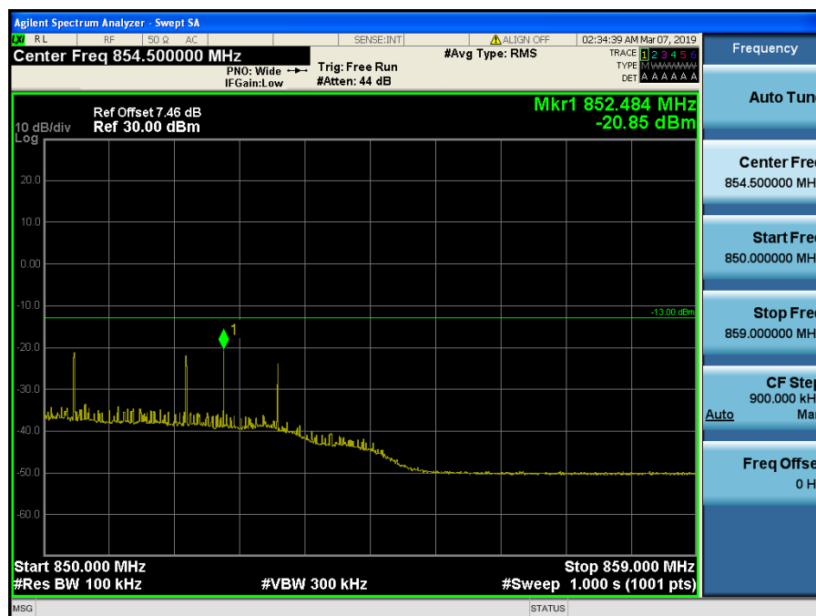
LTE Band 5 / 10MHz / 64QAM - RB Size/Offset (50/0)
