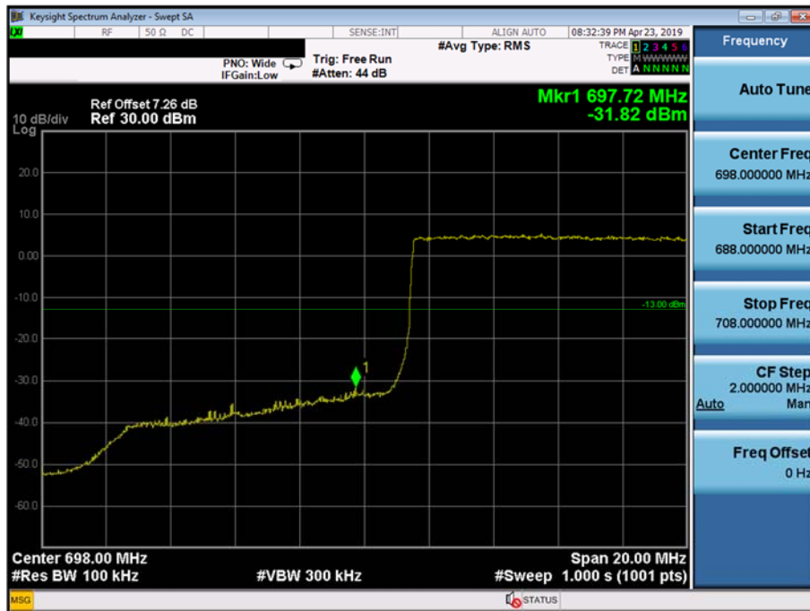
LTE Band 12,17 / 10MHz / 64QAM - RB Size/Offset (50/0)
