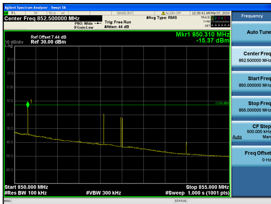
LTE Band 5 / 3MHz / 64QAM - RB Size/Offset (8/7)
