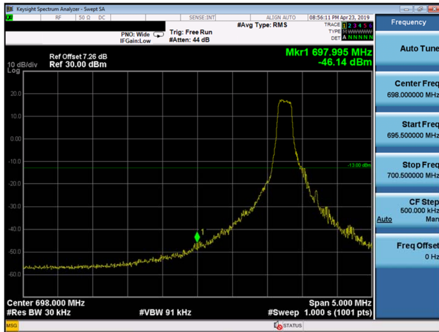
LTE Band 12 / 1.4MHz / 64QAM - RB Size/Offset (1/0)
