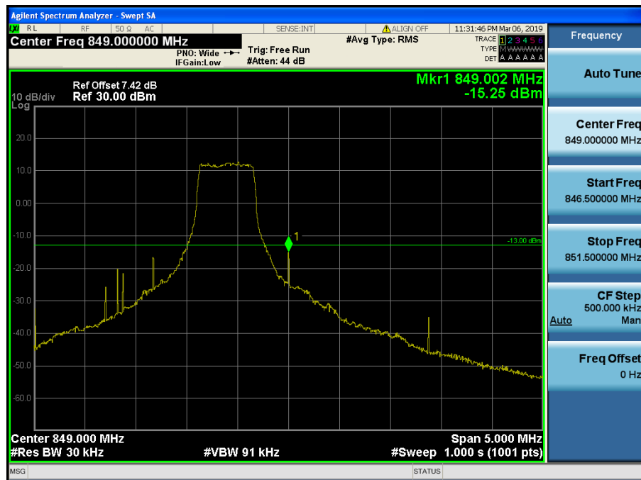
LTE Band 5 / 1.4MHz / 64QAM - RB Size/Offset (3/2)
