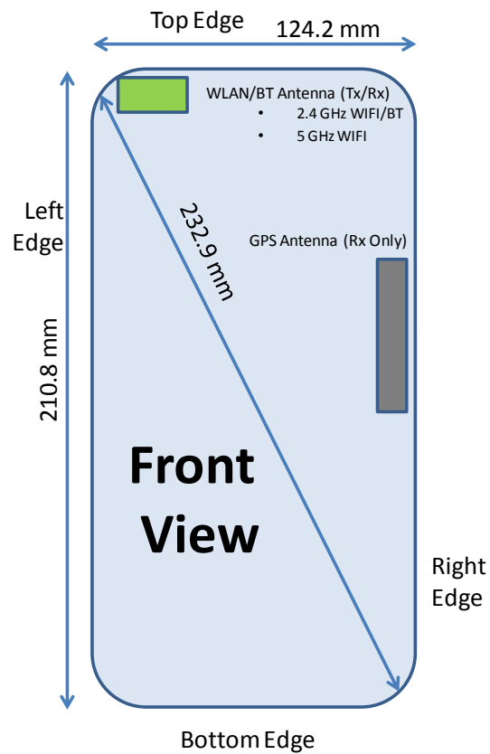
Figure F-1 DUT Antenna Locations
